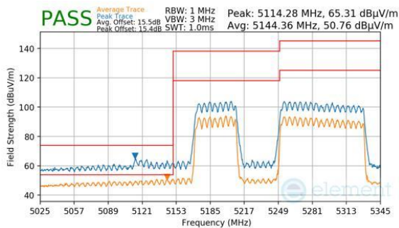
Plot 7-951. CDD Primary (Peak & Average, RU996+484, Index 95, Ch.50, MCS11)
