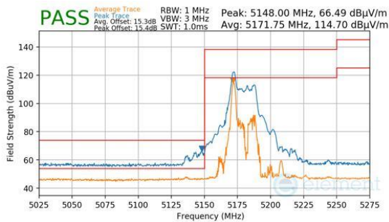
Plot 7-1034. CDD Diversity (Peak & Average, RU26, Index 0, Ch.38, MCS11)
