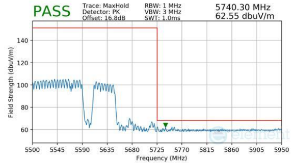
Plot 7-984. CDD Primary (Peak, RU996+484+242, Index 97 (H), Ch.114 (FCC ONLY), MCS11)
