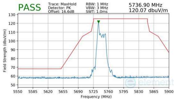
Plot 7-996. CDD Diversity (Peak, RU26, Index 0, Ch.149, MCS11)
