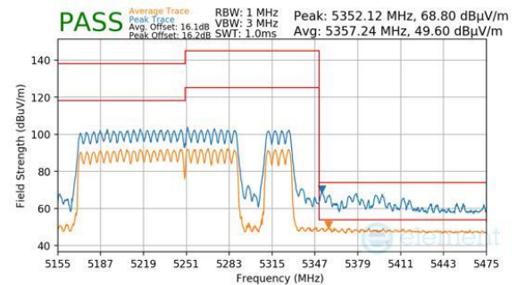
Plot 7-972. CDD Primary (Peak & Average, RU996+484+242, Index 98, Ch.50, MCS11)
