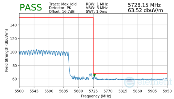
Plot 7-993. CDD Primary (Peak, RU996X2, Index 68, Ch.114 FCC ONLY, MCS11)
