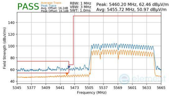
Plot 7-974. CDD Primary (Peak & Average, RU996+484+242, Index 96 (L), Ch.114 (FCC ONLY), MCS11)
