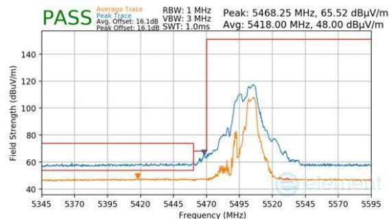
Plot 7-1011. CDD Diversity (Peak & Average, RU52+26, Index 72, Ch.100, MCS11)
