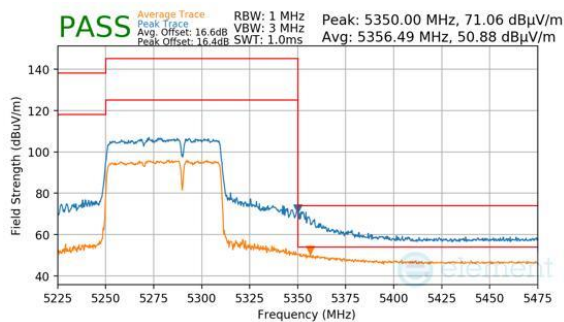
Plot 7-1078. CDD Diversity (Peak & Average, RU484+242, Index 93, Ch.58, MCS11)
