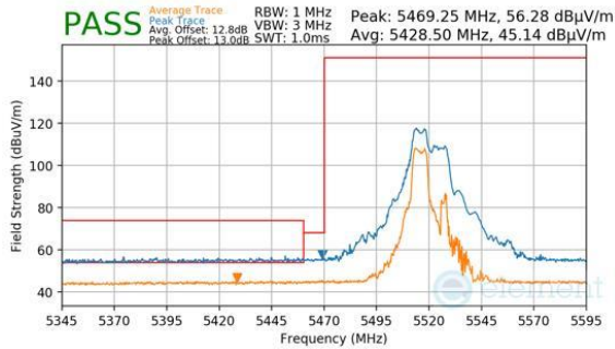
Plot 7-1012. CDD Diversity (Peak & Average, RU52+26, Index 70, Ch.104, MCS11)
