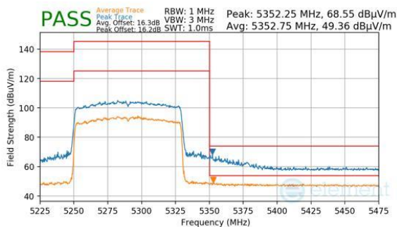
Plot 7-1100. CDD Diversity (Peak & Average, RU996, Index 67, Ch.58, MCS11)
