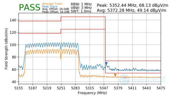
Plot 7-953. CDD Primary (Peak & Average, RU996+484, Index 95, Ch.50, MCS11)
