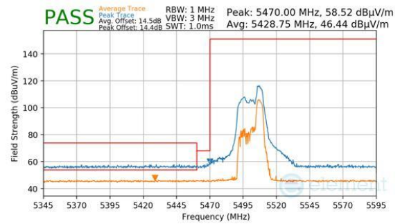
Plot 7-1003. CDD Diversity (Peak & Average, RU52, Index 40, Ch.100, MCS11)
