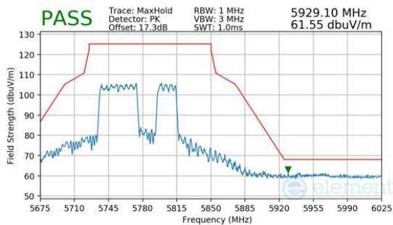
Plot 7-933. CDD Primary (Peak, RU484+242, Index 92, Ch.155, MCS11)
