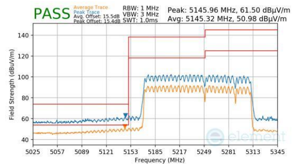
Plot 7-967. CDD Primary (Peak & Average, RU996+484+242, Index 99, Ch.50, MCS11)
