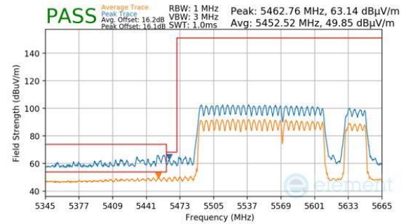
Plot 7-978. CDD Primary (Peak & Average, RU996+484+242, Index 98 (H), Ch.114 (FCC ONLY), MCS11)
