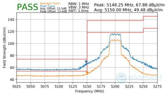
Plot 7-1023. CDD Diversity (Peak & Average, RU242, Index 61, Ch.40, MCS11)
