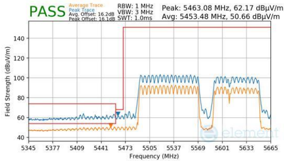
Plot 7-975. CDD Primary (Peak & Average, RU996+484+242, Index 96 (H), Ch.114 (FCC ONLY), MCS11)
