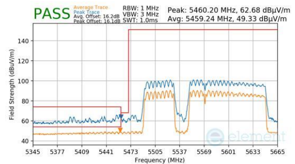
Plot 7-979. CDD Primary (Peak & Average, RU996+484+242, Index 98 (L), Ch.114 (FCC ONLY), MCS11)
