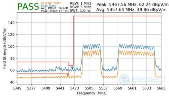
Plot 7-956. CDD Primary (Peak & Average, RU996+484, Index 95 (L), Ch.114 (FCC ONLY), MCS11)
