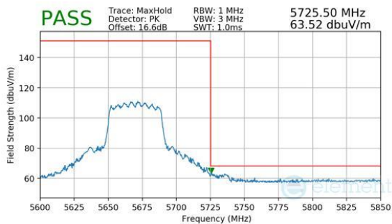
Plot 7-1056. CDD Diversity (Peak, RU484, Index 65, Ch.134, MCS11)
