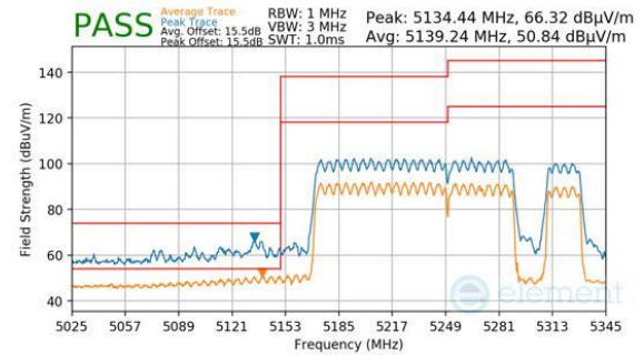
Plot 7-966. CDD Primary (Peak & Average, RU996+484+242, Index 98, Ch.50, MCS11)
