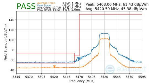
Plot 7-1027. CDD Diversity (Peak & Average, RU242, Index 61, Ch.104, MCS11)
