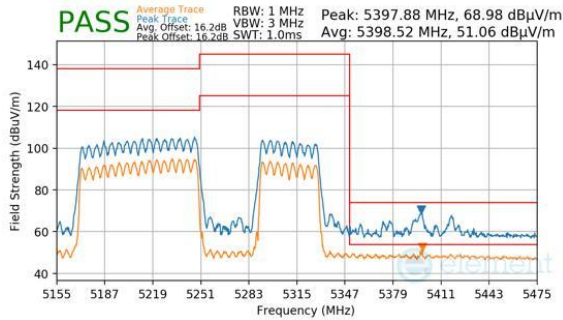
Plot 7-968. CDD Primary (Peak & Average, RU996+484+242, Index 94, Ch.50, MCS11)
