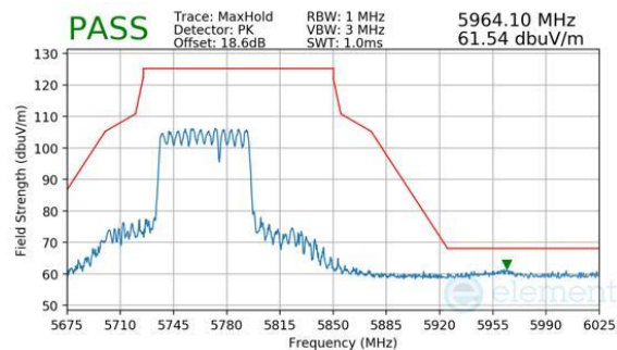
Plot 7-934. CDD Primary (Peak, RU484+242, Index 93, Ch.155, MCS11)
