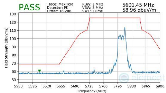
Plot 7-1062. CDD Diversity (Peak, RU26, Index 36, Ch.155, MCS11)
