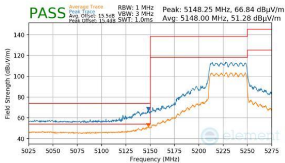
Plot 7-1049. CDD Diversity (Peak & Average, RU484, Index 65, Ch.46, MCS11)
