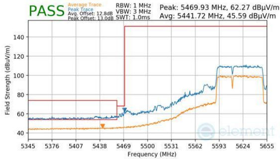
Plot 7-1083. CDD Diversity (Peak & Average, RU484+242, Index 90, Ch.122 (FCC ONLY), MCS11)
