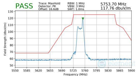
Plot 7-997. CDD Diversity (Peak, RU26, Index 8, Ch.149, MCS11)
