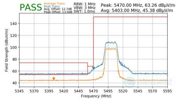
Plot 7-1026. CDD Diversity (Peak & Average, RU242, Index 61, Ch.100, MCS11)
