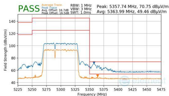
Plot 7-1075. CDD Diversity (Peak & Average, RU484+242, Index 90, Ch.58, MCS11)
