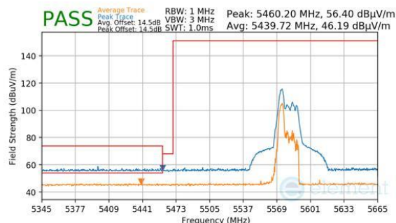
Plot 7-946. CDD Primary (Peak & Average, RU52, Index 37, Ch.114 (FCC ONLY), MCS11)
