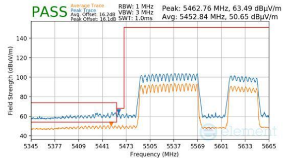
Plot 7-955. CDD Primary (Peak & Average, RU996+484, Index 94 (H), Ch.114 (FCC ONLY), MCS11)
