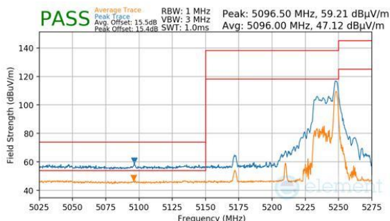
Plot 7-1060. CDD Diversity (Peak & Average, RU26, Index 36, Ch.42, MCS11)
