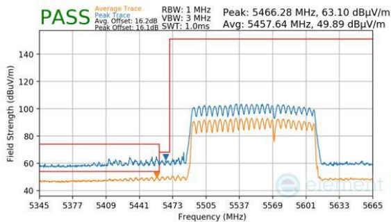
Plot 7-957. CDD Primary (Peak & Average, RU996+484, Index 95 (H), Ch.114 (FCC ONLY), MCS11)
