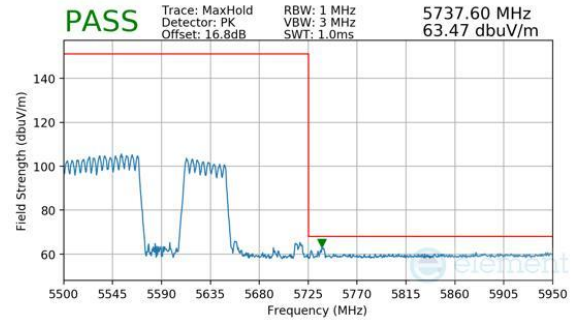
Plot 7-959. CDD Primary (Peak, RU996+484, Index 94 (H), Ch.114 (FCC ONLY), MCS11)
