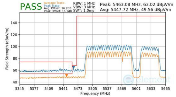
Plot 7-977. CDD Primary (Peak & Average, RU996+484+242, Index 97 (H), Ch.114 (FCC ONLY), MCS11)
