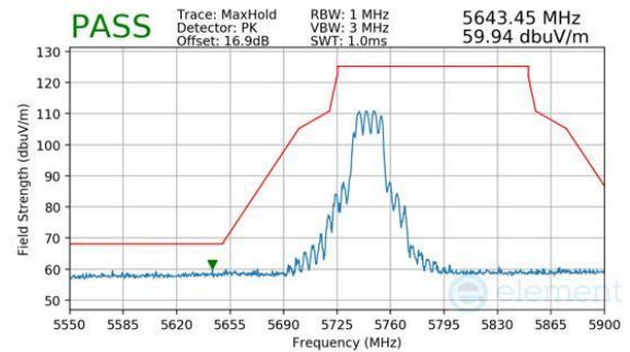
Plot 7-1032. CDD Diversity (Peak, RU242, Index 61, Ch.149, MCS11)
