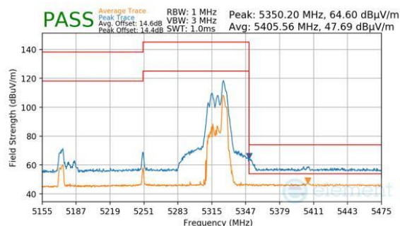
Plot 7-945. CDD Primary (Peak & Average, RU52, Index 52 (H), Ch.50, MCS11)
