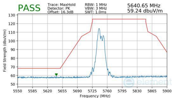
Plot 7-1018. CDD Diversity (Peak, RU52+26, Index 70, Ch.149, MCS11)
