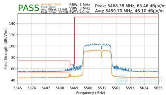
Plot 7-1082. CDD Diversity (Peak & Average, RU484+242, Index 93, Ch.106, MCS11)
