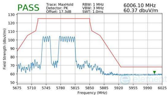
Plot 7-1096. CDD Diversity (Peak, RU484+242, Index 91, Ch.155, MCS11)
