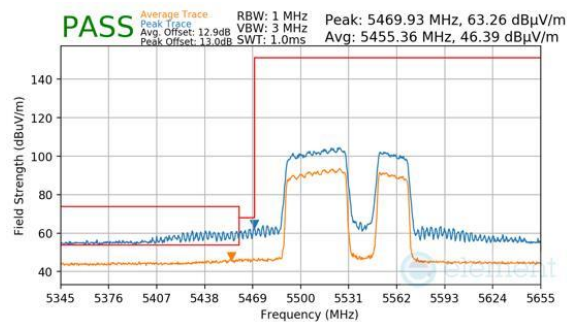
Plot 7-1081. CDD Diversity (Peak & Average, RU484+242, Index 92, Ch.106, MCS11)
