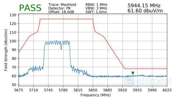
Plot 7-1098. CDD Diversity (Peak, RU484+242, Index 93, Ch.155, MCS11)
