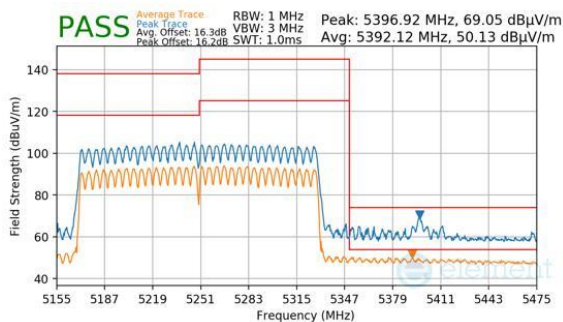
Plot 7-991. CDD Primary (Peak & Average, RU996X2, Index 68, Ch.50, MCS11)
