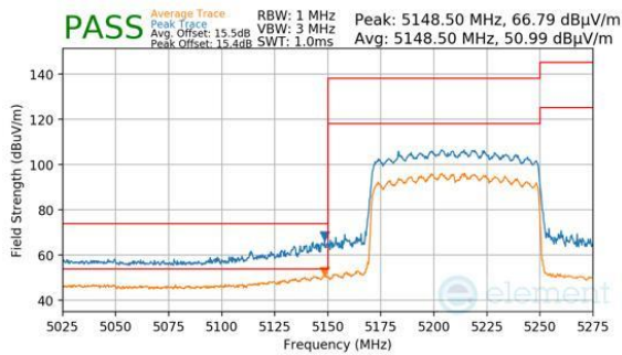
Plot 7-1099. CDD Diversity (Peak & Average, RU996, Index 67, Ch.42, MCS11)
