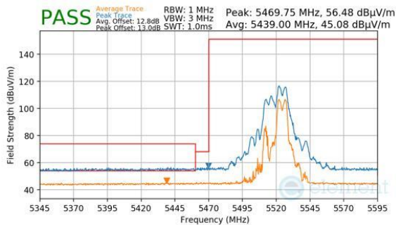
Plot 7-1013. CDD Diversity (Peak & Average, RU52+26, Index 72, Ch.104, MCS11)
