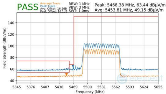
Plot 7-937. CDD Primary (Peak & Average, RU996, Index 67, Ch.106, MCS11)
