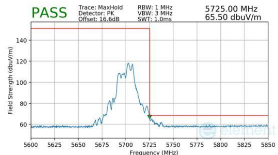
Plot 7-1017. CDD Diversity (Peak, RU52+26, Index 72, Ch.140, MCS11)
