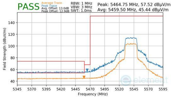
Plot 7-1028. CDD Diversity (Peak & Average, RU242, Index 61, Ch.108, MCS11)
