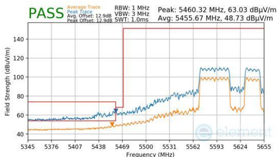
Plot 7-1085. CDD Diversity (Peak & Average, RU484+242, Index 92, Ch.122 (FCC ONLY), MCS11)
