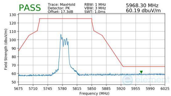
Plot 7-1038. CDD Diversity (Peak, RU26, Index 0, Ch.159, MCS11)
