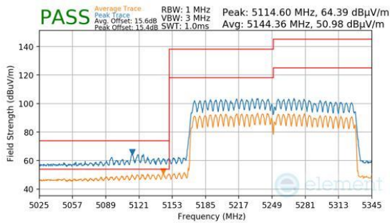
Plot 7-990. CDD Primary (Peak & Average, RU996X2, Index 68, Ch.50, MCS11)
