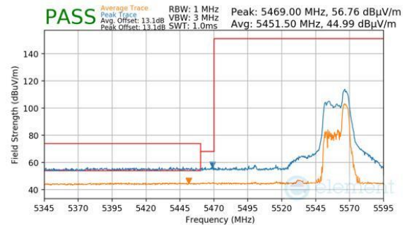
Plot 7-1045. CDD Diversity (Peak & Average, RU52, Index 44, Ch.110, MCS11)
