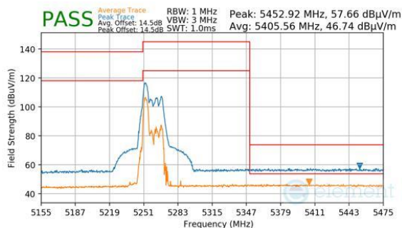
Plot 7-944. CDD Primary (Peak & Average, RU52, Index 37, Ch.50, MCS11)
