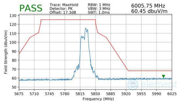
Plot 7-1021. CDD Diversity (Peak, RU52+26, Index 72, Ch.165, MCS11)
