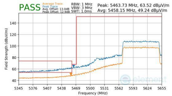
Plot 7-1102. CDD Diversity (Peak & Average, RU996, Index 67, Ch.122 (FCC ONLY), MCS11)
