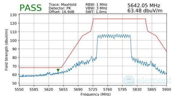
Plot 7-1104. CDD Diversity (Peak, RU996, Index 67, Ch.155, MCS11)
