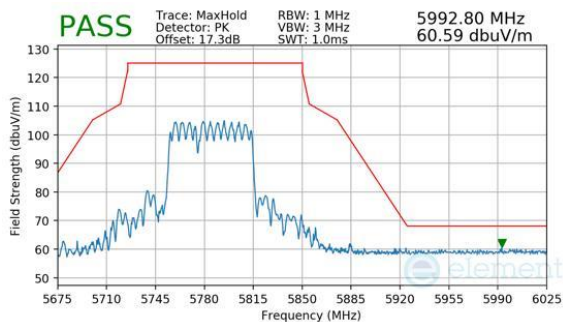
Plot 7-1095. CDD Diversity (Peak, RU484+242, Index 90, Ch.155, MCS11)
