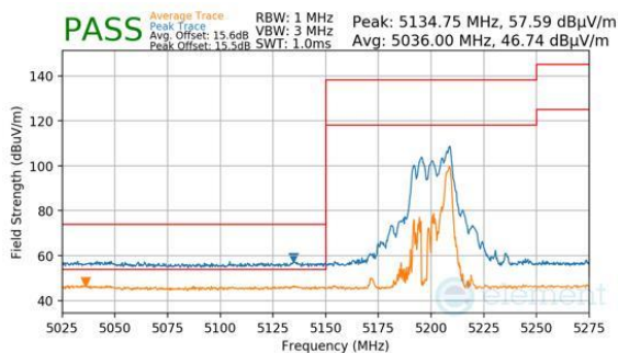
Plot 7-1035. CDD Diversity (Peak & Average, RU26, Index 17, Ch.38, MCS11)
