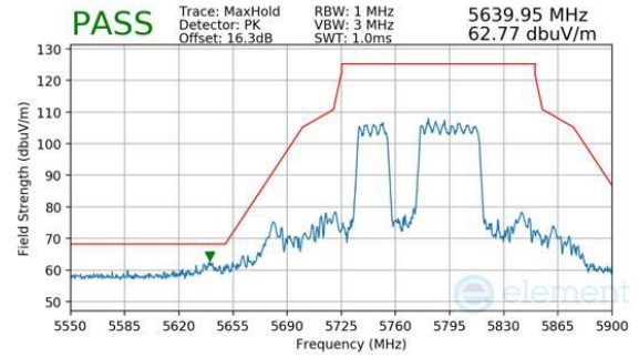
Plot 7-1092. CDD Diversity (Peak, RU484+242, Index 91, Ch.155, MCS11)
