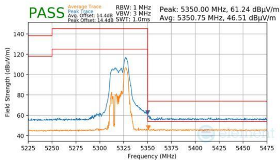
Plot 7-1001. CDD Diversity (Peak & Average, RU52, Index 40, Ch.64, MCS11)
