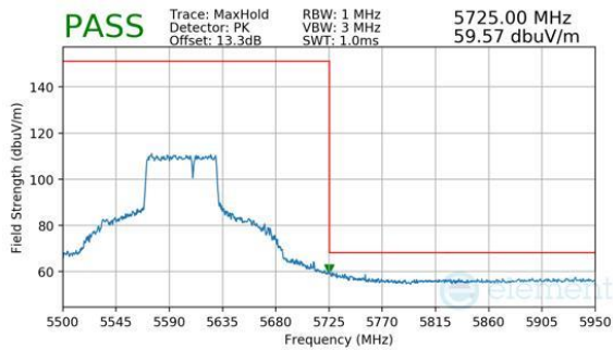
Plot 7-1090. CDD Diversity (Peak, RU484+242, Index 93, Ch.122 (FCC ONLY), MCS11)
