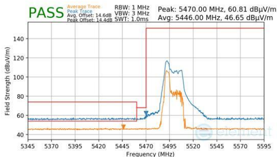
Plot 7-1002. CDD Diversity (Peak & Average, RU52, Index 37, Ch.100, MCS11)
