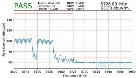
Plot 7-982. CDD Primary (Peak, RU996+484+242, Index 96 (H), Ch.114 (FCC ONLY), MCS11)
