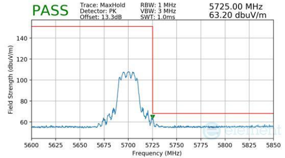
Plot 7-1031. CDD Diversity (Peak, RU242, Index 61, Ch.140, MCS11)
