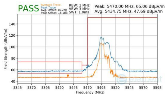
Plot 7-1010. CDD Diversity (Peak & Average, RU52+26, Index 70, Ch.100, MCS11)
