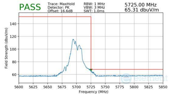
Plot 7-1016. CDD Diversity (Peak, RU52+26, Index 70, Ch.140, MCS11)
