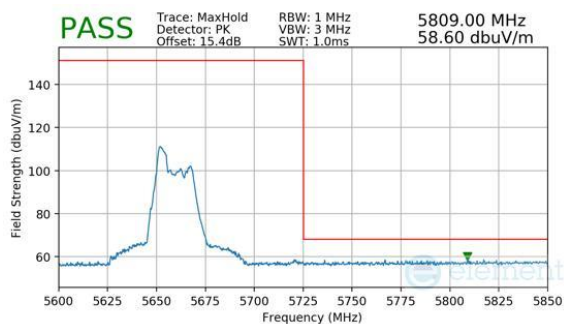
Plot 7-1046. CDD Diversity (Peak, RU52, Index 37, Ch.134, MCS11)
