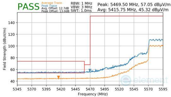
Plot 7-1054. CDD Diversity (Peak & Average, RU484, Index 65, Ch.118 (FCC ONLY), MCS11)
