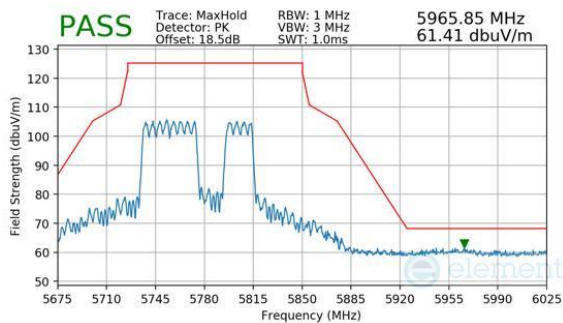
Plot 7-1097. CDD Diversity (Peak, RU484+242, Index 92, Ch.155, MCS11)
