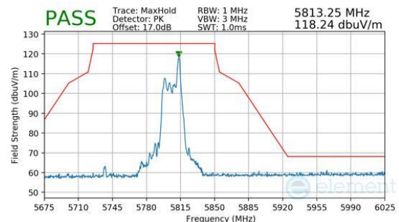
Plot 7-1064. CDD Diversity (Peak, RU26, Index 36, Ch.155, MCS11)
