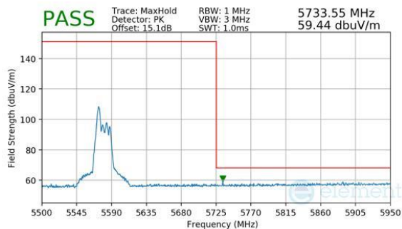
Plot 7-948. CDD Primary (Peak, RU52, Index 37, Ch.114 (FCC ONLY), MCS11)
