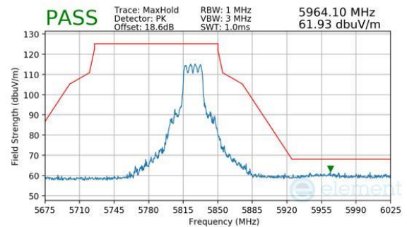
Plot 7-1033. CDD Diversity (Peak, RU242, Index 61, Ch.165, MCS11)
