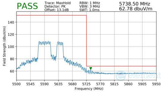
Plot 7-1089. CDD Diversity (Peak, RU484+242, Index 92, Ch.122 (FCC ONLY), MCS11)
