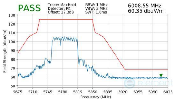
Plot 7-931. CDD Primary (Peak, RU484+242, Index 90, Ch.155, MCS11)
