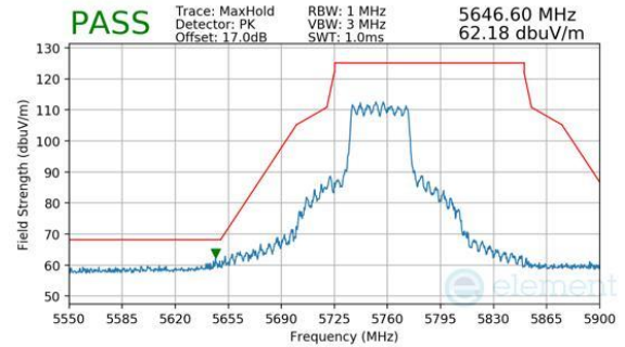
Plot 7-1057. CDD Diversity (Peak, RU484, Index 65, Ch.151, MCS11)
