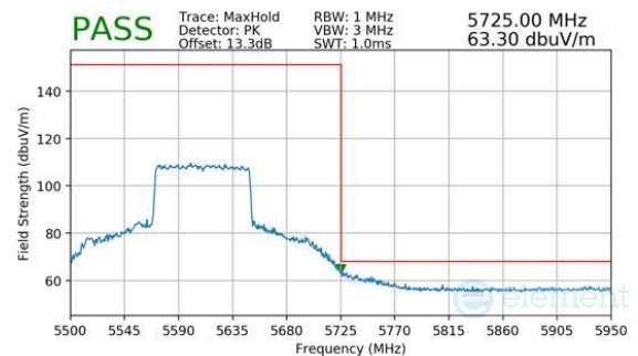
Plot 7-1103. CDD Diversity (Peak, RU996, Index 67, Ch.122 (FCC ONLY), MCS11)
