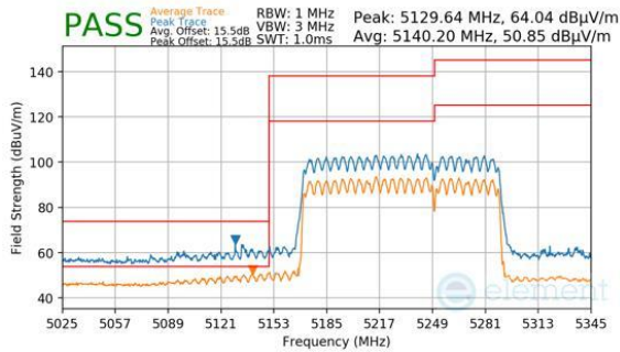
Plot 7-963. CDD Primary (Peak & Average, RU996+484+242, Index 95, Ch.50, MCS11)
