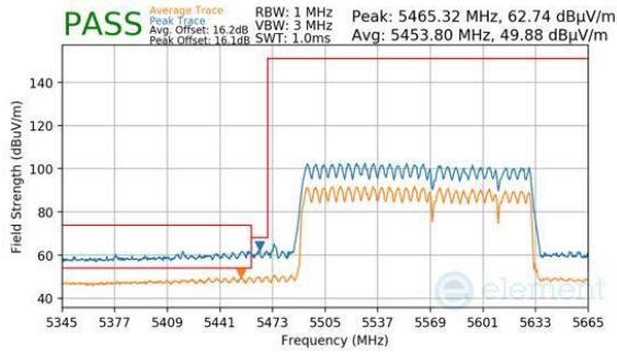
Plot 7-980. CDD Primary (Peak & Average, RU996+484+242, Index 99 (H), Ch.114 (FCC ONLY), MCS11)
