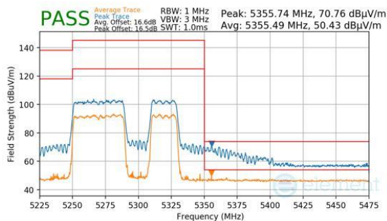
Plot 7-1077. CDD Diversity (Peak & Average, RU484+242, Index 92, Ch.58, MCS11)
