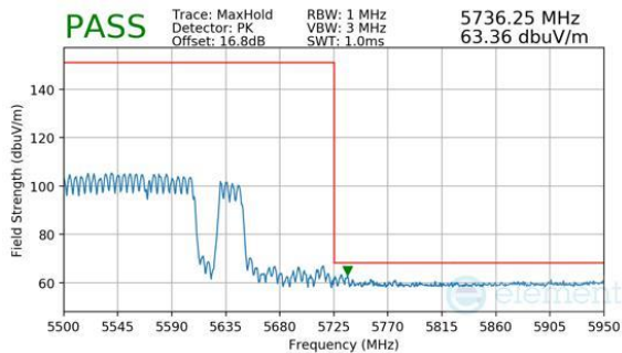
Plot 7-987. CDD Primary (Peak, RU996+484+242, Index 98 (H), Ch.114 (FCC ONLY), MCS11)
