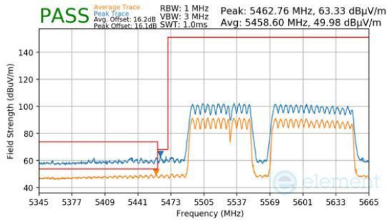
Plot 7-981. CDD Primary (Peak & Average, RU996+484+242, Index 99 (L), Ch.114 (FCC ONLY), MCS11)
