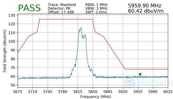
Plot 7-1020. CDD Diversity (Peak, RU52+26, Index 70, Ch.165, MCS11)
