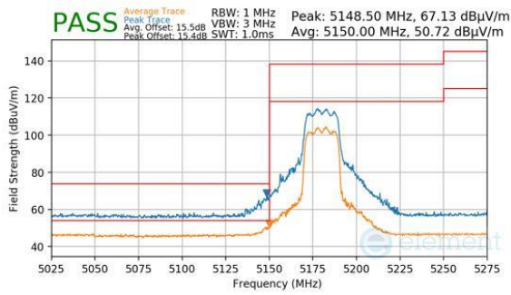
Plot 7-1022. CDD Diversity (Peak & Average, RU242, Index 61, Ch.36, MCS11)
