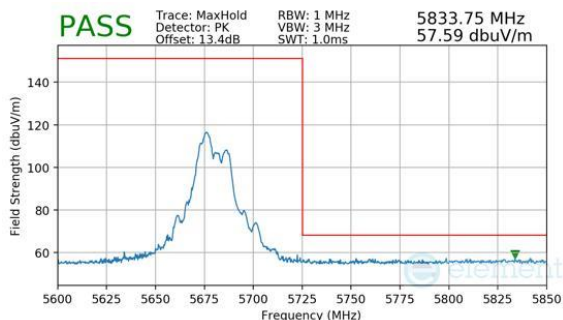
Plot 7-1014. CDD Diversity (Peak, RU52+26, Index 70, Ch.136, MCS11)
