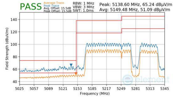
Plot 7-965. CDD Primary (Peak & Average, RU996+484+242, Index 97, Ch.50, MCS11)
