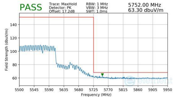
Plot 7-960. CDD Primary (Peak, RU996+484, Index 95 (H), Ch.114 (FCC ONLY), MCS11)
