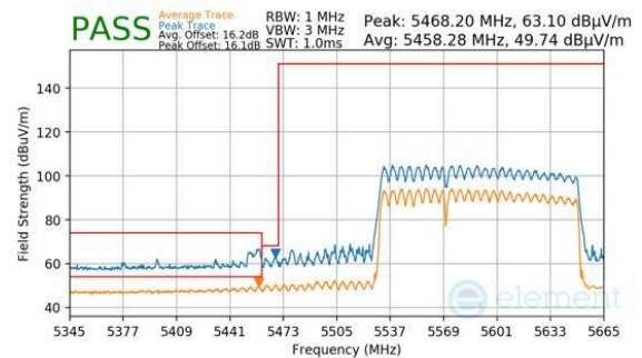
Plot 7-954. CDD Primary (Peak & Average, RU996+484, Index 94 (L), Ch.114 (FCC ONLY), MCS11)
