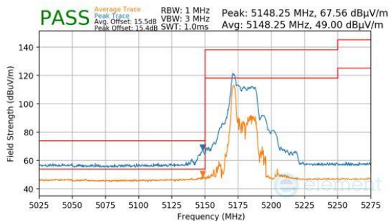
Plot 7-994. CDD Diversity (Peak & Average, RU26, Index 0, Ch.36, MCS11)
