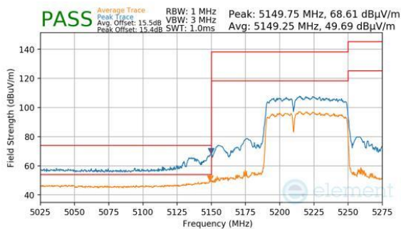
Plot 7-1071. CDD Diversity (Peak & Average, RU484+242, Index 90, Ch.42, MCS11)
