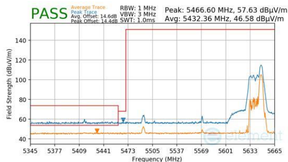
Plot 7-947. CDD Primary (Peak & Average, RU52, Index 52 (H), Ch.114 (FCC ONLY), MCS11)
