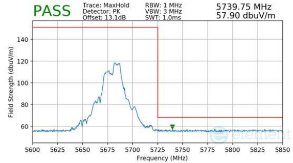
Plot 7-1015. CDD Diversity (Peak, RU52+26, Index 72, Ch.136, MCS11)
