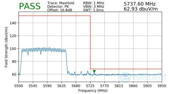
Plot 7-983. CDD Primary (Peak, RU996+484+242, Index 96 (L), Ch.114 (FCC ONLY), MCS11)
