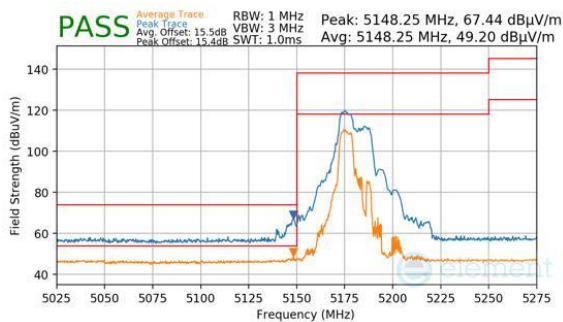
Plot 7-1006. CDD Diversity (Peak & Average, RU52+26, Index 70, Ch.36, MCS11)
