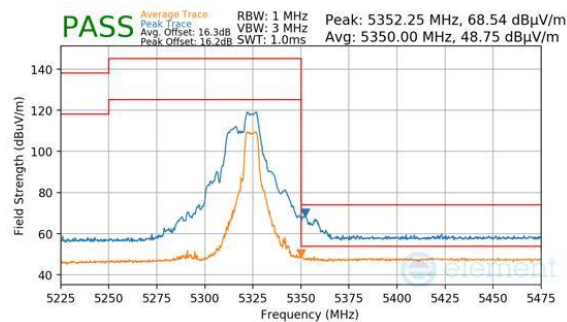
Plot 7-1009. CDD Diversity (Peak & Average, RU52+26, Index 72, Ch.64, MCS11)
