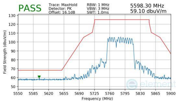
Plot 7-1091. CDD Diversity (Peak, RU484+242, Index 90, Ch.155, MCS11)
