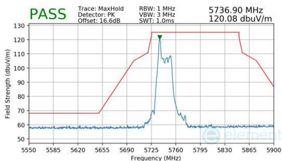
Plot 7-1036. CDD Diversity (Peak, RU26, Index 0, Ch.151, MCS11)
