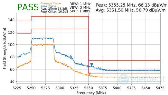
Plot 7-1050. CDD Diversity (Peak & Average, RU484, Index 65, Ch.54, MCS11)
