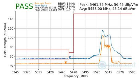
Plot 7-1044. CDD Diversity (Peak & Average, RU52, Index 37, Ch.110, MCS11)
