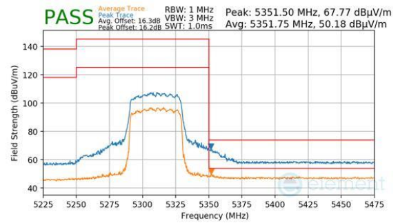
Plot 7-1051. CDD Diversity (Peak & Average, RU484, Index 65, Ch.62, MCS11)
