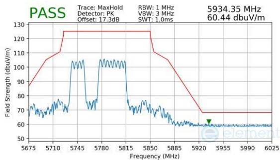
Plot 7-932. CDD Primary (Peak, RU484+242, Index 91, Ch.155, MCS11)
