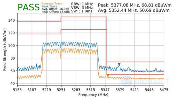
Plot 7-952. CDD Primary (Peak & Average, RU996+484, Index 94, Ch.50, MCS11)
