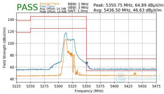
Plot 7-1000. CDD Diversity (Peak & Average, RU52, Index 37, Ch.64, MCS11)
