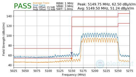
Plot 7-935. CDD Primary (Peak & Average, RU996, Index 67, Ch.42, MCS11)
