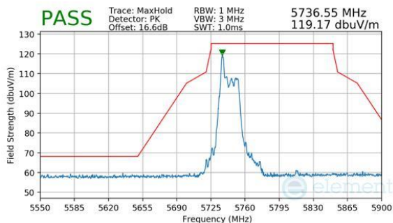
Plot 7-1061. CDD Diversity (Peak, RU26, Index 0, Ch.155, MCS11)
