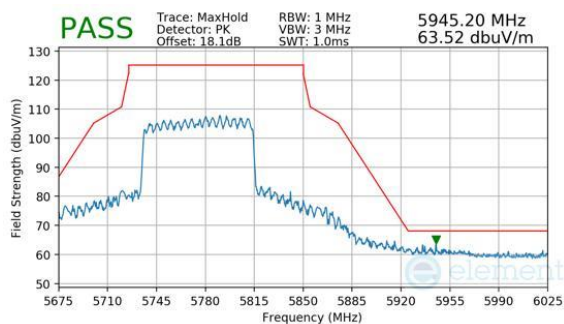
Plot 7-941. CDD Primary (Peak, RU996, Index 67, Ch.155, MCS11)
