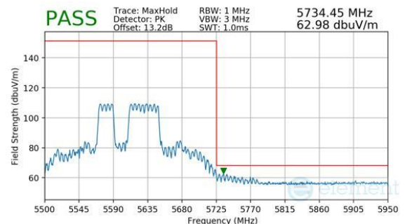
Plot 7-1088. CDD Diversity (Peak, RU484+242, Index 91, Ch.122 (FCC ONLY), MCS11)
