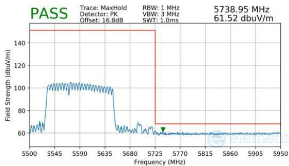
Plot 7-958. CDD Primary (Peak, RU996+484, Index 94 (L), Ch.114 (FCC ONLY), MCS11)
