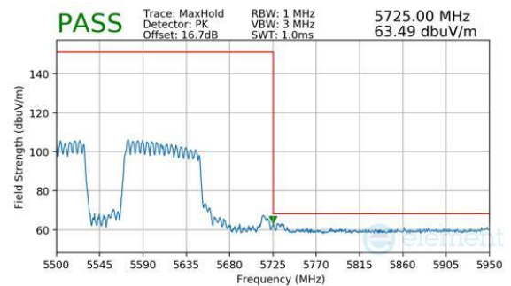
Plot 7-961. CDD Primary (Peak, RU996+484, Index 95 (L), Ch.114 (FCC ONLY), MCS11)
