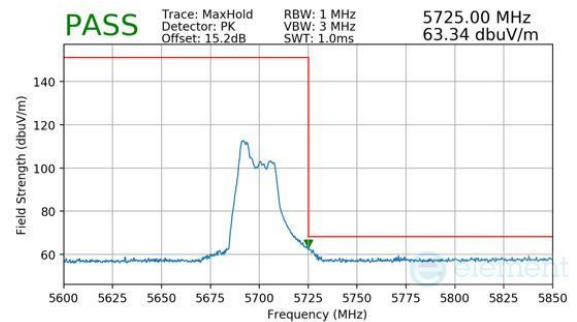
Plot 7-1004. CDD Diversity (Peak, RU52, Index 37, Ch.140, MCS11)
