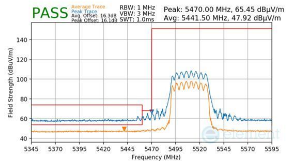
Plot 7-1052. CDD Diversity (Peak & Average, RU484, Index 65, Ch.102, MCS11)
