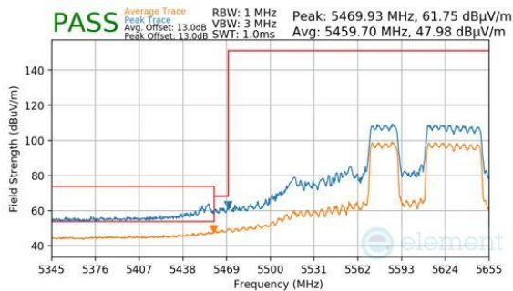
Plot 7-1084. CDD Diversity (Peak & Average, RU484+242, Index 91, Ch.122 (FCC ONLY), MCS11)
