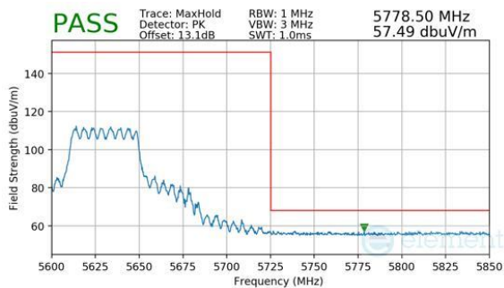
Plot 7-1055. CDD Diversity (Peak, RU484, Index 65, Ch.126 (FCC ONLY), MCS11)
