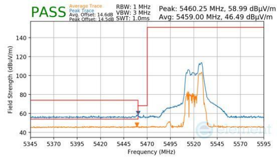
Plot 7-1043. CDD Diversity (Peak & Average, RU52, Index 44, Ch.102, MCS11)
