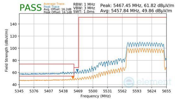
Plot 7-938. CDD Primary (Peak & Average, RU996, Index 67, Ch.122 (FCC ONLY), MCS11)
