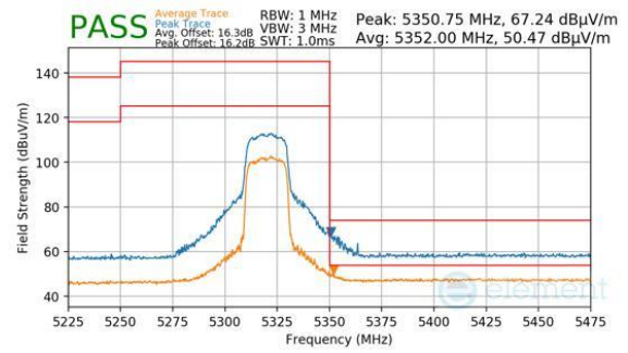
Plot 7-1025. CDD Diversity (Peak & Average, RU242, Index 61, Ch.64, MCS11)
