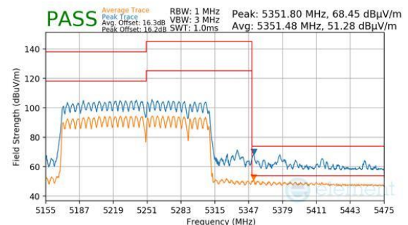
Plot 7-973. CDD Primary (Peak & Average, RU996+484+242, Index 99, Ch.50, MCS11)
