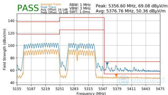
Plot 7-970. CDD Primary (Peak & Average, RU996+484+242, Index 96, Ch.50, MCS11)
