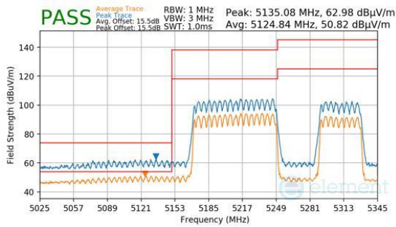
Plot 7-950. CDD Primary (Peak & Average, RU996+484, Index 94, Ch.50, MCS11)
