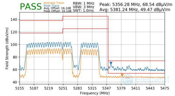
Plot 7-971. CDD Primary (Peak & Average, RU996+484+242, Index 97, Ch.50, MCS11)
