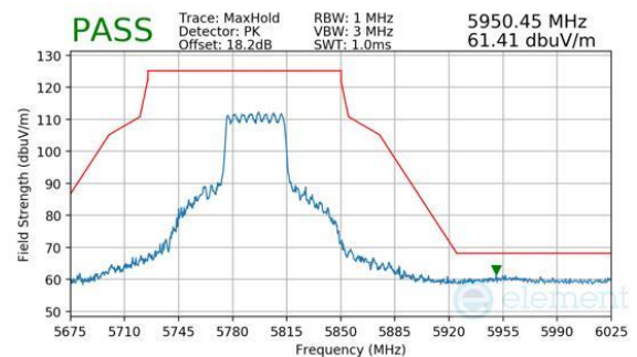
Plot 7-1058. CDD Diversity (Peak, RU484, Index 65, Ch.159, MCS11)
