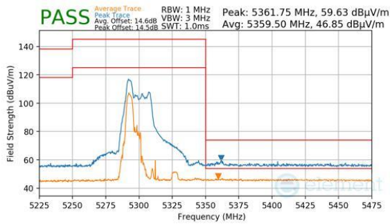
Plot 7-1040. CDD Diversity (Peak & Average, RU52, Index 37, Ch.62, MCS11)
