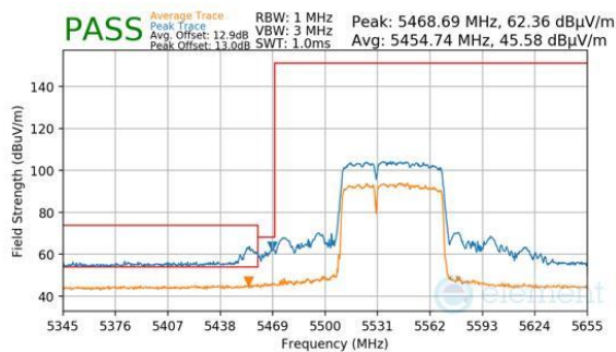
Plot 7-1079. CDD Diversity (Peak & Average, RU484+242, Index 90, Ch.106, MCS11)
