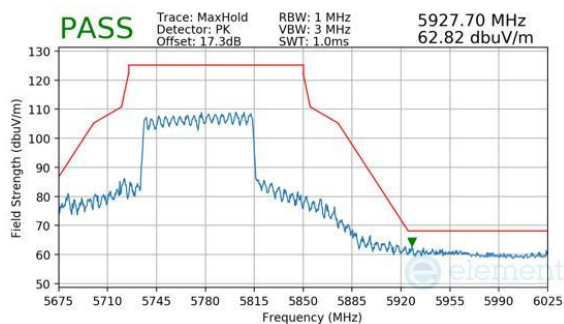
Plot 7-1105. CDD Diversity (Peak, RU996, Index 67, Ch.155, MCS11)
