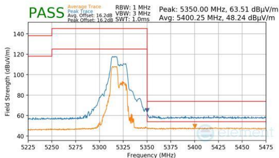
Plot 7-1008. CDD Diversity (Peak & Average, RU52+26, Index 70, Ch.64, MCS11)
