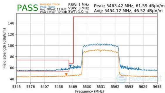
Plot 7-1101. CDD Diversity (Peak & Average, RU996, Index 67, Ch.106, MCS11)
