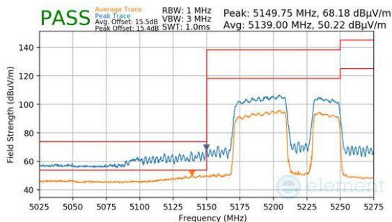
Plot 7-1073. CDD Diversity (Peak & Average, RU484+242, Index 92, Ch.42, MCS11)
