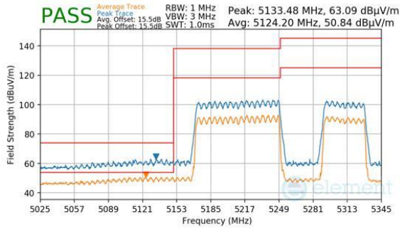
Plot 7-962. CDD Primary (Peak & Average, RU996+484+242, Index 94, Ch.50, MCS11)
