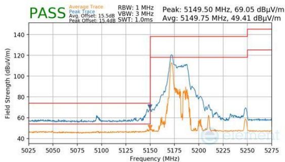
Plot 7-1059. CDD Diversity (Peak & Average, RU26, Index 0, Ch.42, MCS11)
