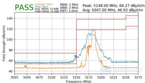
Plot 7-1007. CDD Diversity (Peak & Average, RU52+26, Index 72, Ch.36, MCS11)
