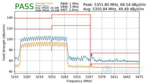
Plot 7-969. CDD Primary (Peak & Average, RU996+484+242, Index 95, Ch.50, MCS11)
