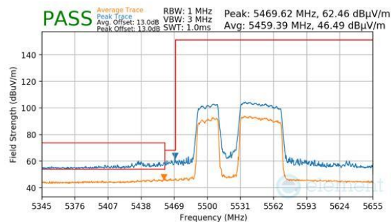
Plot 7-1080. CDD Diversity (Peak & Average, RU484+242, Index 91, Ch.106, MCS11)
