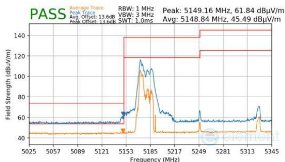
Plot 7-942. CDD Primary (Peak & Average, RU52, Index 37, Ch.50, MCS11)
