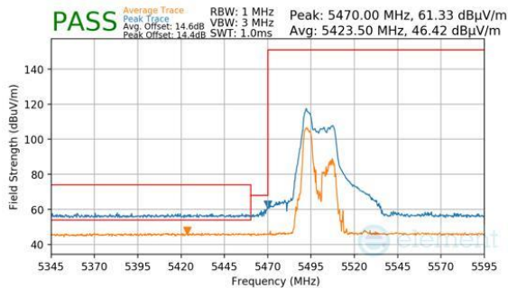
Plot 7-1042. CDD Diversity (Peak & Average, RU52, Index 37, Ch.102, MCS11)
