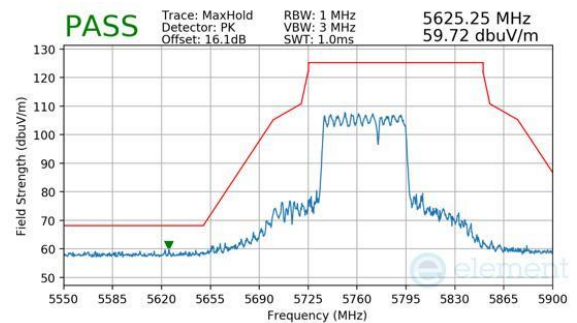
Plot 7-1094. CDD Diversity (Peak, RU484+242, Index 93, Ch.155, MCS11)
