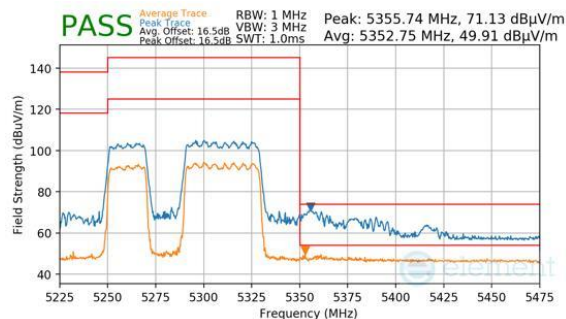
Plot 7-1076. CDD Diversity (Peak & Average, RU484+242, Index 91, Ch.58, MCS11)
