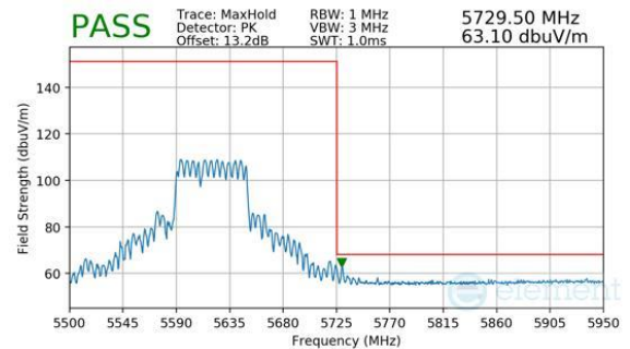
Plot 7-1087. CDD Diversity (Peak, RU484+242, Index 90, Ch.122 (FCC ONLY), MCS11)
