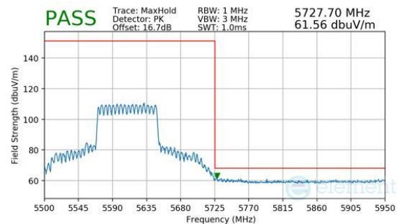
Plot 7-939. CDD Primary (Peak, RU996, Index 67, Ch.122 (FCC ONLY), MCS11)
