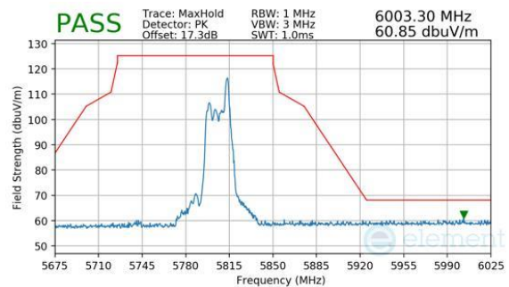
Plot 7-1039. CDD Diversity (Peak, RU26, Index 17, Ch.159, MCS11)
