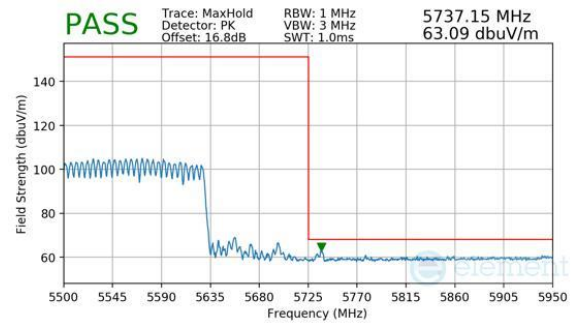
Plot 7-989. CDD Primary (Peak, RU996+484+242, Index 99 (H), Ch.114 (FCC ONLY), MCS11)
