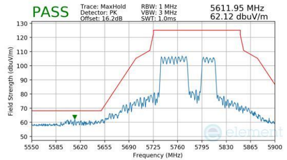
Plot 7-1093. CDD Diversity (Peak, RU484+242, Index 92, Ch.155, MCS11)
