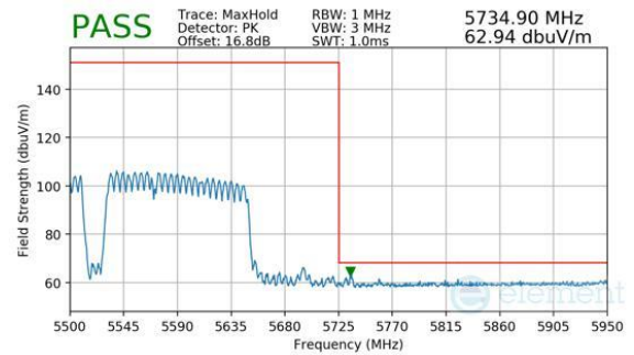
Plot 7-985. CDD Primary (Peak, RU996+484+242, Index 97 (L), Ch.114 (FCC ONLY), MCS11)
