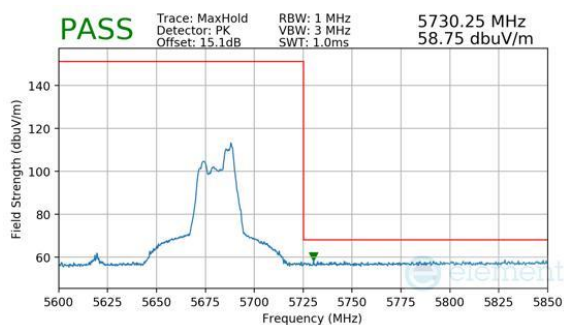
Plot 7-1047. CDD Diversity (Peak, RU52, Index 44, Ch.134, MCS11)
