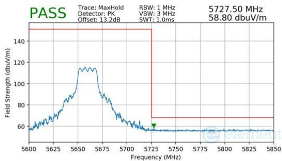
Plot 7-1029. CDD Diversity (Peak, RU242, Index 61, Ch.132, MCS11)
