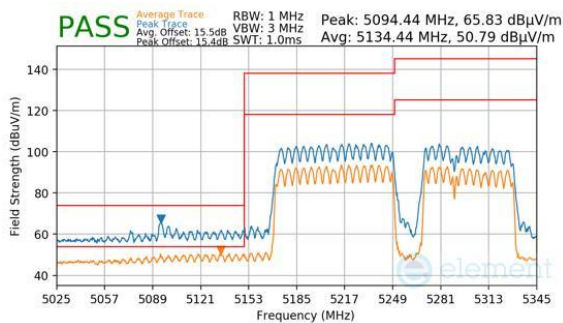
Plot 7-964. CDD Primary (Peak & Average, RU996+484+242, Index 96, Ch.50, MCS11)
