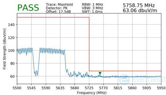
Plot 7-988. CDD Primary (Peak, RU996+484+242, Index 99 (L), Ch.114 (FCC ONLY), MCS11)
