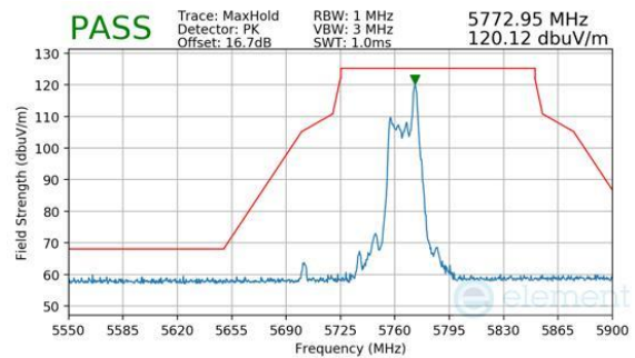
Plot 7-1037. CDD Diversity (Peak, RU26, Index 17, Ch.151, MCS11)
