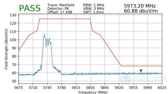
Plot 7-1063. CDD Diversity (Peak, RU26, Index 0, Ch.155, MCS11)
