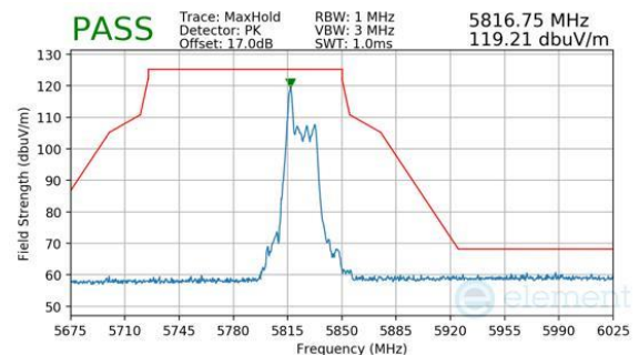
Plot 7-998. CDD Diversity (Peak, RU26, Index 0, Ch.165, MCS11)
