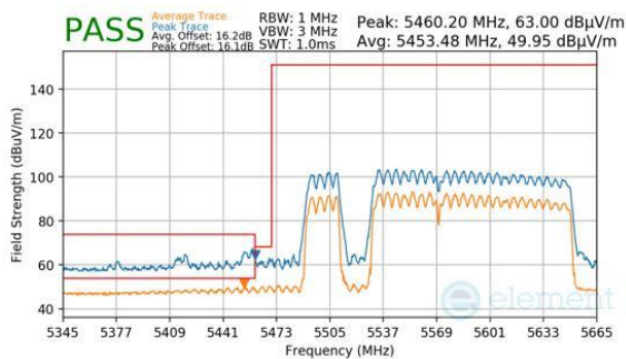
Plot 7-976. CDD Primary (Peak & Average, RU996+484+242, Index 97 (L), Ch.114 (FCC ONLY), MCS11)
