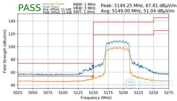
Plot 7-1048. CDD Diversity (Peak & Average, RU484, Index 65, Ch.38, MCS11)
