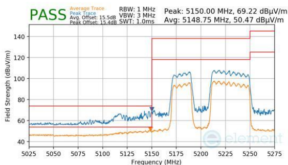
Plot 7-1072. CDD Diversity (Peak & Average, RU484+242, Index 91, Ch.42, MCS11)
