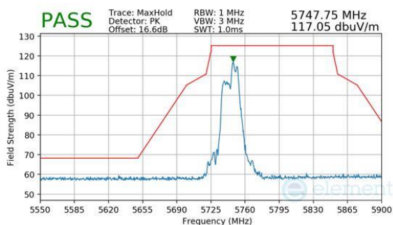
Plot 7-1019. CDD Diversity (Peak, RU52+26, Index 72, Ch.149, MCS11)
