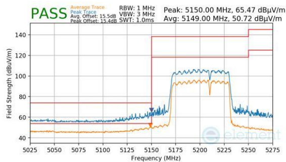
Plot 7-1074. CDD Diversity (Peak & Average, RU484+242, Index 93, Ch.42, MCS11)
