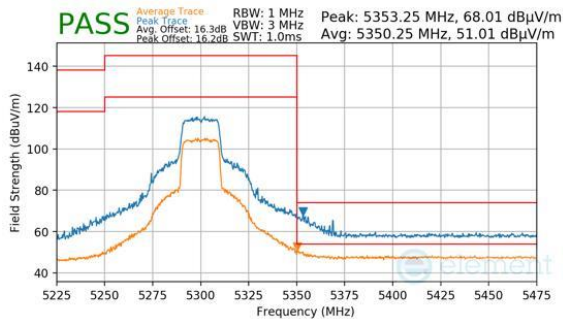
Plot 7-1024. CDD Diversity (Peak & Average, RU242, Index 61, Ch.60, MCS11)
