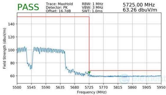
Plot 7-986. CDD Primary (Peak, RU996+484+242, Index 98 (L), Ch.114 (FCC ONLY), MCS11)
