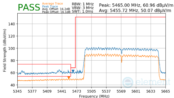
Plot 7-992. CDD Primary (Peak & Average, RU996X2, Index 68, Ch.114 FCC ONLY, MCS11)
