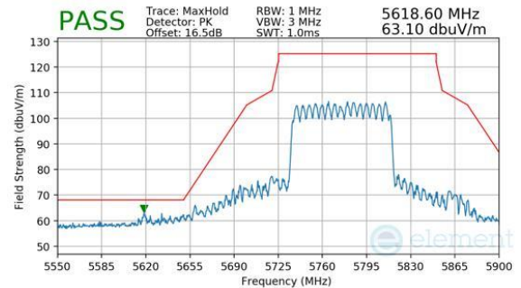
Plot 7-940. CDD Primary (Peak, RU996, Index 67, Ch.155, MCS11)
