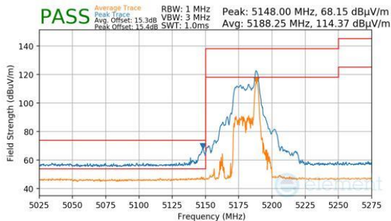
Plot 7-995. CDD Diversity (Peak & Average, RU26, Index 8, Ch.36, MCS11)
