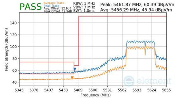
Plot 7-1086. CDD Diversity (Peak & Average, RU484+242, Index 93, Ch.122 (FCC ONLY), MCS11)
