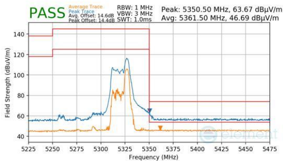
Plot 7-1041. CDD Diversity (Peak & Average, RU52, Index 44, Ch.62, MCS11)
