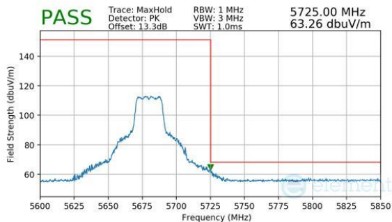
Plot 7-1030. CDD Diversity (Peak, RU242, Index 61, Ch.136, MCS11)
