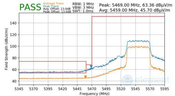
Plot 7-1053. CDD Diversity (Peak & Average, RU484, Index 65, Ch.110, MCS11)
