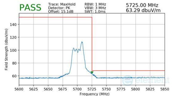
Plot 7-1005. CDD Diversity (Peak, RU52, Index 40, Ch.140, MCS11)
