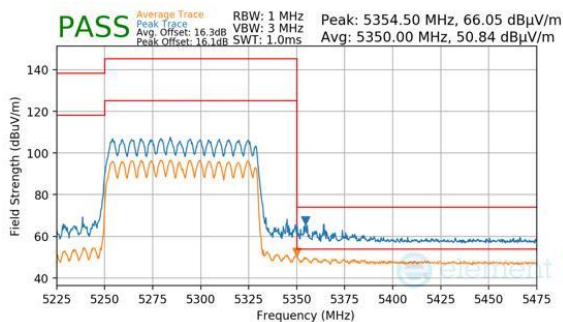
Plot 7-936. CDD Primary (Peak & Average, RU996, Index 67, Ch.58, MCS11)
