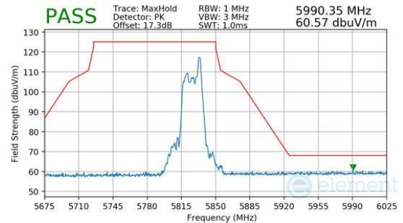
Plot 7-999. CDD Diversity (Peak, RU26, Index 8, Ch.165, MCS11)
