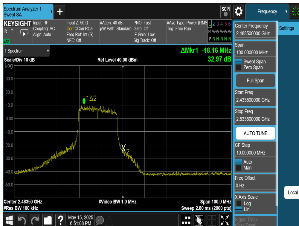
Plot 7-55. Band Edge Plot Antenna 4a (802.11n (2.4GHz) – Ch. 13)
