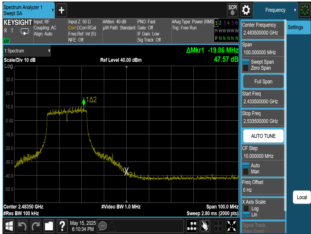
Plot 7-40. Band Edge Plot Antenna 4a (802.11g – Ch. 10)
