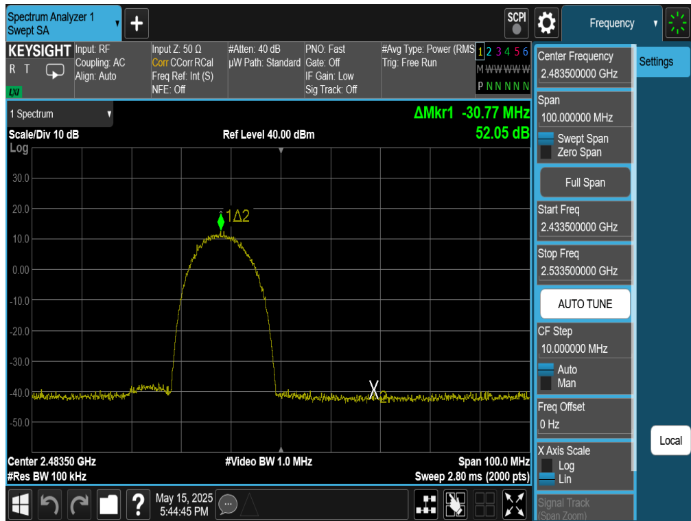
Plot 7-31. Band Edge Plot Antenna 4a (802.11b – Ch. 13)
