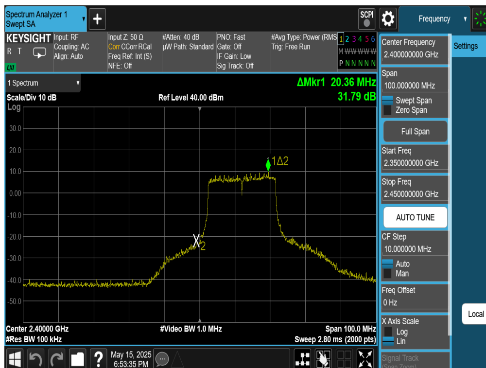
Plot 7-56. Band Edge Plot Antenna 4a (802.11be (SU - 2.4GHz) – Ch. 1)
