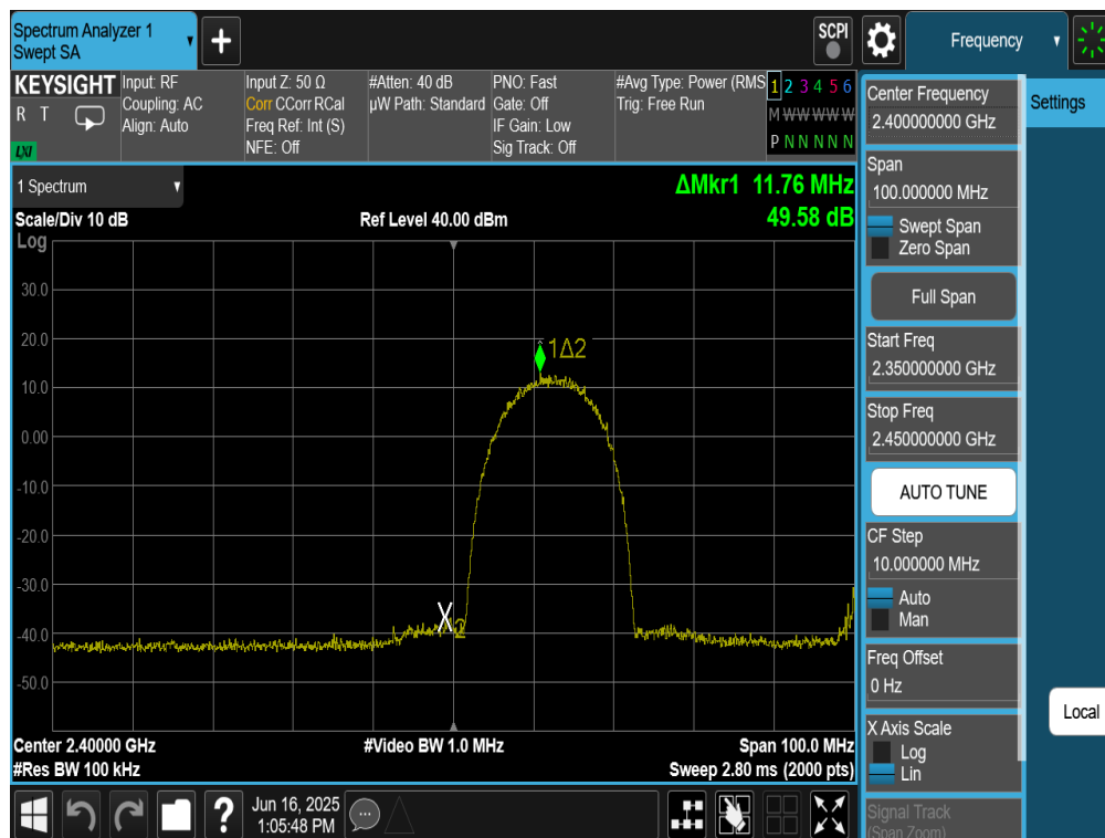
Plot 7-25. Band Edge Plot Antenna 4a (802.11b – Ch. 1)
