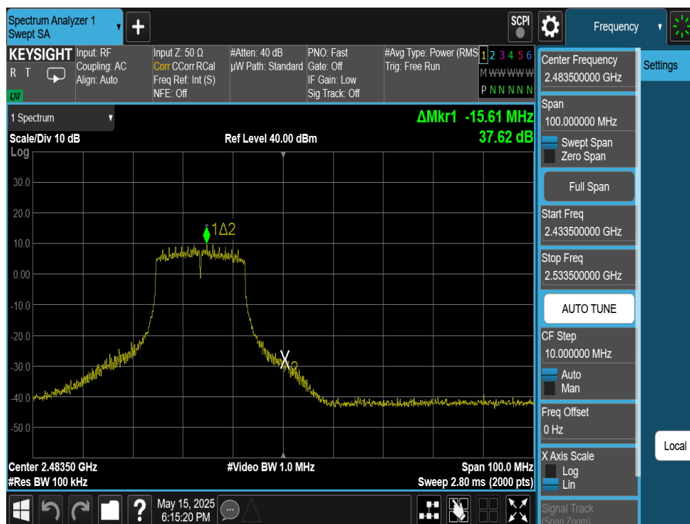
Plot 7-42. Band Edge Plot Antenna 4a (802.11g – Ch. 12)
