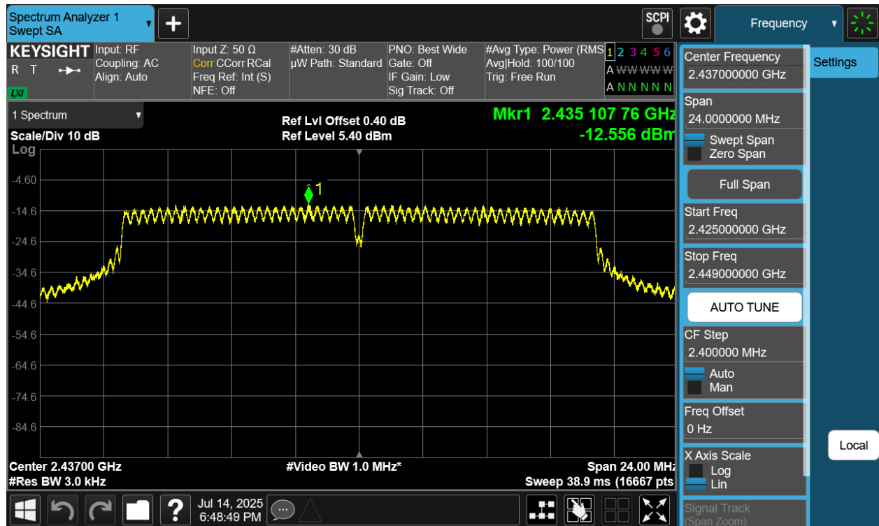
Plot 7-15 PSD Antenna 2a (20MHz BW 802.11n - Ch.6)
