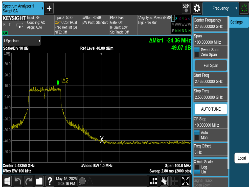
Plot 7-39. Band Edge Plot Antenna 4a (802.11g – Ch. 9)
