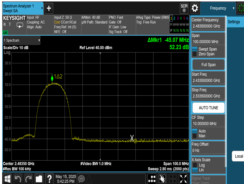
Plot 7-28. Band Edge Plot Antenna 4a (802.11b – Ch. 10)
