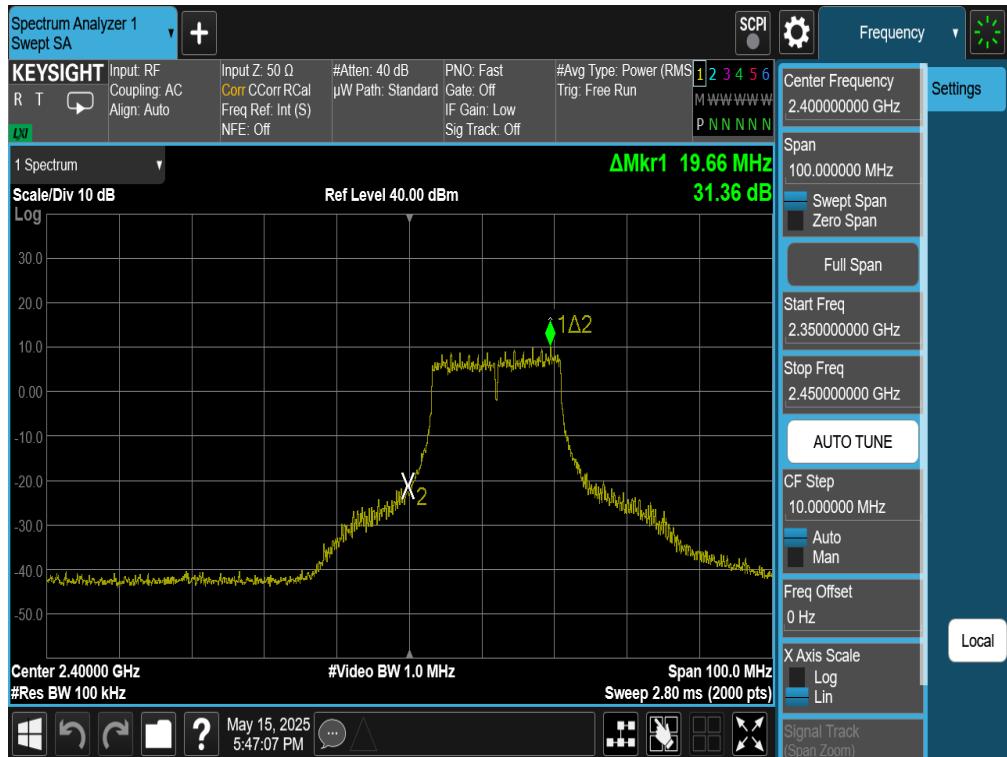
Plot 7-32. Band Edge Plot Antenna 4a (802.11g – Ch. 1)
