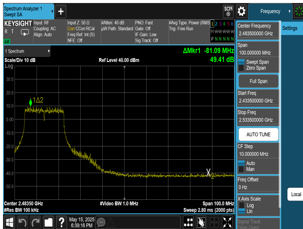
Plot 7-50. Band Edge Plot Antenna 4a (802.11n (2.4GHz) – Ch. 8)
