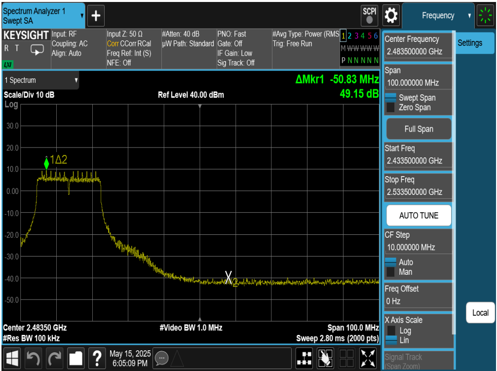
Plot 7-38. Band Edge Plot Antenna 4a (802.11g – Ch. 8)
