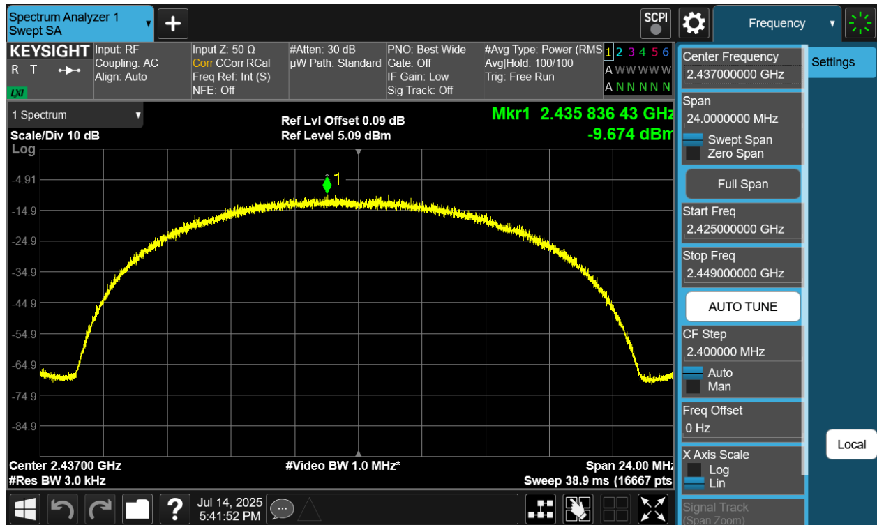
Plot 7-17 PSD CDD Antenna 4a (20MHz BW 802.11b - Ch.6)
