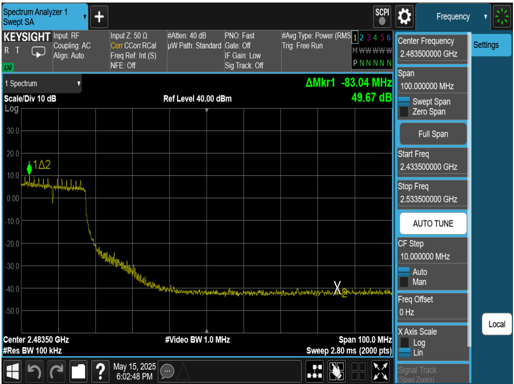
Plot 7-37. Band Edge Plot Antenna 4a (802.11g – Ch. 7)
