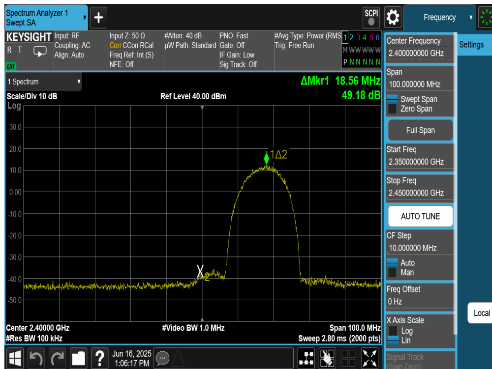
Plot 7-26. Band Edge Plot Antenna 4a (802.11b – Ch. 2)
