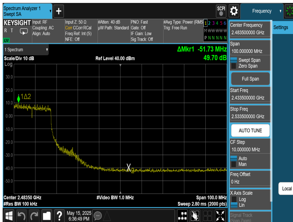
Plot 7-49. Band Edge Plot Antenna 4a (802.11n (2.4GHz) – Ch. 7)
