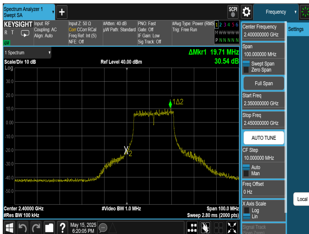
Plot 7-44. Band Edge Plot Antenna 4a (802.11n (2.4GHz) – Ch. 1)
