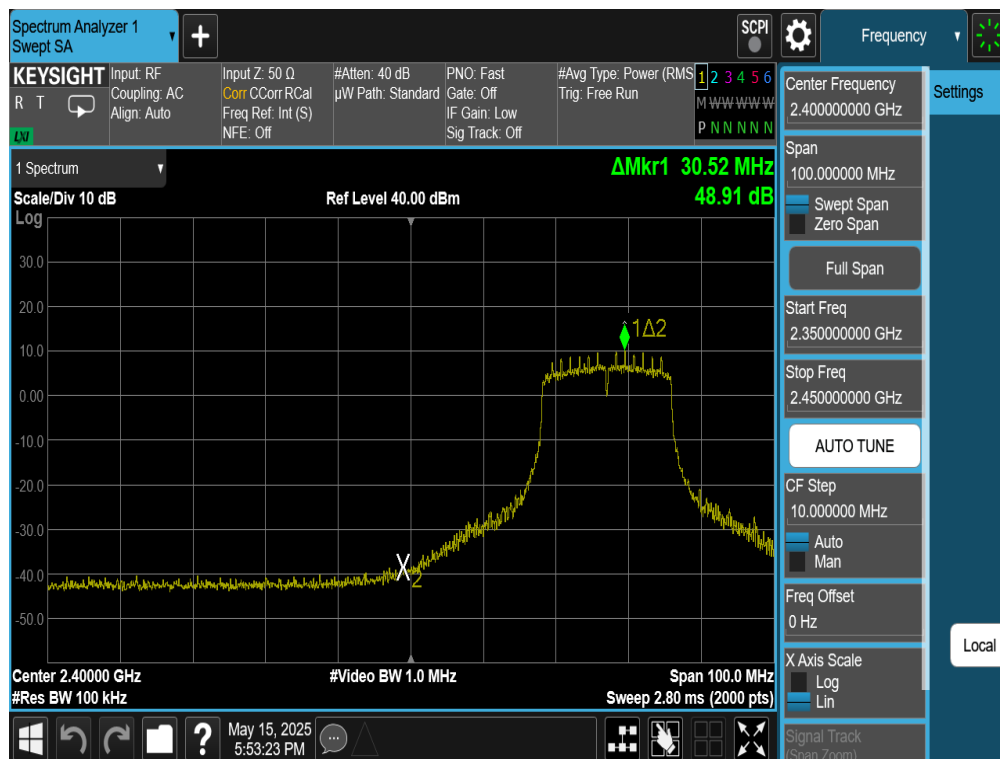
Plot 7-35. Band Edge Plot Antenna 4a (802.11g – Ch. 4)
