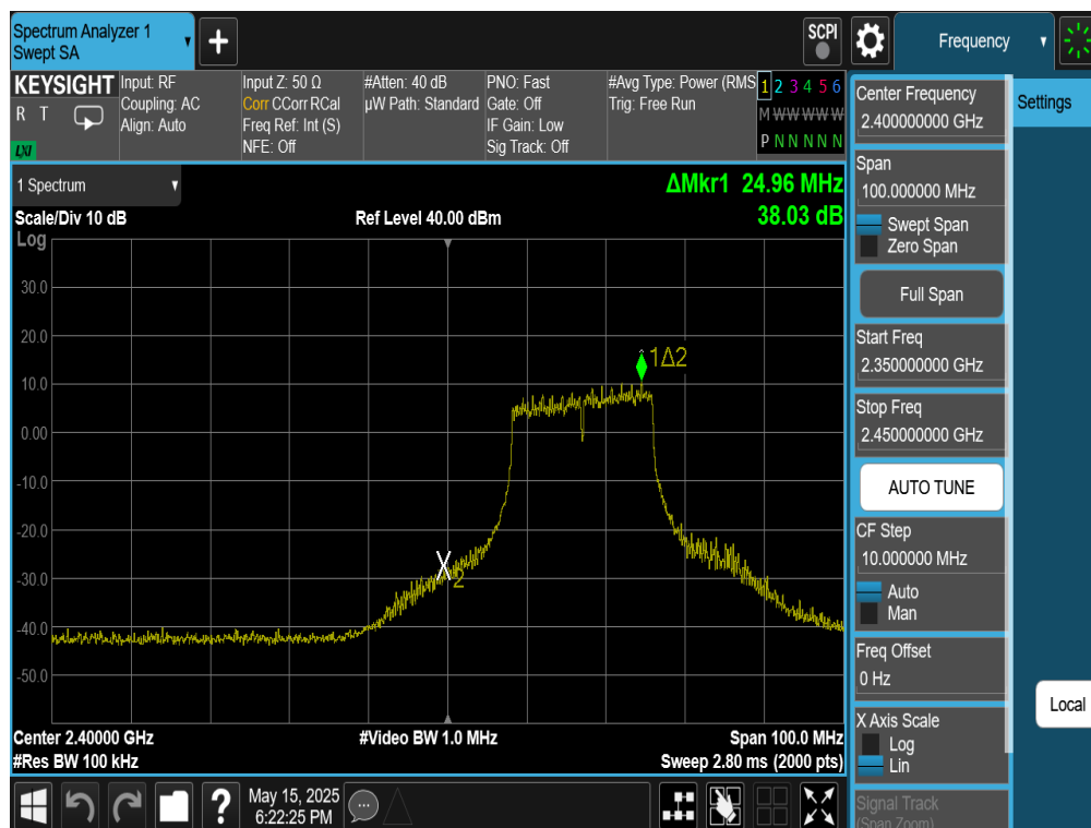
Plot 7-45. Band Edge Plot Antenna 4a (802.11n (2.4GHz) – Ch. 2)
