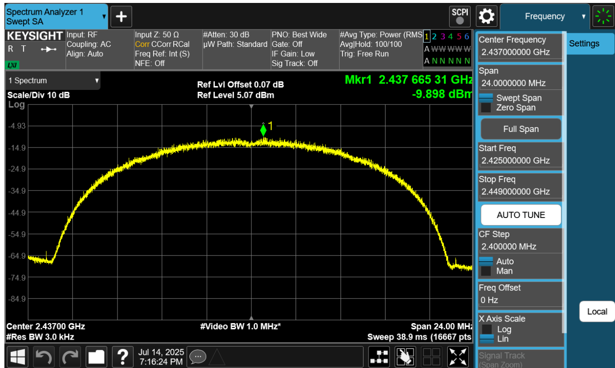
Plot 7-21 PSD CDD Antenna 2a (20MHz BW 802.11b - Ch.6)
