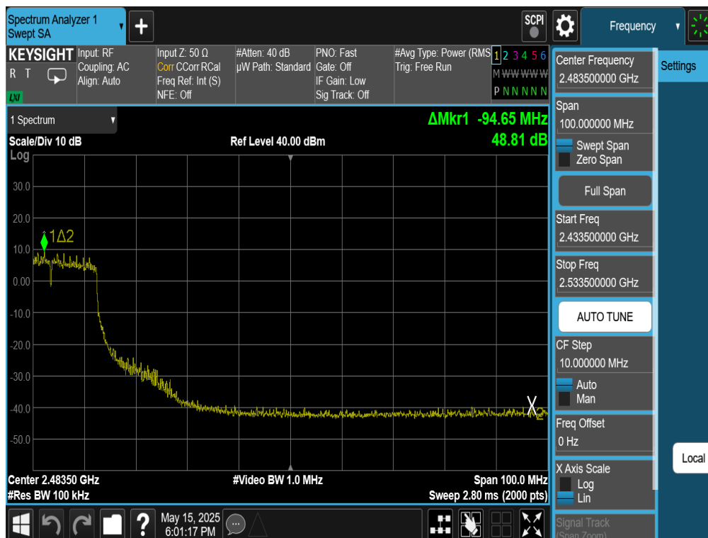
Plot 7-36. Band Edge Plot Antenna 4a (802.11g – Ch. 6)
