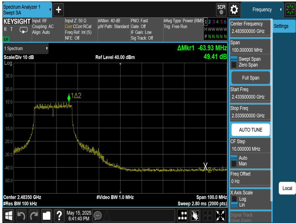
Plot 7-51. Band Edge Plot Antenna 4a (802.11n (2.4GHz) – Ch. 9)
