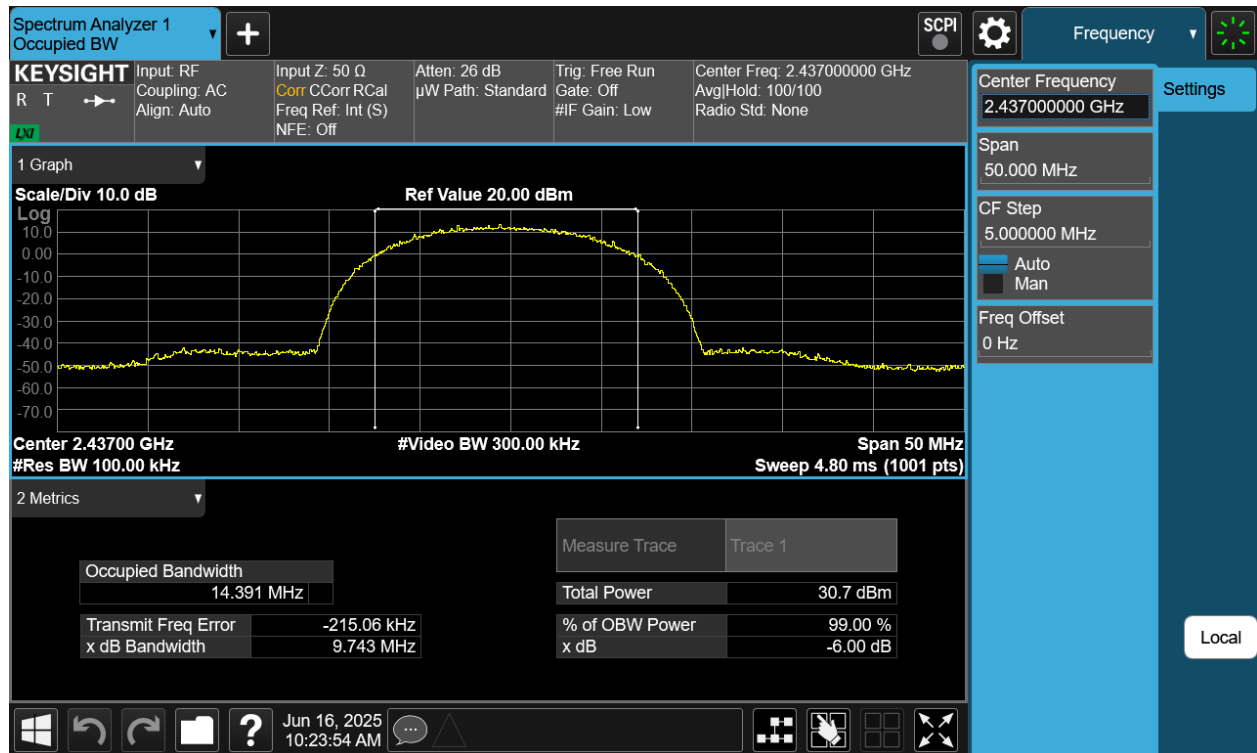
Plot 7-1 6dB BW & 99% OBW Antenna 4a (20MHz BW 802.11b - Ch.6)
