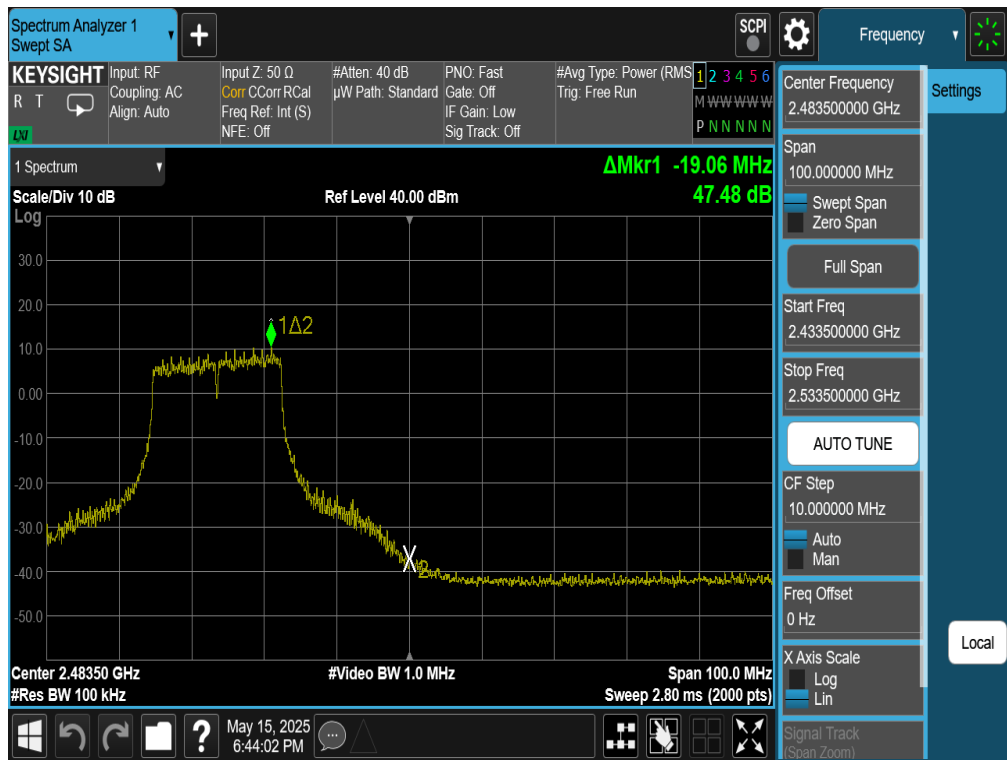
Plot 7-52. Band Edge Plot Antenna 4a (802.11n (2.4GHz) – Ch. 10)
