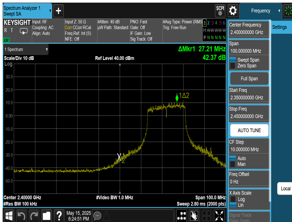
Plot 7-46. Band Edge Plot Antenna 4a (802.11n (2.4GHz) – Ch. 3)
