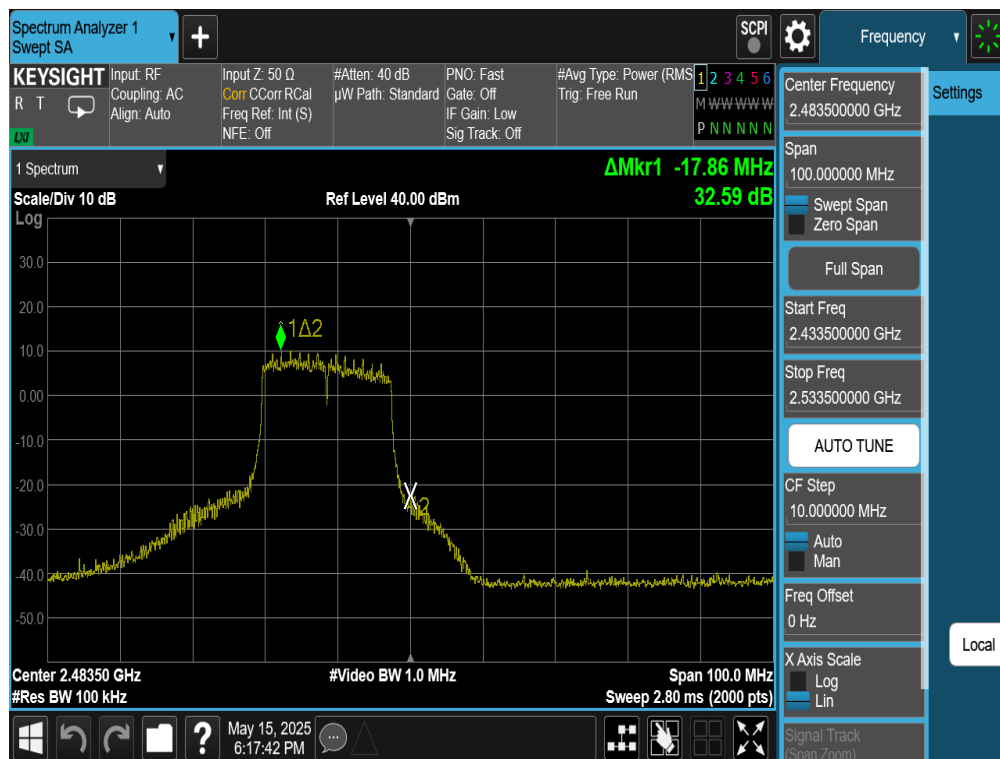
Plot 7-43. Band Edge Plot Antenna 4a (802.11g – Ch. 13)
