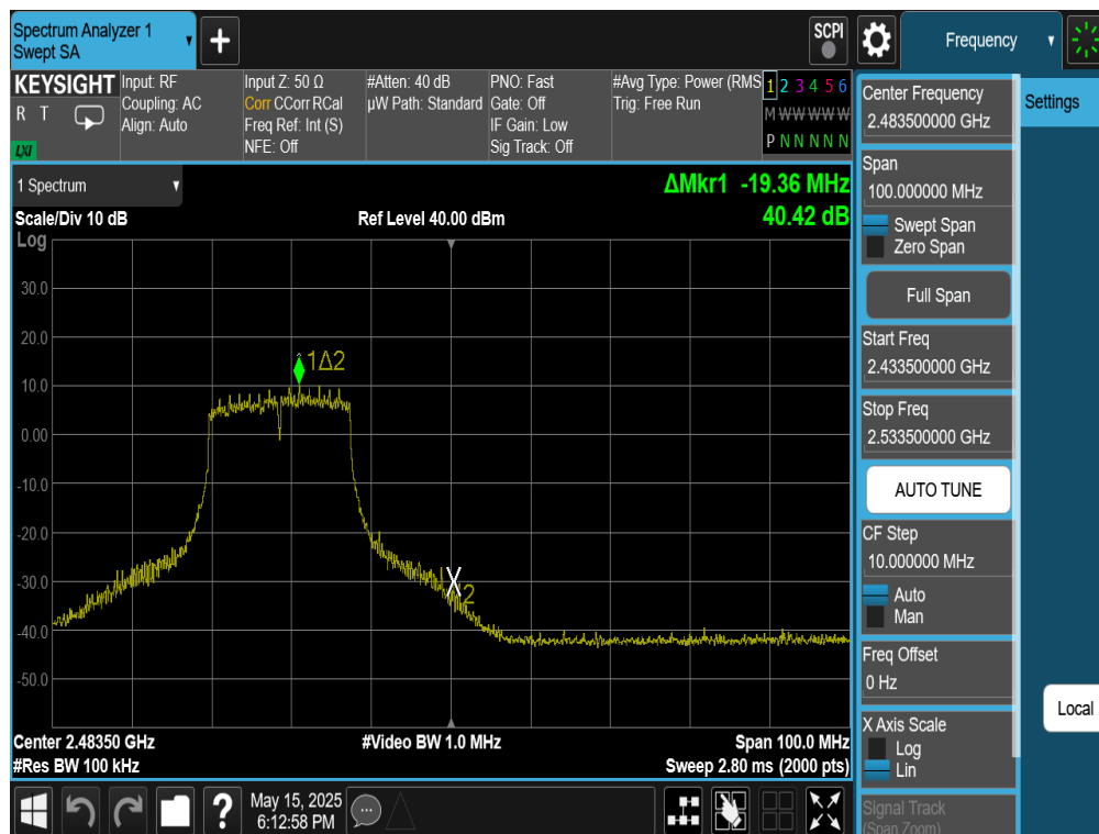
Plot 7-41. Band Edge Plot Antenna 4a (802.11g – Ch. 11)
