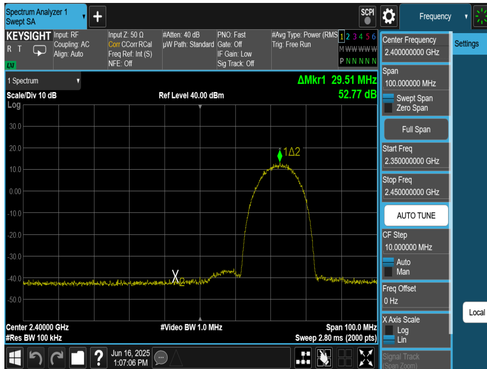
Plot 7-27. Band Edge Plot Antenna 4a (802.11b – Ch. 3)
