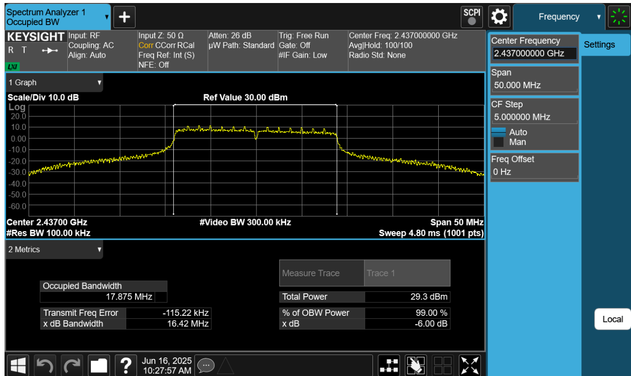
Plot 7-2 6dB BW & 99% OBW Antenna 4a (20MHz BW 802.11g - Ch.6)
