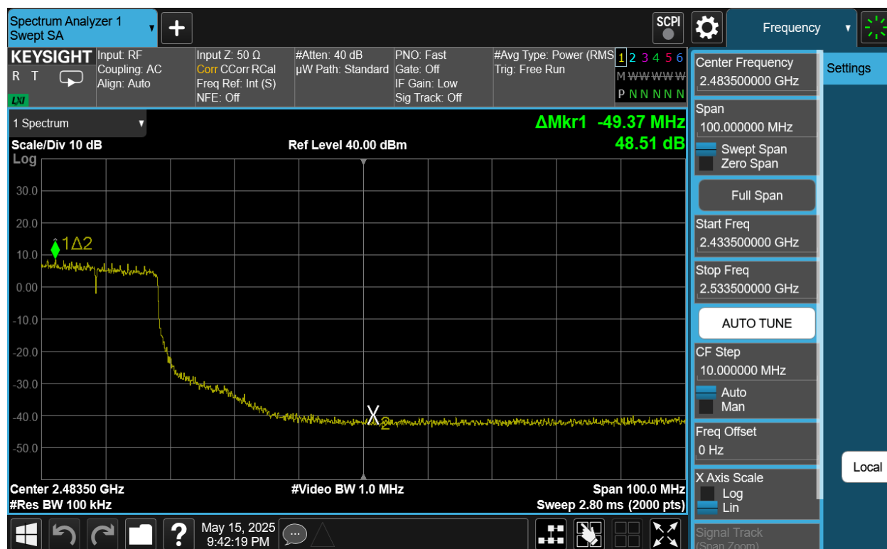
Plot 7-36. Band Edge Antenna 4a (802.11be OFDMA – RU242 – Ch. 7)
