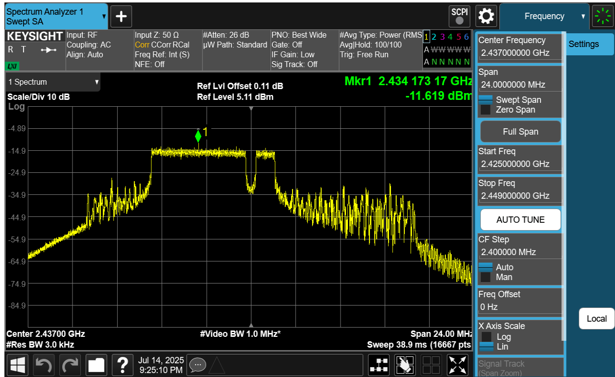
Plot 7-19 PSD CDD Antenna 4a (20MHz BW 802.11be(RU) RU52+26 Index71 - Ch.6)
