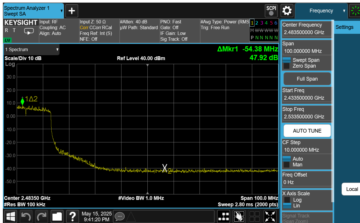
Plot 7-35. Band Edge Antenna 4a (802.11be OFDMA – RU242 – Ch. 6(High Channel))
