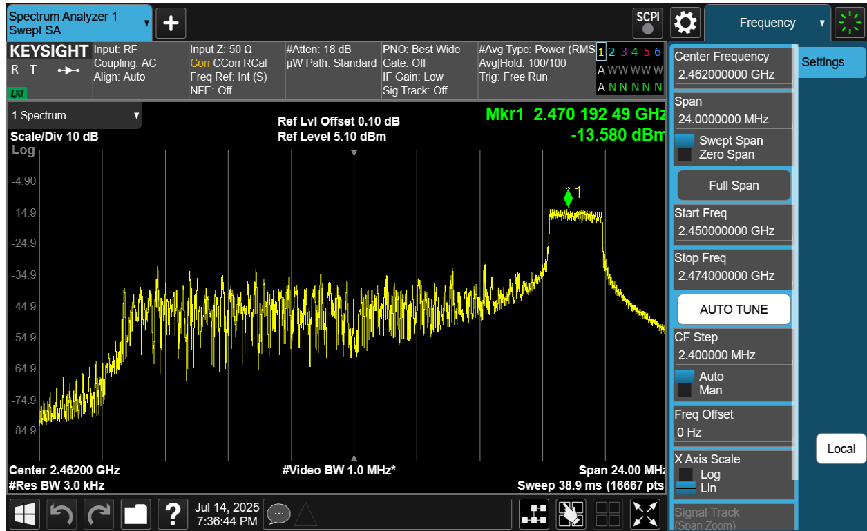
Plot 7-21 PSD CDD Antenna 2a (20MHz BW 802.11be(RU) RU26 Index8 - Ch.11)
