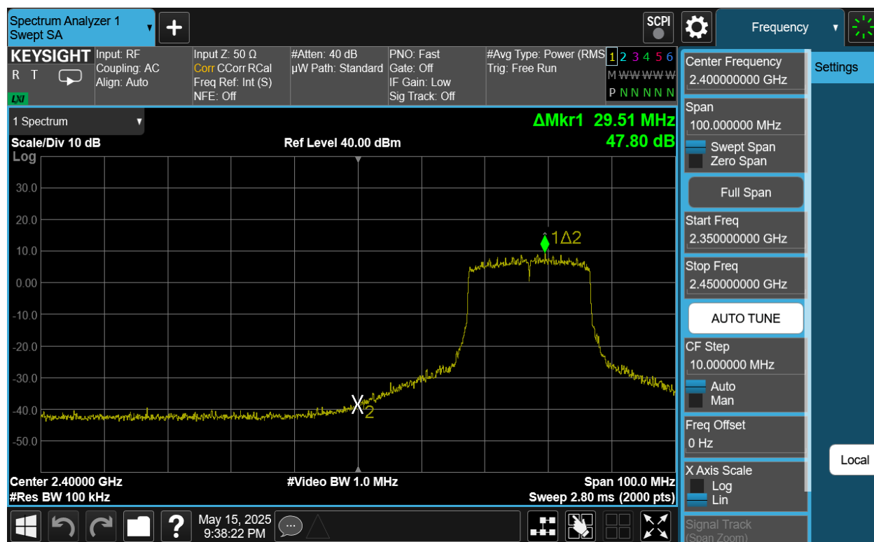
Plot 7-32. Band Edge Antenna 4a (802.11be OFDMA – RU242 – Ch. 4)
