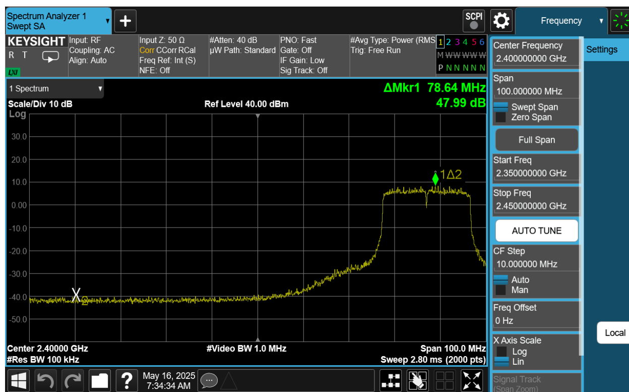
Plot 7-52. Band Edge Antenna 2a (802.11be OFDMA – RU242 – Ch. 6(Low Channel))
