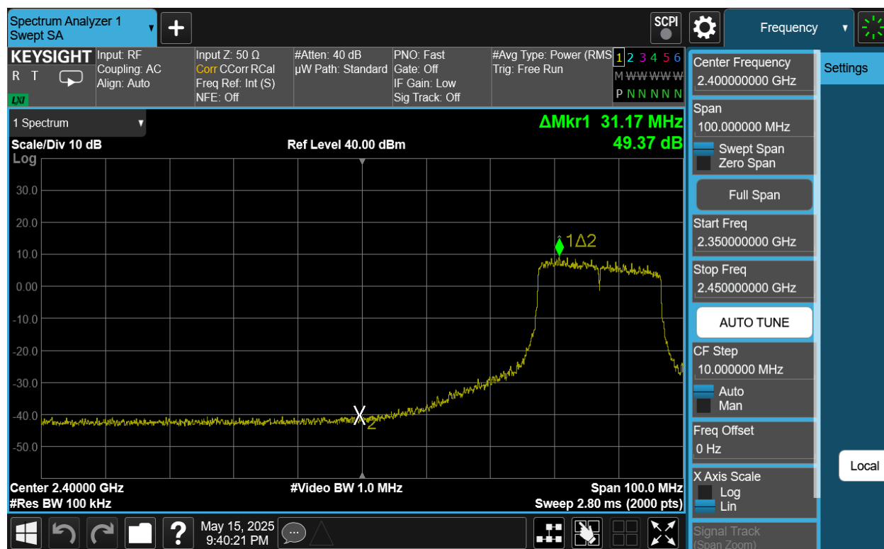
Plot 7-34. Band Edge Antenna 4a (802.11be OFDMA – RU242 – Ch. 6(Low Channel))
