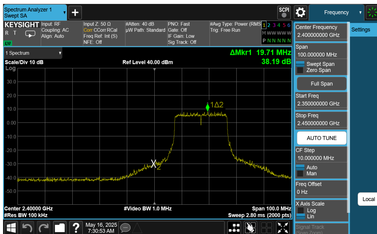
Plot 7-48. Band Edge Antenna 2a (802.11be OFDMA – RU242 – Ch. 2)
