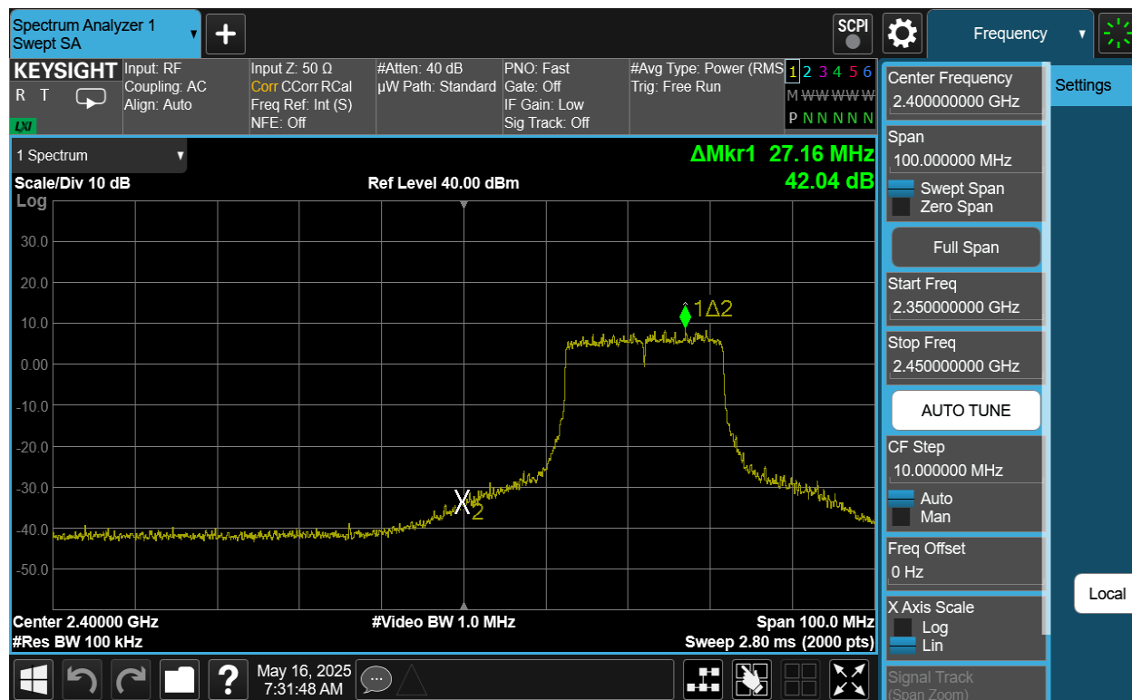
Plot 7-49. Band Edge Antenna 2a (802.11be OFDMA - RU242 - Ch. 3)
