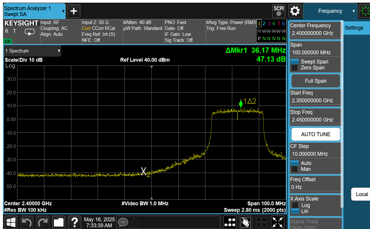
Plot 7-51. Band Edge Antenna 2a (802.11be OFDMA – RU242 – Ch. 5)
