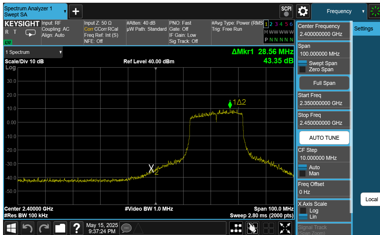
Plot 7-31. Band Edge Antenna 4a (802.11be OFDMA – RU242 – Ch. 3)
