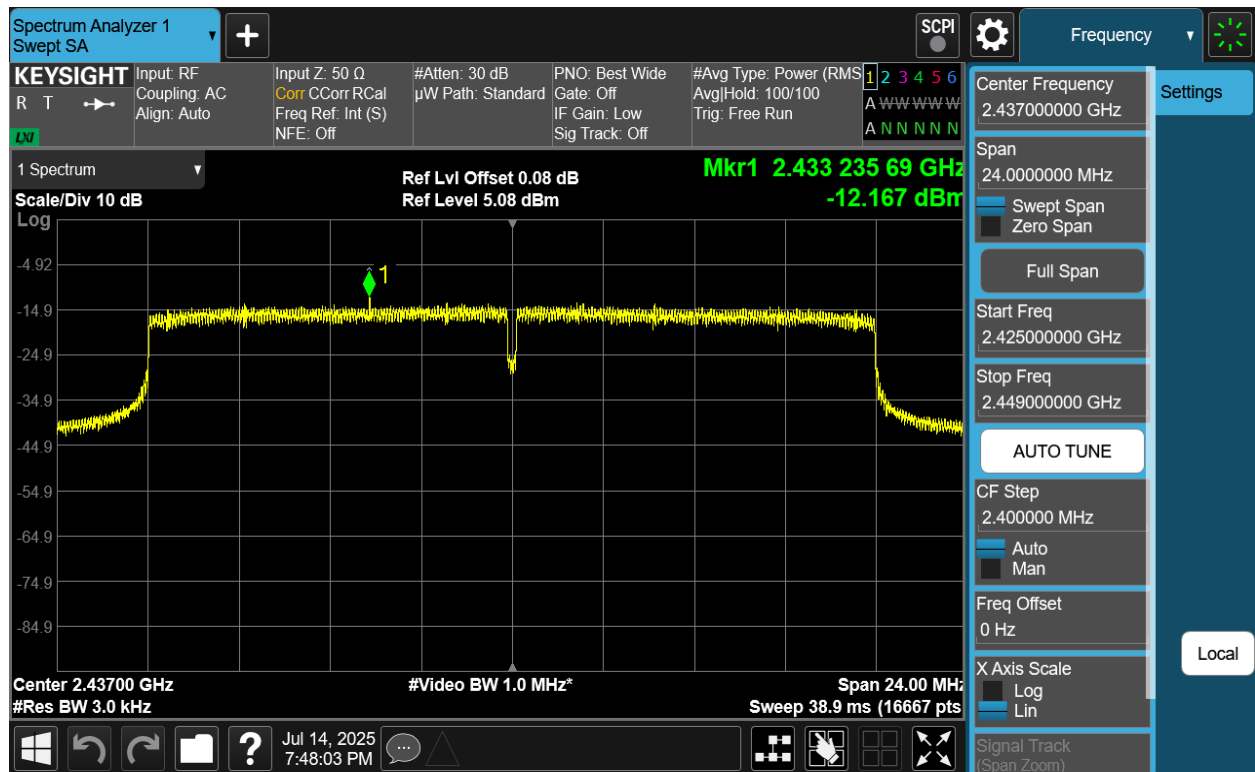
Plot 7-22 PSD CDD Antenna 2a (20MHz BW 802.11be(RU) RU242 Index61 - Ch.6)
