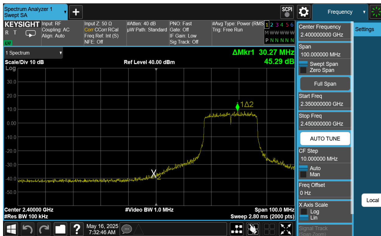
Plot 7-50. Band Edge Antenna 2a (802.11be OFDMA - RU242 - Ch. 4)
