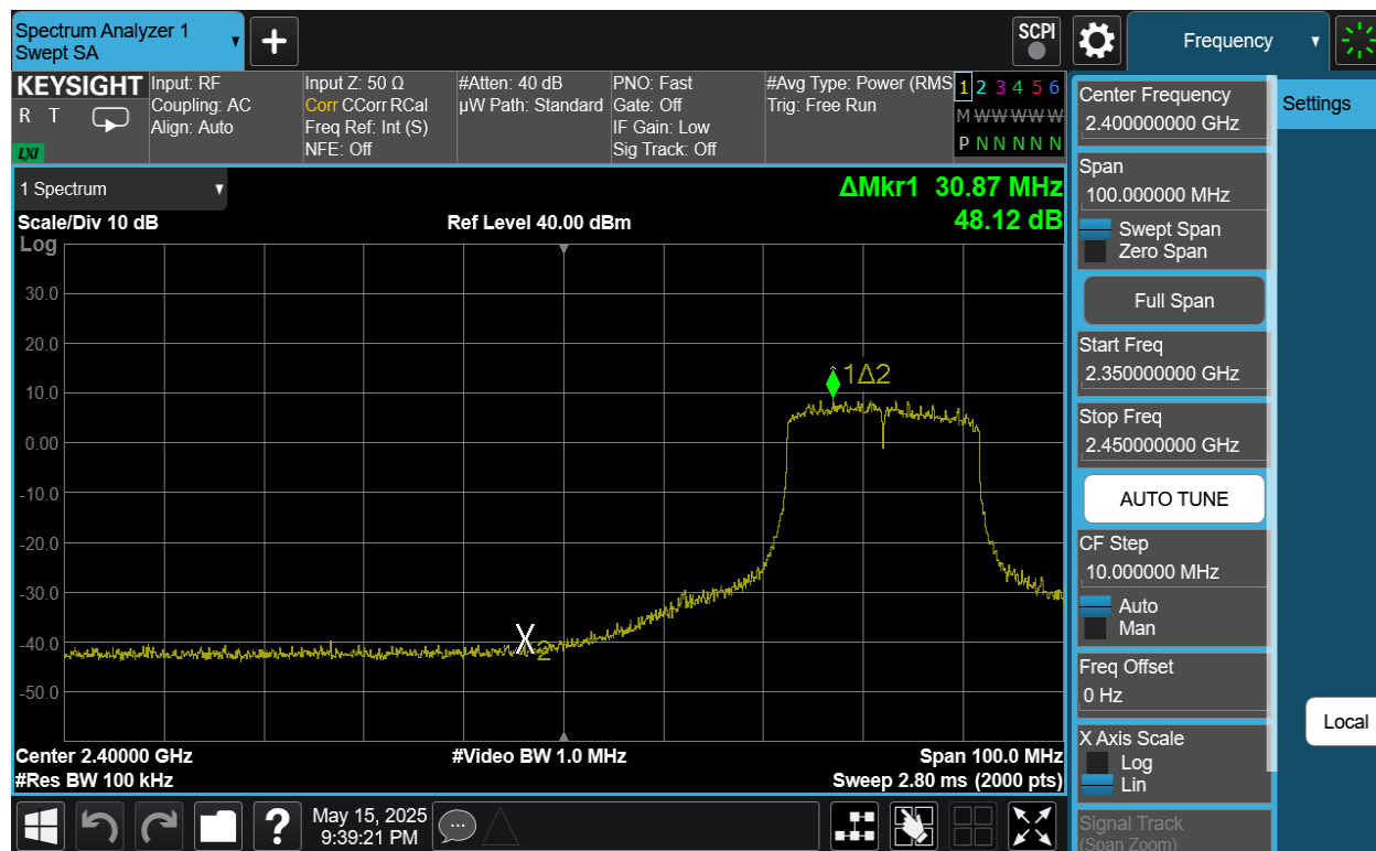
Plot 7-33. Band Edge Antenna 4a (802.11be OFDMA – RU242 – Ch. 5)
