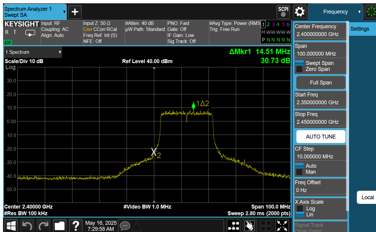
Plot 7-47. Band Edge Antenna 2a (802.11be OFDMA – RU242 – Ch. 1)
