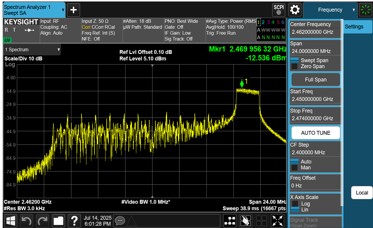
Plot 7-17 PSD CDD Antenna 4a (20MHz BW 802.11be(RU) RU26 Index8 - Ch.11)
