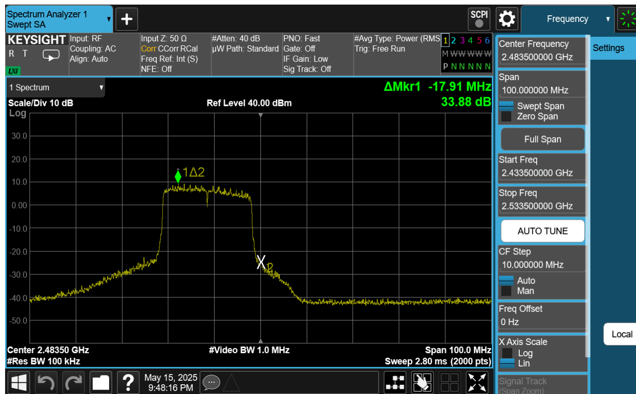
Plot 7-42. Band Edge Antenna 4a (802.11be OFDMA – RU242 – Ch. 13)
