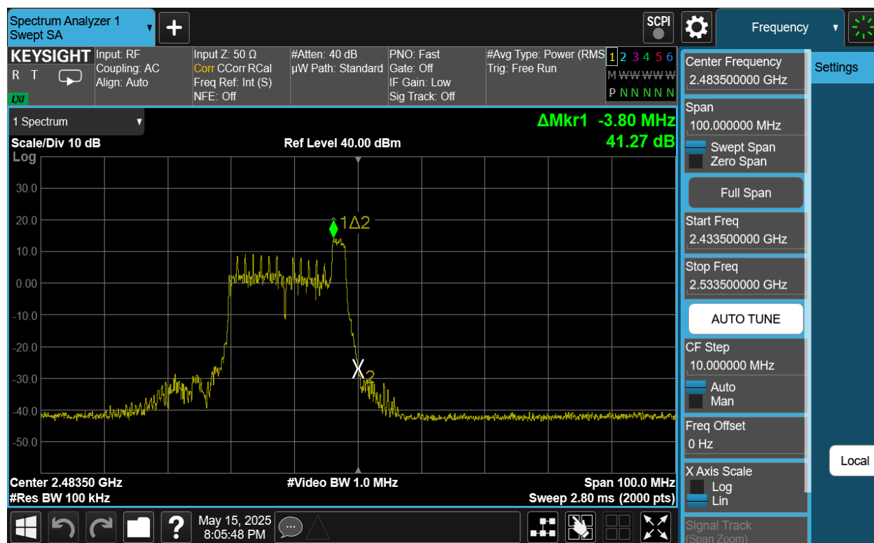
Plot 7-28. Band Edge Antenna 4a (802.11be OFDMA – RU26 Index 8 – Ch. 13)
