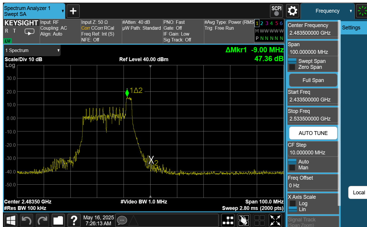
Plot 7-45. Band Edge Antenna 2a (802.11be OFDMA – RU26 Index 8 – Ch. 12)
