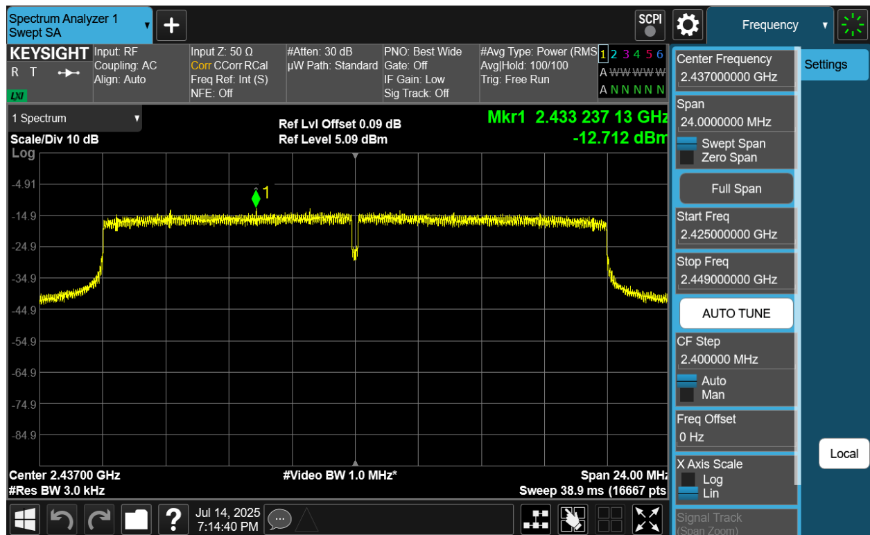
Plot 7-14 PSD Antenna 2a (20MHz BW 802.11be(RU) RU242 Index61 - Ch.6)
