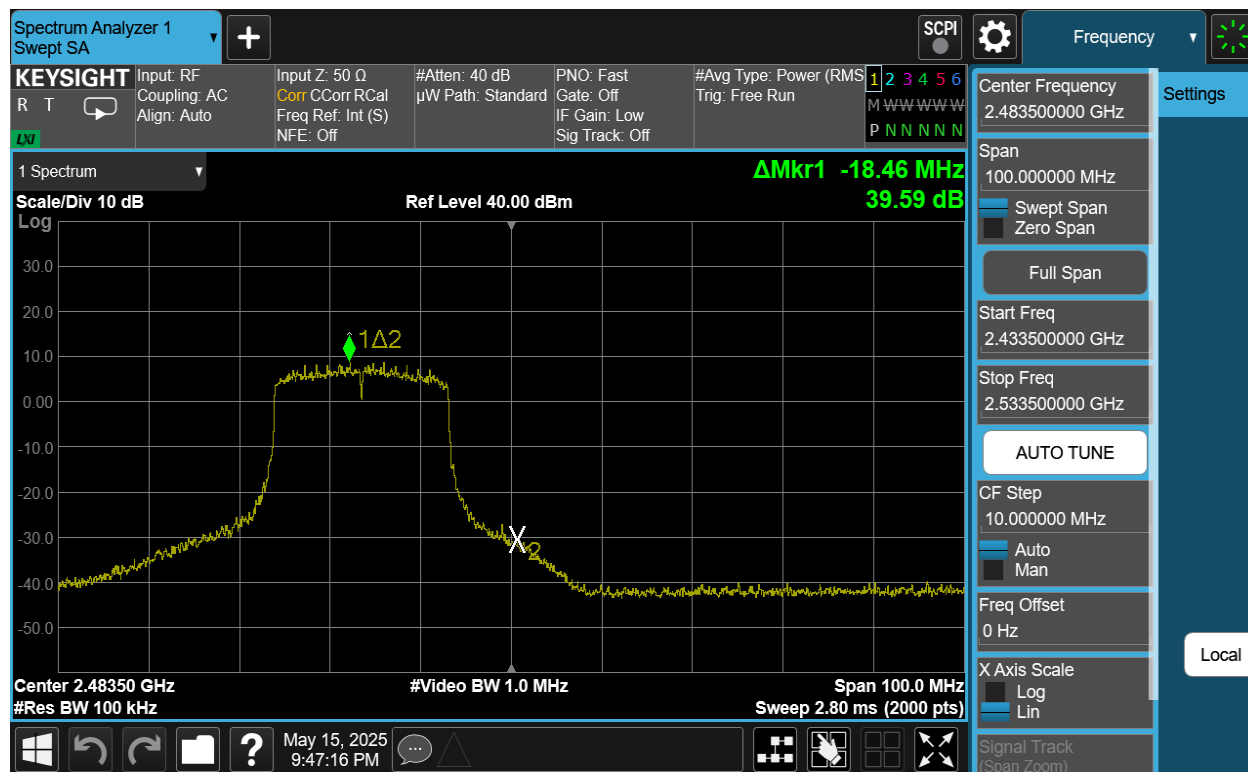
Plot 7-41. Band Edge Antenna 4a (802.11be OFDMA – RU242 – Ch. 12)
