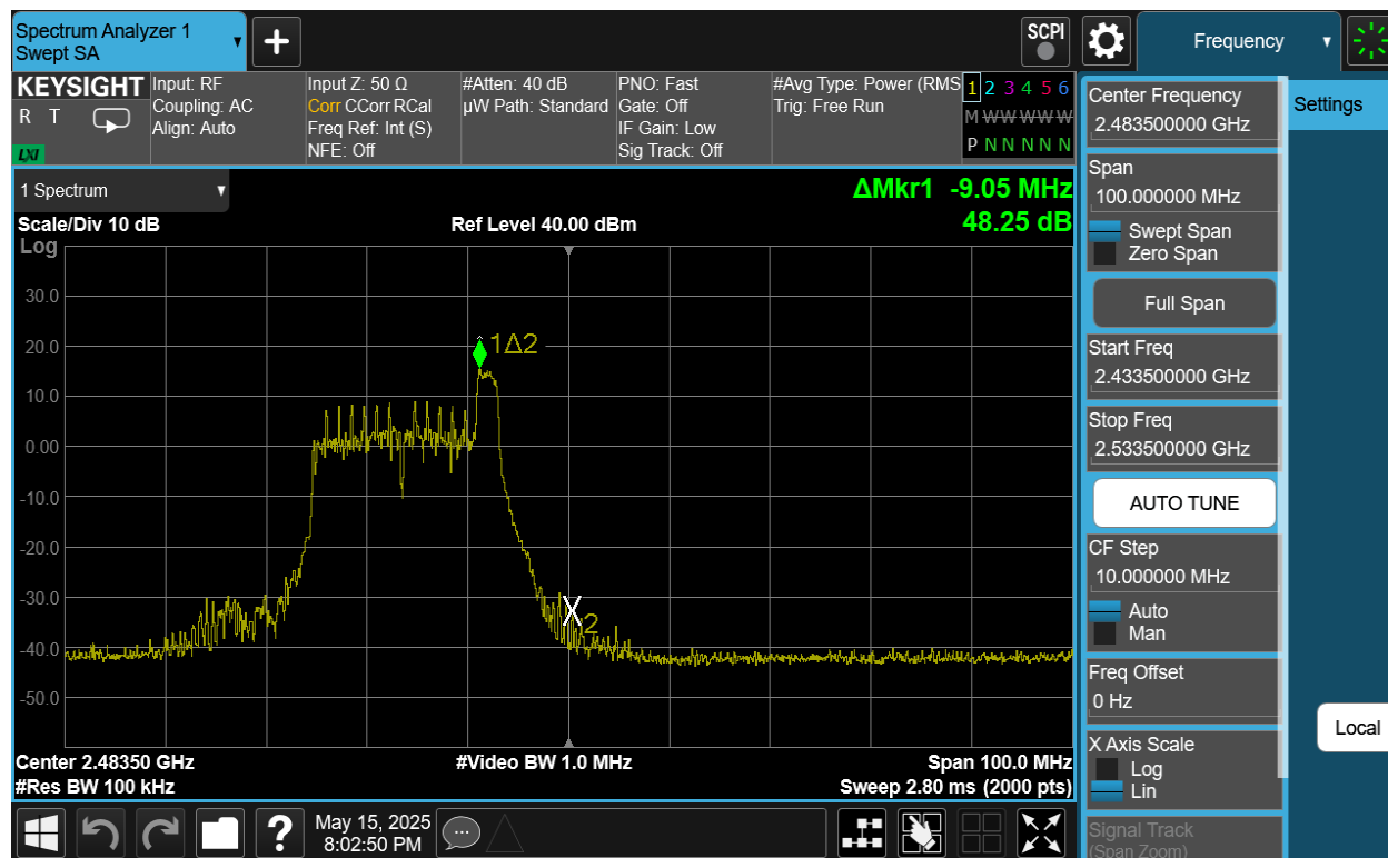
Plot 7-27. Band Edge Antenna 4a (802.11be OFDMA – RU26 Index 8 – Ch. 12)
