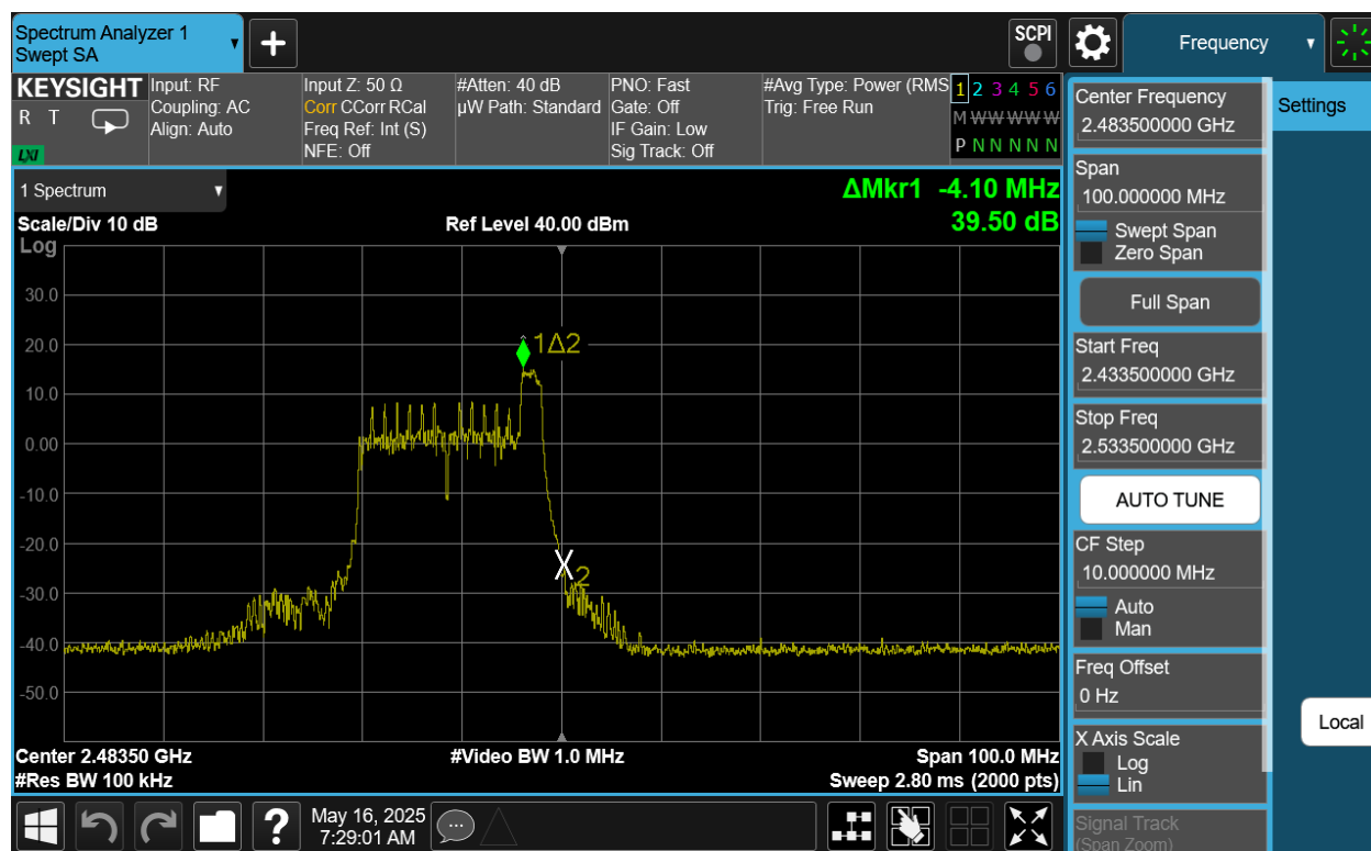
Plot 7-46. Band Edge Antenna 2a (802.11be OFDMA – RU26 Index 8 – Ch. 13)
