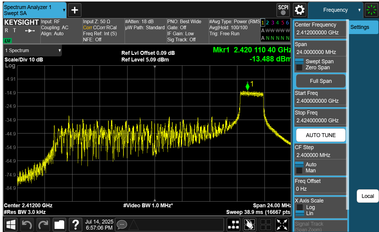
Plot 7-13 PSD Antenna 2a (20MHz BW 802.11be(RU) RU26 Index8 - Ch.1)
