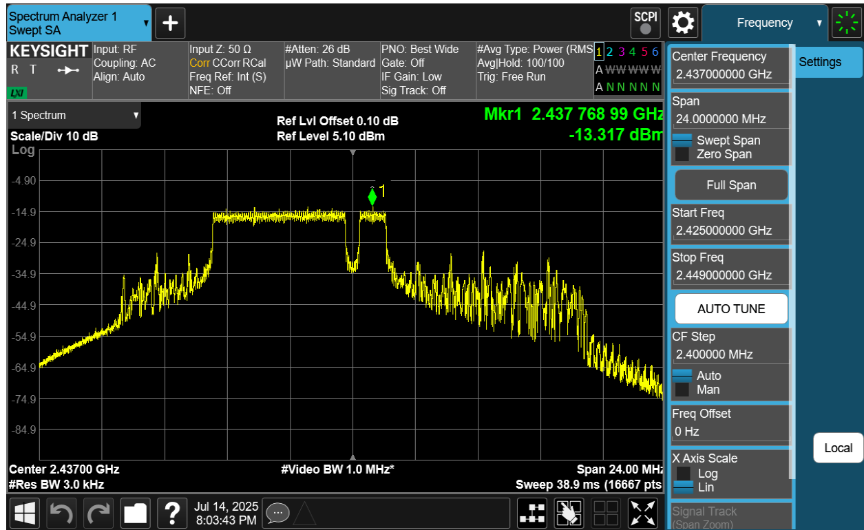
Plot 7-23 PSD CDD Antenna 2a (20MHz BW 802.11be(RU) RU52+26 Index71 - Ch.6)
