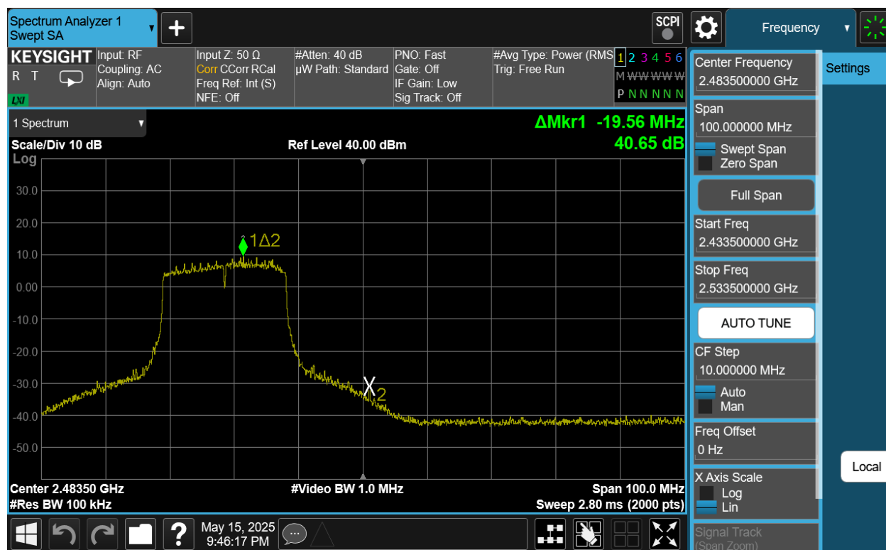
Plot 7-40. Band Edge Antenna 4a (802.11be OFDMA – RU242 – Ch. 11)
