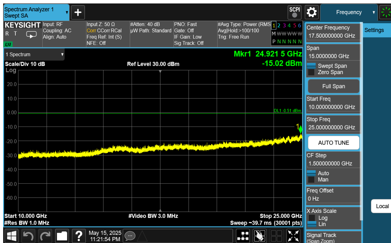
Plot 7-72. Conducted Spurious Plot Antenna 4a (802.11be OFDMA – RU242 – Ch. 11)
