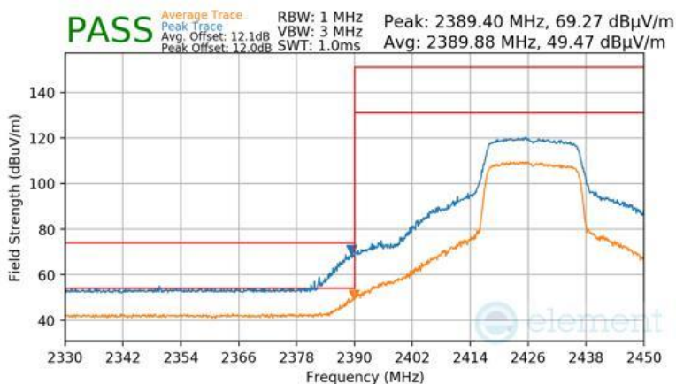
Plot 7-124 Radiated Restricted Lower Band Edge Measurement Antenna 4a (Peak & Average – RU242)
