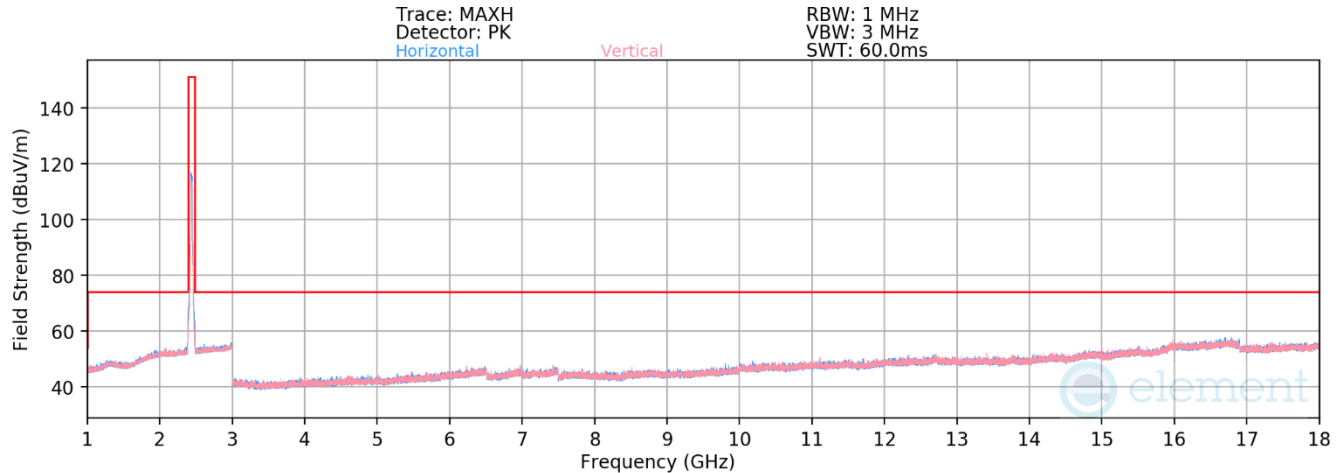
Plot 7-90. Radiated Spurious Emissions above 1GHz CDD (802.11be OFDMA – RU242 – Ch. 6)
