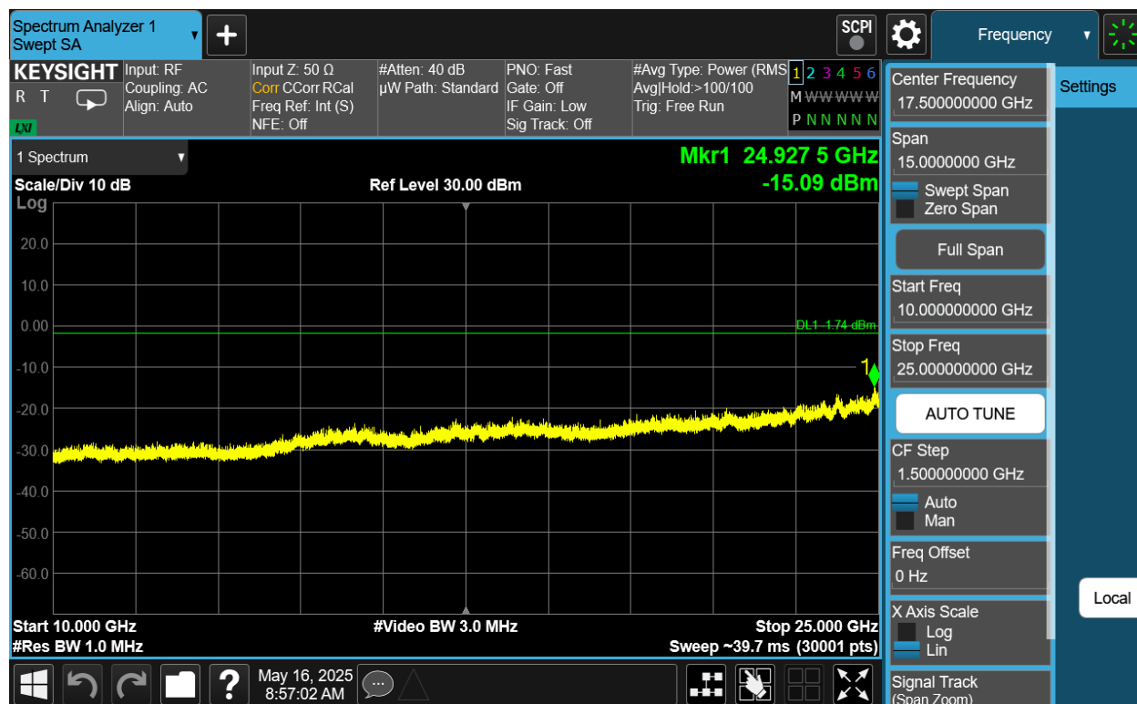
Plot 7-80. Conducted Spurious Plot Antenna 2a (802.11be OFDMA – RU242 – Ch. 1)
