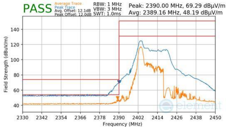
Plot 7-135 Radiated Restricted Lower Band Edge Measurement Antenna 2a (Peak & Average – RU26)
