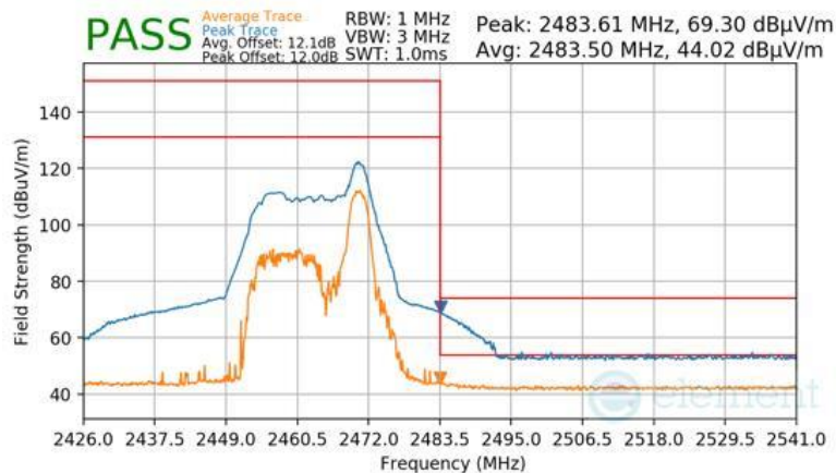
Plot 7-94 Radiated Restricted Upper Band Edge Measurement Antenna 4a (Peak & Average – RU26)
