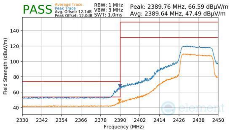
Plot 7-126 Radiated Restricted Lower Band Edge Measurement Antenna 4a (Peak & Average – RU242)
