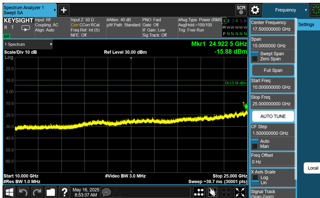
Plot 7-78. Conducted Spurious Plot Antenna 2a (802.11be OFDMA – RU26 – Ch. 11)
