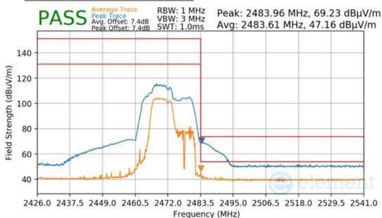
Plot 7-119 Radiated Restricted Upper Band Edge Measurement Antenna 4a (Peak & Average – RU52+26)
