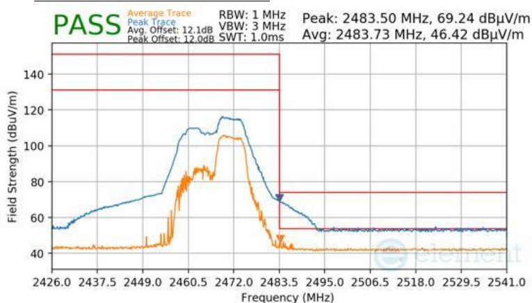
Plot 7-117 Radiated Restricted Upper Band Edge Measurement Antenna 4a (Peak & Average – RU52+26)
