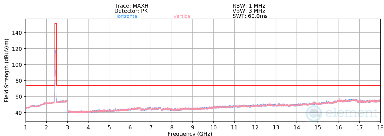
Plot 7-89. Radiated Spurious Emissions above 1GHz CDD (802.11be OFDMA – RU242 – Ch. 1)
