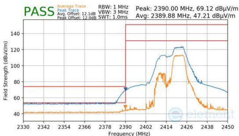
Plot 7-102 Radiated Restricted Lower Band Edge Measurement Antenna 4a (Peak & Average – RU52+26)
