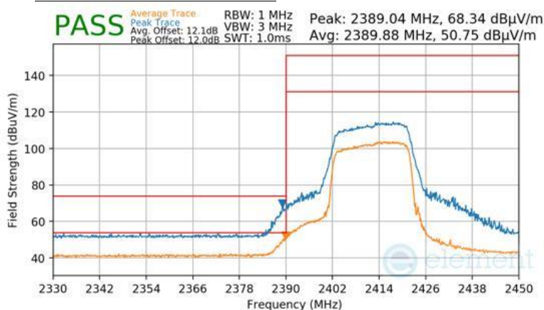
Plot 7-121 Radiated Restricted Lower Band Edge Measurement Antenna 4a (Peak & Average – RU242)
