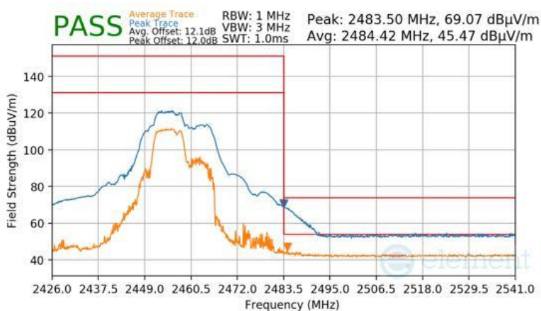
Plot 7-110 Radiated Restricted Upper Band Edge Measurement Antenna 4a (Peak & Average – RU52+26)
