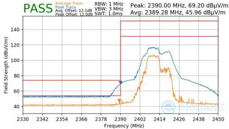
Plot 7-98 Radiated Restricted Lower Band Edge Measurement Antenna 4a (Peak & Average – RU52+26)
