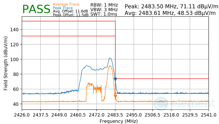
Plot 7-96 Radiated Restricted Upper Band Edge Measurement Antenna 4a (Peak & Average – RU26)
