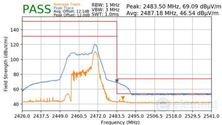
Plot 7-136 Radiated Restricted Upper Band Edge Measurement Antenna 2a (Peak & Average – RU26)
