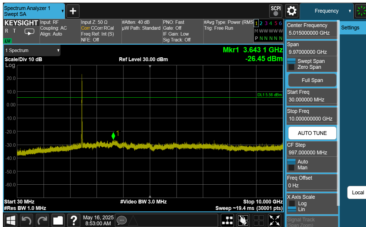
Plot 7-77. Conducted Spurious Plot Antenna 2a (802.11be OFDMA – RU26 – Ch. 11)
