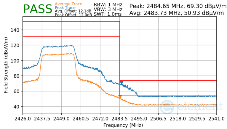
Plot 7-129 Radiated Restricted Upper Band Edge Measurement Antenna 4a (Peak & Average – RU242)
