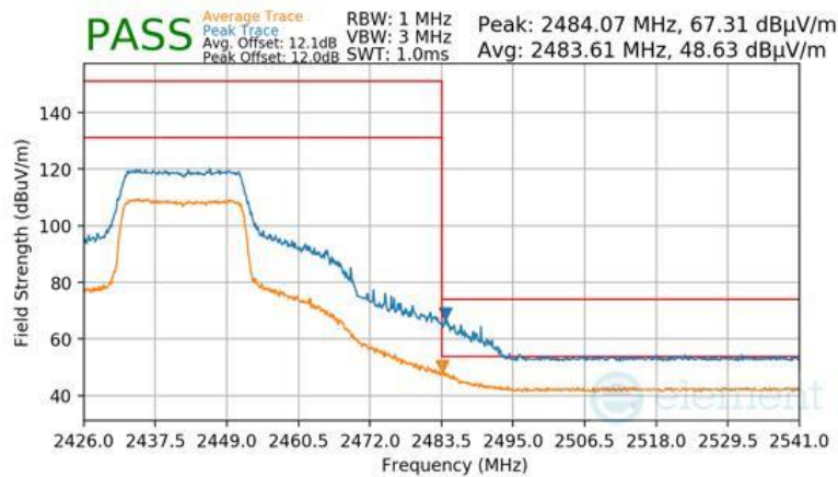
Plot 7-128 Radiated Restricted Upper Band Edge Measurement Antenna 4a (Peak & Average – RU242)
