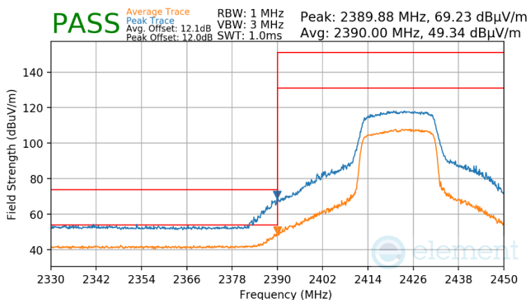
Plot 7-123 Radiated Restricted Lower Band Edge Measurement Antenna 4a (Peak & Average – RU242)
