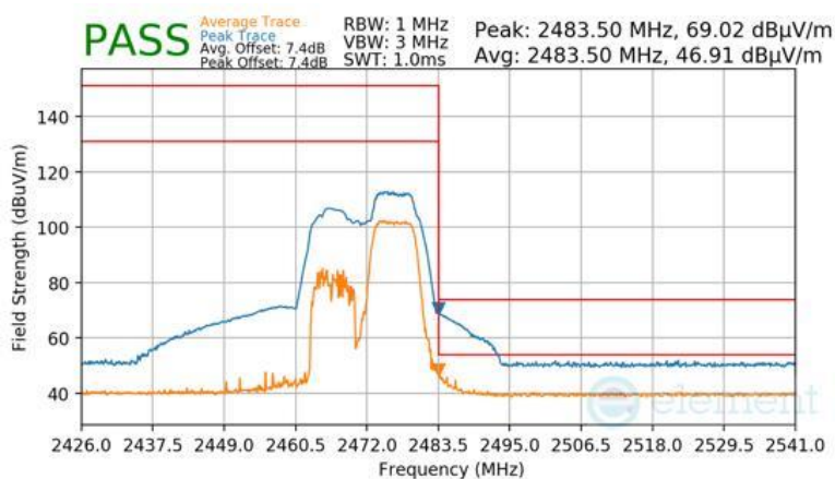
Plot 7-120 Radiated Restricted Upper Band Edge Measurement Antenna 4a (Peak & Average – RU52+26)
