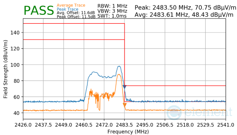
Plot 7-138 Radiated Restricted Upper Band Edge Measurement Antenna 2a (Peak & Average – RU26)
