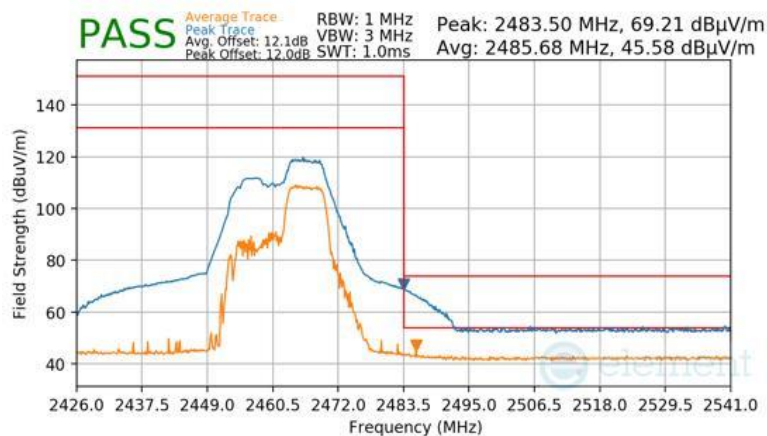
Plot 7-114 Radiated Restricted Upper Band Edge Measurement Antenna 4a (Peak & Average – RU52+26)
