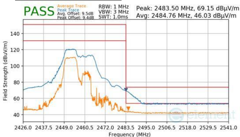
Plot 7-109 Radiated Restricted Upper Band Edge Measurement Antenna 4a (Peak & Average – RU52+26)
