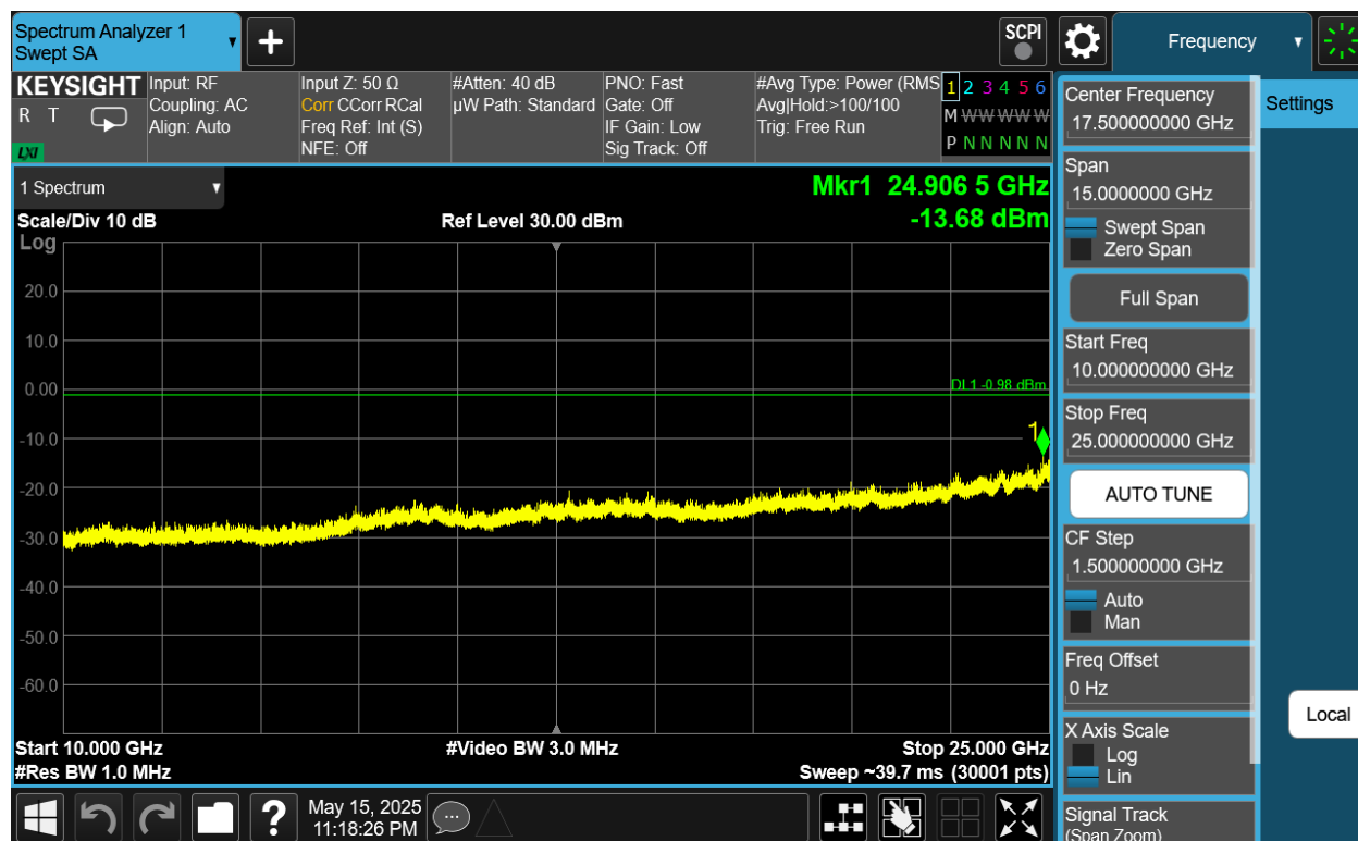
Plot 7-68. Conducted Spurious Plot Antenna 4a (802.11be OFDMA – RU242 – Ch. 1)
