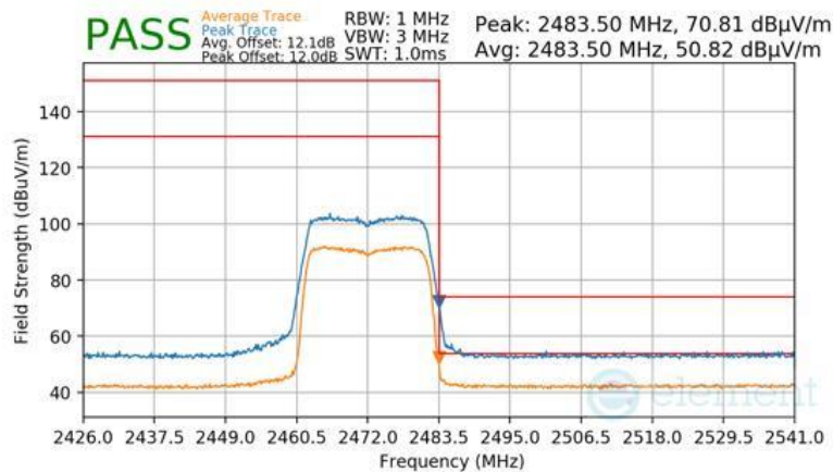
Plot 7-134 Radiated Restricted Upper Band Edge Measurement Antenna 4a (Peak & Average – RU242)
