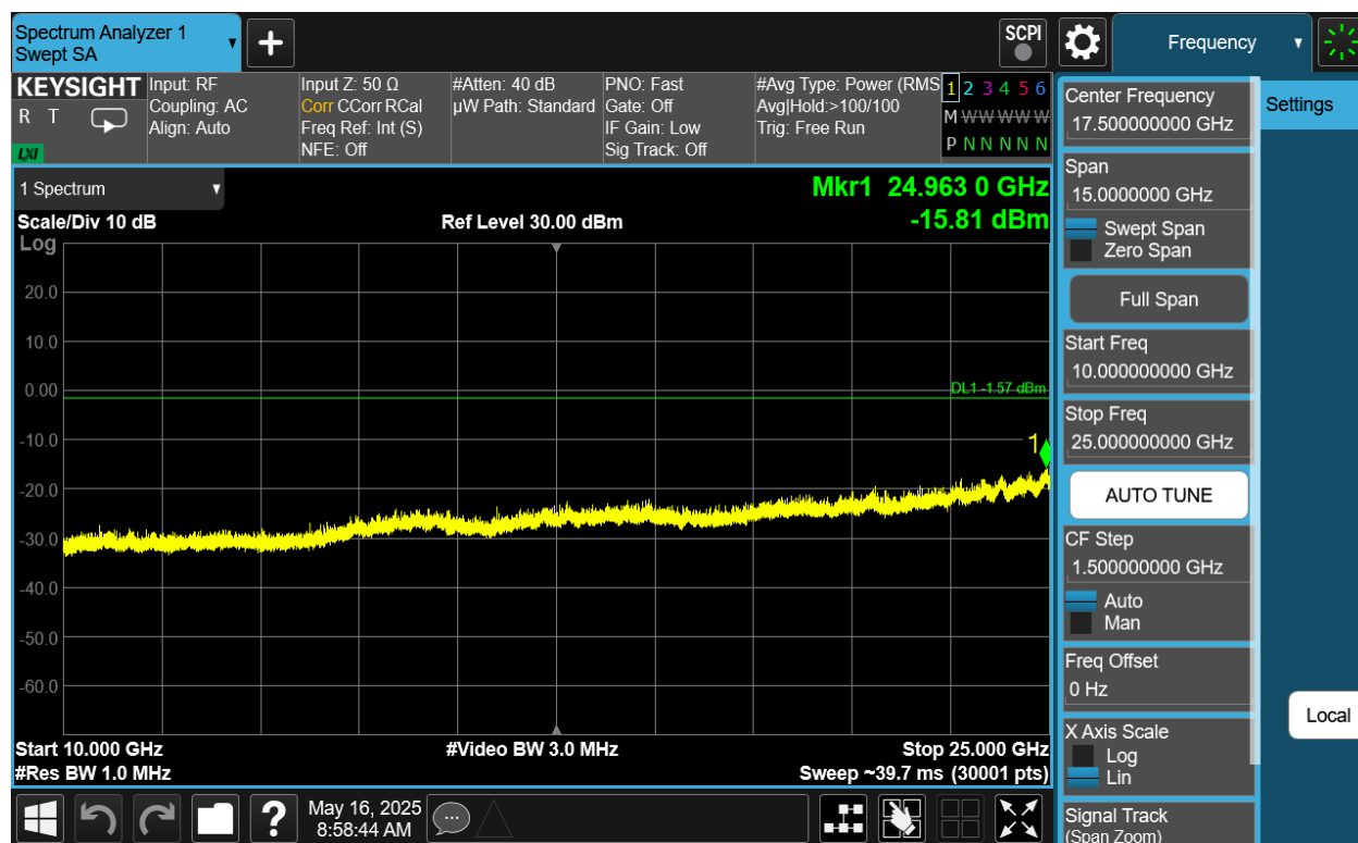
Plot 7-82. Conducted Spurious Plot Antenna 2a (802.11be OFDMA – RU242 – Ch. 6)
