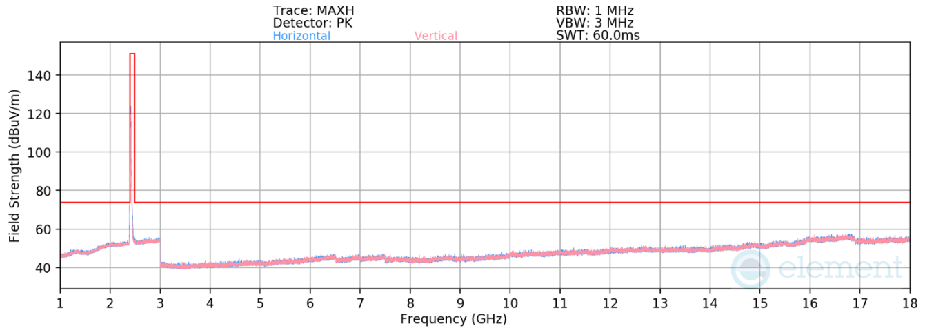
Plot 7-85. Radiated Spurious Emissions above 1GHz CDD (802.11be OFDMA – RU26 – Ch. 1)
