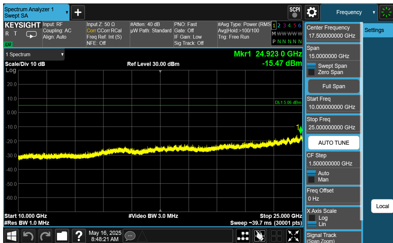
Plot 7-76. Conducted Spurious Plot Antenna 2a (802.11be OFDMA – RU26 – Ch. 6)
