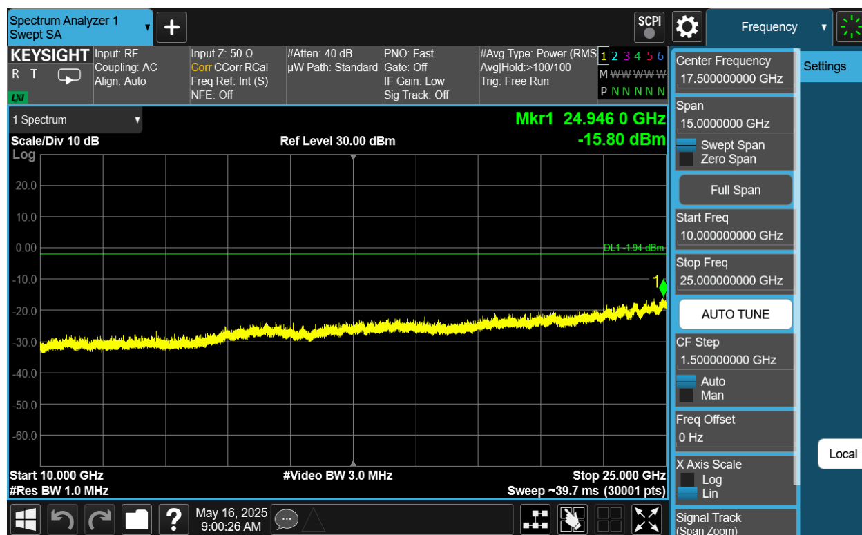
Plot 7-84. Conducted Spurious Plot Antenna 2a (802.11be OFDMA – RU242 – Ch. 11)
