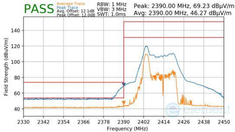
Plot 7-93 Radiated Restricted Lower Band Edge Measurement Antenna 4a (Peak & Average – RU26)
