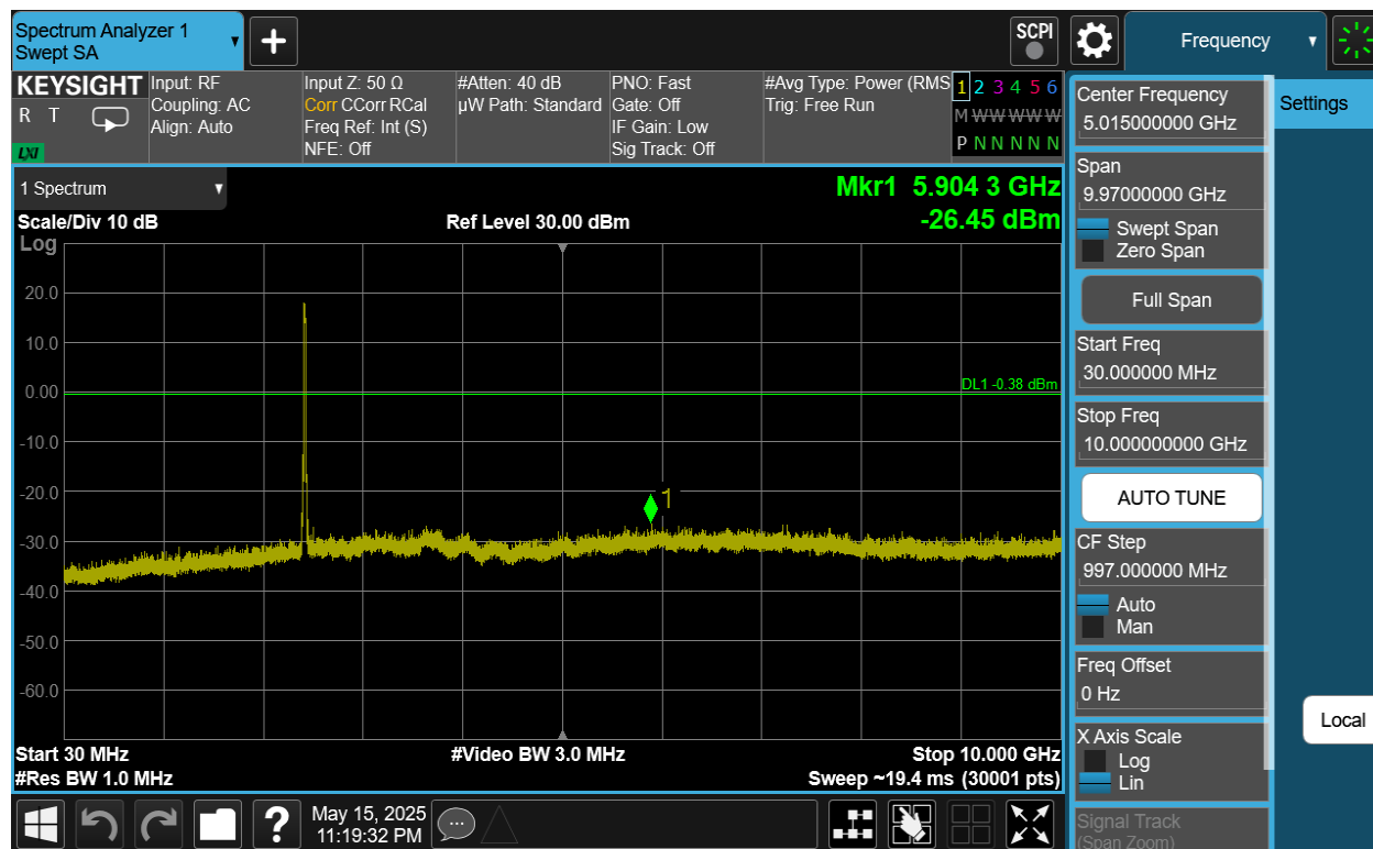
Plot 7-69. Conducted Spurious Plot Antenna 4a (802.11be OFDMA – RU242 – Ch. 6)
