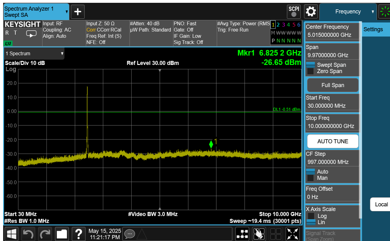
Plot 7-71. Conducted Spurious Plot Antenna 4a (802.11be OFDMA – RU242 – Ch. 11)
