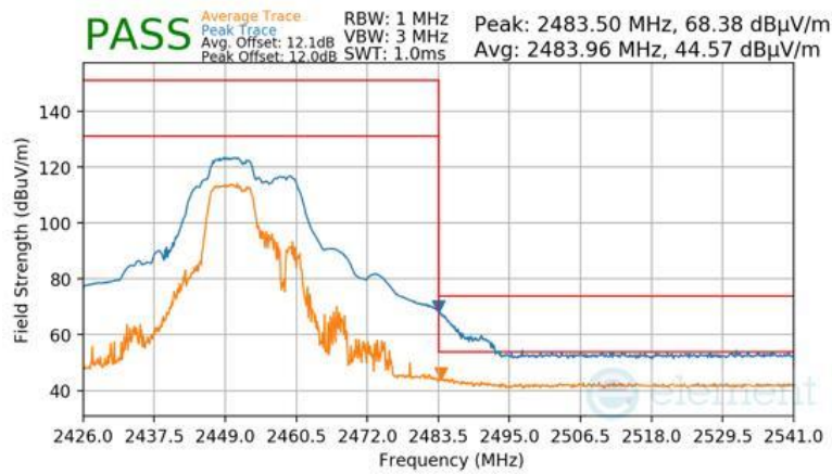
Plot 7-107 Radiated Restricted Upper Band Edge Measurement Antenna 4a (Peak & Average – RU52+26)
