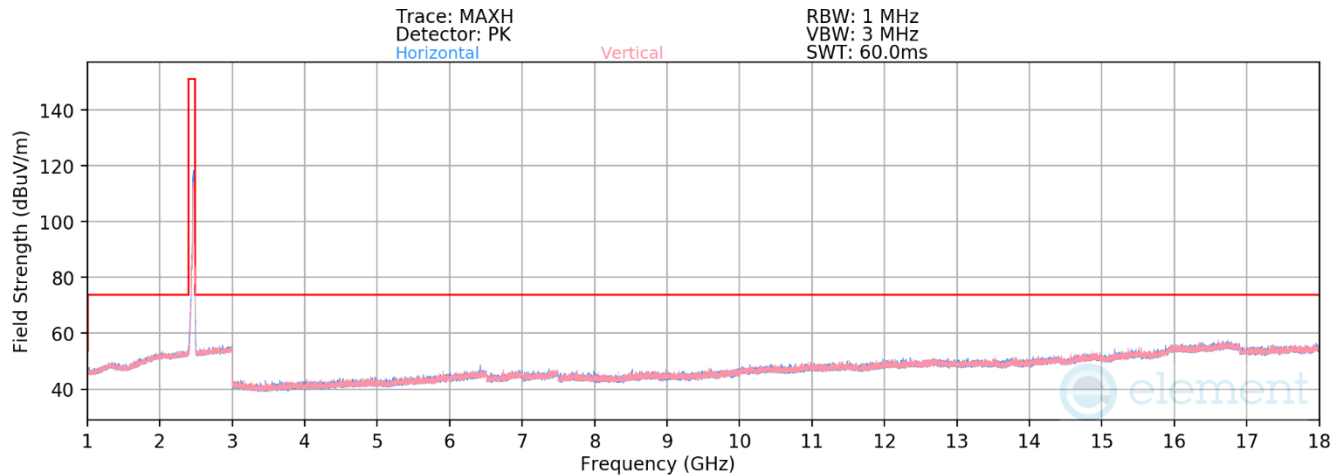
Plot 7-92. Radiated Spurious Emissions above 1GHz CDD (802.11be OFDMA – RU242 – Ch. 11)
