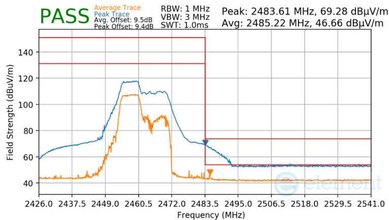
Plot 7-112 Radiated Restricted Upper Band Edge Measurement Antenna 4a (Peak & Average – RU52+26)
