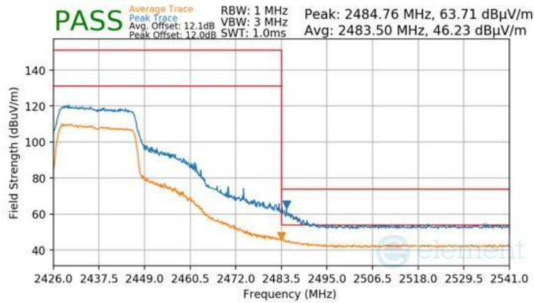
Plot 7-127 Radiated Restricted Upper Band Edge Measurement Antenna 4a (Peak & Average – RU242)
