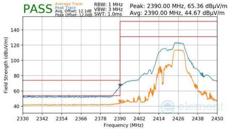
Plot 7-105 Radiated Restricted Lower Band Edge Measurement Antenna 4a (Peak & Average – RU52+26)
