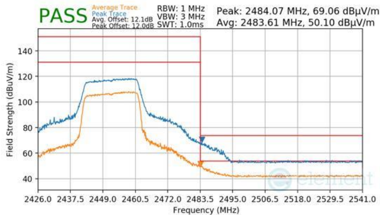
Plot 7-130 Radiated Restricted Upper Band Edge Measurement Antenna 4a (Peak & Average – RU242)
