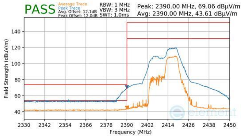
Plot 7-99 Radiated Restricted Lower Band Edge Measurement Antenna 4a (Peak & Average – RU52+26)
