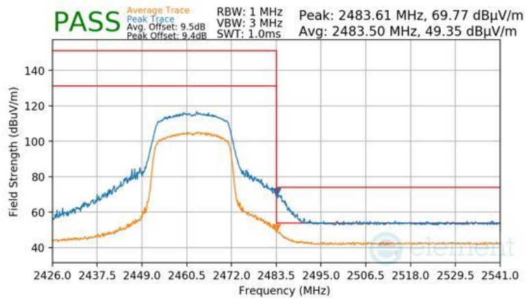
Plot 7-132 Radiated Restricted Upper Band Edge Measurement Antenna 4a (Peak & Average – RU242)
