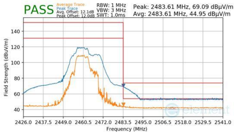
Plot 7-113 Radiated Restricted Upper Band Edge Measurement Antenna 4a (Peak & Average – RU52+26)
