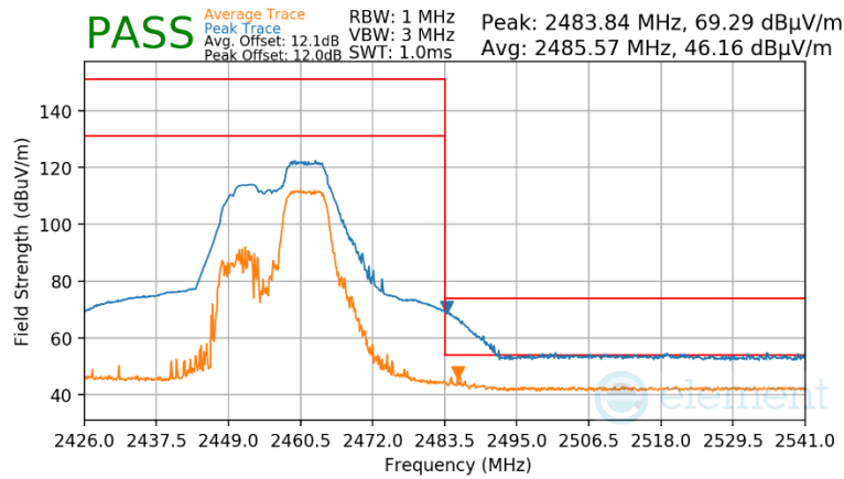
Plot 7-111 Radiated Restricted Upper Band Edge Measurement Antenna 4a (Peak & Average – RU52+26)
