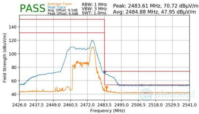
Plot 7-137 Radiated Restricted Upper Band Edge Measurement Antenna 2a (Peak & Average – RU26)
