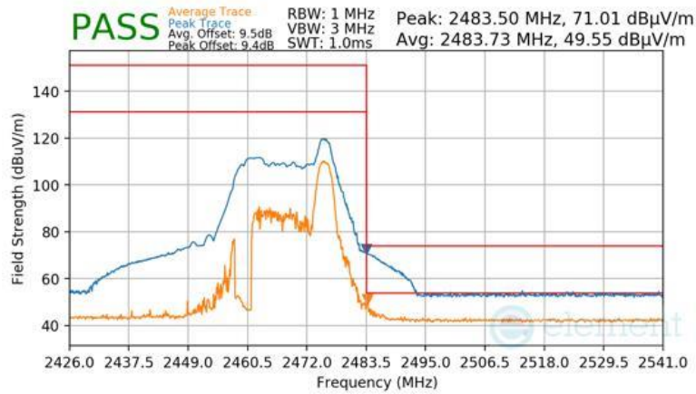
Plot 7-95 Radiated Restricted Upper Band Edge Measurement Antenna 4a (Peak & Average – RU26)
