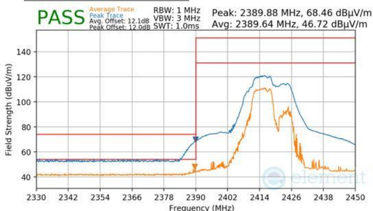
Plot 7-101 Radiated Restricted Lower Band Edge Measurement Antenna 4a (Peak & Average – RU52+26)
