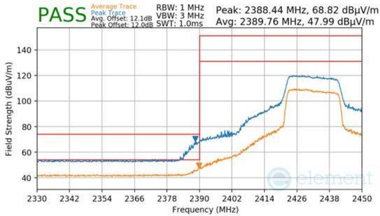
Plot 7-125 Radiated Restricted Lower Band Edge Measurement Antenna 4a (Peak & Average – RU242)
