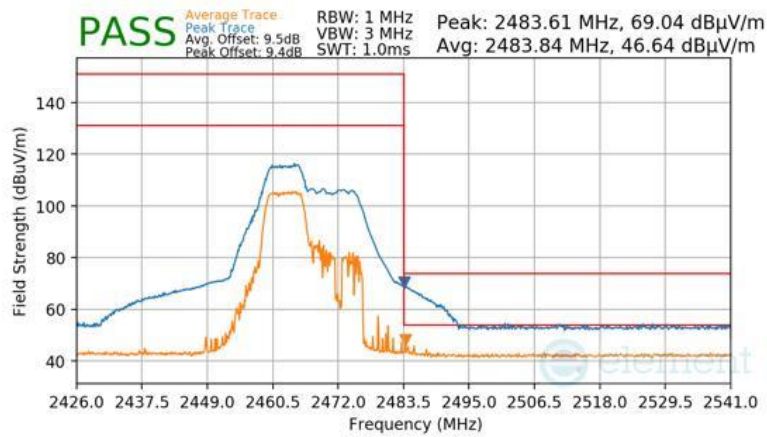
Plot 7-115 Radiated Restricted Upper Band Edge Measurement Antenna 4a (Peak & Average – RU52+26)
