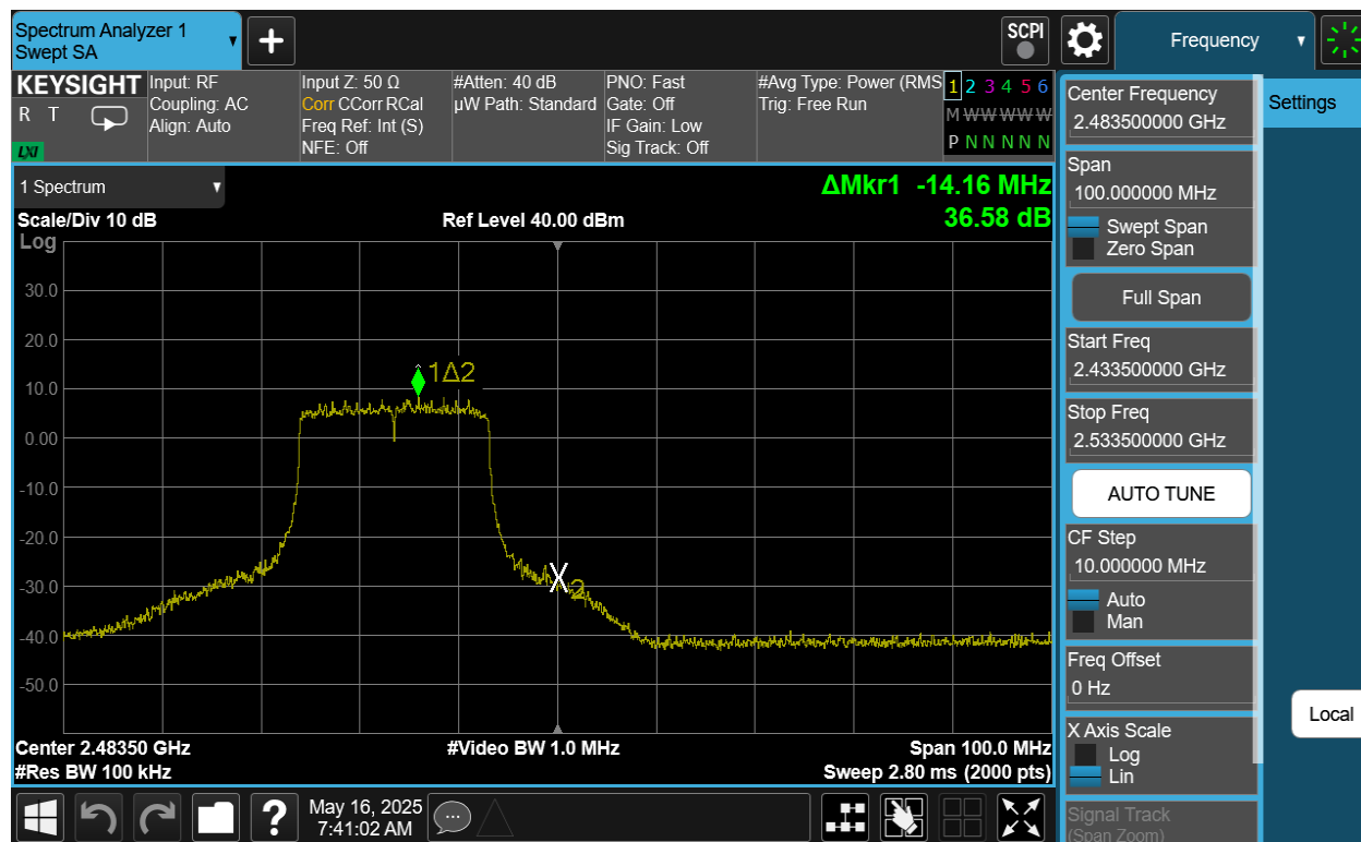
Plot 7-59. Band Edge Antenna 2a (802.11be OFDMA – RU242 – Ch. 12)
