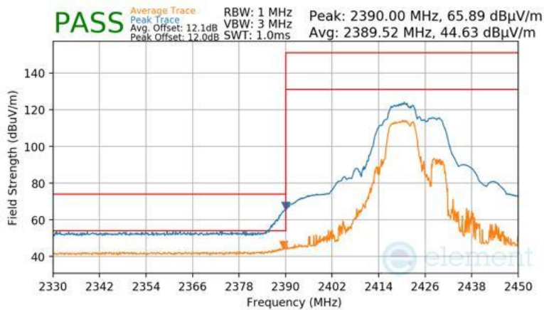
Plot 7-104 Radiated Restricted Lower Band Edge Measurement Antenna 4a (Peak & Average – RU52+26)
