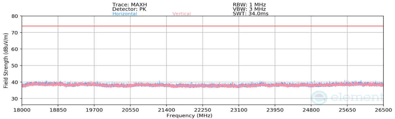
Plot 7-87. Radiated Spurious Emissions above 18GHz CDD (802.11be OFDMA – RU26 – Ch. 6)
