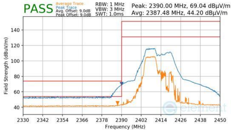
Plot 7-97 Radiated Restricted Lower Band Edge Measurement Antenna 4a (Peak & Average – RU52+26)
