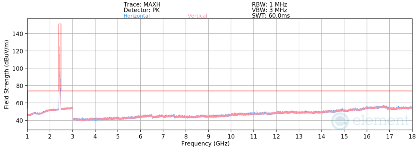
Plot 7-86. Radiated Spurious Emissions above 1GHz CDD (802.11be OFDMA – RU26 – Ch. 6)
