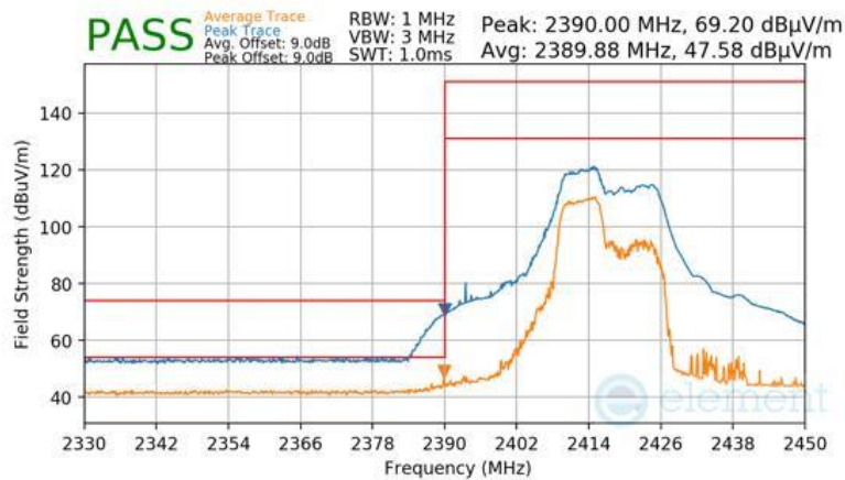
Plot 7-100 Radiated Restricted Lower Band Edge Measurement Antenna 4a (Peak & Average – RU52+26)
