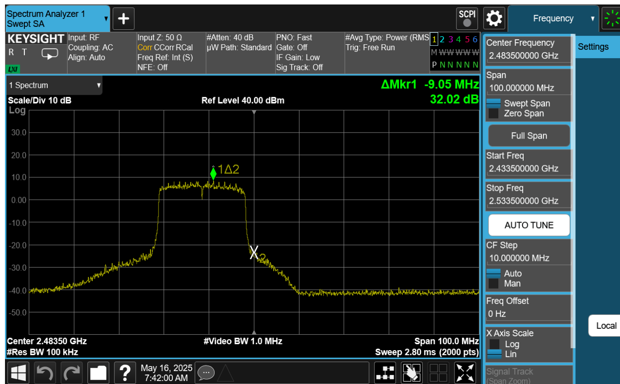
Plot 7-60. Band Edge Antenna 2a (802.11be OFDMA – RU242 – Ch. 13)
