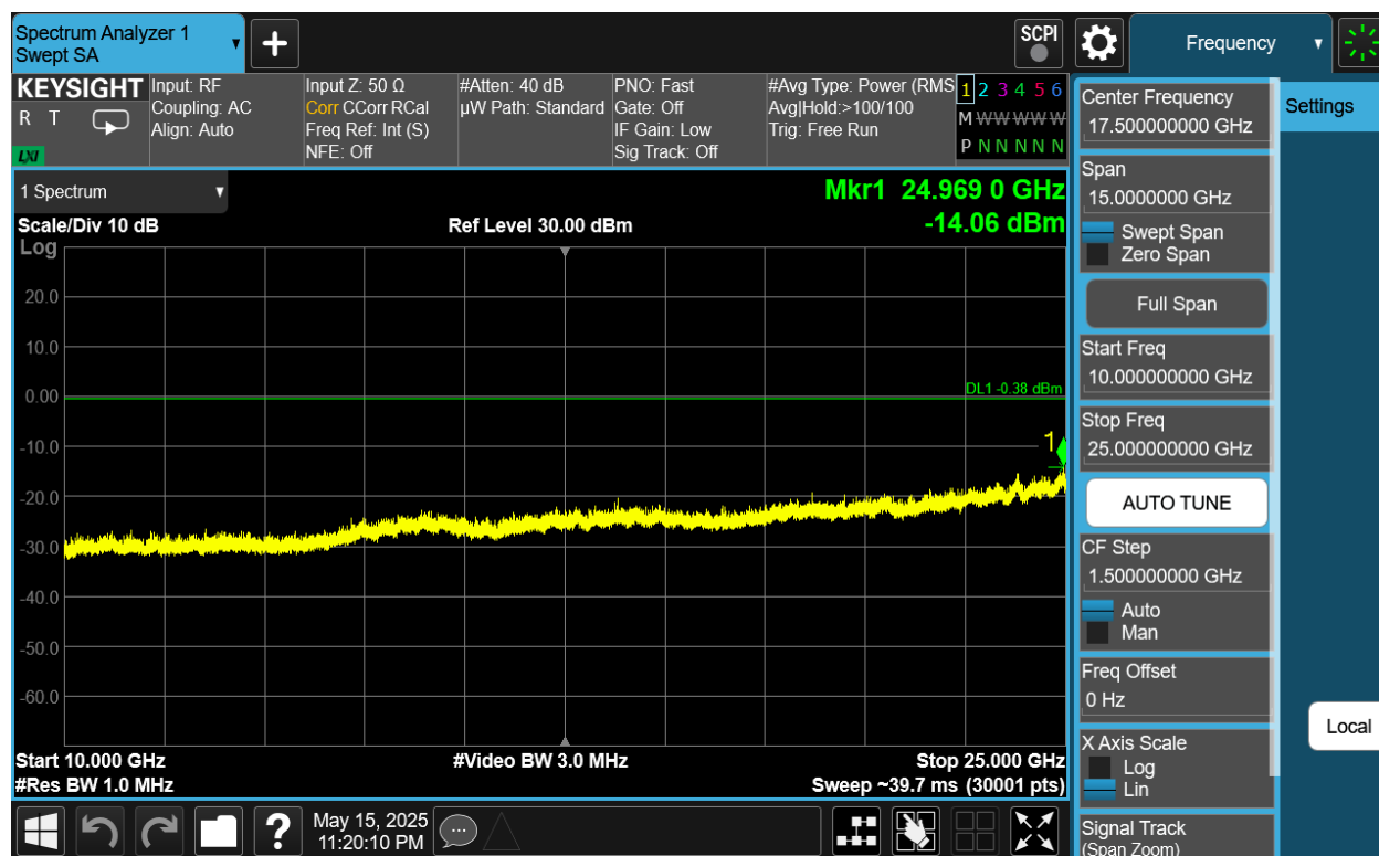
Plot 7-70. Conducted Spurious Plot Antenna 4a (802.11be OFDMA – RU242 – Ch. 6)
