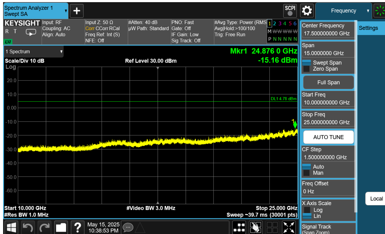
Plot 7-62. Conducted Spurious Plot Antenna 4a (802.11be OFDMA – RU26 – Ch. 1)
