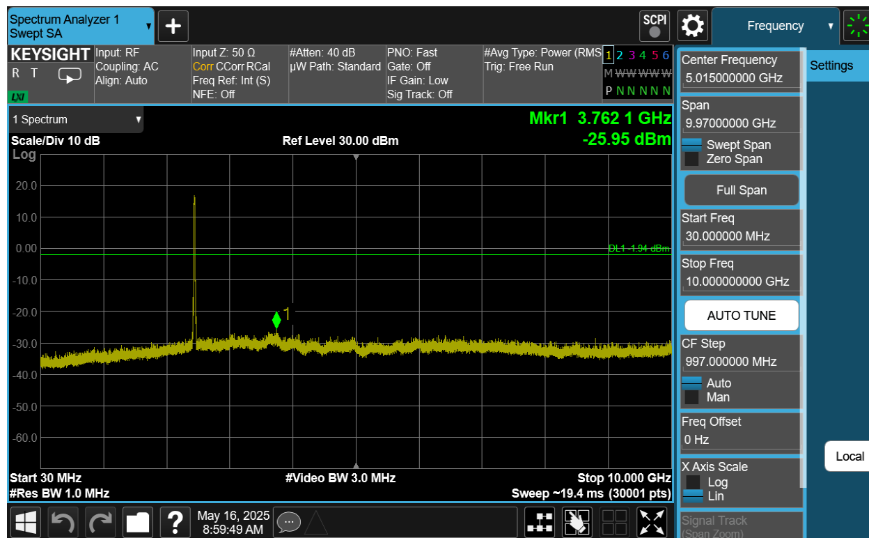
Plot 7-83. Conducted Spurious Plot Antenna 2a (802.11be OFDMA – RU242 – Ch. 11)
