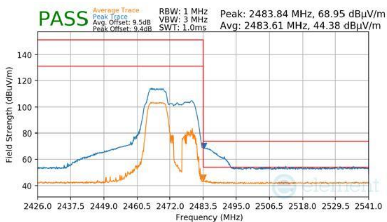
Plot 7-118 Radiated Restricted Upper Band Edge Measurement Antenna 4a (Peak & Average – RU52+26)
