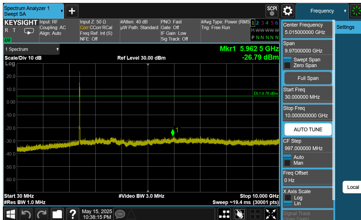
Plot 7-61. Conducted Spurious Plot Antenna 4a (802.11be OFDMA – RU26 – Ch. 1)
