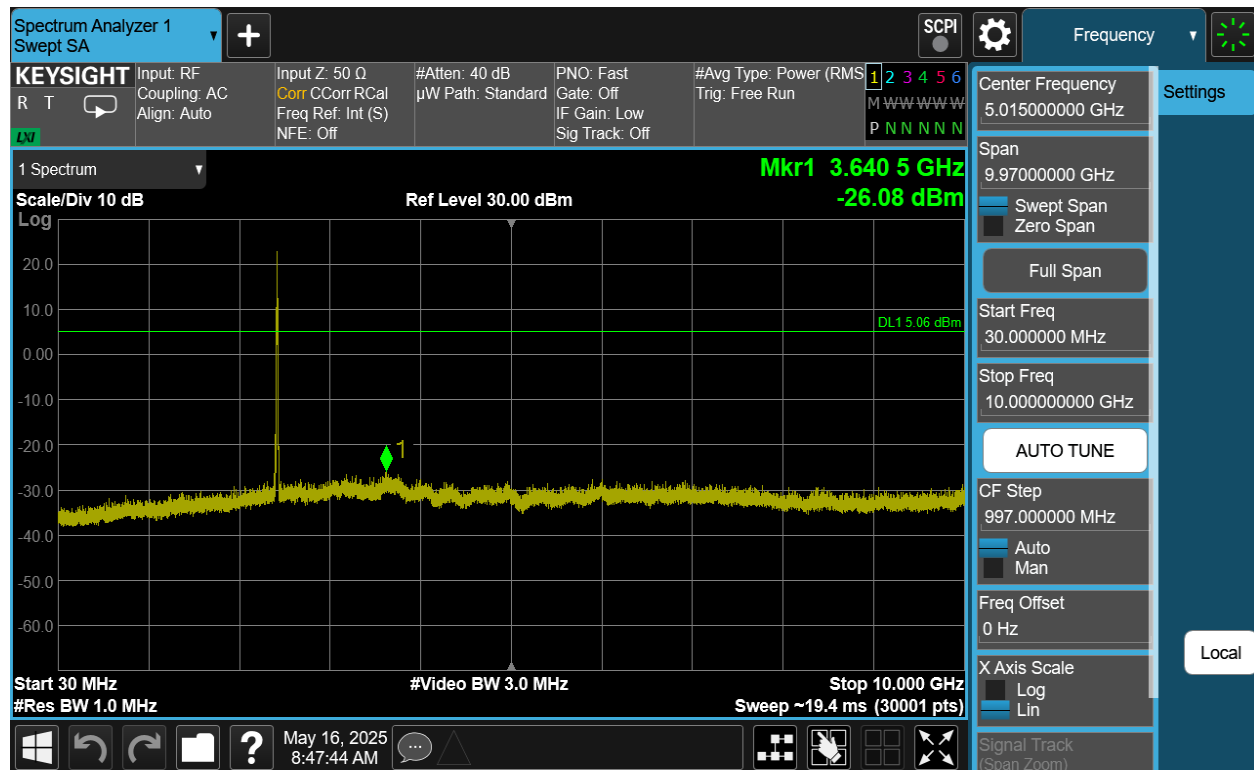
Plot 7-75. Conducted Spurious Plot Antenna 2a (802.11be OFDMA – RU26 – Ch. 6)
