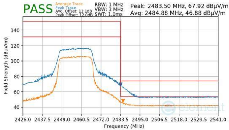
Plot 7-131 Radiated Restricted Upper Band Edge Measurement Antenna 4a (Peak & Average – RU242)
