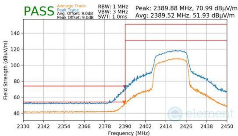
Plot 7-122 Radiated Restricted Lower Band Edge Measurement Antenna 4a (Peak & Average – RU242)
