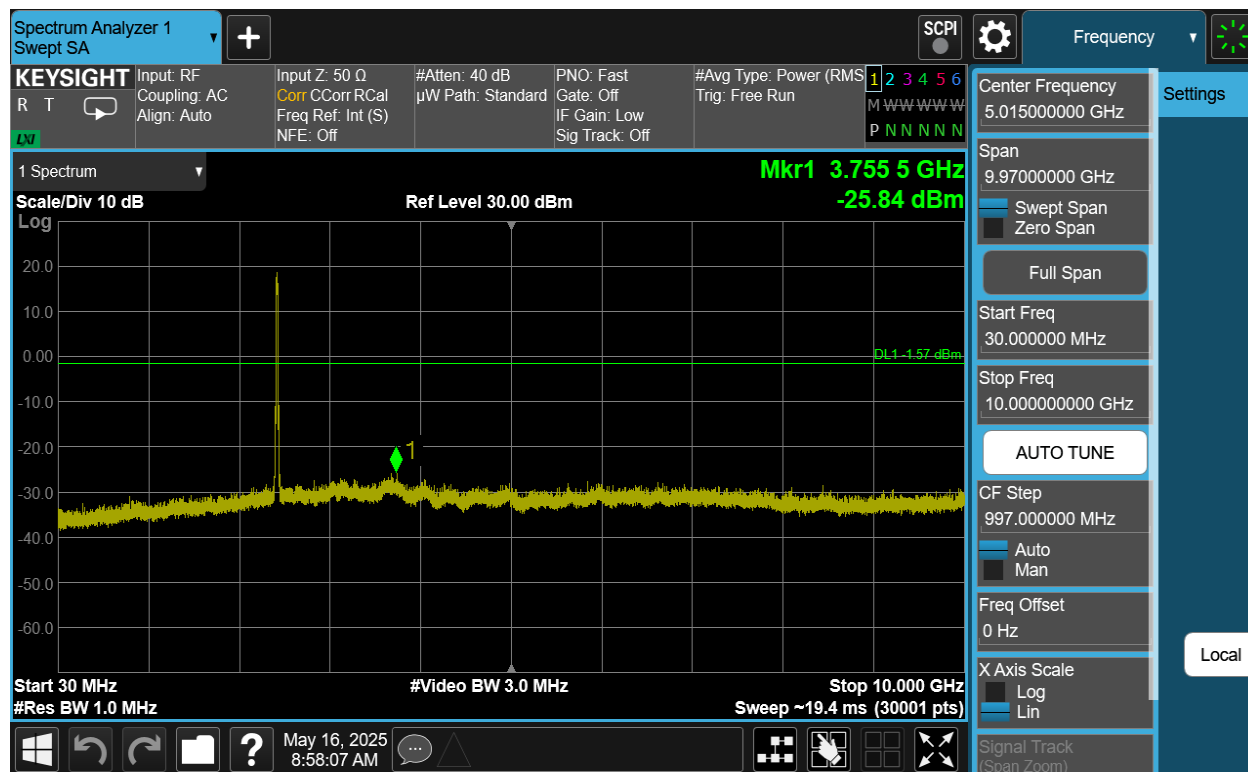
Plot 7-81. Conducted Spurious Plot Antenna 2a (802.11be OFDMA – RU242 – Ch. 6)
