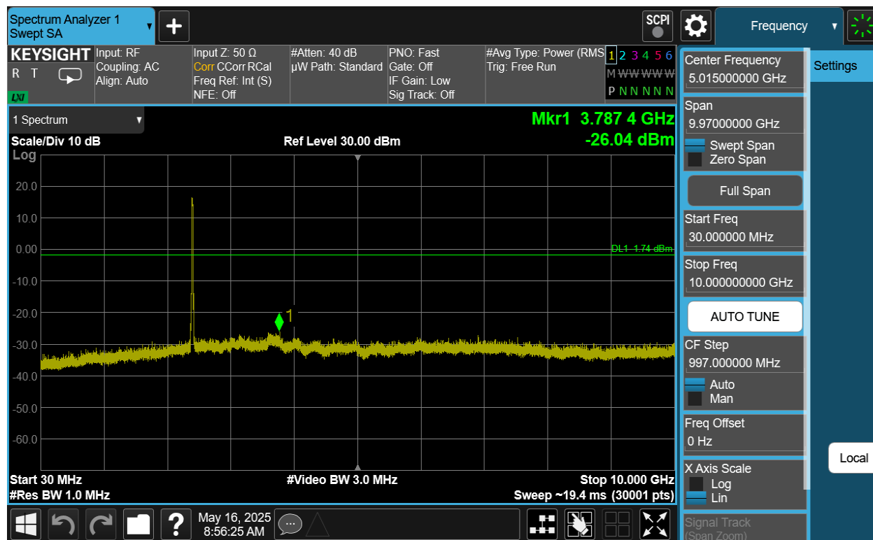
Plot 7-79. Conducted Spurious Plot Antenna 2a (802.11be OFDMA – RU242 – Ch. 1)
