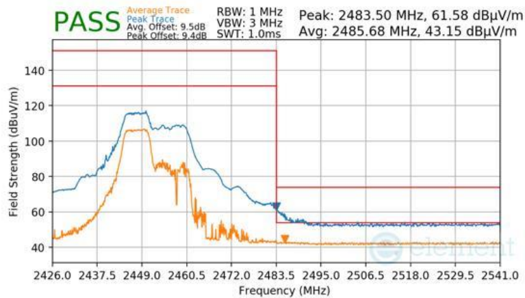
Plot 7-106 Radiated Restricted Upper Band Edge Measurement Antenna 4a (Peak & Average – RU52+26)
