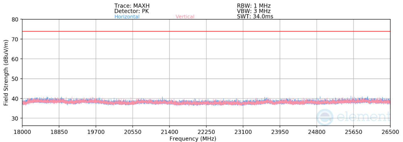
Plot 7-91. Radiated Spurious Emissions above 18GHz CDD (802.11be OFDMA – RU242 – Ch. 6)
