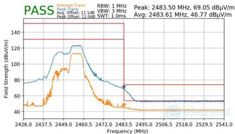
Plot 7-108 Radiated Restricted Upper Band Edge Measurement Antenna 4a (Peak & Average – RU52+26)
