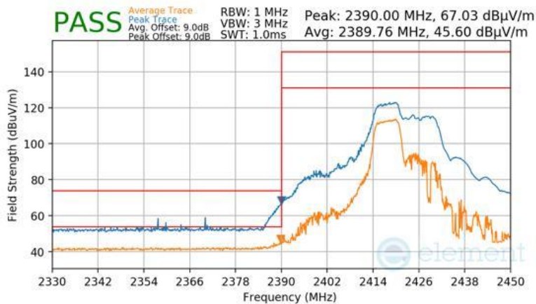
Plot 7-103 Radiated Restricted Lower Band Edge Measurement Antenna 4a (Peak & Average – RU52+26)
