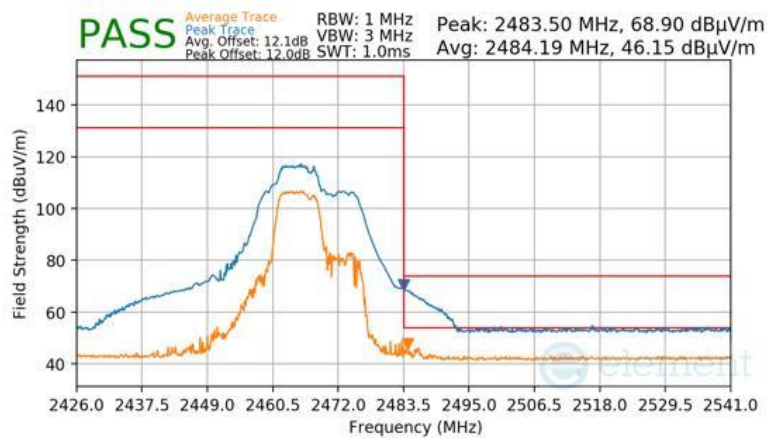
Plot 7-116 Radiated Restricted Upper Band Edge Measurement Antenna 4a (Peak & Average – RU52+26)
