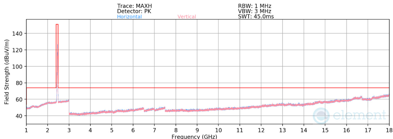
Plot 7-88. Radiated Spurious Emissions above 1GHz CDD (802.11be OFDMA – RU26 – Ch. 11)
