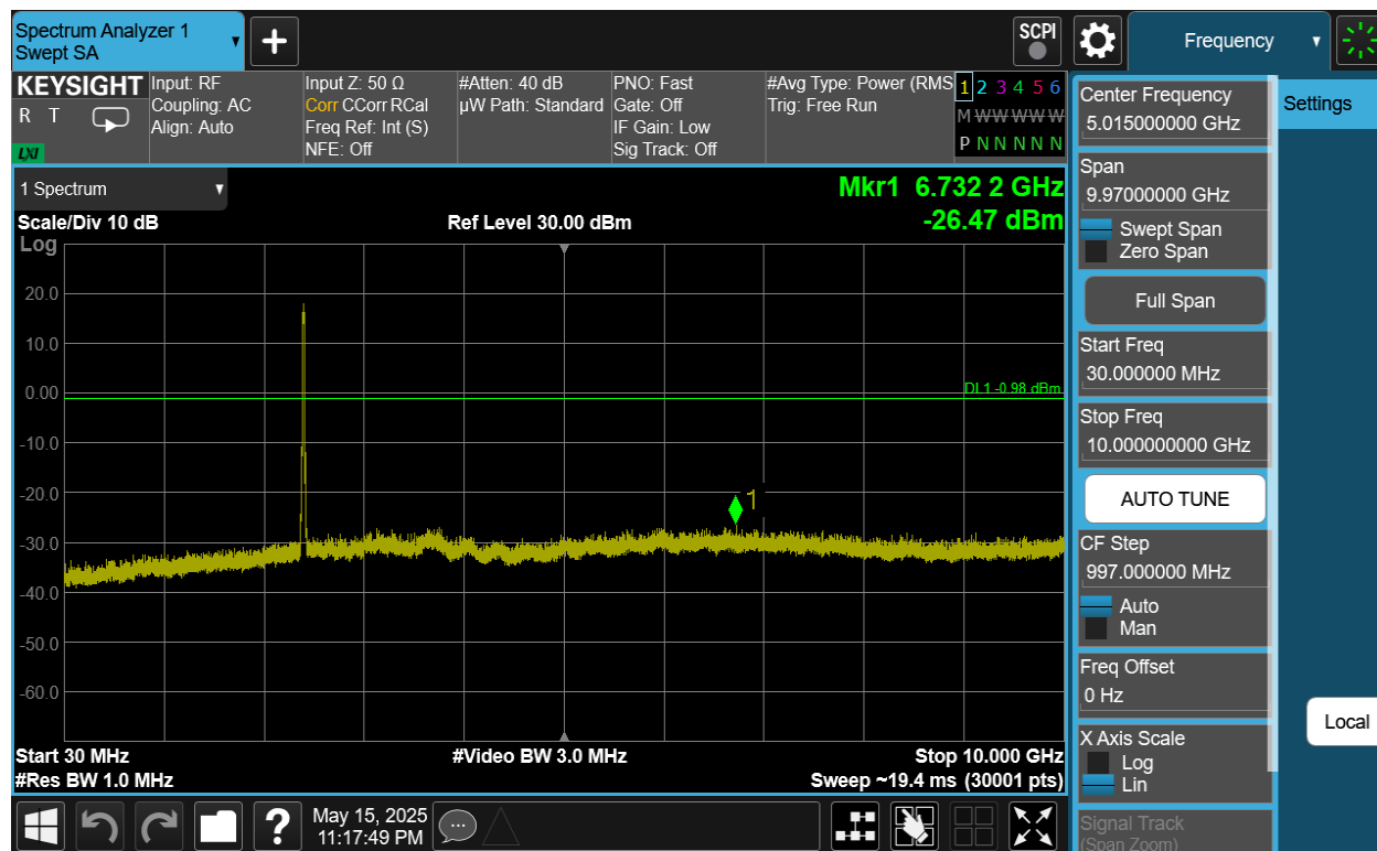
Plot 7-67. Conducted Spurious Plot Antenna 4a (802.11be OFDMA – RU242 – Ch. 1)
