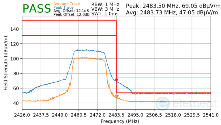
Plot 7-133 Radiated Restricted Upper Band Edge Measurement Antenna 4a (Peak & Average – RU242)
