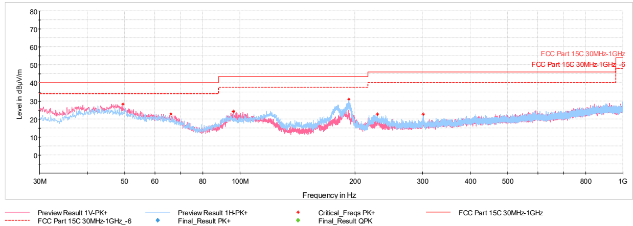
Plot 7-214. Radiated Spurious Emissions Below 1GHz CDD Ch.6 (RU26), with AC/DC Adapter
