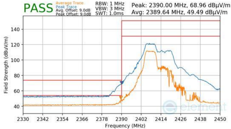
Plot 7-139 Radiated Restricted Lower Band Edge Measurement Antenna 2a (Peak & Average – RU52+26)
