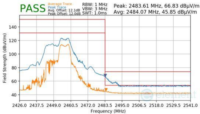
Plot 7-188 Radiated Restricted Upper Band Edge Measurement CDD (Peak & Average – RU52+26)
