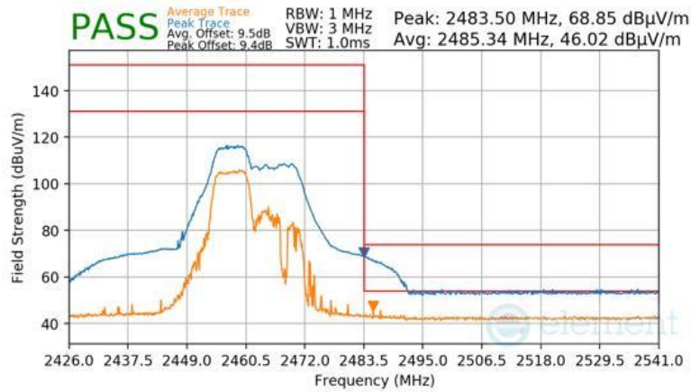
Plot 7-151 Radiated Restricted Upper Band Edge Measurement Antenna 2a (Peak & Average – RU52+26)
