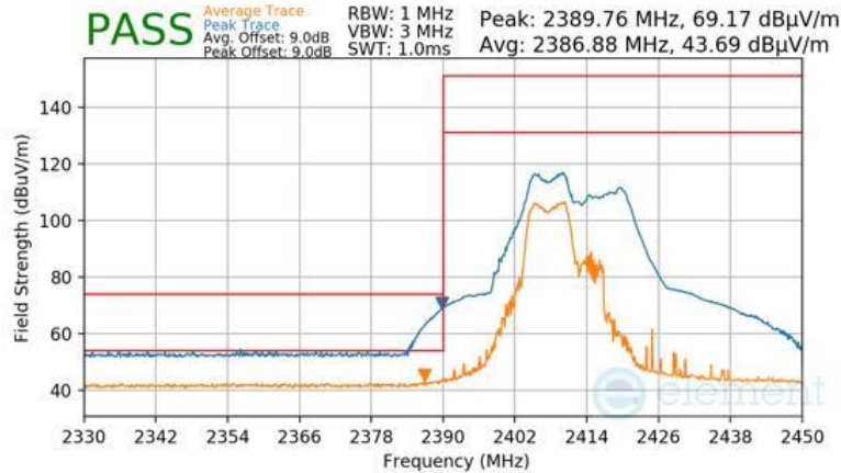
Plot 7-177 Radiated Restricted Lower Band Edge Measurement CDD (Peak & Average – RU52+26)
