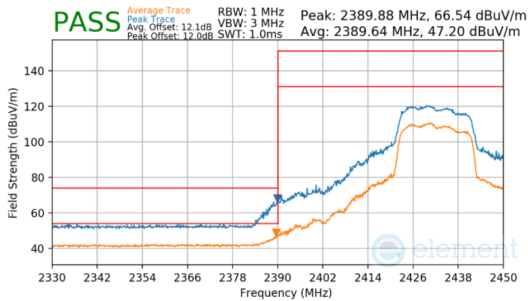
Plot 7-205 Radiated Restricted Lower Band Edge Measurement CDD (Peak & Average – RU242)
