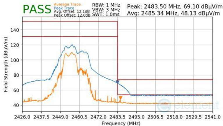
Plot 7-190 Radiated Restricted Upper Band Edge Measurement CDD (Peak & Average – RU52+26)
