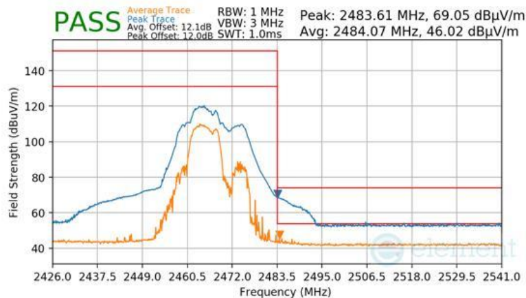
Plot 7-196 Radiated Restricted Upper Band Edge Measurement CDD (Peak & Average – RU52+26)
