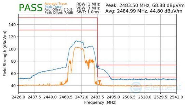
Plot 7-158 Radiated Restricted Upper Band Edge Measurement Antenna 2a (Peak & Average – RU52+26)
