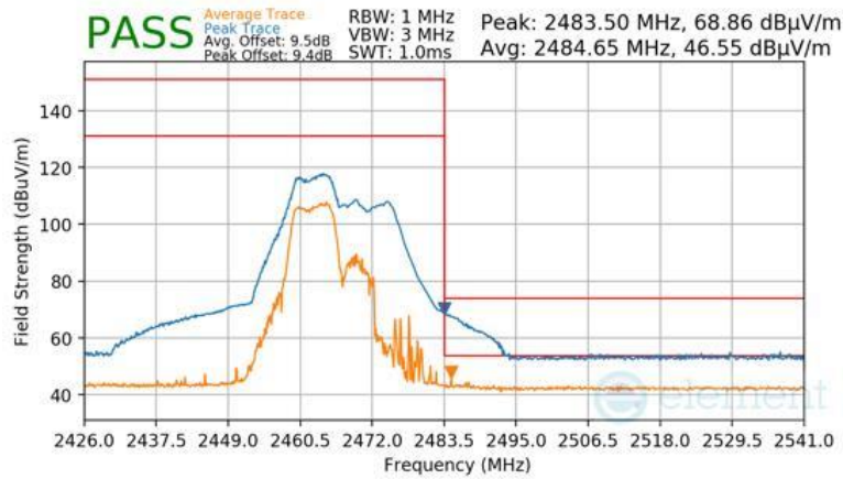
Plot 7-195 Radiated Restricted Upper Band Edge Measurement CDD (Peak & Average – RU52+26)
