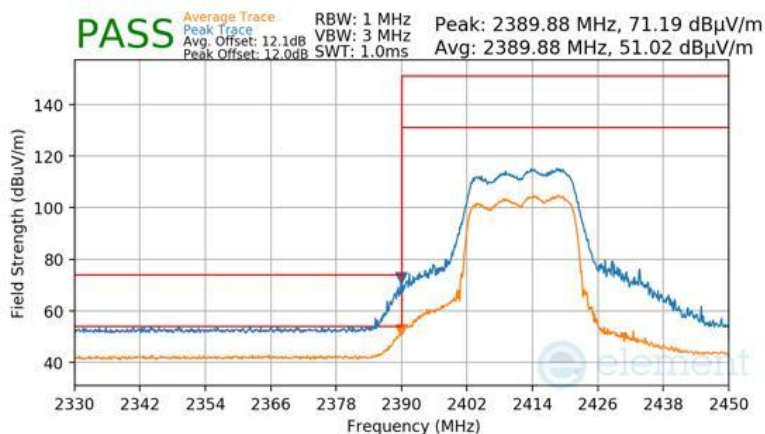
Plot 7-201 Radiated Restricted Lower Band Edge Measurement CDD (Peak & Average – RU242)
