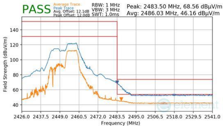
Plot 7-147 Radiated Restricted Upper Band Edge Measurement Antenna 2a (Peak & Average – RU52+26)
