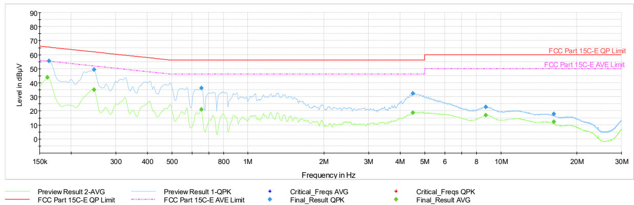
Plot 7-222. AC Line Conducted Emissions with 802.11be CDD (RU242) Ch.6 (N, with AC/DC Adapter)
