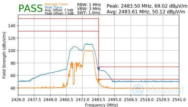
Plot 7-159 Radiated Restricted Upper Band Edge Measurement Antenna 2a (Peak & Average – RU52+26)
