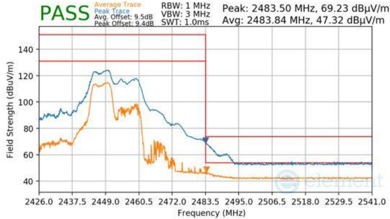
Plot 7-186 Radiated Restricted Upper Band Edge Measurement CDD (Peak & Average – RU52+26)
