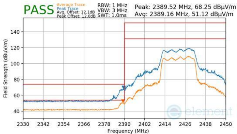
Plot 7-203 Radiated Restricted Lower Band Edge Measurement CDD (Peak & Average – RU242)
