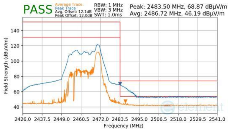
Plot 7-174 Radiated Restricted Upper Band Edge Measurement CDD (Peak & Average – RU26)
