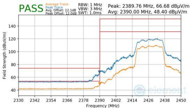
Plot 7-204 Radiated Restricted Lower Band Edge Measurement CDD (Peak & Average – RU242)
