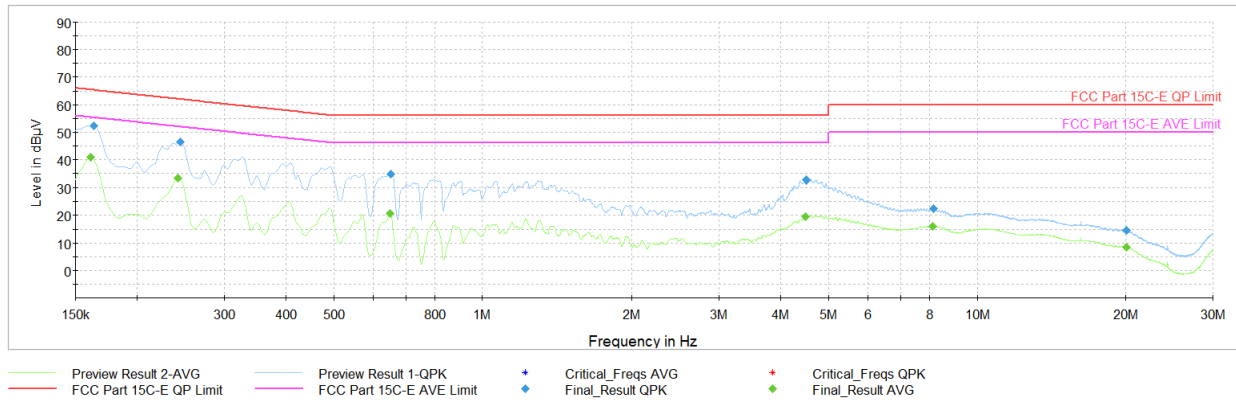
Plot 7-220. AC Line Conducted Emissions with 802.11be CDD (RU78) Ch.6 (N, with AC/DC Adapter)
