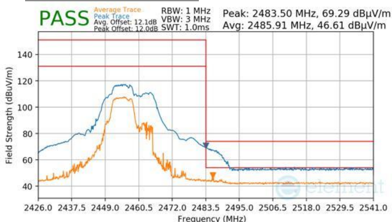
Plot 7-149 Radiated Restricted Upper Band Edge Measurement Antenna 2a (Peak & Average – RU52+26)
