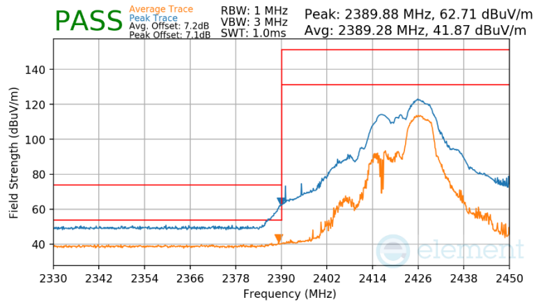
Plot 7-185 Radiated Restricted Lower Band Edge Measurement CDD (Peak & Average – RU52+26)
