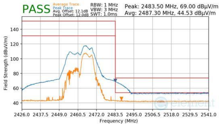
Plot 7-194 Radiated Restricted Upper Band Edge Measurement CDD (Peak & Average – RU52+26)
