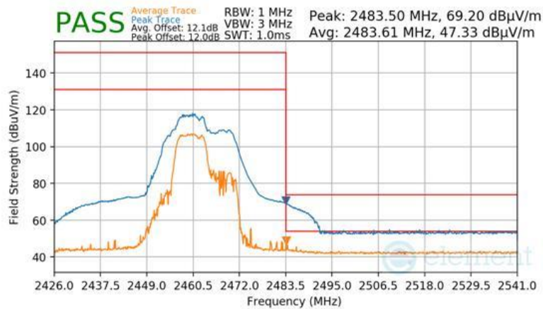
Plot 7-152 Radiated Restricted Upper Band Edge Measurement Antenna 2a (Peak & Average – RU52+26)
