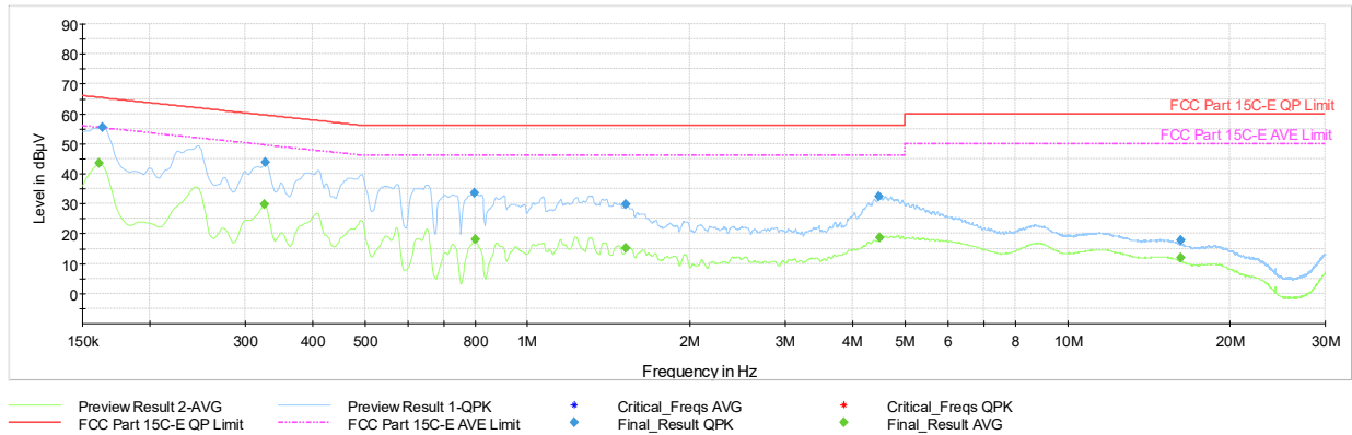
Plot 7-217. AC Line Conducted Emissions with 802.11be CDD (RU26) Ch.6 (L1, with AC/DC Adapter)
