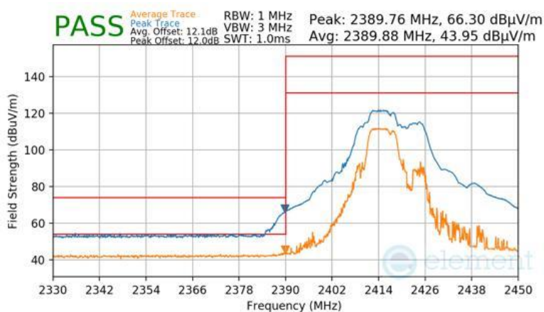
Plot 7-142 Radiated Restricted Lower Band Edge Measurement Antenna 2a (Peak & Average – RU52+26)
