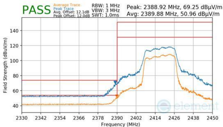
Plot 7-202 Radiated Restricted Lower Band Edge Measurement CDD (Peak & Average – RU242)
