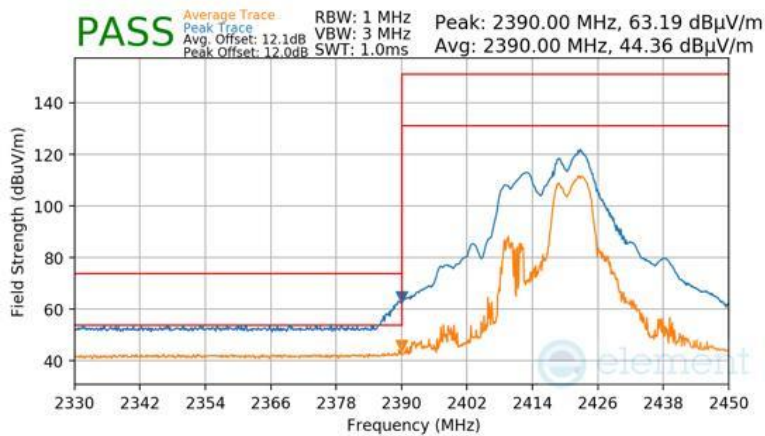
Plot 7-182 Radiated Restricted Lower Band Edge Measurement CDD (Peak & Average – RU52+26)
