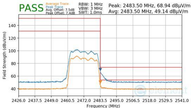
Plot 7-213 Radiated Restricted Upper Band Edge Measurement CDD (Peak & Average – RU242)
