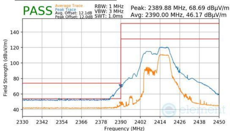
Plot 7-141 Radiated Restricted Lower Band Edge Measurement Antenna 2a (Peak & Average – RU52+26)
