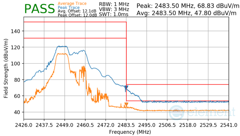
Plot 7-145 Radiated Restricted Upper Band Edge Measurement Antenna 2a (Peak & Average – RU52+26)
