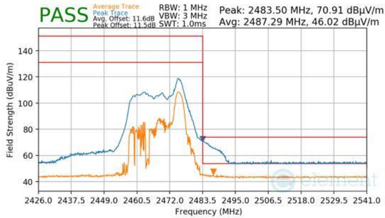
Plot 7-175 Radiated Restricted Upper Band Edge Measurement CDD (Peak & Average – RU26)
