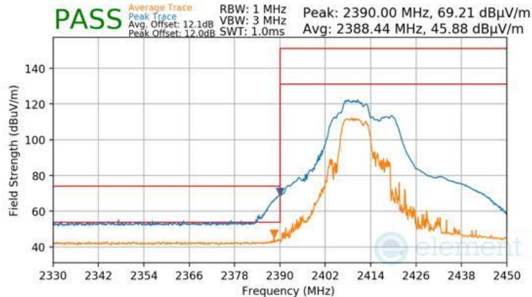
Plot 7-140 Radiated Restricted Lower Band Edge Measurement Antenna 2a (Peak & Average – RU52+26)
