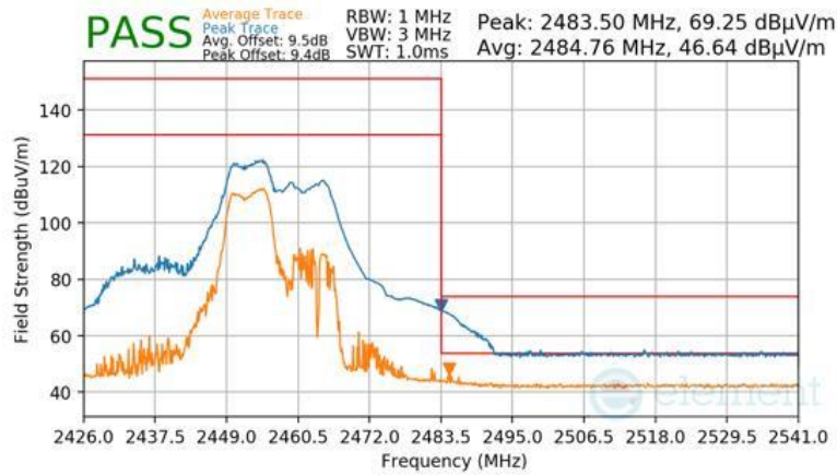
Plot 7-189 Radiated Restricted Upper Band Edge Measurement CDD (Peak & Average – RU52+26)
