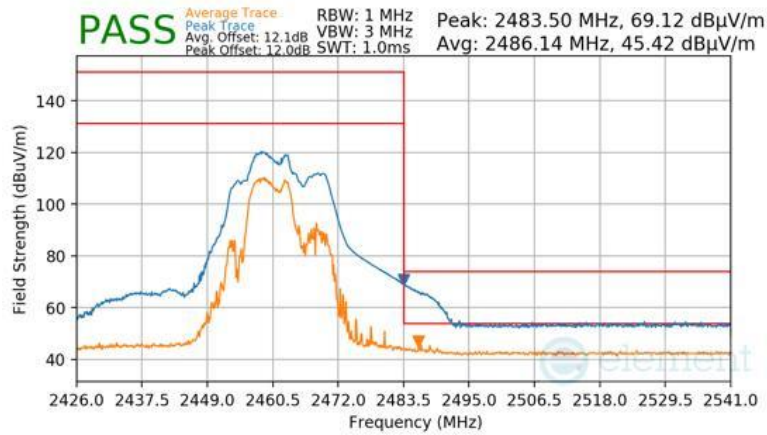
Plot 7-193 Radiated Restricted Upper Band Edge Measurement CDD (Peak & Average – RU52+26)
