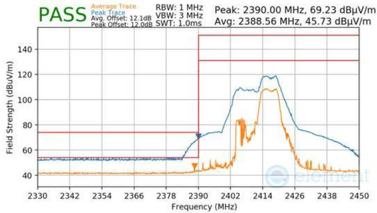
Plot 7-179 Radiated Restricted Lower Band Edge Measurement CDD (Peak & Average – RU52+26)
