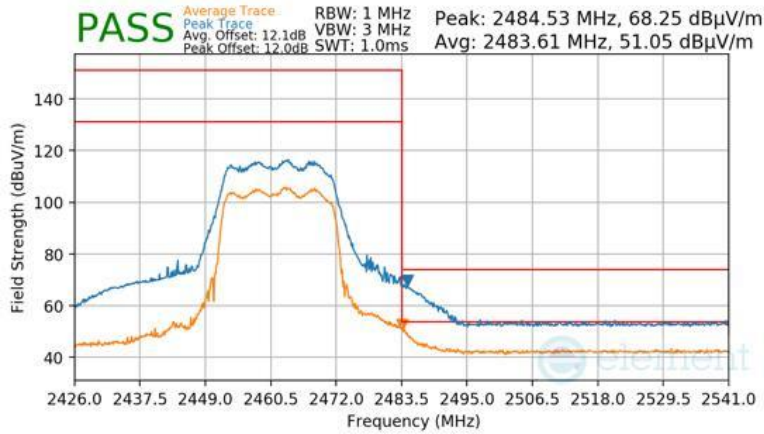
Plot 7-211 Radiated Restricted Upper Band Edge Measurement CDD (Peak & Average – RU242)
