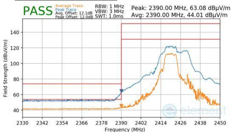
Plot 7-143 Radiated Restricted Lower Band Edge Measurement Antenna 2a (Peak & Average – RU52+26)
