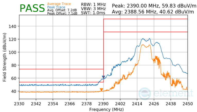
Plot 7-184 Radiated Restricted Lower Band Edge Measurement CDD (Peak & Average – RU52+26)
