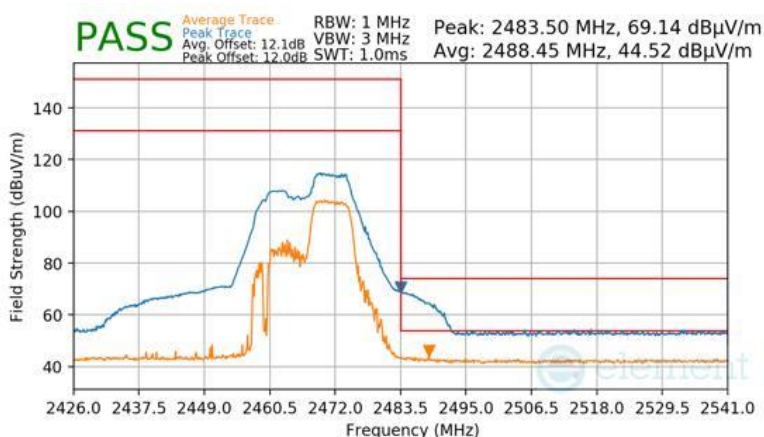
Plot 7-156 Radiated Restricted Upper Band Edge Measurement Antenna 2a (Peak & Average – RU52+26)
