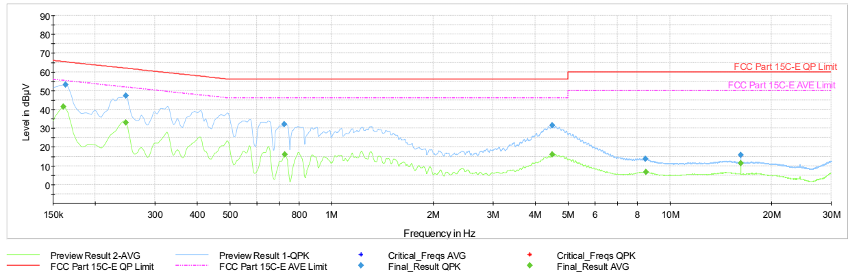
Plot 7-221. AC Line Conducted Emissions with 802.11be CDD (RU242) Ch.6 (L1, with AC/DC Adapter)
