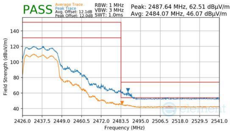
Plot 7-206 Radiated Restricted Upper Band Edge Measurement CDD (Peak & Average – RU242)
