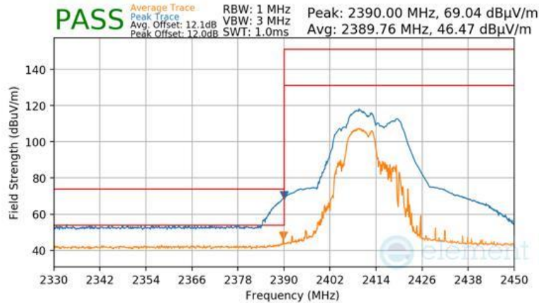
Plot 7-178 Radiated Restricted Lower Band Edge Measurement CDD (Peak & Average – RU52+26)
