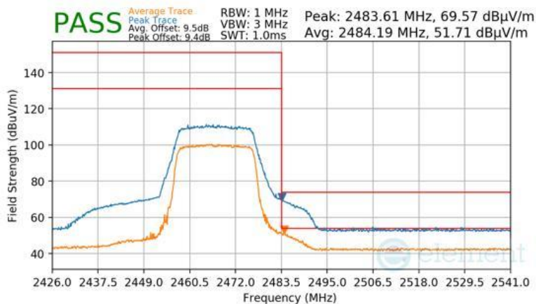
Plot 7-171 Radiated Restricted Upper Band Edge Measurement Antenna 2a (Peak & Average – RU242)
