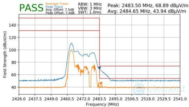
Plot 7-176 Radiated Restricted Upper Band Edge Measurement CDD (Peak & Average – RU26)
