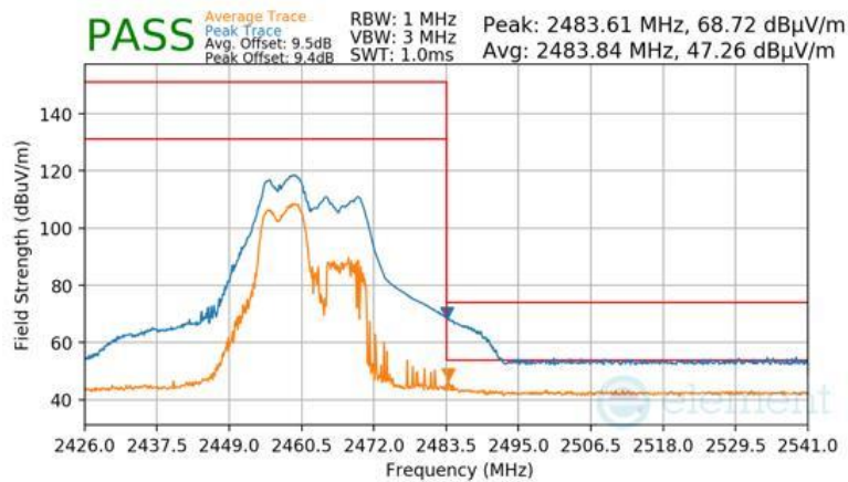
Plot 7-192 Radiated Restricted Upper Band Edge Measurement CDD (Peak & Average – RU52+26)
