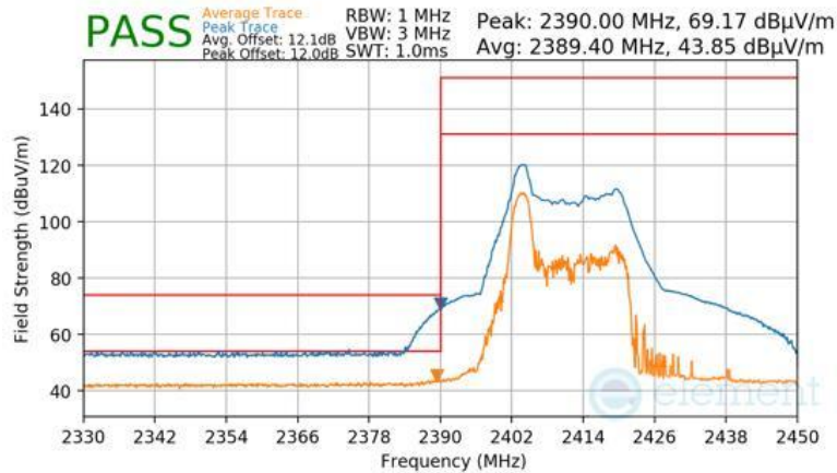
Plot 7-173 Radiated Restricted Lower Band Edge Measurement CDD (Peak & Average – RU26)
