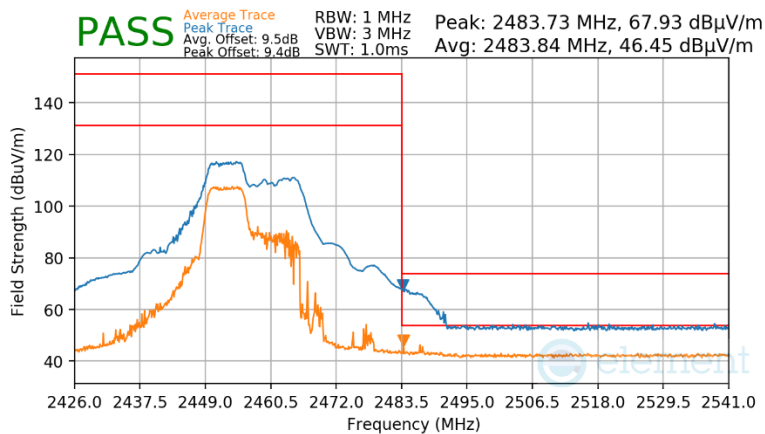
Plot 7-148 Radiated Restricted Upper Band Edge Measurement Antenna 2a (Peak & Average – RU52+26)
