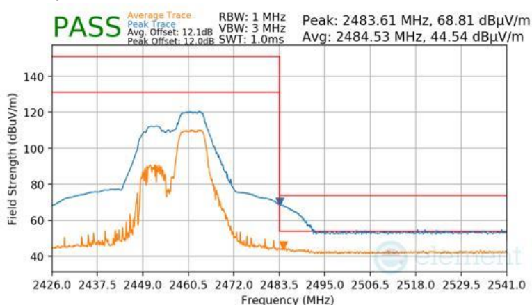
Plot 7-150 Radiated Restricted Upper Band Edge Measurement Antenna 2a (Peak & Average – RU52+26)
