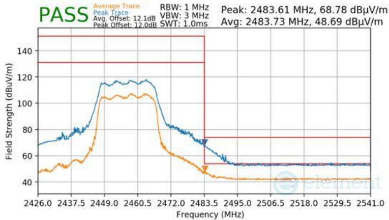
Plot 7-210 Radiated Restricted Upper Band Edge Measurement CDD (Peak & Average – RU242)
