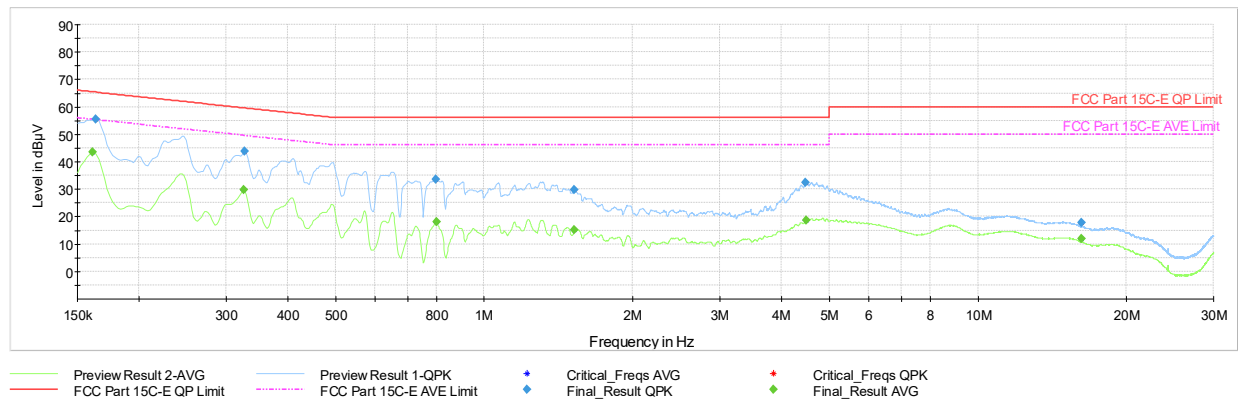
Plot 7-218. AC Line Conducted Emissions with 802.11be CDD (RU26) Ch.6 (N, with AC/DC Adapter)
