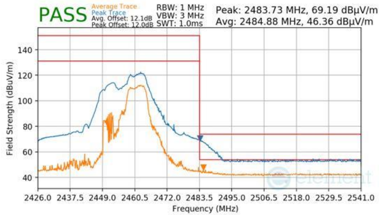
Plot 7-191 Radiated Restricted Upper Band Edge Measurement CDD (Peak & Average – RU52+26)
