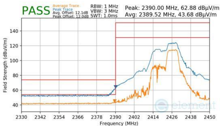
Plot 7-144 Radiated Restricted Lower Band Edge Measurement Antenna 2a (Peak & Average – RU52+26)
