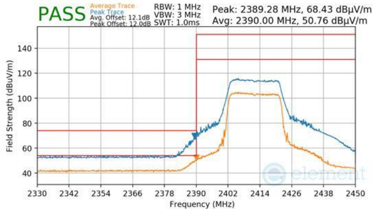
Plot 7-160 Radiated Restricted Lower Band Edge Measurement Antenna 2a (Peak & Average – RU242)
