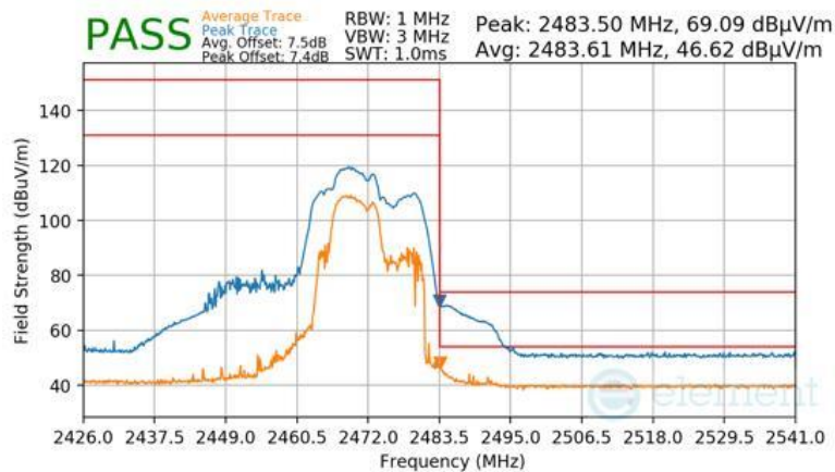
Plot 7-199 Radiated Restricted Upper Band Edge Measurement CDD (Peak & Average – RU52+26)
