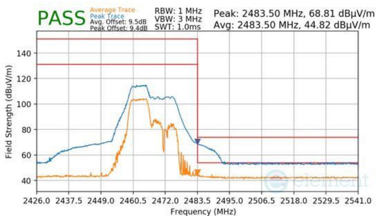
Plot 7-154 Radiated Restricted Upper Band Edge Measurement Antenna 2a (Peak & Average – RU52+26)
