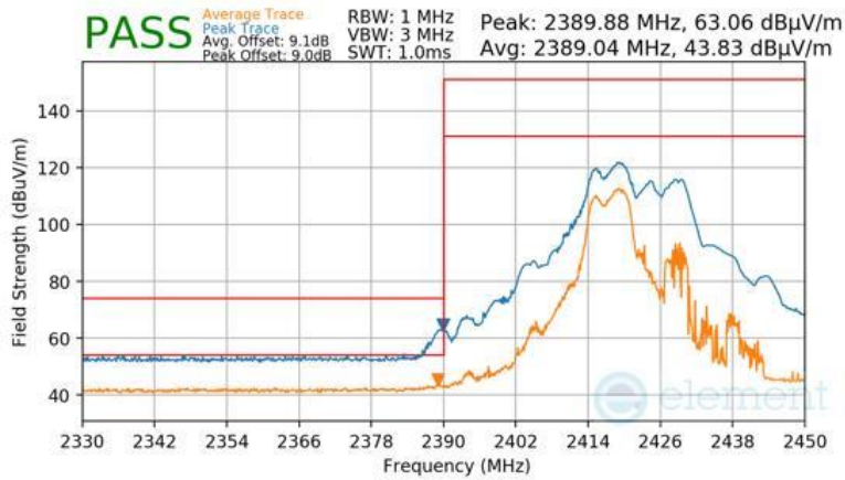
Plot 7-183 Radiated Restricted Lower Band Edge Measurement CDD (Peak & Average – RU52+26)
