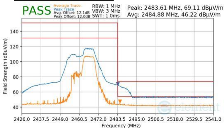
Plot 7-153 Radiated Restricted Upper Band Edge Measurement Antenna 2a (Peak & Average – RU52+26)
