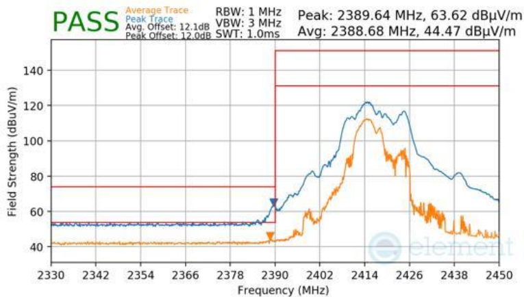
Plot 7-181 Radiated Restricted Lower Band Edge Measurement CDD (Peak & Average – RU52+26)
