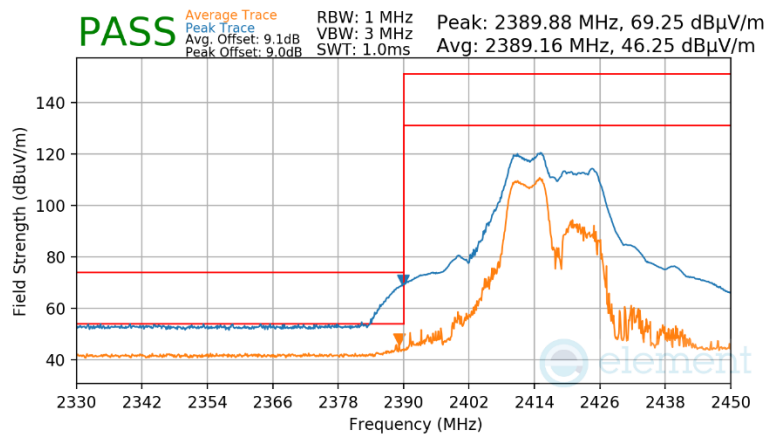
Plot 7-180 Radiated Restricted Lower Band Edge Measurement CDD (Peak & Average – RU52+26)
