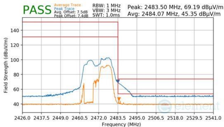
Plot 7-200 Radiated Restricted Upper Band Edge Measurement CDD (Peak & Average – RU52+26)
