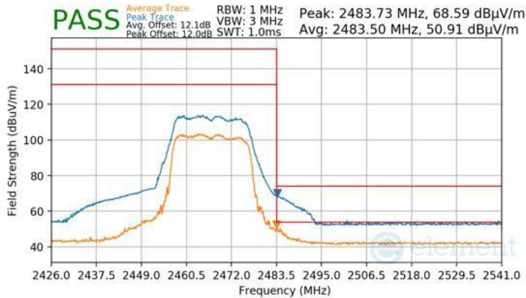
Plot 7-212 Radiated Restricted Upper Band Edge Measurement CDD (Peak & Average – RU242)
