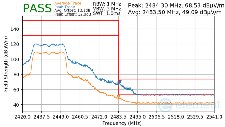
Plot 7-207 Radiated Restricted Upper Band Edge Measurement CDD (Peak & Average – RU242)
