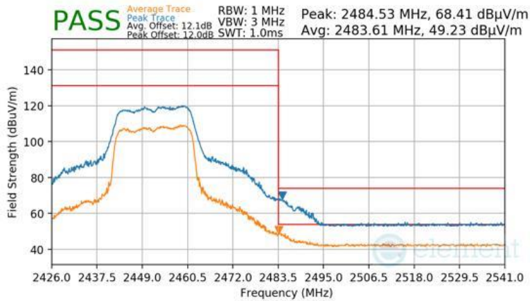
Plot 7-209 Radiated Restricted Upper Band Edge Measurement CDD (Peak & Average – RU242)
