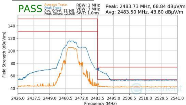
Plot 7-155 Radiated Restricted Upper Band Edge Measurement Antenna 2a (Peak & Average – RU52+26)
