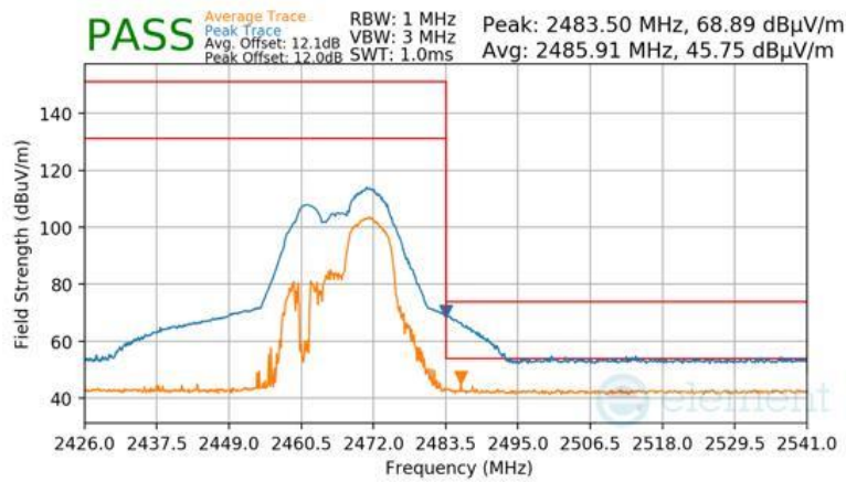
Plot 7-197 Radiated Restricted Upper Band Edge Measurement CDD (Peak & Average – RU52+26)
