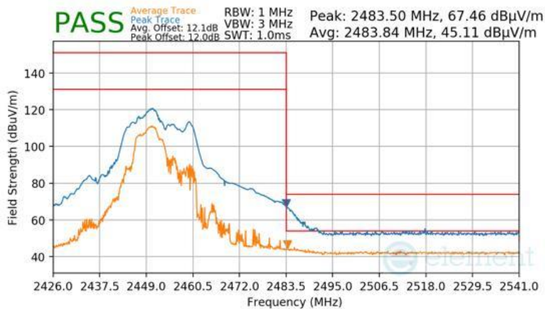
Plot 7-187 Radiated Restricted Upper Band Edge Measurement CDD (Peak & Average – RU52+26)
