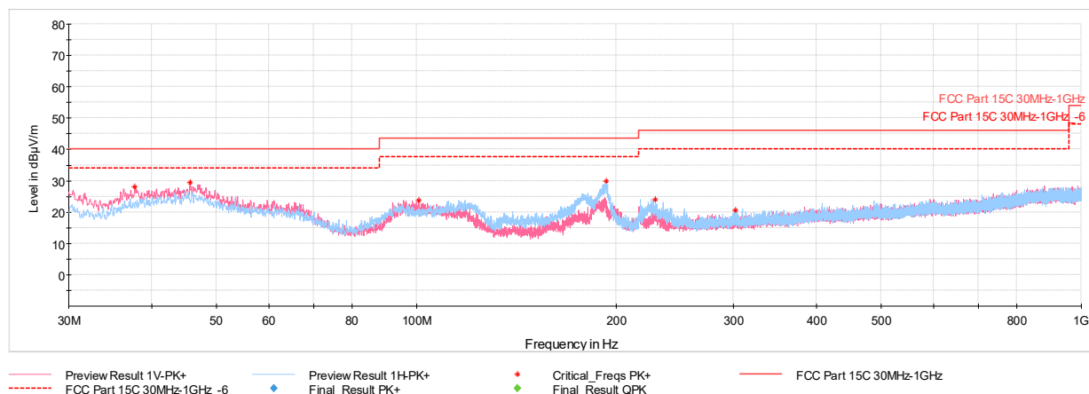
Plot 7-216. Radiated Spurious Emissions Below 1GHz CDD Ch.6 (RU242), with AC/DC Adapter
