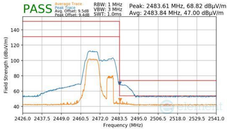
Plot 7-157 Radiated Restricted Upper Band Edge Measurement Antenna 2a (Peak & Average – RU52+26)
