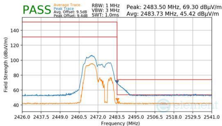
Plot 7-198 Radiated Restricted Upper Band Edge Measurement CDD (Peak & Average – RU52+26)
