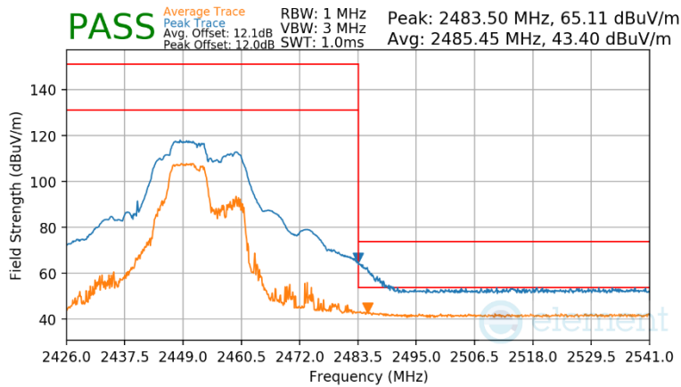
Plot 7-146 Radiated Restricted Upper Band Edge Measurement Antenna 2a (Peak & Average – RU52+26)
