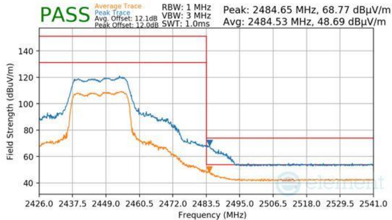
Plot 7-208 Radiated Restricted Upper Band Edge Measurement CDD (Peak & Average – RU242)
