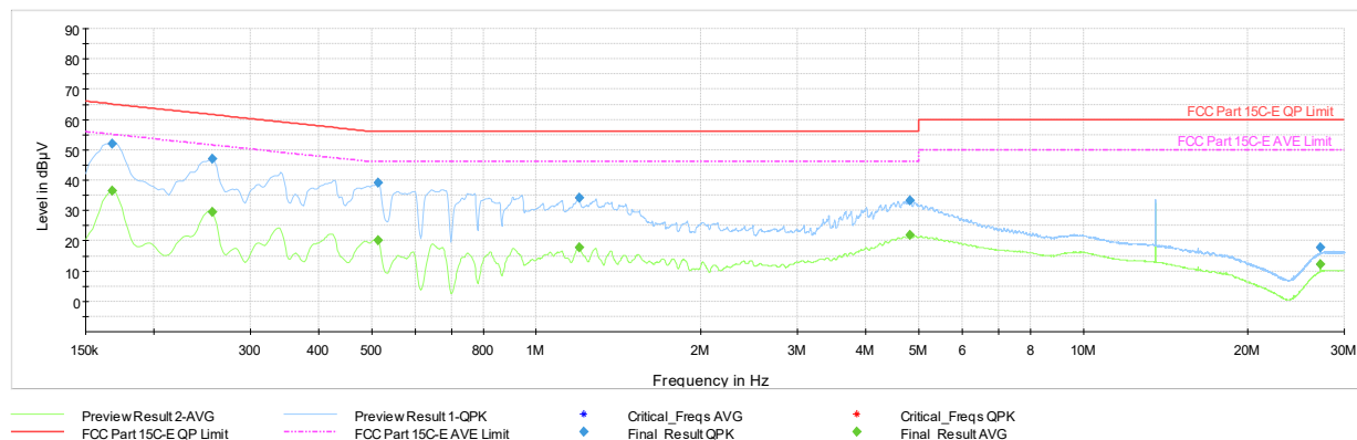
Plot 7-4. AC Line-Conducted Plot (L1, Charging Rate 2.6C, with AC/DC Adapter)
