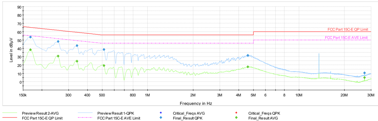
Plot 7-5. AC Line-Conducted Plot (N, Charging Rate 2.6C, with AC/DC Adapter)
