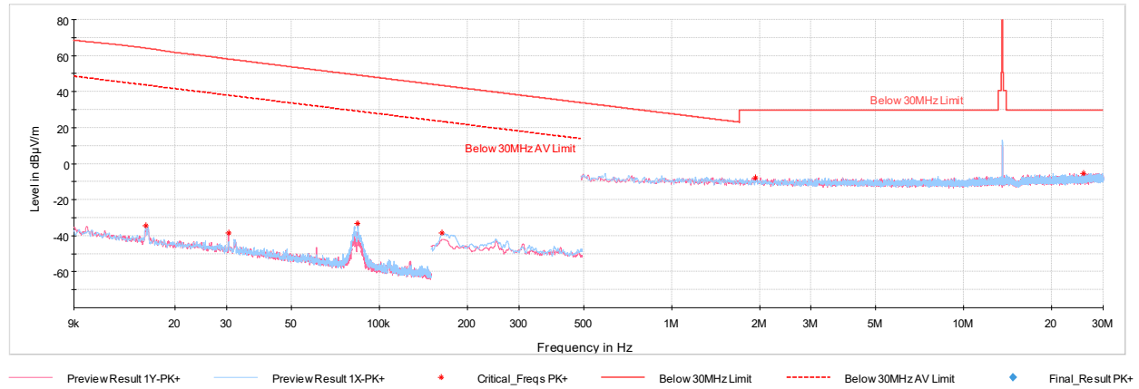
Plot 7-2. Radiated Spurious Plot 9kHz – 30MHz (Charging Rate 2.6C, with AC/DC Adapter)
