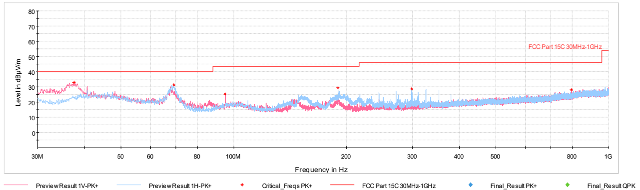
Plot 7-3. Radiated Spurious Emissions 30MHz – 1GHz (Charging Rate 2.6C, with AC/DC Adapter)
