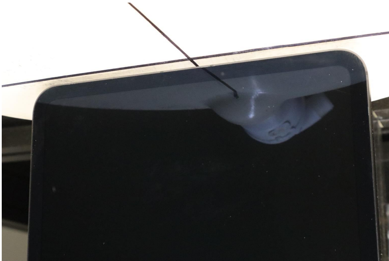
SAR Test Setup Photo 4: Body, Bottom Edge at 5.0 mm
