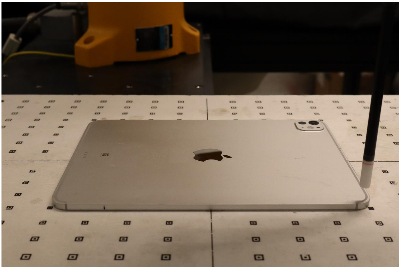
Near Field Power Density Test Setup Photo 19: Body, Back Side at 9.69mm – 4a
