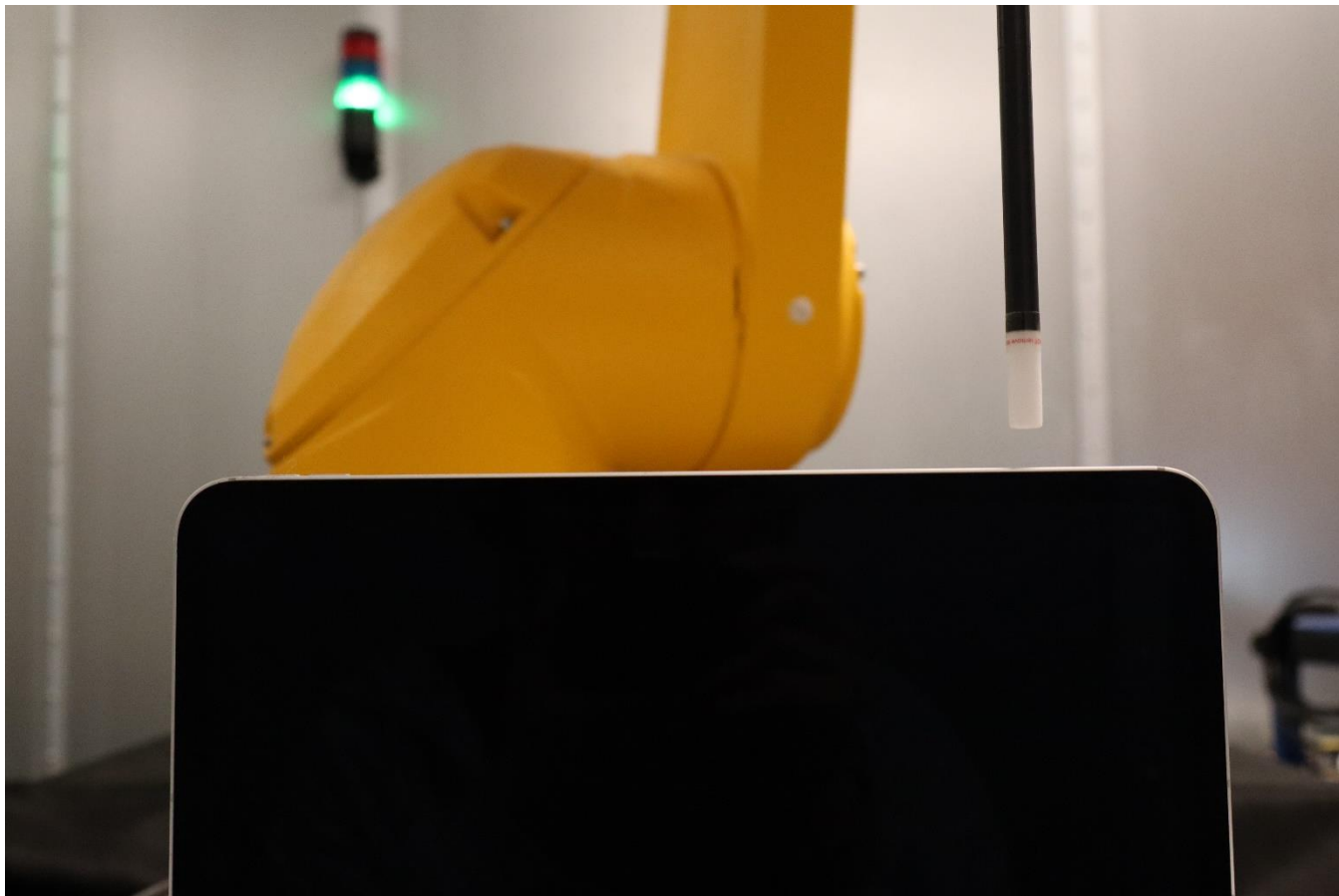
Near Field Power Density Test Setup Photo 21: Body, Right Edge at 9.22mm – WF5B
