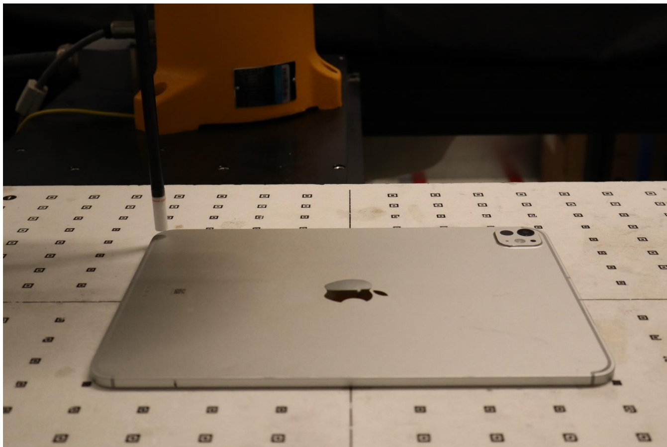
Near Field Power Density Test Setup Photo 14: Body, Back Side at 2mm – 2a
