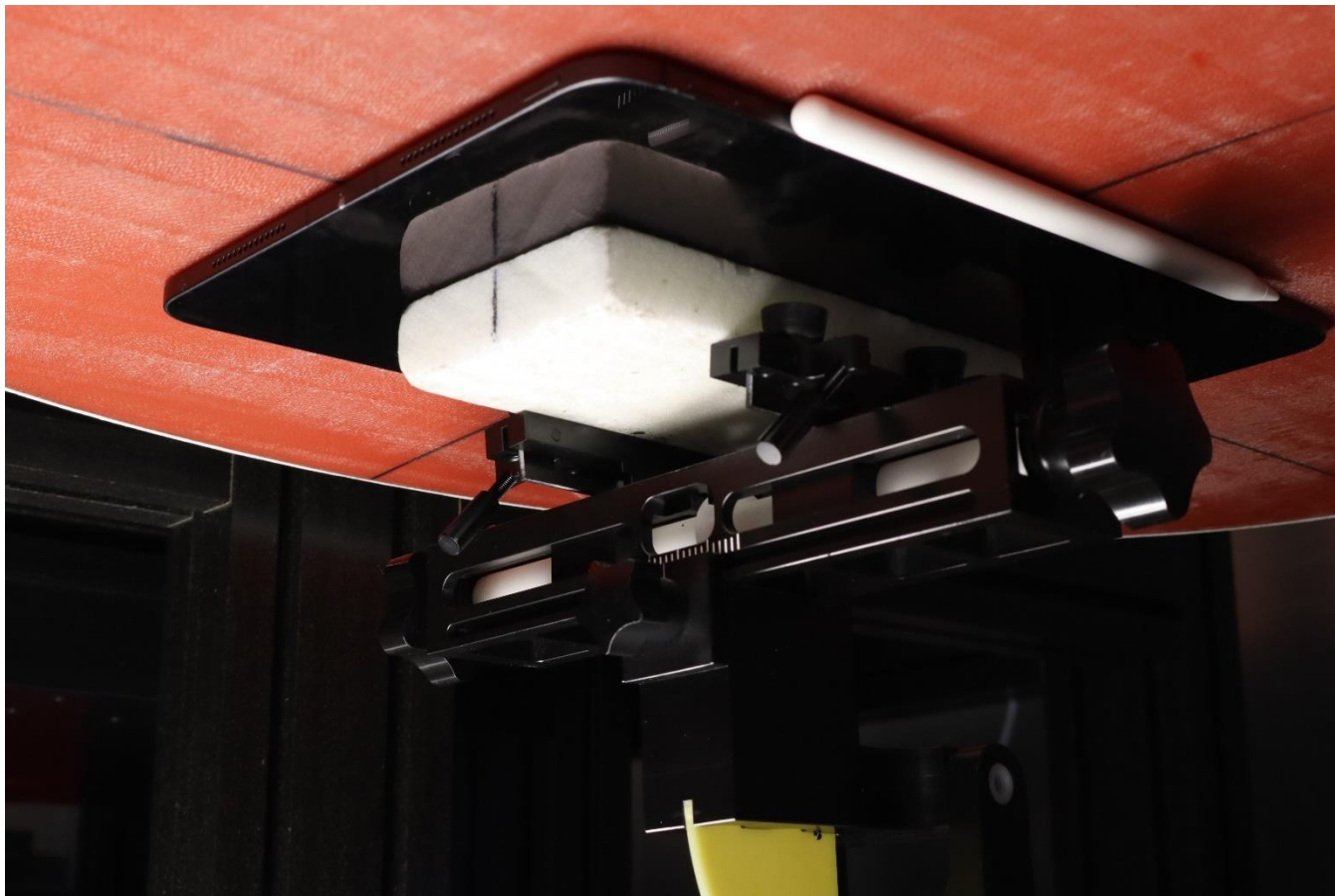
Wireless Power Transfer (wPT) Test Setup Photo 9: Back Side at 5.0 mm
