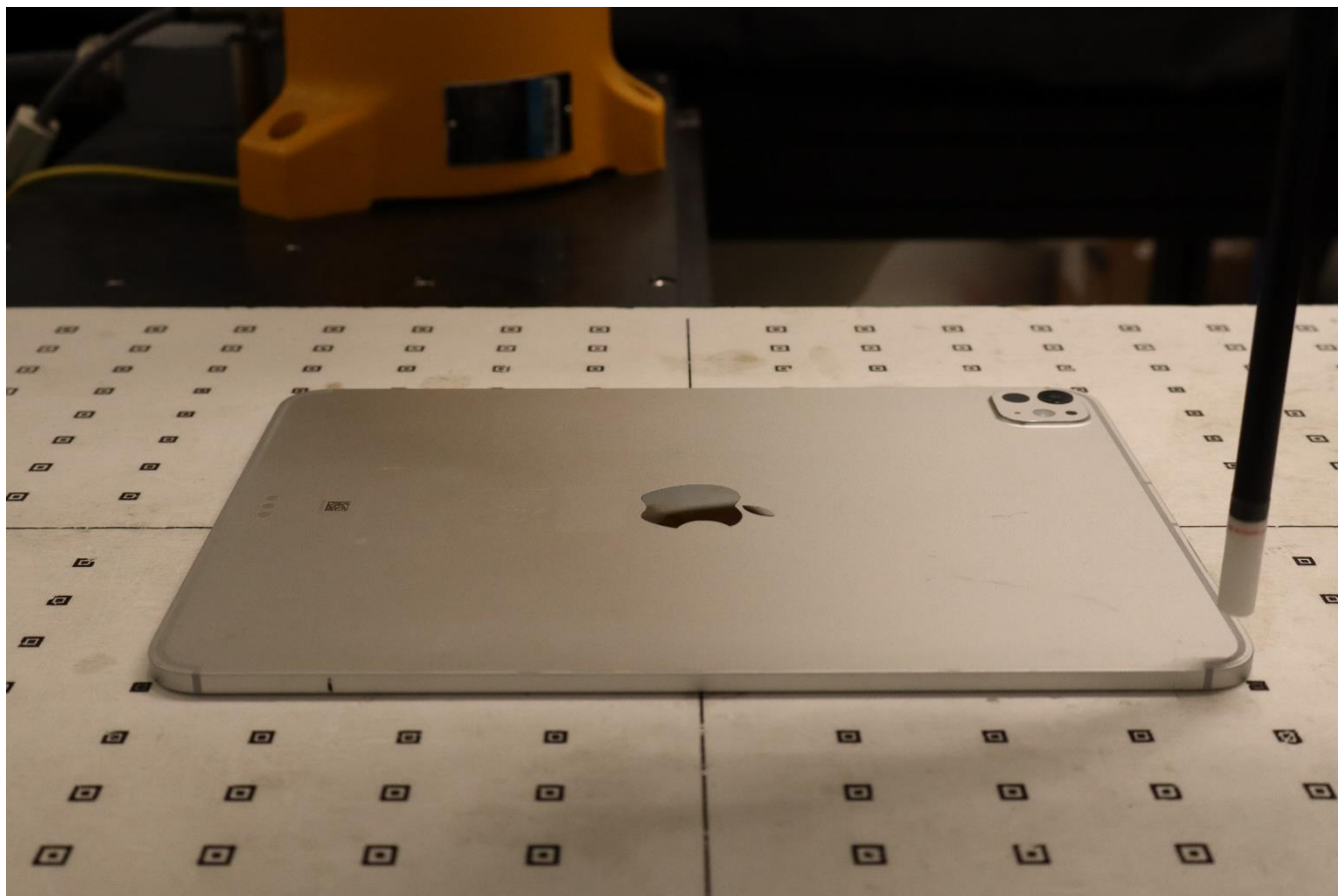
Near Field Power Density Test Setup Photo 18: Body, Back Side at 9.22mm – 4a
