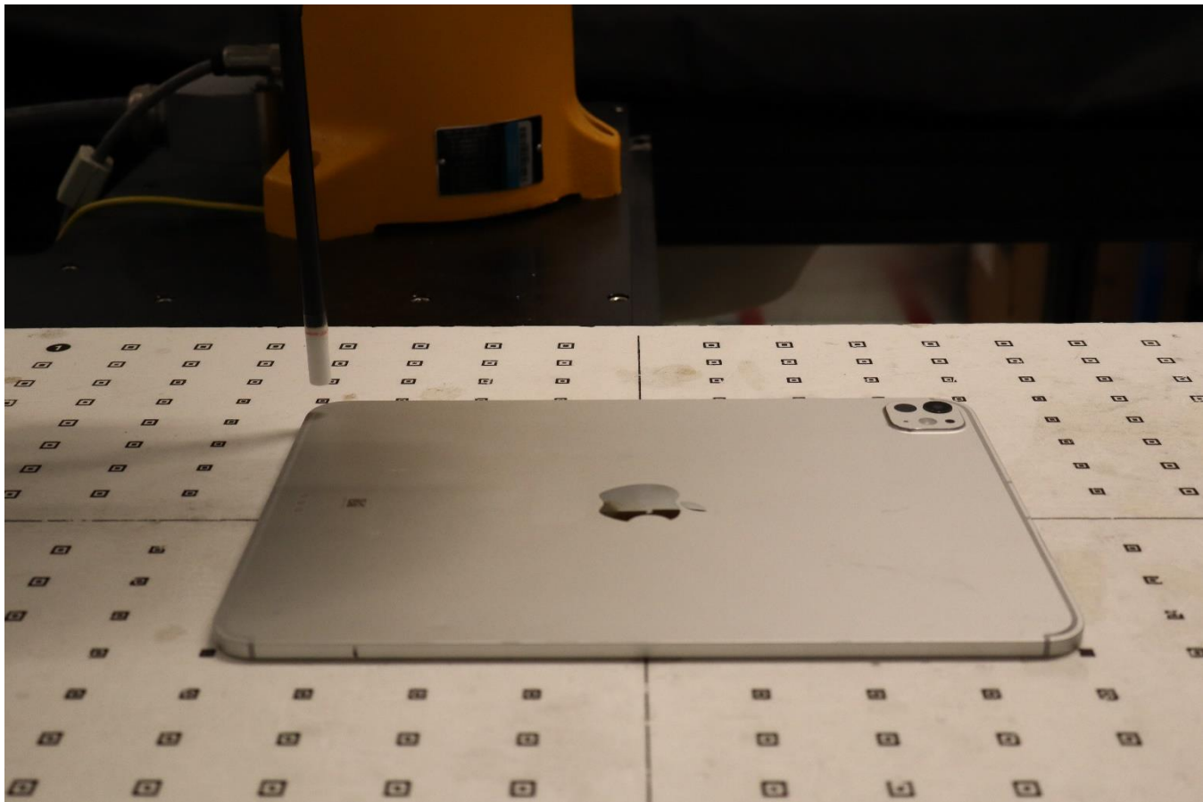
Near Field Power Density Test Setup 15: Body, Back Side at 9.34mm – 2a
