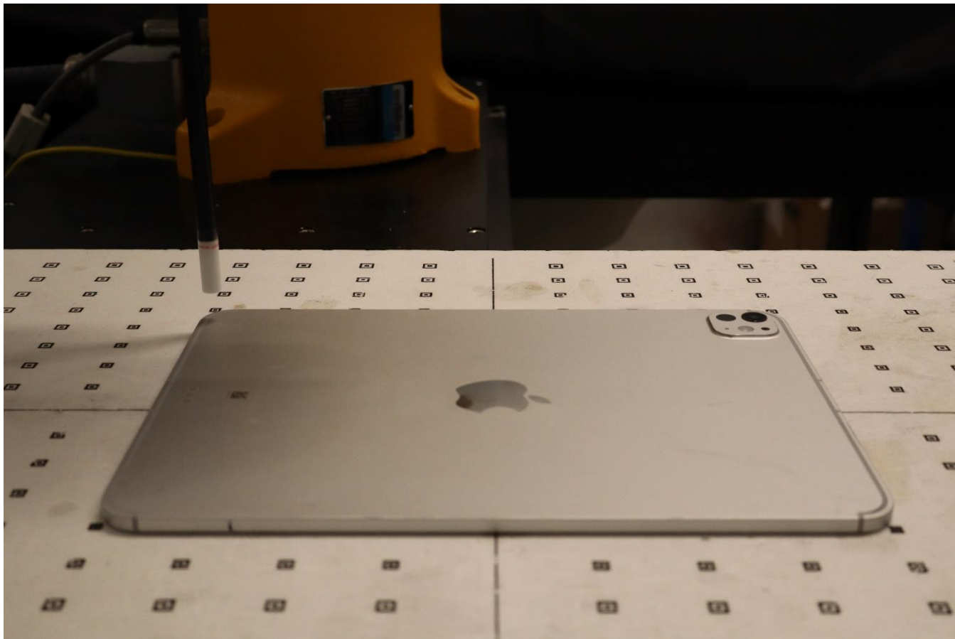
Near Field Power Density Test Setup 16: Body, Back Side at 9.95mm – 2a
