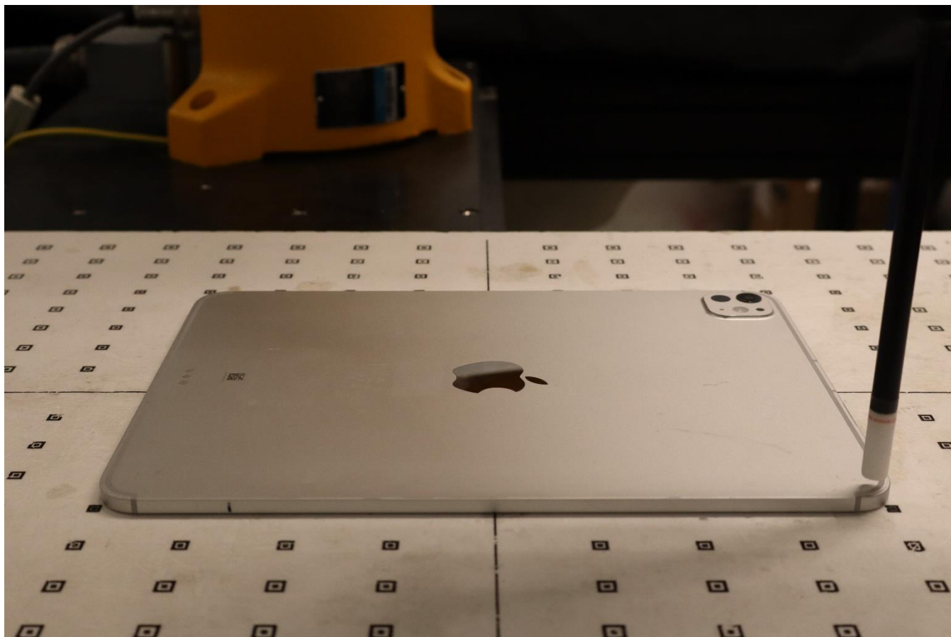
Near Field Power Density Test Setup Photo 17: Body, Back Side at 2mm – 4a
