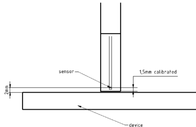
Figure K-2 EUMmWVx Probe
