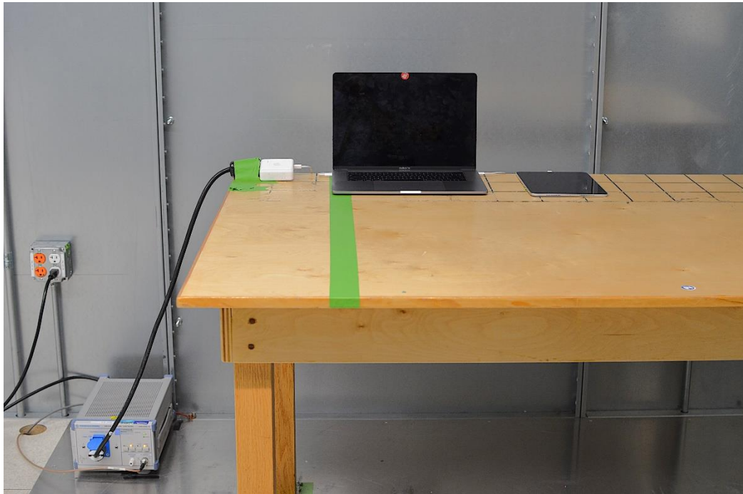
Figure 3: AC Line Conducted Emissions (Front View)
