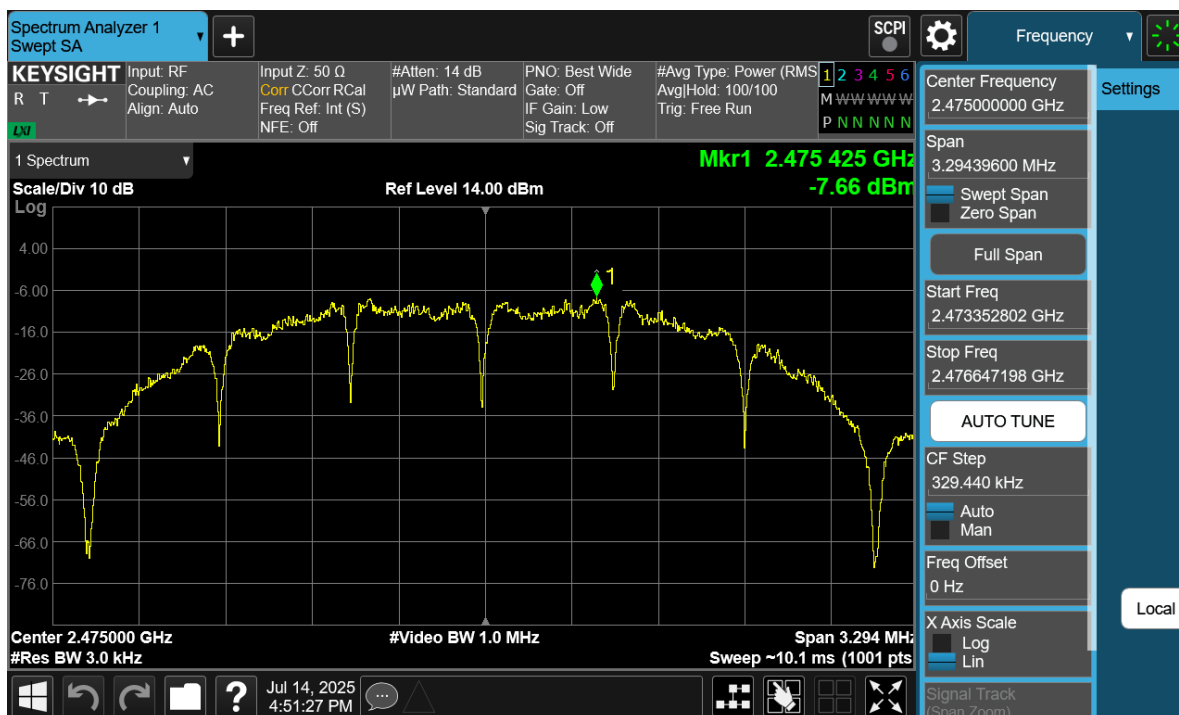
Plot 7-15. Power Spectral Density Antenna WF8 (802.15.4, iPA – Ch. 25)
