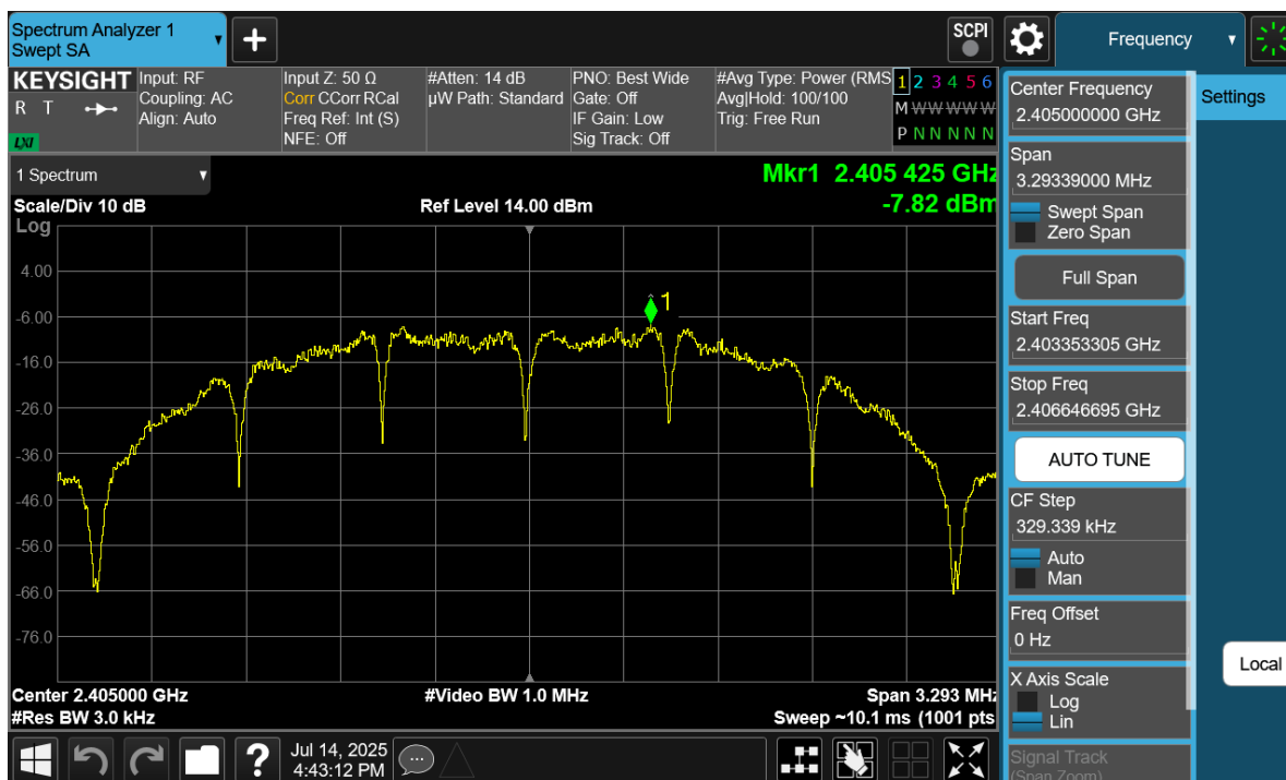
Plot 7-25. Power Spectral Density Antenna WF9 (802.15.4, iPA – Ch. 11)
