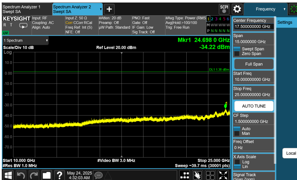
Plot 7-45. Conducted Spurious Antenna WF7 (802.15.4, ePA – Ch. 25)
