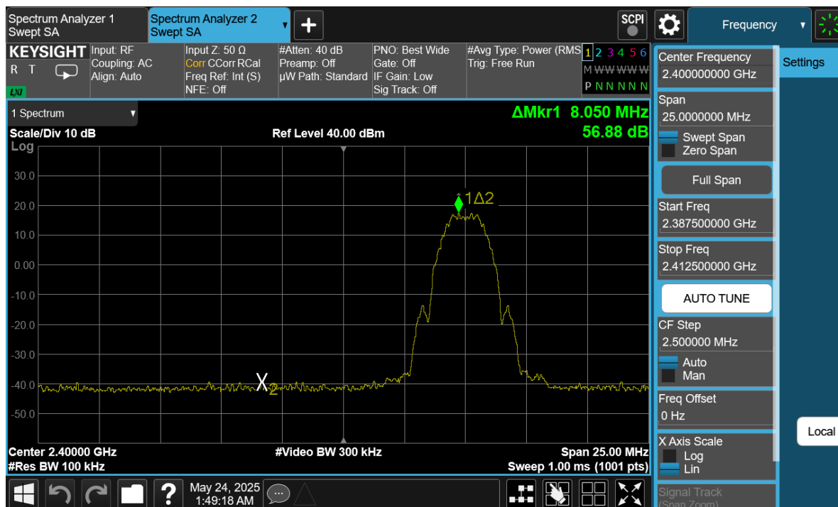
Plot 7-28. Band Edge Antenna WF8 (802.15.4, ePA – Ch. 11)
