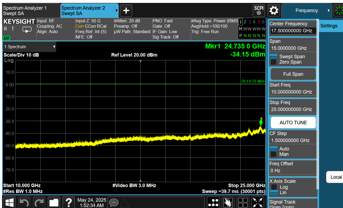
Plot 7-37. Conducted Spurious Antenna WF8 (802.15.4, ePA – Ch. 18)
