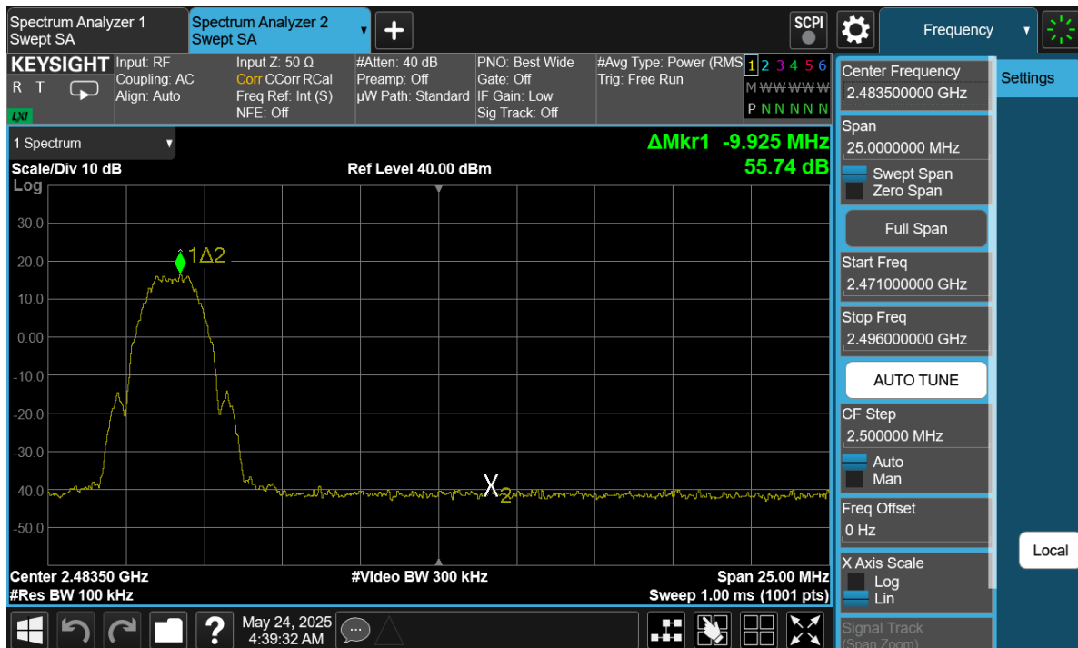
Plot 7-33. Band Edge Antenna WF9 (802.15.4, ePA – Ch. 25)
