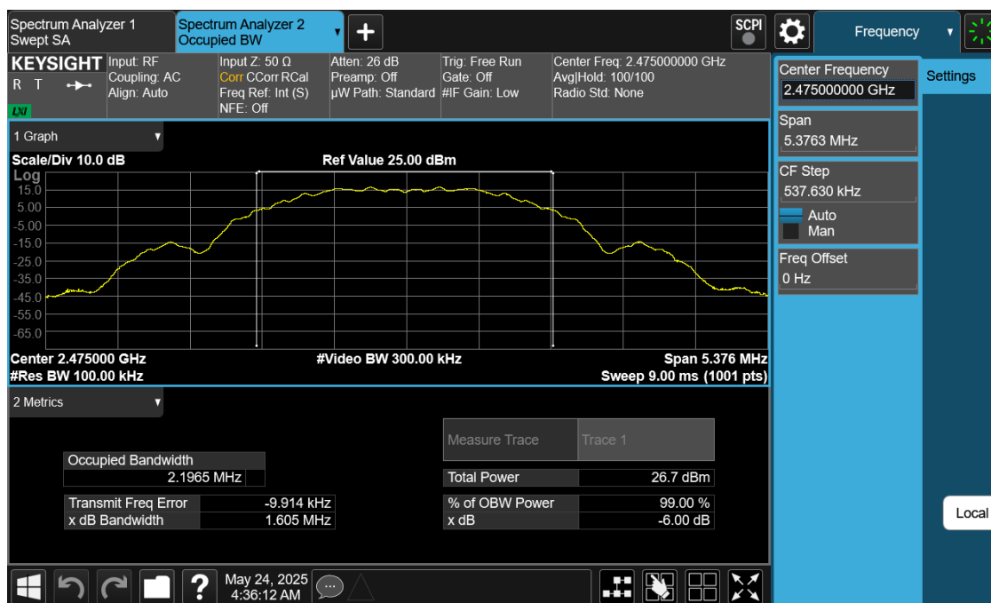
Plot 7-9. 6dB BW & 99% OBW Antenna WF9(802.15.4, Ch. 25)
