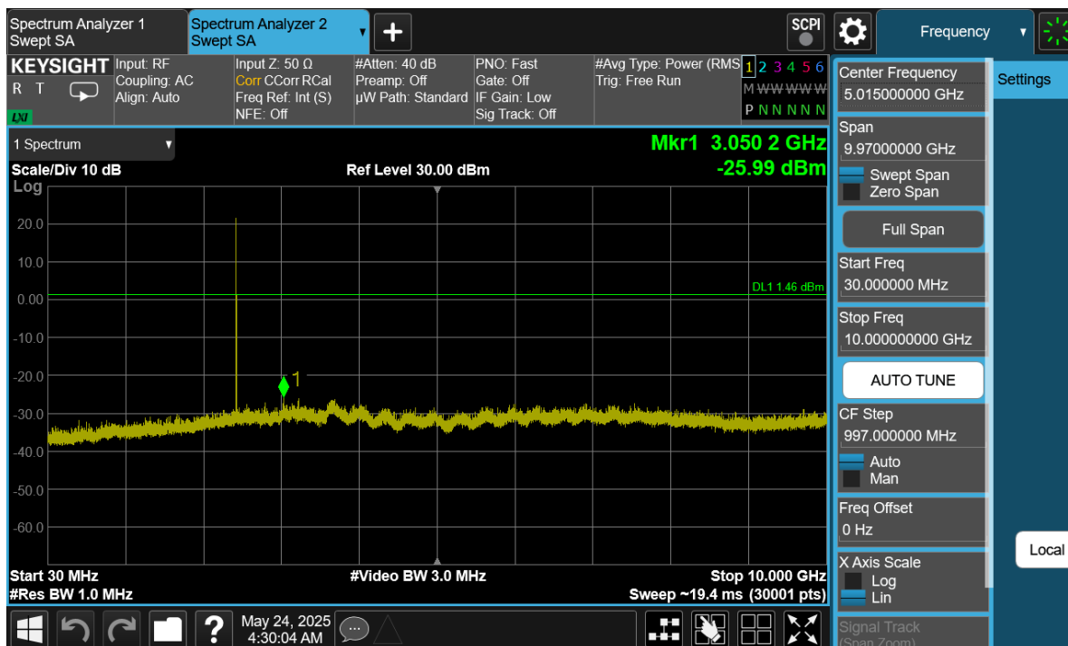
Plot 7-42. Conducted Spurious Antenna WF7 (802.15.4, ePA – Ch. 18)
