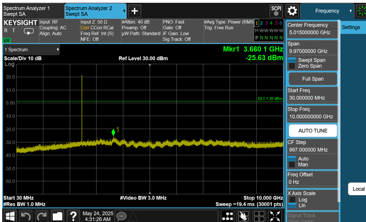
Plot 7-44. Conducted Spurious Antenna WF7 (802.15.4, ePA – Ch. 25)
