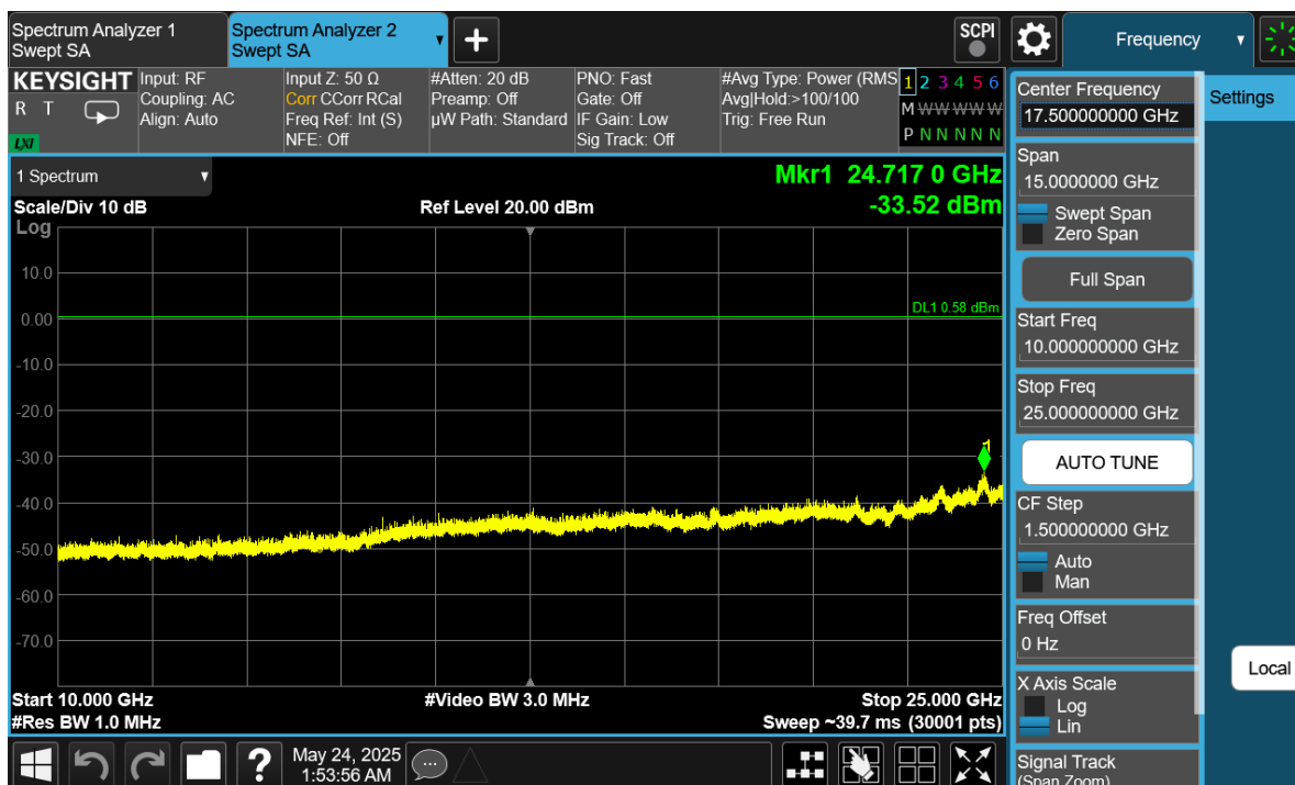
Plot 7-39. Conducted Spurious Antenna WF8 (802.15.4, ePA – Ch. 25)
