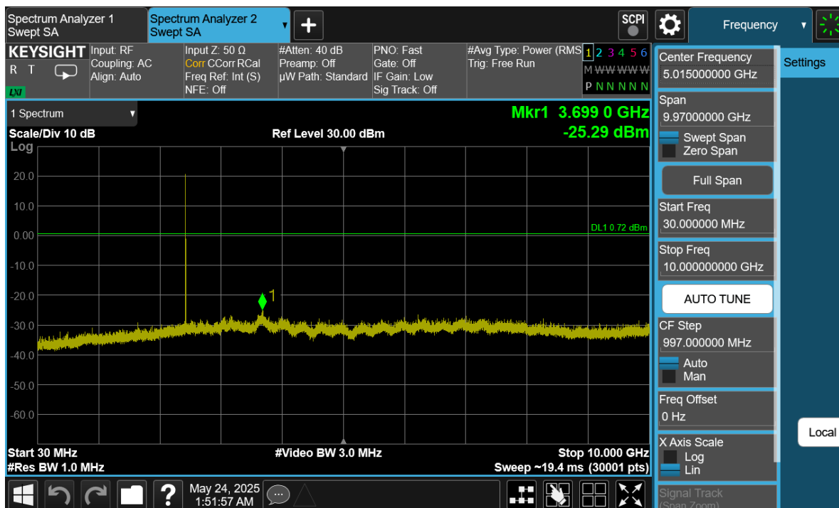
Plot 7-36. Conducted Spurious Antenna WF8 (802.15.4, ePA – Ch. 18)
