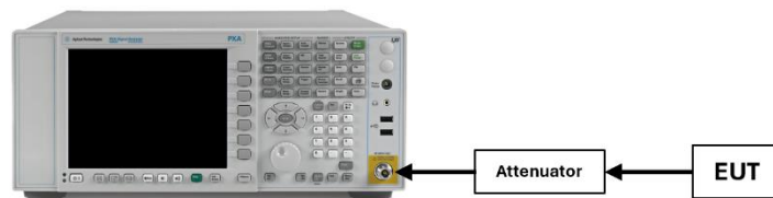
Figure 7-5. Test Instrument & Measurement Setup
