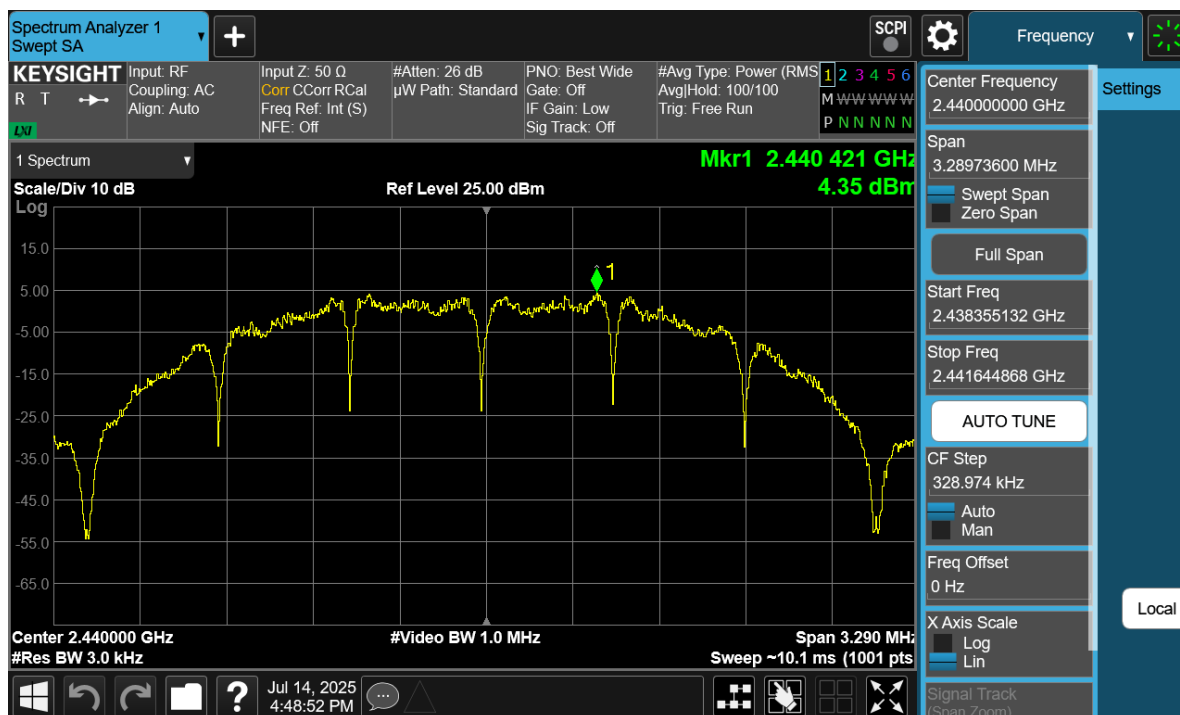
Plot 7-11. Power Spectral Density Antenna WF8 (802.15.4, ePA – Ch. 18)
