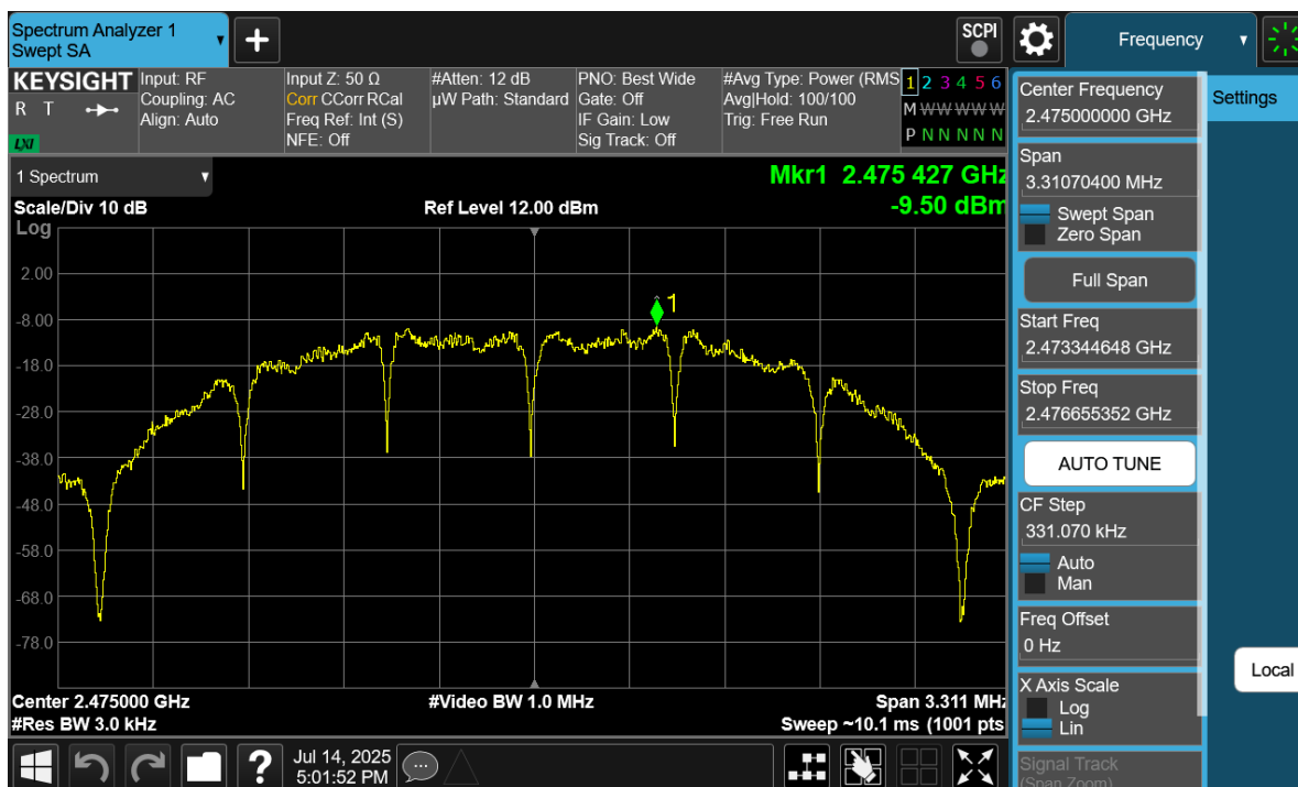
Plot 7-21. Power Spectral Density Antenna WF7 (802.15.4, iPA – Ch. 25)
