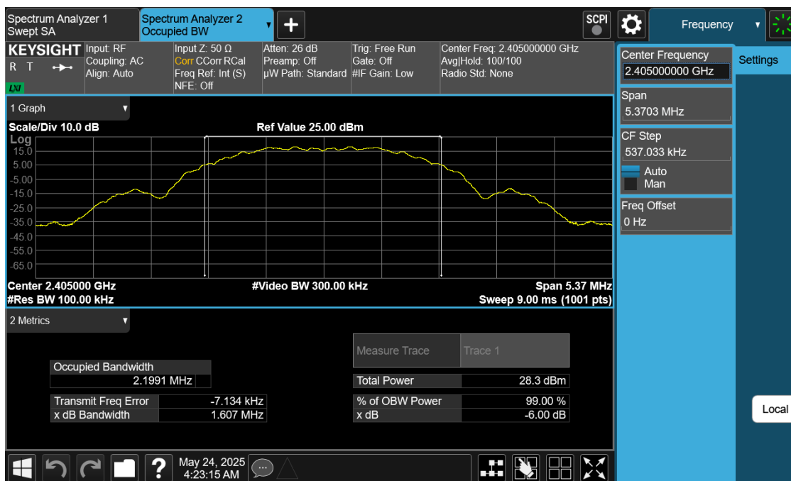
Plot 7-4. 6dB BW & 99% OBW Antenna WF7 (802.15.4, Ch. 11)
