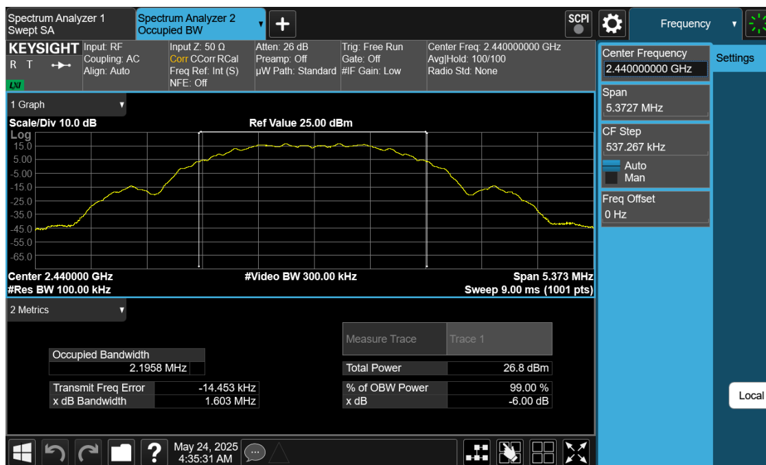
Plot 7-8. 6dB BW & 99% OBW Antenna WF9 (802.15.4, Ch. 18)
