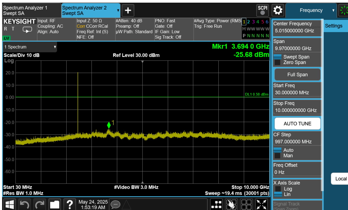
Plot 7-38. Conducted Spurious Antenna WF8 (802.15.4, ePA – Ch. 25)
