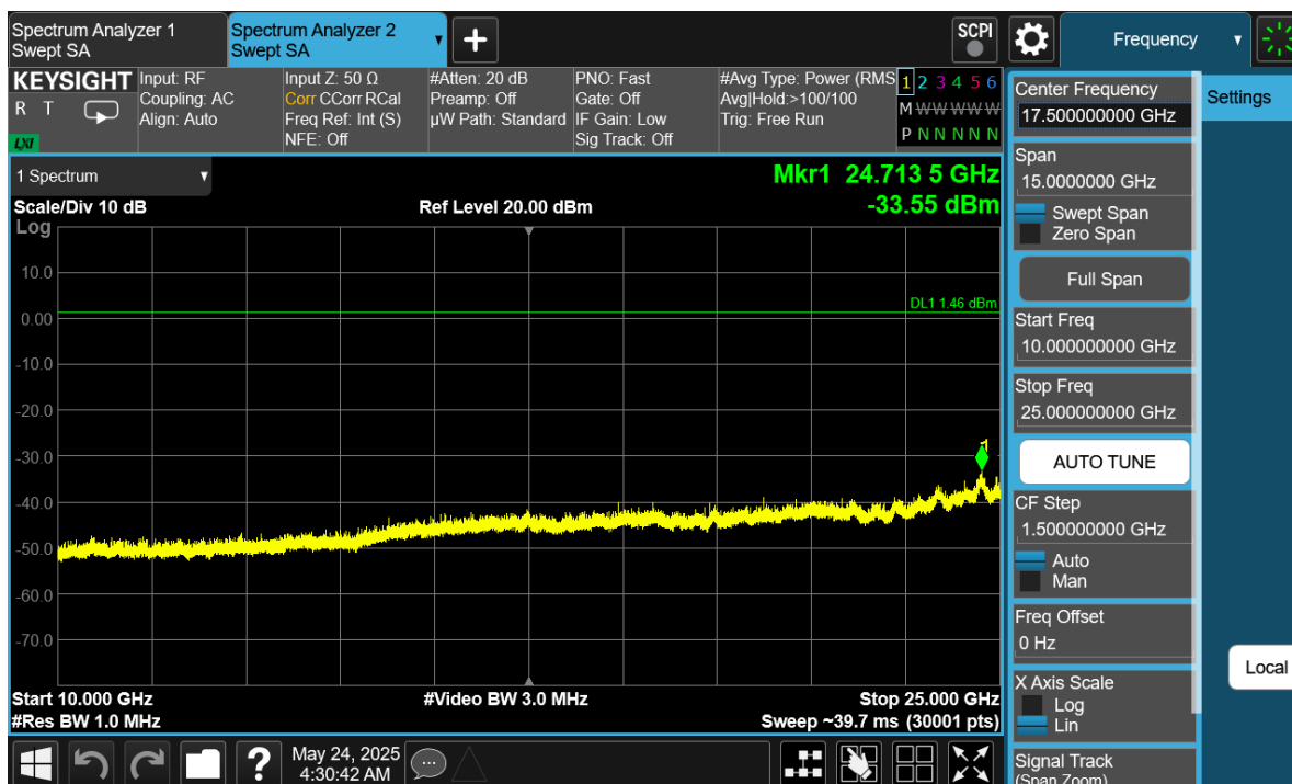
Plot 7-43. Conducted Spurious Antenna WF7 (802.15.4, ePA – Ch. 18)
