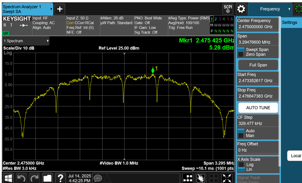
Plot 7-24. Power Spectral Density Antenna WF9 (802.15.4, ePA – Ch. 25)
