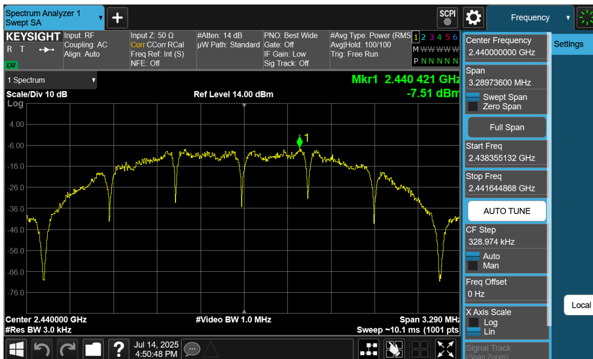
Plot 7-14. Power Spectral Density Antenna WF8 (802.15.4, iPA – Ch. 18)
