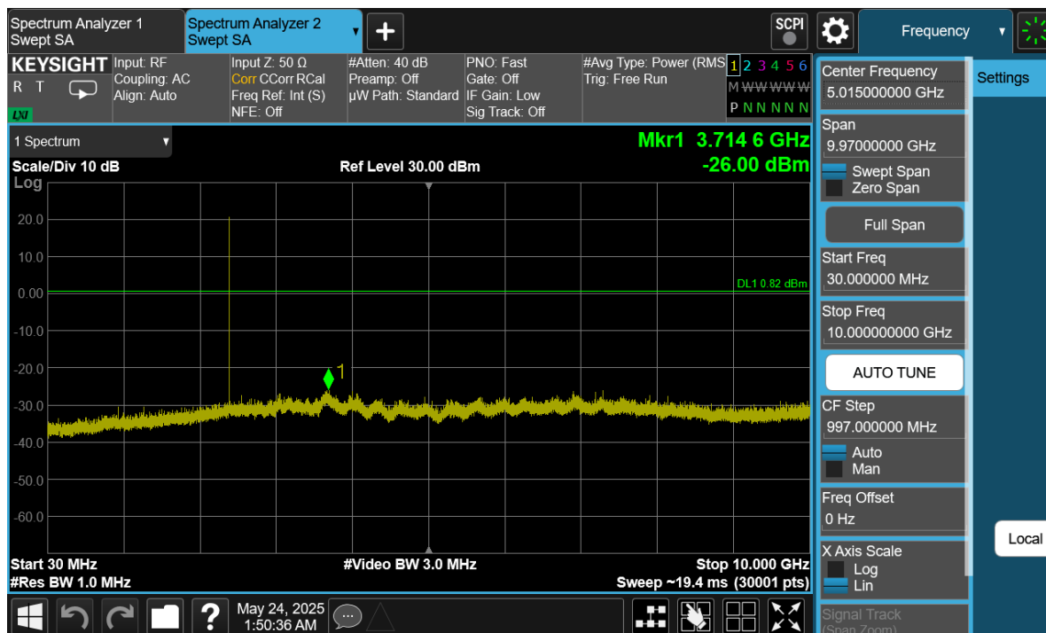
Plot 7-34. Conducted Spurious Antenna WF8 (802.15.4, ePA – Ch. 11)
