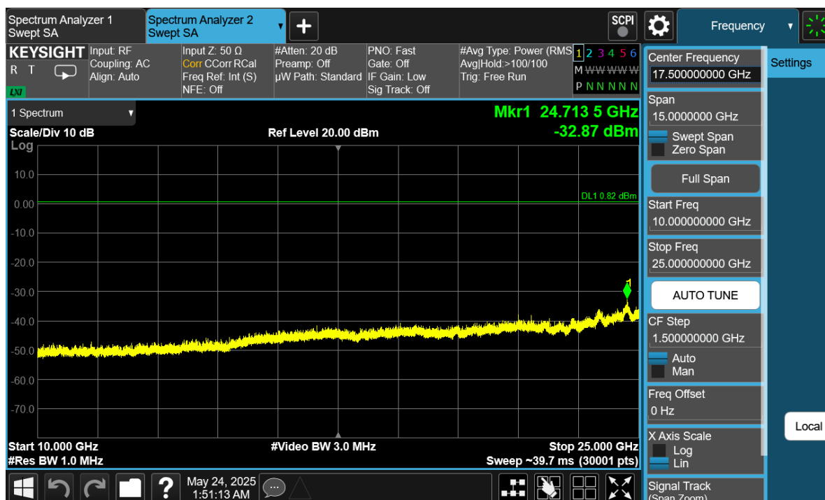
Plot 7-35. Conducted Spurious Antenna WF8 (802.15.4, ePA – Ch. 11)
