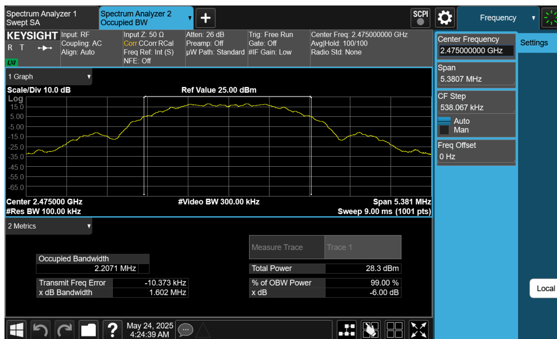
Plot 7-6. 6dB BW & 99% OBW Antenna WF7(802.15.4, Ch. 25)
