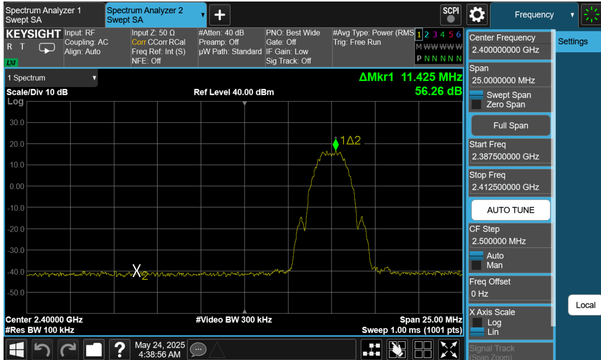
Plot 7-32. Band Edge Antenna WF9 (802.15.4, ePA – Ch. 11)
