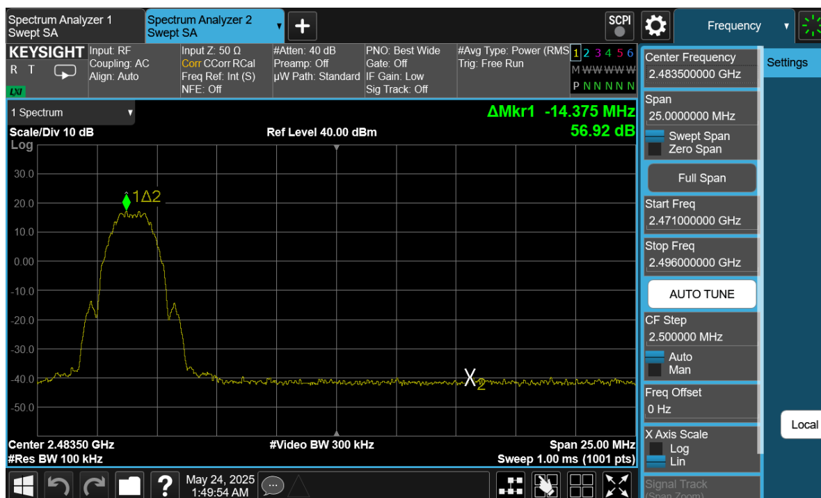
Plot 7-29. Band Edge Antenna WF8 (802.15.4, ePA – Ch. 25)
