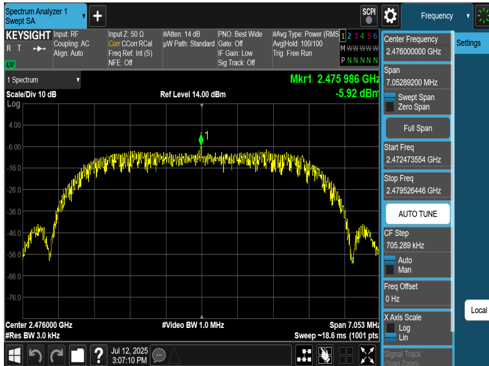
Plot 7-81. Power Spectral Density Plot Antenna WF8 (Bluetooth (HDRPM16), 16Mbps, ePA – Ch. 73)
