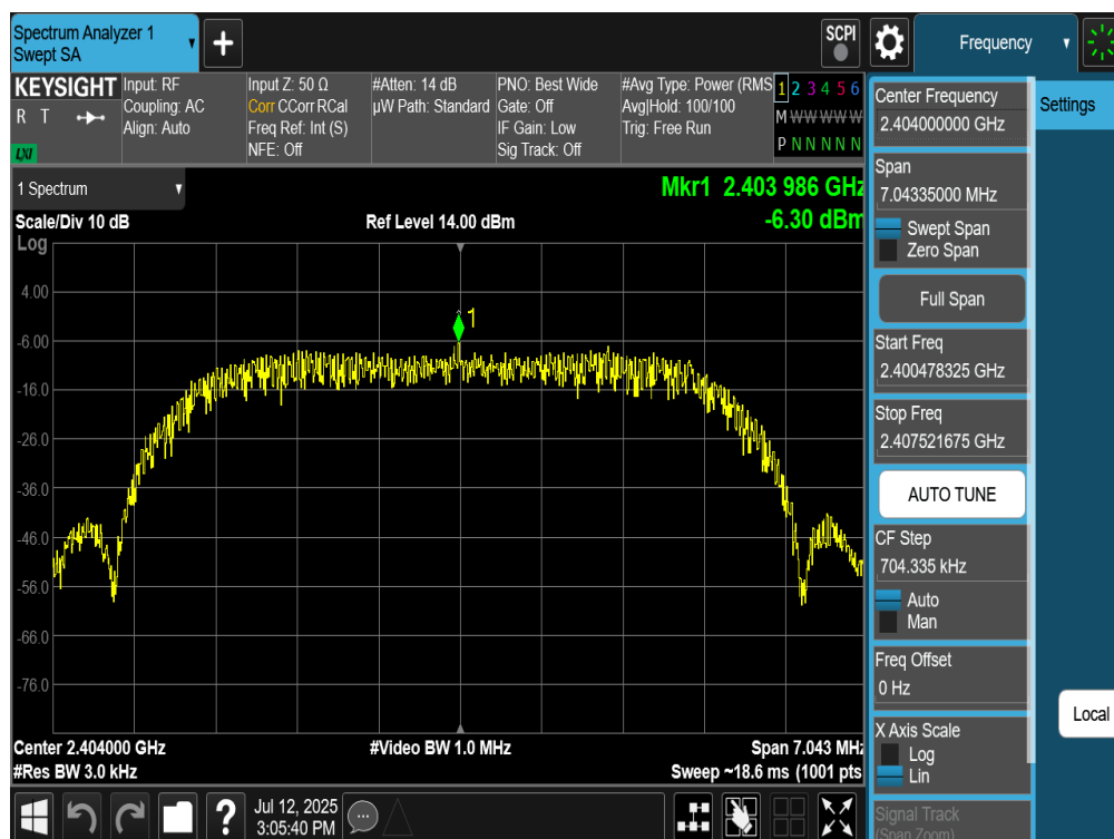
Plot 7-79. Power Spectral Density Plot Antenna WF8 (Bluetooth (HDRPM16), 16Mbps, ePA – Ch. 1)
