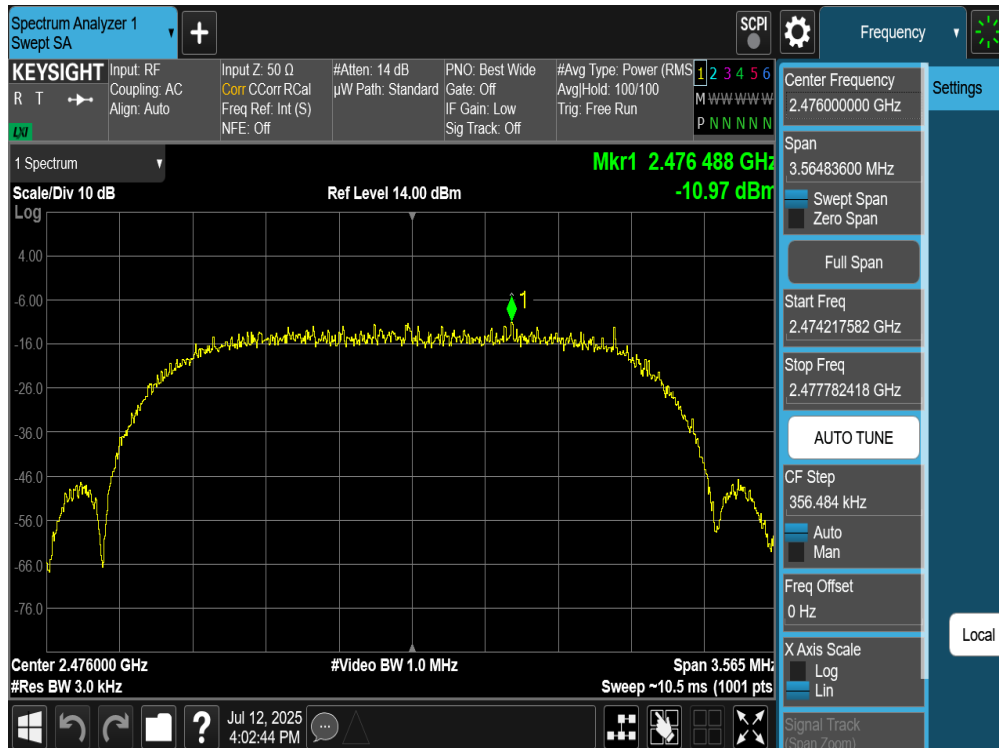
Plot 7-108. Power Spectral Density Plot Antenna WF7 (Bluetooth (HDRPS2), 2Mbps, iPA – Ch. 73)
