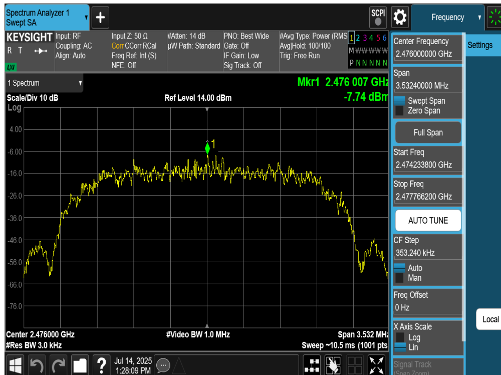
Plot 7-60. Power Spectral Density Plot Antenna WF8 (Bluetooth (HDR4), 4Mbps, iPA – Ch. 73)
