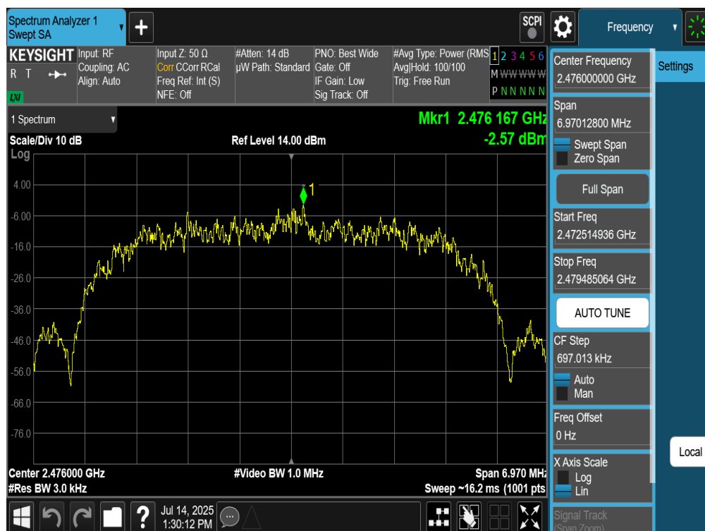
Plot 7-63. Power Spectral Density Plot Antenna WF8 (Bluetooth (HDR8), 8Mbps, ePA – Ch. 73)
