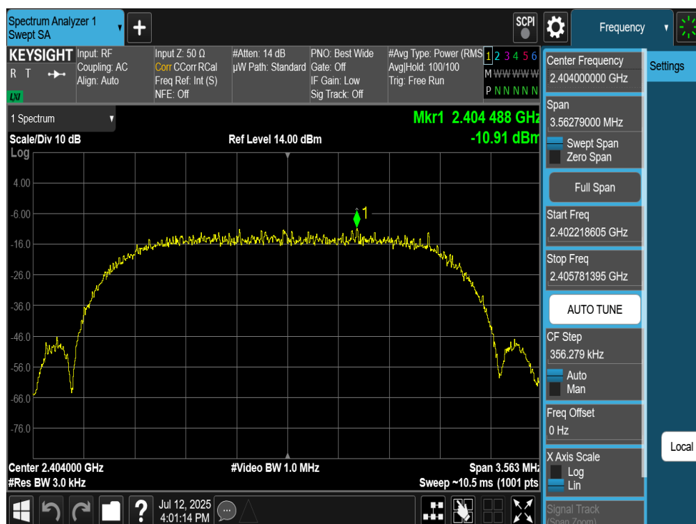
Plot 7-106. Power Spectral Density Plot Antenna WF7 (Bluetooth (HDRPS2), 2Mbps, iPA – Ch. 1)
