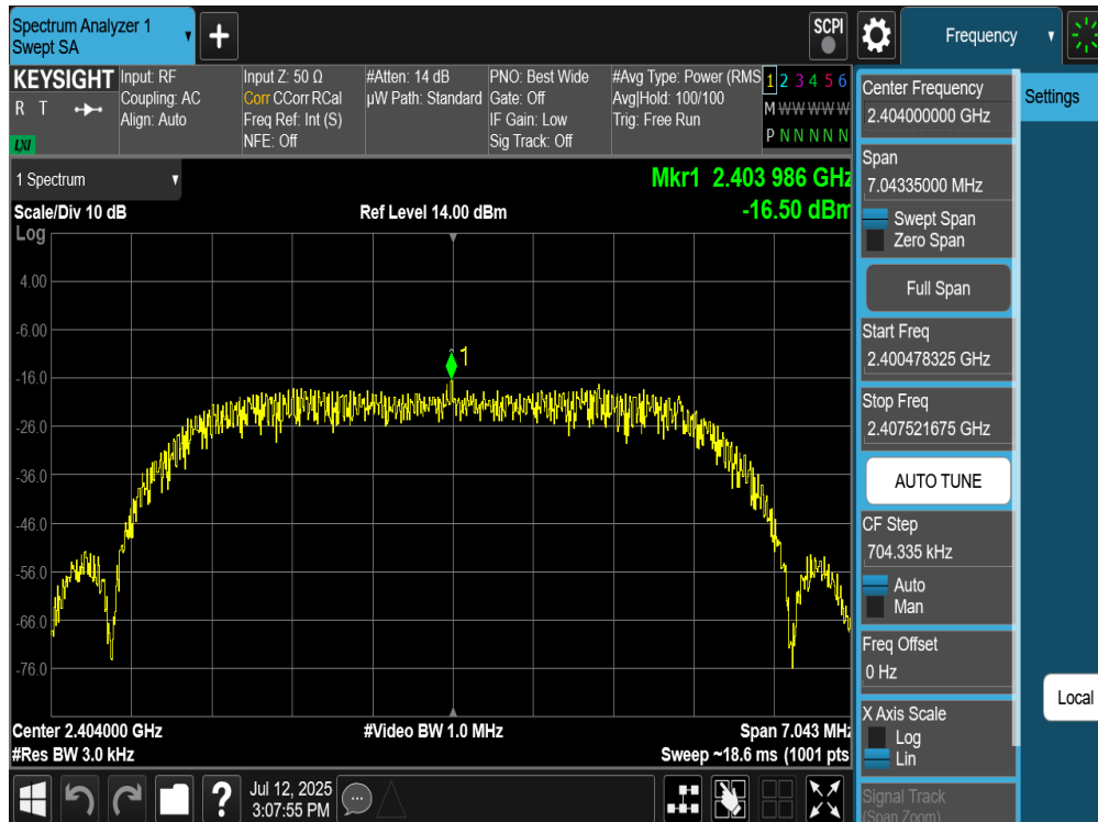
Plot 7-82. Power Spectral Density Plot Antenna WF8 (Bluetooth (HDRPM16), 16Mbps, iPA – Ch. 1)
