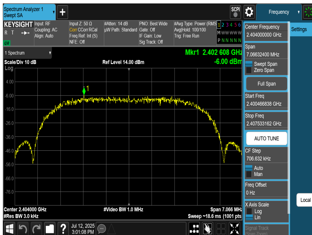
Plot 7-73. Power Spectral Density Plot Antenna WF8 (Bluetooth (XHDRPM6), 6Mbps, ePA – Ch. 1)
