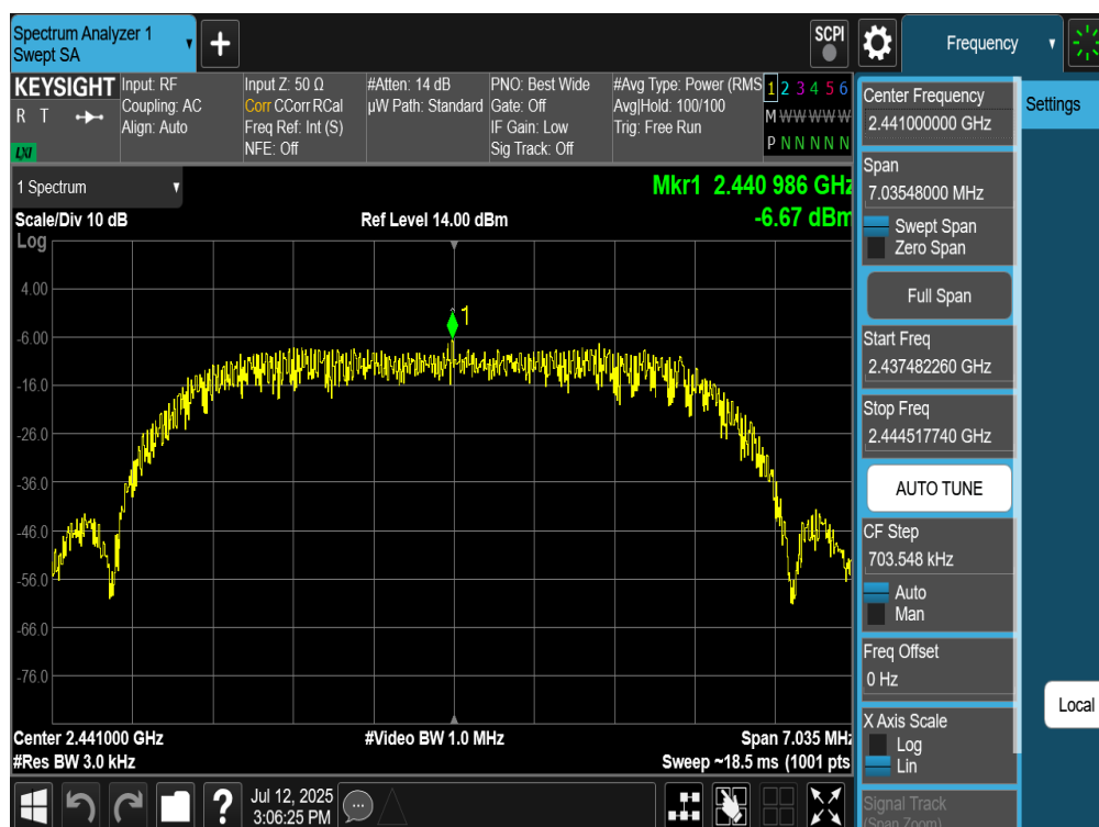
Plot 7-80. Power Spectral Density Plot Antenna WF8 (Bluetooth (HDRPM16), 16Mbps, ePA – Ch. 38)
