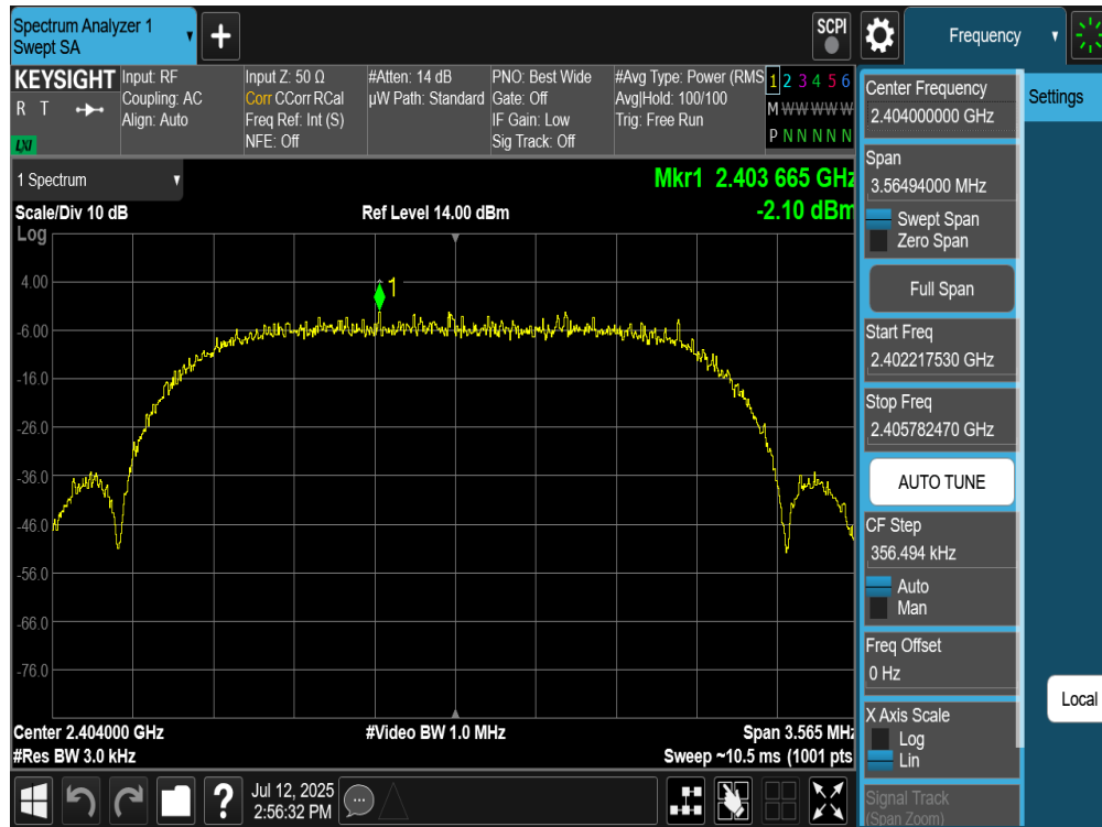
Plot 7-67. Power Spectral Density Plot Antenna WF8 (Bluetooth (HDRPS2), 2Mbps, ePA – Ch. 1)
