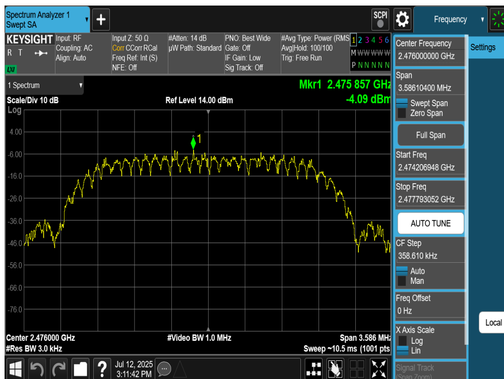
Plot 7-87. Power Spectral Density Plot Antenna WF8 (Bluetooth (HDT2), 2Mbps, ePA – Ch. 73)
