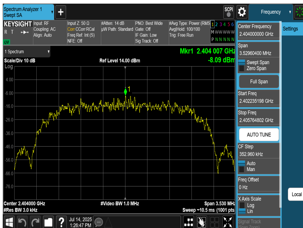
Plot 7-58. Power Spectral Density Plot Antenna WF8 (Bluetooth (HDR4), 4Mbps, iPA – Ch. 1)
