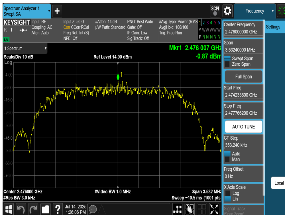
Plot 7-57. Power Spectral Density Plot Antenna WF8 (Bluetooth (HDR4), 4Mbps, ePA – Ch. 73)
