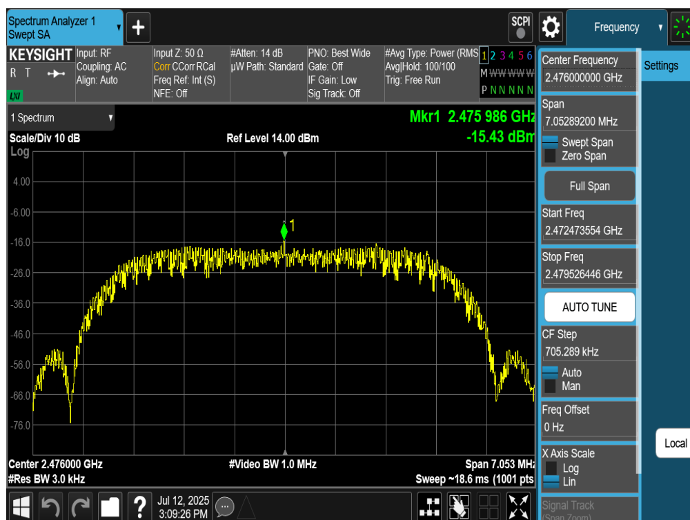
Plot 7-84. Power Spectral Density Plot Antenna WF8 (Bluetooth (HDRPM16), 16Mbps, iPA – Ch. 73)
