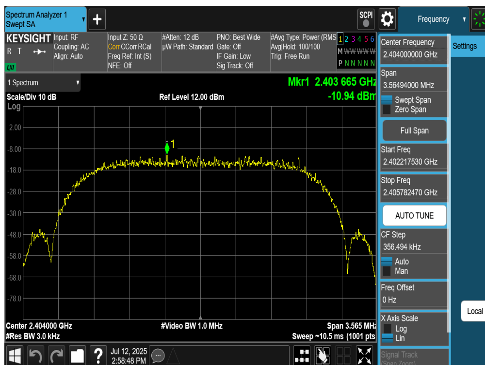
Plot 7-70. Power Spectral Density Plot Antenna WF8 (Bluetooth (HDRPS2), 2Mbps, iPA – Ch. 1)
