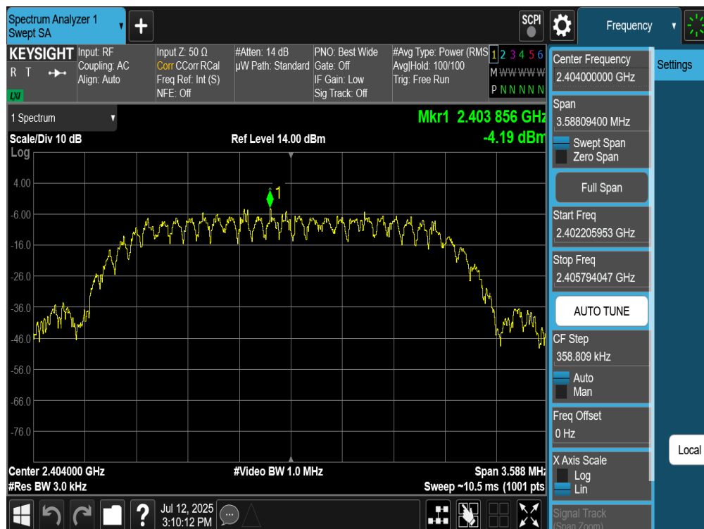
Plot 7-85. Power Spectral Density Plot Antenna WF8 (Bluetooth (HDT2), 2Mbps, ePA – Ch. 1)
