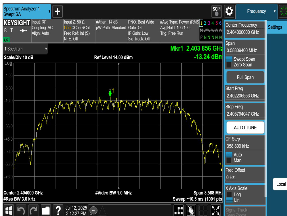
Plot 7-88. Power Spectral Density Plot Antenna WF8 (Bluetooth (HDT2), 2Mbps, iPA – Ch. 1)
