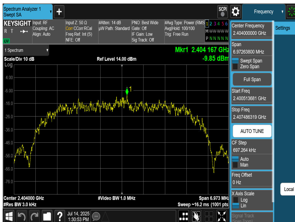
Plot 7-64. Power Spectral Density Plot Antenna WF8 (Bluetooth (HDR8), 8Mbps, iPA – Ch. 1)
