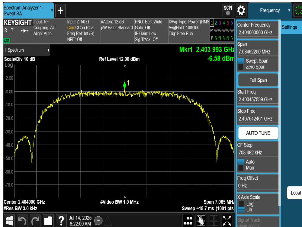
Plot 7-200. Power Spectral Density Plot Tx BF Primary Antenna WF7 (Bluetooth (XHDRPM6), 6Mbps, ePA – Ch. 1)
