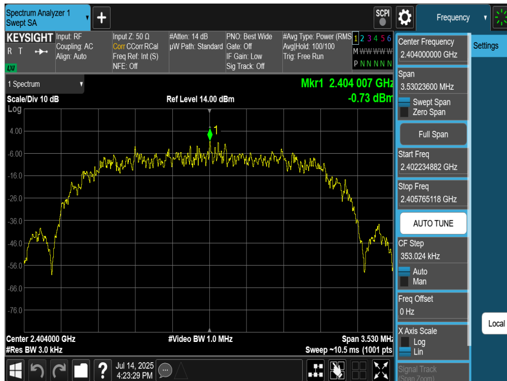
Plot 7-236. Power Spectral Density Plot Tx BF Diversity Antenna WF9 (Bluetooth (HDR4), 4Mbps, ePA – Ch. 1)
