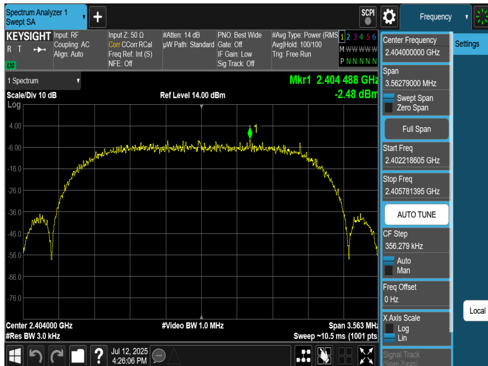
Plot 7-188. Power Spectral Density Plot Tx BF Primary Antenna WF7 (Bluetooth (HDRPS2), 2Mbps, ePA – Ch. 1)
