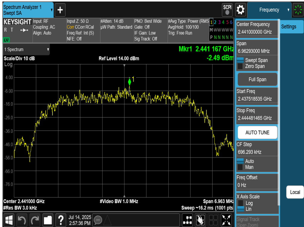
Plot 7-178. Power Spectral Density Plot TxBF Primary Antenna WF7 (Bluetooth (HDR8), 8Mbps, ePA – Ch. 38)
