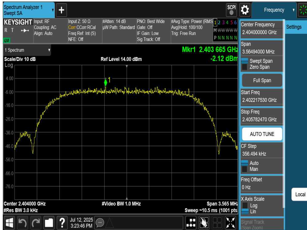
Plot 7-187. Power Spectral Density Plot Tx BF Primary Antenna WF8 (Bluetooth (HDRPS2), 2Mbps, ePA – Ch. 1)
