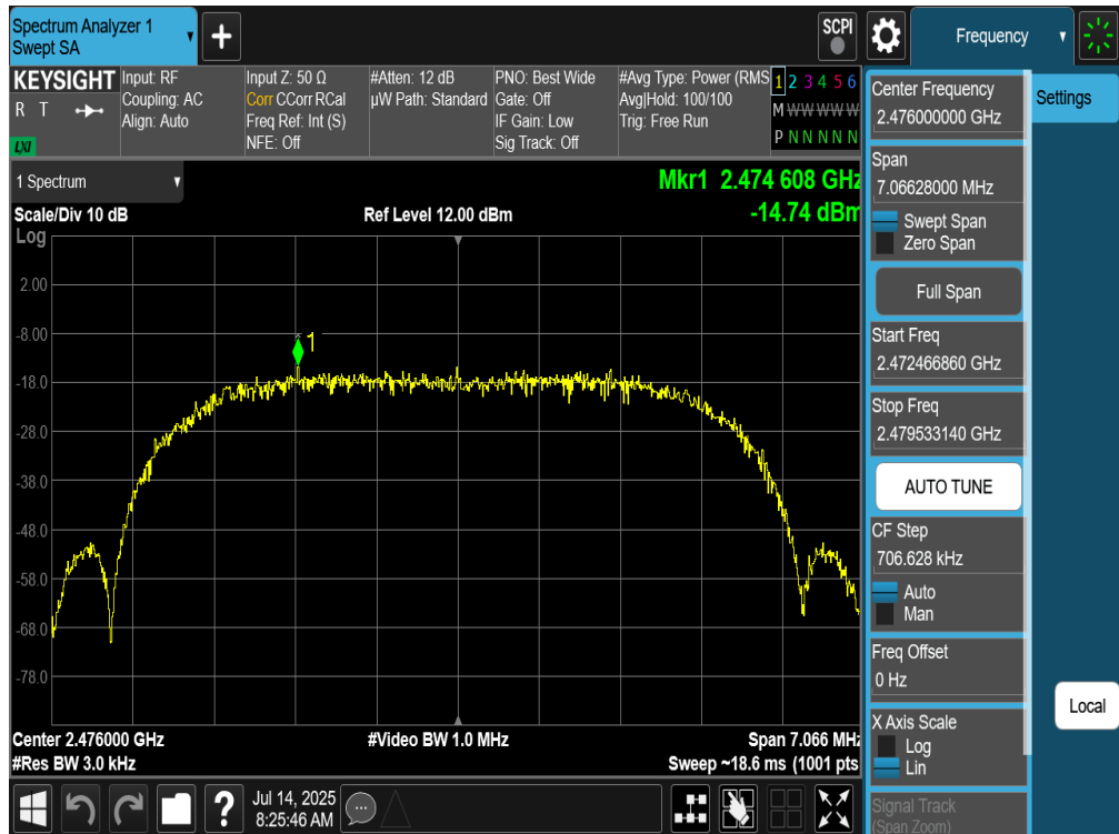
Plot 7-210. Power Spectral Density Plot TxBF Primary Antenna WF7 (Bluetooth (XHDRPM6), 6Mbps, iPA – Ch. 73)
