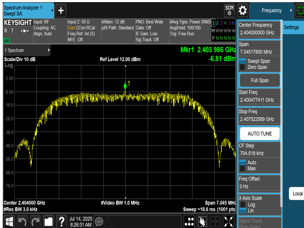
Plot 7-212. Power Spectral Density Plot Tx BF Primary Antenna WF7 (Bluetooth (HDRPM16), 16Mbps, ePA – Ch. 1)
