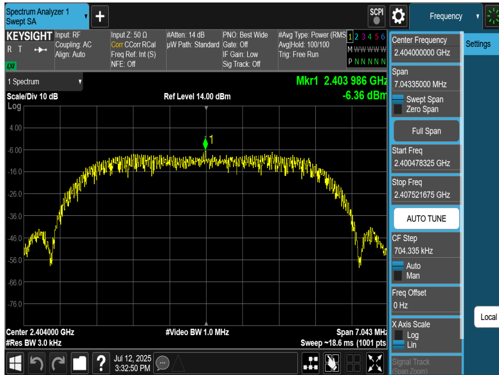
Plot 7-211. Power Spectral Density Plot Tx BF Primary Antenna WF8 (Bluetooth (HDRPM16), 16Mbps, ePA – Ch. 1)
