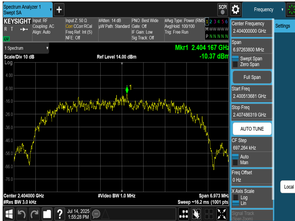
Plot 7-181. Power Spectral Density Plot Tx BF Primary Antenna WF8 (Bluetooth (HDR8), 8Mbps, iPA – Ch. 1)
