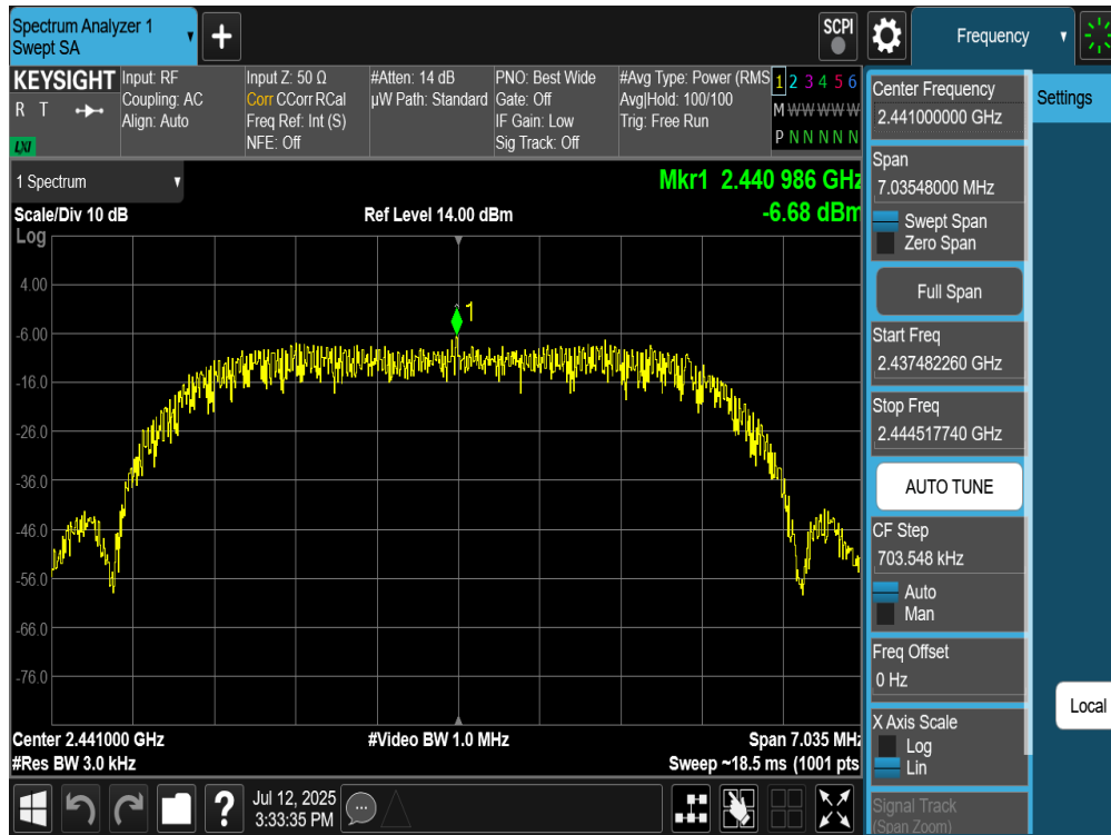
Plot 7-213. Power Spectral Density Plot Tx BF Primary Antenna WF8 (Bluetooth (HDRPM16), 16Mbps, ePA – Ch. 38)
