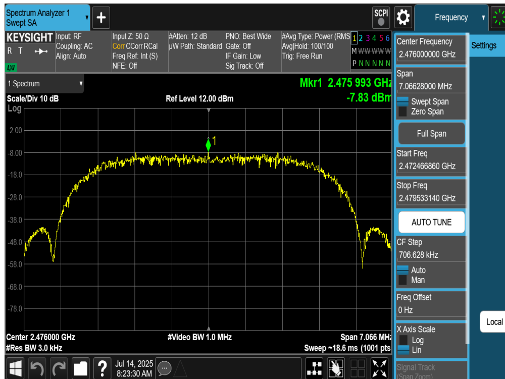
Plot 7-204. Power Spectral Density Plot TxBF Primary Antenna WF7 (Bluetooth (XHDRPM6), 6Mbps, ePA – Ch. 73)
