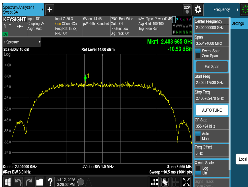
Plot 7-193. Power Spectral Density Plot Tx BF Primary Antenna WF8 (Bluetooth (HDRPS2), 2Mbps, iPA – Ch. 1)
