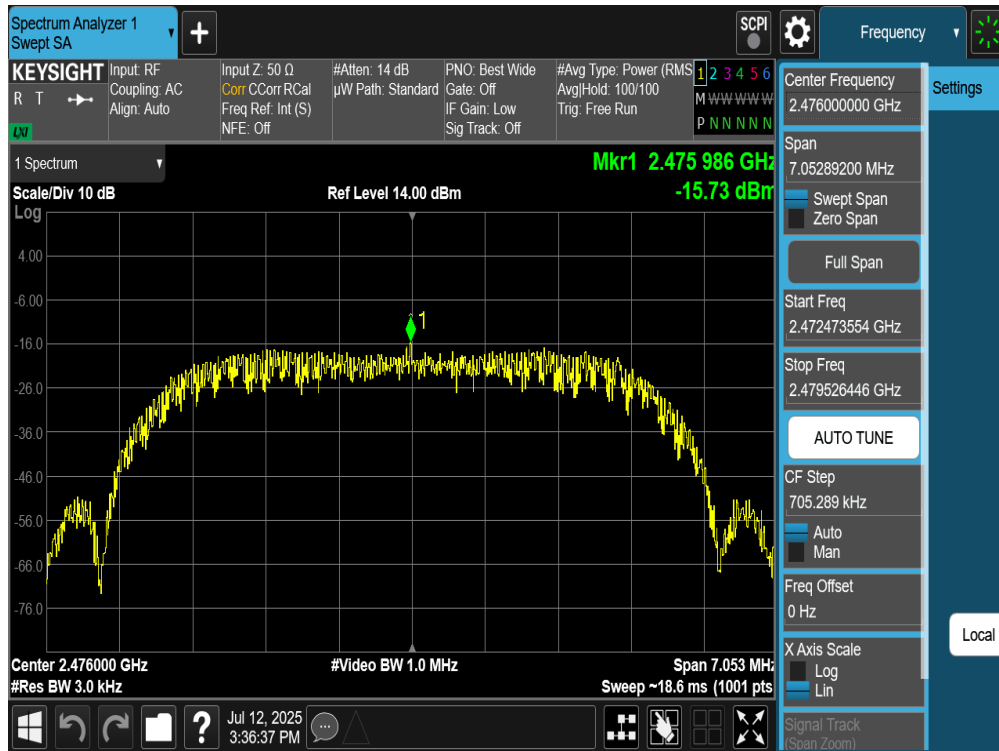
Plot 7-221. Power Spectral Density Plot TxBF Primary Antenna WF8 (Bluetooth (HDRPM16), 16Mbps, iPA – Ch. 73)
