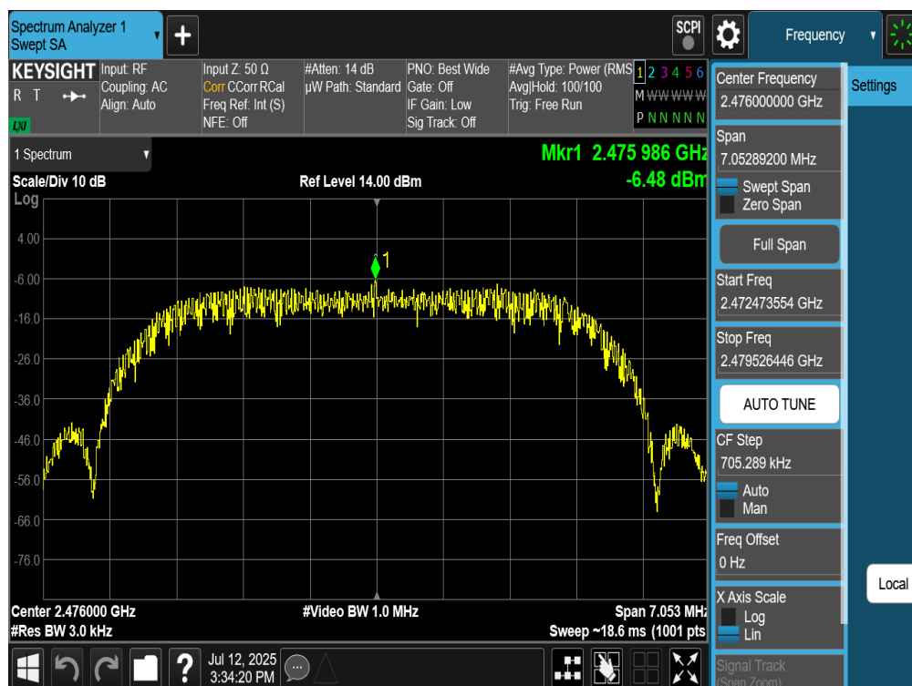
Plot 7-215. Power Spectral Density Plot Tx BF Primary Antenna WF8 (Bluetooth (HDRPM16), 16Mbps, ePA – Ch. 73)
