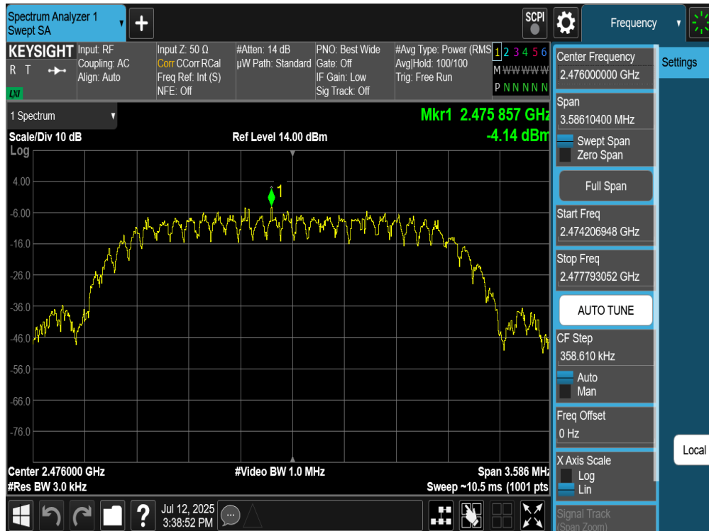
Plot 7-227. Power Spectral Density Plot TxBF Primary Antenna WF8 (Bluetooth (HDT2), 2Mbps, ePA – Ch. 73)
