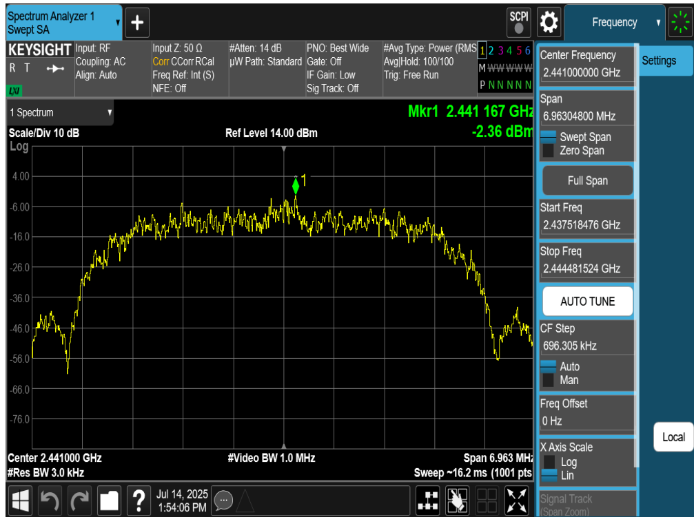
Plot 7-177. Power Spectral Density Plot TxBF Primary Antenna WF8 (Bluetooth (HDR8), 8Mbps, ePA – Ch. 38)
