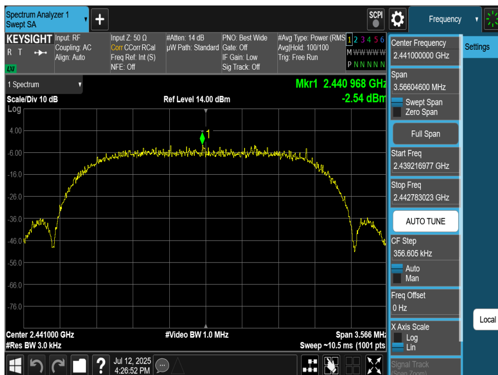
Plot 7-190. Power Spectral Density Plot Tx BF Primary Antenna WF7 (Bluetooth (HDRPS2), 2Mbps, ePA – Ch. 38)
