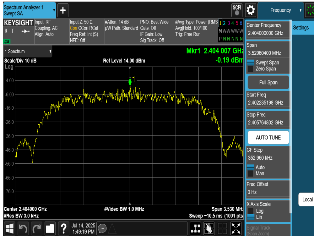
Plot 7-235. Power Spectral Density Plot Tx BF Diversity Antenna WF8 (Bluetooth (HDR4), 4Mbps, ePA – Ch. 1)
