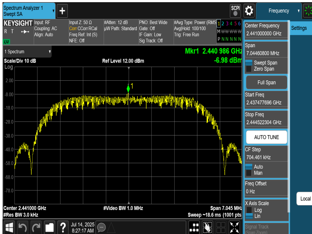
Plot 7-214. Power Spectral Density Plot Tx BF Primary Antenna WF7 (Bluetooth (HDRPM16), 16Mbps, ePA – Ch. 38)
