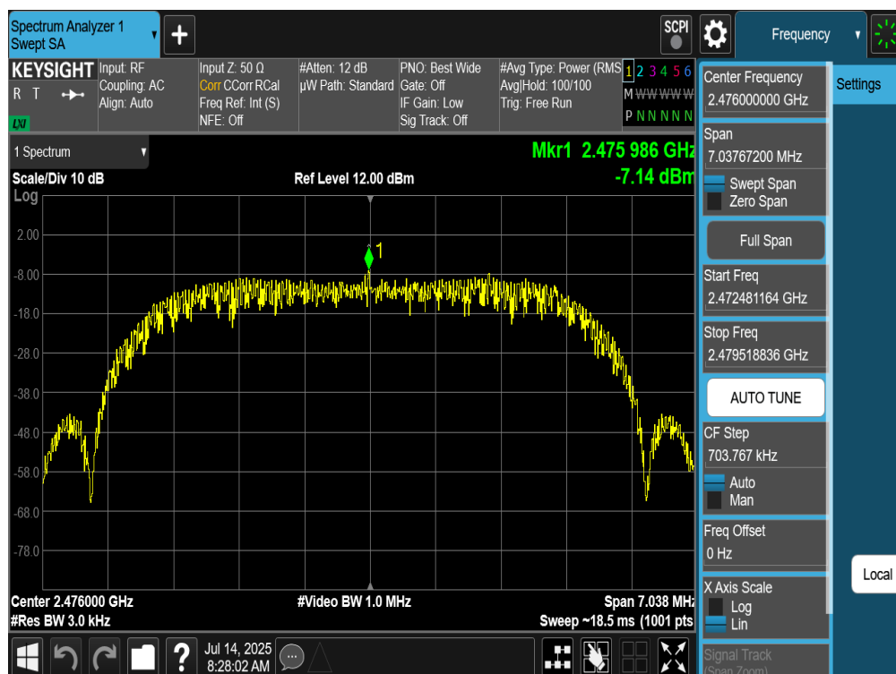
Plot 7-216. Power Spectral Density Plot Tx BF Primary Antenna WF7 (Bluetooth (HDRPM16), 16Mbps, ePA – Ch. 73)
