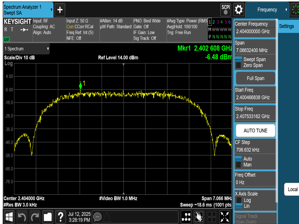
Plot 7-199. Power Spectral Density Plot Tx BF Primary Antenna WF8 (Bluetooth (XHDRPM6), 6Mbps, ePA – Ch. 1)
