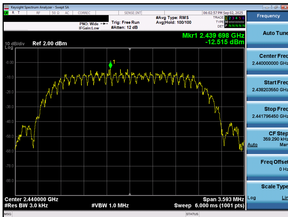
Plot 7-231. Power Spectral Density Plot TxBF Primary Antenna WF8 (Bluetooth (HDT2), 2Mbps, iPA – Ch. 37)
