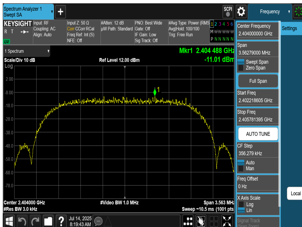
Plot 7-194. Power Spectral Density Plot Tx BF Primary Antenna WF7 (Bluetooth (HDRPS2), 2Mbps, iPA – Ch. 1)
