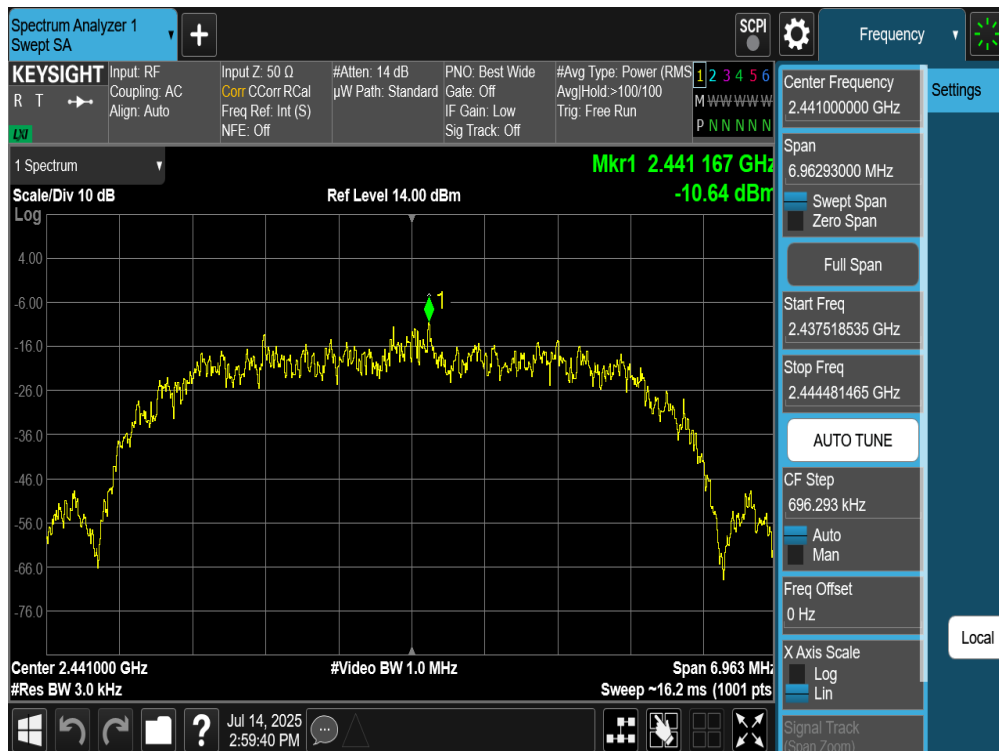
Plot 7-184. Power Spectral Density Plot TxBF Primary Antenna WF7 (Bluetooth (HDR8), 8Mbps, iPA – Ch. 38)
