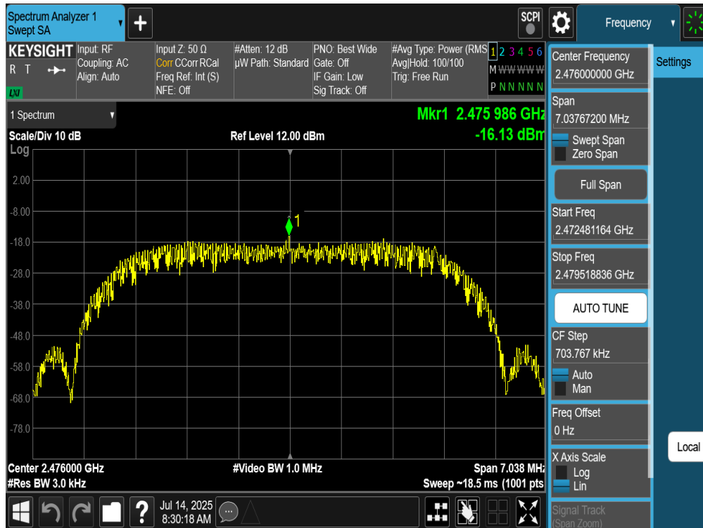
Plot 7-222. Power Spectral Density Plot TxBF Primary Antenna WF7 (Bluetooth (HDRPM16), 16Mbps, iPA – Ch. 73)
