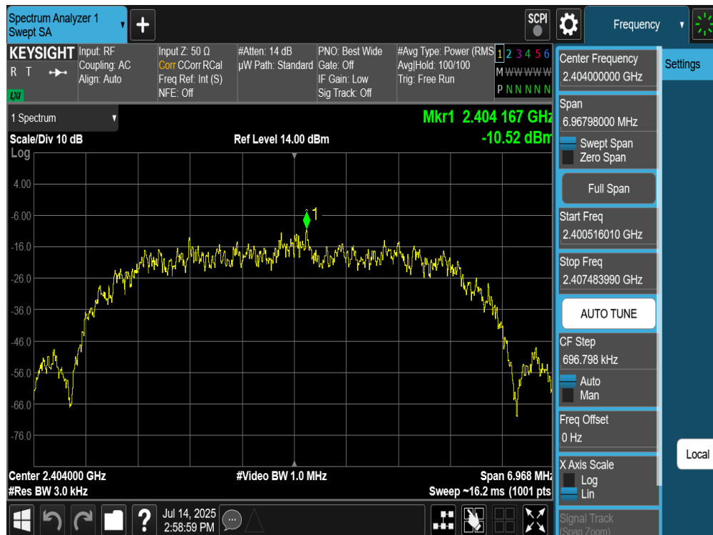
Plot 7-182. Power Spectral Density Plot Tx BF Primary Antenna WF7 (Bluetooth (HDR8), 8Mbps, iPA – Ch. 1)
