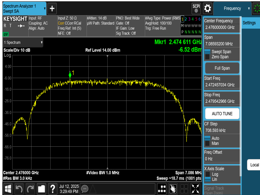
Plot 7-203. Power Spectral Density Plot TxBF Primary Antenna WF8 (Bluetooth (XHDRPM6), 6Mbps, ePA – Ch. 73)
