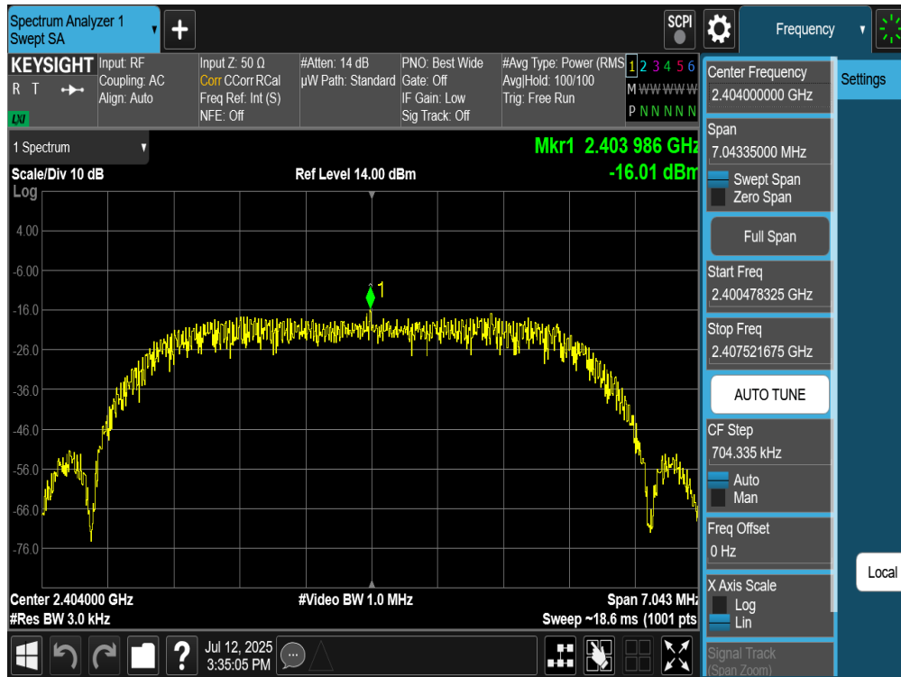
Plot 7-217. Power Spectral Density Plot Tx BF Primary Antenna WF8 (Bluetooth (HDRPM16), 16Mbps, iPA – Ch. 1)
