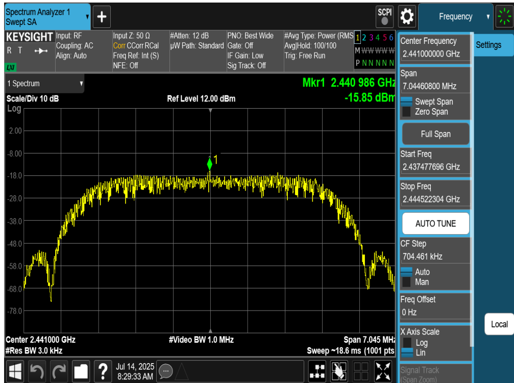
Plot 7-220. Power Spectral Density Plot TxBF Primary Antenna WF7 (Bluetooth (HDRPM16), 16Mbps, iPA – Ch. 38)
