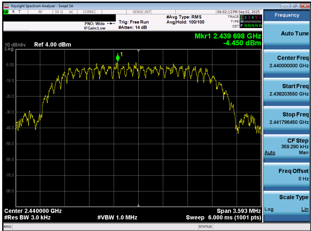
Plot 7-225. Power Spectral Density Plot TxBF Primary Antenna WF8 (Bluetooth (HDT2), 2Mbps, ePA – Ch. 37)
