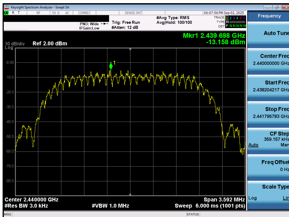
Plot 7-232. Power Spectral Density Plot TxBF Primary Antenna WF7 (Bluetooth (HDT2), 2Mbps, iPA – Ch. 37)
