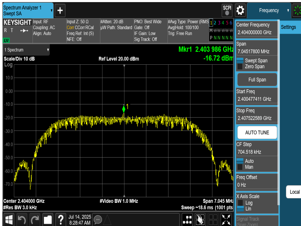
Plot 7-218. Power Spectral Density Plot Tx BF Primary Antenna WF7 (Bluetooth (HDRPM16), 16Mbps, iPA – Ch. 1)
