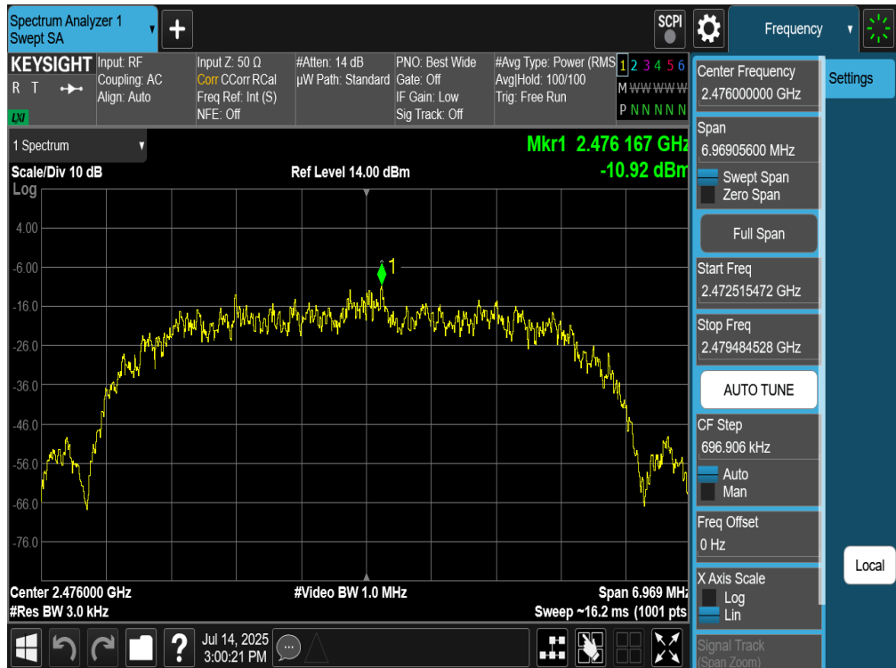
Plot 7-186. Power Spectral Density Plot TxBF Primary Antenna WF7 (Bluetooth (HDR8), 8Mbps, iPA – Ch. 73)
