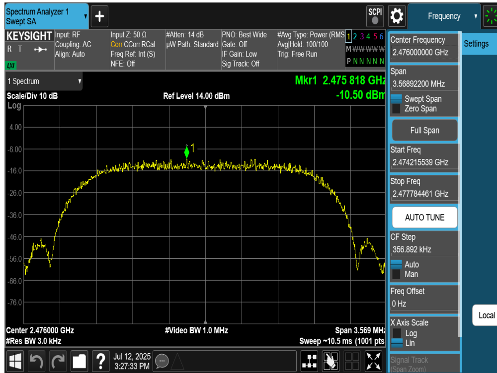
Plot 7-269. Power Spectral Density Plot Tx BF Diversity Antenna WF8 (Bluetooth (HDRPS2), 2Mbps, iPA – Ch. 73)
