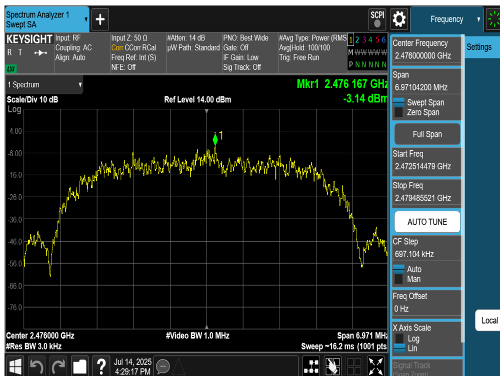
Plot 7-252. Power Spectral Density Plot Tx BF Diversity Antenna WF9 (Bluetooth (HDR8), 8Mbps, ePA – Ch. 73)
