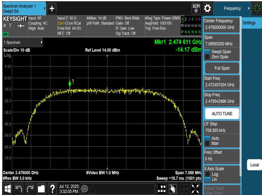
Plot 7-281. Power Spectral Density Plot TxBF Diversity Antenna WF8 (Bluetooth (XHDRPM6), 6Mbps, iPA – Ch. 73)
