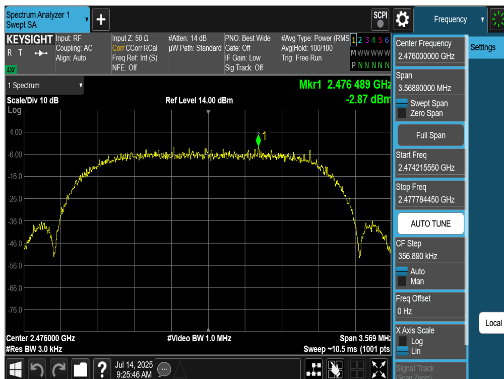
Plot 7-264. Power Spectral Density Plot TxBF Diversity Antenna WF9 (Bluetooth (HDRPS2), 2Mbps, ePA – Ch. 73)
