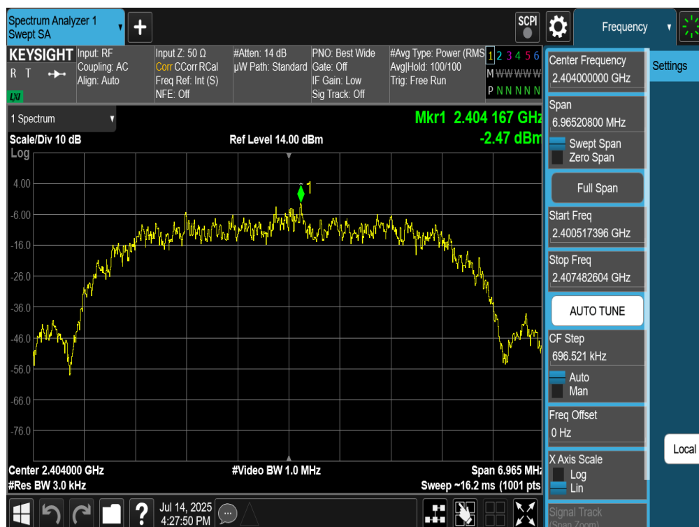
Plot 7-248. Power Spectral Density Plot TxBF Diversity Antenna WF9 (Bluetooth (HDR8), 8Mbps, ePA – Ch. 1)
