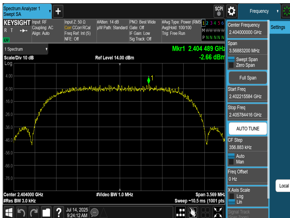
Plot 7-260. Power Spectral Density Plot Tx BF Diversity Antenna WF9 (Bluetooth (HDRPS2), 2Mbps, ePA – Ch. 1)
