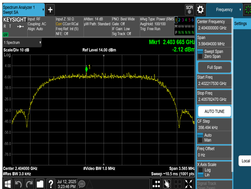
Plot 7-259. Power Spectral Density Plot Tx BF Diversity Antenna WF8 (Bluetooth (HDRPS2), 2Mbps, ePA – Ch. 1)
