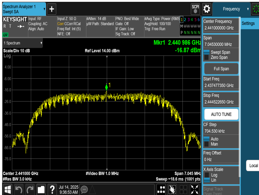
Plot 7-292. Power Spectral Density Plot Tx BF Diversity Antenna WF9 (Bluetooth (HDRPM16), 16Mbps, iPA – Ch. 38)
