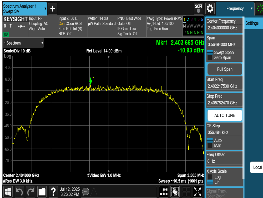
Plot 7-265. Power Spectral Density Plot TxBF Diversity Antenna WF8 (Bluetooth (HDRPS2), 2Mbps, iPA – Ch. 1)
