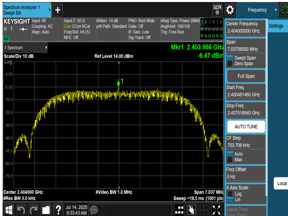
Plot 7-284. Power Spectral Density Plot Tx BF Diversity Antenna WF9 (Bluetooth (HDRPM16), 16Mbps, ePA – Ch. 1)
