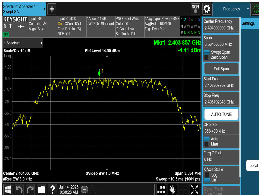
Plot 7-296. Power Spectral Density Plot TxBF Diversity Antenna WF9 (Bluetooth (HDT2), 2Mbps, ePA – Ch. 1)
