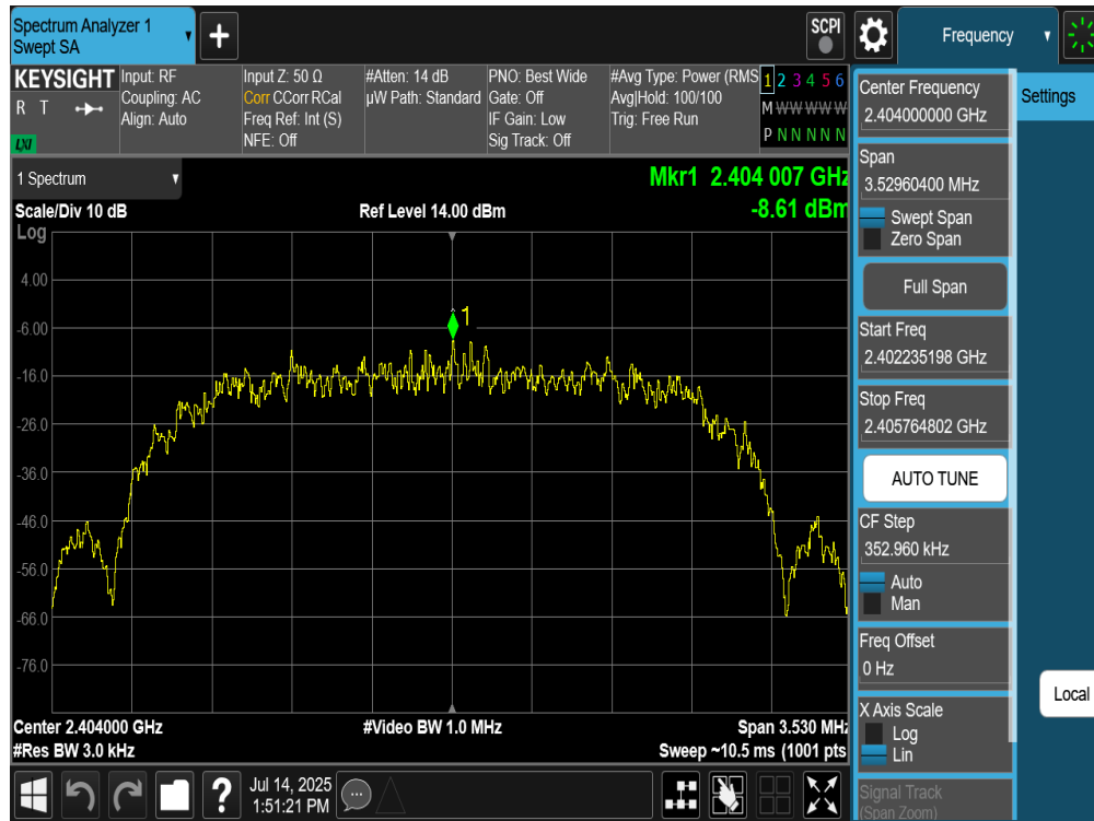
Plot 7-241. Power Spectral Density Plot TxBF Diversity Antenna WF8 (Bluetooth (HDR4), 4Mbps, iPA – Ch. 1)
