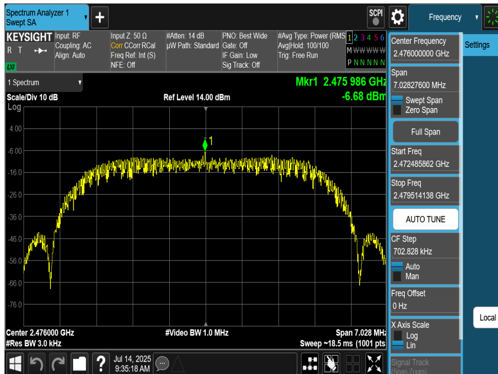
Plot 7-288. Power Spectral Density Plot Tx BF Diversity Antenna WF9 (Bluetooth (HDRPM16), 16Mbps, ePA – Ch. 73)
