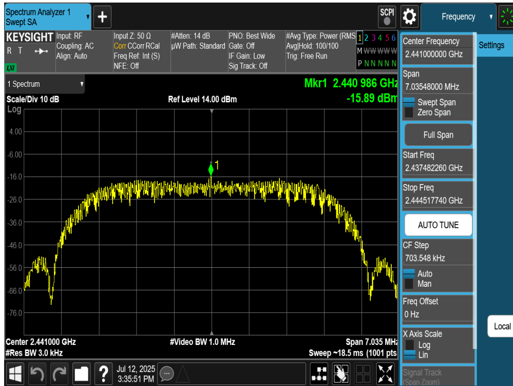
Plot 7-291. Power Spectral Density Plot Tx BF Diversity Antenna WF8 (Bluetooth (HDRPM16), 16Mbps, iPA – Ch. 38)
