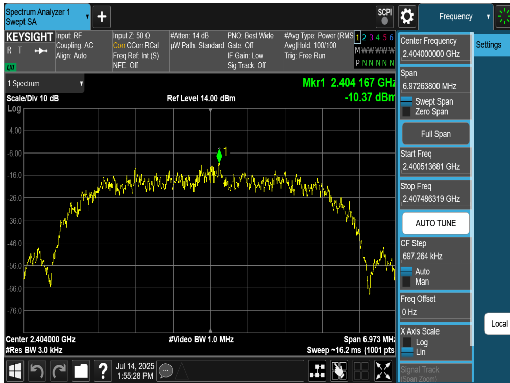
Plot 7-253. Power Spectral Density Plot TxBF Diversity Antenna WF8 (Bluetooth (HDR8), 8Mbps, iPA – Ch. 1)
