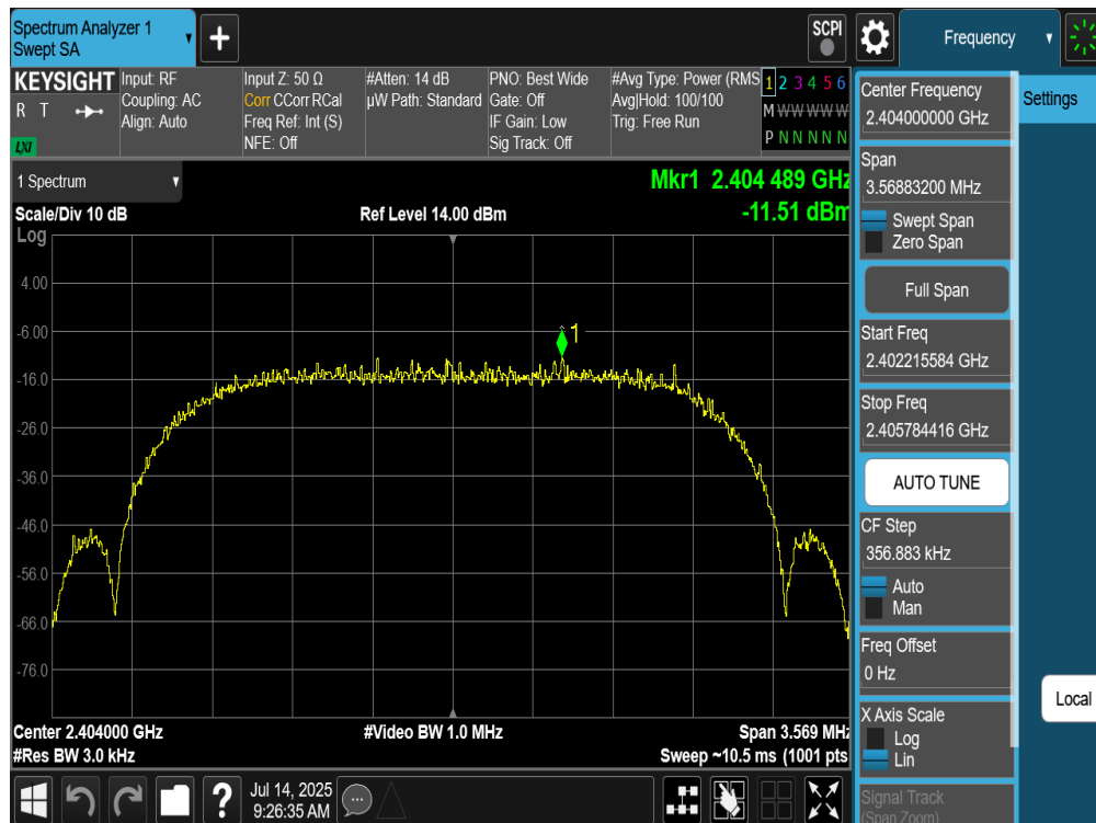
Plot 7-266. Power Spectral Density Plot TxBF Diversity Antenna WF9 (Bluetooth (HDRPS2), 2Mbps, iPA – Ch. 1)
