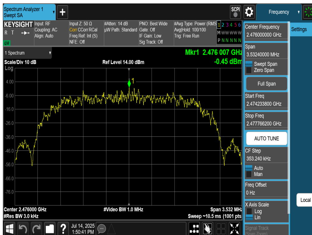
Plot 7-239. Power Spectral Density Plot Tx BF Diversity Antenna WF8 (Bluetooth (HDR4), 4Mbps, ePA – Ch. 73)
