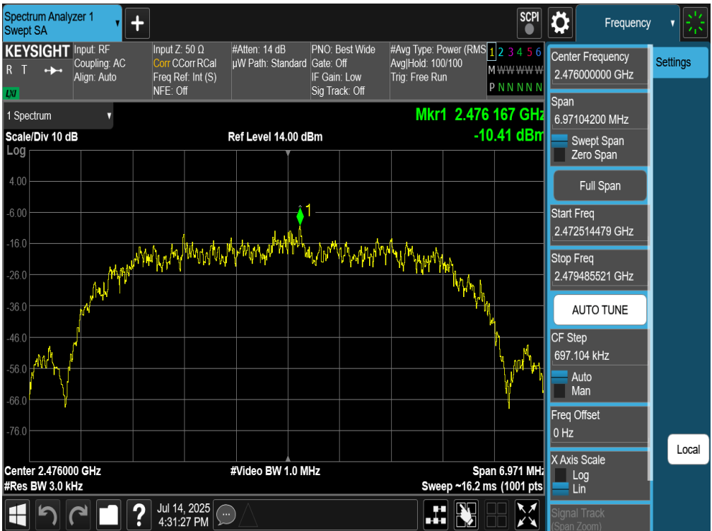
Plot 7-258. Power Spectral Density Plot Tx BF Diversity Antenna WF9 (Bluetooth (HDR8), 8Mbps, iPA – Ch. 73)
