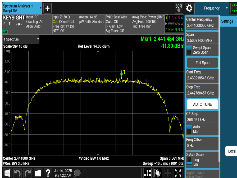
Plot 7-268. Power Spectral Density Plot Tx BF Diversity Antenna WF9 (Bluetooth (HDRPS2), 2Mbps, iPA – Ch. 38)
