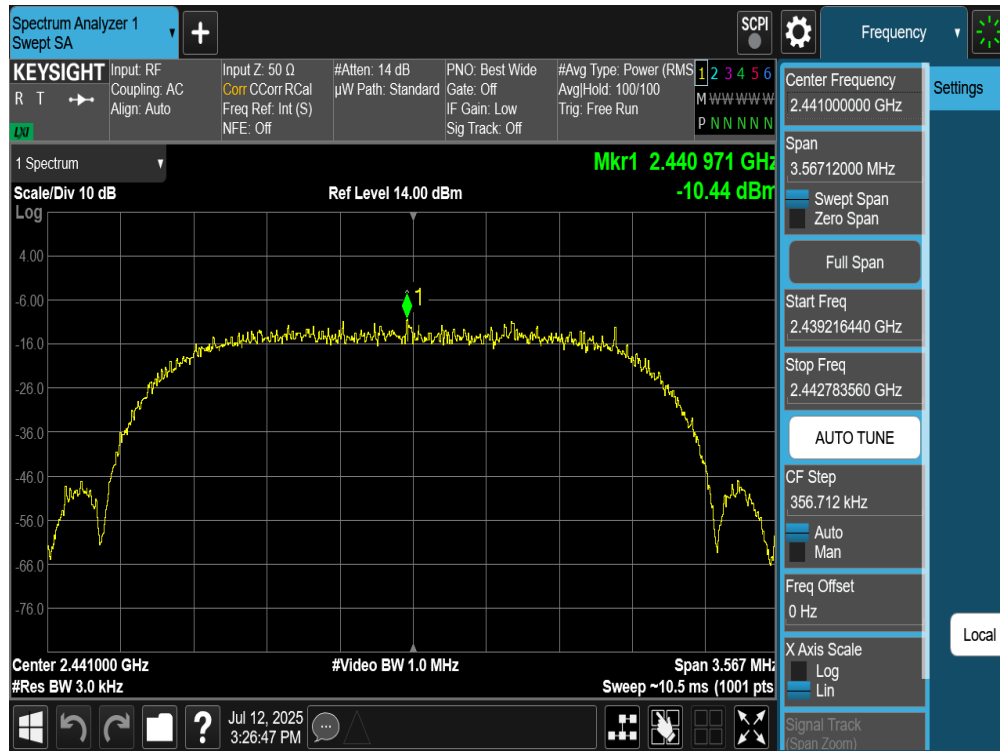
Plot 7-267. Power Spectral Density Plot Tx BF Diversity Antenna WF8 (Bluetooth (HDRPS2), 2Mbps, iPA – Ch. 38)
