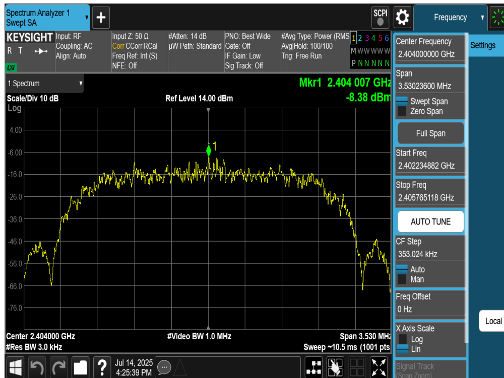
Plot 7-242. Power Spectral Density Plot TxBF Diversity Antenna WF9 (Bluetooth (HDR4), 4Mbps, iPA – Ch. 1)
