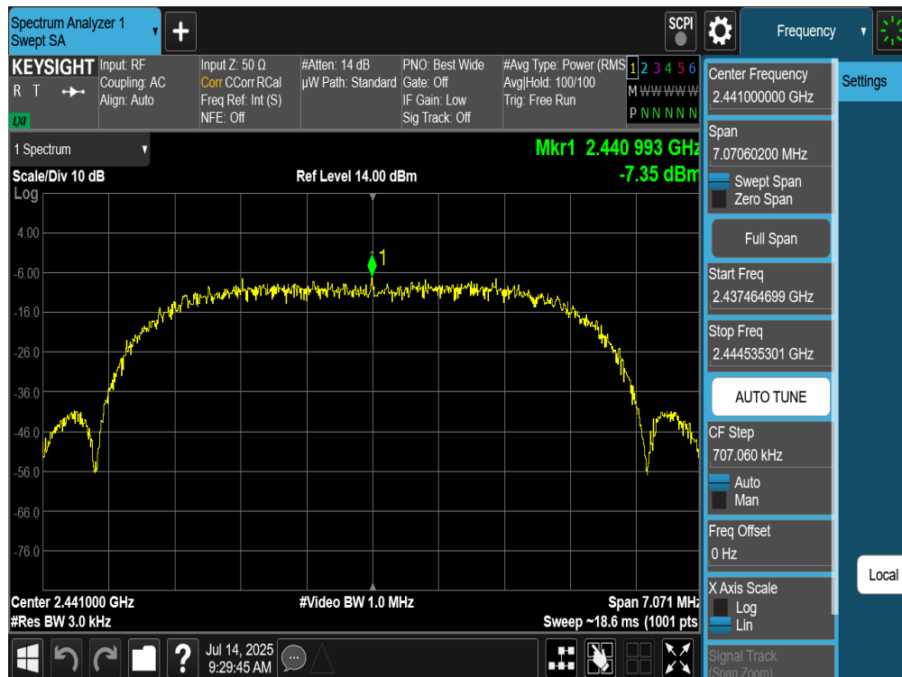
Plot 7-274. Power Spectral Density Plot TxBF Diversity Antenna WF9 (Bluetooth (XHDRPM6), 6Mbps, ePA – Ch. 38)
