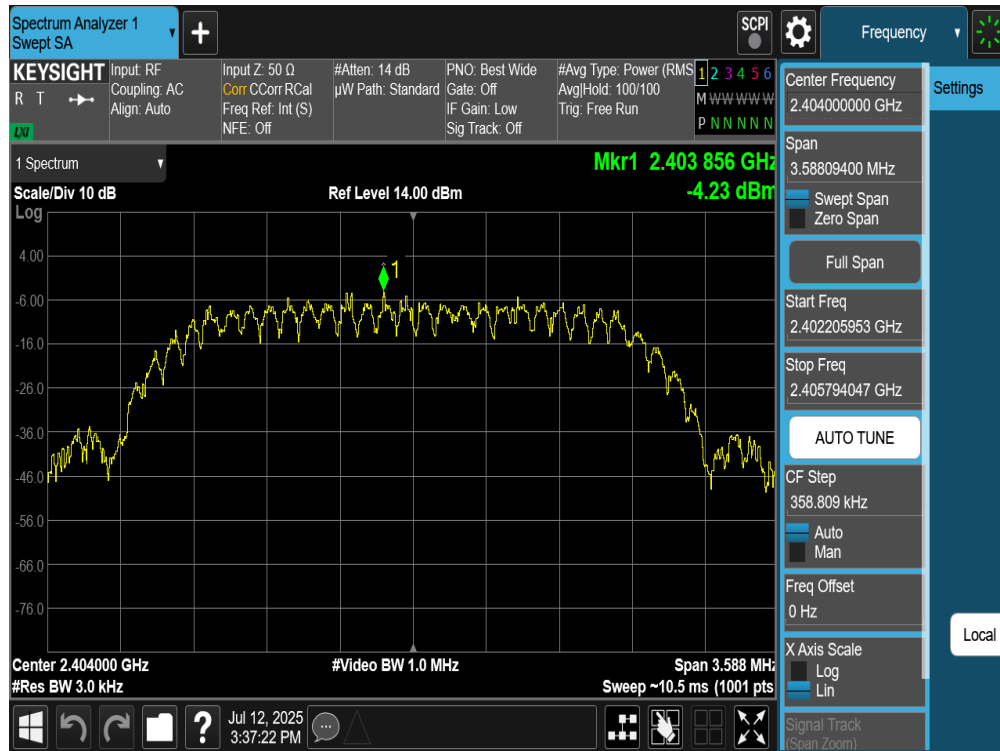
Plot 7-295. Power Spectral Density Plot TxBF Diversity Antenna WF8 (Bluetooth (HDT2), 2Mbps, ePA – Ch. 1)
