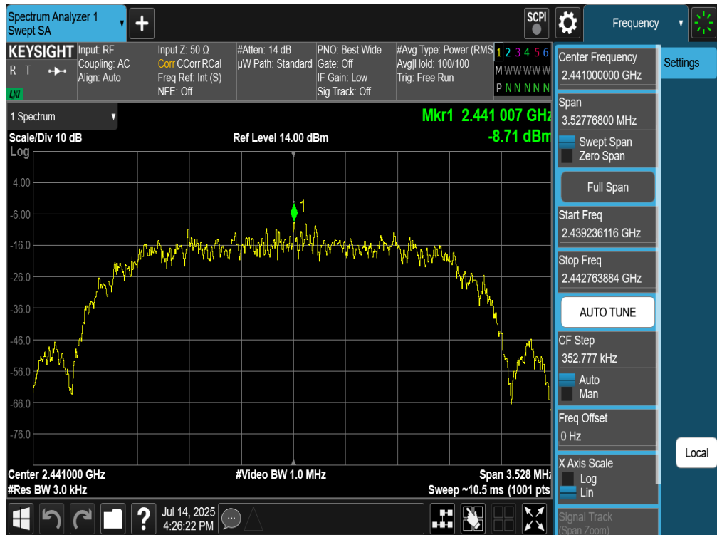
Plot 7-244. Power Spectral Density Plot Tx BF Diversity Antenna WF9 (Bluetooth (HDR4), 4Mbps, iPA – Ch. 38)
