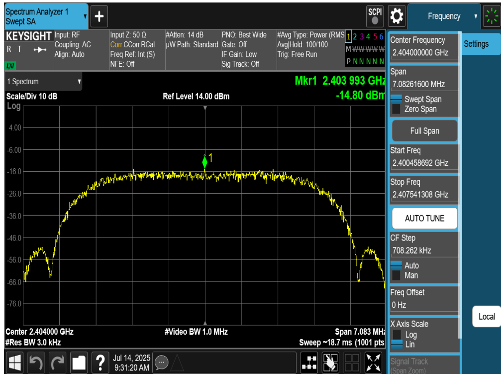
Plot 7-278. Power Spectral Density Plot TxBF Diversity Antenna WF9 (Bluetooth (XHDRPM6), 6Mbps, iPA – Ch. 1)
