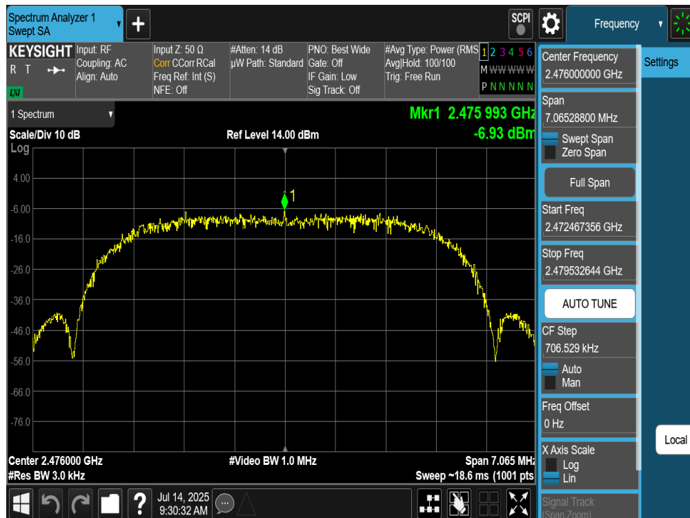
Plot 7-276. Power Spectral Density Plot Tx BF Diversity Antenna WF9 (Bluetooth (XHDRPM6), 6Mbps, ePA – Ch. 73)
