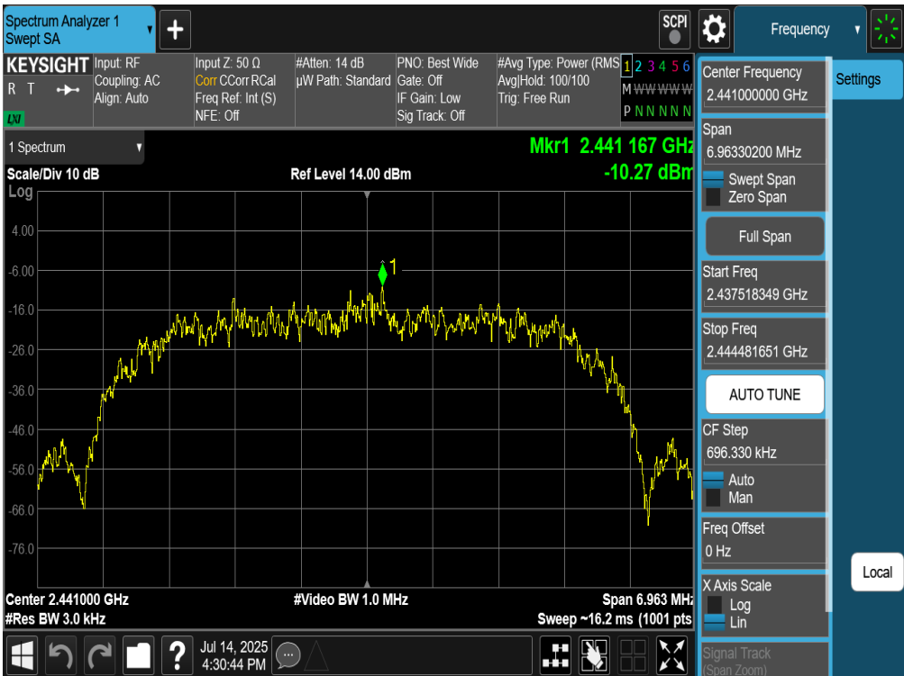
Plot 7-256. Power Spectral Density Plot Tx BF Diversity Antenna WF9 (Bluetooth (HDR8), 8Mbps, iPA – Ch. 38)
