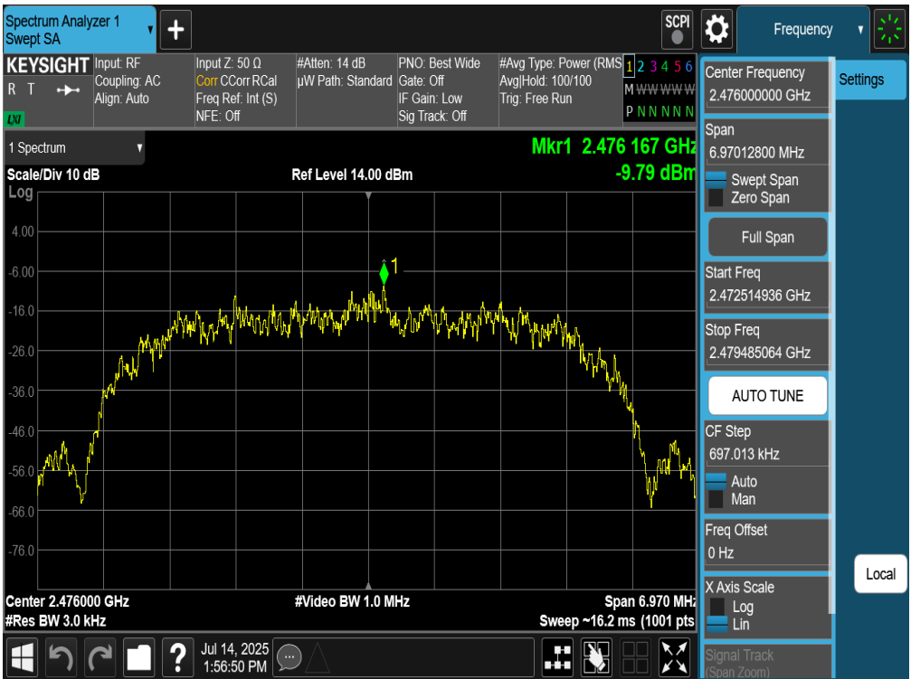
Plot 7-257. Power Spectral Density Plot Tx BF Diversity Antenna WF8 (Bluetooth (HDR8), 8Mbps, iPA – Ch. 73)
