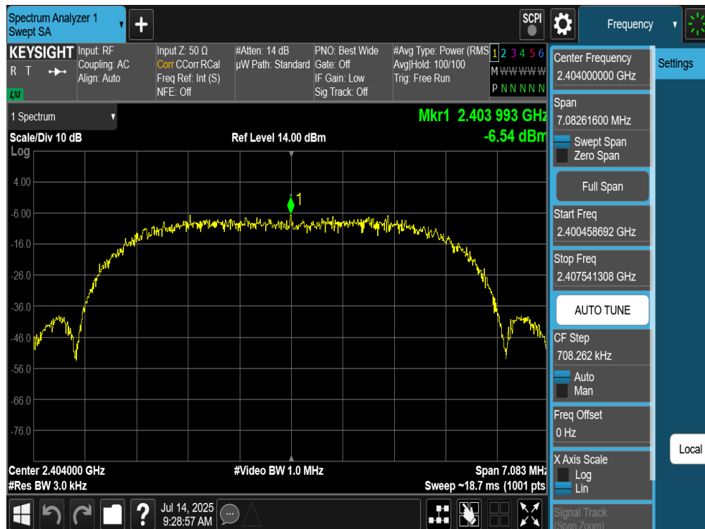
Plot 7-272. Power Spectral Density Plot Tx BF Diversity Antenna WF9 (Bluetooth (XHDRPM6), 6Mbps, ePA – Ch. 1)
