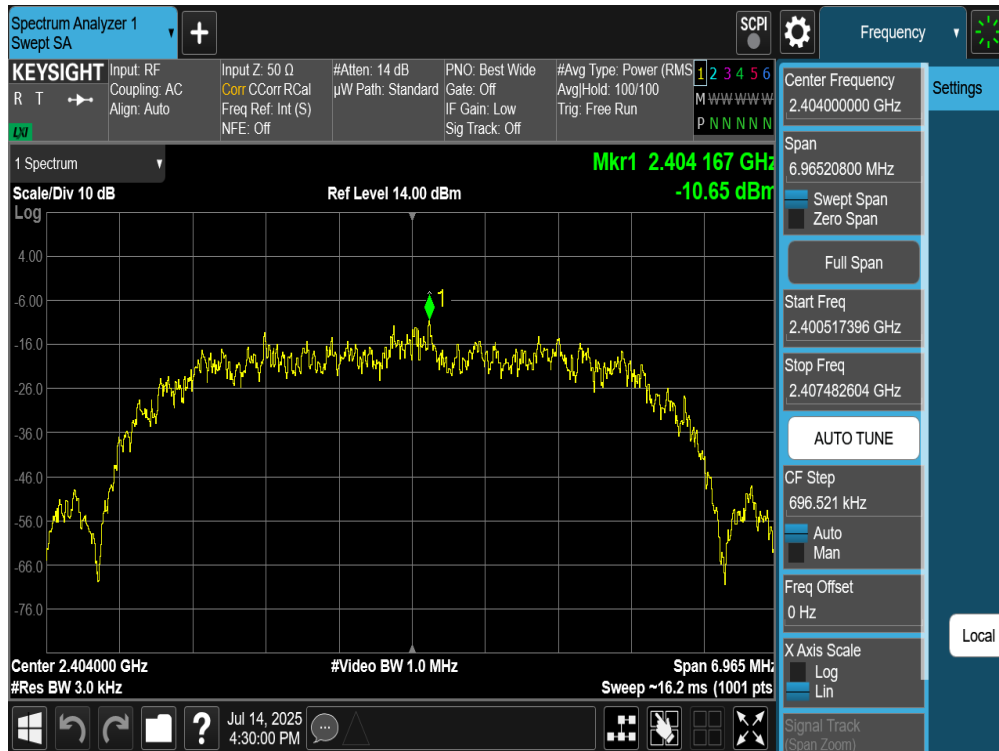
Plot 7-254. Power Spectral Density Plot TxBF Diversity Antenna WF9 (Bluetooth (HDR8), 8Mbps, iPA – Ch. 1)
