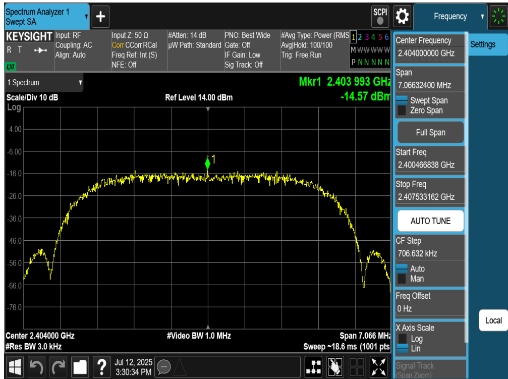
Plot 7-277. Power Spectral Density Plot TxBF Diversity Antenna WF8 (Bluetooth (XHDRPM6), 6Mbps, iPA – Ch. 1)
