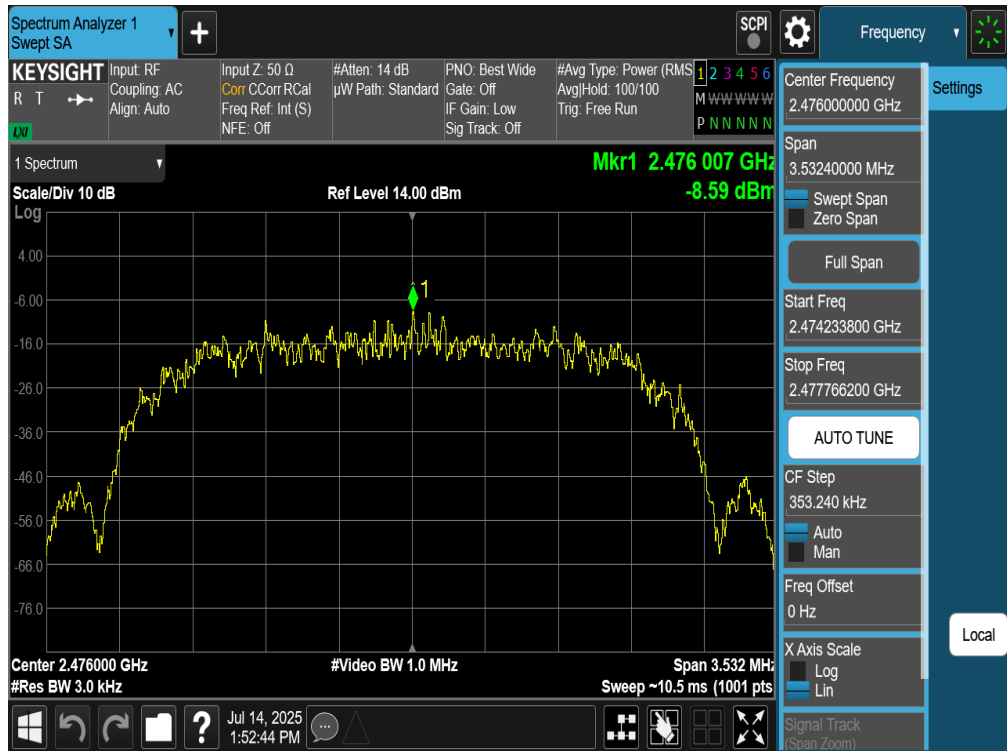
Plot 7-245. Power Spectral Density Plot TxBF Diversity Antenna WF8 (Bluetooth (HDR4), 4Mbps, iPA – Ch. 73)
