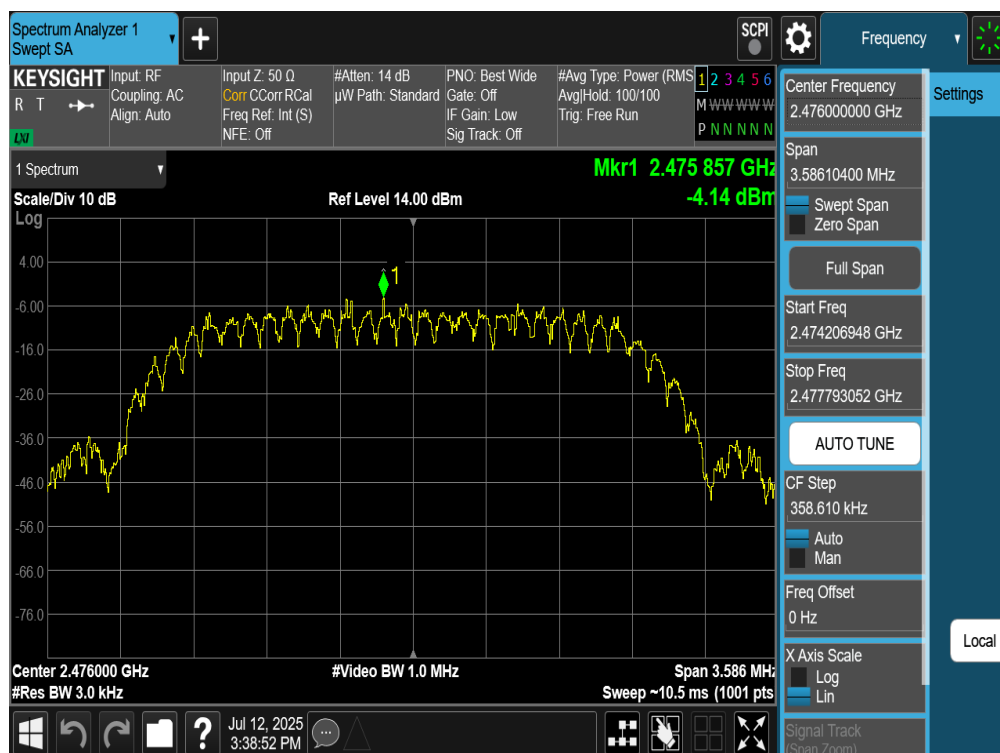
Plot 7-299. Power Spectral Density Plot Tx BF Diversity Antenna WF8 (Bluetooth (HDT2), 2Mbps, ePA – Ch. 73)
