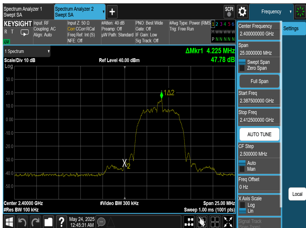
Plot 7-309. Band Edge Plot Antenna WF8 (Bluetooth (HDR8), ePA – Ch. 1)
