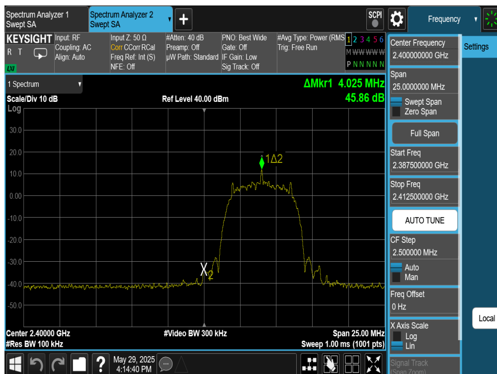
Plot 7-327. Band Edge Plot Antenna WF7 (Bluetooth (HDRPM16), 16Mbps, ePA – Ch. 1)
