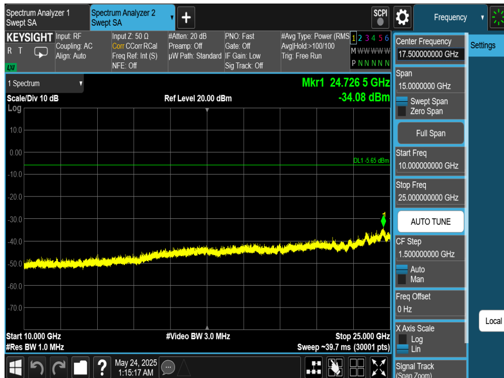
Plot 7-348. Conducted Spurious Plot Antenna WF8 (Bluetooth (HDR4), 4 Mbps, ePA – Ch. 73)
