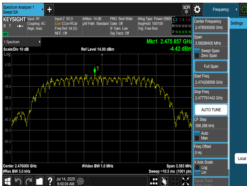
Plot 7-300. Power Spectral Density Plot Tx BF Diversity Antenna WF9 (Bluetooth (HDT2), 2Mbps, ePA – Ch. 73)
