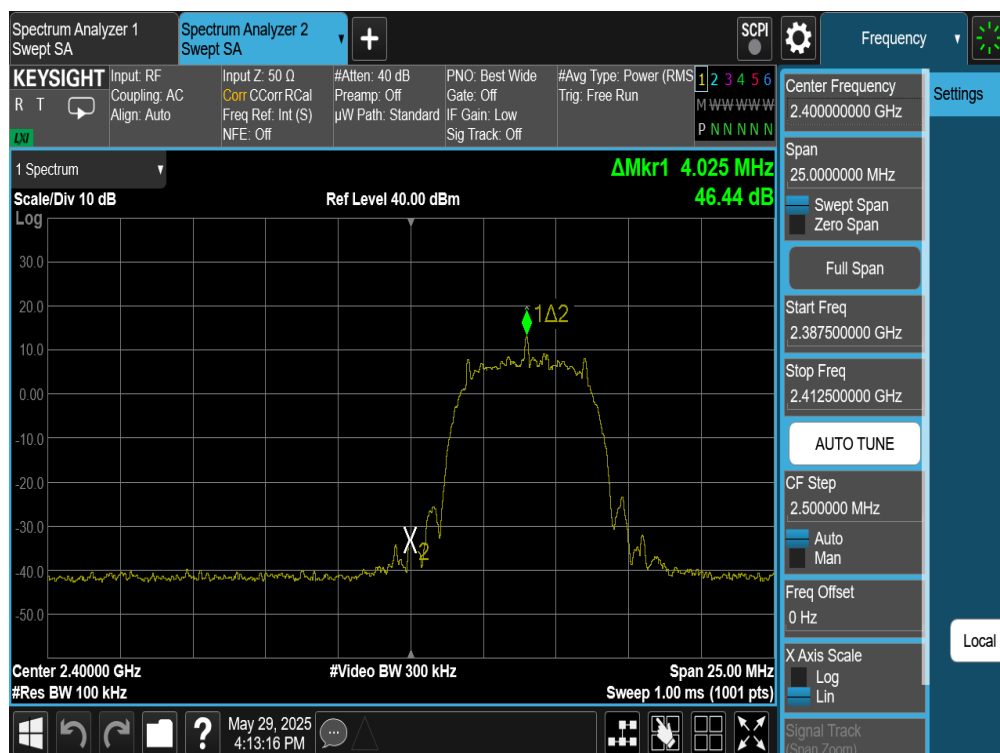
Plot 7-325. Band Edge Plot Antenna WF7 (Bluetooth (XHDRPM6), 6Mbps, ePA – Ch. 1)
