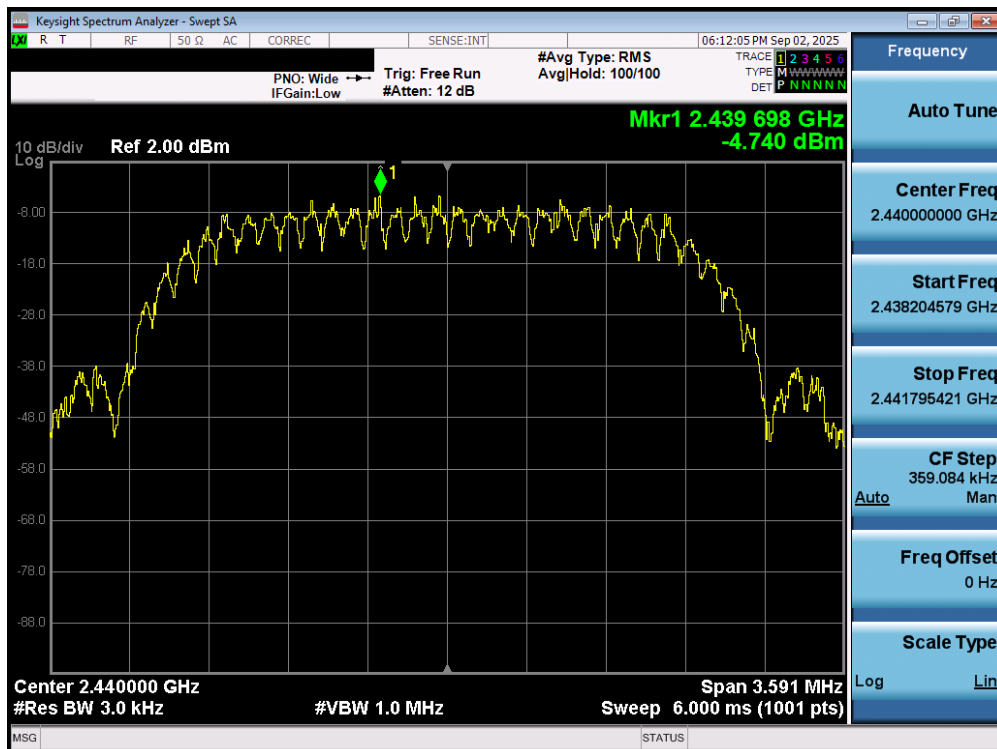
Plot 7-298. Power Spectral Density Plot Tx BF Diversity Antenna WF9 (Bluetooth (HDT2), 2Mbps, ePA – Ch. 37)
