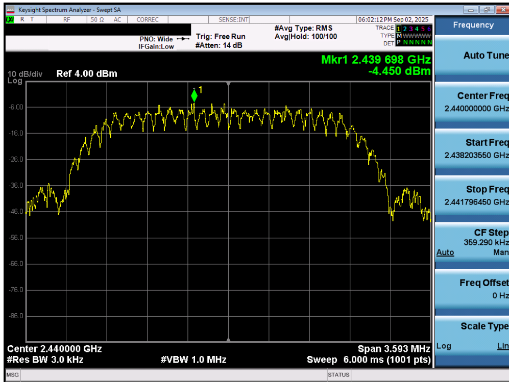
Plot 7-297. Power Spectral Density Plot Tx BF Diversity Antenna WF8 (Bluetooth (HDT2), 2Mbps, ePA – Ch. 37)
