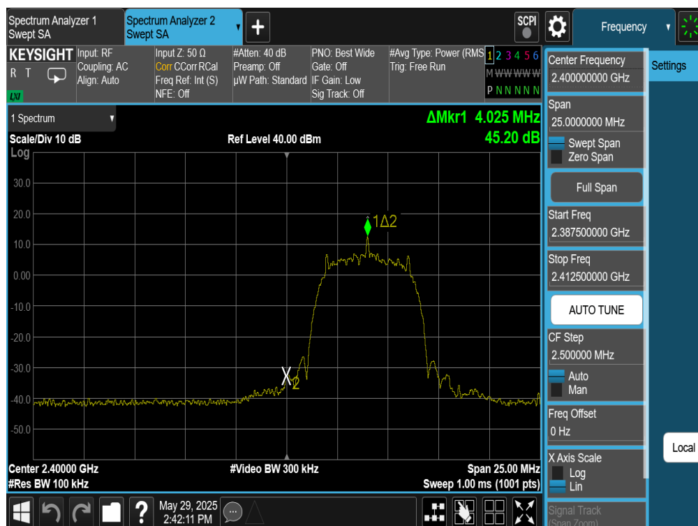
Plot 7-315. Band Edge Plot Antenna WF8 (Bluetooth (HDRPM16), 16Mbps, ePA – Ch. 1)
