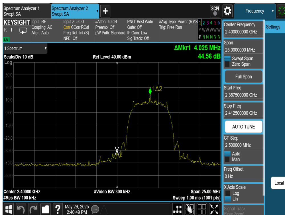
Plot 7-313. Band Edge Plot Antenna WF8 (Bluetooth (XHDRPM6), 6Mbps, ePA – Ch. 1)
