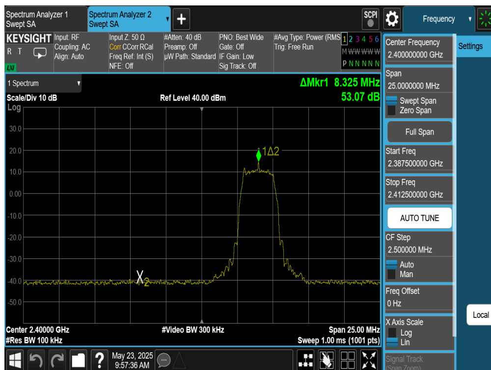
Plot 7-311. Band Edge Plot Antenna WF8 (Bluetooth (HDRPS2), 8Mbps, ePA – Ch. 1)
