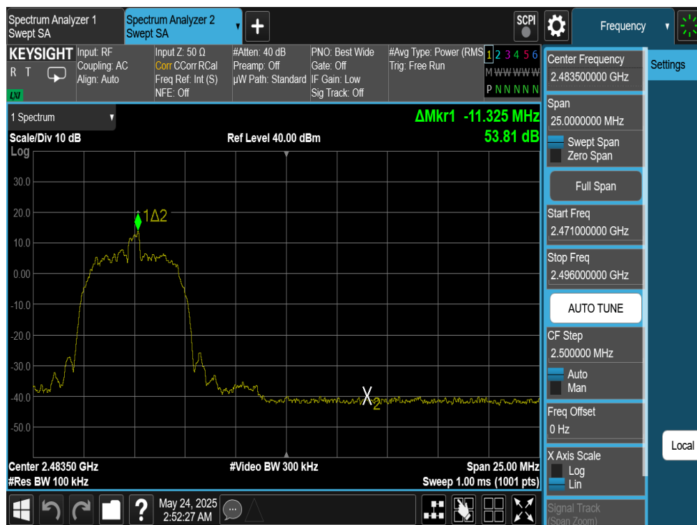
Plot 7-322. Band Edge Plot Antenna WF7 (Bluetooth (HDR8), ePA – Ch. 73)
