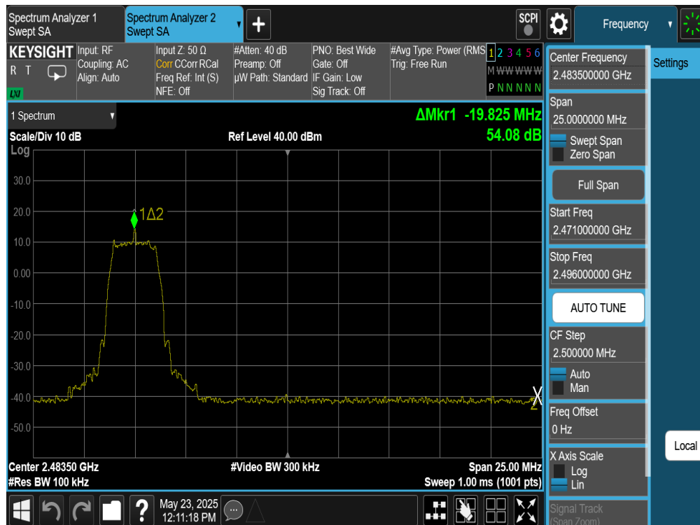
Plot 7-324. Band Edge Plot Antenna WF7 (Bluetooth (HDRPS2), 8Mbps, ePA – Ch. 73)
