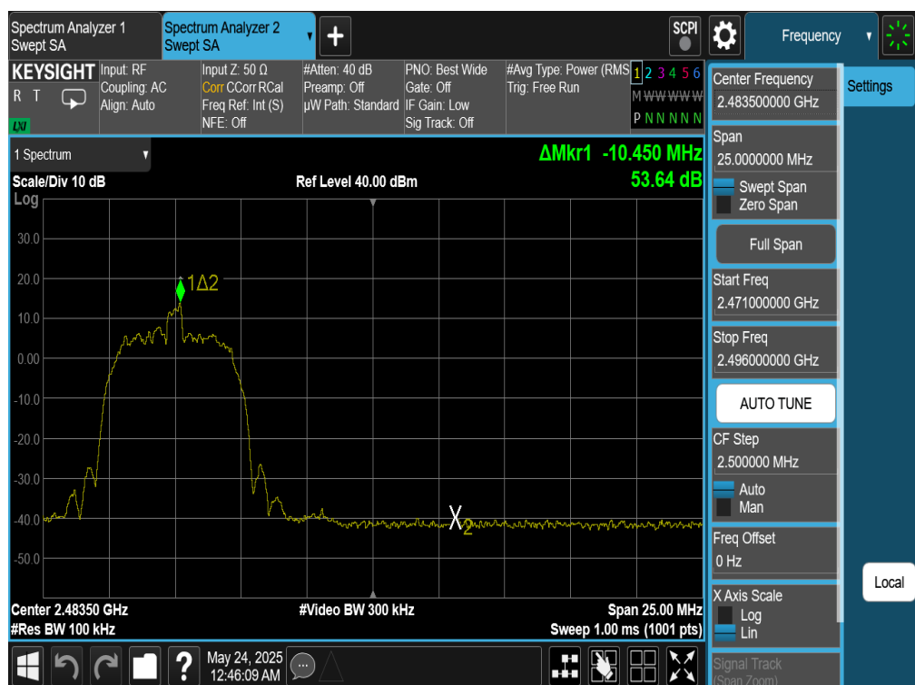
Plot 7-310. Band Edge Plot Antenna WF8 (Bluetooth (HDR8), ePA – Ch. 73)
