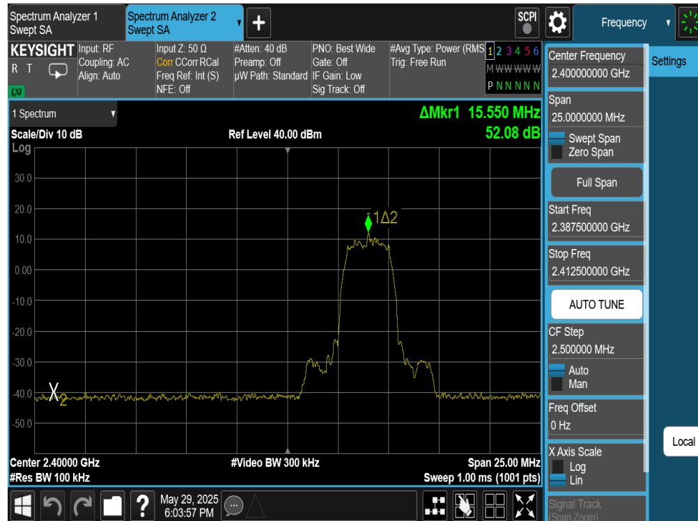
Plot 7-341. Band Edge Plot Antenna WF9 (Bluetooth (HDT2), 2Mbps, ePA – Ch. 1)
