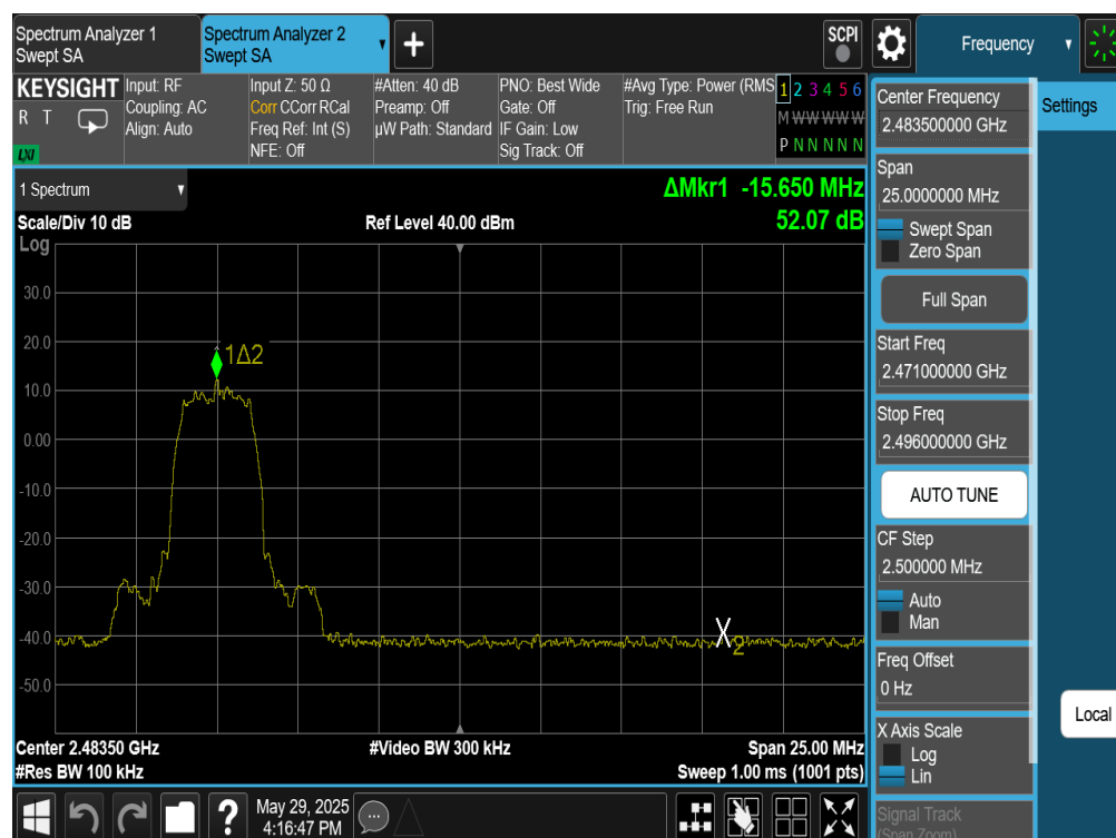
Plot 7-330. Band Edge Plot Antenna WF7 (Bluetooth (HDT2), 2Mbps, ePA – Ch. 73)
