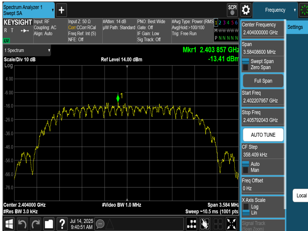
Plot 7-302. Power Spectral Density Plot TxBF Diversity Antenna WF9 (Bluetooth (HDT2), 2Mbps, iPA – Ch. 1)
