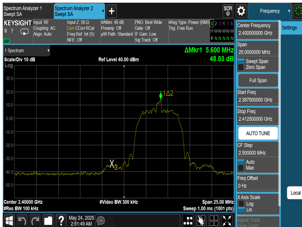
Plot 7-321. Band Edge Plot Antenna WF7 (Bluetooth (HDR8), ePA – Ch. 1)
