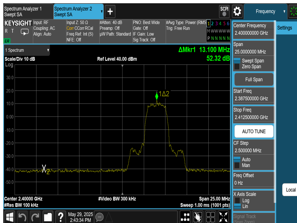
Plot 7-317. Band Edge Plot Antenna WF8 (Bluetooth (HDT2), 2Mbps, ePA – Ch. 1)
