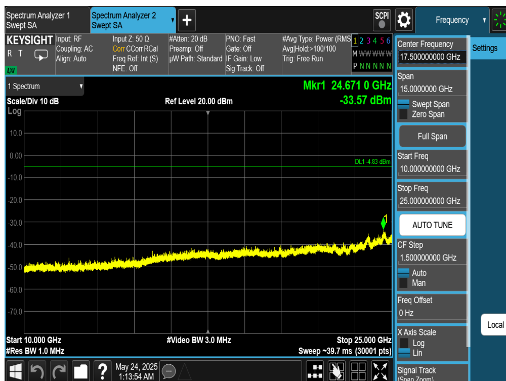
Plot 7-346. Conducted Spurious Plot Antenna WF8 (Bluetooth (HDR4), 4 Mbps, ePA – Ch. 38)
