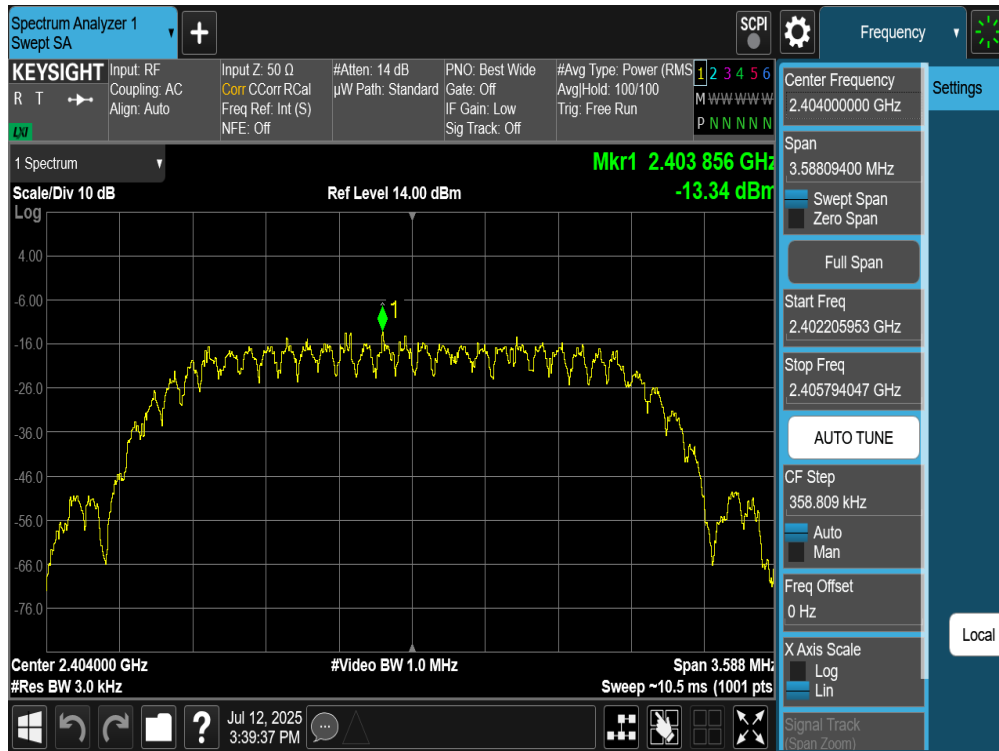
Plot 7-301. Power Spectral Density Plot TxBF Diversity Antenna WF8 (Bluetooth (HDT2), 2Mbps, iPA – Ch. 1)
