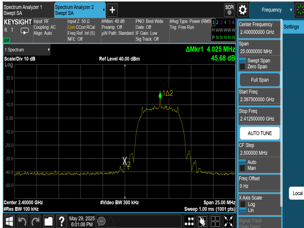
Plot 7-337. Band Edge Plot Antenna WF9 (Bluetooth (XHDRPM6), 6Mbps, ePA – Ch. 1)
