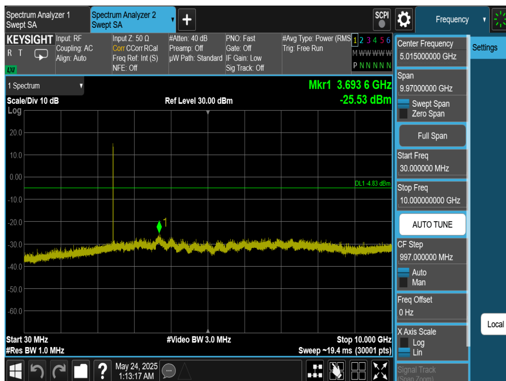
Plot 7-345. Conducted Spurious Plot Antenna WF8 (Bluetooth (HDR4), 4 Mbps, ePA – Ch. 38)
