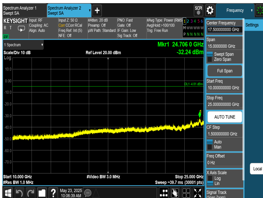
Plot 7-350. Conducted Spurious Plot Antenna WF8 (Bluetooth (HDRPS2), 2Mbps, ePA – Ch. 1)
