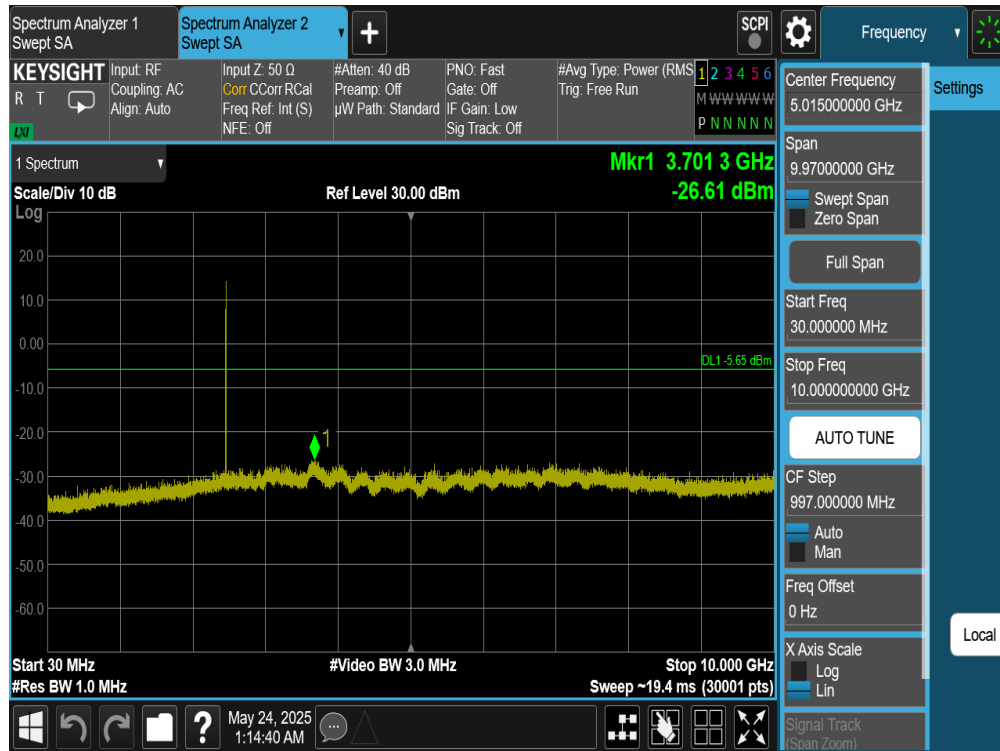
Plot 7-347. Conducted Spurious Plot Antenna WF8 (Bluetooth (HDR4), 4 Mbps, ePA – Ch. 73)
