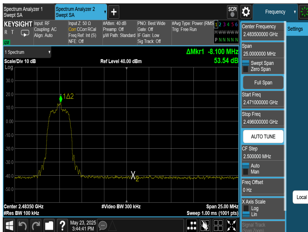
Plot 7-332. Band Edge Plot Antenna WF9 (Bluetooth (HDR4), ePA – Ch. 73)
