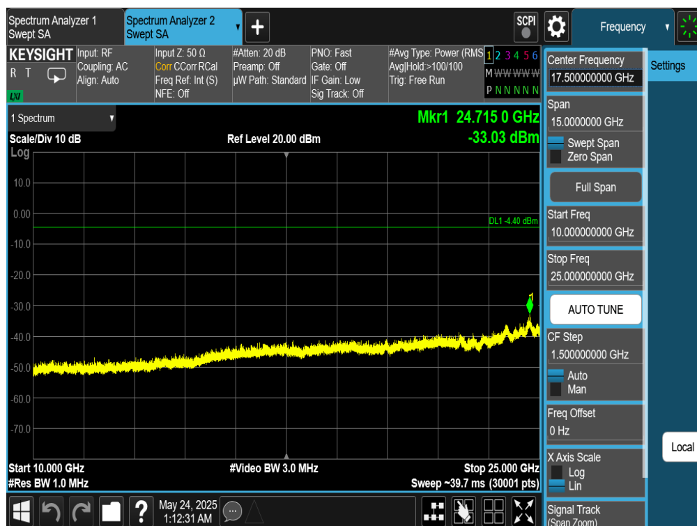
Plot 7-344. Conducted Spurious Plot Antenna WF8 (Bluetooth (HDR4), 4 Mbps, ePA – Ch. 1)
