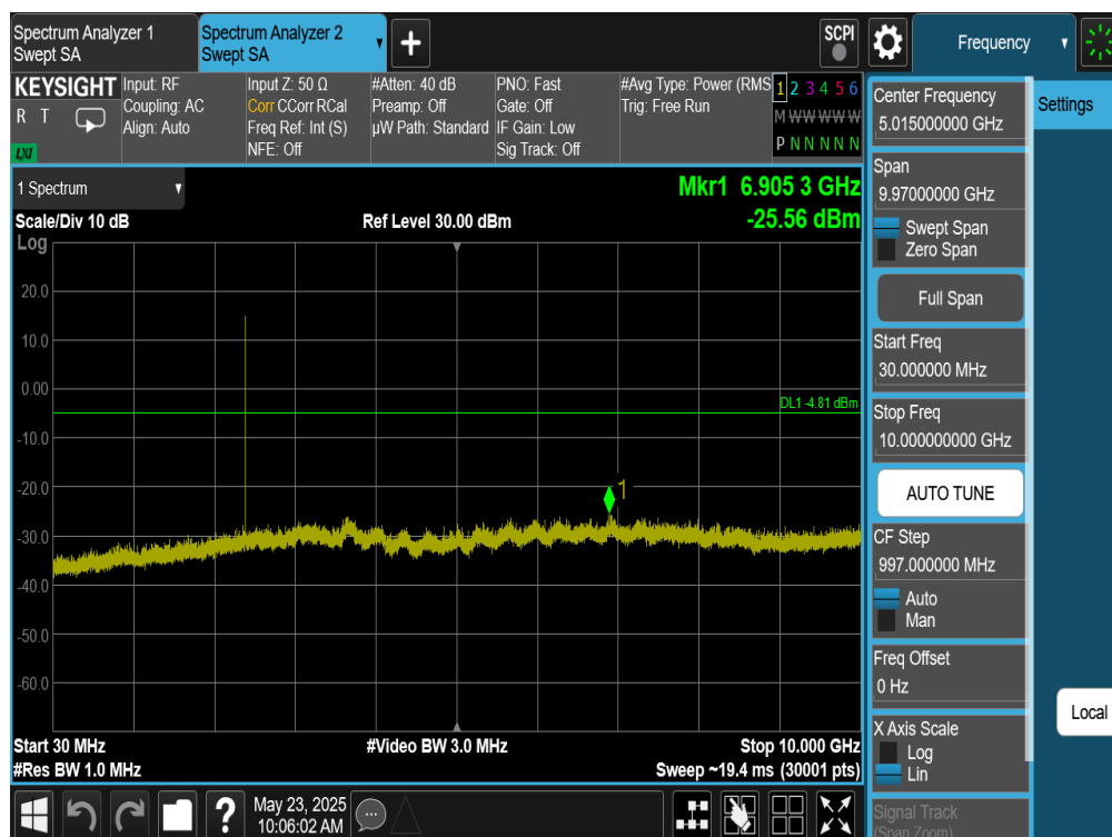
Plot 7-349. Conducted Spurious Plot Antenna WF8 (Bluetooth (HDRPS2), 2Mbps, ePA – Ch. 1)
