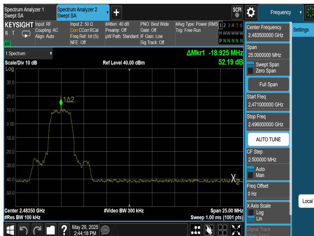
Plot 7-318. Band Edge Plot Antenna WF8 (Bluetooth (HDT2), 2Mbps, ePA – Ch. 73)
