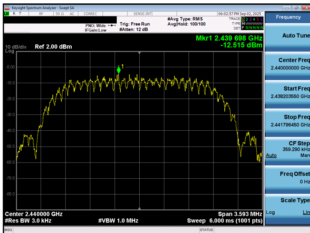
Plot 7-303. Power Spectral Density Plot TxBF Diversity Antenna WF8 (Bluetooth (HDT2), 2Mbps, iPA – Ch. 37)
