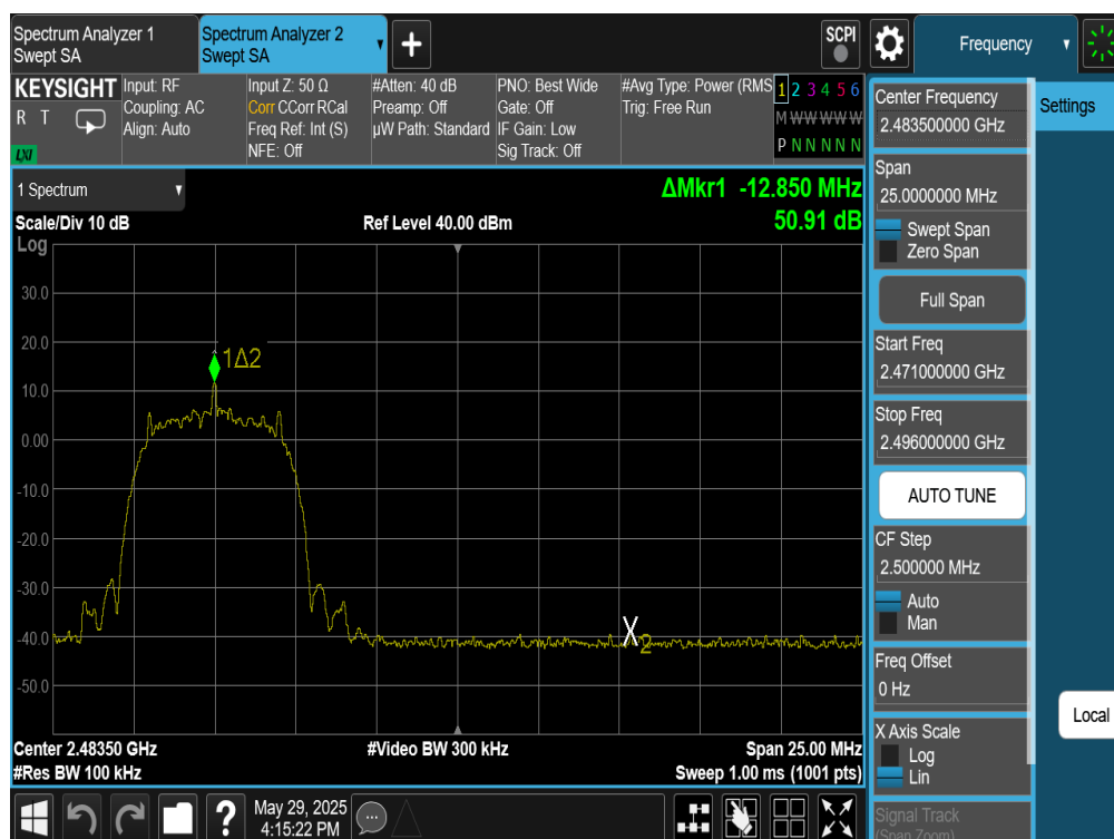
Plot 7-328. Band Edge Plot Antenna WF7 (Bluetooth (HDRPM16), 16Mbps, ePA – Ch. 73)
