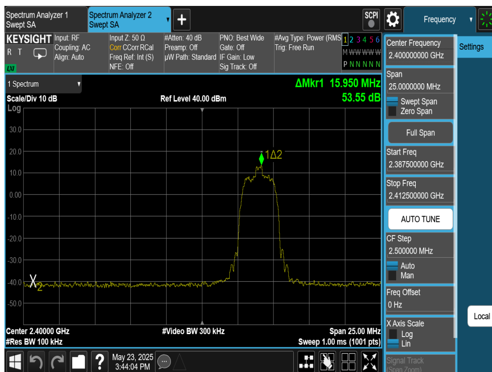
Plot 7-331. Band Edge Plot Antenna WF9 (Bluetooth (HDR4), ePA – Ch. 1)
