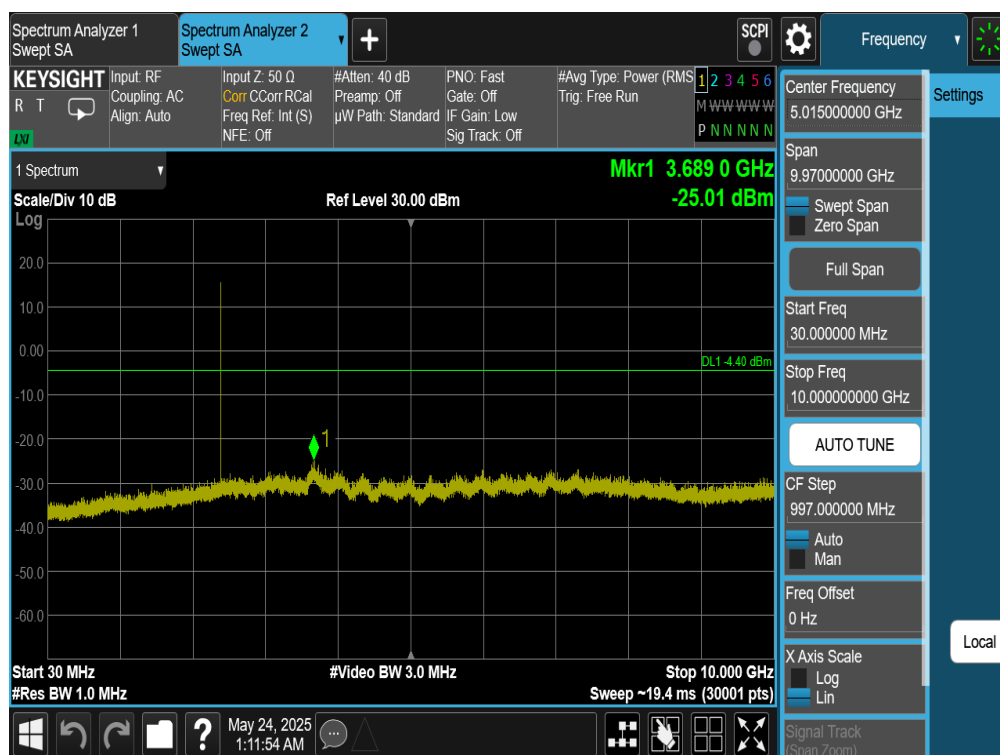
Plot 7-343. Conducted Spurious Plot Antenna WF8 (Bluetooth (HDR4), 4 Mbps, ePA – Ch. 1)
