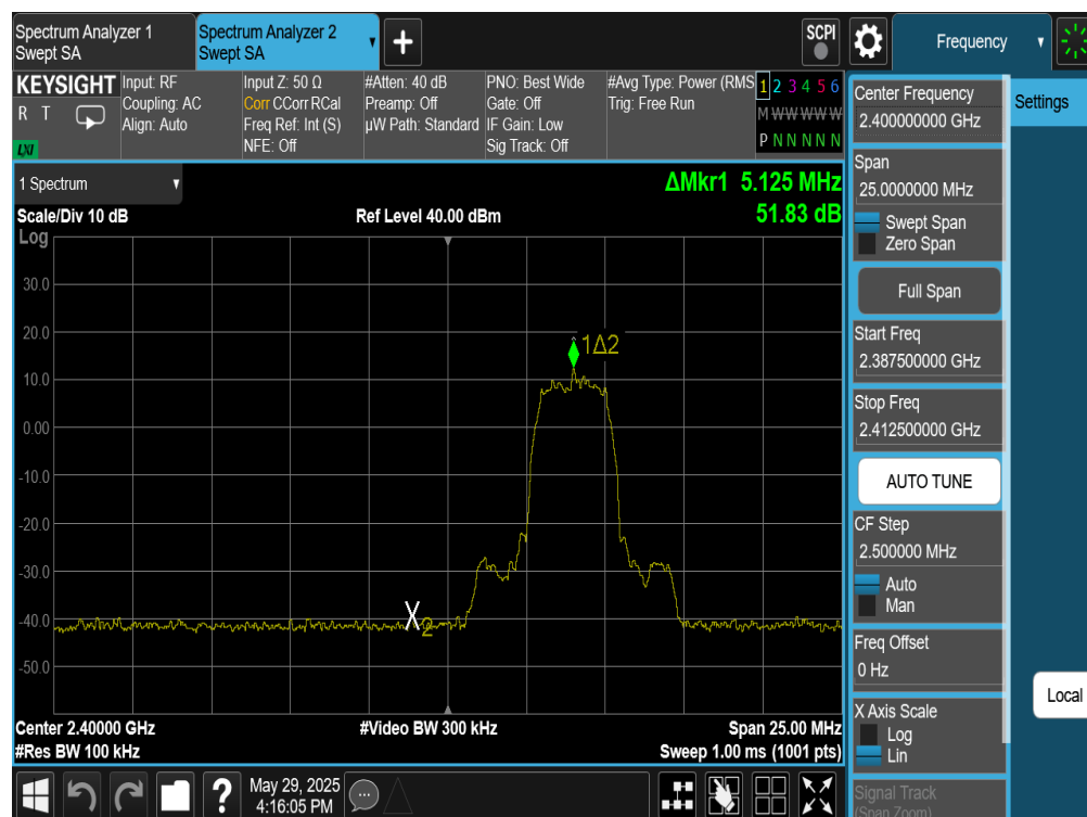
Plot 7-329. Band Edge Plot Antenna WF7 (Bluetooth (HDT2), 2Mbps, ePA – Ch. 1)
