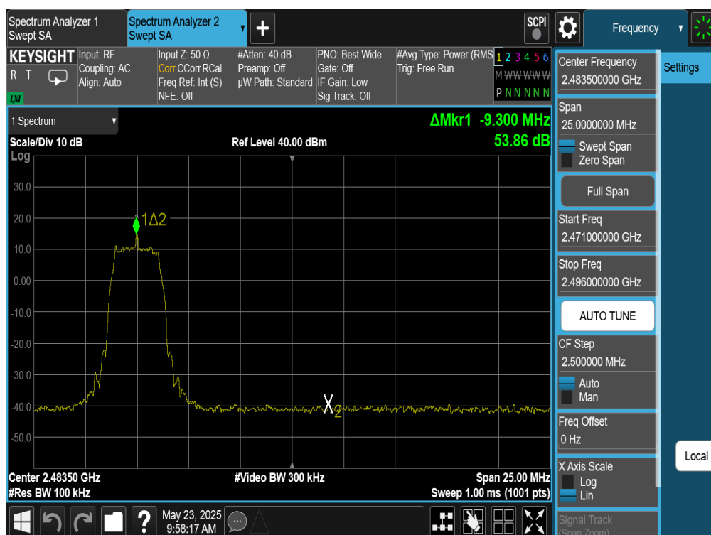
Plot 7-312. Band Edge Plot Antenna WF8 (Bluetooth (HDRPS2), 8Mbps, ePA – Ch. 73)
