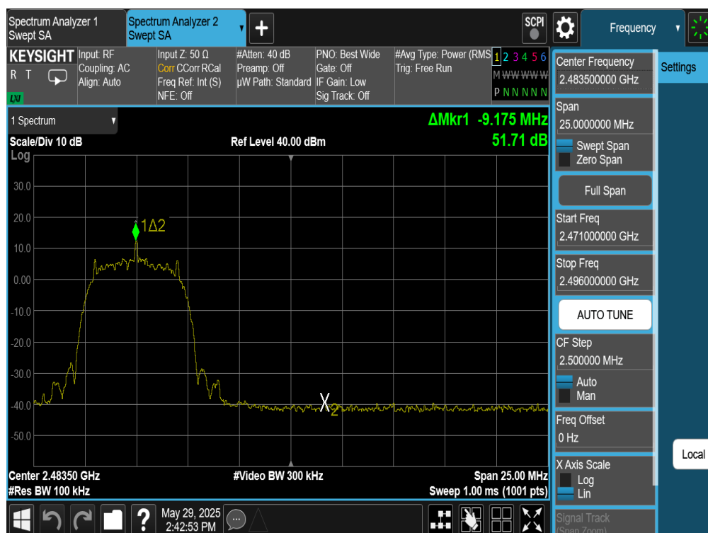
Plot 7-316. Band Edge Plot Antenna WF8 (Bluetooth (HDRPM16), 16Mbps, ePA – Ch. 73)
