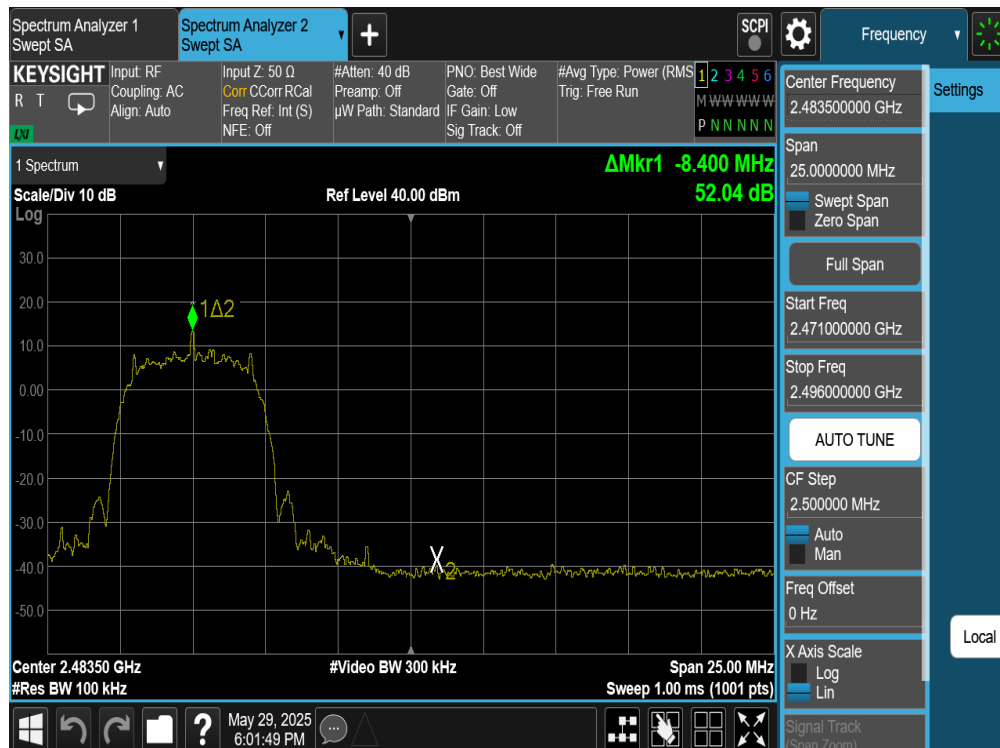
Plot 7-338. Band Edge Plot Antenna WF9 (Bluetooth (XHDRPM6), 6Mbps, ePA – Ch. 73)
