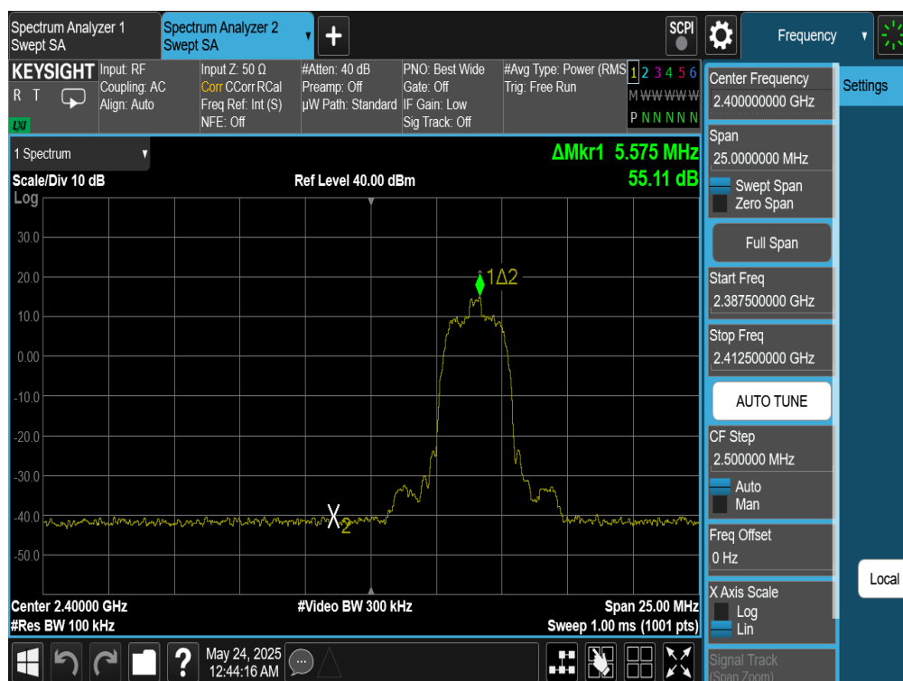
Plot 7-307. Band Edge Plot Antenna WF8 (Bluetooth (HDR4), ePA – Ch. 1)
