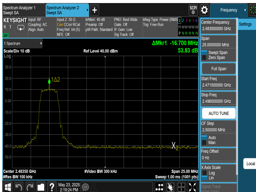
Plot 7-336. Band Edge Plot Antenna WF9 (Bluetooth (HDRPS2), 8Mbps, ePA – Ch. 73)
