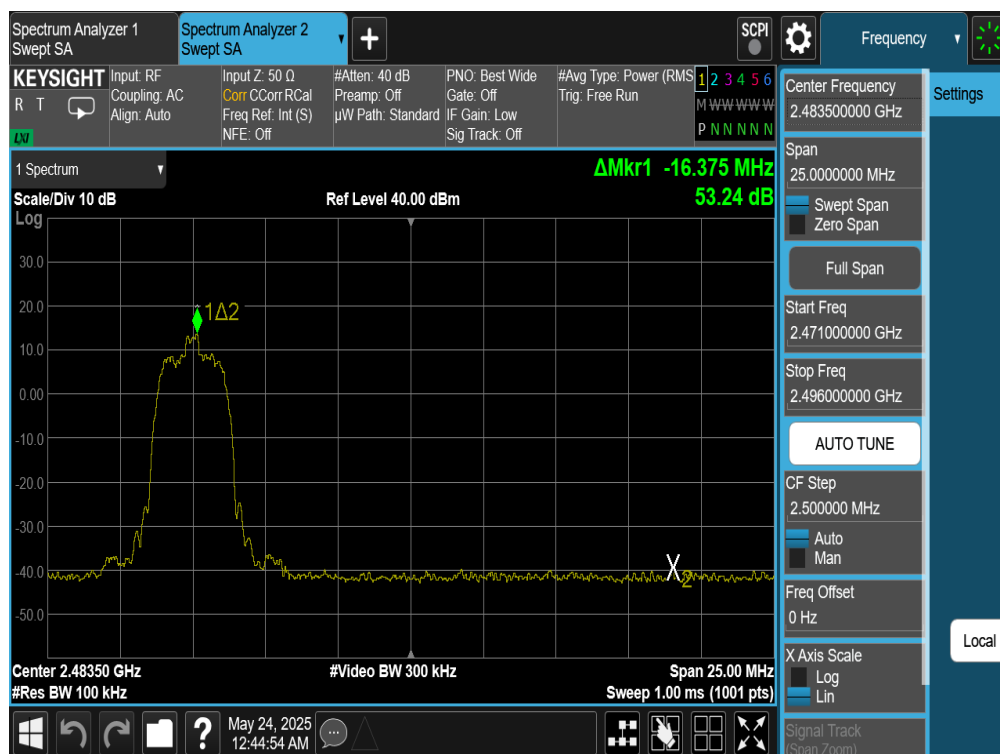
Plot 7-308. Band Edge Plot Antenna WF8 (Bluetooth (HDR4), ePA – Ch. 73)
