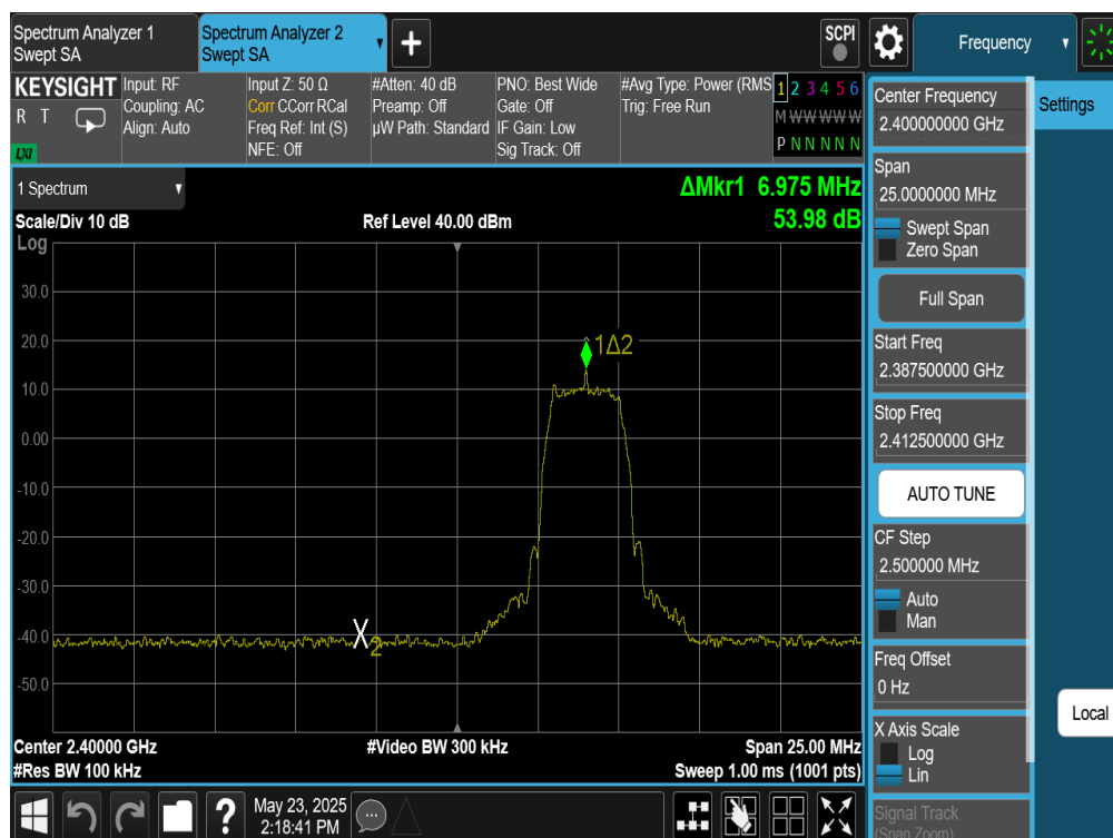
Plot 7-335. Band Edge Plot Antenna WF9 (Bluetooth (HDRPS2), 8Mbps, ePA – Ch. 1)
