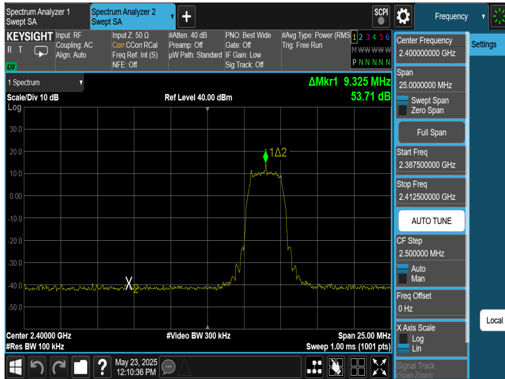
Plot 7-323. Band Edge Plot Antenna WF7 (Bluetooth (HDRPS2), 8Mbps, ePA – Ch. 1)
