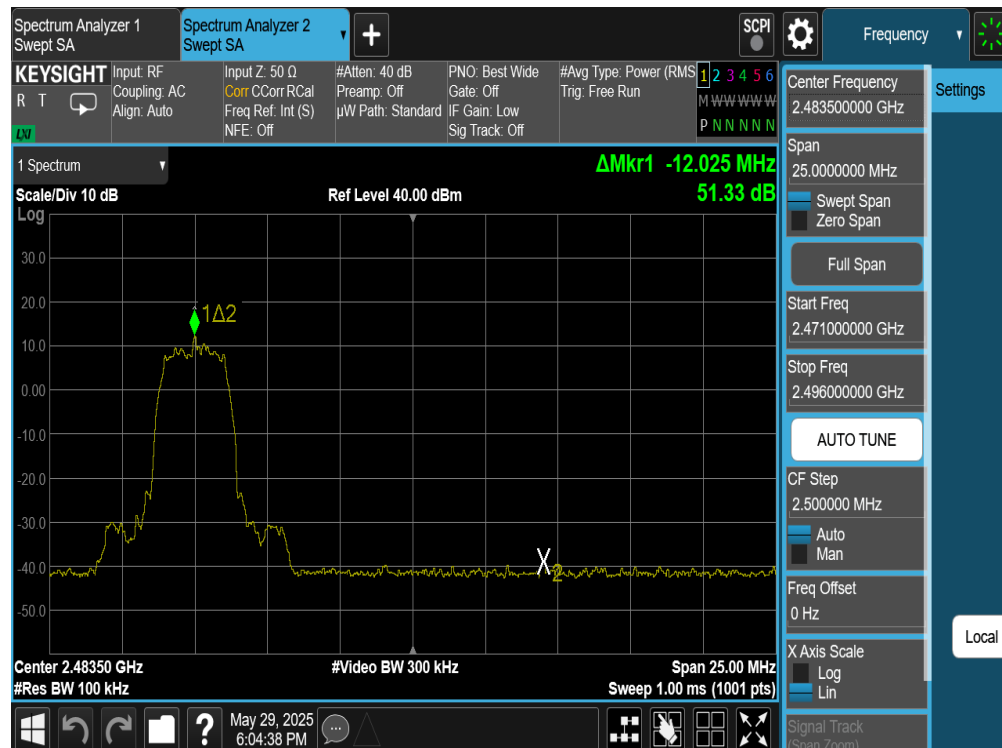
Plot 7-342. Band Edge Plot Antenna WF9 (Bluetooth (HDT2), 2Mbps, ePA – Ch. 73)
