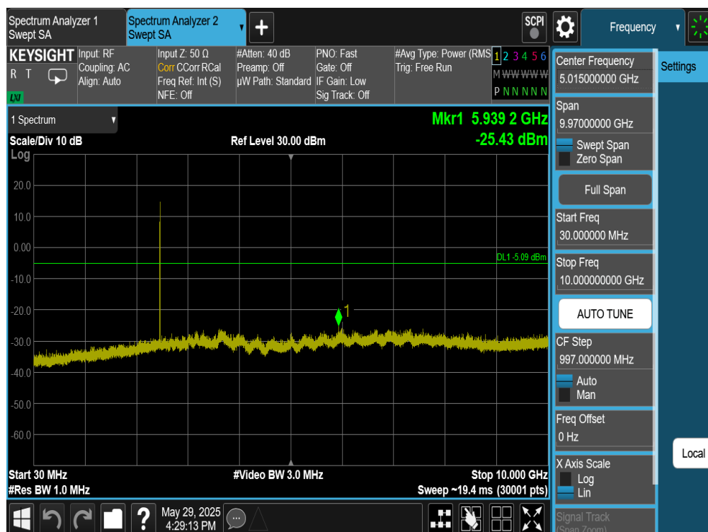
Plot 7-401. Conducted Spurious Plot Antenna WF7 (Bluetooth (HDT2), 2Mbps, ePA – Ch. 73)
