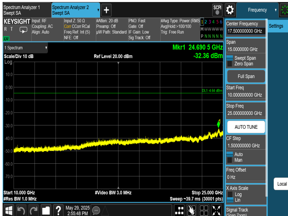
Plot 7-370. Conducted Spurious Plot Antenna WF8 (Bluetooth (HDT2), 2Mbps, ePA – Ch. 37)
