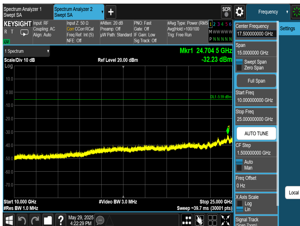
Plot 7-390. Conducted Spurious Plot Antenna WF7 (Bluetooth (XHDRPM6), 6Mbps, ePA – Ch. 73)
