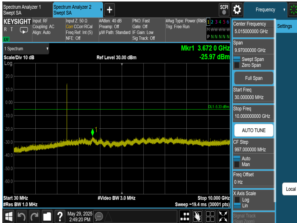
Plot 7-359. Conducted Spurious Plot Antenna WF8 (Bluetooth (XHDRPM6), 6Mbps, ePA – Ch. 73)
