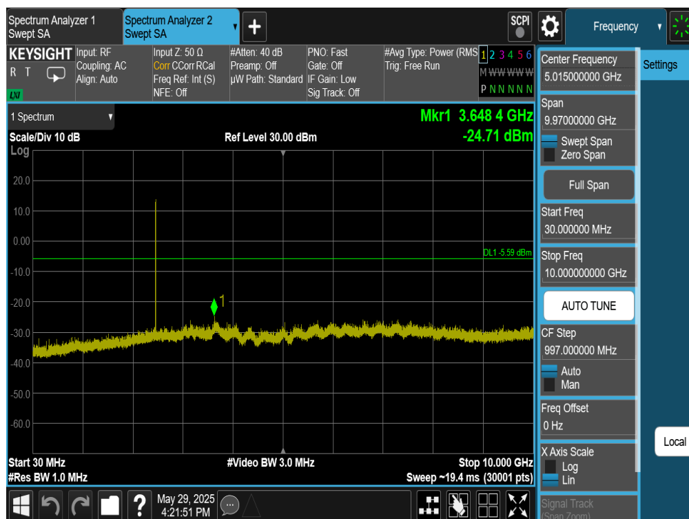
Plot 7-389. Conducted Spurious Plot Antenna WF7 (Bluetooth (XHDRPM6), 6Mbps, ePA – Ch. 73)
