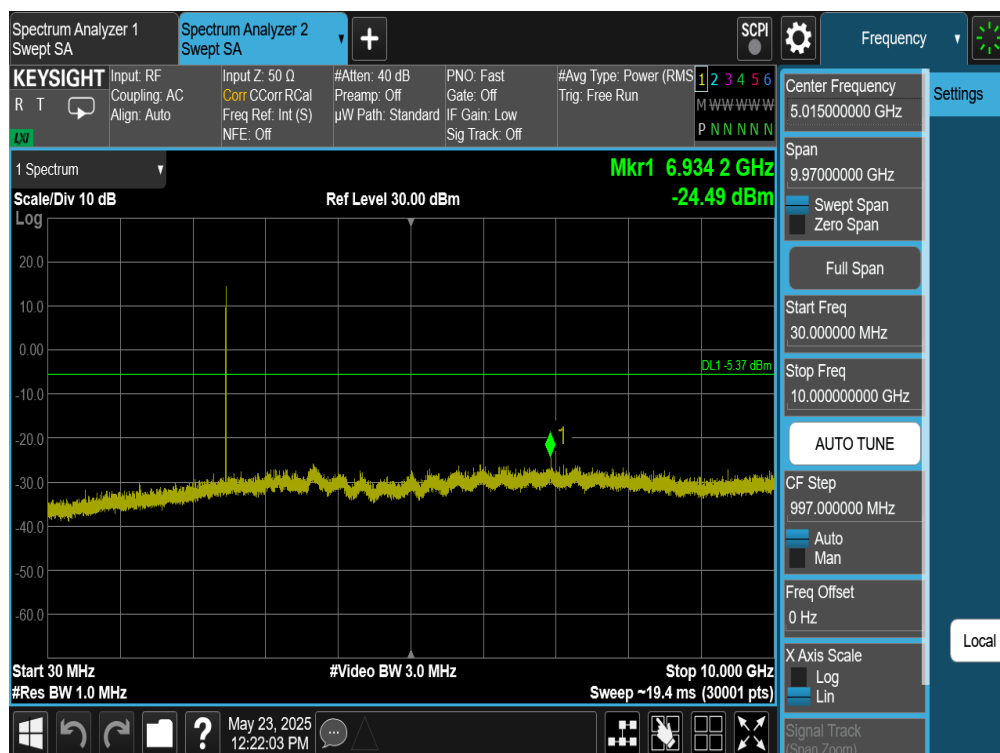
Plot 7-383. Conducted Spurious Plot Antenna WF7 (Bluetooth (HDRPS2), 2Mbps, ePA – Ch. 73)
