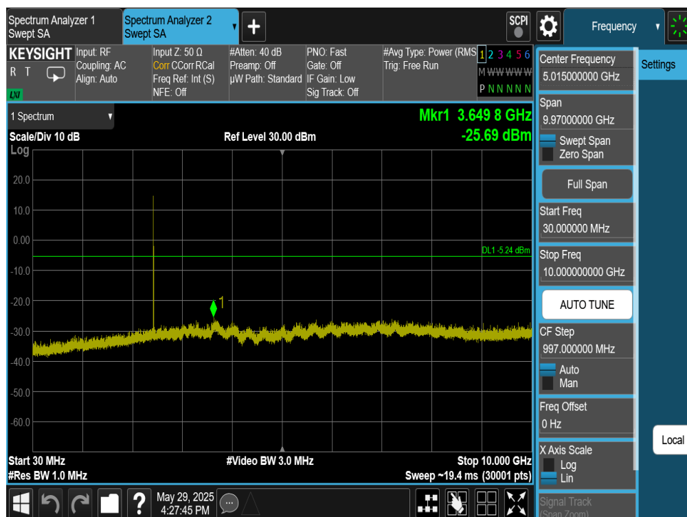
Plot 7-399. Conducted Spurious Plot Antenna WF7 (Bluetooth (HDT2), 2Mbps, ePA – Ch. 37)
