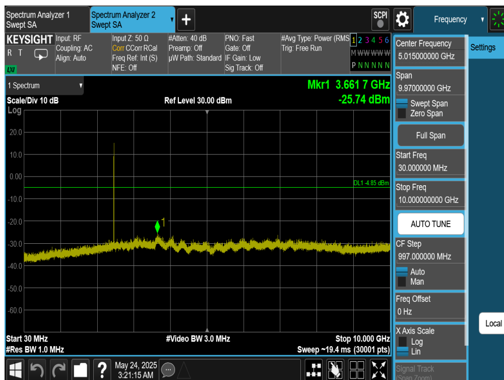
Plot 7-377. Conducted Spurious Plot Antenna WF7 (Bluetooth (HDR4), 4 Mbps, ePA – Ch. 73)
