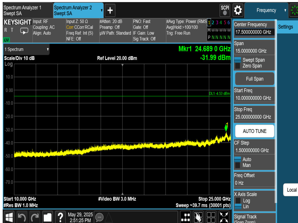
Plot 7-362. Conducted Spurious Plot Antenna WF8 (Bluetooth (HDRPM16), 16Mbps, ePA – Ch. 1)
