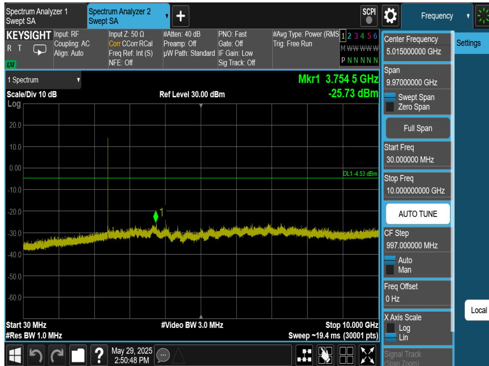
Plot 7-361. Conducted Spurious Plot Antenna WF8 (Bluetooth (HDRPM16), 16Mbps, ePA – Ch. 1)
