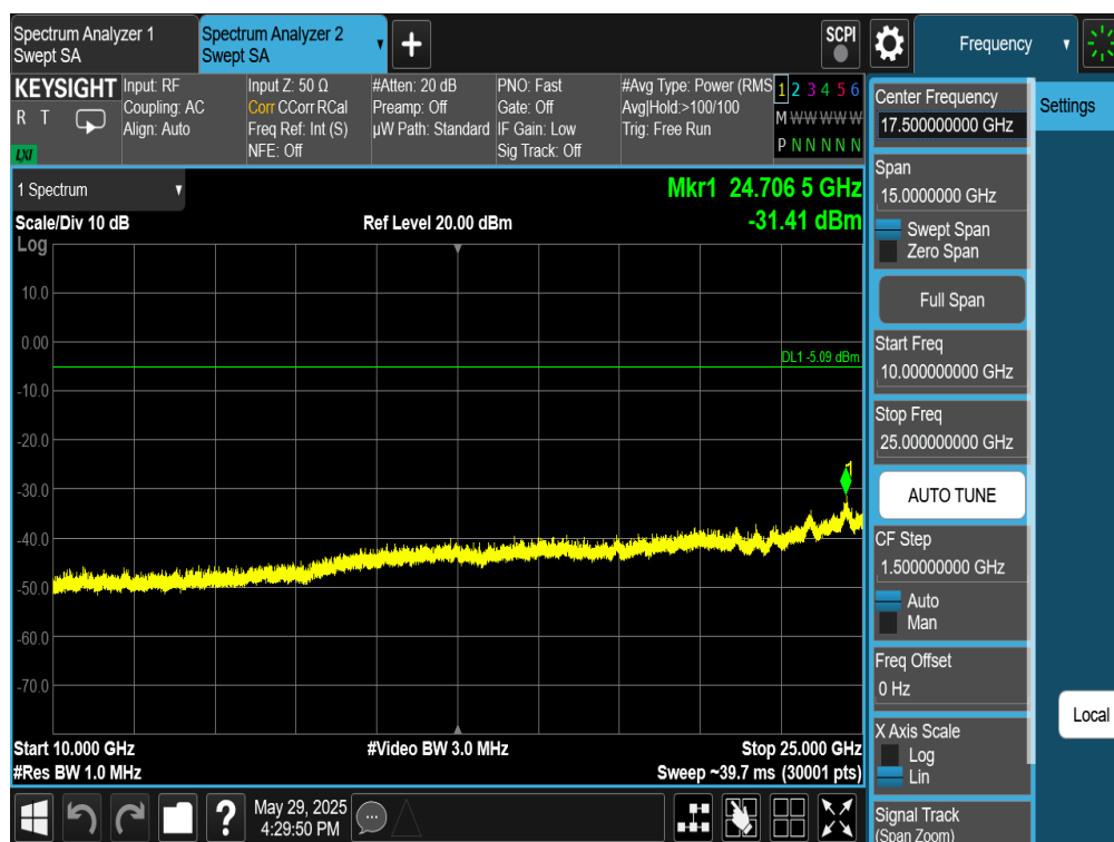
Plot 7-402. Conducted Spurious Plot Antenna WF7 (Bluetooth (HDT2), 2Mbps, ePA – Ch. 73)
