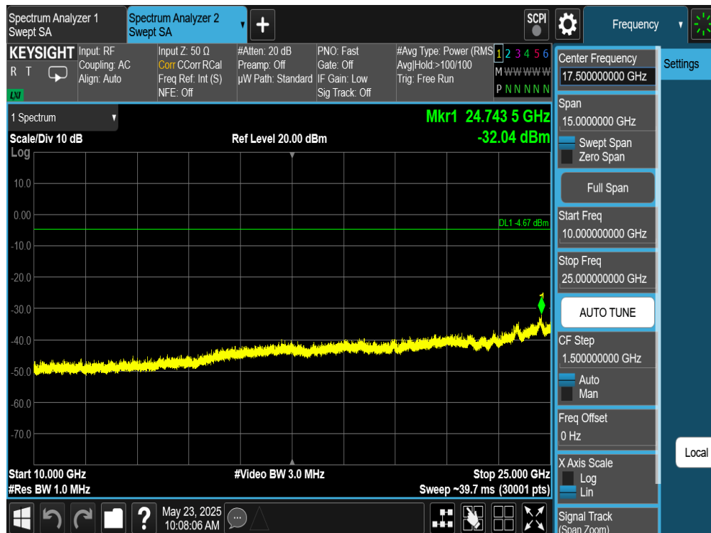
Plot 7-352. Conducted Spurious Plot Antenna WF8 (Bluetooth (HDRPS2), 2Mbps, ePA – Ch. 38)
