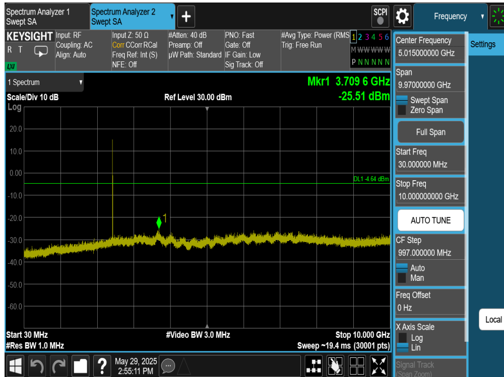
Plot 7-369. Conducted Spurious Plot Antenna WF8 (Bluetooth (HDT2), 2Mbps, ePA – Ch. 37)
