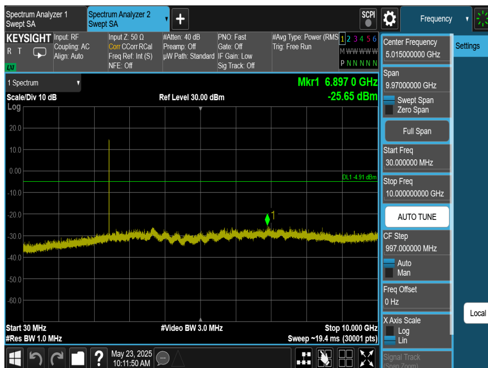
Plot 7-357. Conducted Spurious Plot Antenna WF8 (Bluetooth (XHDRPM6), 6Mbps, ePA – Ch. 38)
