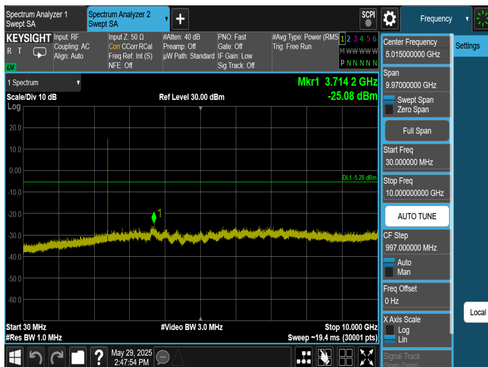
Plot 7-355. Conducted Spurious Plot Antenna WF8 (Bluetooth (XHDRPM6), 6Mbps, ePA – Ch. 1)
