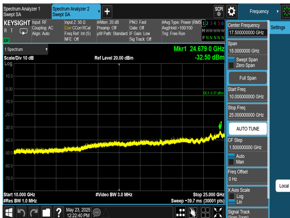
Plot 7-384. Conducted Spurious Plot Antenna WF7 (Bluetooth (HDRPS2), 2Mbps, ePA – Ch. 73)
