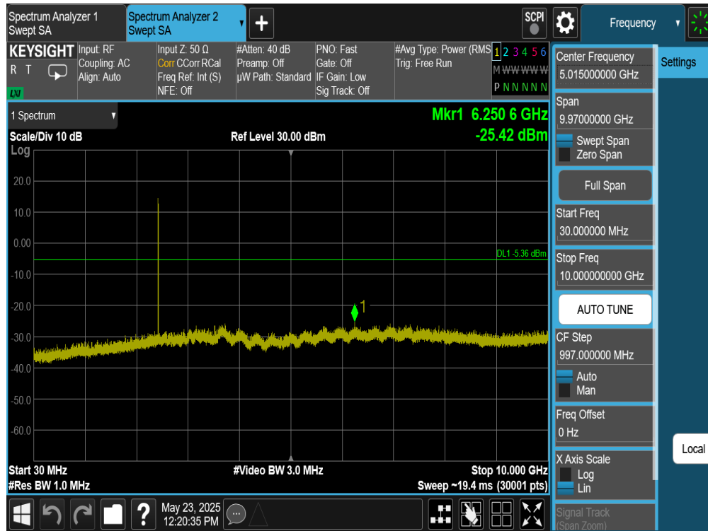
Plot 7-381. Conducted Spurious Plot Antenna WF7 (Bluetooth (HDRPS2), 2Mbps, ePA – Ch. 38)
