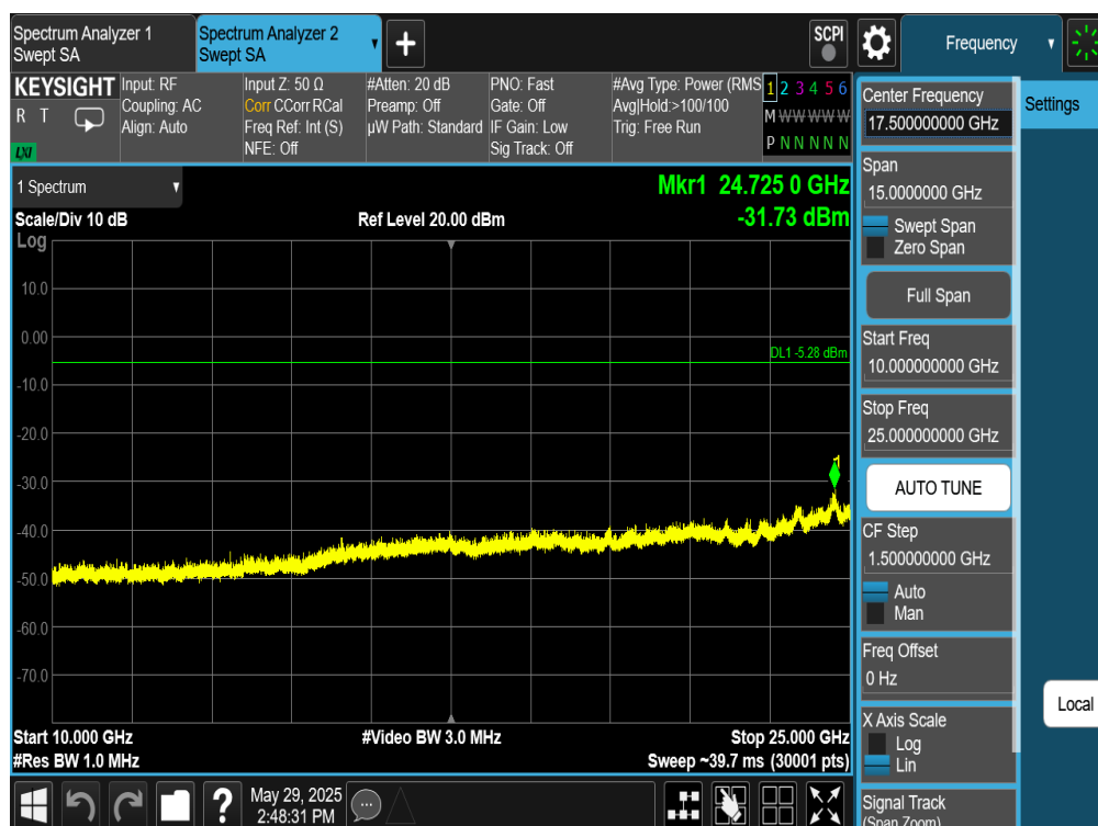
Plot 7-356. Conducted Spurious Plot Antenna WF8 (Bluetooth (XHDRPM6), 6Mbps, ePA – Ch. 1)
