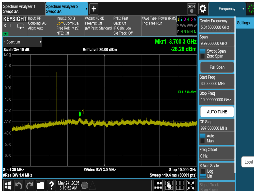
Plot 7-375. Conducted Spurious Plot Antenna WF7 (Bluetooth (HDR4), 4 Mbps, ePA – Ch. 38)
