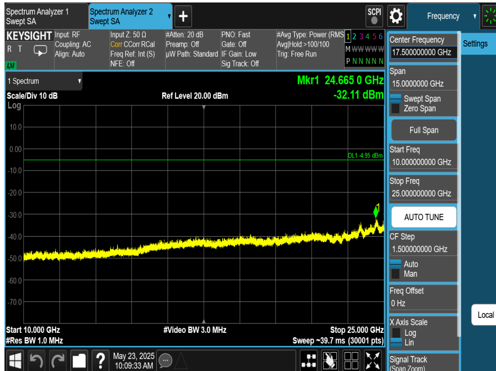
Plot 7-354. Conducted Spurious Plot Antenna WF8 (Bluetooth (HDRPS2), 2Mbps, ePA – Ch. 73)
