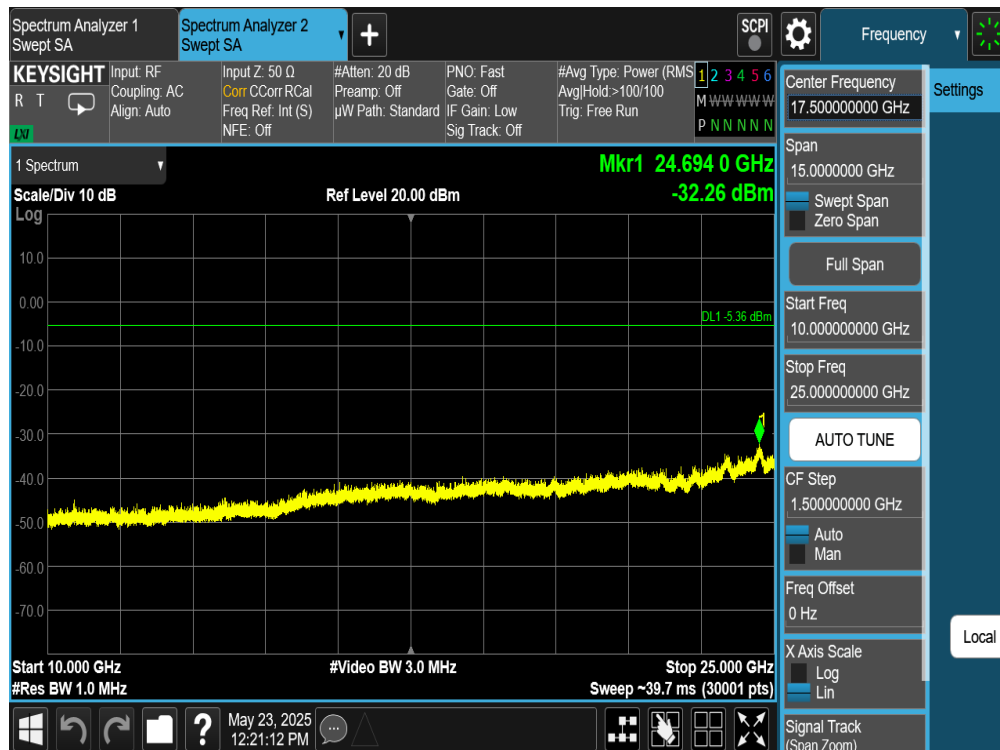
Plot 7-382. Conducted Spurious Plot Antenna WF7 (Bluetooth (HDRPS2), 2Mbps, ePA – Ch. 38)
