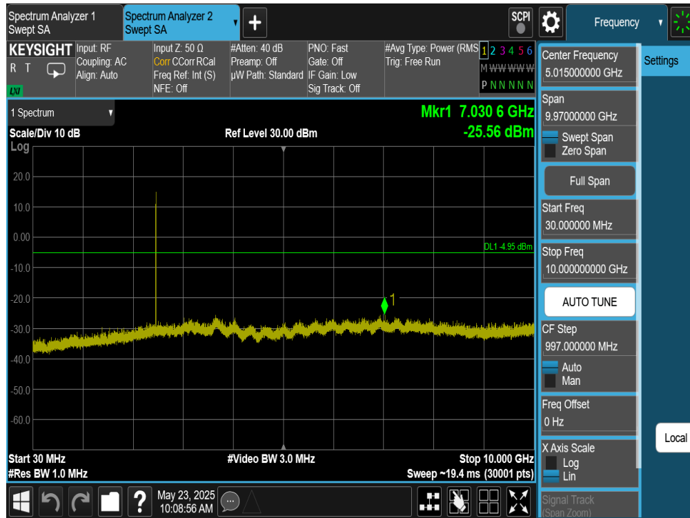
Plot 7-353. Conducted Spurious Plot Antenna WF8 (Bluetooth (HDRPS2), 2Mbps, ePA – Ch. 73)
