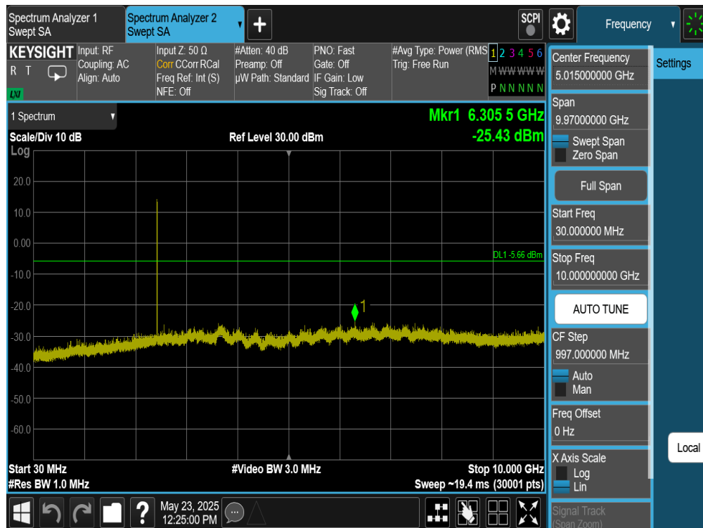
Plot 7-387. Conducted Spurious Plot Antenna WF7 (Bluetooth (XHDRPM6), 6Mbps, ePA – Ch. 38)
