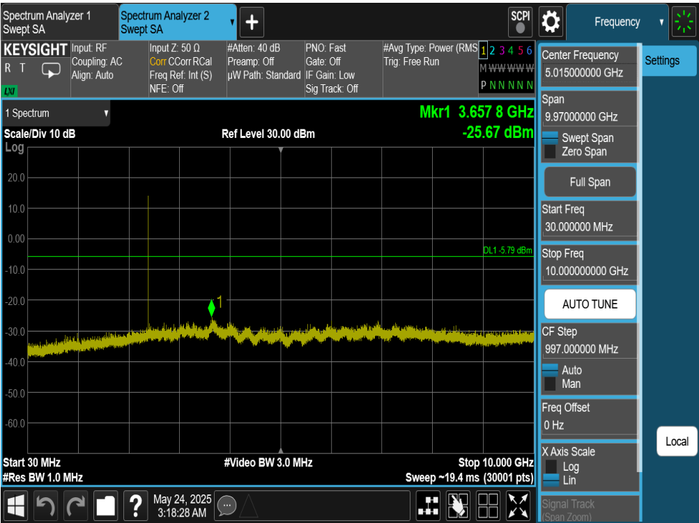
Plot 7-373. Conducted Spurious Plot Antenna WF7 (Bluetooth (HDR4), 4 Mbps, ePA – Ch. 1)
