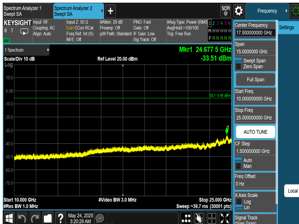
Plot 7-376. Conducted Spurious Plot Antenna WF7 (Bluetooth (HDR4), 4 Mbps, ePA – Ch. 38)
