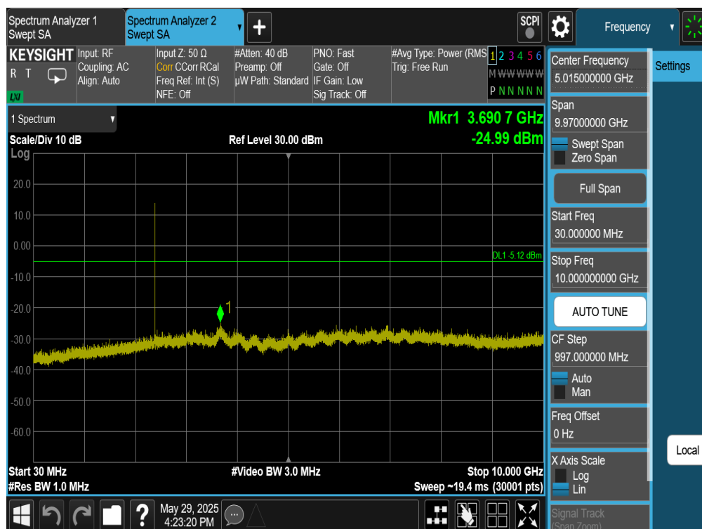
Plot 7-391. Conducted Spurious Plot Antenna WF7 (Bluetooth (HDRPM16), 16Mbps, ePA – Ch. 1)
