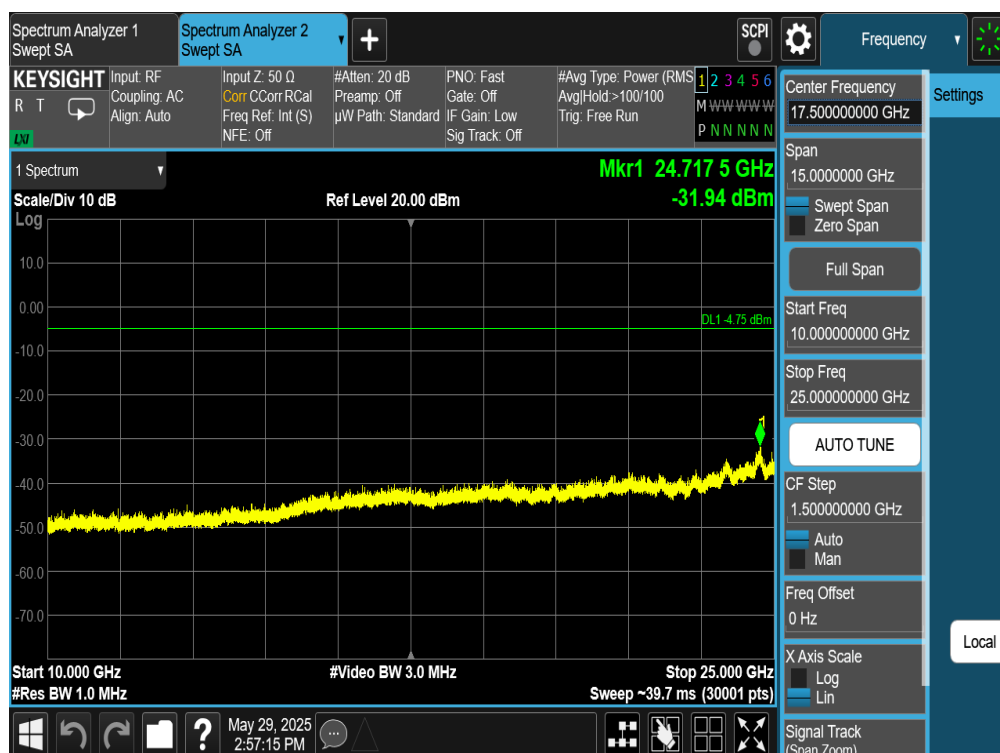
Plot 7-372. Conducted Spurious Plot Antenna WF8 (Bluetooth (HDT2), 2Mbps, ePA – Ch. 73)
