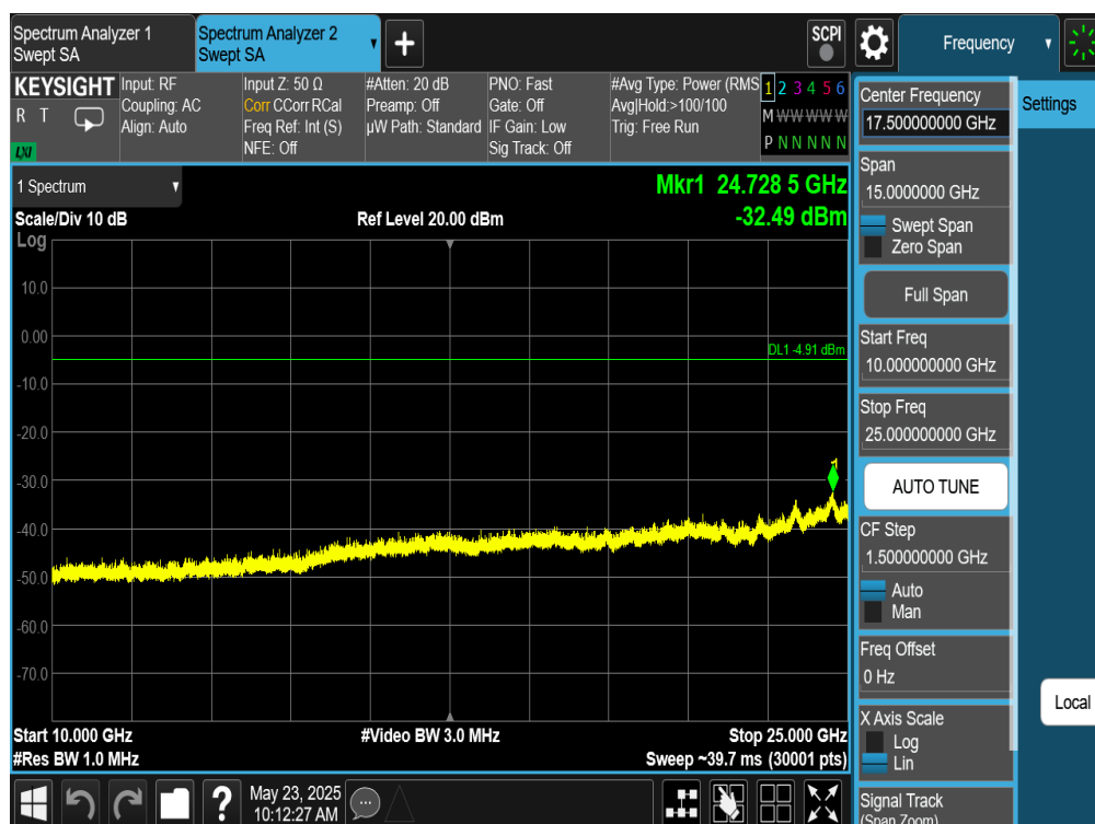
Plot 7-358. Conducted Spurious Plot Antenna WF8 (Bluetooth (XHDRPM6), 6Mbps, ePA – Ch. 38)
