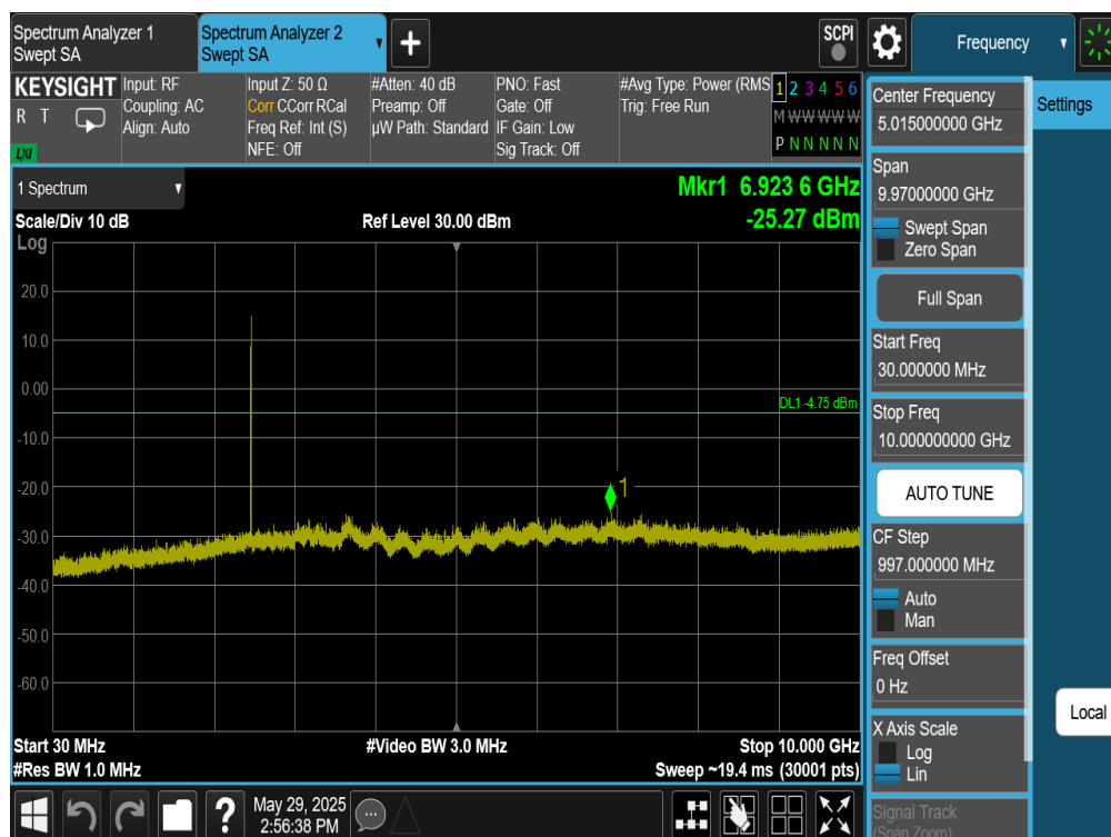
Plot 7-371. Conducted Spurious Plot Antenna WF8 (Bluetooth (HDT2), 2Mbps, ePA – Ch. 73)
