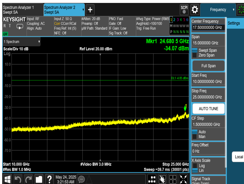
Plot 7-378. Conducted Spurious Plot Antenna WF7 (Bluetooth (HDR4), 4 Mbps, ePA – Ch. 73)
