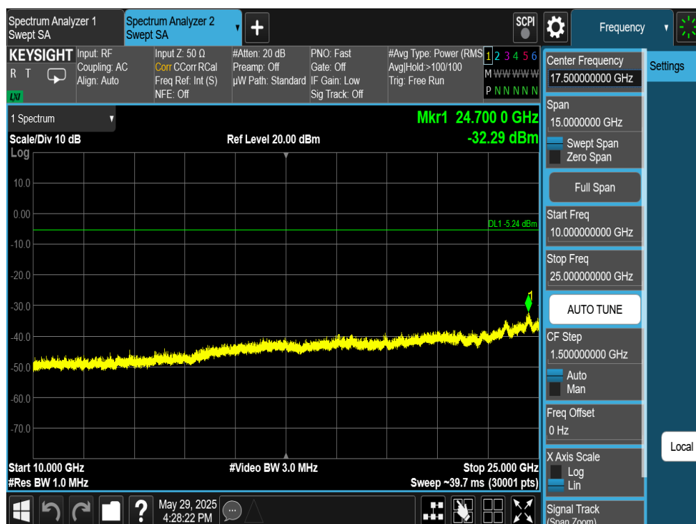
Plot 7-400. Conducted Spurious Plot Antenna WF7 (Bluetooth (HDT2), 2Mbps, ePA – Ch. 37)
