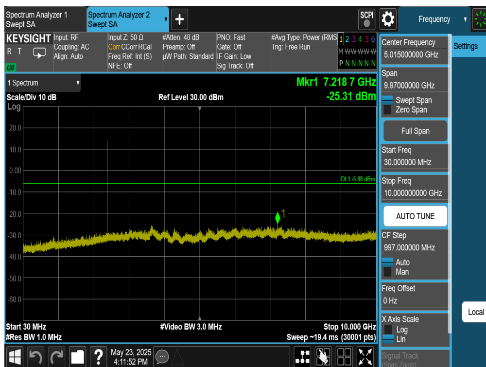
Plot 7-403. Conducted Spurious Plot Antenna WF9 (Bluetooth (HDR4), 4 Mbps, ePA – Ch. 1)
