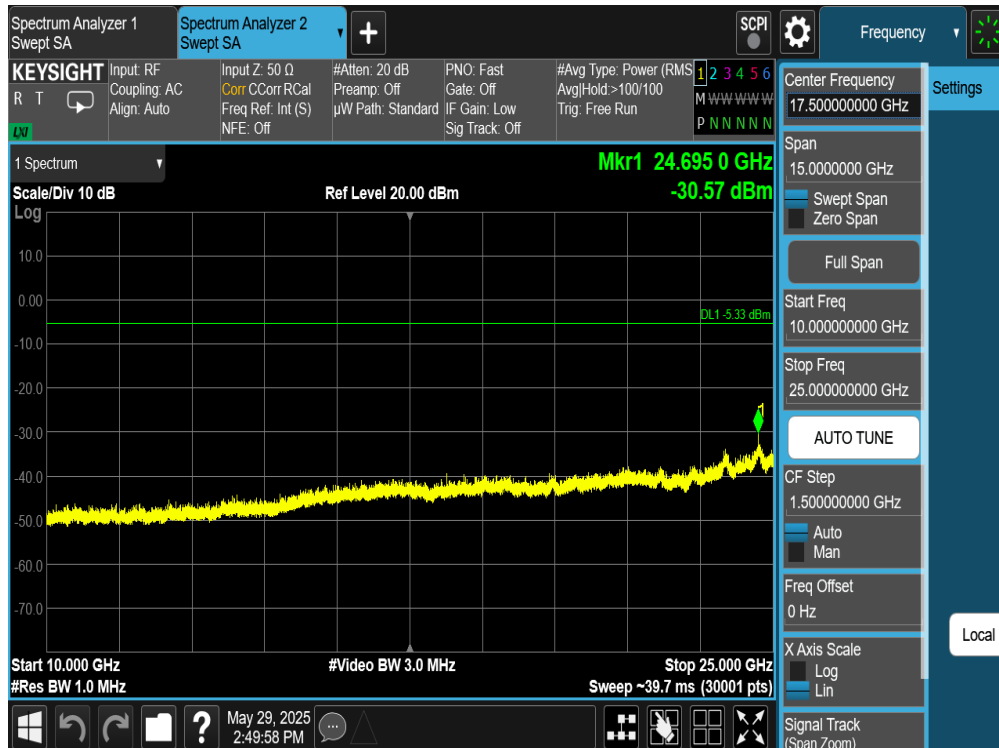
Plot 7-360. Conducted Spurious Plot Antenna WF8 (Bluetooth (XHDRPM6), 6Mbps, ePA – Ch. 73)
