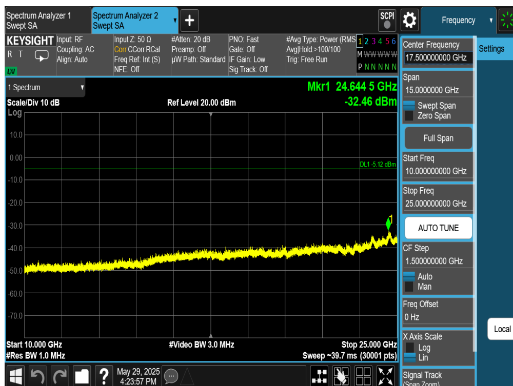
Plot 7-392. Conducted Spurious Plot Antenna WF7 (Bluetooth (HDRPM16), 16Mbps, ePA – Ch. 1)
