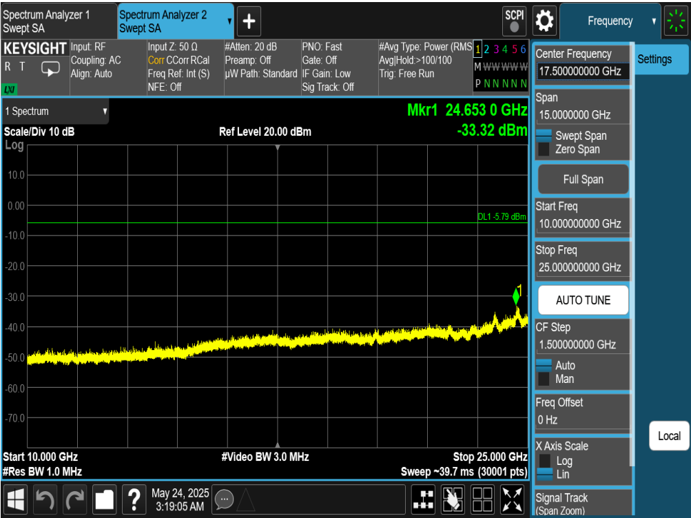
Plot 7-374. Conducted Spurious Plot Antenna WF7 (Bluetooth (HDR4), 4 Mbps, ePA – Ch. 1)
