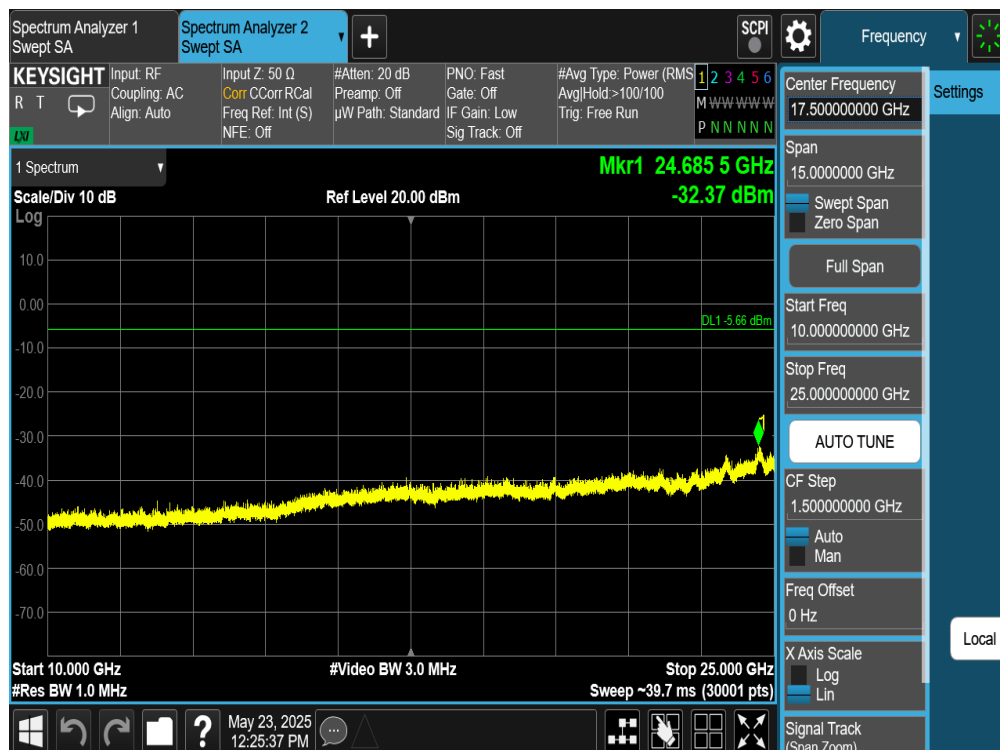
Plot 7-388. Conducted Spurious Plot Antenna WF7 (Bluetooth (XHDRPM6), 6Mbps, ePA – Ch. 38)
