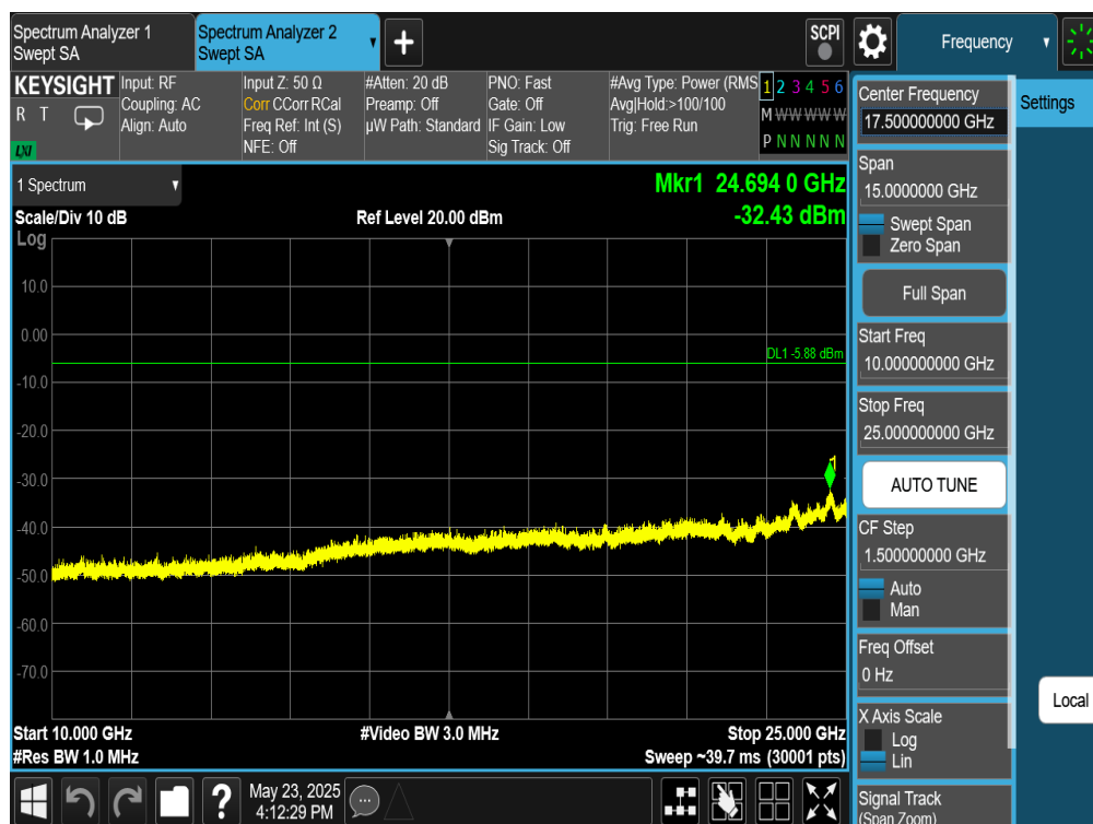
Plot 7-404. Conducted Spurious Plot Antenna WF9 (Bluetooth (HDR4), 4 Mbps, ePA – Ch. 1)
