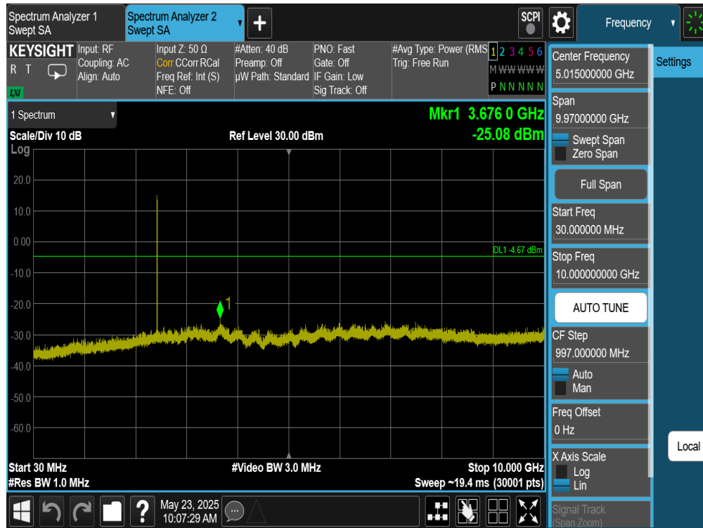
Plot 7-351. Conducted Spurious Plot Antenna WF8 (Bluetooth (HDRPS2), 2Mbps, ePA – Ch. 38)
