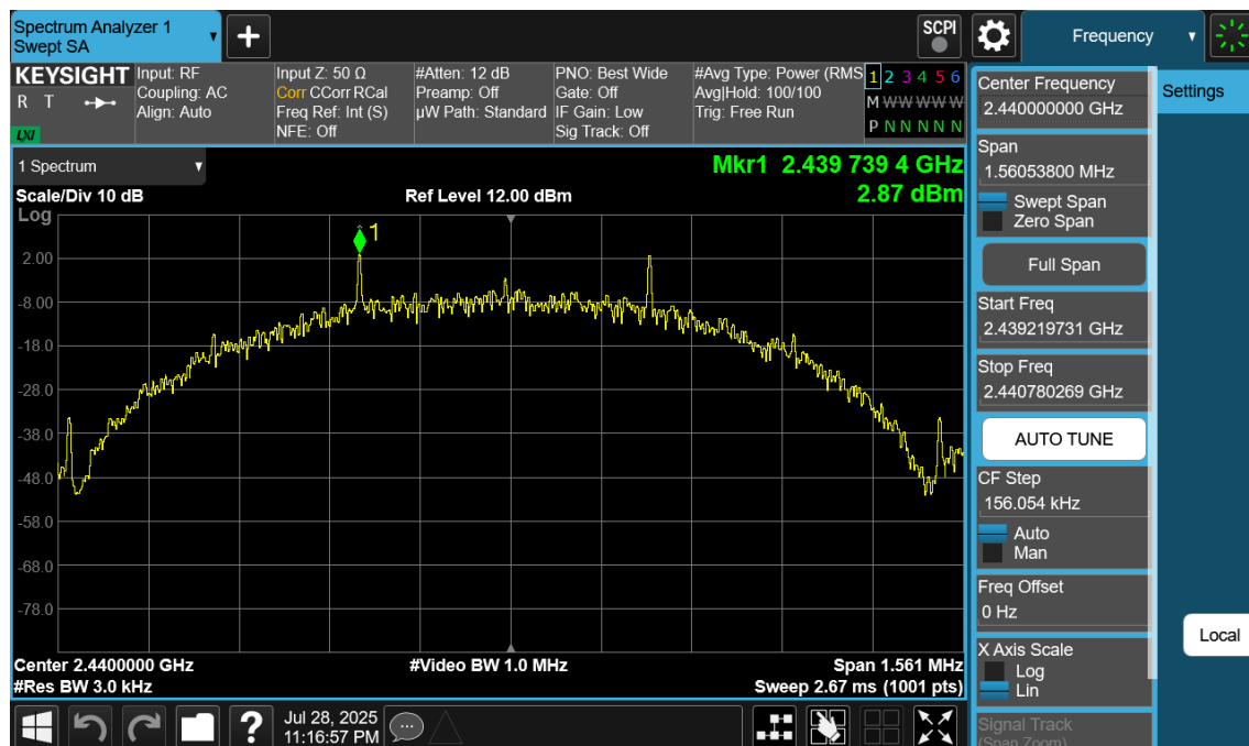
Plot 7-123. Power Spectral Density Plot Antenna WF8 (Bluetooth (LE), 500kbps, ePA – Ch. 19)
