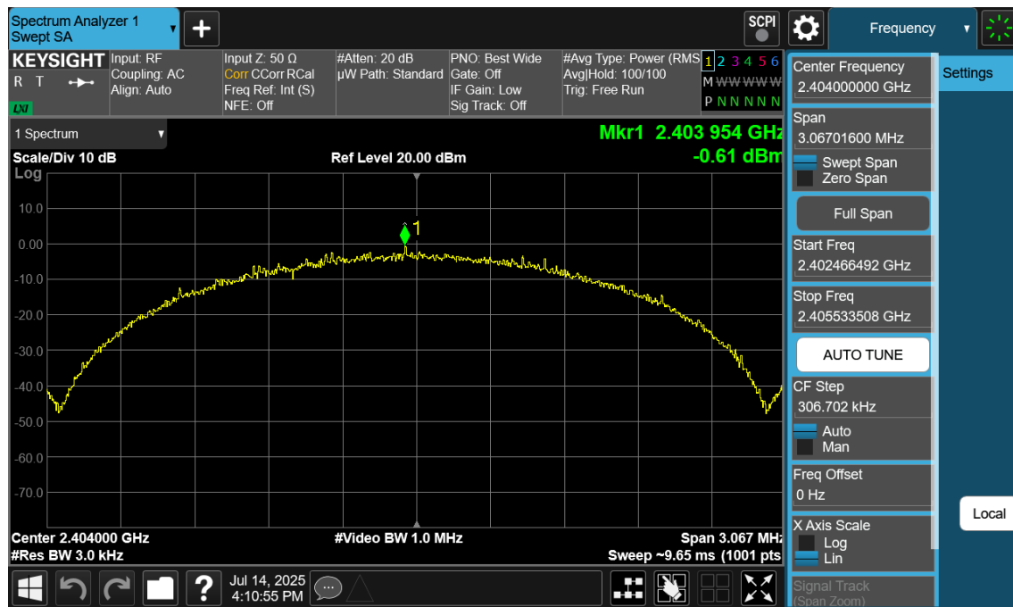
Plot 7-194. Power Spectral Density Plot Antenna WF9 (Bluetooth (LE), 2Mbps, ePA – Ch. 1)
