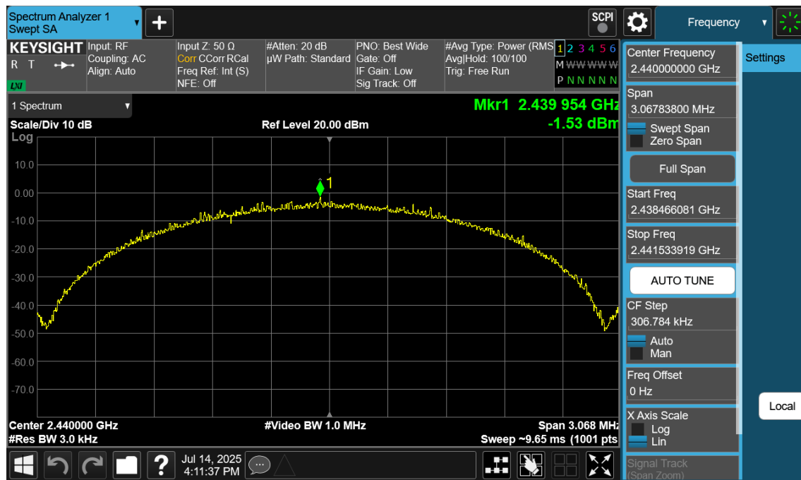
Plot 7-196. Power Spectral Density Plot Antenna WF9 (Bluetooth (LE), 2Mbps, ePA – Ch. 19)
