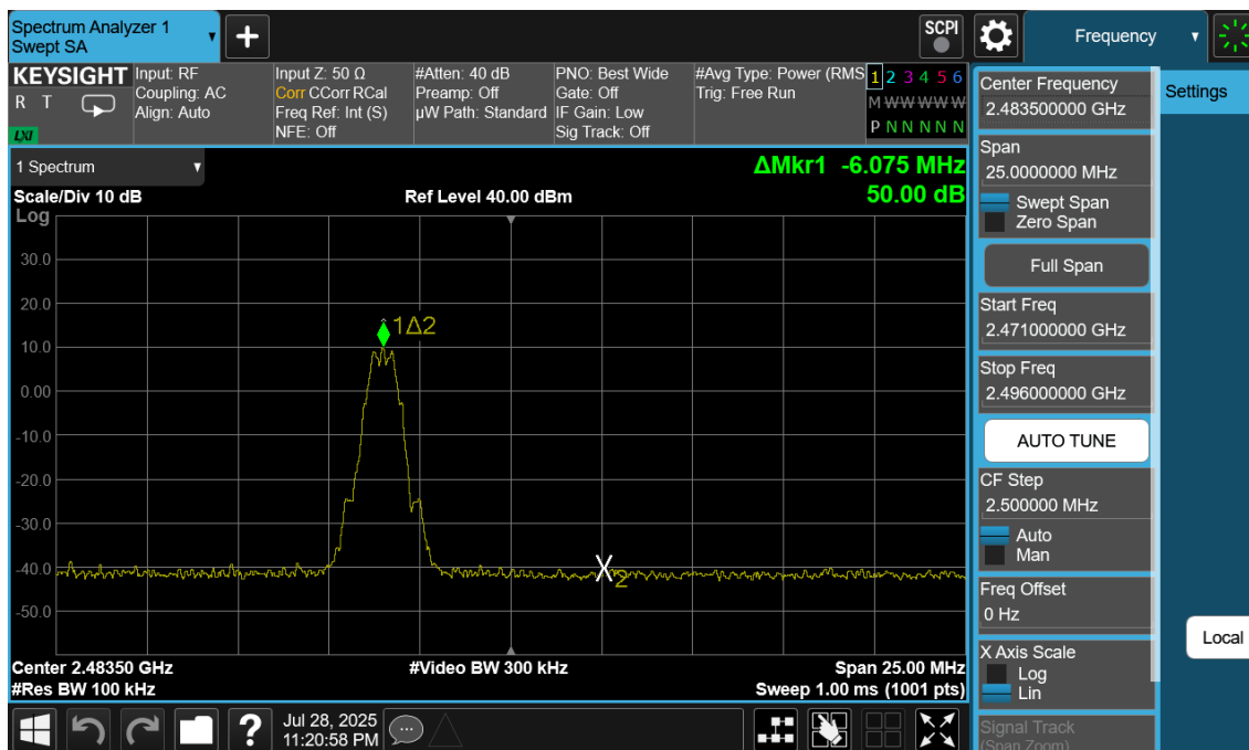
Plot 7-206. Band Edge Plot Antenna WF8 (Bluetooth (LE), 125kbps, ePA – Ch. 39)
