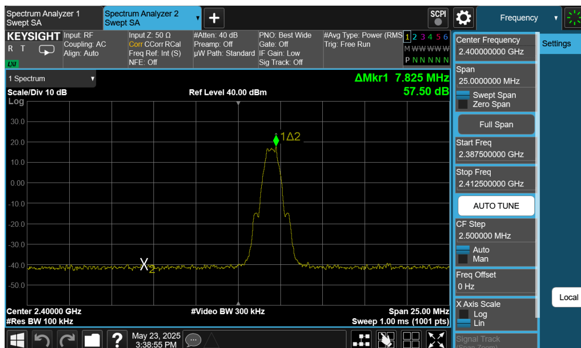
Plot 7-225. Band Edge Plot Antenna WF9 (Bluetooth (LE), 1Mbps, ePA – Ch.0)
