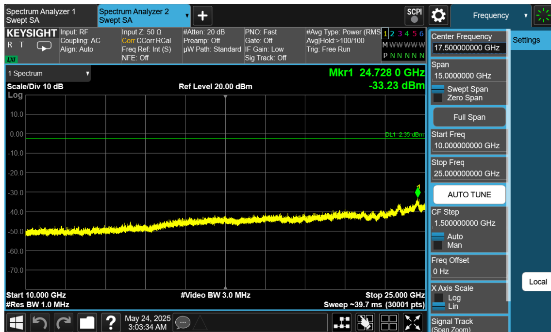
Plot 7-238. Conducted Spurious Plot Antenna WF7 (Bluetooth (LE), 1Mbps, ePA – Ch. 19)
