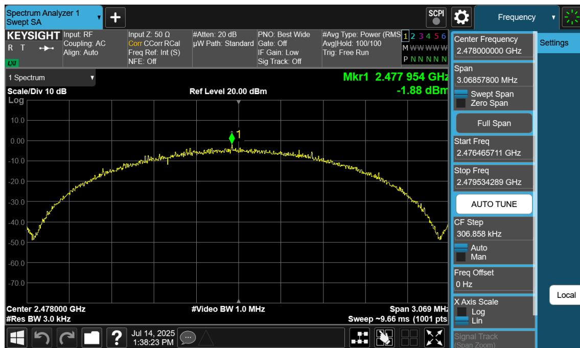
Plot 7-197. Power Spectral Density Plot Antenna WF8 (Bluetooth (LE), 2Mbps, ePA – Ch. 38)
