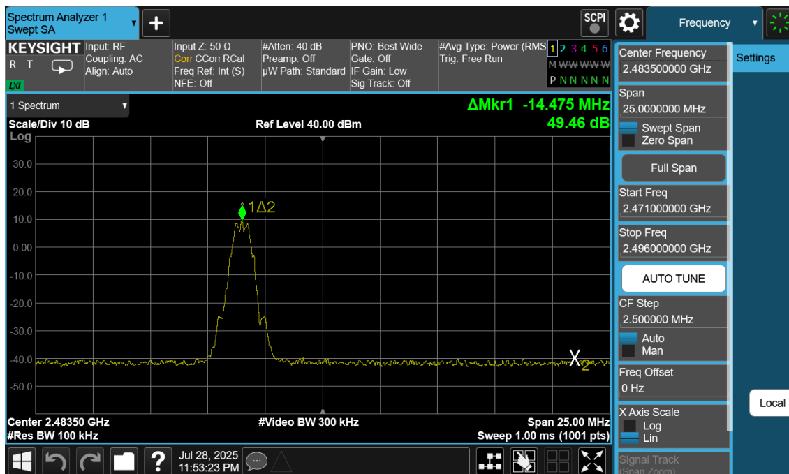
Plot 7-214. Band Edge Plot Antenna WF7 (Bluetooth (LE), 125kbps, ePA – Ch. 39)
