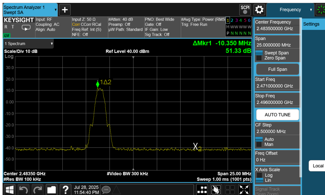
Plot 7-216. Band Edge Plot Antenna WF7 (Bluetooth (LE), 500kbps, ePA – Ch. 39)
