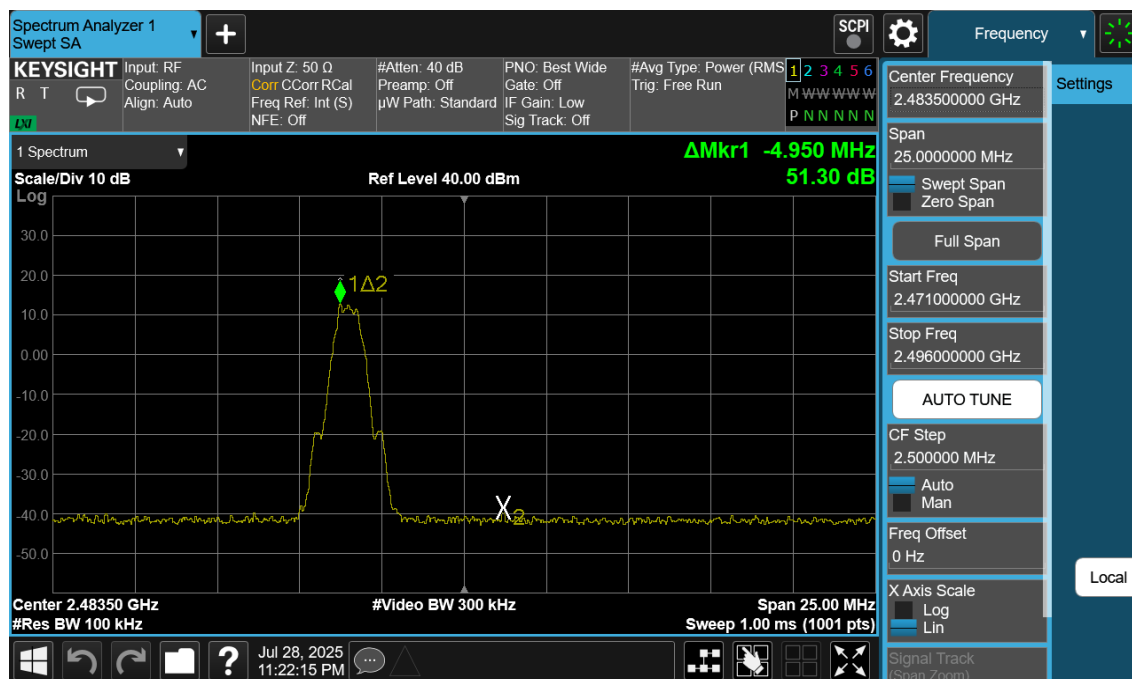
Plot 7-208. Band Edge Plot Antenna WF8 (Bluetooth (LE), 500kbps, ePA – Ch. 39)
