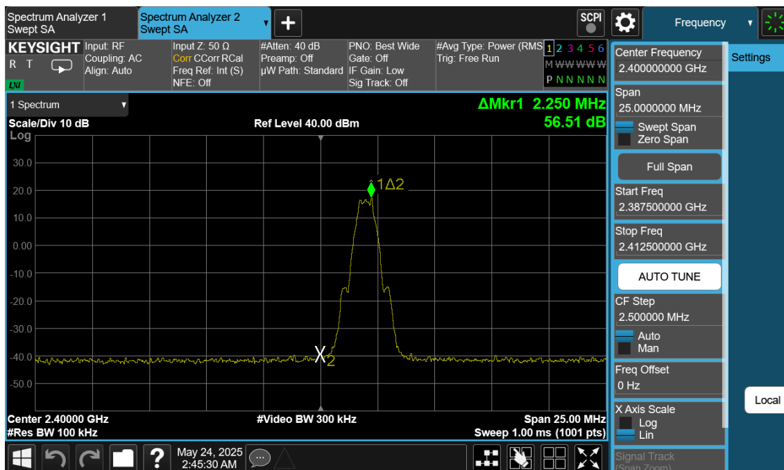
Plot 7-217. Band Edge Plot Antenna WF7 (Bluetooth (LE), 1Mbps, ePA – Ch.0)
