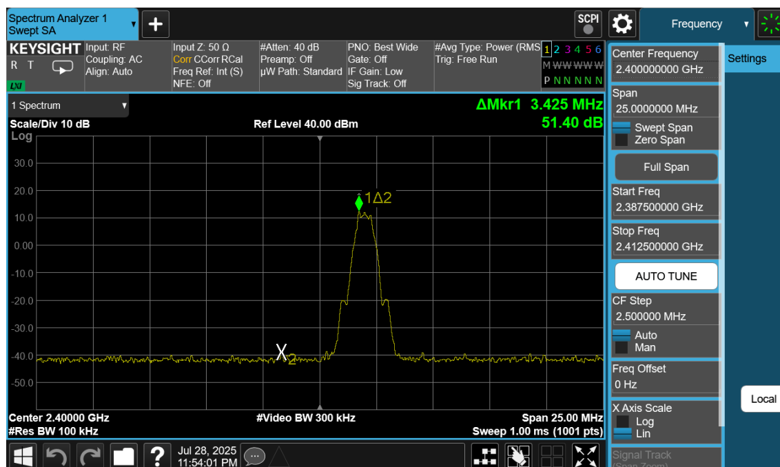
Plot 7-215. Band Edge Plot Antenna WF7 (Bluetooth (LE), 500kbps, ePA – Ch.0)
