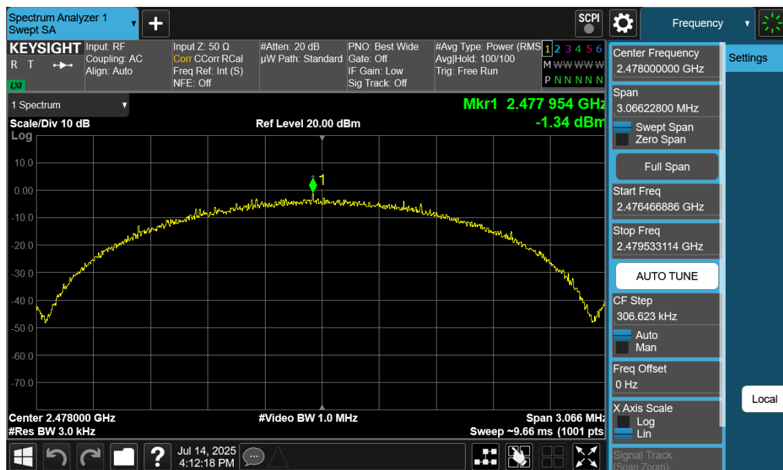
Plot 7-198. Power Spectral Density Plot Antenna WF9 (Bluetooth (LE), 2Mbps, ePA – Ch. 38)
