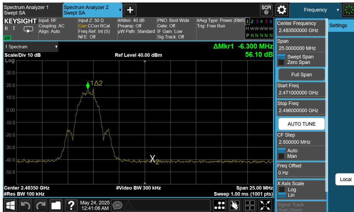
Plot 7-212. Band Edge Plot Antenna WF8 (Bluetooth (LE), 2Mbps, ePA – Ch. 38)
