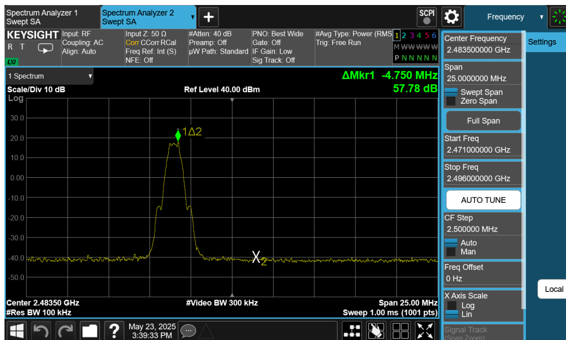
Plot 7-226. Band Edge Plot Antenna WF9 (Bluetooth (LE), 1Mbps, ePA – Ch. 39)
