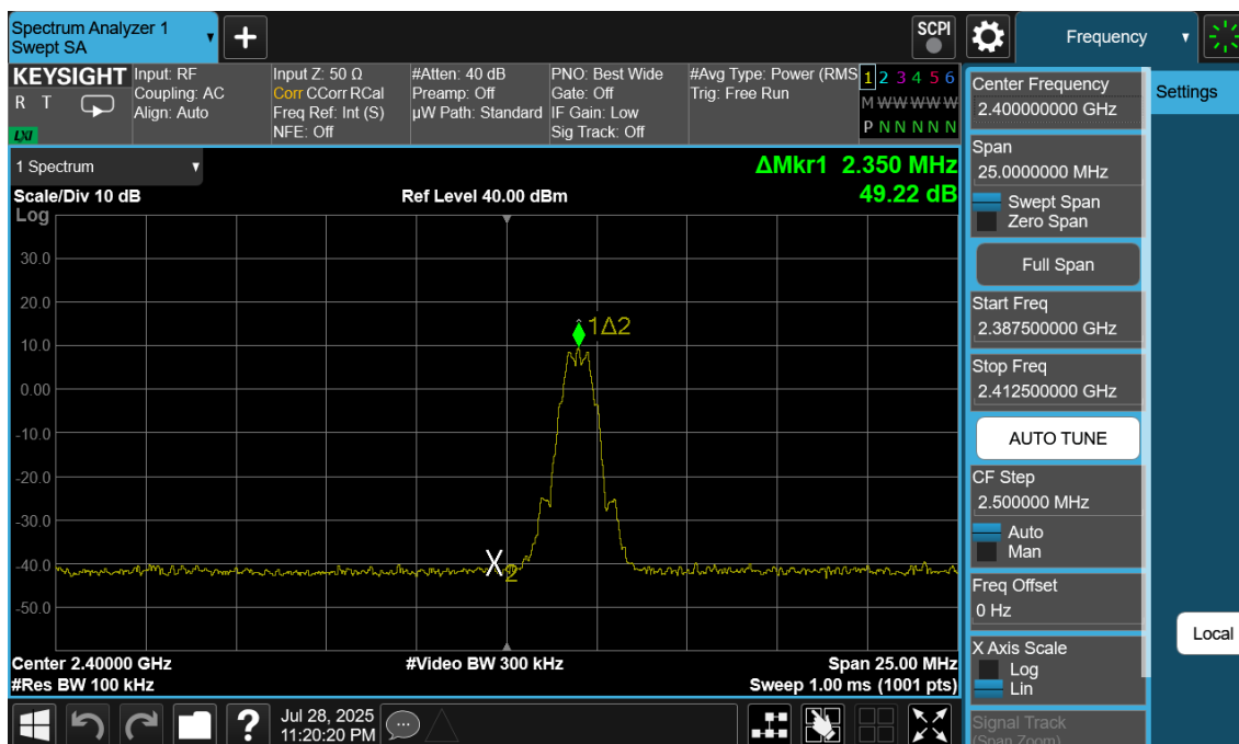
Plot 7-205. Band Edge Plot Antenna WF8 (Bluetooth (LE), 125kbps, ePA – Ch.0)
