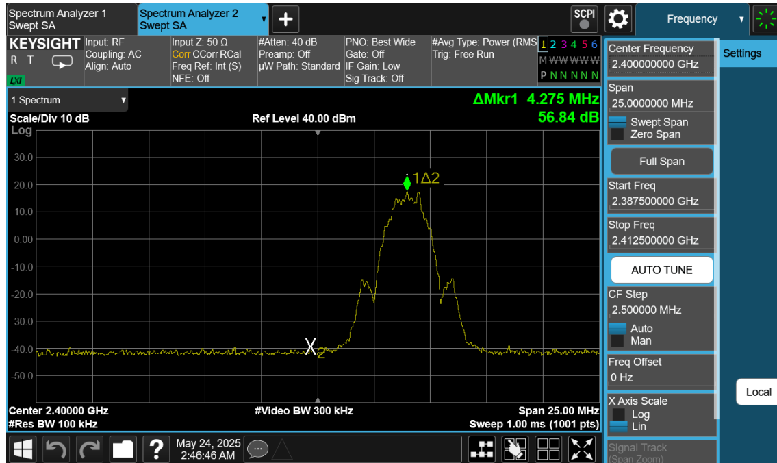
Plot 7-219. Band Edge Plot Antenna WF7 (Bluetooth (LE), 2Mbps, ePA – Ch. 1)
