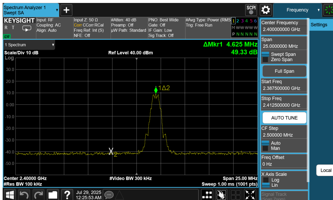
Plot 7-221. Band Edge Plot Antenna WF9 (Bluetooth (LE), 125kbps, ePA – Ch.0)
