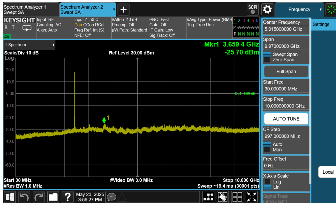
Plot 7-243. Conducted Spurious Plot Antenna WF9 (Bluetooth (LE), 1Mbps, ePA – Ch. 19)
