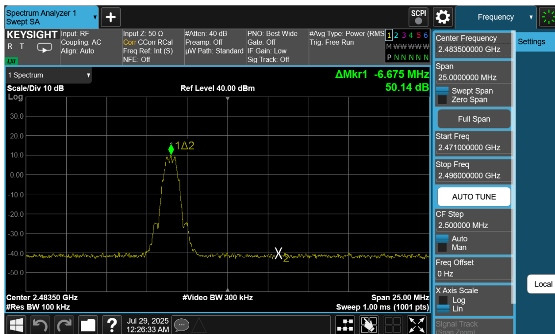
Plot 7-222. Band Edge Plot Antenna WF9 (Bluetooth (LE), 125kbps, ePA – Ch. 39)
