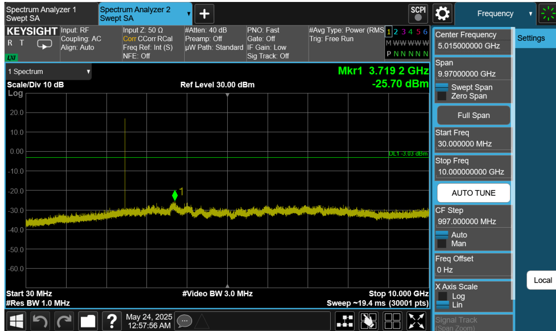
Plot 7-233. Conducted Spurious Plot Antenna WF8 (Bluetooth (LE), 1Mbps, ePA – Ch. 39)
