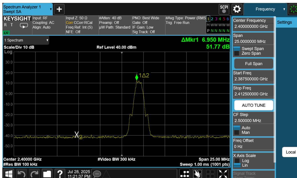
Plot 7-207. Band Edge Plot Antenna WF8 (Bluetooth (LE), 500kbps, ePA – Ch.0)
