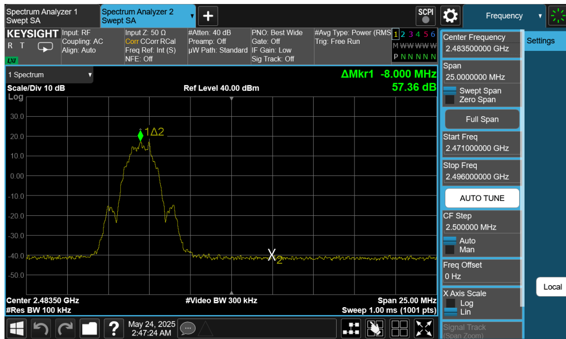
Plot 7-220. Band Edge Plot Antenna WF7 (Bluetooth (LE), 2Mbps, ePA – Ch. 38)
