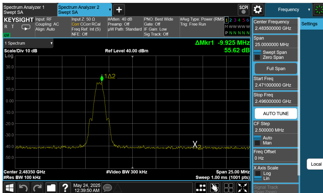
Plot 7-210. Band Edge Plot Antenna WF8 (Bluetooth (LE), 1Mbps, ePA – Ch. 39)
