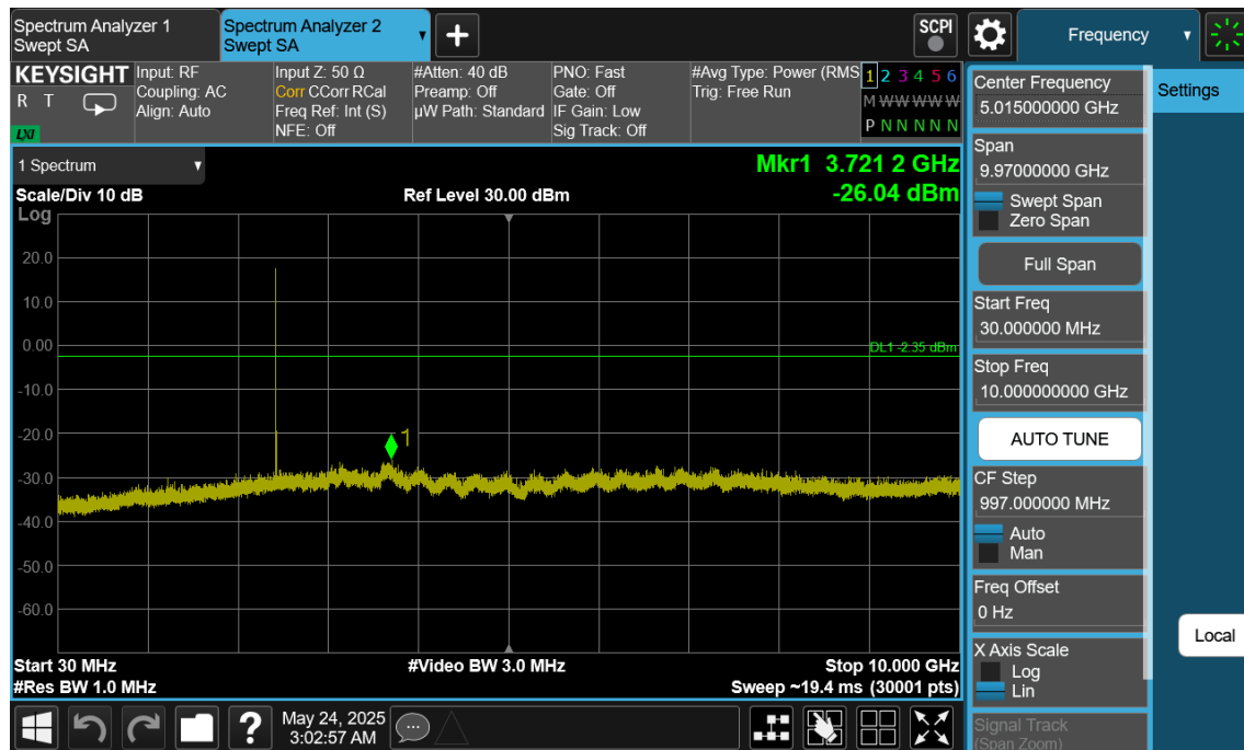
Plot 7-237. Conducted Spurious Plot Antenna WF7 (Bluetooth (LE), 1Mbps, ePA – Ch. 19)
