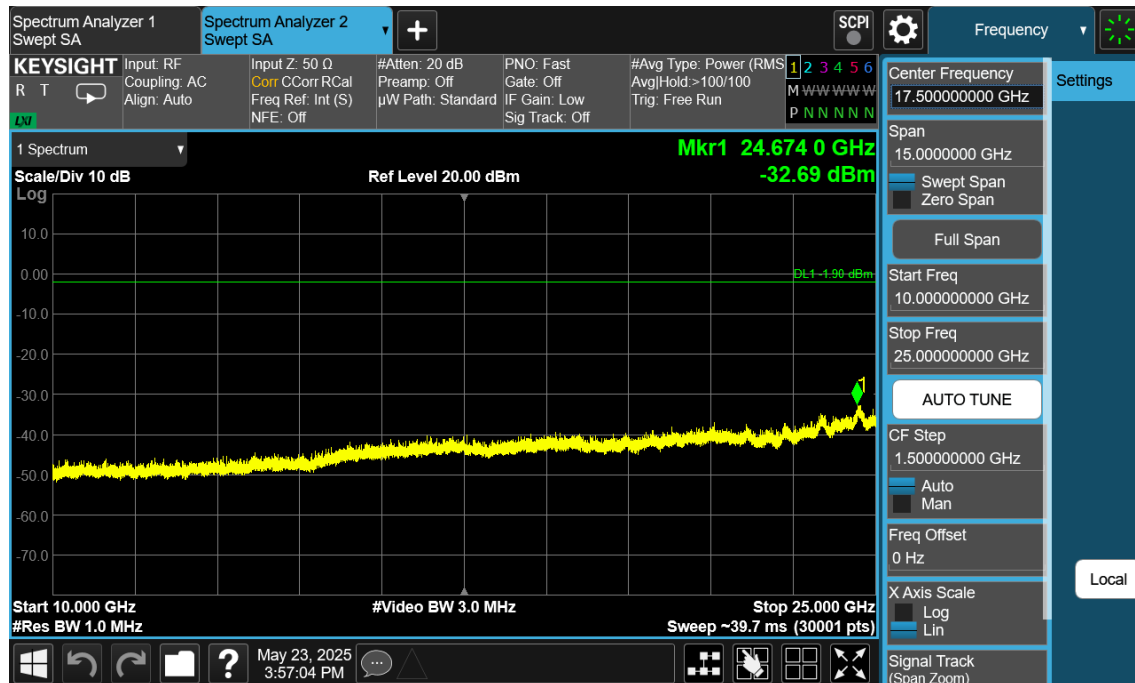
Plot 7-244. Conducted Spurious Plot Antenna WF9 (Bluetooth (LE), 1Mbps, ePA – Ch. 19)
