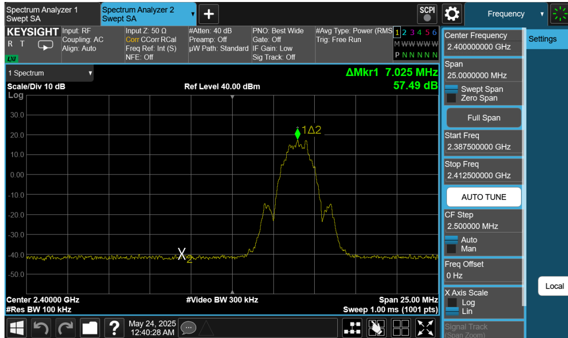
Plot 7-211. Band Edge Plot Antenna WF8 (Bluetooth (LE), 2Mbps, ePA – Ch. 1)
