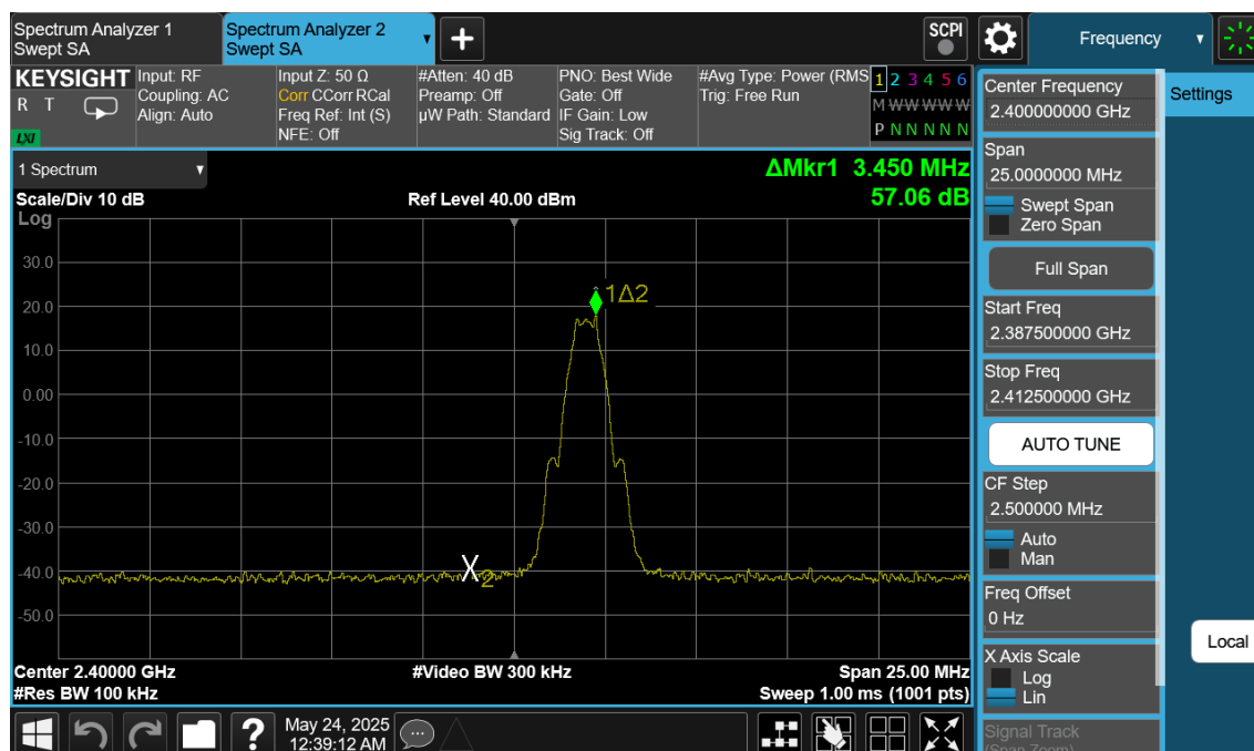
Plot 7-209. Band Edge Plot Antenna WF8 (Bluetooth (LE), 1Mbps, ePA – Ch.0)
