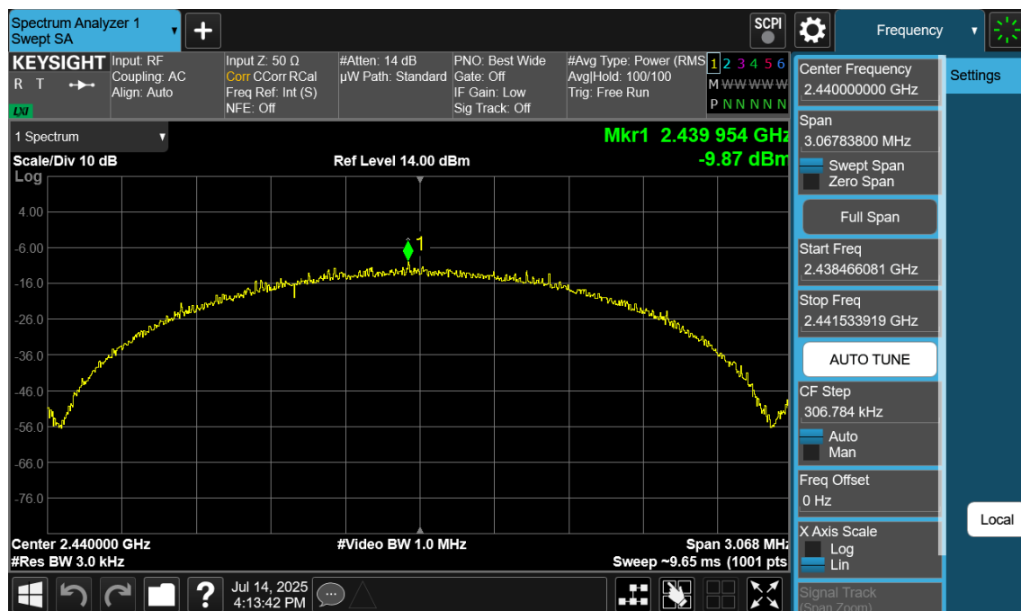
Plot 7-202. Power Spectral Density Plot Antenna WF9 (Bluetooth (LE), 2Mbps, iPA – Ch. 19)
