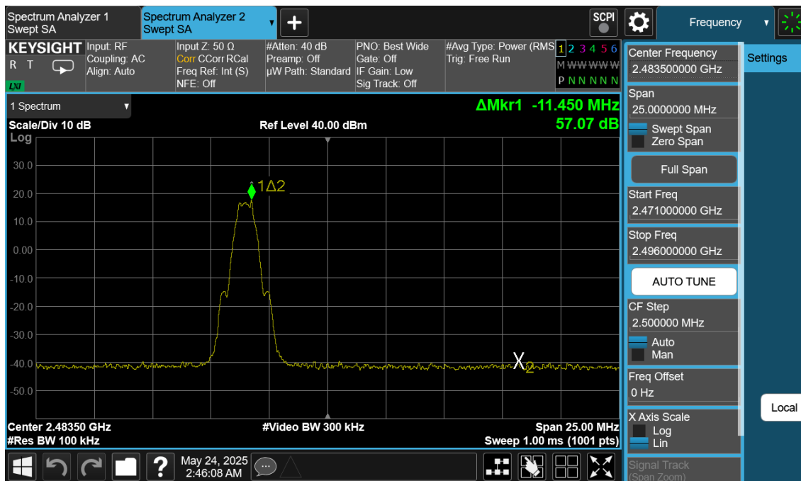
Plot 7-218. Band Edge Plot Antenna WF7 (Bluetooth (LE), 1Mbps, ePA – Ch. 39)
