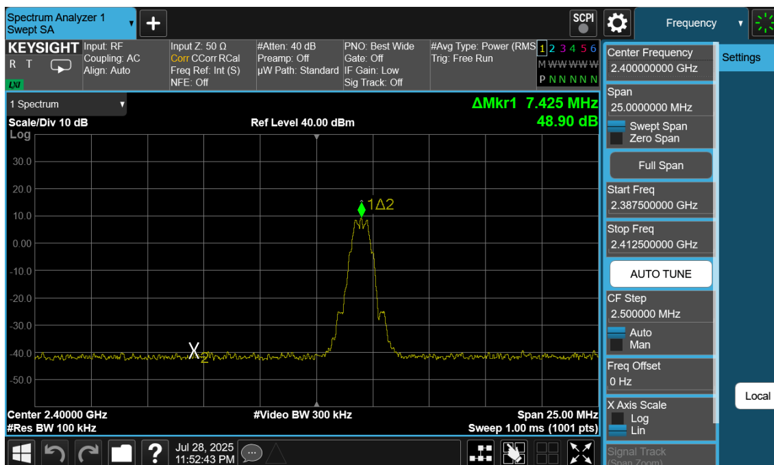
Plot 7-213. Band Edge Plot Antenna WF7 (Bluetooth (LE), 125kbps, ePA – Ch.0)
