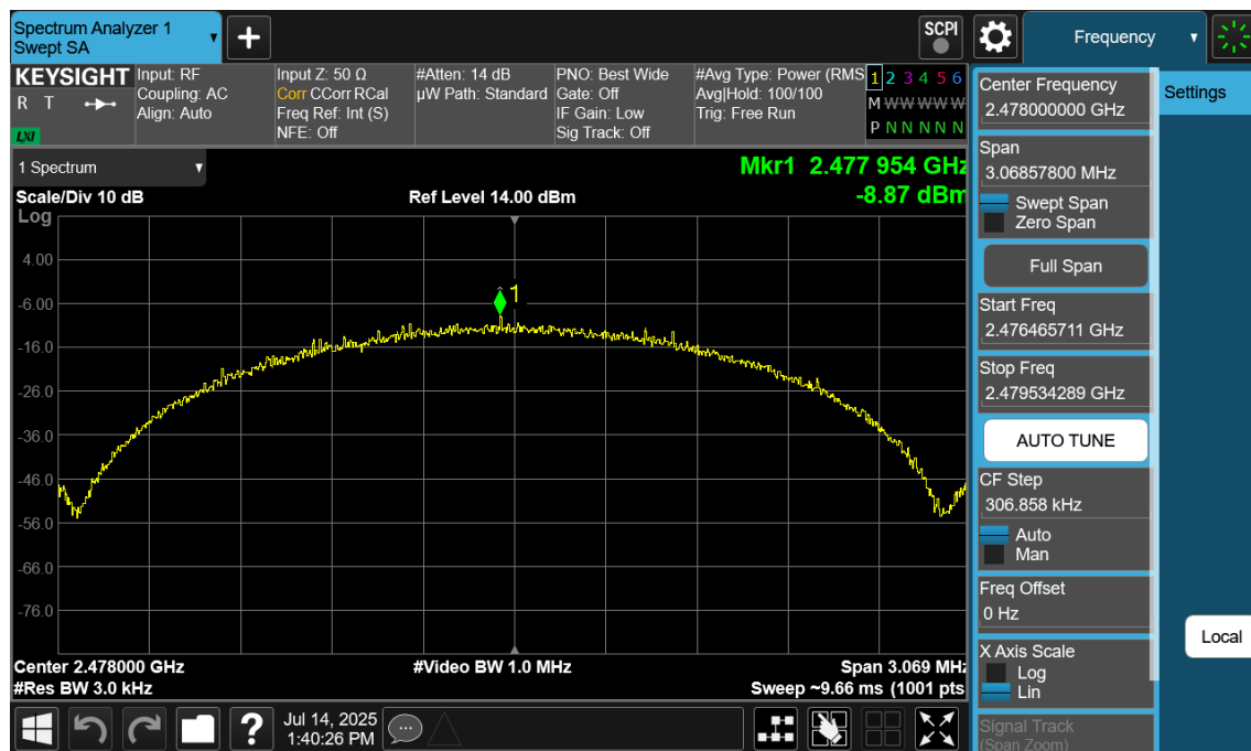
Plot 7-203. Power Spectral Density Plot Antenna WF8 (Bluetooth (LE), 2Mbps, iPA – Ch. 38)
