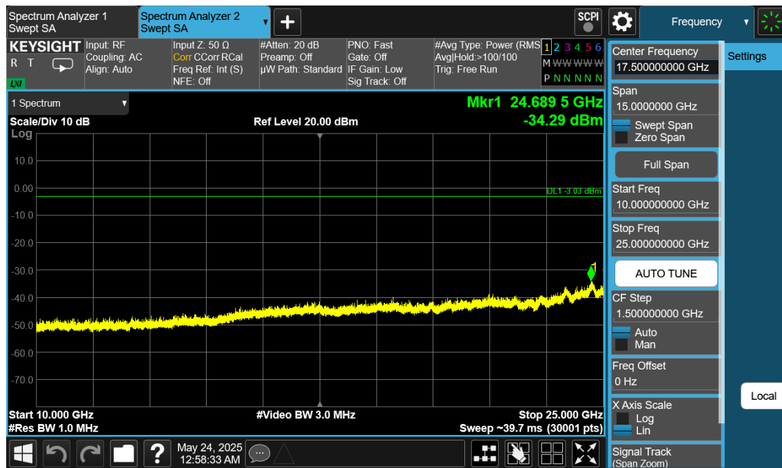
Plot 7-234. Conducted Spurious Plot Antenna WF8 (Bluetooth (LE), 1Mbps, ePA – Ch. 39)
