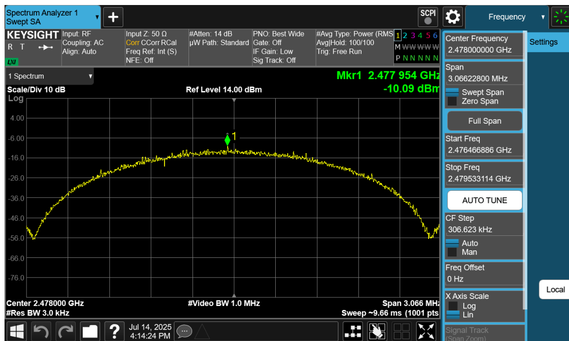
Plot 7-204. Power Spectral Density Plot Antenna WF9 (Bluetooth (LE), 2Mbps, iPA – Ch. 38)
