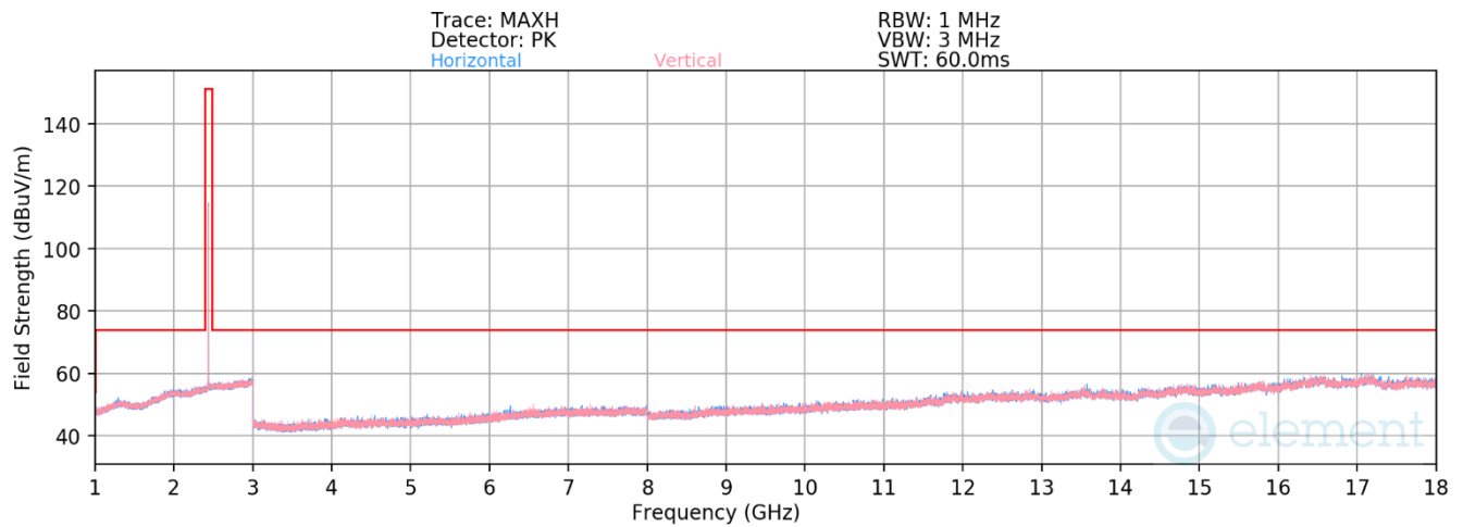
Plot 7-252. Radiated Spurious Emissions 1-18GHz TxBF Diversity (1Mbps, ePA – Ch. 19)
