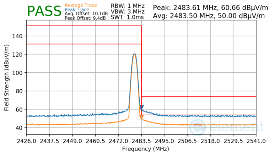
Plot 7-272. Radiated Restricted Upper Band Edge Measurement TxBF Diversity (Average & Peak)
