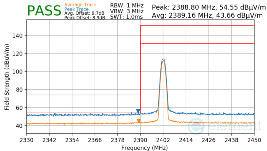
Plot 7-263. Radiated Restricted Lower Band Edge Measurement Antenna WF9 (Average & Peak)
