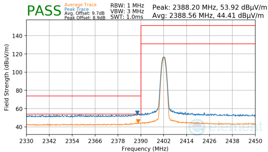
Plot 7-259. Radiated Restricted Lower Band Edge Measurement Antenna WF7 (Average & Peak)
