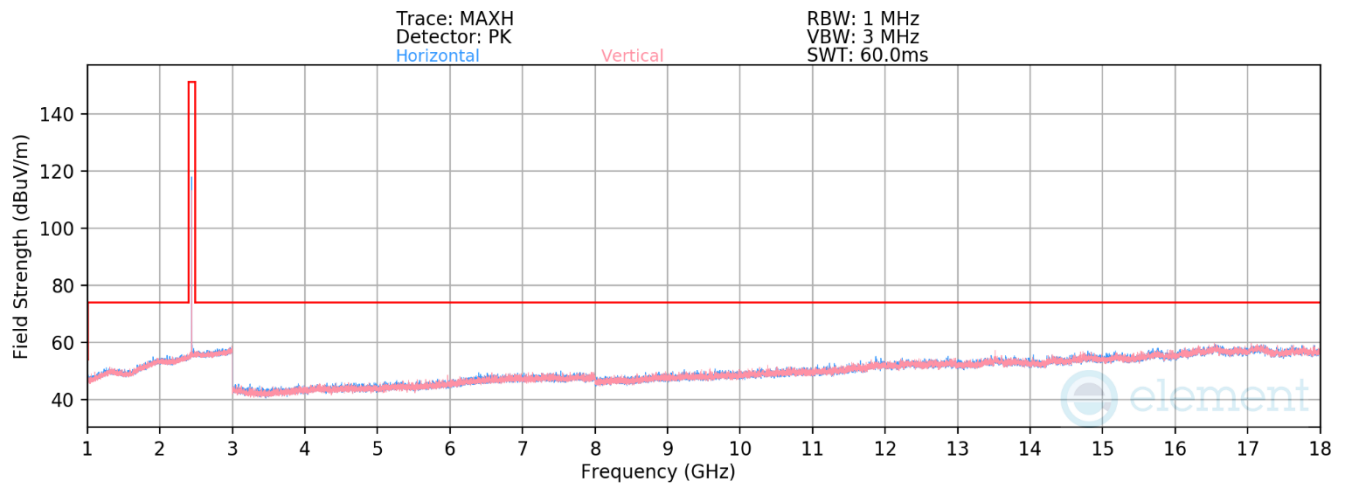
Plot 7-248. Radiated Spurious Emissions 1-18GHz TxBF Primary (1Mbps, ePA – Ch. 19)
