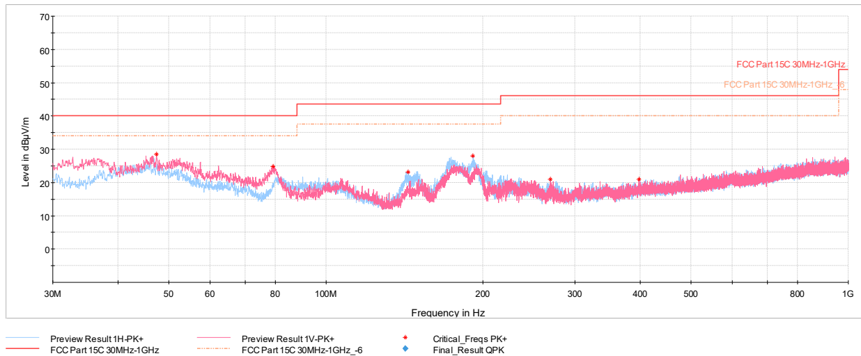
Plot 7-275. Radiated Spurious Emissions Below 1GHz TxBF Primary (1Mbps, ePA – Ch.19, Pol. H & V, with AC/DC Adapter)
