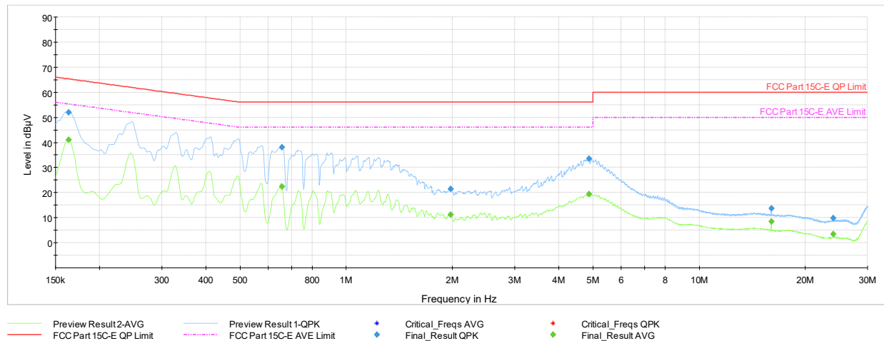
Plot 7-280. AC Line Conducted Plot with Bluetooth LE Tx BF Diversity (N, 1Mbps ePA – Ch.19, with AC/DC Adapter)
