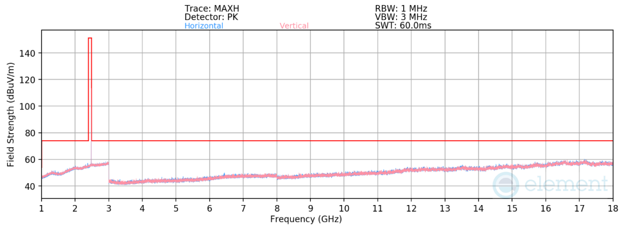
Plot 7-249. Radiated Spurious Emissions 1-18GHz TxBF Primary (1Mbps ePA – Ch. 39)
