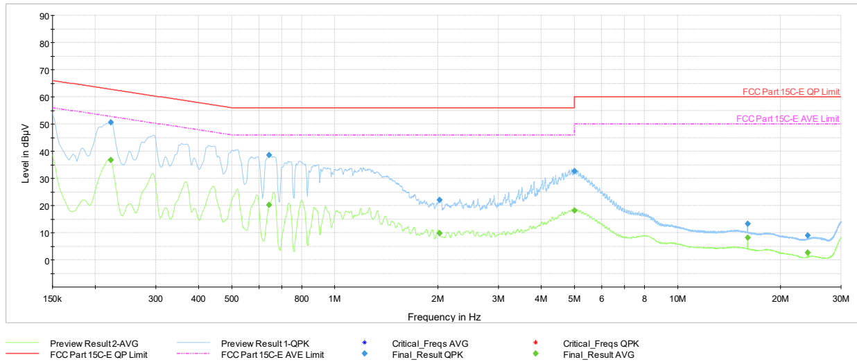
Plot 7-278. AC Line Conducted Plot with Bluetooth LE Tx BF Primary (N, 1Mbps ePA – Ch.19, with AC/DC Adapter)
