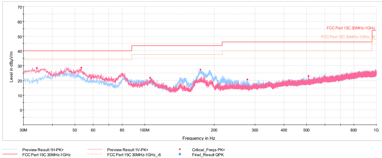
Plot 7-276. Radiated Spurious Emissions Below 1GHz TxBF Diversity (1Mbps, ePA – Ch.19, Pol. H & V, with AC/DC Adapter)
