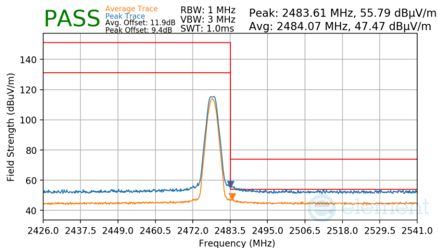
Plot 7-266. Radiated Restricted Upper Band Edge Measurement Antenna WF9 (Average & Peak)
