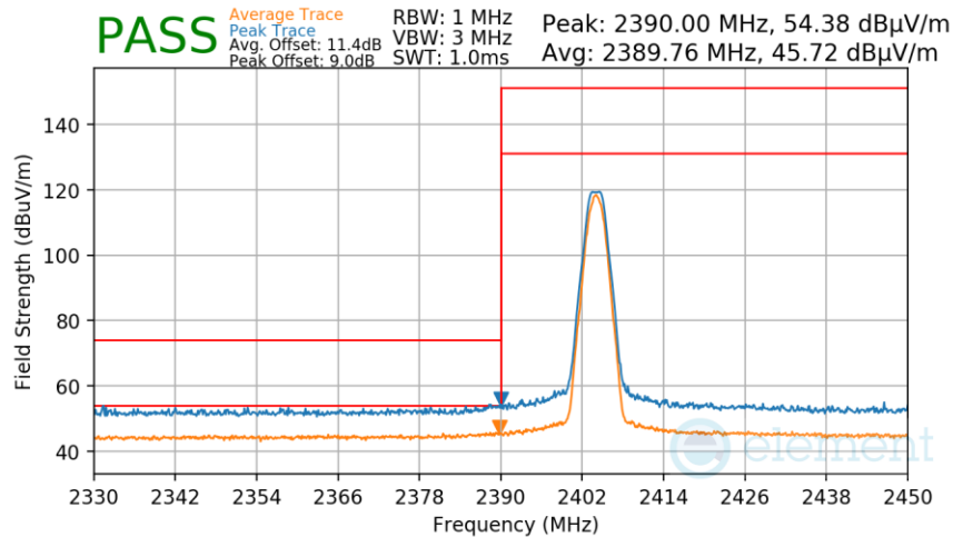
Plot 7-273. Radiated Restricted Lower Band Edge Measurement TxBF Diversity (Average & Peak)
