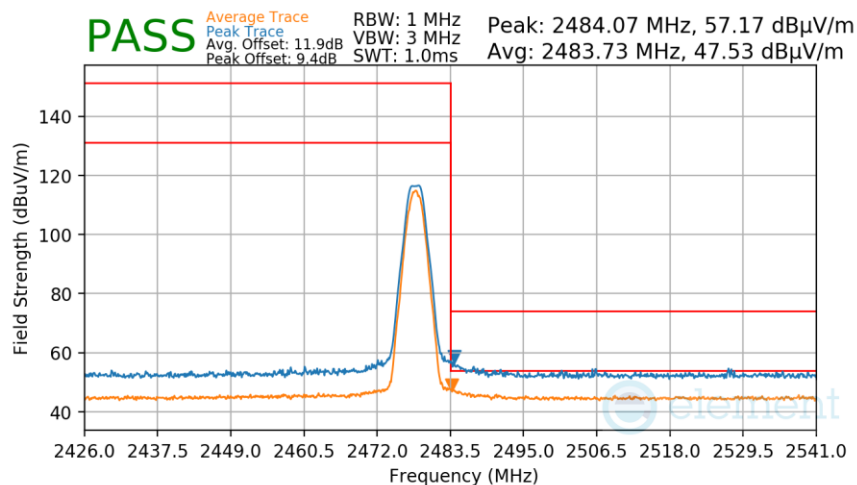
Plot 7-262. Radiated Restricted Upper Band Edge Measurement Antenna WF7 (Average & Peak)
