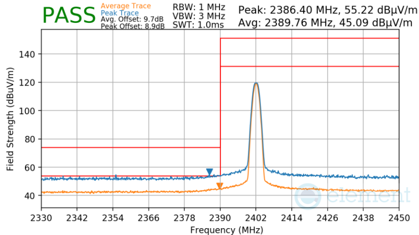
Plot 7-267. Radiated Restricted Lower Band Edge Measurement TxBF Primary (Average & Peak)
