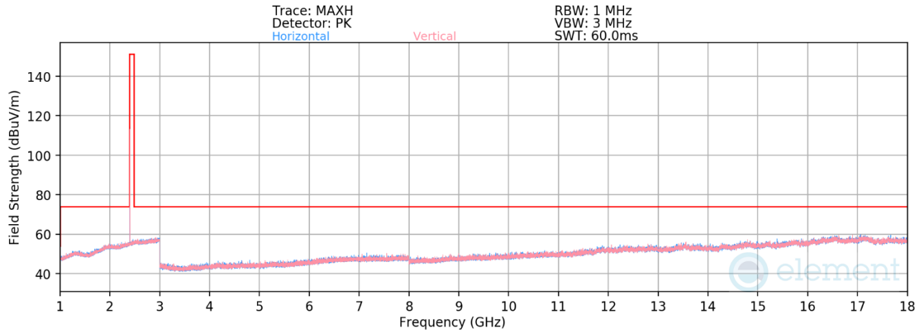
Plot 7-251. Radiated Spurious Emissions 1-18GHz TxBF Diversity (1Mbps, ePA – Ch. 0)
