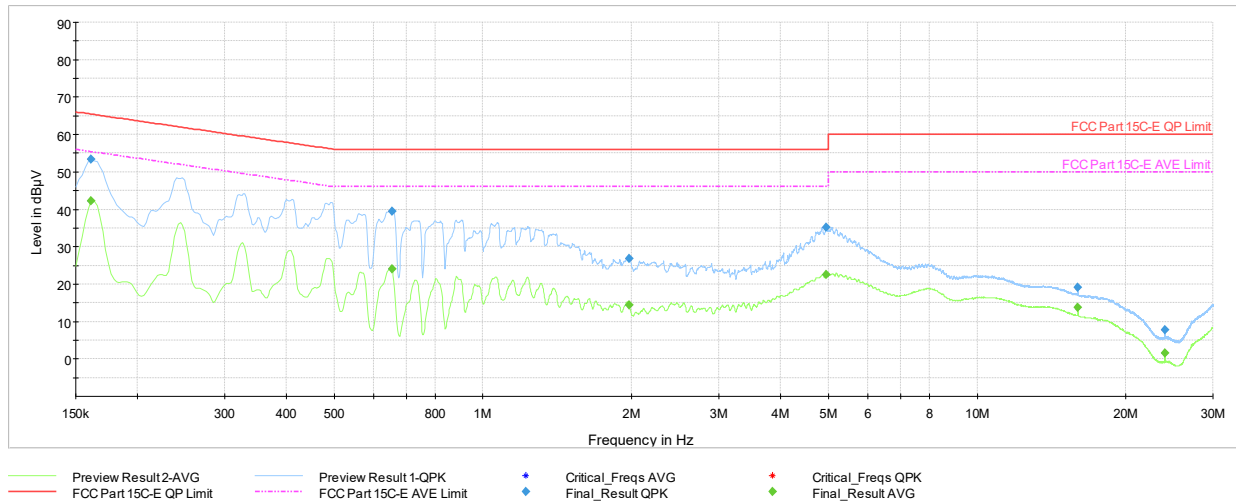
Plot 7-277. AC Line Conducted Plot with Bluetooth LE Tx BF Primary (L1, 1Mbps ePA – Ch.19 with AC/DC Adapter)
