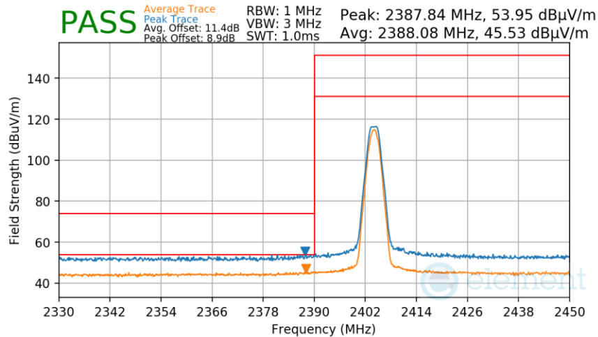
Plot 7-261. Radiated Restricted Lower Band Edge Measurement Antenna WF7 (Average & Peak)
