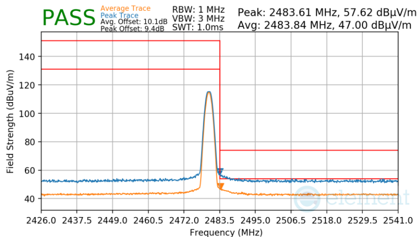
Plot 7-264. Radiated Restricted Upper Band Edge Measurement Antenna WF9 (Average & Peak)
