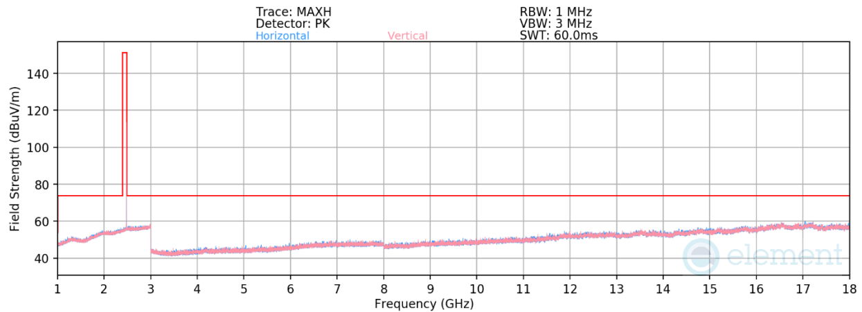
Plot 7-253. Radiated Spurious Emissions 1-18GHz TxBF Diversity (1Mbps ePA – Ch. 39)
