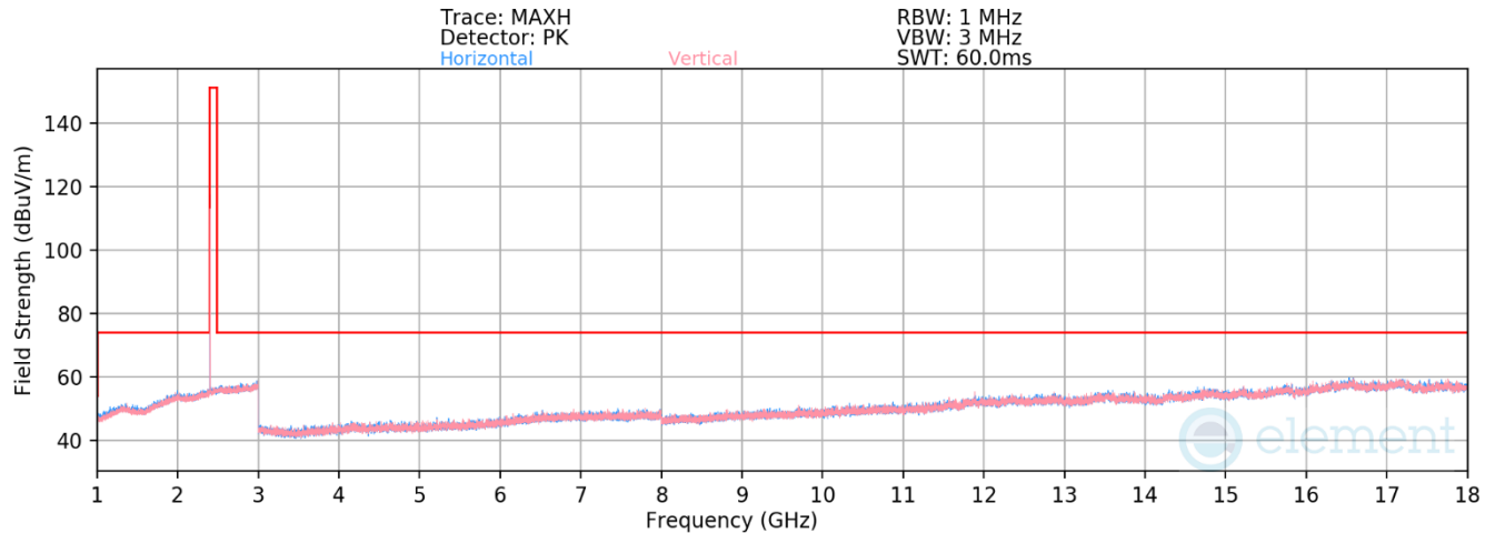
Plot 7-247. Radiated Spurious Emissions 1-18GHz TxBF Primary (1Mbps, ePA – Ch. 0)
