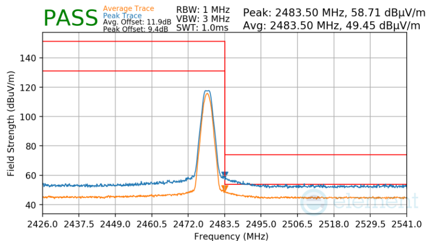
Plot 7-258. Radiated Restricted Upper Band Edge Measurement Antenna WF8 (Average & Peak)
