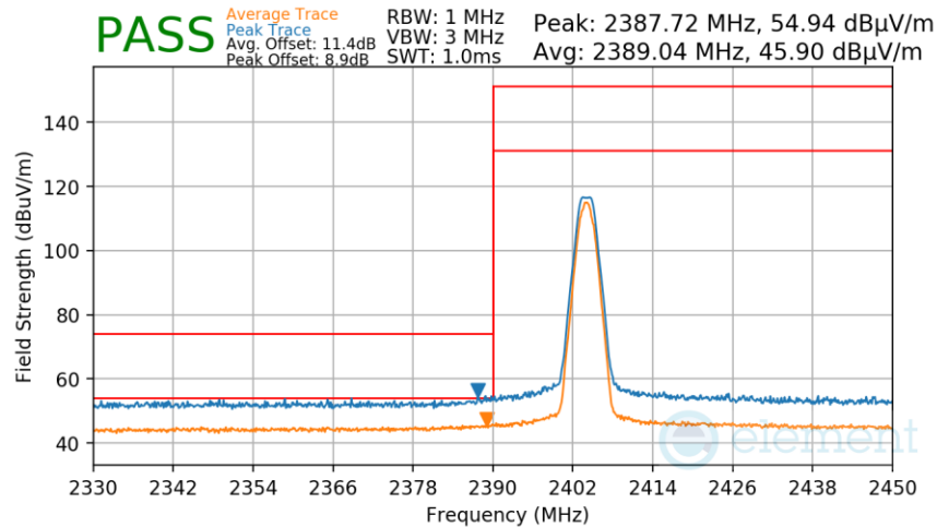
Plot 7-257. Radiated Restricted Lower Band Edge Measurement Antenna WF8 (Average & Peak)
