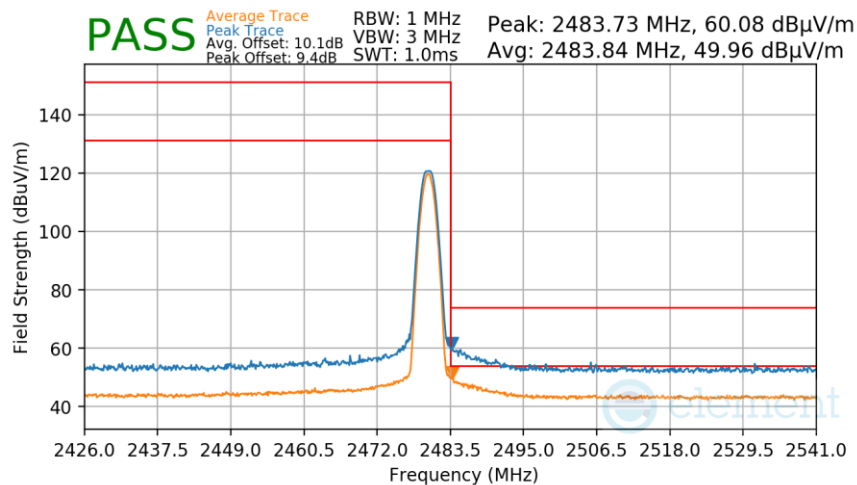
Plot 7-268. Radiated Restricted Upper Band Edge Measurement TxBF Primary (Average & Peak)
