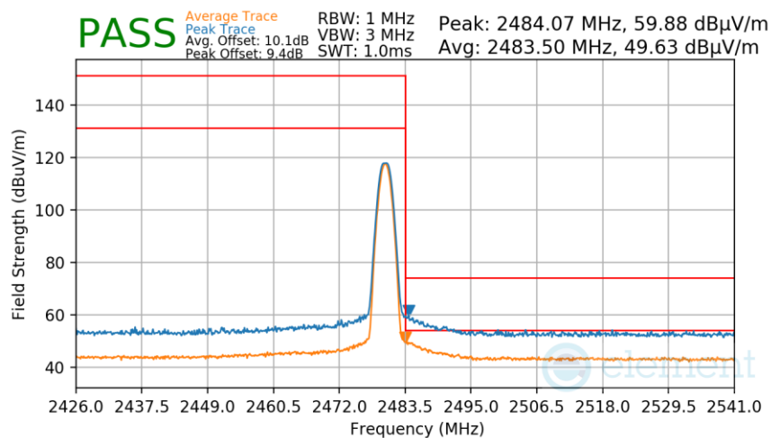
Plot 7-256. Radiated Restricted Upper Band Edge Measurement Antenna WF8 (Average & Peak)
