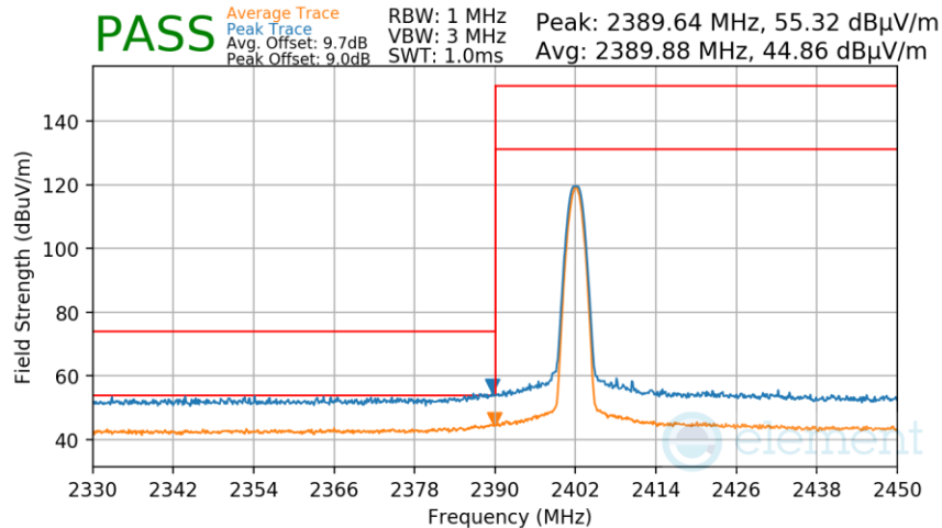
Plot 7-271. Radiated Restricted Lower Band Edge Measurement TxBF Diversity (Average & Peak)
