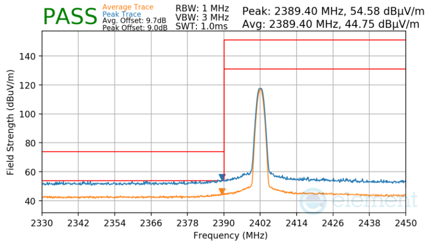
Plot 7-255. Radiated Restricted Lower Band Edge Measurement Antenna WF8 (Average & Peak)
