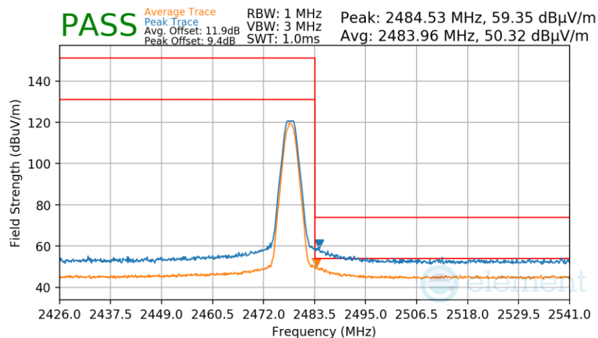
Plot 7-270. Radiated Restricted Upper Band Edge Measurement TxBF Primary (Average & Peak)
