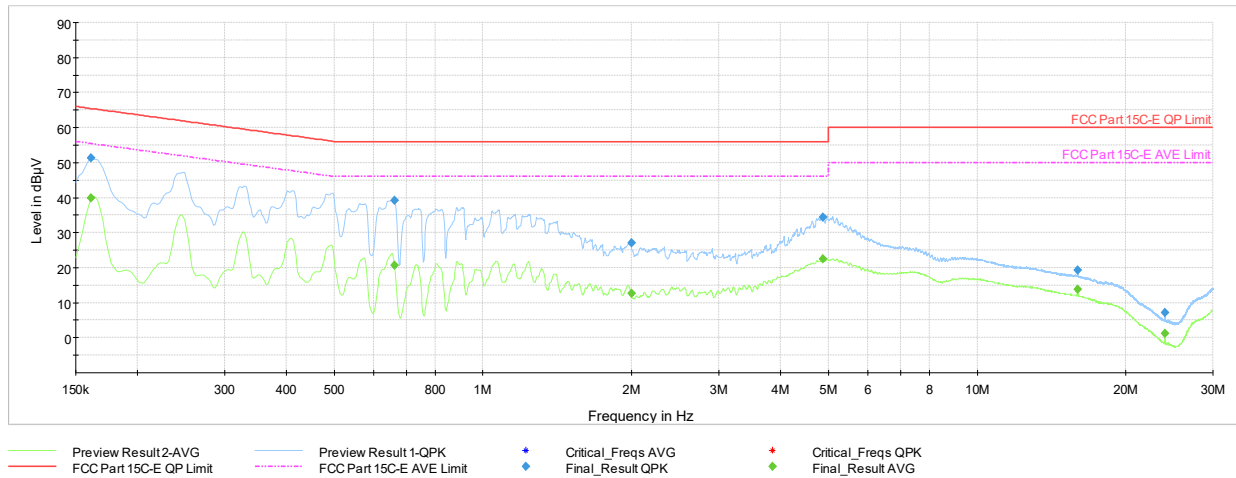
Plot 7-279. AC Line Conducted Plot with Bluetooth LE TxBF Diversity (L1, 1Mbps ePA – Ch.19 with AC/DC Adapter)
