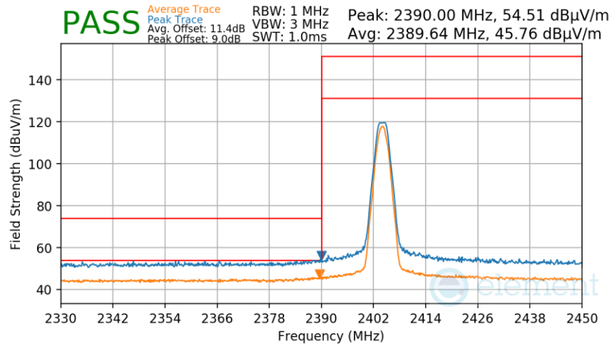
Plot 7-269. Radiated Restricted Lower Band Edge Measurement TxBF Primary (Average & Peak)
