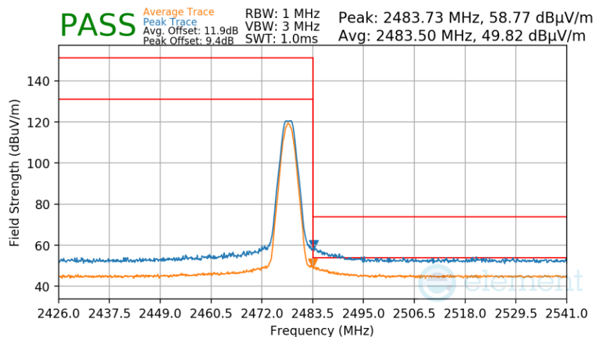
Plot 7-274. Radiated Restricted Upper Band Edge Measurement TxBF Diversity (Average & Peak)
