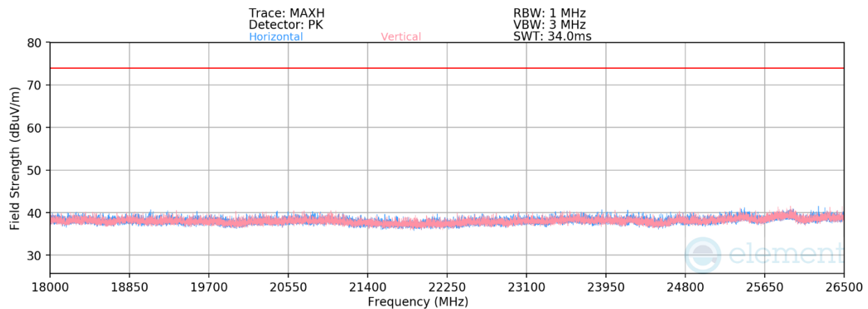
Plot 7-254. Radiated Spurious Emissions Above 18GHz TxBF Diversity (1Mbps ePA – Ch. 39)
