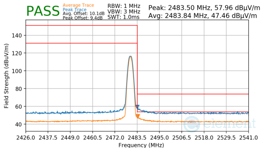
Plot 7-260. Radiated Restricted Upper Band Edge Measurement Antenna WF7 (Average & Peak)
