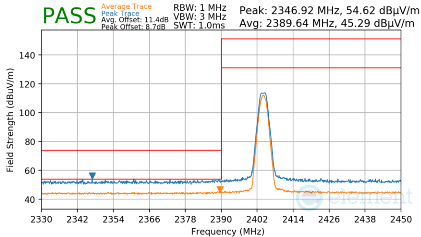
Plot 7-265. Radiated Restricted Lower Band Edge Measurement Antenna WF9 (Average & Peak)
