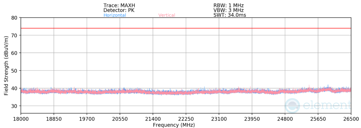
Plot 7-250. Radiated Spurious Emissions Above 18GHz TxBF Primary (1Mbps ePA – Ch. 39)
