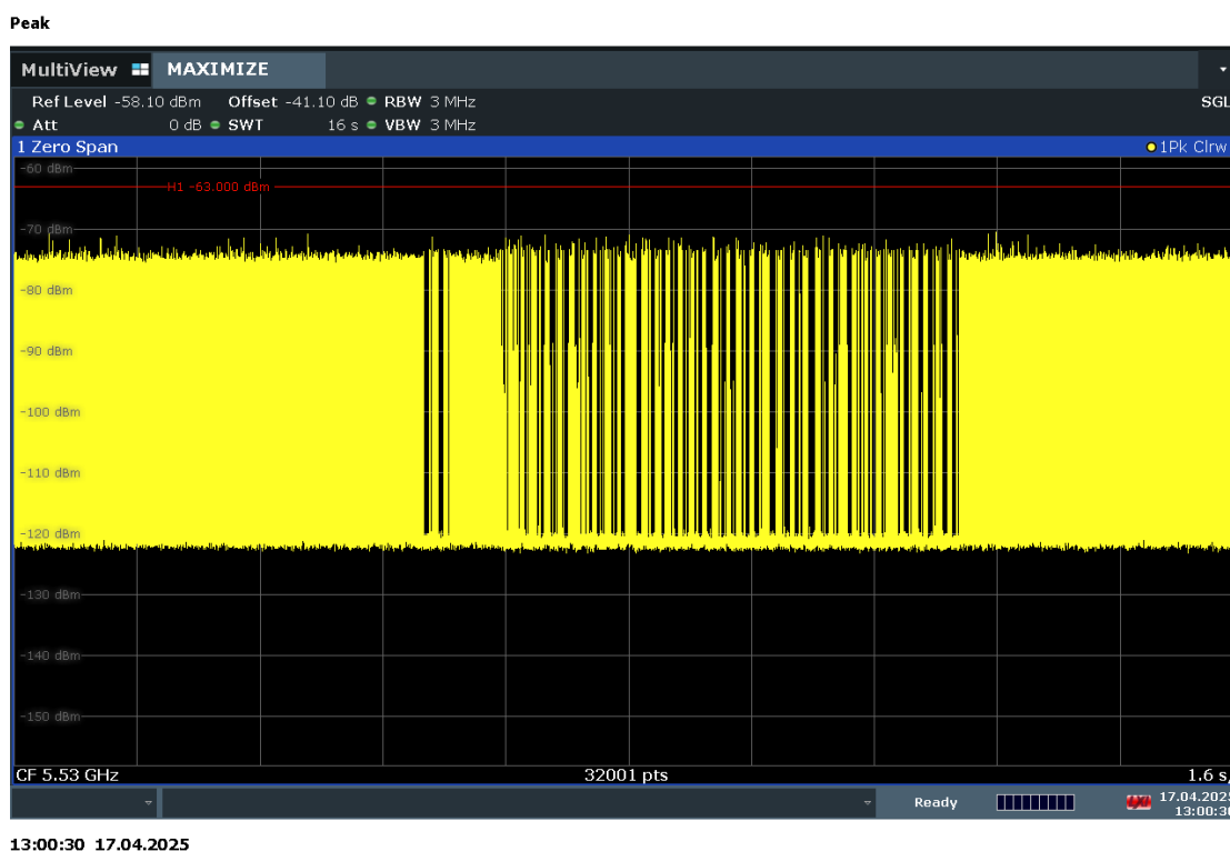
Figure 9-1. 5530MHz - Channel Loading - Mode 1 (80MHz)
