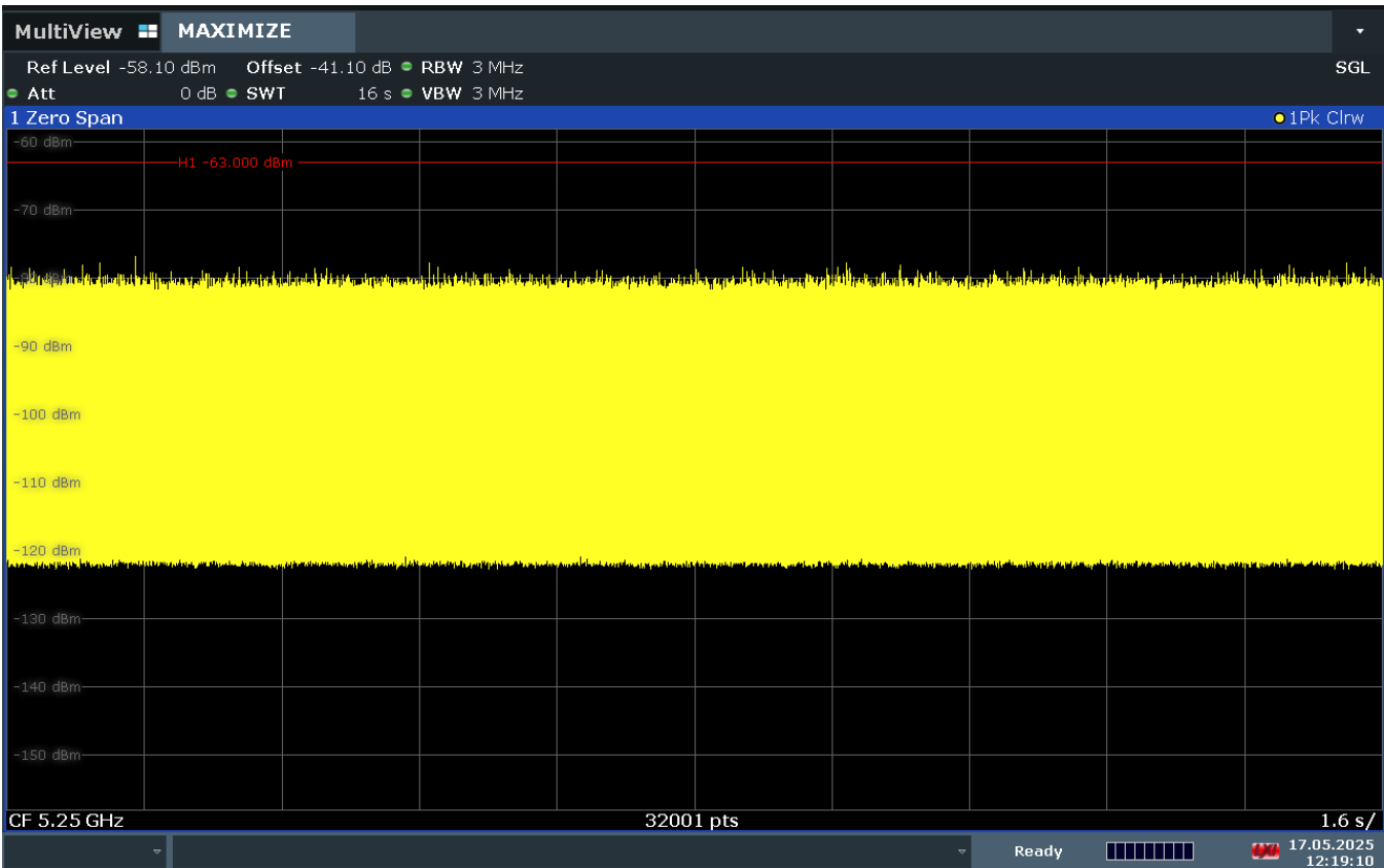
Figure 9-3. 5250MHz - Channel Loading - Mode 1 (160MHz)
