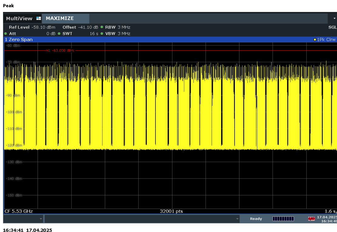
Figure 9-9. 5530 MHz - Channel Loading - Mode 4 (80MHz)
