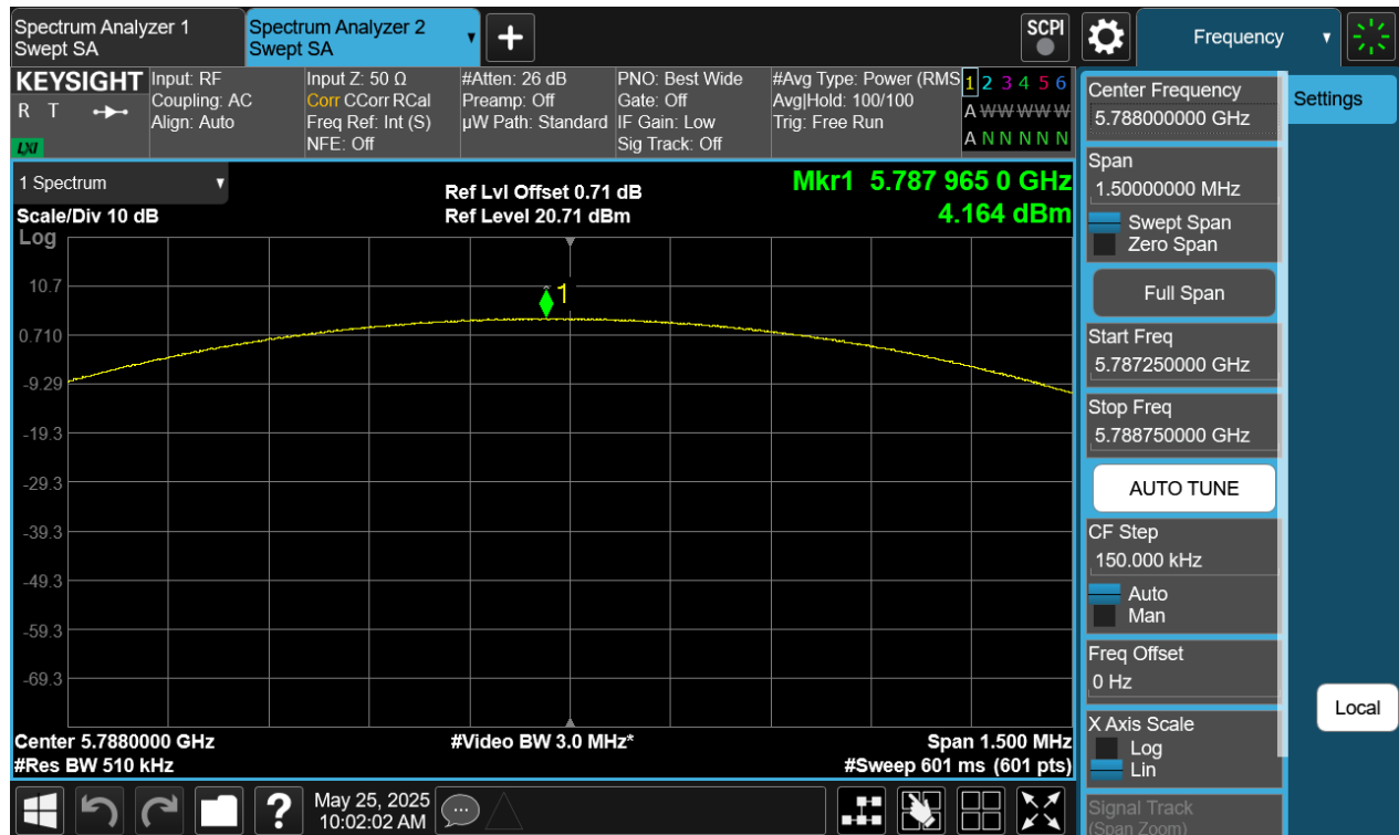
Plot 7-108. PSD Antenna WF5B (NB UNII LE1M, iPA – 5788MHz)
