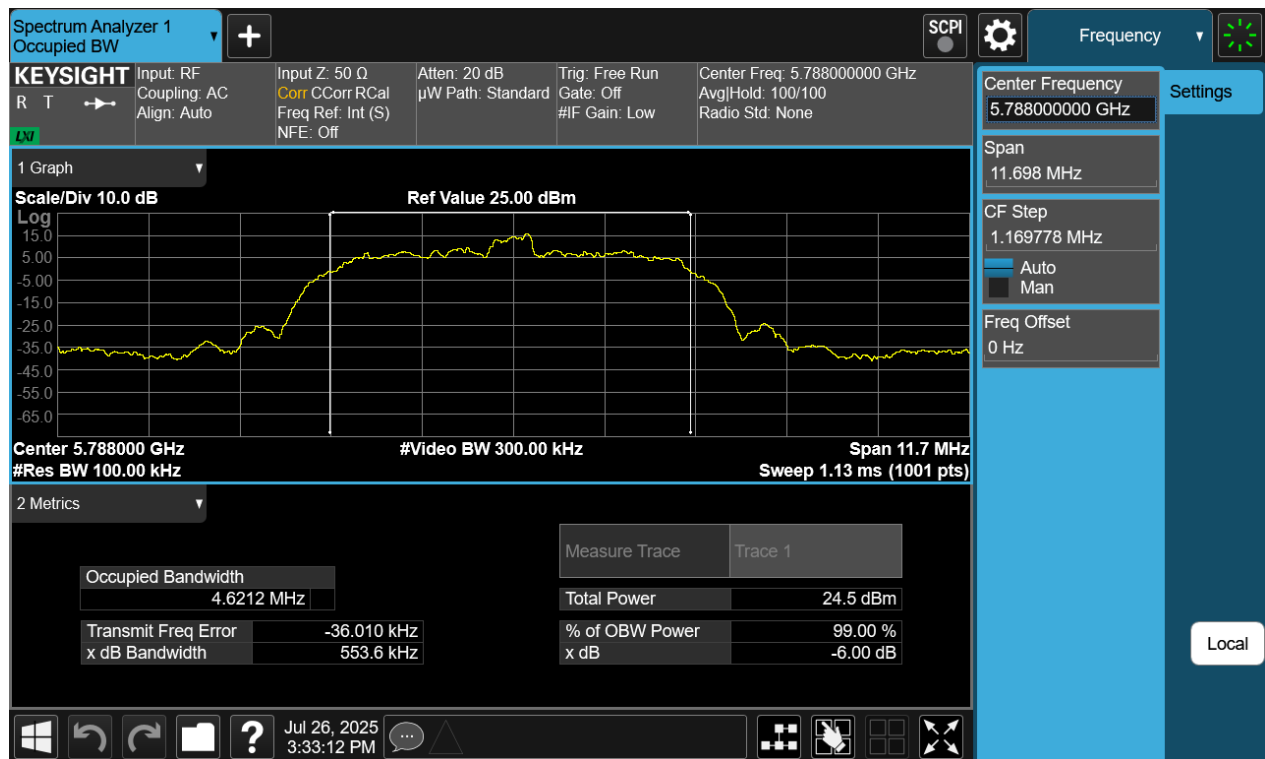
Plot 7-70. 6dB BW & 99% OBW Antenna WF7 (NB UNII HDR8, ePA – 5788MHz)
