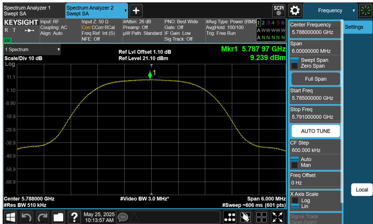
Plot 7-111. PSD Antenna WF5B (NB UNII HDR4, ePA – 5788MHz)
