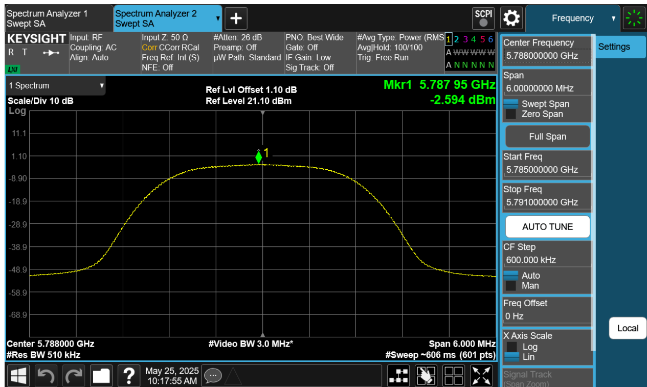
Plot 7-112. PSD Antenna WF5B (NB UNII HDR4, iPA – 5788MHz)
