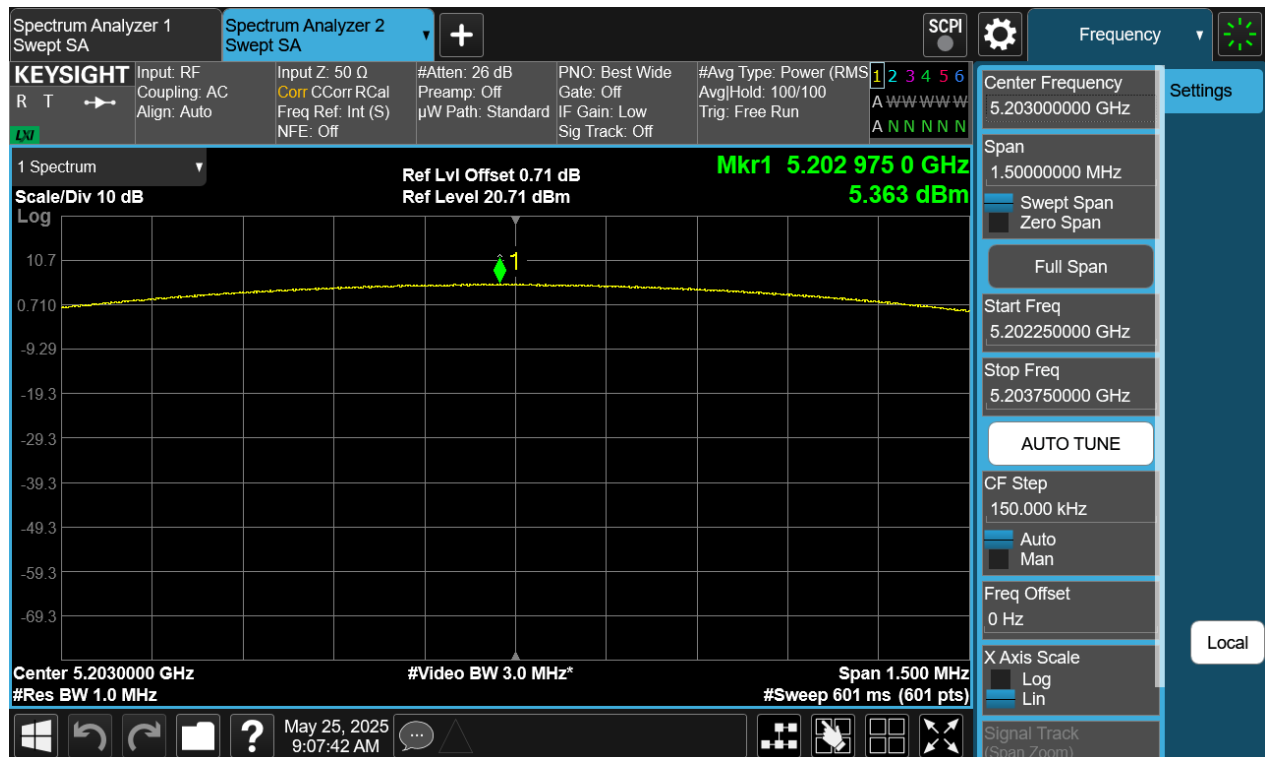
Plot 7-82. PSD Antenna WF5B (NB UNII LE1M, iPA – 5203MHz)
