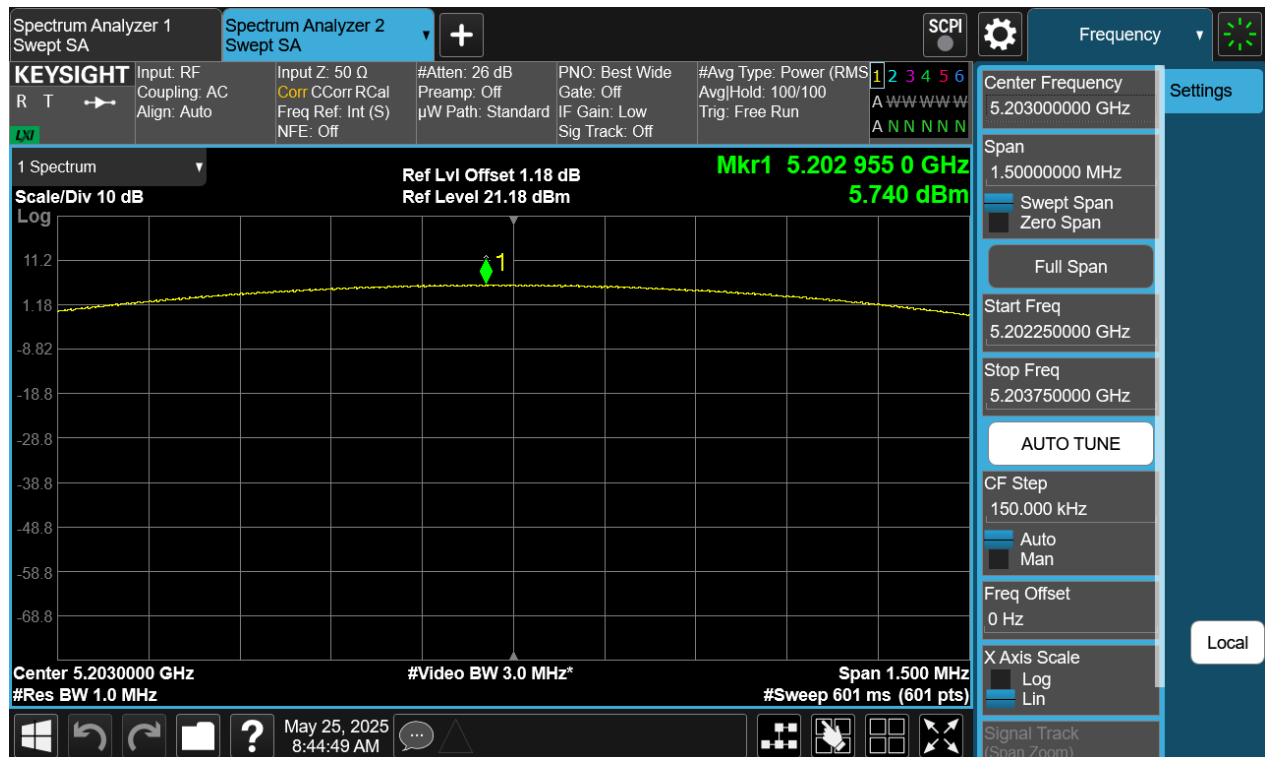
Plot 7-80. PSD Antenna WF5B (NB UNII BDR, iPA – 5203MHz)
