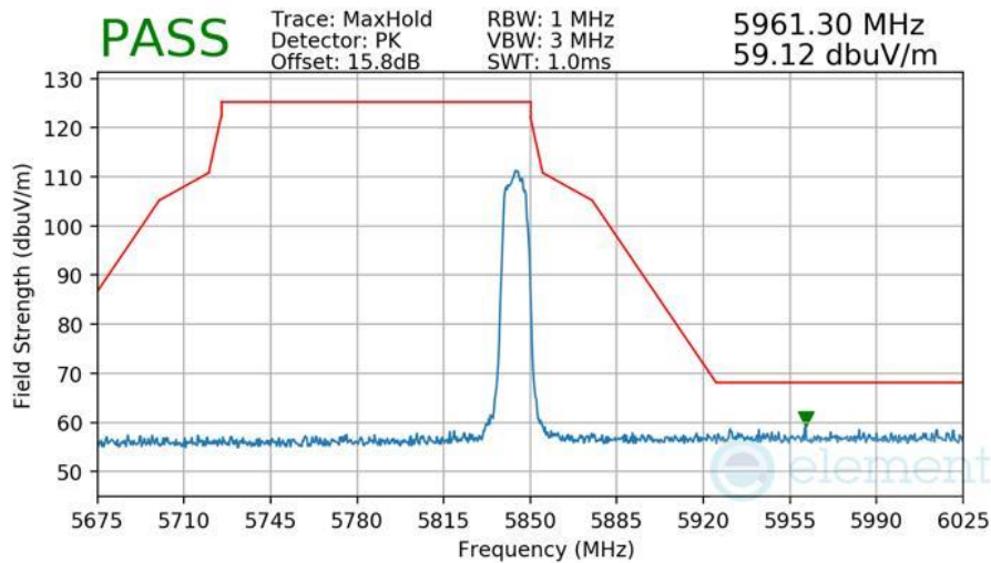
Plot 7-596 Radiated Higher Band Edge Measurement Antenna WF7
