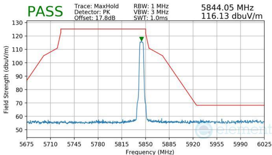
Plot 7-557 Radiated Higher Band Edge Measurement Antenna WF8
