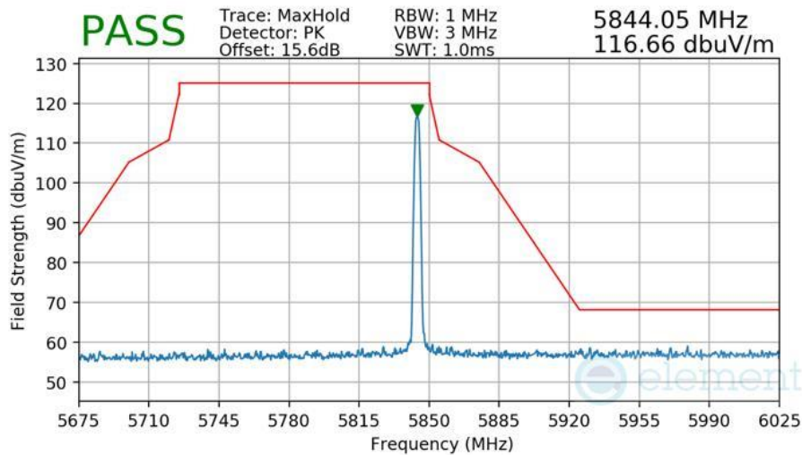
Plot 7-588 Radiated Higher Band Edge Measurement Antenna WF7
