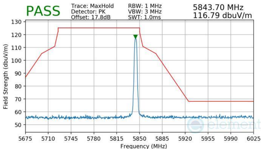
Plot 7-561 Radiated Higher Band Edge Measurement Antenna WF8
