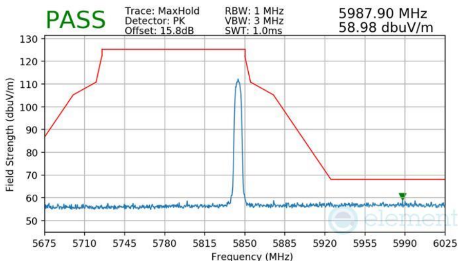
Plot 7-594 Radiated Higher Band Edge Measurement Antenna WF7
