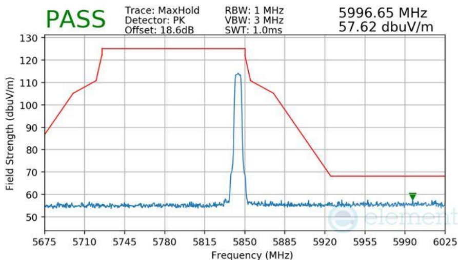
Plot 7-593 Radiated Higher Band Edge Measurement Antenna WF7
