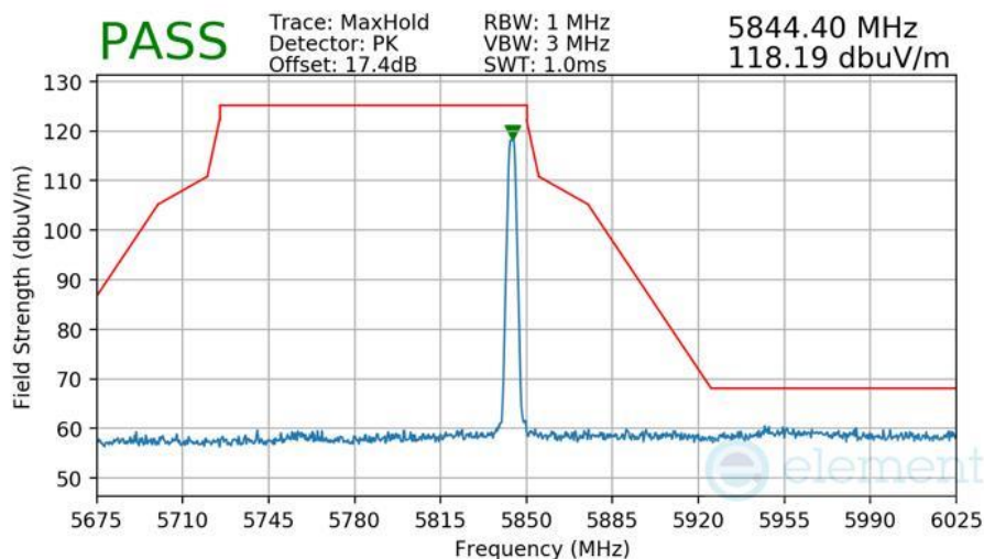
Plot 7-589 Radiated Higher Band Edge Measurement Antenna WF7
