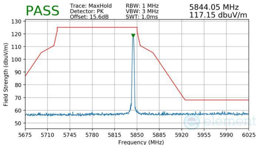
Plot 7-551 Radiated Higher Band Edge Measurement Antenna WF8
