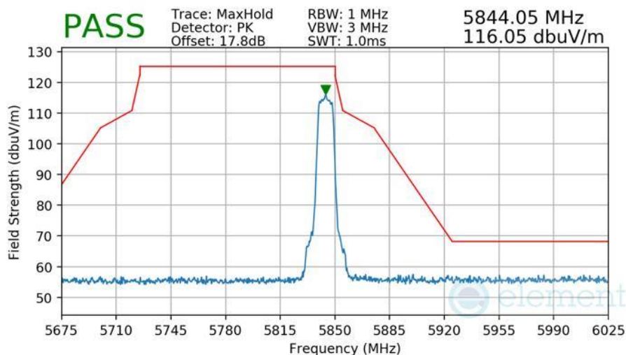
Plot 7-559 Radiated Higher Band Edge Measurement Antenna WF8
