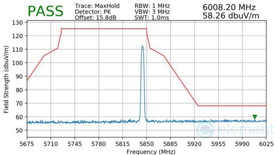
Plot 7-598 Radiated Higher Band Edge Measurement Antenna WF7
