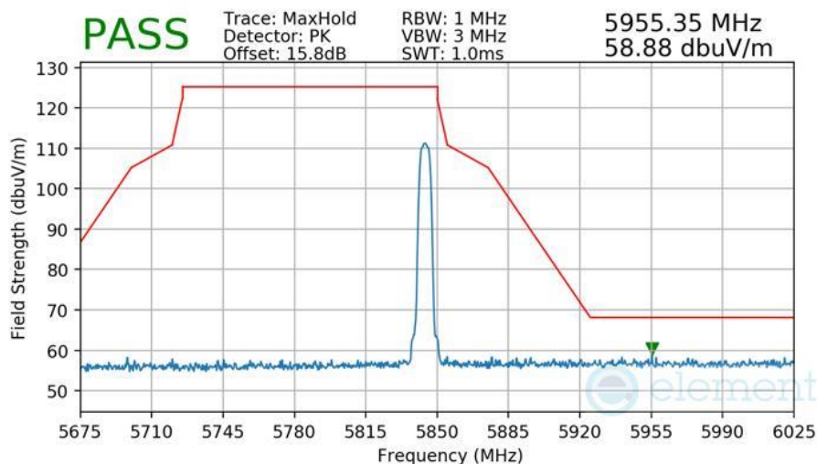
Plot 7-591 Radiated Higher Band Edge Measurement Antenna WF7
