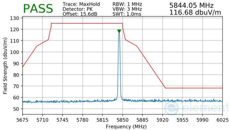
Plot 7-587 Radiated Higher Band Edge Measurement Antenna WF7
