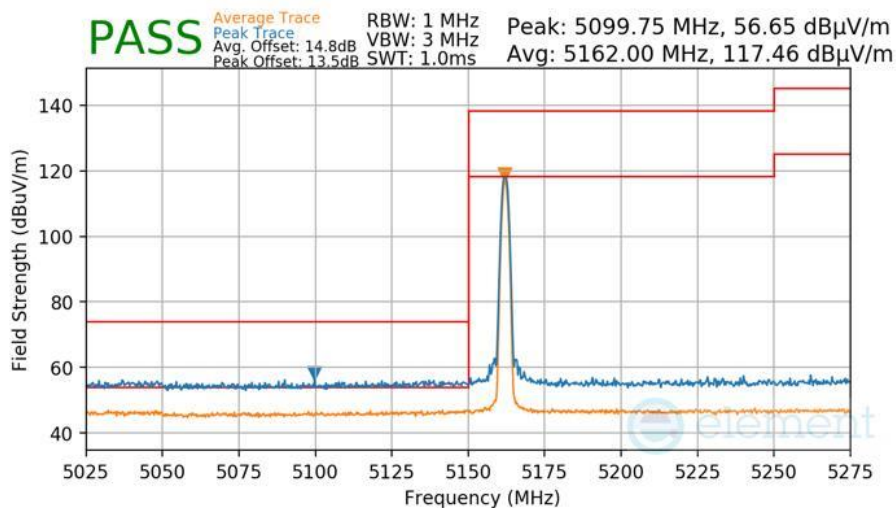
Plot 7-599 Radiated Lower Band Edge Measurement Antenna TxBF Primary
