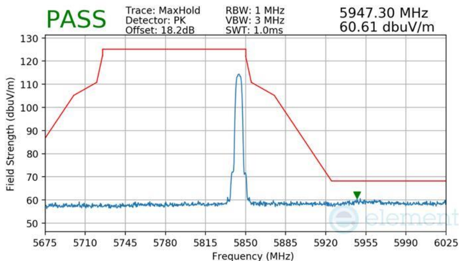
Plot 7-555 Radiated Higher Band Edge Measurement Antenna WF8
