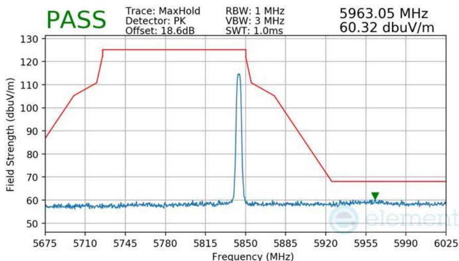
Plot 7-590 Radiated Higher Band Edge Measurement Antenna WF7
