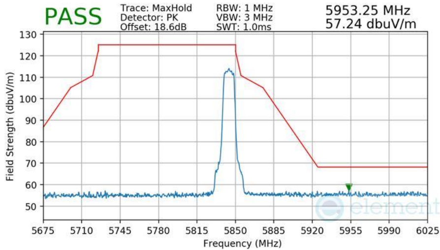
Plot 7-595 Radiated Higher Band Edge Measurement Antenna WF7
