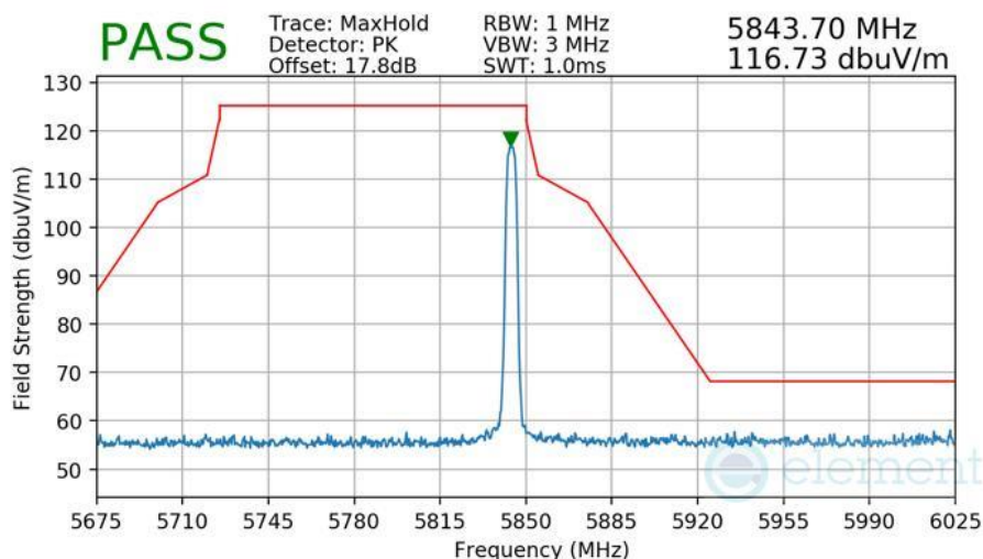
Plot 7-556 Radiated Higher Band Edge Measurement Antenna WF8
