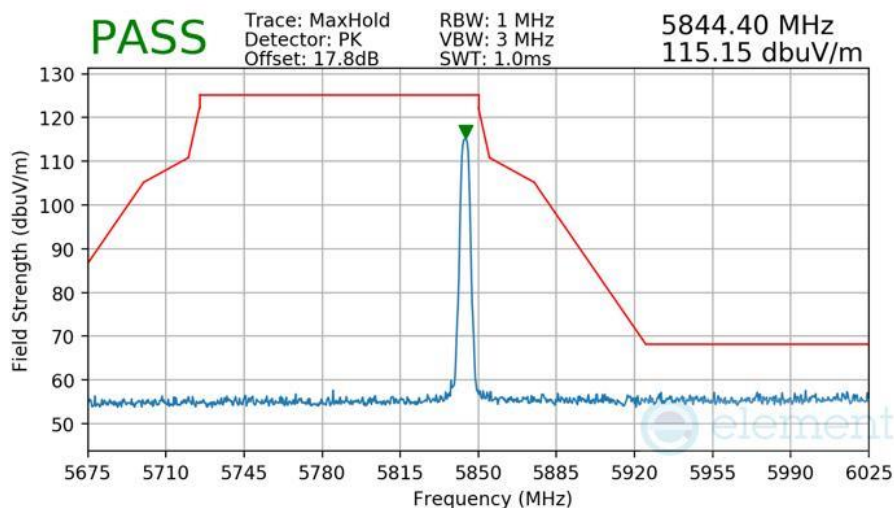
Plot 7-597 Radiated Higher Band Edge Measurement Antenna WF7
