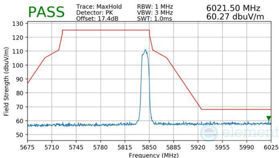
Plot 7-524 Radiated Higher Band Edge Measurement Antenna WF5B
