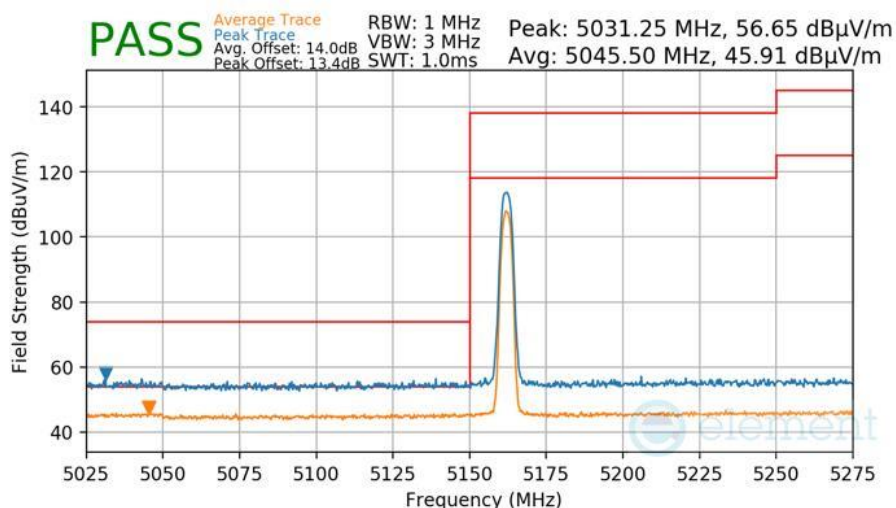
Plot 7-538 Radiated Lower Band Edge Measurement Antenna WF8
