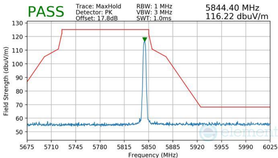
Plot 7-525 Radiated Higher Band Edge Measurement Antenna WF5B
