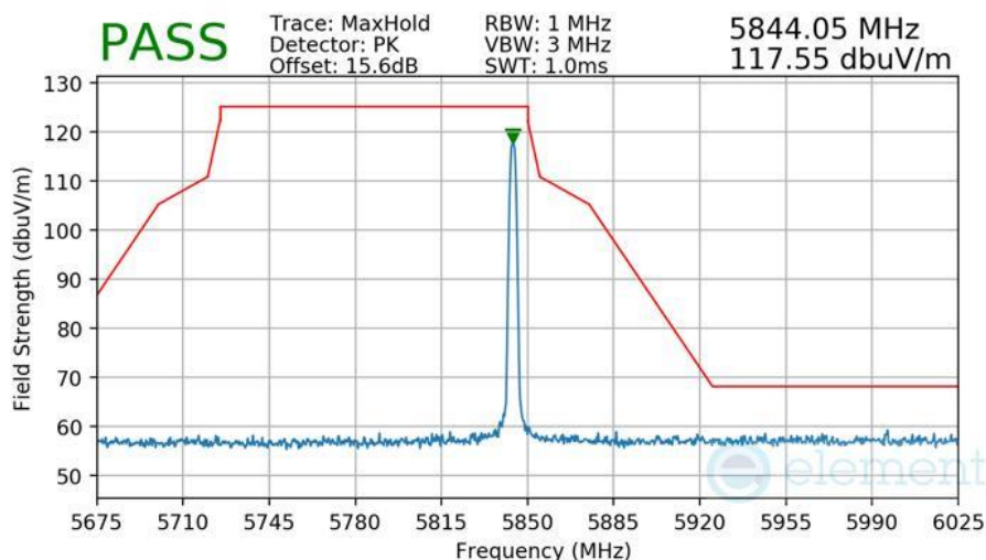
Plot 7-552 Radiated Higher Band Edge Measurement Antenna WF8
