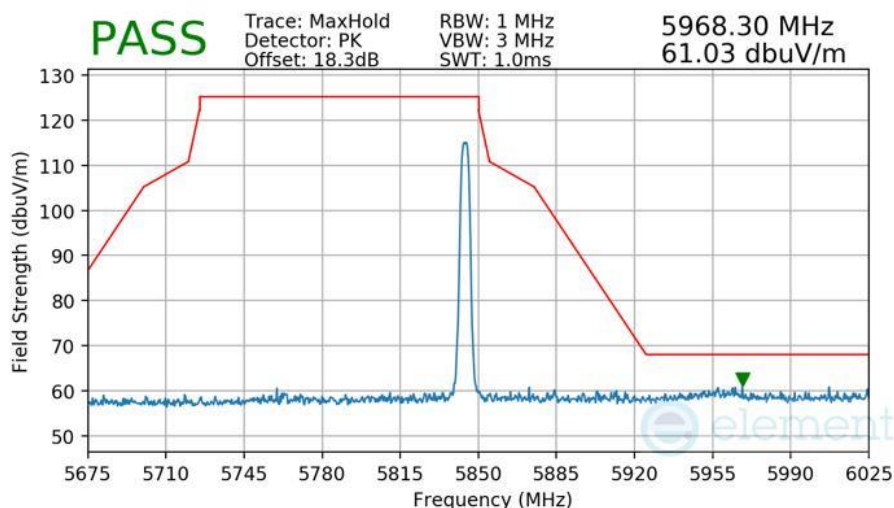
Plot 7-554 Radiated Higher Band Edge Measurement Antenna WF8
