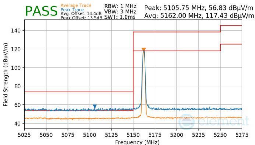
Plot 7-600 Radiated Lower Band Edge Measurement Antenna TxBF Primary
