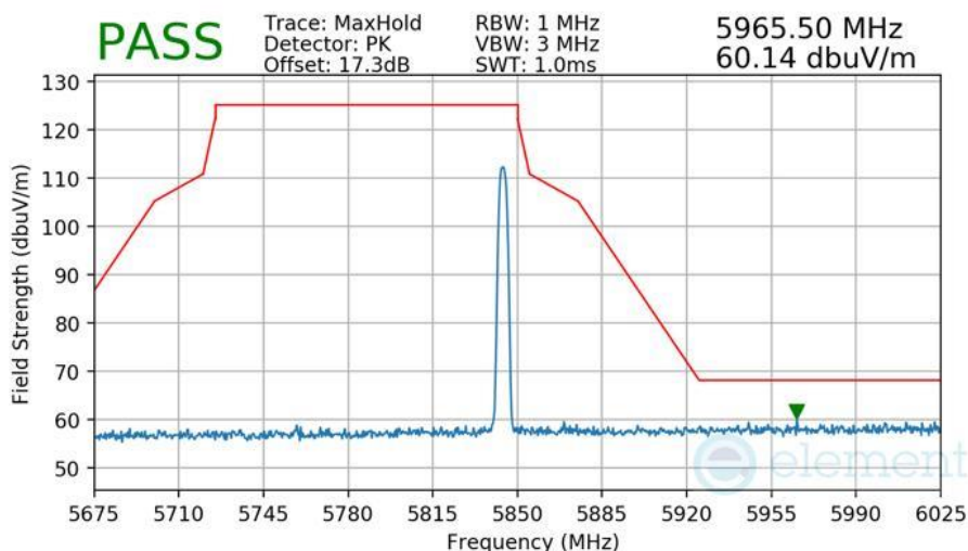
Plot 7-526 Radiated Higher Band Edge Measurement Antenna WF5B
