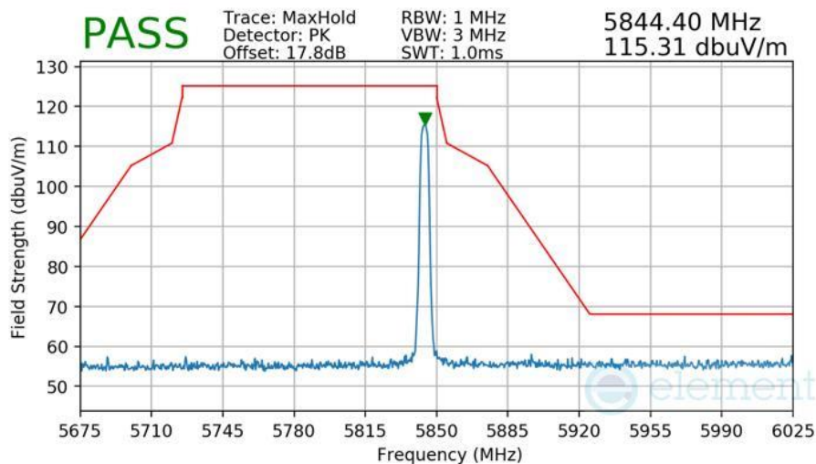
Plot 7-592 Radiated Higher Band Edge Measurement Antenna WF7
