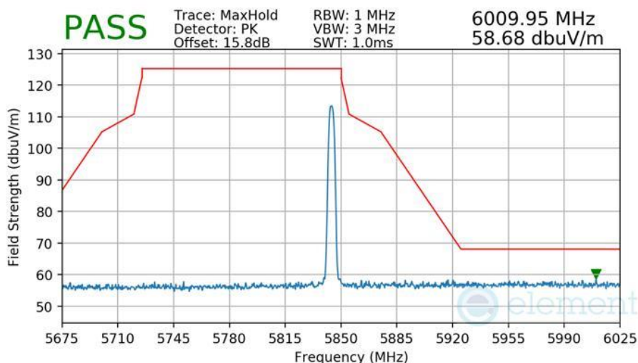
Plot 7-562 Radiated Higher Band Edge Measurement Antenna WF8
