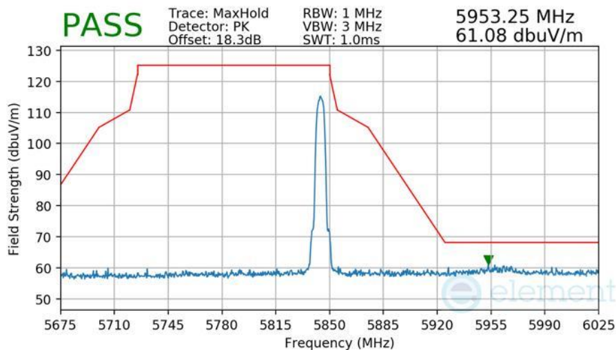
Plot 7-558 Radiated Higher Band Edge Measurement Antenna WF8
