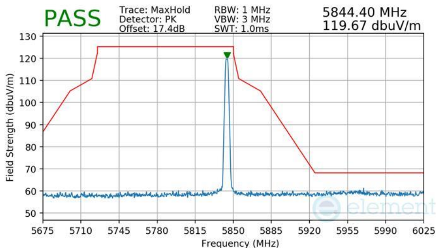
Plot 7-553 Radiated Higher Band Edge Measurement Antenna WF8
