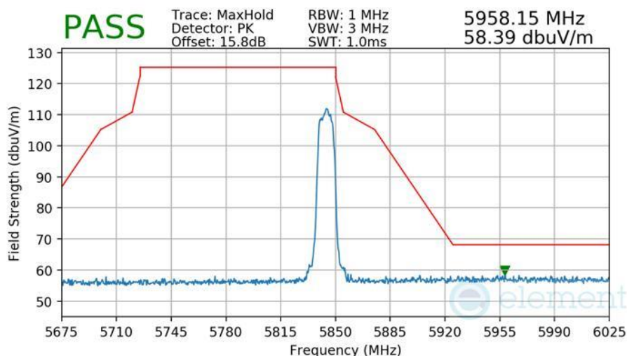
Plot 7-560 Radiated Higher Band Edge Measurement Antenna WF8
