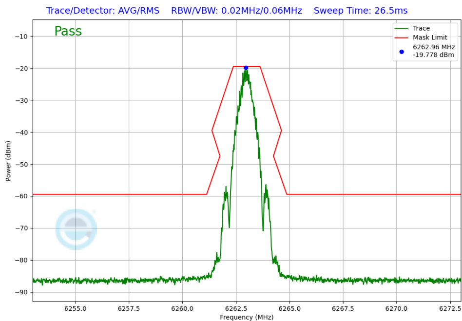
Plot 7-223. In-Band Emissions Antenna WF5B (NB UNII BDR, iPA – 6263MHz)
