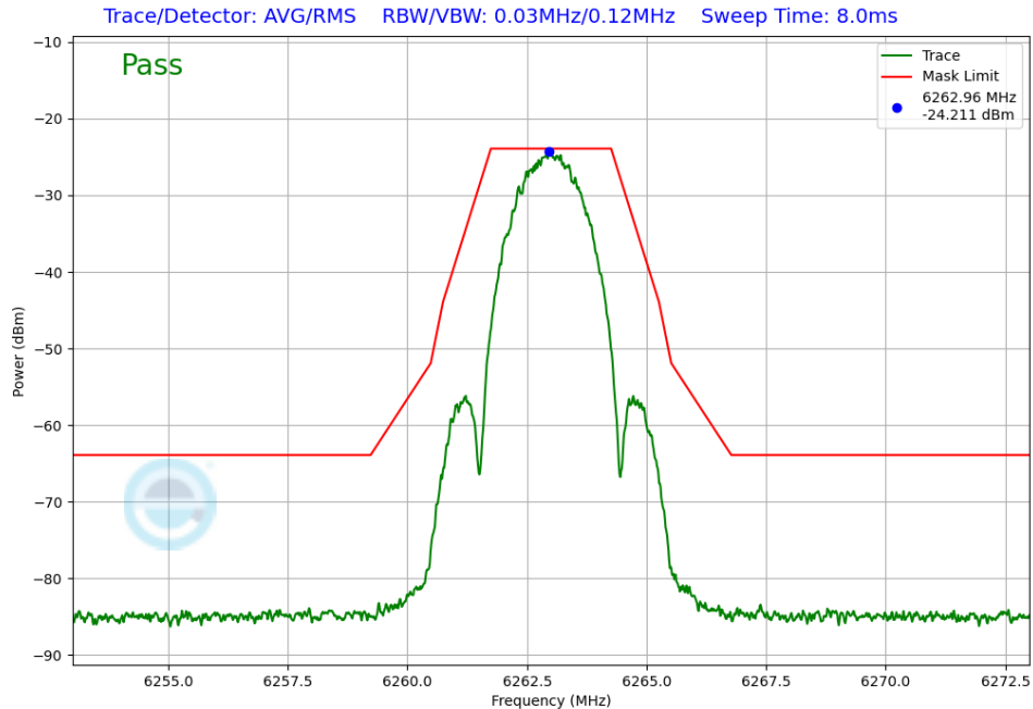
Plot 7-253. In-Band Emissions Antenna WF8 (NB UNII LE2M, iPA – 6263MHz)
