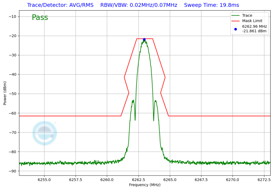
Plot 7-225. In-Band Emissions Antenna WF5B (NB UNII LE1M, iPA – 6263MHz)
