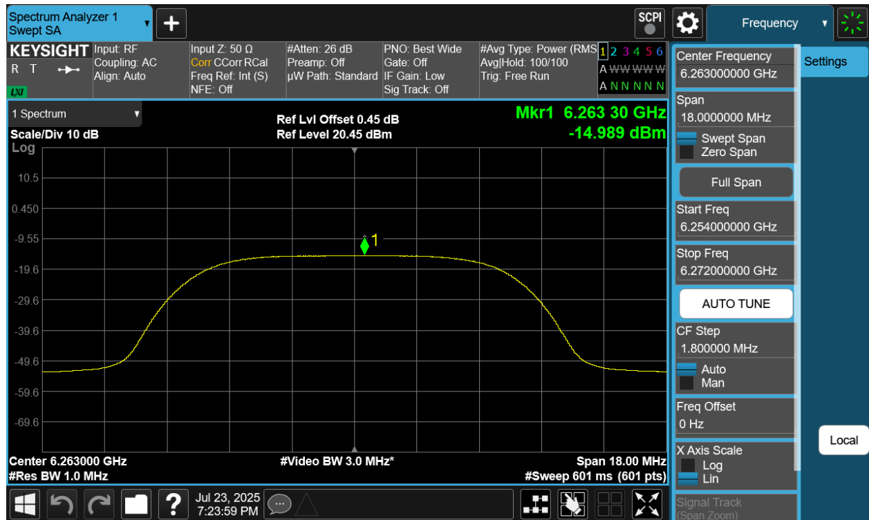
Plot 7-202. PSD Tx BF Diversity Antenna WF8 (NB UNII HDRPL12, ePA - 6263MHz)
