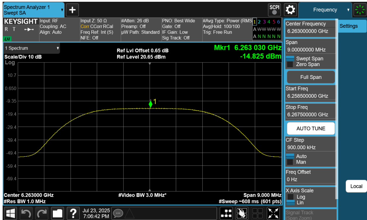
Plot 7-194. PSD Tx BF Diversity Antenna WF8 (NB UNII XHDRPM6, ePA – 6263MHz)
