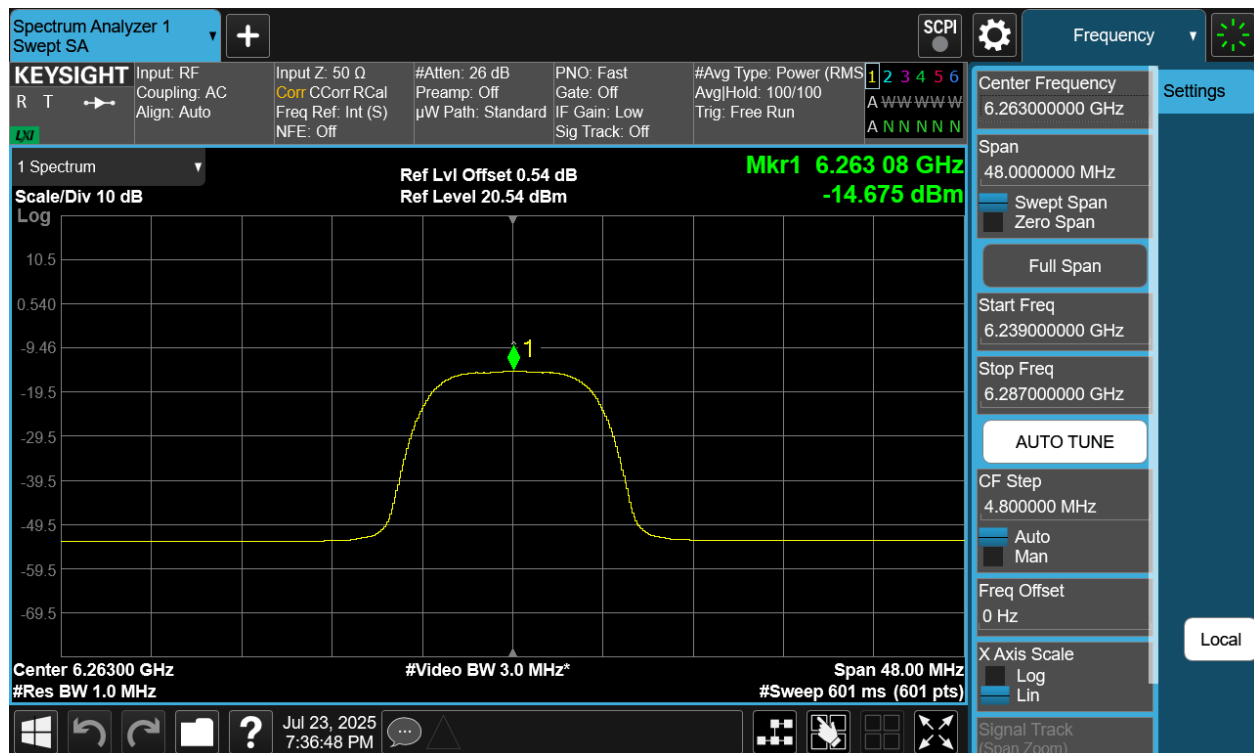
Plot 7-208. PSD TxBF Diversity Antenna WF8 (NB UNII HDRPL32, iPA – 6263MHz)
