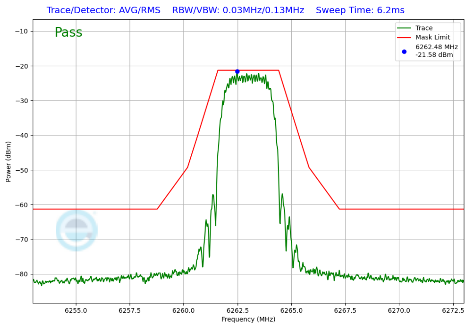
Plot 7-244. In-Band Emissions Antenna WF5B (NB UNII HDT4, ePA – 6263MHz)
