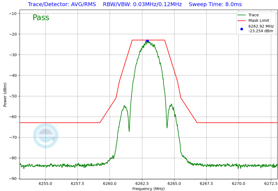
Plot 7-227. In-Band Emissions Antenna WF5B (NB UNII LE2M, iPA – 6263MHz)
