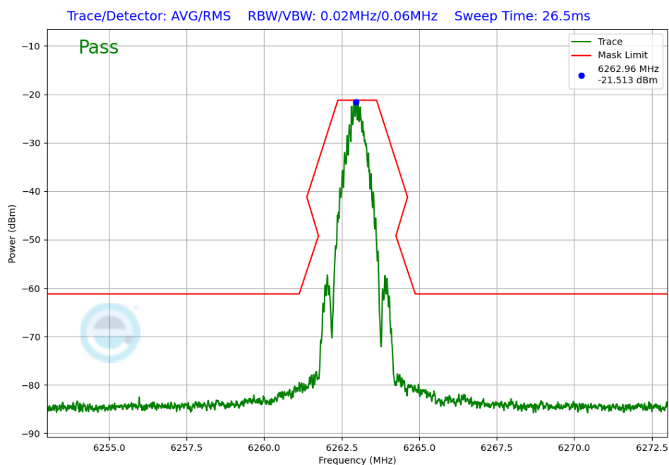
Plot 7-222. In-Band Emissions Antenna WF5B (NB UNII BDR, ePA – 6263MHz)
