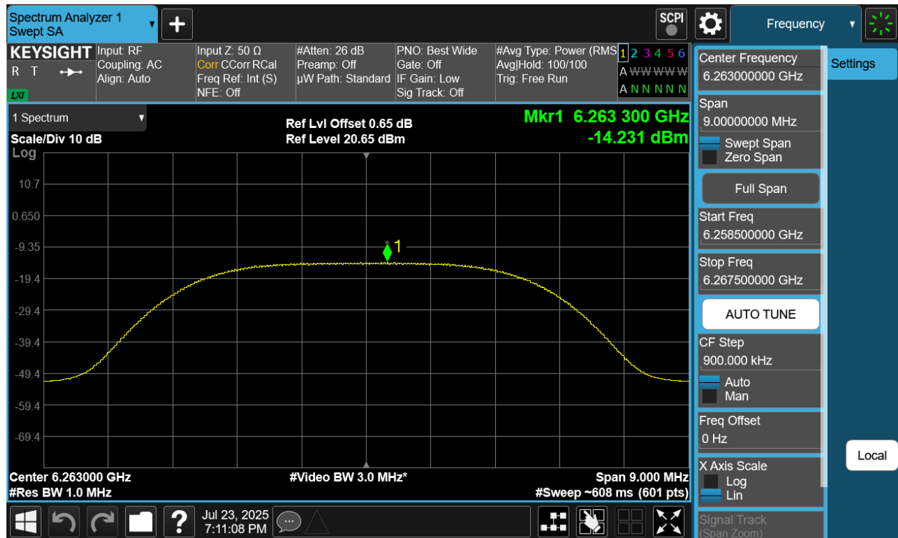
Plot 7-196. PSD TxBF Diversity Antenna WF8 (NB UNII XHDRPM6, iPA – 6263MHz)
