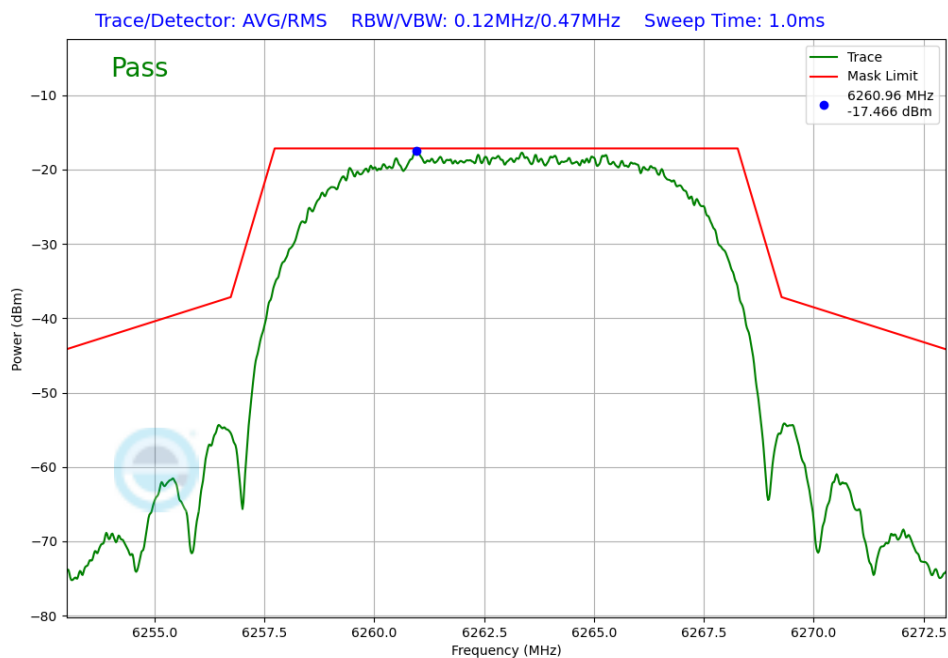
Plot 7-240. In-Band Emissions Antenna WF5B (NB UNII HDRPL32, ePA – 6263MHz)
