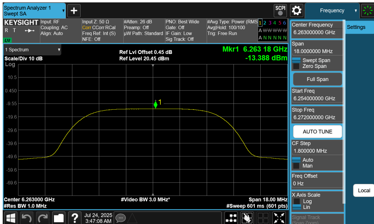
Plot 7-205. PSD TxBF Diversity Antenna WF7 (NB UNII HDRPL12, iPA – 6263MHz)
