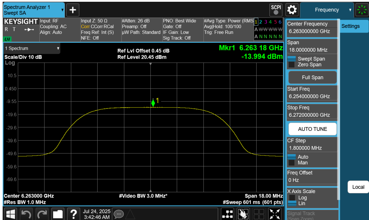
Plot 7-203. PSD Tx BF Diversity Antenna WF7 (NB UNII HDRPL12, ePA - 6263MHz)
