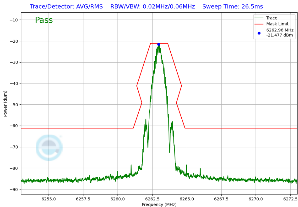
Plot 7-248. In-Band Emissions Antenna WF8 (NB UNII BDR, ePA – 6263MHz)
