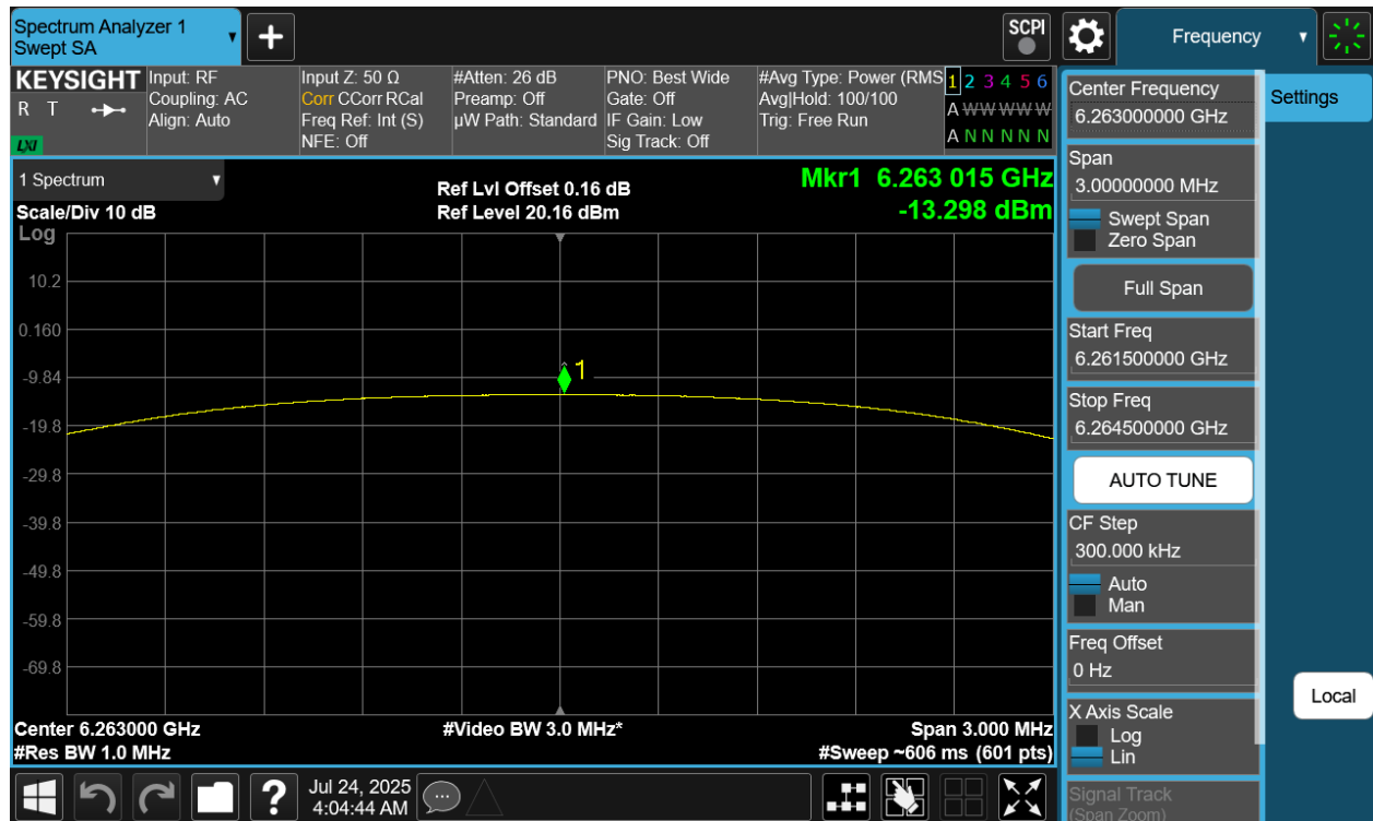
Plot 7-213. PSD Tx BF Diversity Antenna WF7 (NB UNII HDT2, iPA - 6263MHz)
