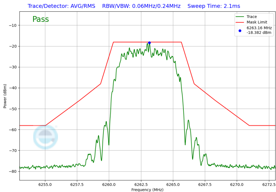
Plot 7-230. In-Band Emissions Antenna WF5B (NB UNII HDR8, ePA – 6263MHz)
