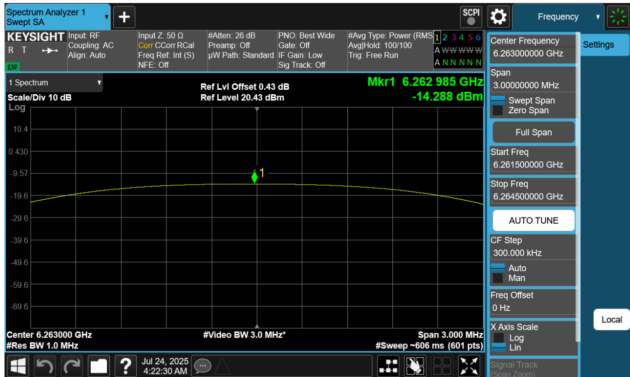
Plot 7-221. PSD TxBF Diversity Antenna WF7 (NB UNII HDT6, iPA – 6263MHz)
