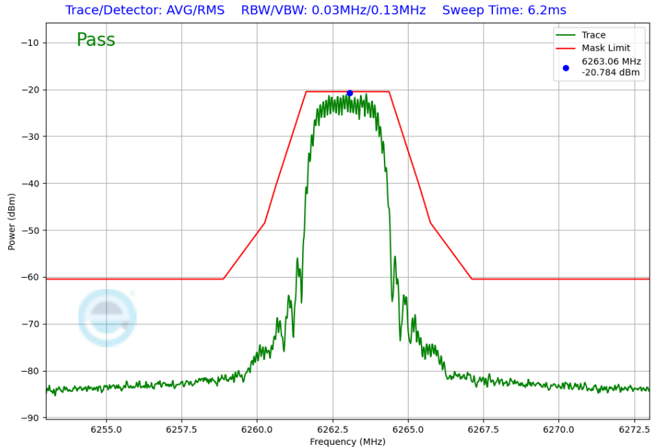
Plot 7-243. In-Band Emissions Antenna WF5B (NB UNII HDT2, iPA – 6263MHz)
