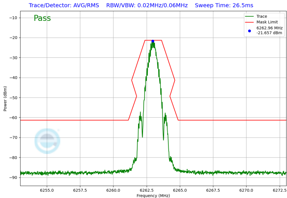
Plot 7-249. In-Band Emissions Antenna WF8 (NB UNII BDR, iPA – 6263MHz)
