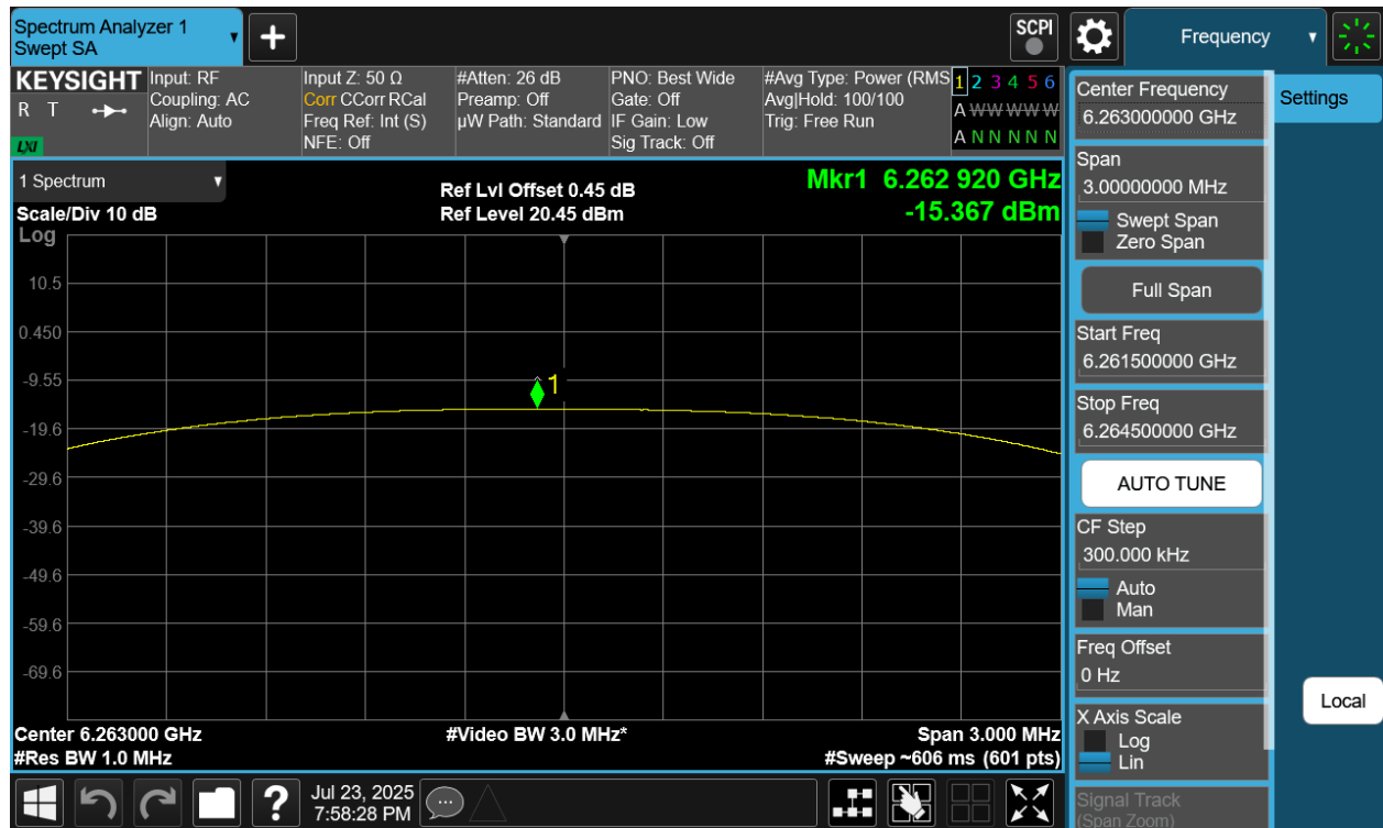
Plot 7-218. PSD Tx BF Diversity Antenna WF8 (NB UNII HDT6, ePA – 6263MHz)
