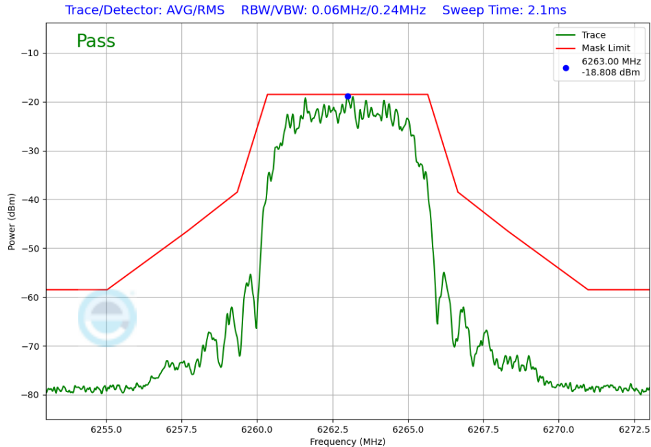
Plot 7-231. In-Band Emissions Antenna WF5B (NB UNII HDR8, iPA – 6263MHz)
