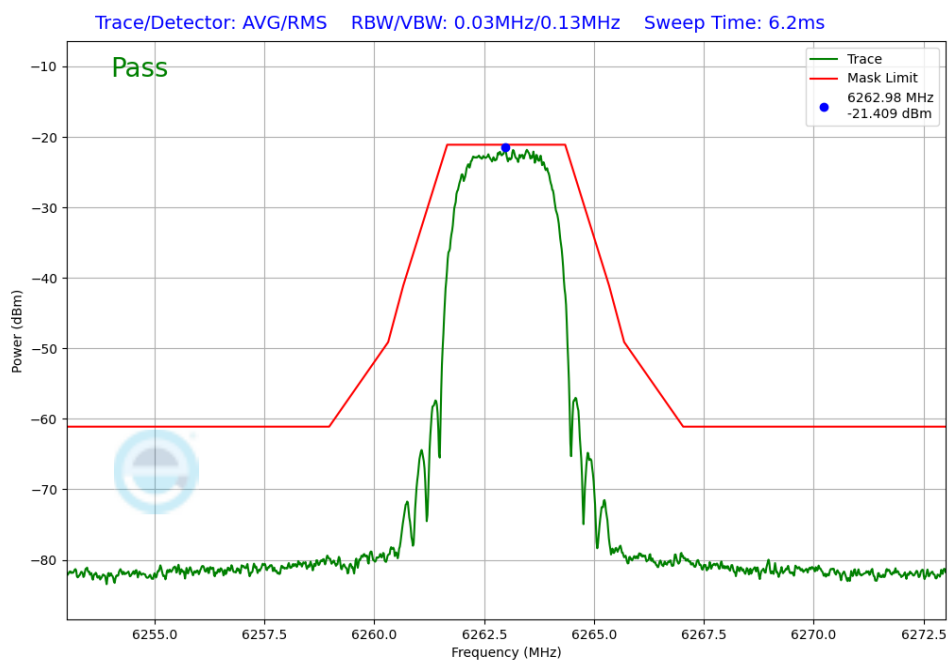
Plot 7-232. In-Band Emissions Antenna WF5B (NB UNII HDRPS2, ePA – 6263MHz)
