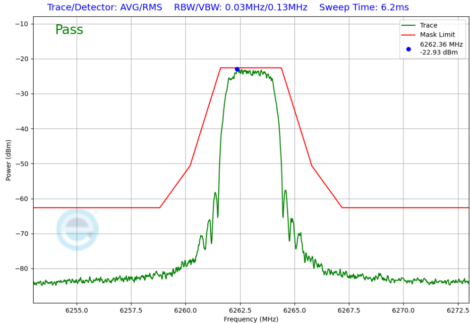
Plot 7-247. In-Band Emissions Antenna WF5B (NB UNII HDT6, iPA – 6263MHz)
