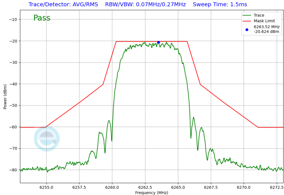
Plot 7-235. In-Band Emissions Antenna WF5B (NB UNII XHDRPM6, iPA – 6263MHz)
