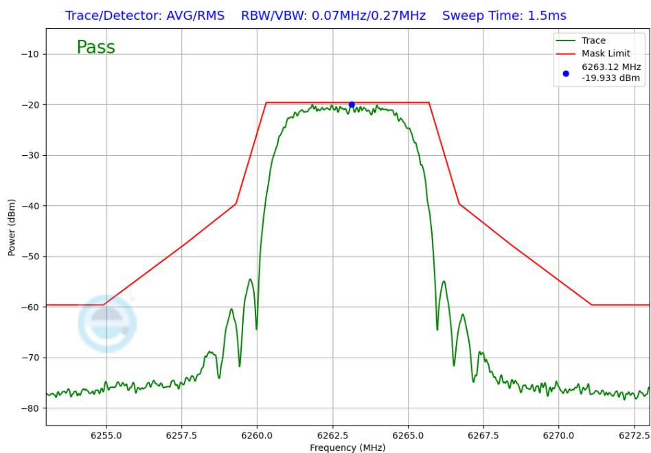
Plot 7-234. In-Band Emissions Antenna WF5B (NB UNII XHDRPM6, ePA – 6263MHz)
