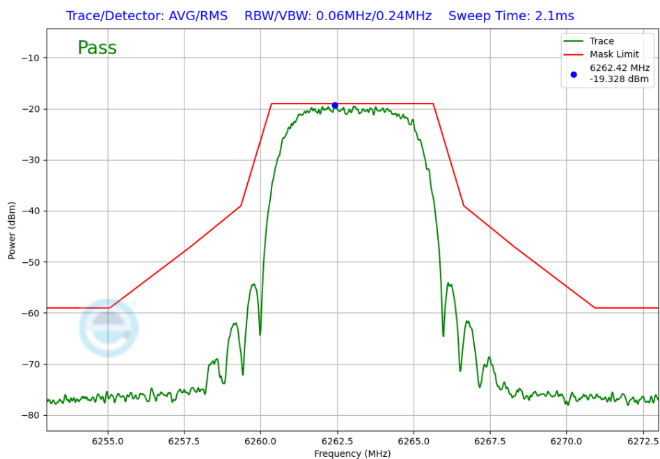
Plot 7-236. In-Band Emissions Antenna WF5B (NB UNII HDRPM16, ePA – 6263MHz)
