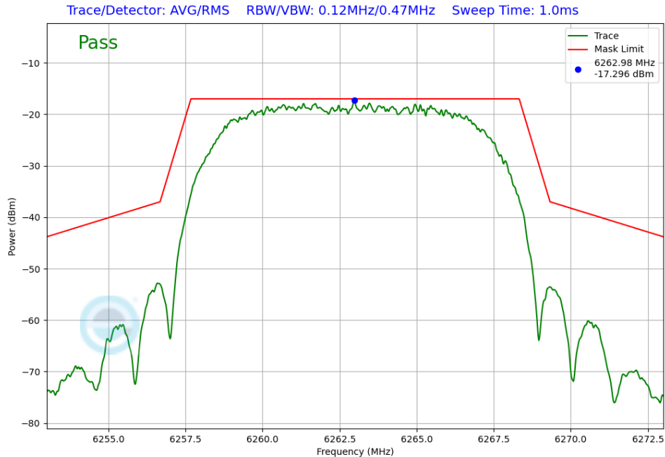
Plot 7-239. In-Band Emissions Antenna WF5B (NB UNII HDRPL12, iPA – 6263MHz)
