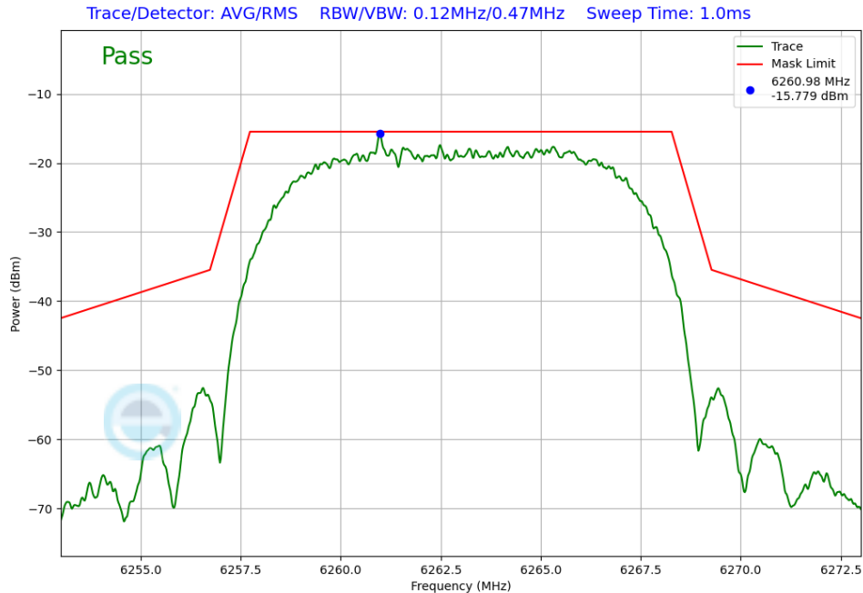
Plot 7-241. In-Band Emissions Antenna WF5B (NB UNII HDRPL32, iPA – 6263MHz)
