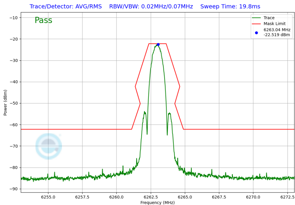
Plot 7-250. In-Band Emissions Antenna WF8 (NB UNII LE1M, ePA – 6263MHz)
