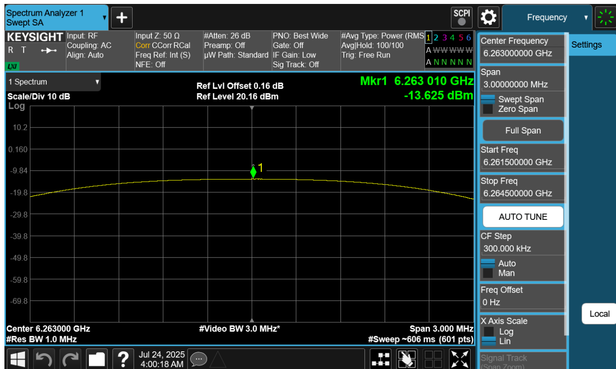
Plot 7-211. PSD Tx BF Diversity Antenna WF7 (NB UNII HDT2, ePA – 6263MHz)
