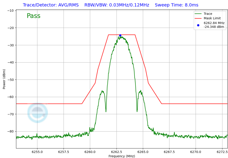
Plot 7-252. In-Band Emissions Antenna WF8 (NB UNII LE2M, ePA – 6263MHz)
