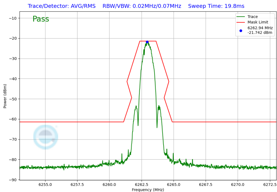
Plot 7-224. In-Band Emissions Antenna WF5B (NB UNII LE1M, ePA – 6263MHz)
