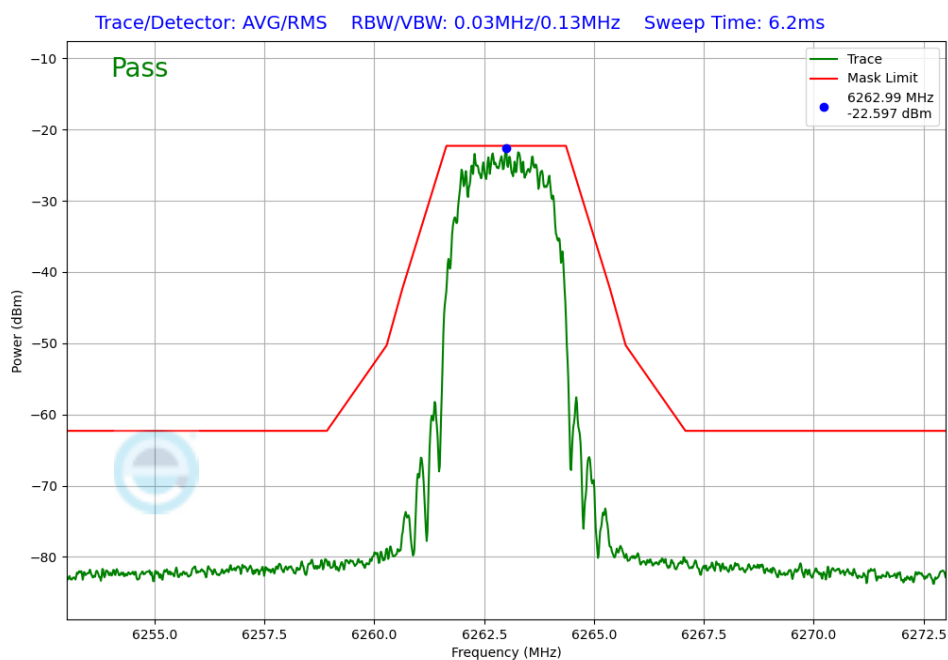
Plot 7-254. In-Band Emissions Antenna WF8 (NB UNII HDR4, ePA – 6263MHz)
