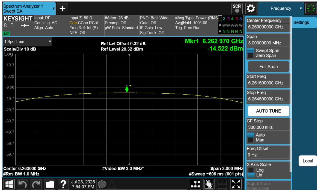
Plot 7-216. PSD Tx BF Diversity Antenna WF8 (NB UNII HDT4, iPA - 6263MHz)
