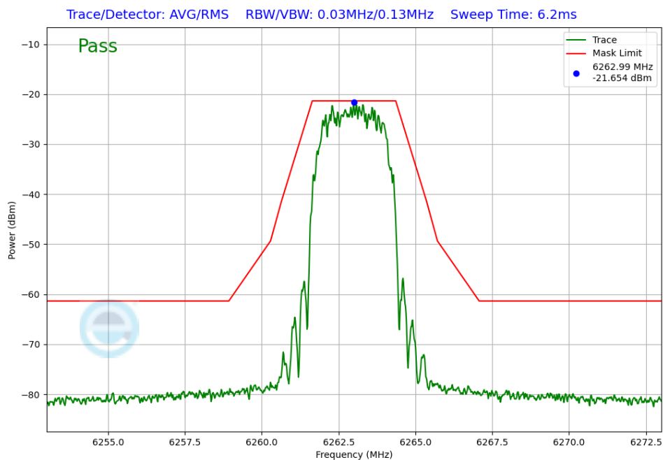
Plot 7-228. In-Band Emissions Antenna WF5B (NB UNII HDR4, ePA – 6263MHz)
