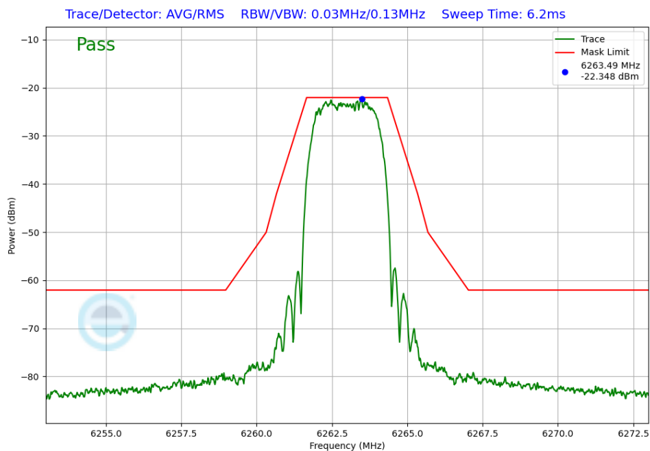
Plot 7-233. In-Band Emissions Antenna WF5B (NB UNII HDRPS2, iPA – 6263MHz)
