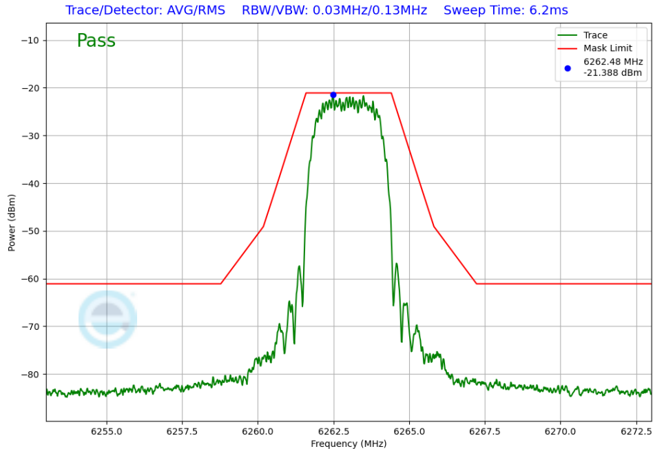
Plot 7-245. In-Band Emissions Antenna WF5B (NB UNII HDT4, iPA – 6263MHz)
