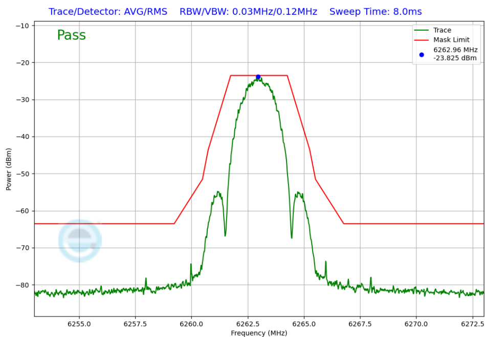
Plot 7-226. In-Band Emissions Antenna WF5B (NB UNII LE2M, ePA – 6263MHz)
