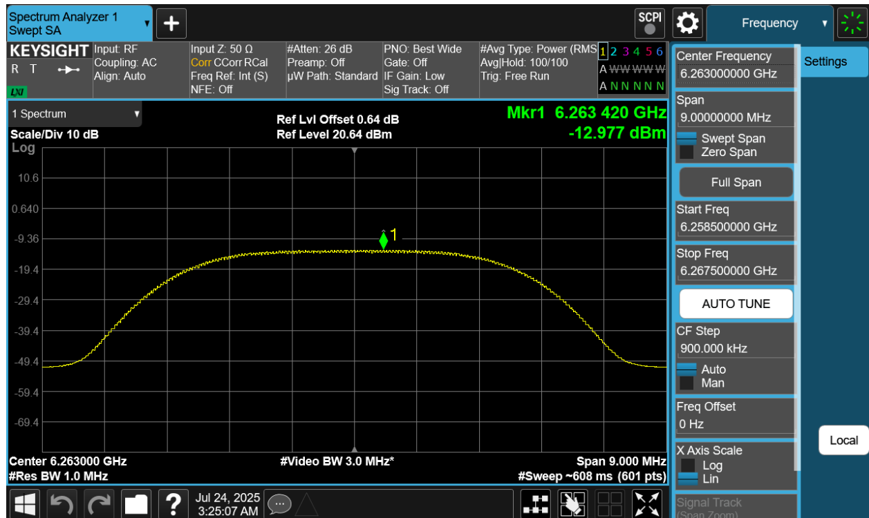
Plot 7-195. PSD Tx BF Diversity Antenna WF7 (NB UNII XHDRPM6, ePA – 6263MHz)
