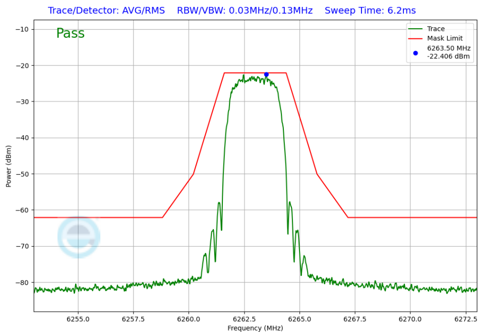
Plot 7-246. In-Band Emissions Antenna WF5B (NB UNII HDT6, ePA – 6263MHz)
