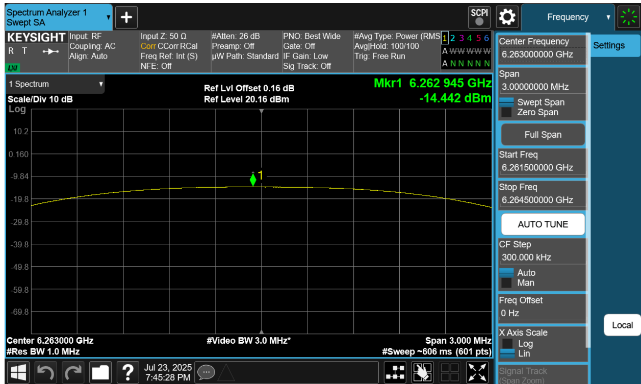
Plot 7-212. PSD Tx BF Diversity Antenna WF8 (NB UNII HDT2, iPA - 6263MHz)
