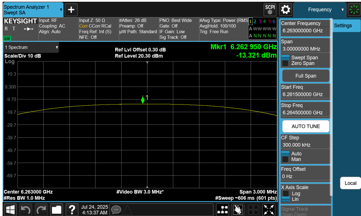
Plot 7-217. PSD Tx BF Diversity Antenna WF7 (NB UNII HDT4, iPA - 6263MHz)
