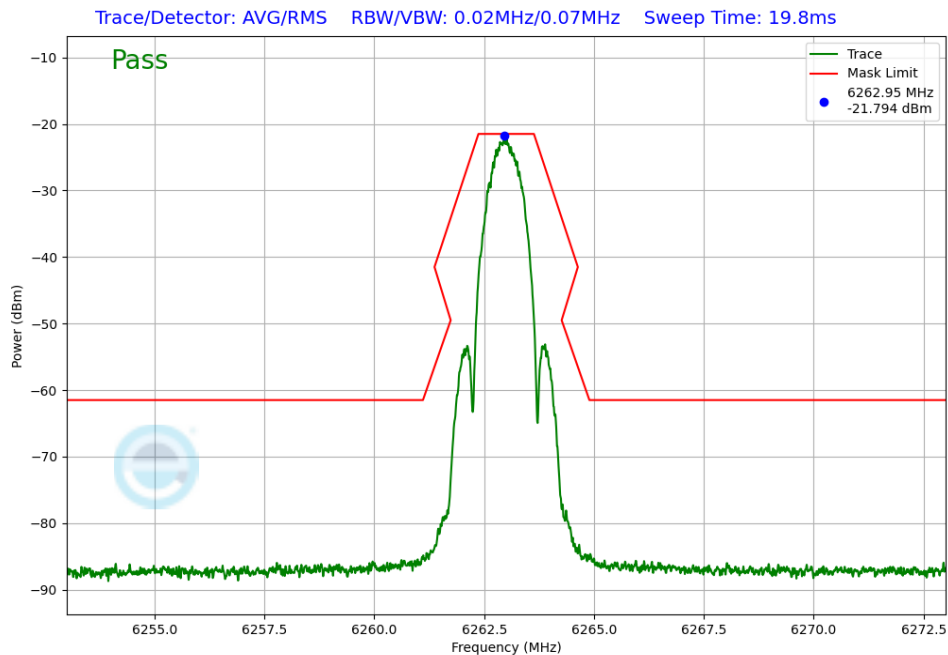
Plot 7-251. In-Band Emissions Antenna WF8 (NB UNII LE1M, iPA – 6263MHz)
