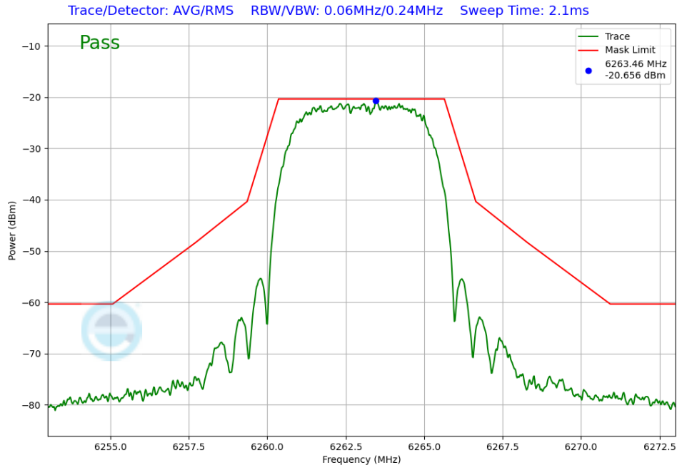
Plot 7-237. In-Band Emissions Antenna WF5B (NB UNII HDRPM16, iPA – 6263MHz)
