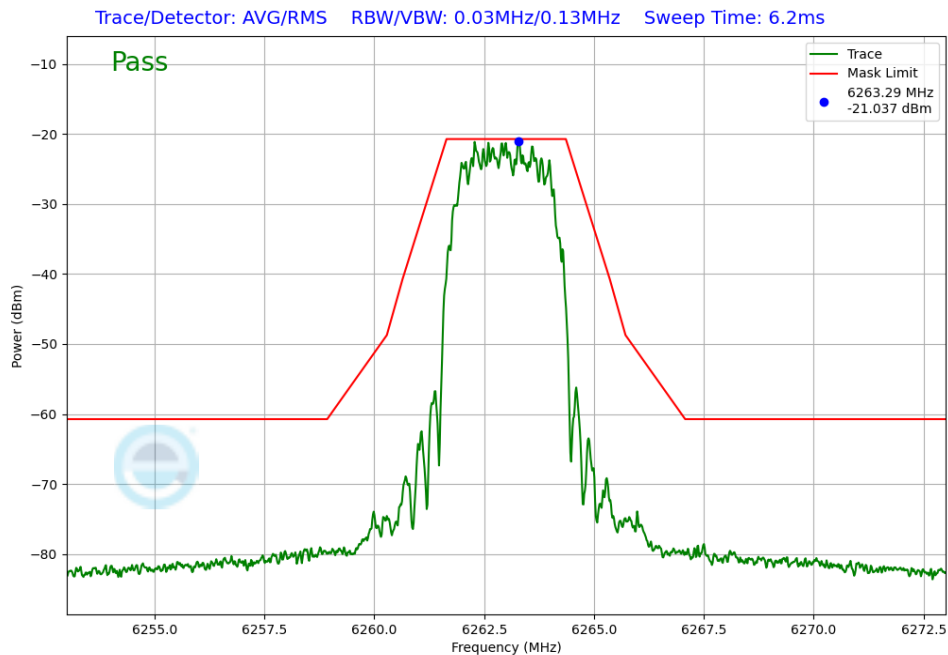
Plot 7-229. In-Band Emissions Antenna WF5B (NB UNII HDR4, iPA – 6263MHz)
