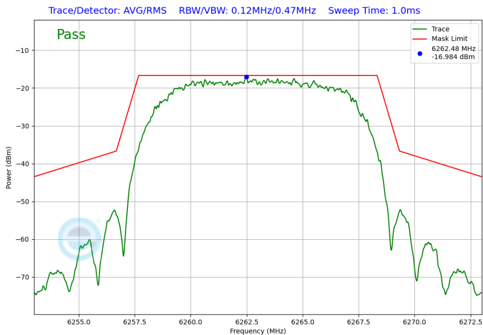
Plot 7-238. In-Band Emissions Antenna WF5B (NB UNII HDRPL12, ePA – 6263MHz)
