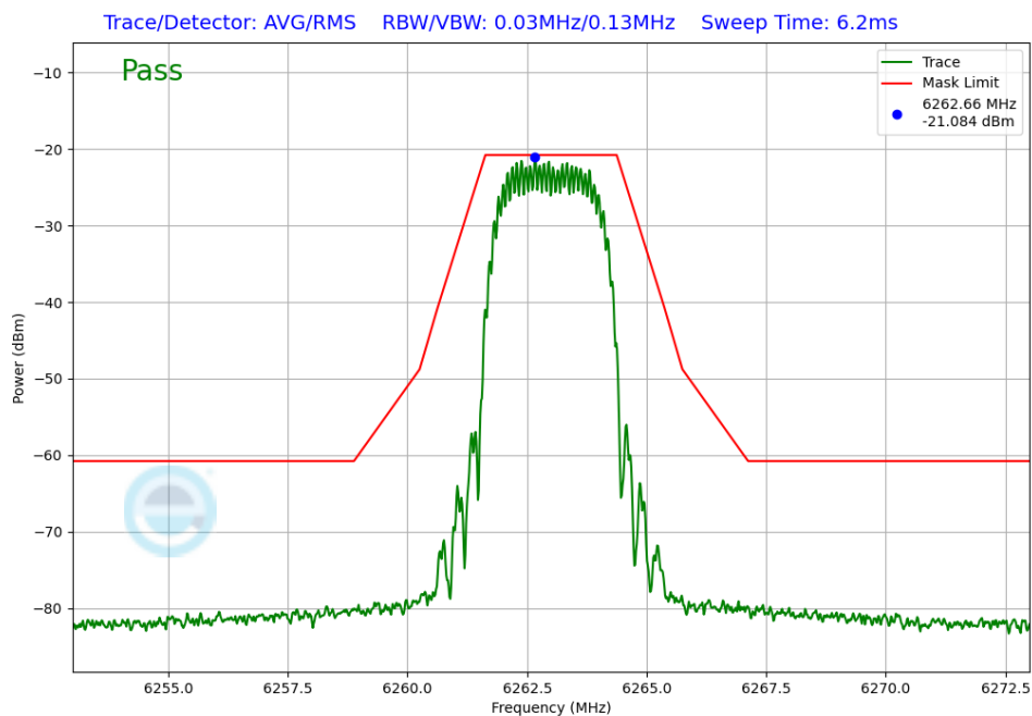
Plot 7-242. In-Band Emissions Antenna WF5B (NB UNII HDT2, ePA – 6263MHz)
