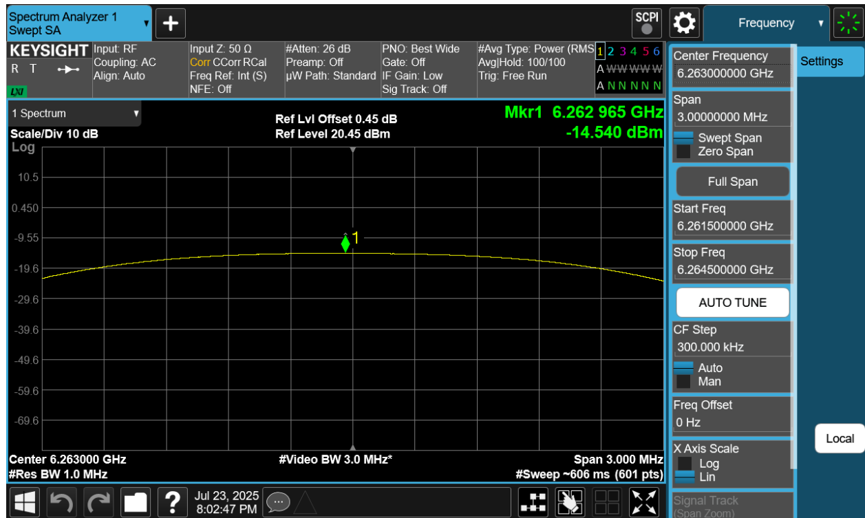
Plot 7-220. PSD TxBF Diversity Antenna WF8 (NB UNII HDT6, iPA – 6263MHz)
