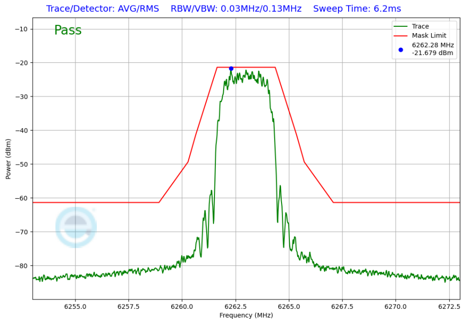
Plot 7-255. In-Band Emissions Antenna WF8 (NB UNII HDR4, iPA – 6263MHz)
