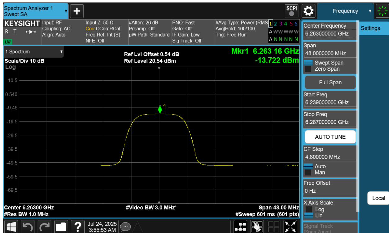
Plot 7-209. PSD TxBF Diversity Antenna WF7 (NB UNII HDRPL32, iPA – 6263MHz)
