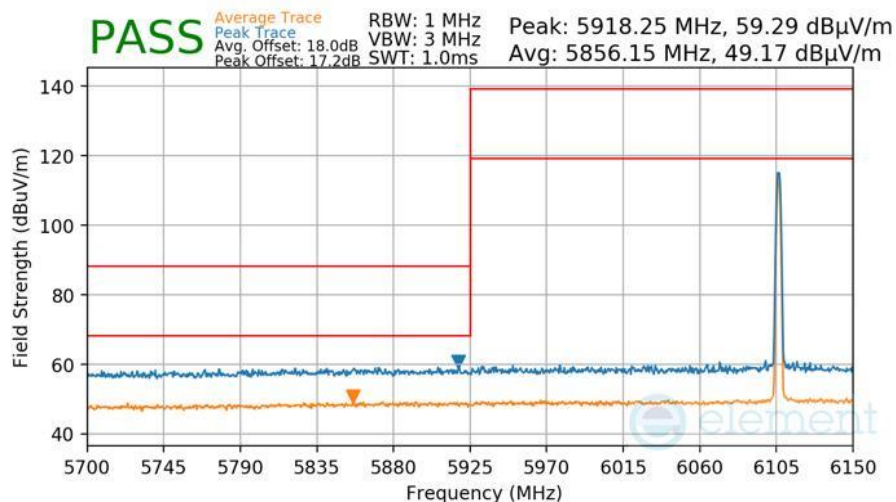
Plot 7-436 Radiated Lower Band Edge Measurement Antenna WF5B
