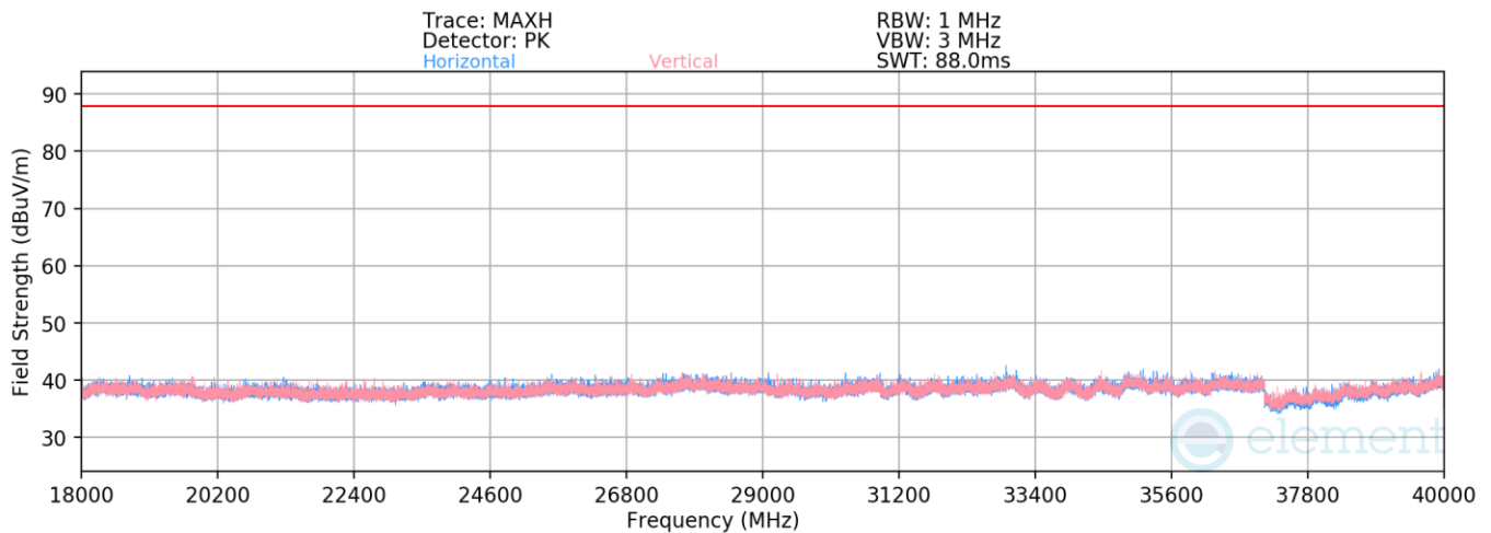
Plot 7-433. Radiated Spurious Emissions Above 18GHz (LE1M ePA – 6263MHz)
