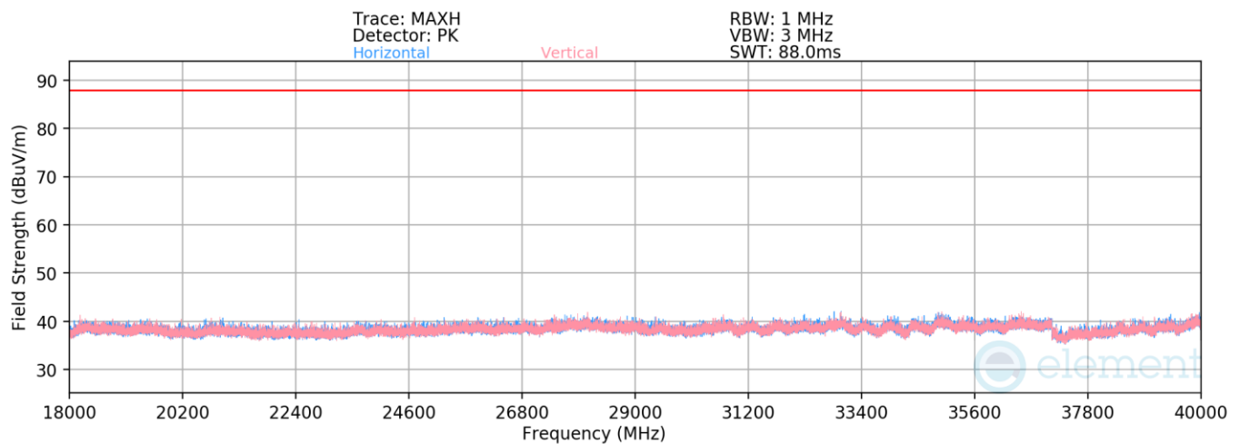
Plot 7-421. Radiated Spurious Emissions Above 18GHz (LE1M ePA – 6263MHz)
