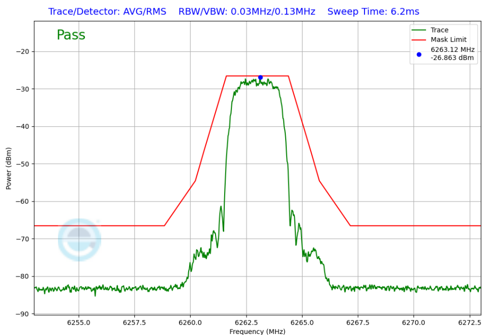
Plot 7-402. In-Band Emissions TxBF Diversity Antenna WF8 (NB UNII HDT6, iPA – 6263MHz)
