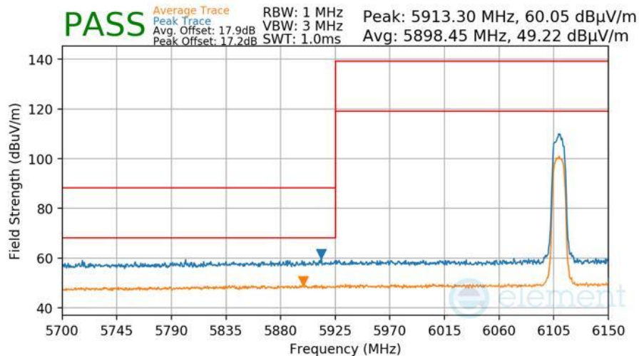
Plot 7-444 Radiated Lower Band Edge Measurement Antenna WF5B
