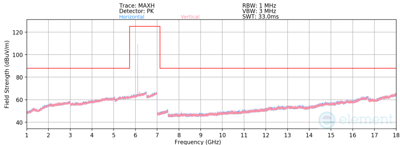
Plot 7-427. Radiated Spurious Emissions 1-18GHz TxBF Diversity (HDR4 ePA – 6108MHz)
