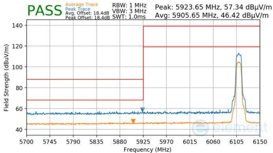
Plot 7-443 Radiated Lower Band Edge Measurement Antenna WF5B
