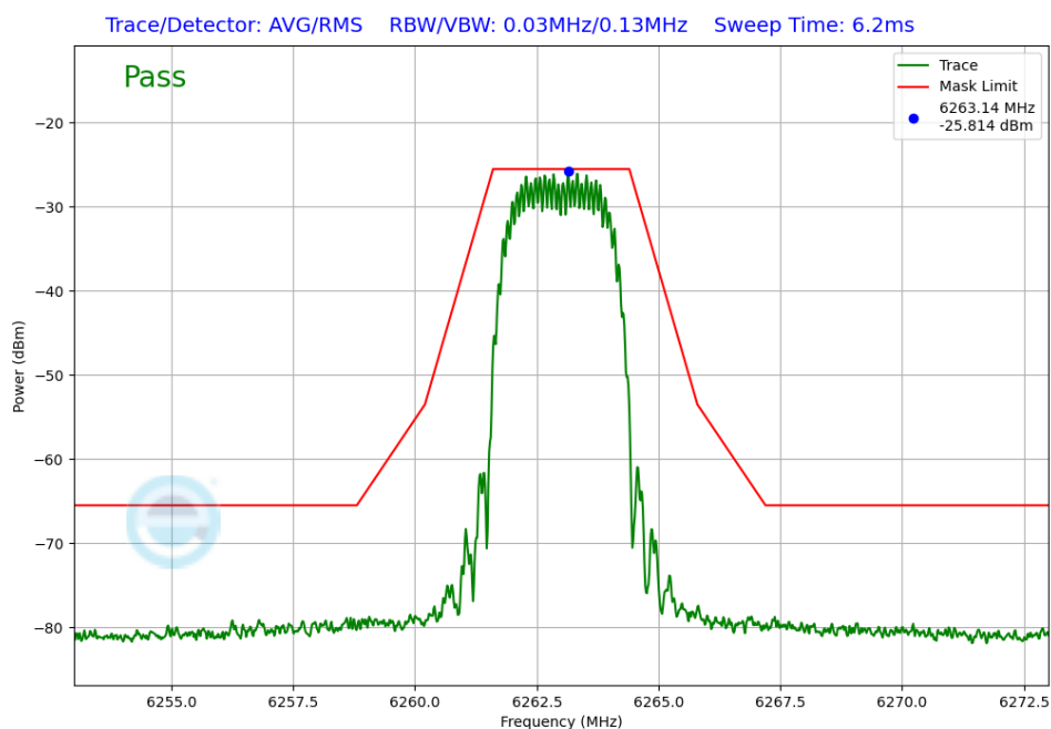
Plot 7-392. In-Band Emissions TxBF Diversity Antenna WF8 (NB UNII HDT2, ePA – 6263MHz)
