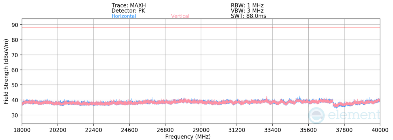
Plot 7-425. Radiated Spurious Emissions Above 18GHz (BDR GFSK ePA – 6263MHz)
