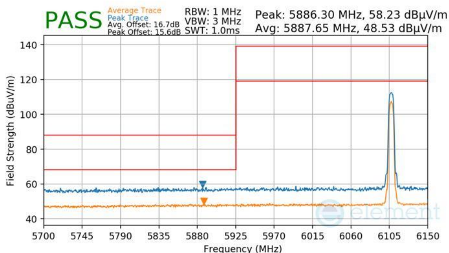
Plot 7-450 Radiated Lower Band Edge Measurement Antenna WF8
