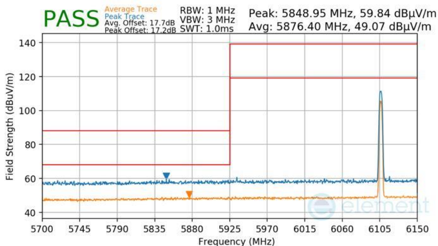
Plot 7-445 Radiated Lower Band Edge Measurement Antenna WF5B
