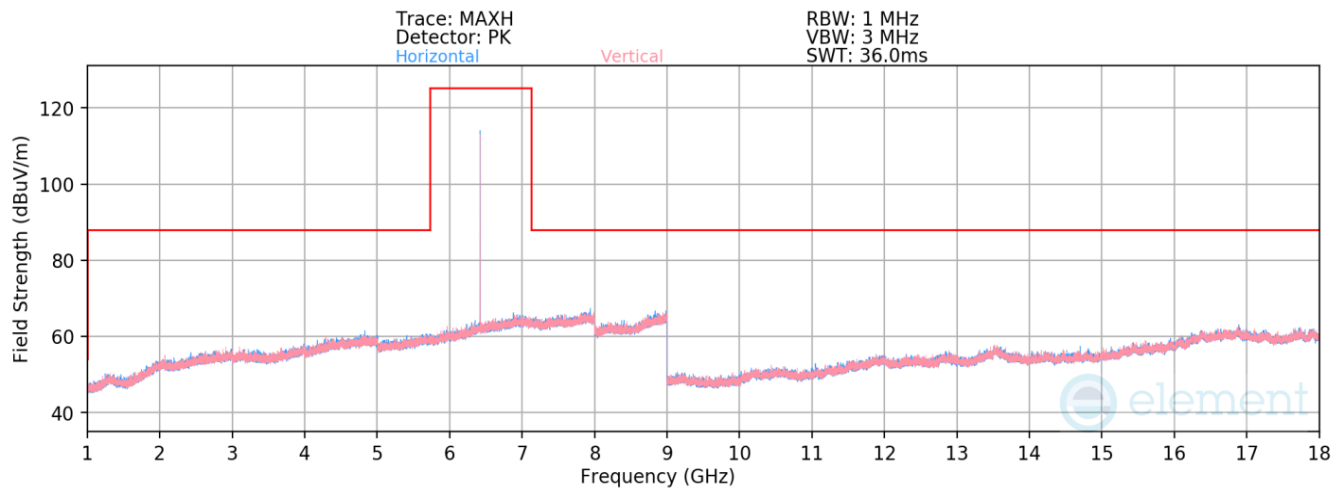
Plot 7-422. Radiated Spurious Emissions 1-18GHz TxBF Primary (LE1M ePA – 6420MHz)
