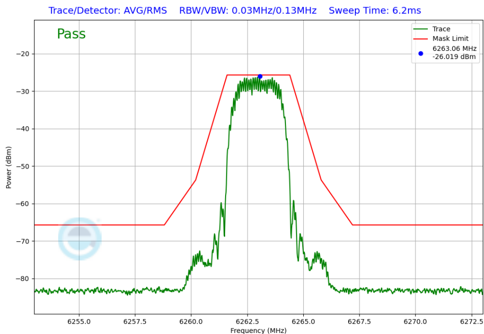
Plot 7-394. In-Band Emissions TxBF Diversity Antenna WF8 (NB UNII HDT2, iPA – 6263MHz)
