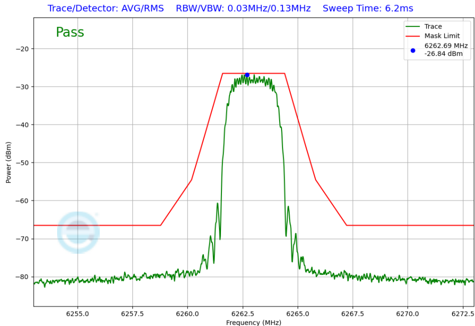
Plot 7-397. In-Band Emissions TxBF Diversity Antenna WF7 (NB UNII HDT4, ePA – 6263MHz)
