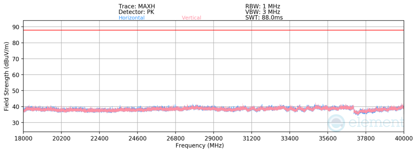
Plot 7-429. Radiated Spurious Emissions Above 18GHz (HDR4 ePA – 6263MHz)
