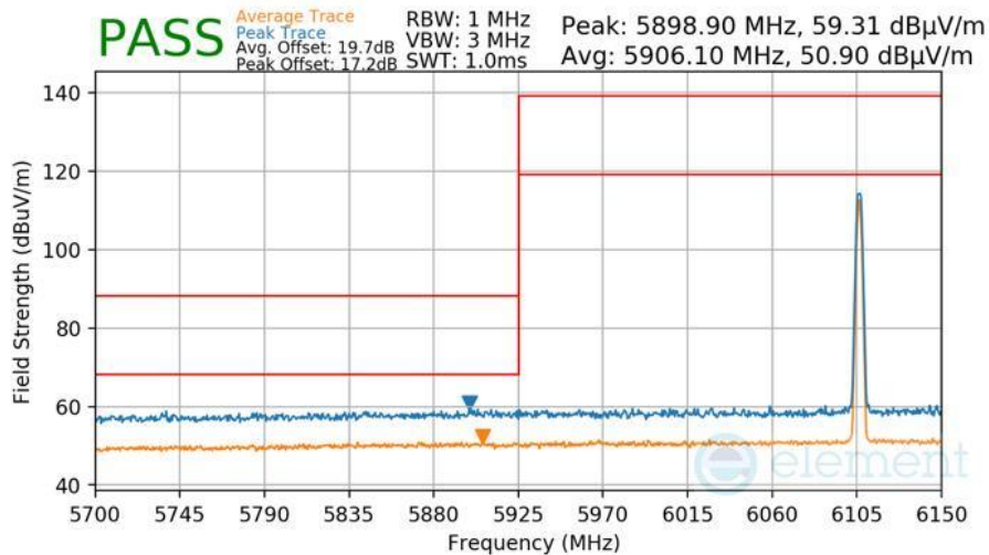
Plot 7-437 Radiated Lower Band Edge Measurement Antenna WF5B
