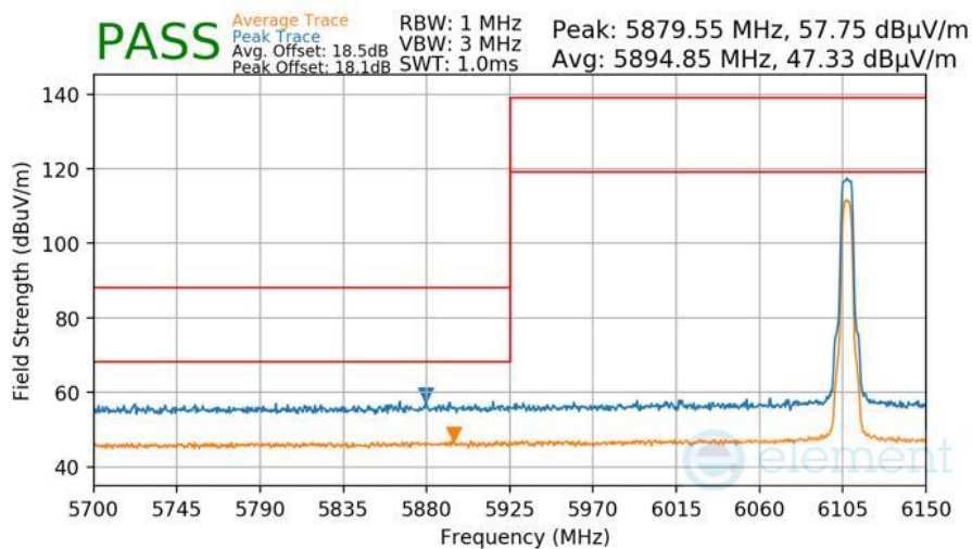
Plot 7-452 Radiated Lower Band Edge Measurement Antenna WF8
