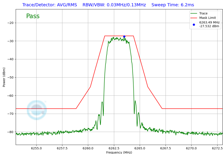
Plot 7-400. In-Band Emissions Tx BF Diversity Antenna WF8 (NB UNII HDT6, ePA – 6263MHz)
