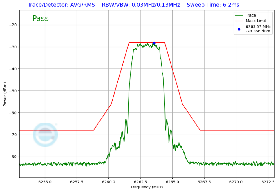
Plot 7-403. In-Band Emissions TxBF Diversity Antenna WF7 (NB UNII HDT6, iPA – 6263MHz)
