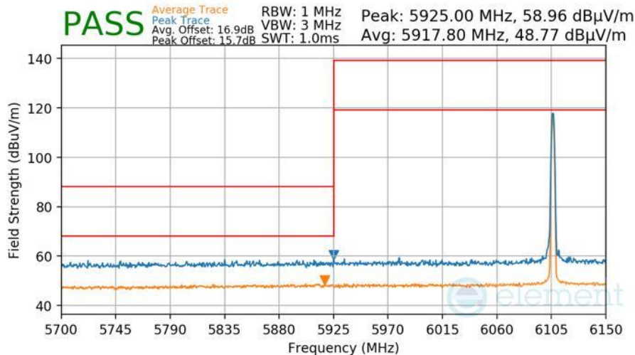
Plot 7-446 Radiated Lower Band Edge Measurement Antenna WF8
