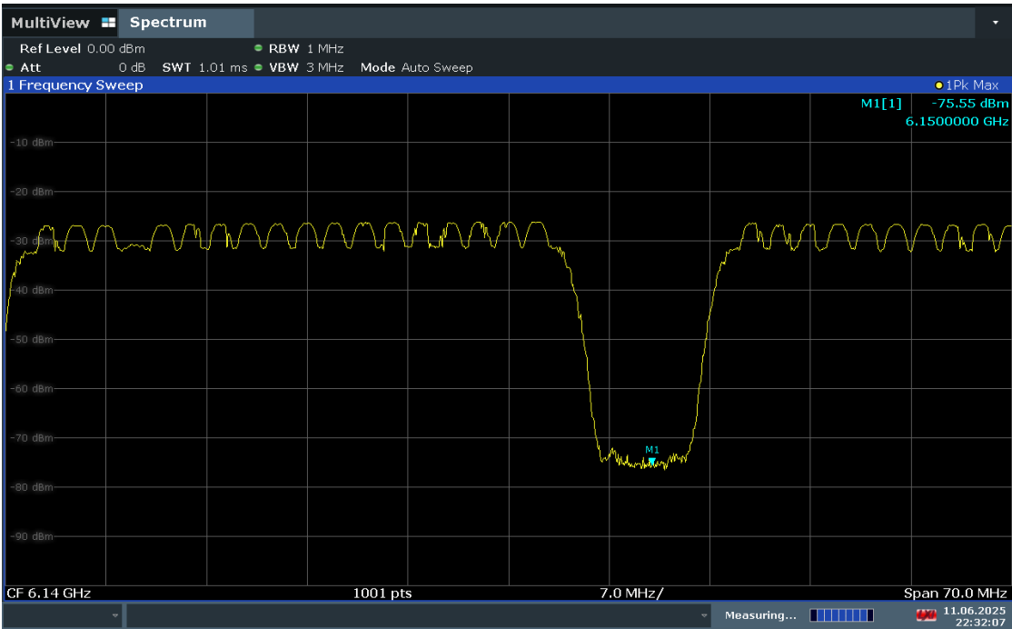
Plot 7-407. After AWGN Signal Injected
