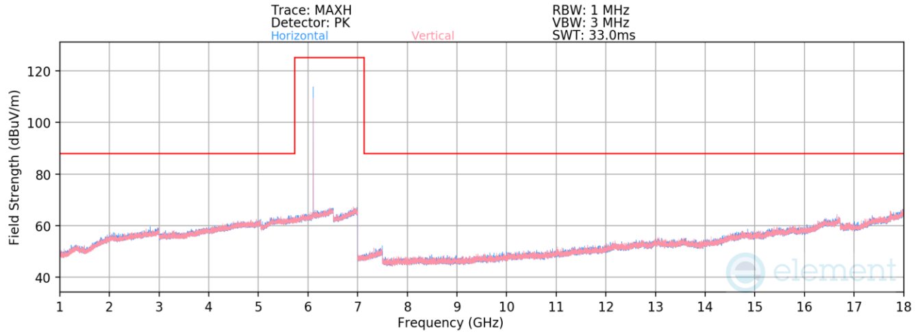
Plot 7-415. Radiated Spurious Emissions 1-18GHz TxBF Primary (HDR4 ePA – 6108MHz)
