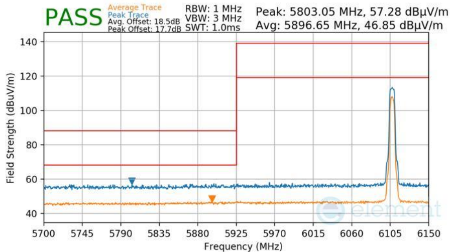
Plot 7-441 Radiated Lower Band Edge Measurement Antenna WF5B
