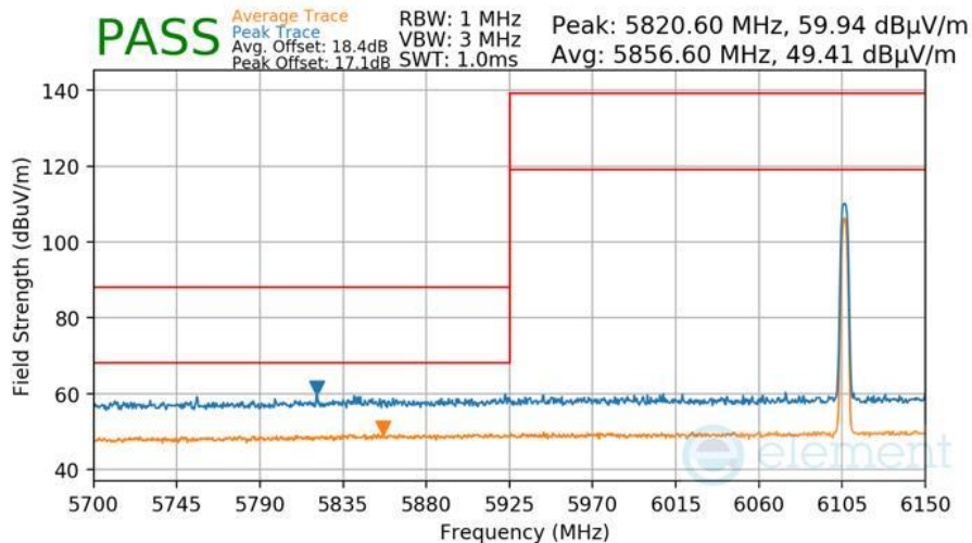
Plot 7-438 Radiated Lower Band Edge Measurement Antenna WF5B
