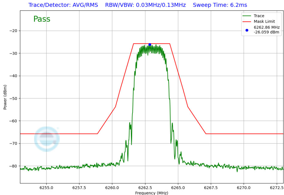
Plot 7-393. In-Band Emissions TxBF Diversity Antenna WF7 (NB UNII HDT2, ePA – 6263MHz)
