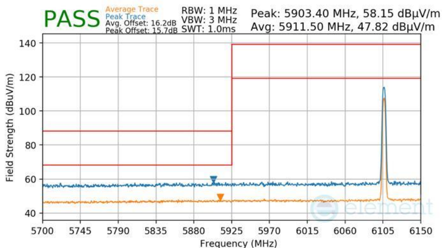
Plot 7-456 Radiated Lower Band Edge Measurement Antenna WF8
