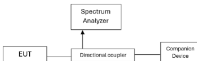
Figure 7-6. Test Instrument & Measurement Setup (No Attenuation)
