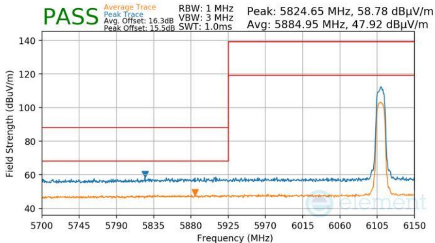
Plot 7-455 Radiated Lower Band Edge Measurement Antenna WF8
