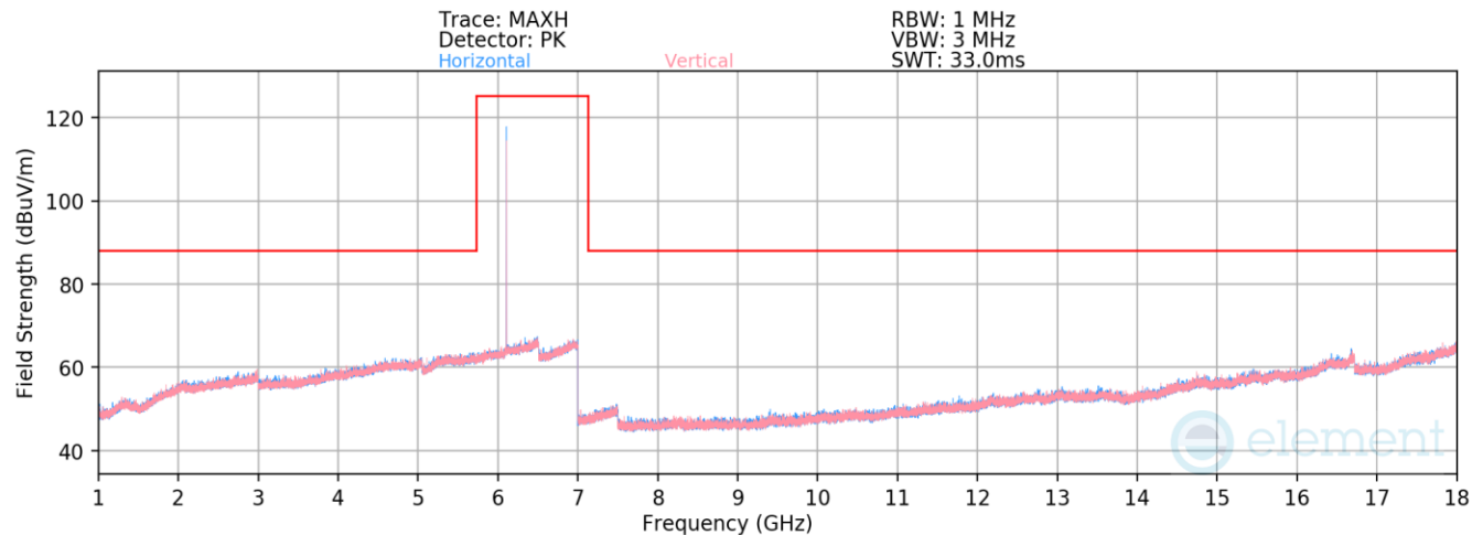
Plot 7-411. Radiated Spurious Emissions 1-18GHz TxBF Primary (BDR GFSK ePA – 6108MHz)
