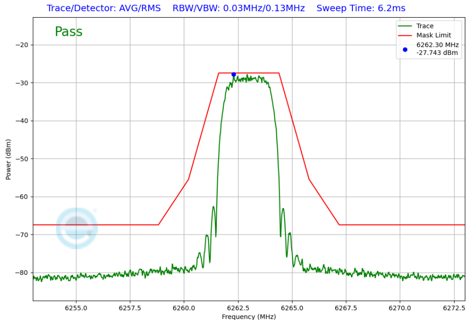
Plot 7-401. In-Band Emissions Tx BF Diversity Antenna WF7 (NB UNII HDT6, ePA – 6263MHz)
