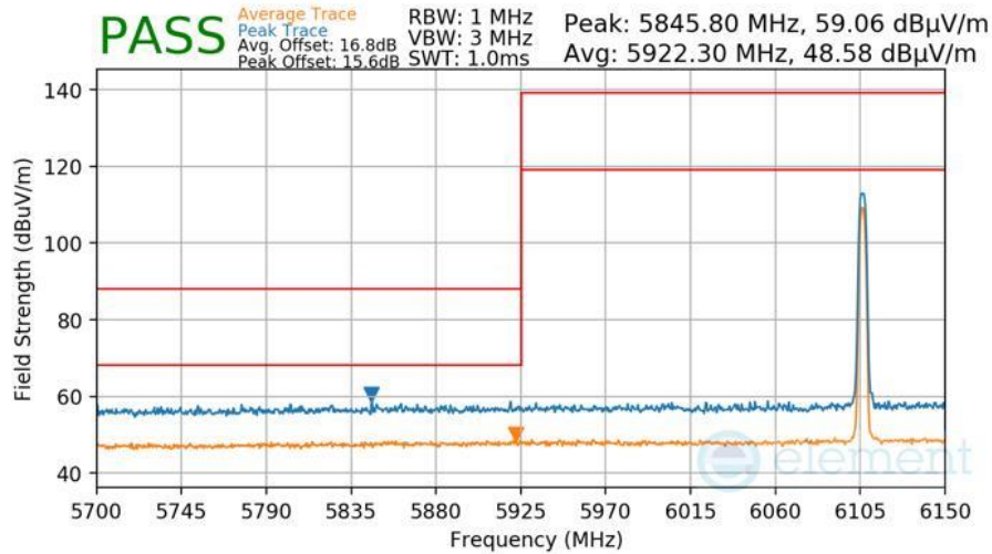
Plot 7-449 Radiated Lower Band Edge Measurement Antenna WF8
