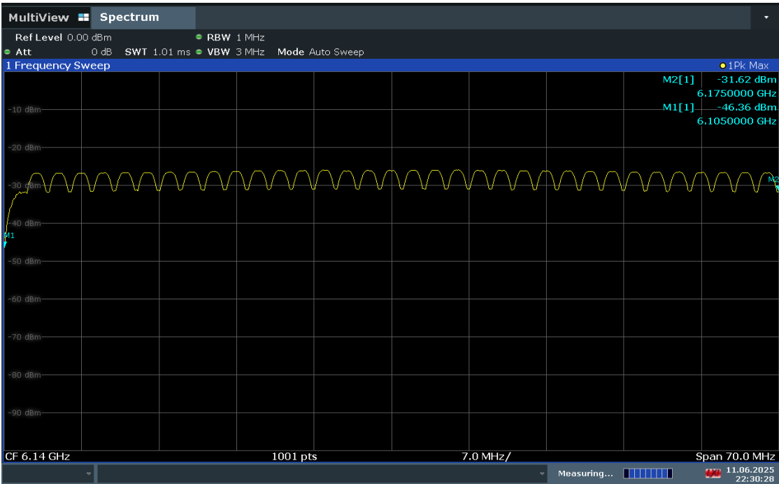
Plot 7-406. Before AWGN Signal Injected
