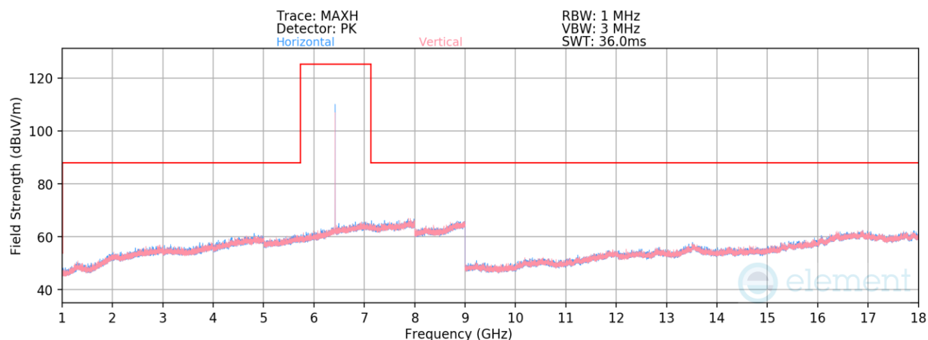
Plot 7-418. Radiated Spurious Emissions 1-18GHz TxBF Primary (HDR4 ePA – 6420MHz)
