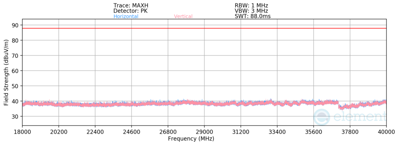
Plot 7-413. Radiated Spurious Emissions Above 18GHz (BDR GFSK ePA – 6263MHz)
