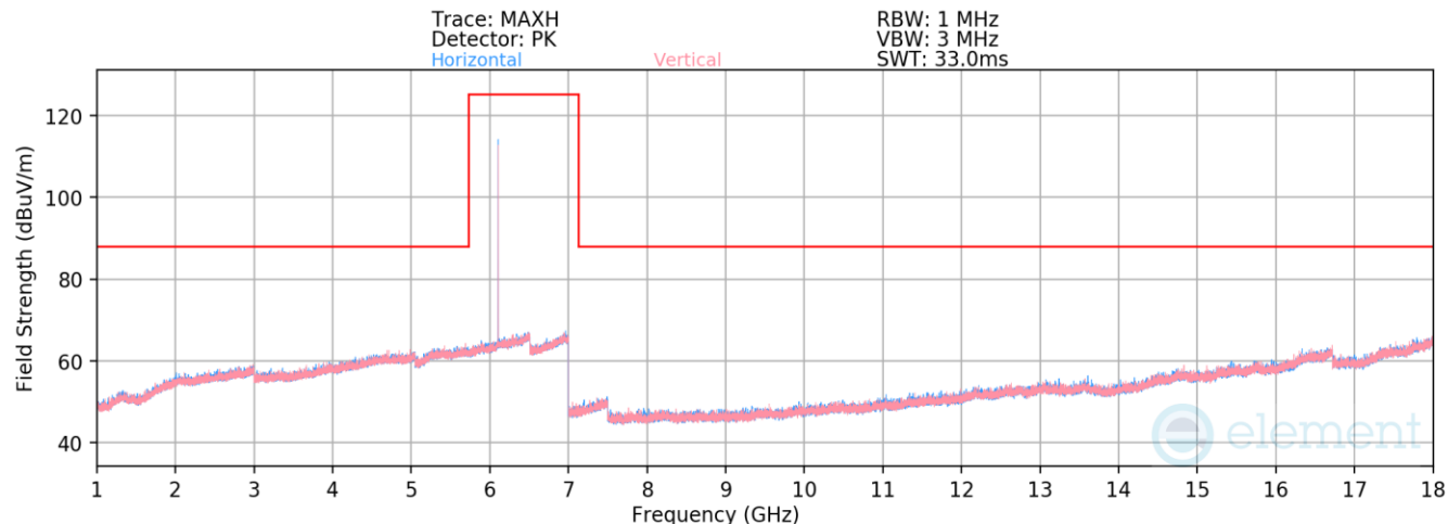
Plot 7-423. Radiated Spurious Emissions 1-18GHz TxBF Diversity (BDR GFSK ePA – 6108MHz)
