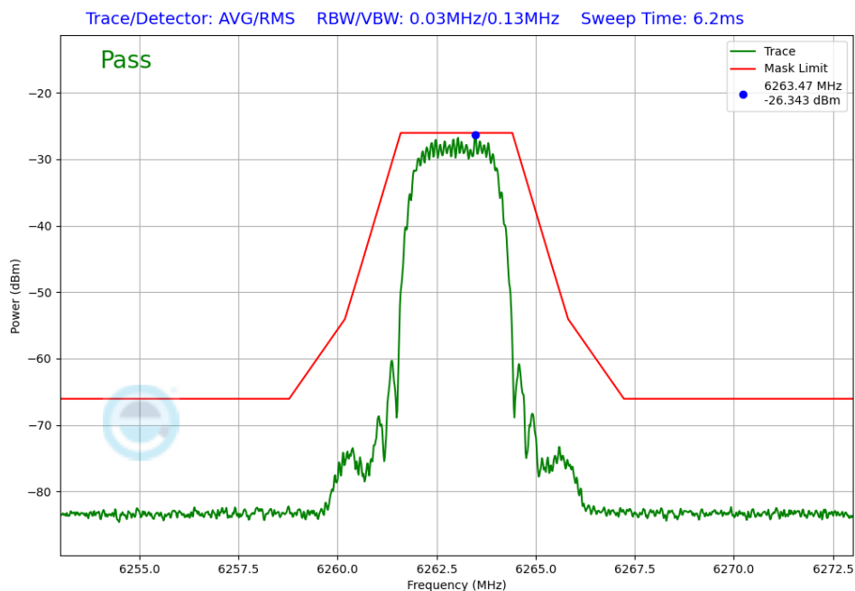
Plot 7-398. In-Band Emissions TxBF Diversity Antenna WF8 (NB UNII HDT4, iPA – 6263MHz)
