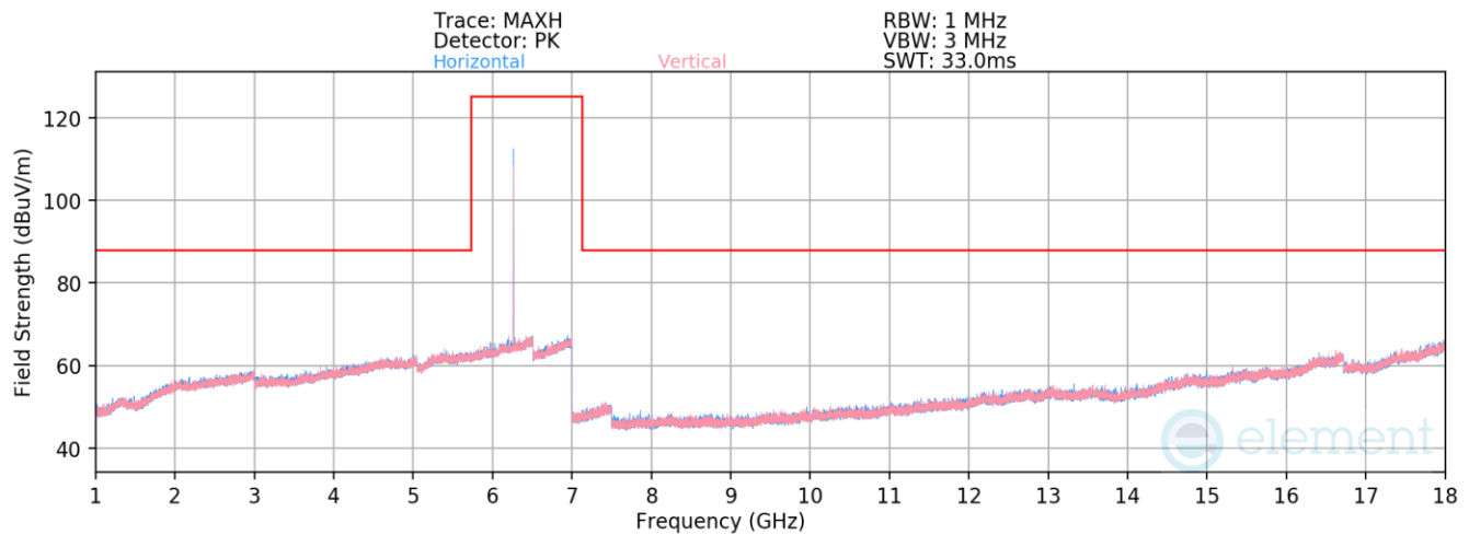
Plot 7-416. Radiated Spurious Emissions 1-18GHz TxBF Primary (HDR4 ePA – 6263MHz)
