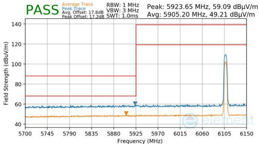
Plot 7-442 Radiated Lower Band Edge Measurement Antenna WF5B
