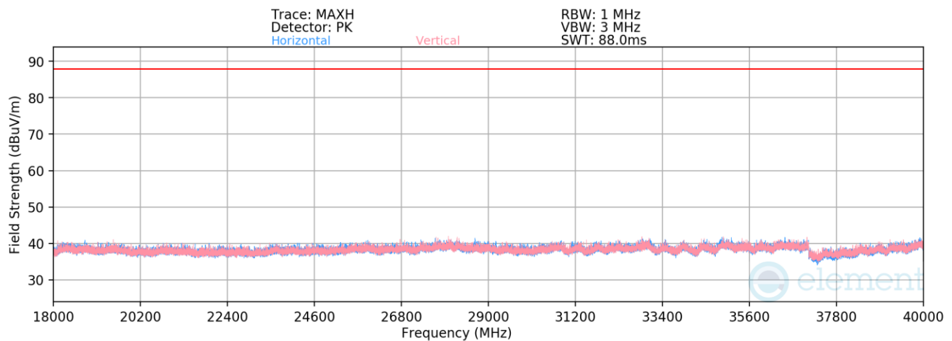
Plot 7-417. Radiated Spurious Emissions Above 18GHz (HDR4 ePA – 6263MHz)
