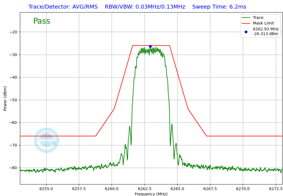
Plot 7-396. In-Band Emissions TxBF Diversity Antenna WF8 (NB UNII HDT4, ePA – 6263MHz)
