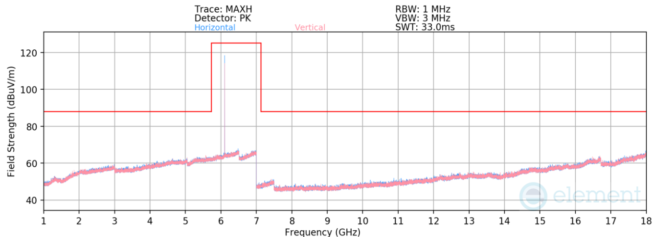
Plot 7-419. Radiated Spurious Emissions 1-18GHz TxBF Primary (LE1M ePA – 6108MHz)
