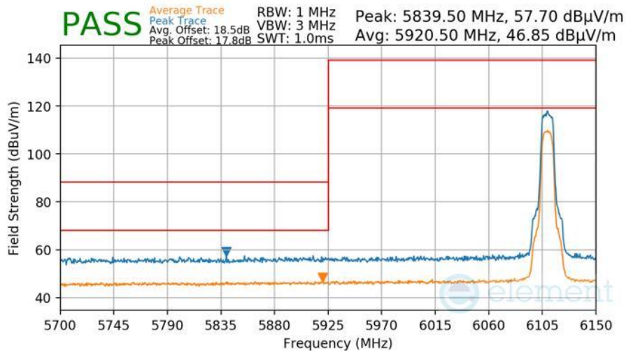
Plot 7-454 Radiated Lower Band Edge Measurement Antenna WF8
