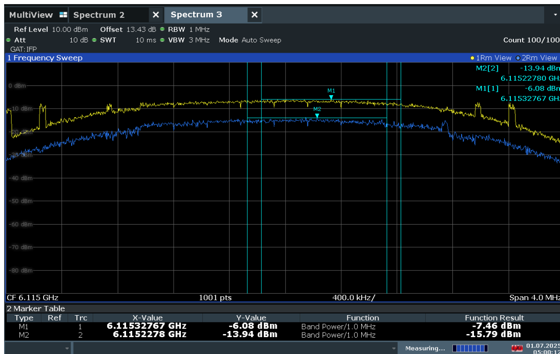
Plot 7-408. Power Density Plot – 6115MHz Antenna WF5B
