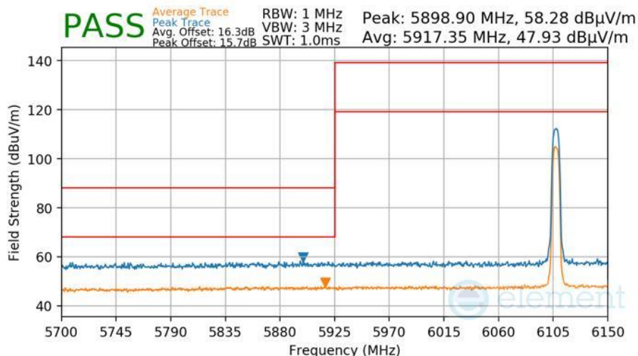
Plot 7-453 Radiated Lower Band Edge Measurement Antenna WF8
