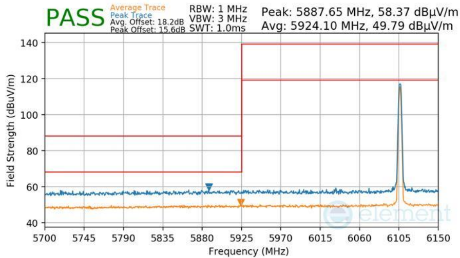
Plot 7-448 Radiated Lower Band Edge Measurement Antenna WF8
