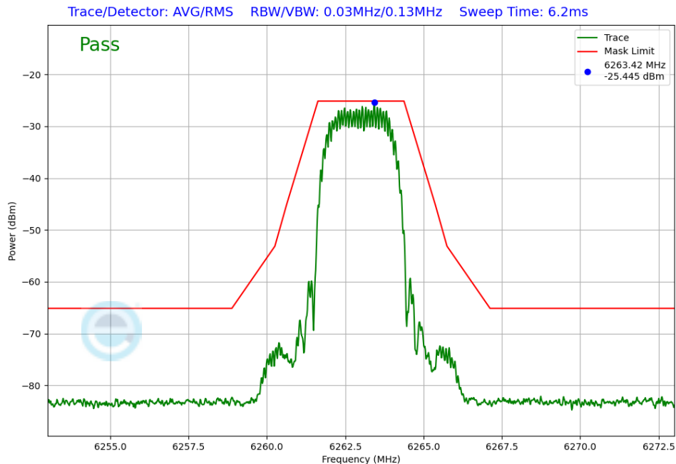
Plot 7-395. In-Band Emissions TxBF Diversity Antenna WF7 (NB UNII HDT2, iPA – 6263MHz)
