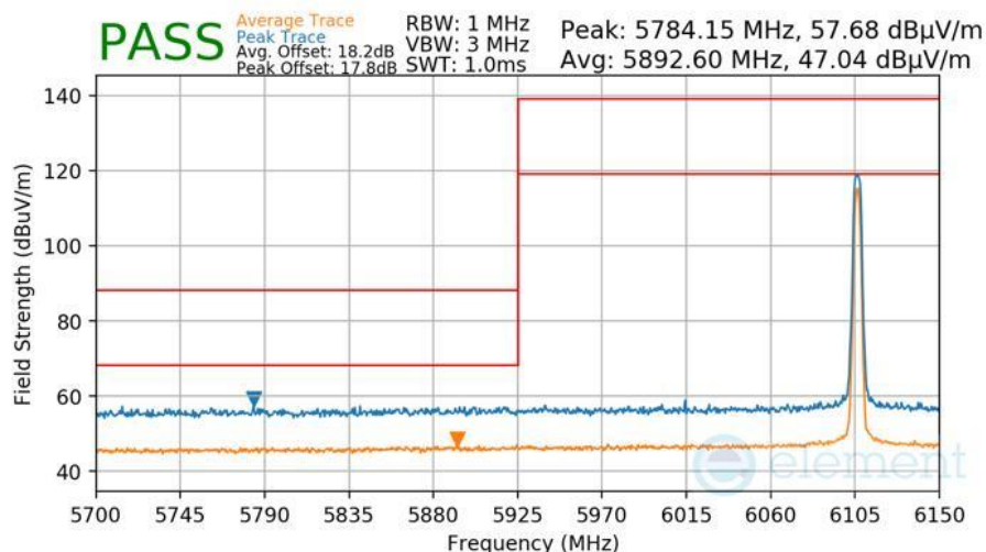
Plot 7-451 Radiated Lower Band Edge Measurement Antenna WF8
