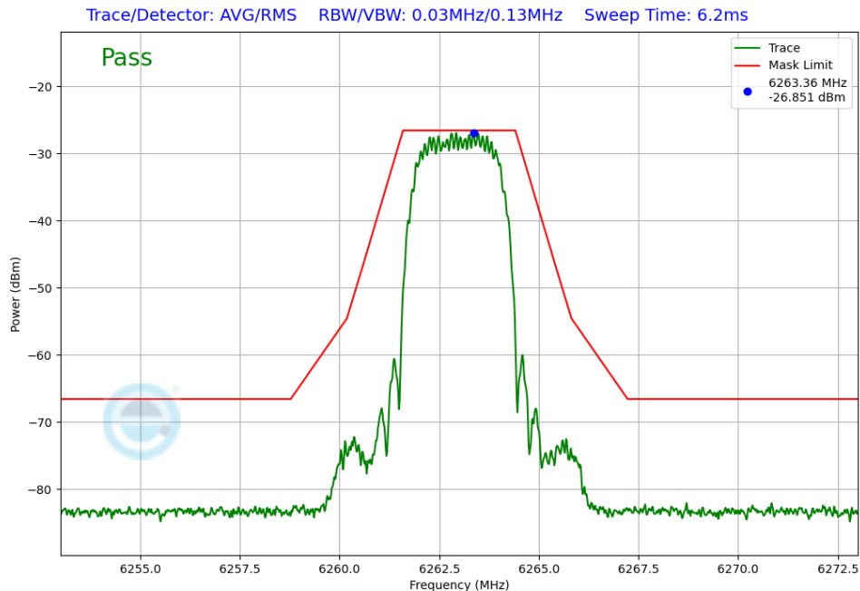
Plot 7-399. In-Band Emissions TxBF Diversity Antenna WF7 (NB UNII HDT4, iPA – 6263MHz)
