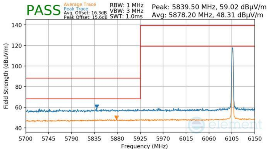
Plot 7-447 Radiated Lower Band Edge Measurement Antenna WF8
