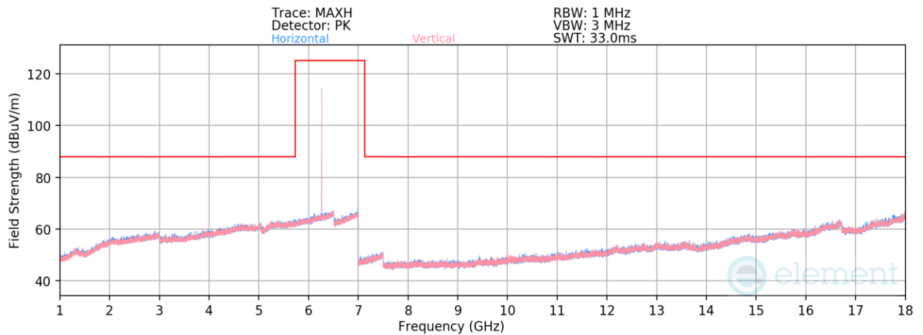
Plot 7-424. Radiated Spurious Emissions 1-18GHz TxBF Diversity (BDR GFSK ePA – 6263MHz)
