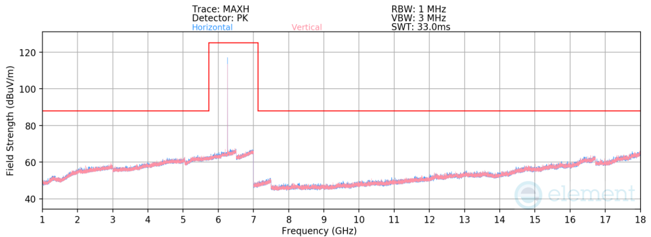
Plot 7-412. Radiated Spurious Emissions 1-18GHz TxBF Primary (BDR GFSK ePA – 6263MHz)
