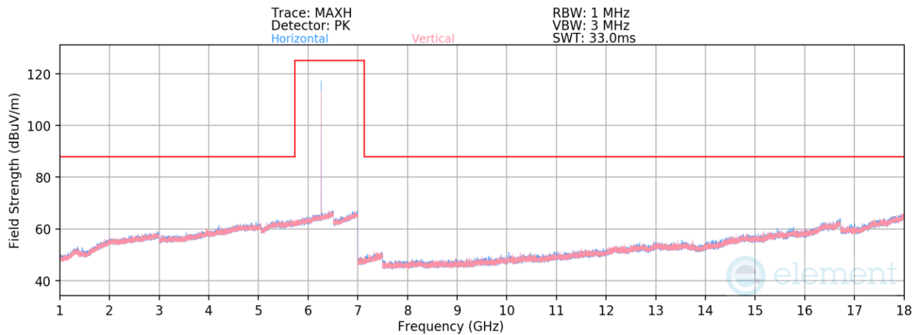
Plot 7-420. Radiated Spurious Emissions 1-18GHz TxBF Primary (LE1M ePA – 6263MHz)
