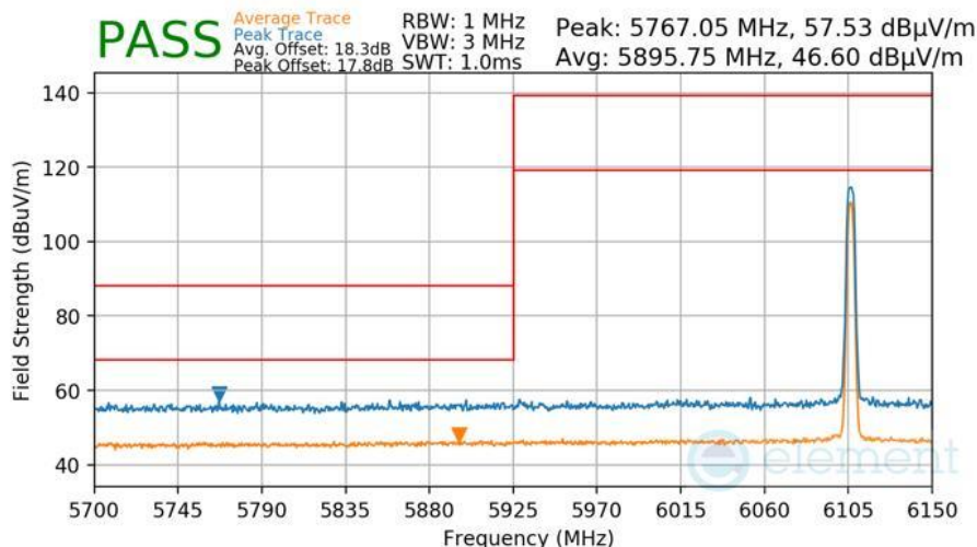
Plot 7-440 Radiated Lower Band Edge Measurement Antenna WF5B
