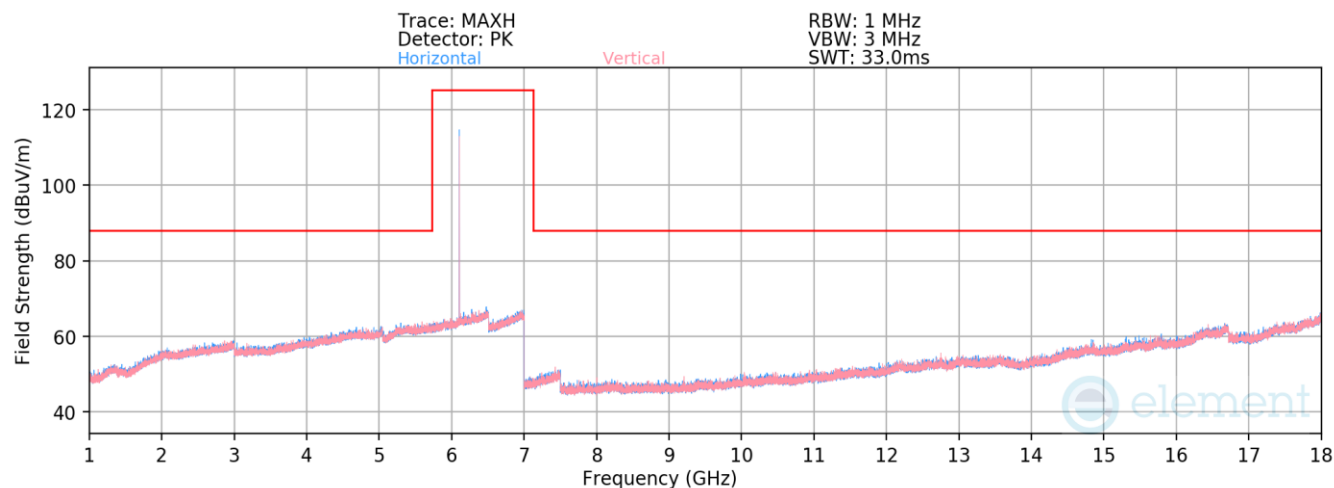
Plot 7-431. Radiated Spurious Emissions 1-18GHz TxBF Diversity (LE1M ePA – 6108MHz)
