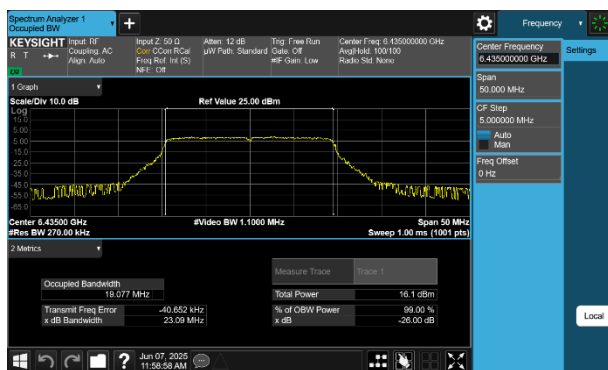
Plot 7-17 26dB BW & 99% OBW Antenna WF5B (20MHz BW 802.11be(SU) - Ch.97)
