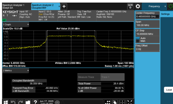
Plot 7-62 26dB BW & 99% OBW Antenna WF7 (40MHz BW 802.11be(SU) - Ch.107)
