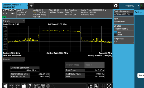
Plot 7-20 26dB BW & 99% OBW Antenna WF5B (160MHz BW 802.11be(SU) - Ch.111)
