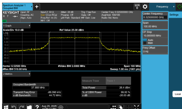
Plot 7-34 26dB BW & 99% OBW Antenna WF8 (40MHz BW 802.11be(SU) - Ch.115)
