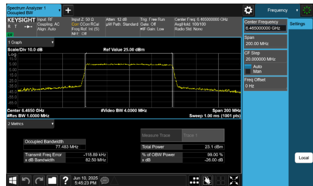
Plot 7-47 26dB BW & 99% OBW Antenna WF8 (80MHz BW 802.11be(SU) - Ch.103)
