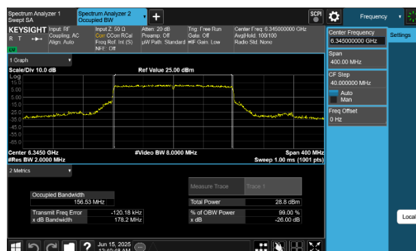
Plot 7-32 26dB BW & 99% OBW Antenna WF8 (160MHz BW 802.11be(SU) - Ch.79)
