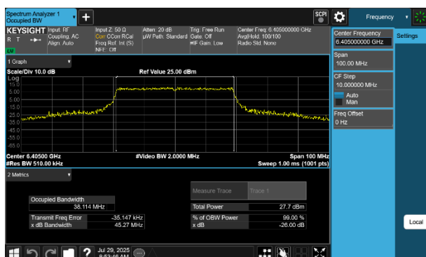
Plot 7-2 26dB BW & 99% OBW Antenna WF5B (40MHz BW 802.11be(SU) - Ch.91)
