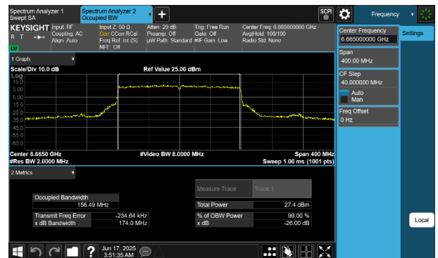
Plot 7-68 26dB BW & 99% OBW Antenna WF7 (160MHz BW 802.11be(SU) - Ch.143)
