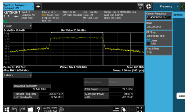
Plot 7-3 26dB BW & 99% OBW Antenna WF5B (80MHz BW 802.11be(SU) - Ch.39)
