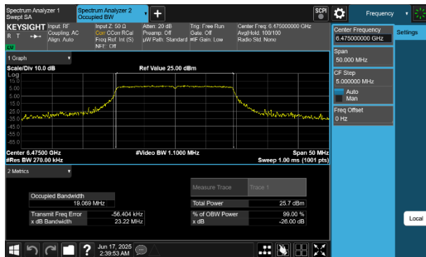
Plot 7-61 26dB BW & 99% OBW Antenna WF7 (20MHz BW 802.11be(SU) - Ch.105)
