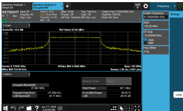
Plot 7-66 26dB BW & 99% OBW Antenna WF7 (40MHz BW 802.11be(SU) - Ch.155)
