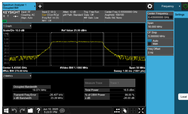
Plot 7-45 26dB BW & 99% OBW Antenna WF8 (20MHz BW 802.11be(SU) - Ch.97)
