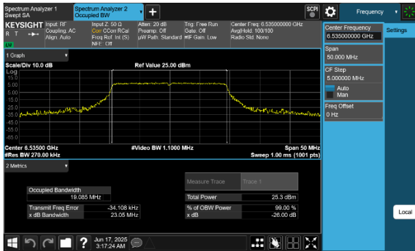
Plot 7-65 26dB BW & 99% OBW Antenna WF7 (20MHz BW 802.11be(SU) - Ch.117)
