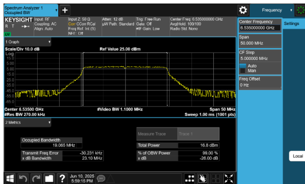
Plot 7-49 26dB BW & 99% OBW Antenna WF8 (20MHz BW 802.11be(SU) - Ch.117)
