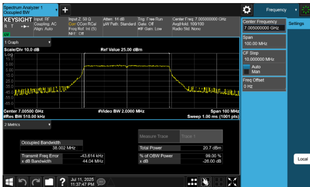
Plot 7-54 26dB BW & 99% OBW Antenna WF8 (40MHz BW 802.11be(SU) - Ch.211)
