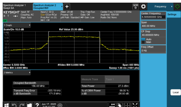
Plot 7-64 26dB BW & 99% OBW Antenna WF7 (160MHz BW 802.11be(SU) - Ch.111)
