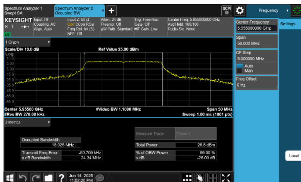
Plot 7-29 26dB BW & 99% OBW Antenna WF8 (20MHz BW 802.11a - Ch.1)
