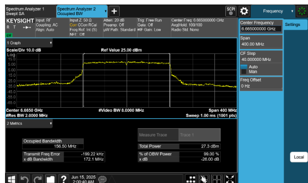
Plot 7-40 26dB BW & 99% OBW Antenna WF8 (160MHz BW 802.11be(SU) - Ch.143)
