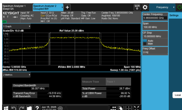
Plot 7-30 26dB BW & 99% OBW Antenna WF8 (40MHz BW 802.11be(SU) - Ch.3)
