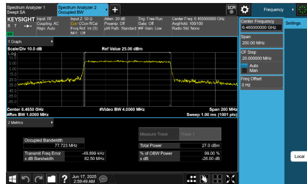
Plot 7-63 26dB BW & 99% OBW Antenna WF7 (80MHz BW 802.11be(SU) - Ch.103)
