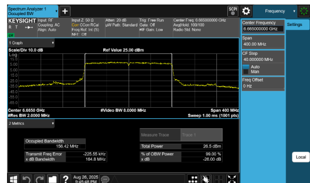
Plot 7-52 26dB BW & 99% OBW Antenna WF8 (160MHz BW 802.11be(SU) - Ch.143)
