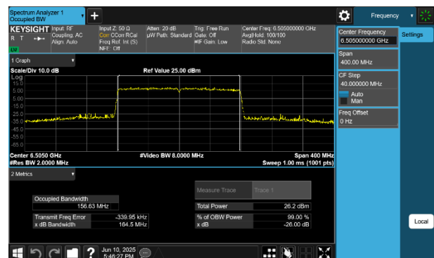
Plot 7-48 26dB BW & 99% OBW Antenna WF8 (160MHz BW 802.11be(SU) - Ch.111)
