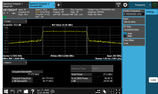
Plot 7-39 26dB BW & 99% OBW Antenna WF8 (80MHz BW 802.11be(SU) - Ch.167)
