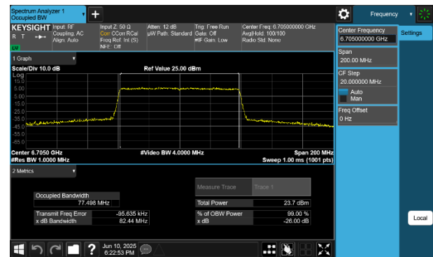
Plot 7-51 26dB BW & 99% OBW Antenna WF8 (80MHz BW 802.11be(SU) - Ch.151)
