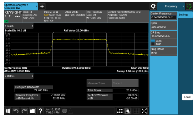
Plot 7-55 26dB BW & 99% OBW Antenna WF8 (80MHz BW 802.11be(SU) - Ch.199)
