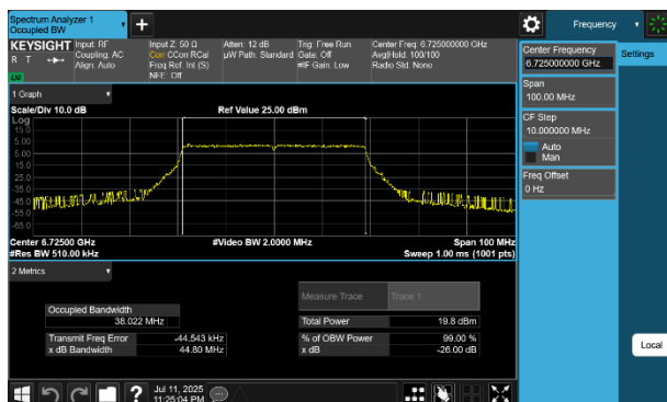
Plot 7-50 26dB BW & 99% OBW Antenna WF8 (40MHz BW 802.11be(SU) - Ch.155)
