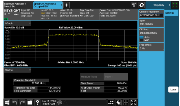
Plot 7-67 26dB BW & 99% OBW Antenna WF7 (80MHz BW 802.11be(SU) - Ch.167)
