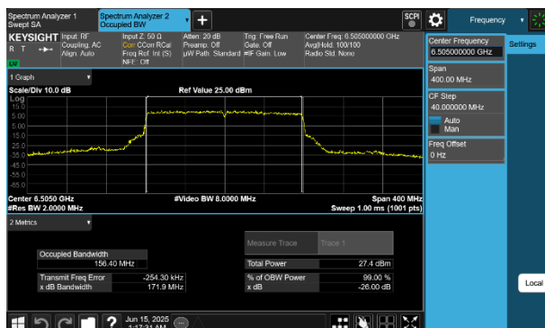
Plot 7-36 26dB BW & 99% OBW Antenna WF8 (160MHz BW 802.11be(SU) - Ch.111)
