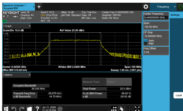
Plot 7-46 26dB BW & 99% OBW Antenna WF8 (40MHz BW 802.11be(SU) - Ch.99)
