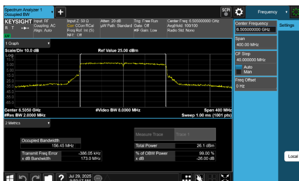
Plot 7-8 26dB BW & 99% OBW Antenna WF5B (160MHz BW 802.11be(SU) - Ch.111)
