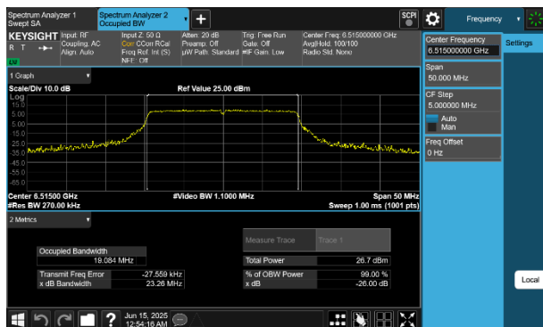
Plot 7-33 26dB BW & 99% OBW Antenna WF8 (20MHz BW 802.11be(SU) - Ch.113)
