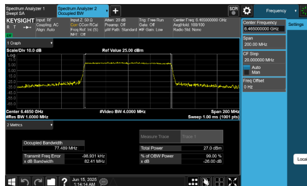
Plot 7-35 26dB BW & 99% OBW Antenna WF8 (80MHz BW 802.11be(SU) - Ch.103)
