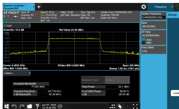
Plot 7-19 26dB BW & 99% OBW Antenna WF5B (80MHz BW 802.11be(SU) - Ch.103)
