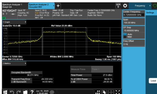
Plot 7-38 26dB BW & 99% OBW Antenna WF8 (40MHz BW 802.11be(SU) - Ch.155)
