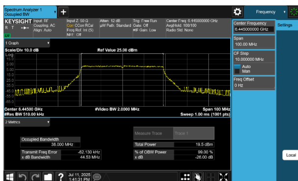
Plot 7-18 26dB BW & 99% OBW Antenna WF5B (40MHz BW 802.11be(SU) - Ch.99)
