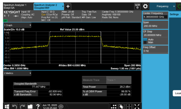
Plot 7-31 26dB BW & 99% OBW Antenna WF8 (80MHz BW 802.11be(SU) - Ch.87)
