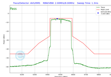
Plot 7-200 In-Band Emission Plot Antenna WF7 (160MHz BW 802.11be(SU) (UNII Band 6) - Ch.111)
