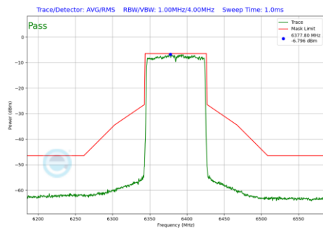
Plot 7-195 In-Band Emission Plot Antenna WF7 (80MHz BW 802.11be(SU) (UNII Band 5) - Ch.87)
