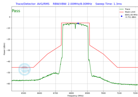
Plot 7-204 In-Band Emission Plot Antenna WF7 (160MHz BW 802.11be(SU) (UNII Band 7) - Ch.175)
