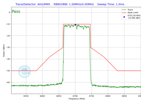
Plot 7-219 In-Band Emission Plot SDM Primary Antenna WF5B (80MHz BW 802.11be(SU) (UNII Band 7) - Ch.151)
