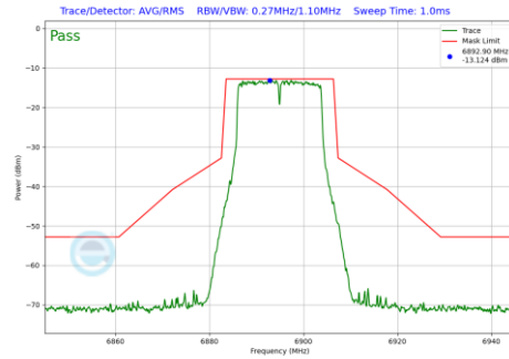
Plot 7-173 In-Band Emission Plot Antenna WF5B (20MHz BW 802.11a (UNII Band 8) - Ch.189)
