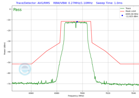
Plot 7-189 In-Band Emission Plot Antenna WF8 (20MHz BW 802.11a (UNII Band 8) - Ch.209)
