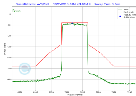
Plot 7-207 In-Band Emission Plot Antenna WF7 (80MHz BW 802.11be(SU) (UNII Band 8) - Ch.215)
