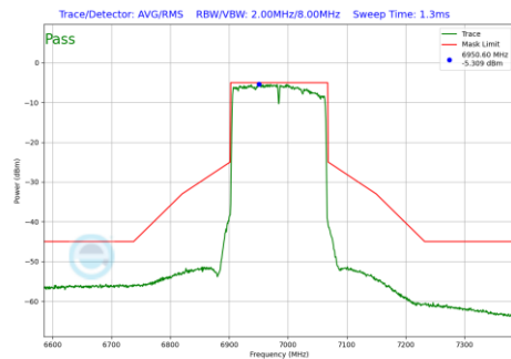
Plot 7-192 In-Band Emission Plot Antenna WF8 (160MHz BW 802.11be(SU) (UNII Band 8) - Ch.207)
