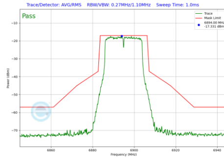
Plot 7-221 In-Band Emission Plot CDD Primary Antenna WF5B (20MHz BW 802.11a (UNII Band 8) - Ch.189)
