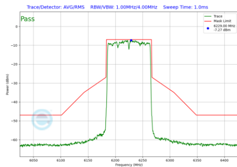
Plot 7-179 In-Band Emission Plot Antenna WF8 (80MHz BW 802.11be(SU) (UNII Band 5) - Ch.55)
