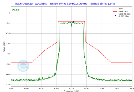
Plot 7-194 In-Band Emission Plot Antenna WF7 (40MHz BW 802.11be(SU) (UNII Band 5) - Ch.35)
