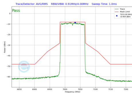
Plot 7-175 In-Band Emission Plot Antenna WF5B (80MHz BW 802.11be(SU) (UNII Band 8) - Ch.215)
