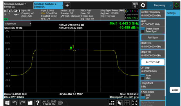
Plot 7-142 PSD SDM Diversity Antenna WF7 (40MHz BW 802.11be(SU) - Ch.99)
