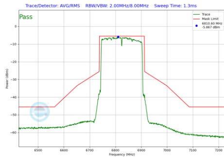
Plot 7-188 In-Band Emission Plot Antenna WF8 (160MHz BW 802.11be(SU) (UNII Band 7) - Ch.175)
