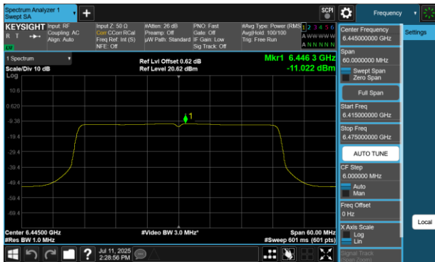
Plot 7-138 PSD SDM Diversity Antenna WF8 (40MHz BW 802.11be(SU) - Ch.99)
