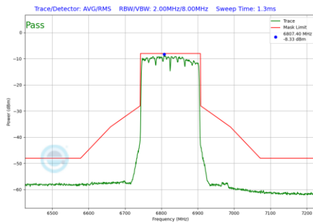
Plot 7-220 In-Band Emission Plot SDM Primary Antenna WF5B (160MHz BW 802.11be(SU) (UNII Band 7) - Ch.175)
