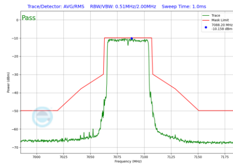
Plot 7-206 In-Band Emission Plot Antenna WF7 (40MHz BW 802.11be(SU) (UNII Band 8) - Ch.227)
