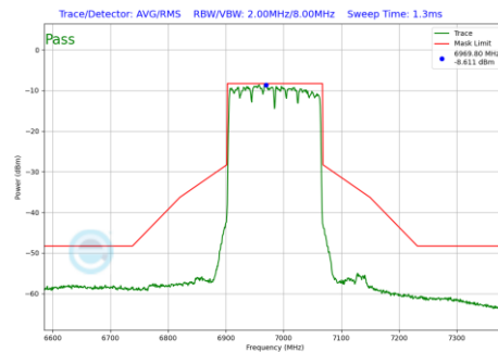
Plot 7-224 In-Band Emission Plot SDM Primary Antenna WF5B (160MHz BW 802.11be(SU) (UNII Band 8) - Ch.207)
