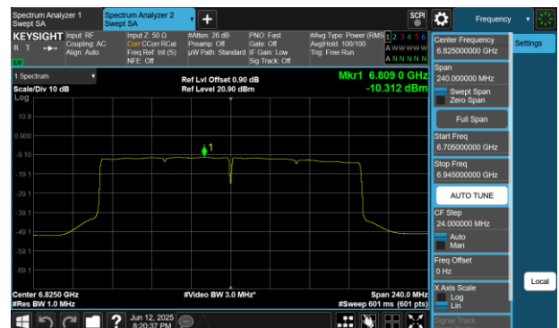
Plot 7-152 PSD SDM Diversity Antenna WF7 (160MHz BW 802.11be(SU) - Ch.175)
