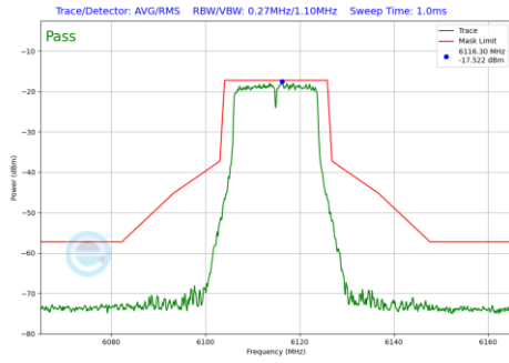
Plot 7-209 In-Band Emission Plot CDD Primary Antenna WF5B (20MHz BW 802.11a (UNII Band 5) - Ch.33)
