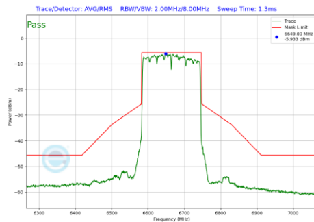
Plot 7-172 In-Band Emission Plot Antenna WF5B (160MHz BW 802.11be(SU) (UNII Band 7) - Ch.143)
