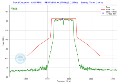
Plot 7-217 In-Band Emission Plot CDD Primary Antenna WF5B (20MHz BW 802.11a (UNII Band 7) - Ch.185)
