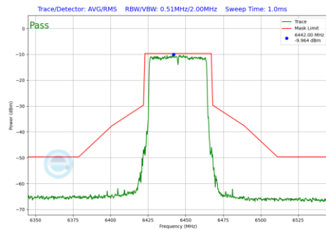
Plot 7-182 In-Band Emission Plot Antenna WF8 (40MHz BW 802.11be(SU) (UNII Band 6) - Ch.99)
