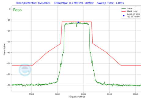
Plot 7-193 In-Band Emission Plot Antenna WF7 (20MHz BW 802.11be(SU) (UNII Band 5) - Ch.93)
