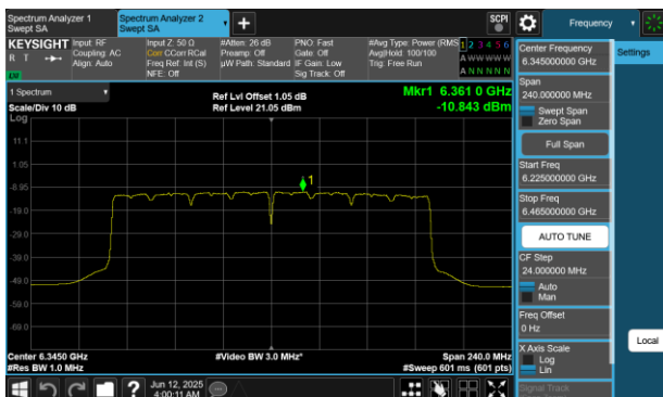
Plot 7-132 PSD SDM Diversity Antenna WF8 (160MHz BW 802.11be(SU) - Ch.79)
