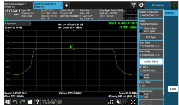
Plot 7-134 PSD SDM Diversity Antenna WF7 (40MHz BW 802.11be(SU) - Ch.91)
