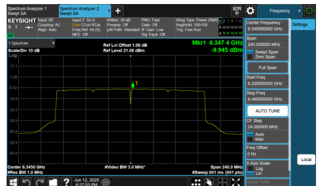
Plot 7-136 PSD SDM Diversity Antenna WF7 (160MHz BW 802.11be(SU) - Ch.79)
