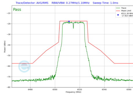
Plot 7-213 In-Band Emission Plot CDD Primary Antenna WF5B (20MHz BW 802.11a (UNII Band 6) - Ch.113)
