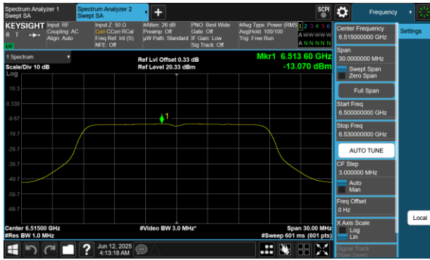
Plot 7-137 PSD CDD Diversity Antenna WF8 (20MHz BW 802.11a - Ch.113)
