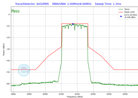
Plot 7-212 In-Band Emission Plot SDM Primary Antenna WF5B (160MHz BW 802.11be(SU) (UNII Band 5) - Ch.47)
