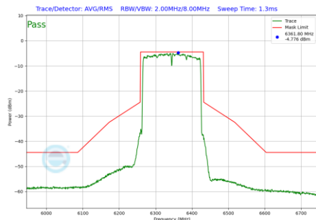
Plot 7-196 In-Band Emission Plot Antenna WF7 (160MHz BW 802.11be(SU) (UNII Band 5) - Ch.79)
