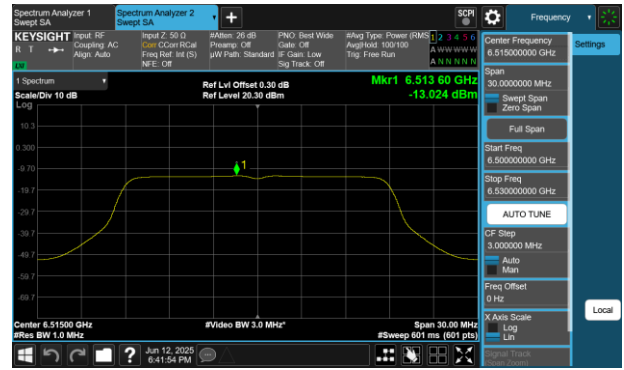
Plot 7-141 PSD CDD Diversity Antenna WF7 (20MHz BW 802.11a - Ch.113)
