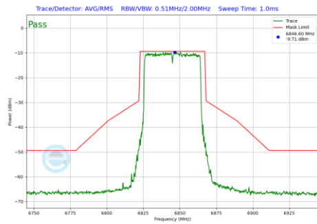
Plot 7-186 In-Band Emission Plot Antenna WF8 (40MHz BW 802.11be(SU) (UNII Band 7) - Ch.179)
