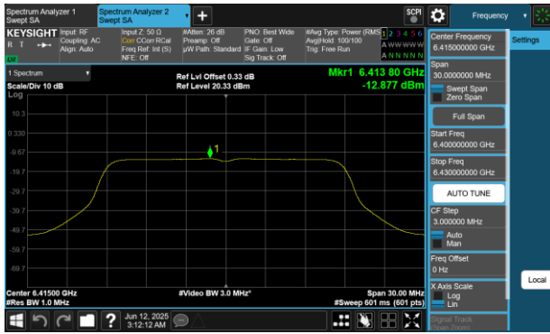
Plot 7-129 PSD CDD Diversity Antenna WF8 (20MHz BW 802.11a - Ch.93)
