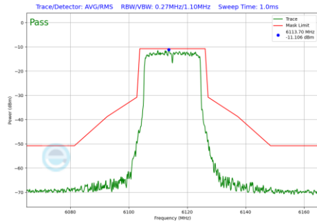
Plot 7-161 In-Band Emission Plot Antenna WF5B (20MHz BW 802.11be(SU) (UNII Band 5) - Ch.33)
