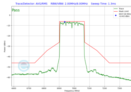
Plot 7-176 In-Band Emission Plot Antenna WF5B (160MHz BW 802.11be(SU) (UNII Band 8) - Ch.207)
