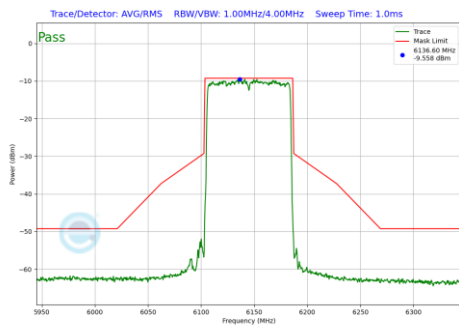
Plot 7-211 In-Band Emission Plot SDM Primary Antenna WF5B (80MHz BW 802.11be(SU) (UNII Band 5) - Ch.39)
