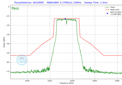
Plot 7-181 In-Band Emission Plot Antenna WF8 (20MHz BW 802.11a (UNII Band 6) - Ch.97)
