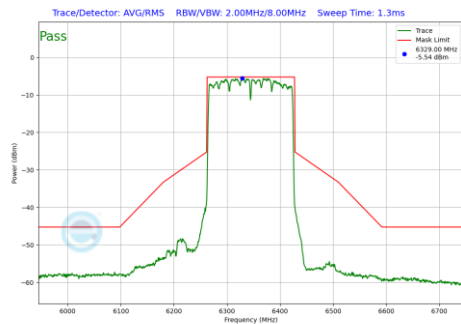
Plot 7-180 In-Band Emission Plot Antenna WF8 (160MHz BW 802.11be(SU) (UNII Band 5) - Ch.79)
