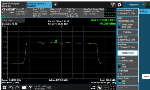
Plot 7-155 PSD SDM Diversity Antenna WF8 (80MHz BW 802.11be(SU) - Ch.199)
