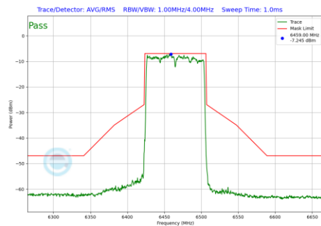
Plot 7-183 In-Band Emission Plot Antenna WF8 (80MHz BW 802.11be(SU) (UNII Band 6) - Ch.103)
