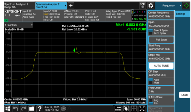
Plot 7-158 PSD SDM Diversity Antenna WF7 (40MHz BW 802.11be(SU) - Ch.187)
