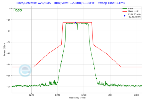
Plot 7-177 In-Band Emission Plot Antenna WF8 (20MHz BW 802.11a (UNII Band 5) - Ch.61)
