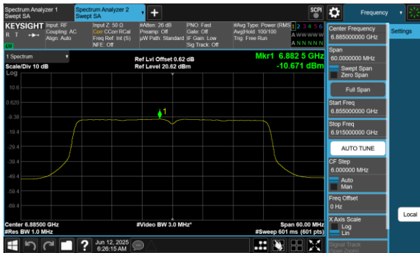
Plot 7-154 PSD SDM Diversity Antenna WF8 (40MHz BW 802.11be(SU) - Ch.187)
