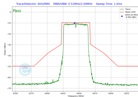
Plot 7-198 In-Band Emission Plot Antenna WF7 (40MHz BW 802.11be(SU) (UNII Band 6) - Ch.99)
