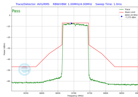
Plot 7-203 In-Band Emission Plot Antenna WF7 (80MHz BW 802.11be(SU) (UNII Band 7) - Ch.151)
