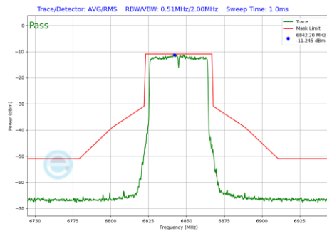
Plot 7-202 In-Band Emission Plot Antenna WF7 (40MHz BW 802.11be(SU) (UNII Band 7) - Ch.179)
