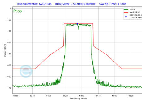
Plot 7-214 In-Band Emission Plot SDM Primary Antenna WF5B (40MHz BW 802.11be(SU) (UNII Band 6) - Ch.99)
