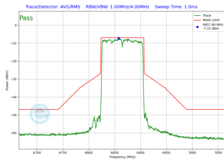
Plot 7-171 In-Band Emission Plot Antenna WF5B (80MHz BW 802.11be(SU) (UNII Band 7) - Ch.183)
