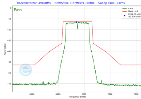
Plot 7-205 In-Band Emission Plot Antenna WF7 (20MHz BW 802.11a (UNII Band 8) - Ch.209)
