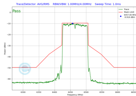
Plot 7-215 In-Band Emission Plot SDM Primary Antenna WF5B (80MHz BW 802.11be(SU) (UNII Band 6) - Ch.103)
