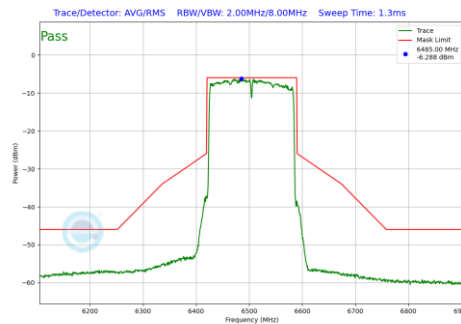
Plot 7-184 In-Band Emission Plot Antenna WF8 (160MHz BW 802.11be(SU) (UNII Band 6) - Ch.111)
