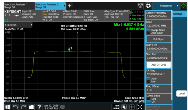
Plot 7-159 PSD SDM Diversity Antenna WF7 (80MHz BW 802.11be(SU) - Ch.199)
