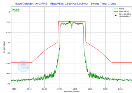
Plot 7-178 In-Band Emission Plot Antenna WF8 (40MHz BW 802.11be(SU) (UNII Band 5) - Ch.59)
