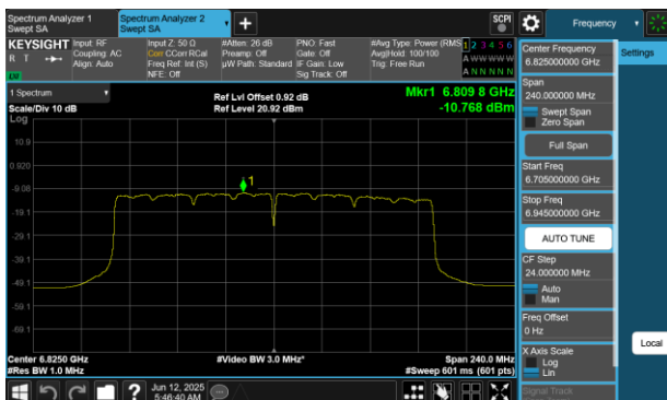
Plot 7-148 PSD SDM Diversity Antenna WF8 (160MHz BW 802.11be(SU) - Ch.175)
