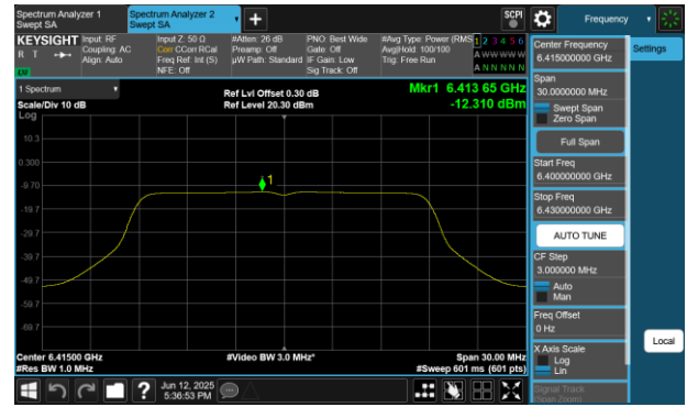
Plot 7-133 PSD CDD Diversity Antenna WF7 (20MHz BW 802.11a - Ch.93)
