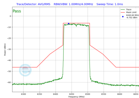
Plot 7-199 In-Band Emission Plot Antenna WF7 (80MHz BW 802.11be(SU) (UNII Band 6) - Ch.103)
