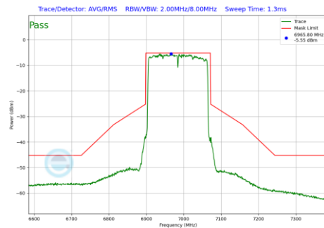
Plot 7-208 In-Band Emission Plot Antenna WF7 (160MHz BW 802.11be(SU) (UNII Band 8) - Ch.207)
