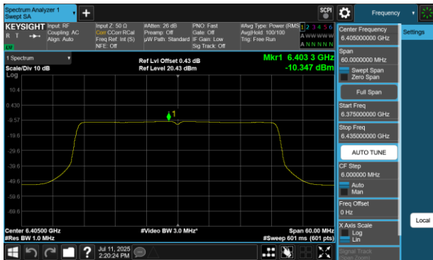
Plot 7-130 PSD SDM Diversity Antenna WF8 (40MHz BW 802.11be(SU) - Ch.91)
