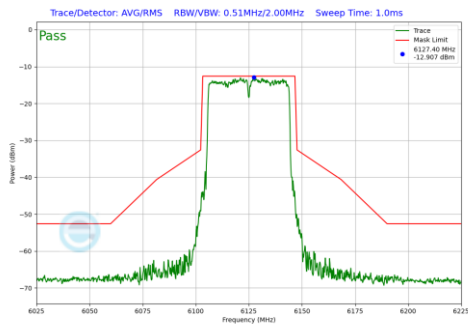
Plot 7-210 In-Band Emission Plot SDM Primary Antenna WF5B (40MHz BW 802.11be(SU) (UNII Band 5) - Ch.35)
