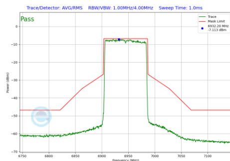
Plot 7-191 In-Band Emission Plot Antenna WF8 (80MHz BW 802.11be(SU) (UNII Band 8) - Ch.199)
