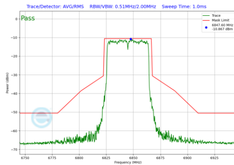
Plot 7-170 In-Band Emission Plot Antenna WF5B (40MHz BW 802.11be(SU) (UNII Band 7) - Ch.179)
