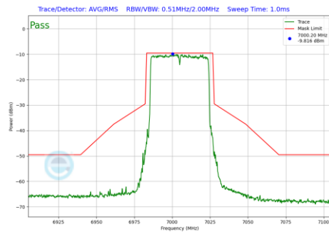
Plot 7-190 In-Band Emission Plot Antenna WF8 (40MHz BW 802.11be(SU) (UNII Band 8) - Ch.211)
