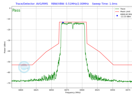
Plot 7-222 In-Band Emission Plot SDM Primary Antenna WF5B (40MHz BW 802.11be(SU) (UNII Band 8) - Ch.187)
