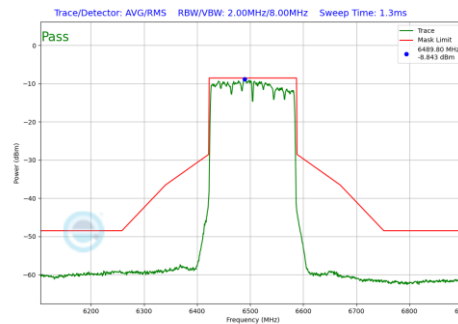
Plot 7-216 In-Band Emission Plot SDM Primary Antenna WF5B (160MHz BW 802.11be(SU) (UNII Band 6) - Ch.111)
