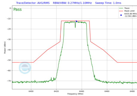
Plot 7-197 In-Band Emission Plot Antenna WF7 (20MHz BW 802.11a (UNII Band 6) - Ch.97)
