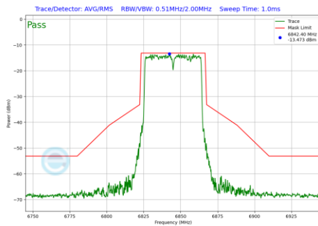
Plot 7-218 In-Band Emission Plot SDM Primary Antenna WF5B (40MHz BW 802.11be(SU) (UNII Band 7) - Ch.179)
