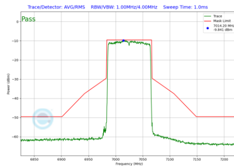
Plot 7-223 In-Band Emission Plot SDM Primary Antenna WF5B (80MHz BW 802.11be(SU) (UNII Band 8) - Ch.215)
