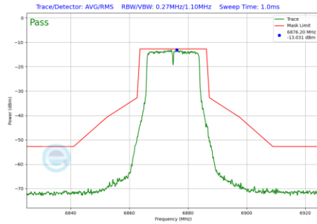
Plot 7-169 In-Band Emission Plot Antenna WF5B (20MHz BW 802.11a (UNII Band 7) - Ch.185)
