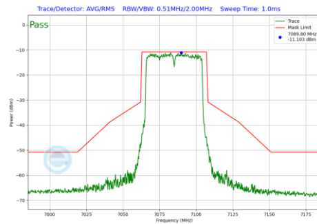
Plot 7-174 In-Band Emission Plot Antenna WF5B (40MHz BW 802.11be(SU) (UNII Band 8) - Ch.227)
