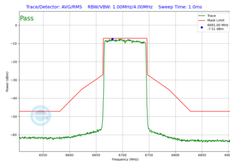
Plot 7-187 In-Band Emission Plot Antenna WF8 (80MHz BW 802.11be(SU) (UNII Band 7) - Ch.151)
