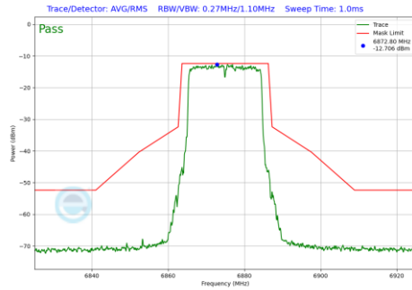
Plot 7-201 In-Band Emission Plot Antenna WF7 (20MHz BW 802.11be(SU) (UNII Band 7) - Ch.185)
