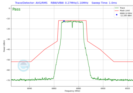
Plot 7-185 In-Band Emission Plot Antenna WF8 (20MHz BW 802.11a (UNII Band 7) - Ch.185)
