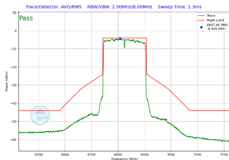
Plot 7-400 In-Band Emission Plot SDM Primary Antenna WF5B (160MHz BW 802.11be(SU) (UNII Band 7) - Ch.175)
