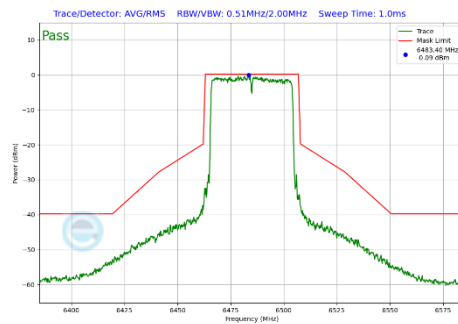
Plot 7-370 In-Band Emission Plot CDD Primary Antenna WF5B (40MHz BW 802.11be(SU) (UNII Band 6) - Ch.107)
