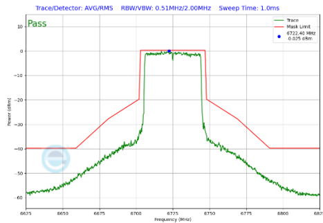
Plot 7-374 In-Band Emission Plot CDD Primary Antenna WF5B (40MHz BW 802.11be(SU) (UNII Band 7) - Ch.155)
