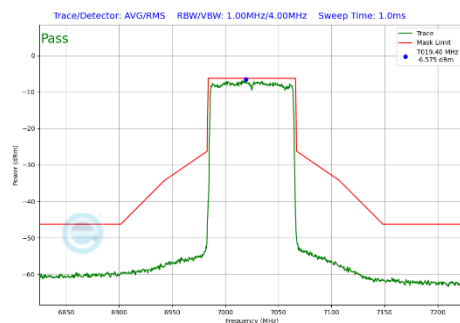
Plot 7-403 In-Band Emission Plot SDM Primary Antenna WF5B (80MHz BW 802.11be(SU) (UNII Band 8) - Ch.215)
