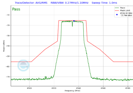
Plot 7-397 In-Band Emission Plot CDD Primary Antenna WF5B (20MHz BW 802.11a (UNII Band 7) - Ch.117)
