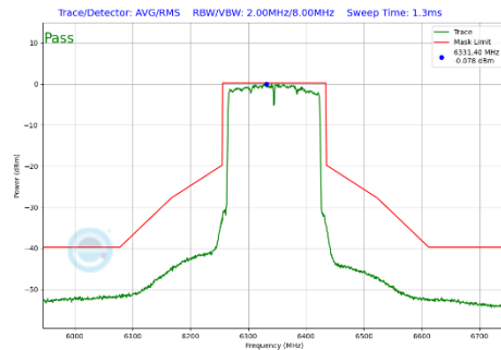
Plot 7-380 In-Band Emission Plot CDD Primary Antenna WF8 (160MHz BW 802.11be(SU) (UNII Band 5) - Ch.79)
