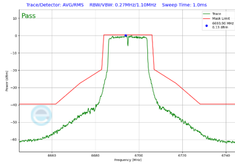
Plot 7-373 In-Band Emission Plot CDD Primary Antenna WF5B (20MHz BW 802.11a (UNII Band 7) - Ch.149)
