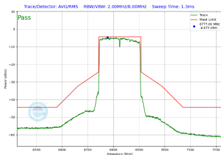
Plot 7-456 In-Band Emission Plot SDM Diversity Antenna WF7 (160MHz BW 802.11be(SU) (UNII Band 7) - Ch.175)
