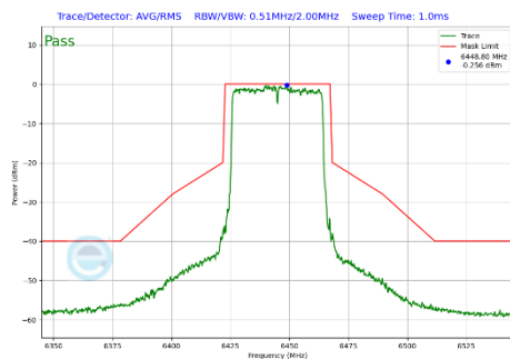
Plot 7-438 In-Band Emission Plot CDD Diversity Antenna WF8 (40MHz BW 802.11be(SU) (UNII Band 6) - Ch.99)
