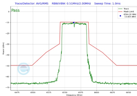
Plot 7-470 In-Band Emission Plot SDM Diversity Antenna WF8 (40MHz BW 802.11be(SU) (UNII Band 7) - Ch.123)
