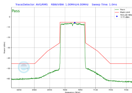
Plot 7-459 In-Band Emission Plot SDM Diversity Antenna WF7 (80MHz BW 802.11be(SU) (UNII Band 8) - Ch.215)
