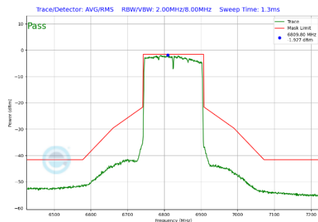
Plot 7-360 In-Band Emission Plot Antenna WF7 (160MHz BW 802.11be(SU) (UNII Band 7) - Ch.175)
