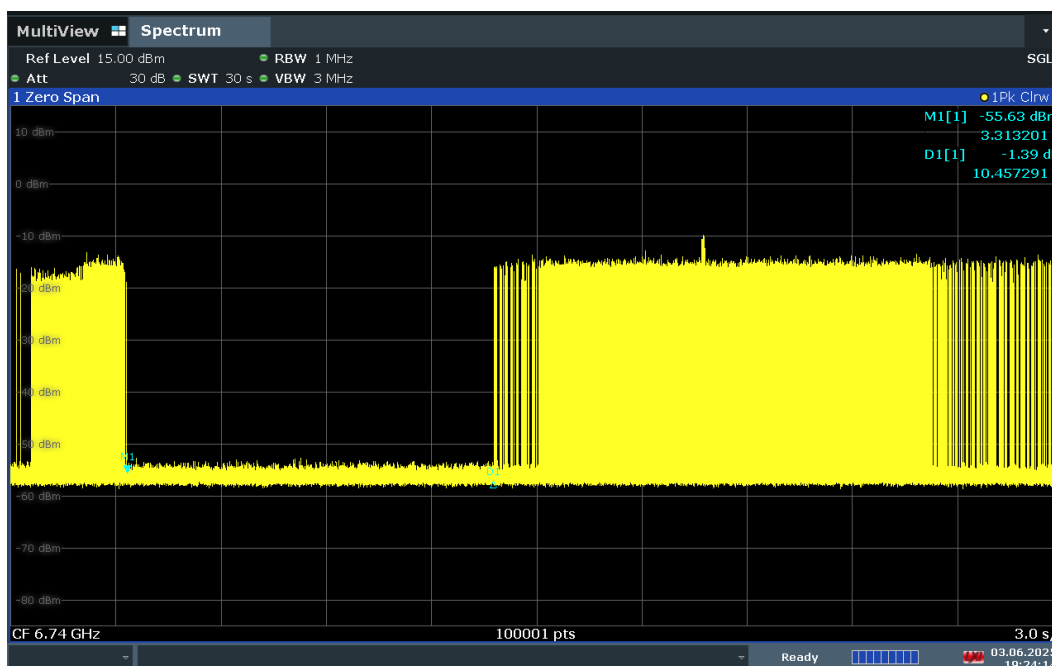
Plot 7-502. Contention Based Protocol Timing Plot – UNII 7 – 160MHz Channel 143 – Low
