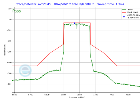
Plot 7-460 In-Band Emission Plot SDM Diversity Antenna WF7 (160MHz BW 802.11be(SU) (UNII Band 8) - Ch.207)
