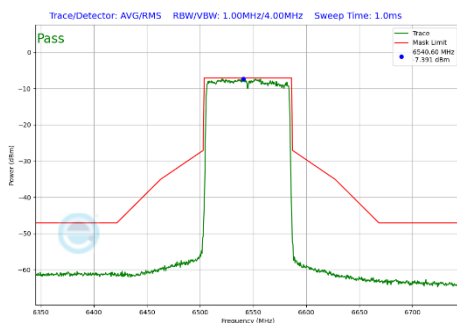
Plot 7-415 In-Band Emission Plot SDM Primary Antenna WF8 (80MHz BW 802.11be(SU) (UNII Band 7) - Ch.119)
