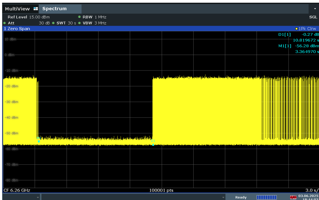
Plot 7-495. Contention Based Protocol Timing Plot –UNII 5 – 160MHz Channel 47 – Mid
