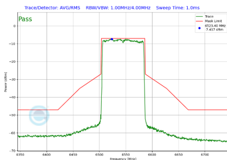
Plot 7-455 In-Band Emission Plot SDM Diversity Antenna WF7 (80MHz BW 802.11be(SU) (UNII Band 7) - Ch.119)
