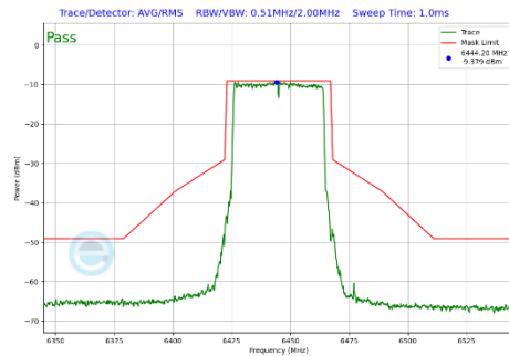
Plot 7-466 In-Band Emission Plot SDM Diversity Antenna WF8 (40MHz BW 802.11be(SU) (UNII Band 6) - Ch.99)
