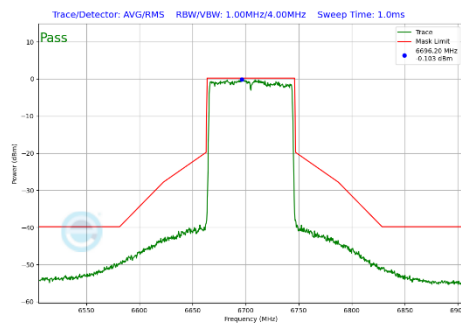
Plot 7-347 In-Band Emission Plot Antenna WF7 (80MHz BW 802.11be(SU) (UNII Band 7) - Ch.151)
