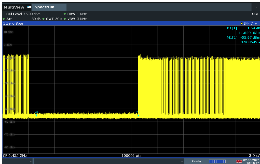
Plot 7-497. Contention Based Protocol Timing Plot – UNII 6 – 20MHz Channel 101
