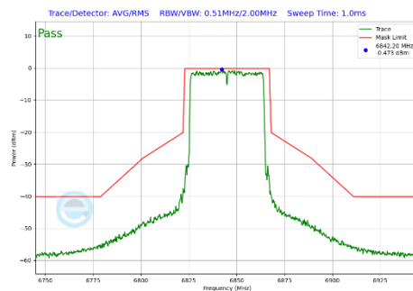
Plot 7-386 In-Band Emission Plot CDD Primary Antenna WF8 (40MHz BW 802.11be(SU) (UNII Band 7) - Ch.179)
