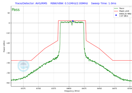
Plot 7-338 In-Band Emission Plot Antenna WF7 (40MHz BW 802.11be(SU) (UNII Band 5) - Ch.91)
