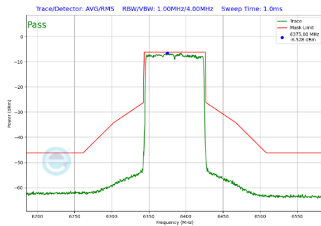
Plot 7-447 In-Band Emission Plot SDM Diversity Antenna WF7 (80MHz BW 802.11be(SU) (UNII Band 5) - Ch.87)
