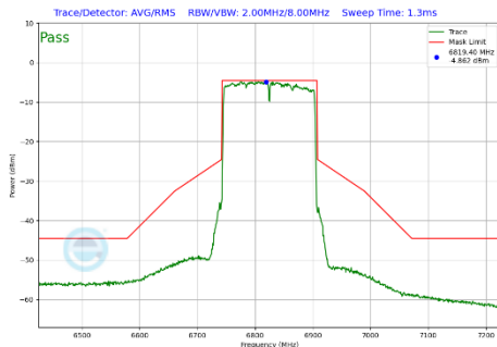
Plot 7-472 In-Band Emission Plot SDM Diversity Antenna WF8 (160MHz BW 802.11be(SU) (UNII Band 7) - Ch.175)
