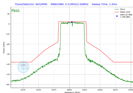
Plot 7-422 In-Band Emission Plot CDD Diversity Antenna WF7 (40MHz BW 802.11be(SU) (UNII Band 5) - Ch.91)
