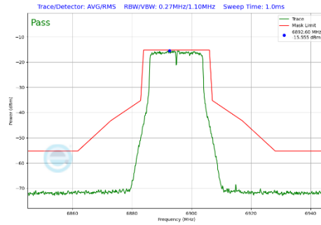
Plot 7-473 In-Band Emission Plot CDD Diversity Antenna WF8 (20MHz BW 802.11a (UNII Band 8) - Ch.189)
