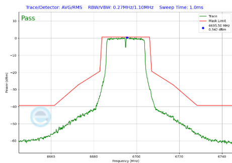
Plot 7-345 In-Band Emission Plot Antenna WF7 (20MHz BW 802.11a (UNII Band 7) - Ch.149)
