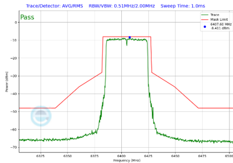
Plot 7-406 In-Band Emission Plot SDM Primary Antenna WF8 (40MHz BW 802.11be(SU) (UNII Band 5) - Ch.91)
