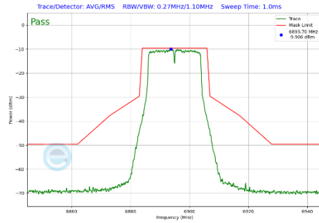
Plot 7-361 In-Band Emission Plot Antenna WF7 (20MHz BW 802.11a (UNII Band 8) - Ch.189)
