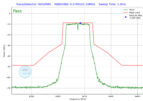
Plot 7-349 In-Band Emission Plot Antenna WF7 (20MHz BW 802.11a (UNII Band 5) - Ch.93)
