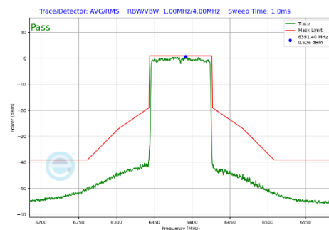
Plot 7-435 In-Band Emission Plot CDD Diversity Antenna WF8 (80MHz BW 802.11be(SU) (UNII Band 5) - Ch.87)
