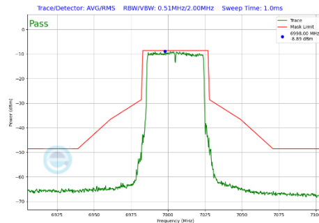
Plot 7-474 In-Band Emission Plot SDM Diversity Antenna WF8 (40MHz BW 802.11be(SU) (UNII Band 8) - Ch.211)
