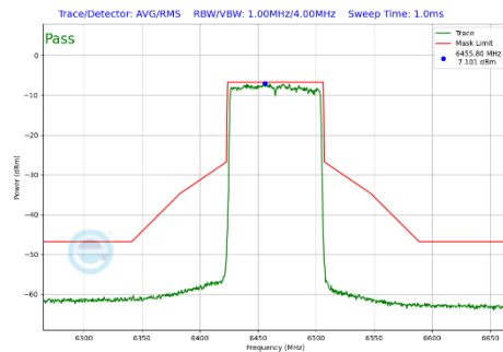
Plot 7-467 In-Band Emission Plot SDM Diversity Antenna WF8 (80MHz BW 802.11be(SU) (UNII Band 6) - Ch.103)
