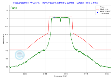
Plot 7-337 In-Band Emission Plot Antenna WF7 (20MHz BW 802.11a (UNII Band 5) - Ch.93)
