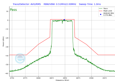
Plot 7-346 In-Band Emission Plot Antenna WF7 (40MHz BW 802.11be(SU) (UNII Band 7) - Ch.179)
