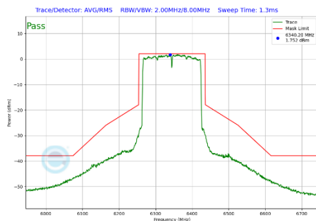
Plot 7-424 In-Band Emission Plot CDD Diversity Antenna WF7 (160MHz BW 802.11be(SU) (UNII Band 5) - Ch.79)
