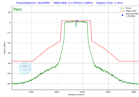
Plot 7-377 In-Band Emission Plot CDD Primary Antenna WF8 (20MHz BW 802.11a (UNII Band 5) - Ch.93)
