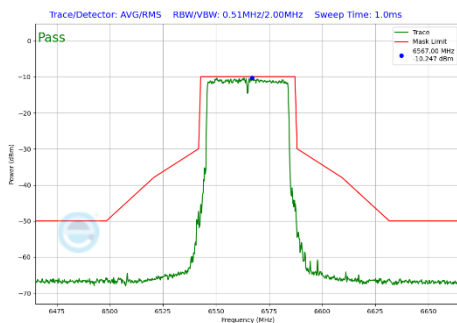
Plot 7-454 In-Band Emission Plot SDM Diversity Antenna WF7 (40MHz BW 802.11be(SU) (UNII Band 7) - Ch.123)
