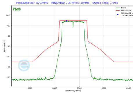
Plot 7-457 In-Band Emission Plot CDD Diversity Antenna WF7 (20MHz BW 802.11a (UNII Band 8) - Ch.189)
