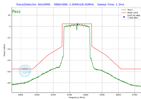
Plot 7-340 In-Band Emission Plot Antenna WF7 (160MHz BW 802.11be(SU) (UNII Band 5) - Ch.79)
