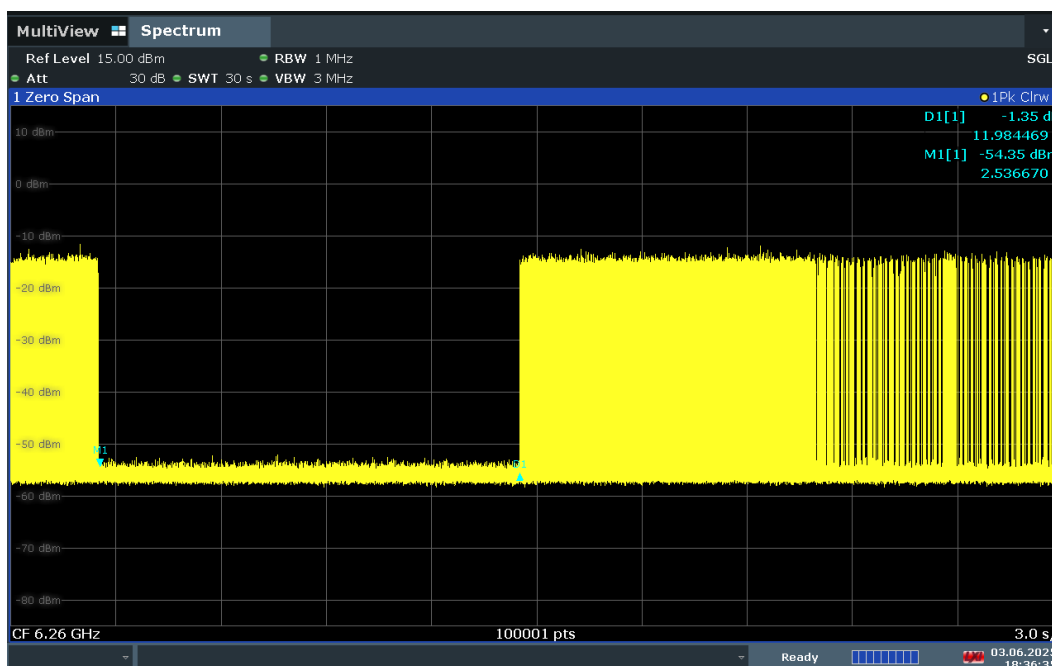
Plot 7-494. Contention Based Protocol Timing Plot – UNII 5 – 160MHz Channel 47 – Low
