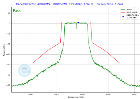
Plot 7-421 In-Band Emission Plot CDD Diversity Antenna WF7 (20MHz BW 802.11a (UNII Band 5) - Ch.93)
