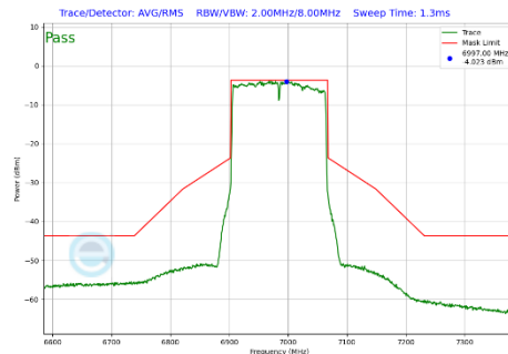
Plot 7-476 In-Band Emission Plot SDM Diversity Antenna WF8 (160MHz BW 802.11be(SU) (UNII Band 8) - Ch.207)
