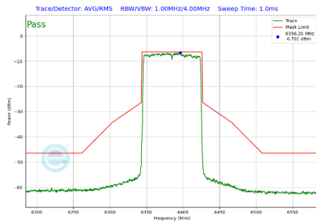
Plot 7-407 In-Band Emission Plot SDM Primary Antenna WF8 (80MHz BW 802.11be(SU) (UNII Band 5) - Ch.87)
