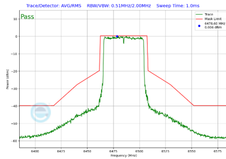
Plot 7-342 In-Band Emission Plot Antenna WF7 (40MHz BW 802.11be(SU) (UNII Band 6) - Ch.107)
