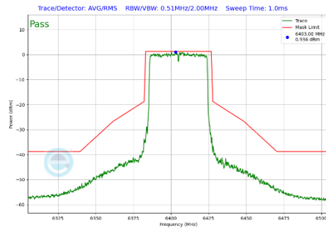
Plot 7-378 In-Band Emission Plot CDD Primary Antenna WF8 (40MHz BW 802.11be(SU) (UNII Band 5) - Ch.91)
