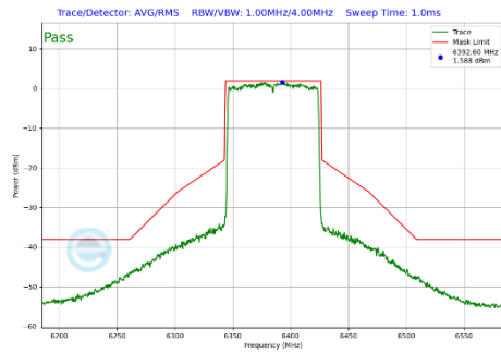
Plot 7-339 In-Band Emission Plot Antenna WF7 (80MHz BW 802.11be(SU) (UNII Band 5) - Ch.87)
