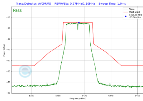
Plot 7-445 In-Band Emission Plot CDD Diversity Antenna WF7 (20MHz BW 802.11a (UNII Band 5) - Ch.93)
