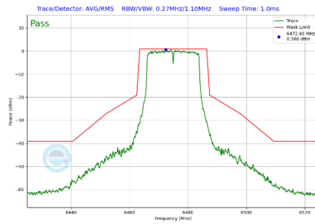
Plot 7-369 In-Band Emission Plot CDD Primary Antenna WF5B (20MHz BW 802.11a (UNII Band 6) - Ch.105)
