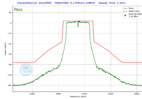
Plot 7-433 In-Band Emission Plot CDD Diversity Antenna WF8 (20MHz BW 802.11a (UNII Band 5) - Ch.93)
