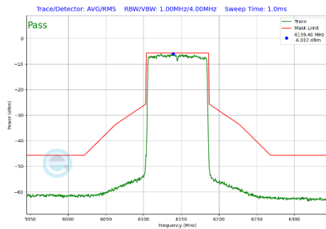
Plot 7-391 In-Band Emission Plot SDM Primary Antenna WF5B (80MHz BW 802.11be(SU) (UNII Band 5) - Ch.39)
