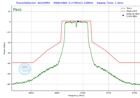
Plot 7-429 In-Band Emission Plot CDD Diversity Antenna WF7 (20MHz BW 802.11a (UNII Band 7) - Ch.149)
