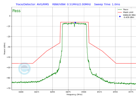
Plot 7-354 In-Band Emission Plot Antenna WF7 (40MHz BW 802.11be(SU) (UNII Band 6) - Ch.107)
