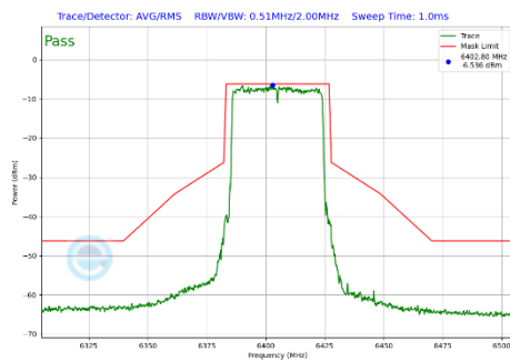
Plot 7-350 In-Band Emission Plot Antenna WF7 (40MHz BW 802.11be(SU) (UNII Band 5) - Ch.91)
