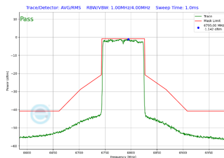
Plot 7-443 In-Band Emission Plot CDD Diversity Antenna WF8 (80MHz BW 802.11be(SU) (UNII Band 7) - Ch.167)
