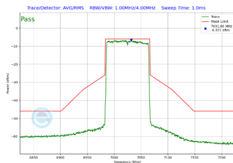
Plot 7-419 In-Band Emission Plot SDM Primary Antenna WF8 (80MHz BW 802.11be(SU) (UNII Band 8) - Ch.215)
