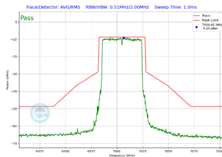
Plot 7-458 In-Band Emission Plot SDM Diversity Antenna WF7 (40MHz BW 802.11be(SU) (UNII Band 8) - Ch.211)
