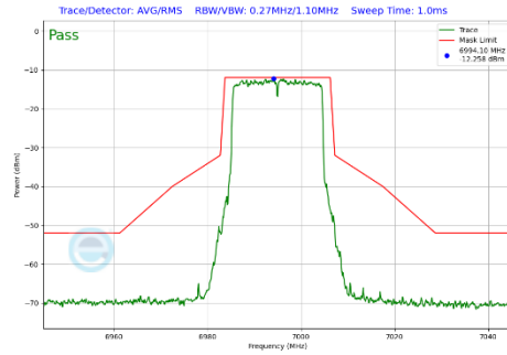
Plot 7-401 In-Band Emission Plot SDM Primary Antenna WF5B (20MHz BW 802.11be(SU) (UNII Band 8) - Ch.209)
