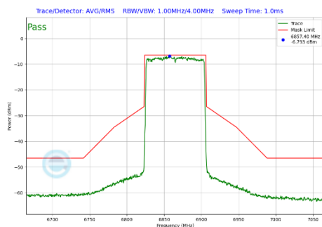
Plot 7-399 In-Band Emission Plot SDM Primary Antenna WF5B (80MHz BW 802.11be(SU) (UNII Band 7) - Ch.183)
