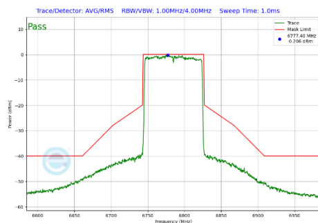
Plot 7-431 In-Band Emission Plot CDD Diversity Antenna WF7 (80MHz BW 802.11be(SU) (UNII Band 7) - Ch.167)
