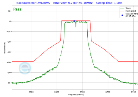
Plot 7-441 In-Band Emission Plot CDD Diversity Antenna WF8 (20MHz BW 802.11a (UNII Band 7) - Ch.149)
