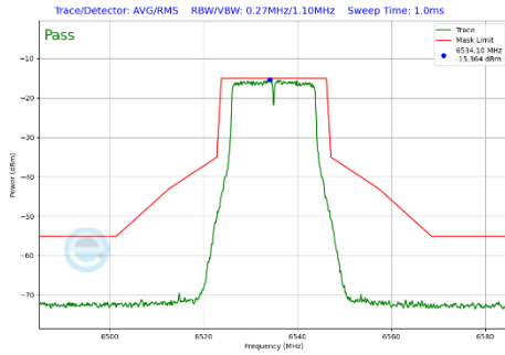
Plot 7-453 In-Band Emission Plot CDD Diversity Antenna WF7 (20MHz BW 802.11a (UNII Band 7) - Ch.117)
