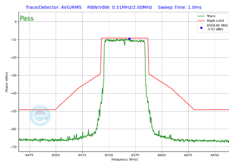
Plot 7-398 In-Band Emission Plot SDM Primary Antenna WF5B (40MHz BW 802.11be(SU) (UNII Band 7) - Ch.123)
