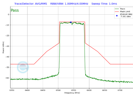
Plot 7-471 In-Band Emission Plot SDM Diversity Antenna WF8 (80MHz BW 802.11be(SU) (UNII Band 7) - Ch.119)
