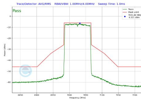
Plot 7-475 In-Band Emission Plot SDM Diversity Antenna WF8 (80MHz BW 802.11be(SU) (UNII Band 8) - Ch.215)
