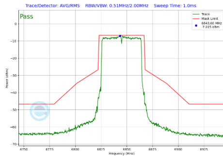
Plot 7-358 In-Band Emission Plot Antenna WF7 (40MHz BW 802.11be(SU) (UNII Band 7) - Ch.179)
