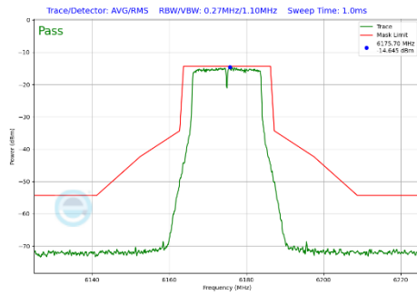
Plot 7-389 In-Band Emission Plot CDD Primary Antenna WF5B (20MHz BW 802.11a (UNII Band 5) - Ch.45)
