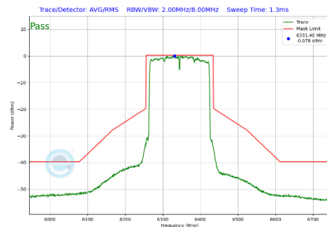
Plot 7-436 In-Band Emission Plot CDD Diversity Antenna WF8 (160MHz BW 802.11be(SU) (UNII Band 5) - Ch.79)
