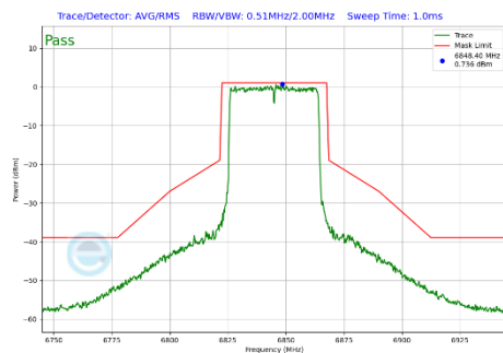
Plot 7-430 In-Band Emission Plot CDD Diversity Antenna WF7 (40MHz BW 802.11be(SU) (UNII Band 7) - Ch.179)
