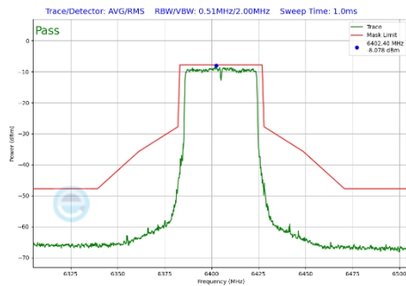
Plot 7-390 In-Band Emission Plot SDM Primary Antenna WF5B (40MHz BW 802.11be(SU) (UNII Band 5) - Ch.91)
