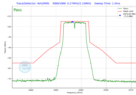
Plot 7-393 In-Band Emission Plot CDD Primary Antenna WF5B (20MHz BW 802.11a (UNII Band 6) - Ch.105)
