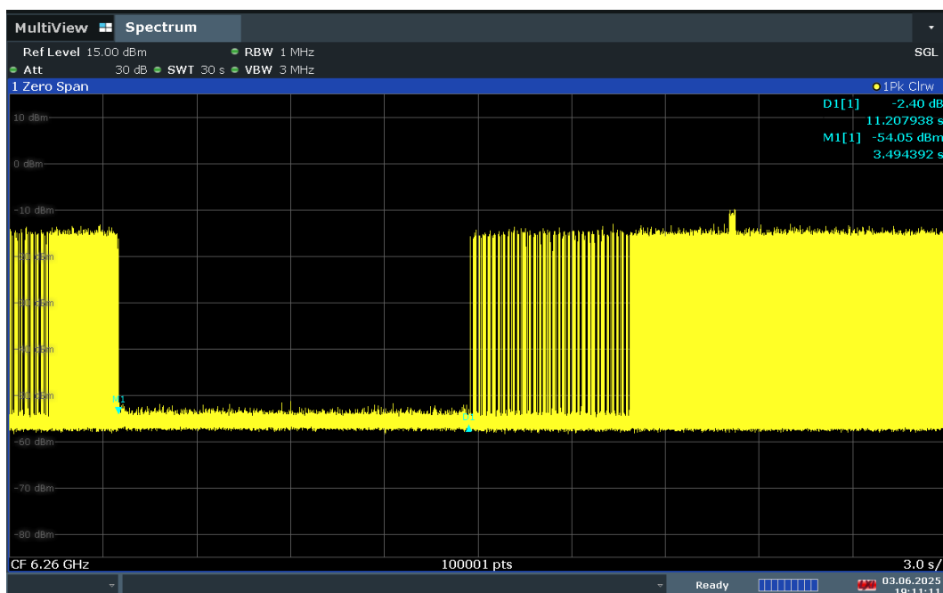
Plot 7-496. Contention Based Protocol Timing Plot – UNII 5 – 160MHz Channel 47 – High
