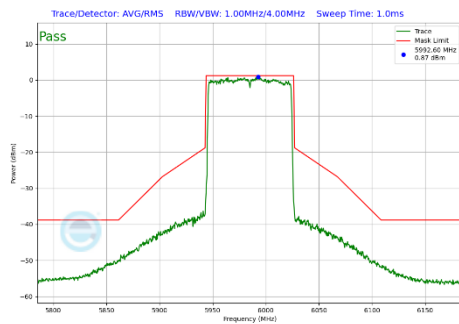
Plot 7-367 In-Band Emission Plot CDD Primary Antenna WF5B (80MHz BW 802.11be(SU) (UNII Band 5) - Ch.7)
