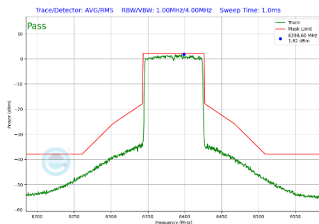
Plot 7-423 In-Band Emission Plot CDD Diversity Antenna WF7 (80MHz BW 802.11be(SU) (UNII Band 5) - Ch.87)
