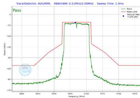
Plot 7-362 In-Band Emission Plot Antenna WF7 (40MHz BW 802.11be(SU) (UNII Band 8) - Ch.227)
