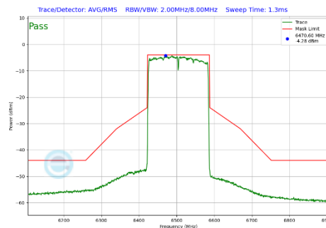
Plot 7-468 In-Band Emission Plot SDM Diversity Antenna WF8 (160MHz BW 802.11be(SU) (UNII Band 6) - Ch.111)
