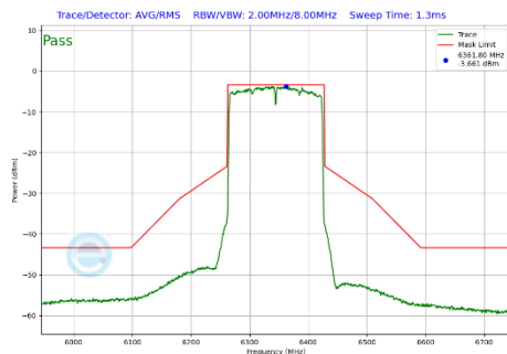
Plot 7-408 In-Band Emission Plot SDM Primary Antenna WF8 (160MHz BW 802.11be(SU) (UNII Band 5) - Ch.79)
