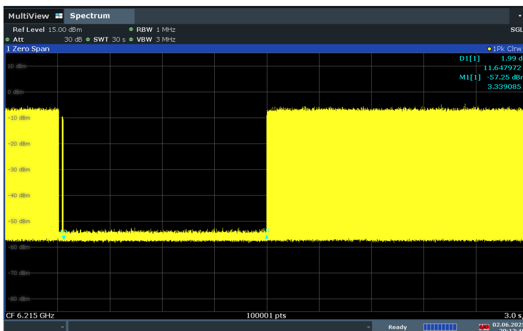
Plot 7-493. Contention Based Protocol Timing Plot – UNII 5 – 20MHz Channel 53
