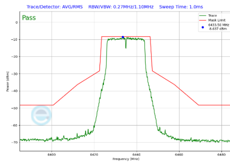
Plot 7-353 In-Band Emission Plot Antenna WF7 (20MHz BW 802.11a (UNII Band 6) - Ch.97)
