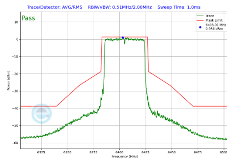
Plot 7-434 In-Band Emission Plot CDD Diversity Antenna WF8 (40MHz BW 802.11be(SU) (UNII Band 5) - Ch.91)
