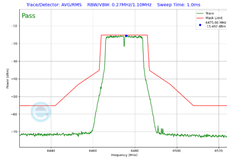
Plot 7-465 In-Band Emission Plot CDD Diversity Antenna WF8 (20MHz BW 802.11a (UNII Band 6) - Ch.105)
