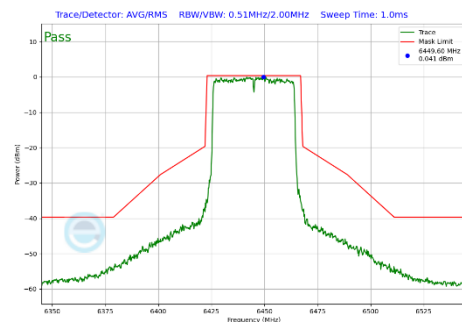
Plot 7-426 In-Band Emission Plot CDD Diversity Antenna WF7 (40MHz BW 802.11be(SU) (UNII Band 6) - Ch.99)
