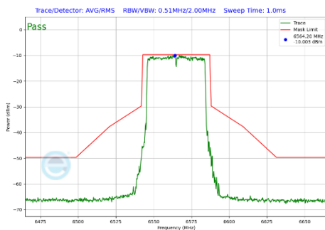
Plot 7-414 In-Band Emission Plot SDM Primary Antenna WF8 (40MHz BW 802.11be(SU) (UNII Band 7) - Ch.123)
