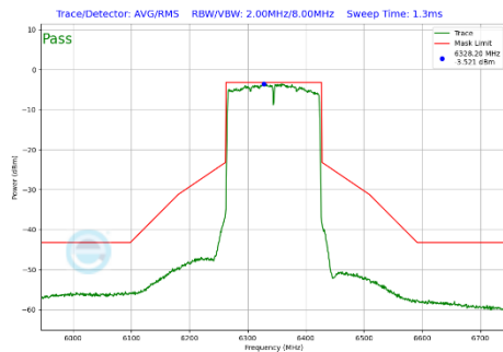
Plot 7-448 In-Band Emission Plot SDM Diversity Antenna WF7 (160MHz BW 802.11be(SU) (UNII Band 5) - Ch.79)
