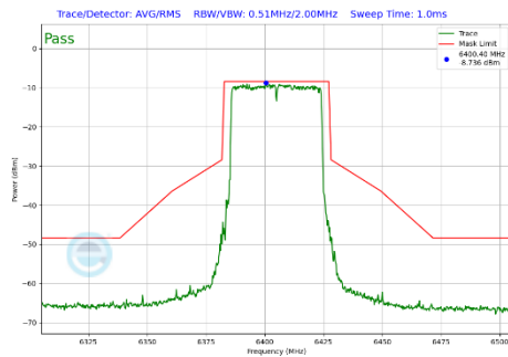
Plot 7-446 In-Band Emission Plot SDM Diversity Antenna WF7 (40MHz BW 802.11be(SU) (UNII Band 5) - Ch.91)
