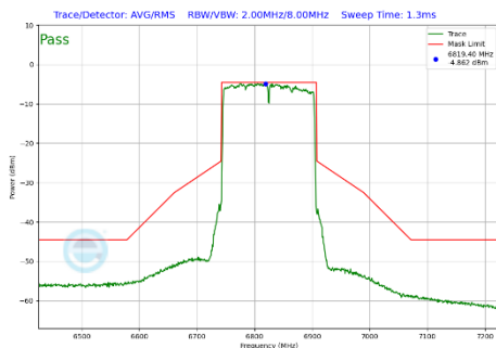
Plot 7-416 In-Band Emission Plot SDM Primary Antenna WF8 (160MHz BW 802.11be(SU) (UNII Band 7) - Ch.175)
