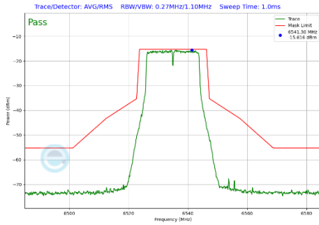
Plot 7-469 In-Band Emission Plot CDD Diversity Antenna WF8 (20MHz BW 802.11a (UNII Band 7) - Ch.117)
