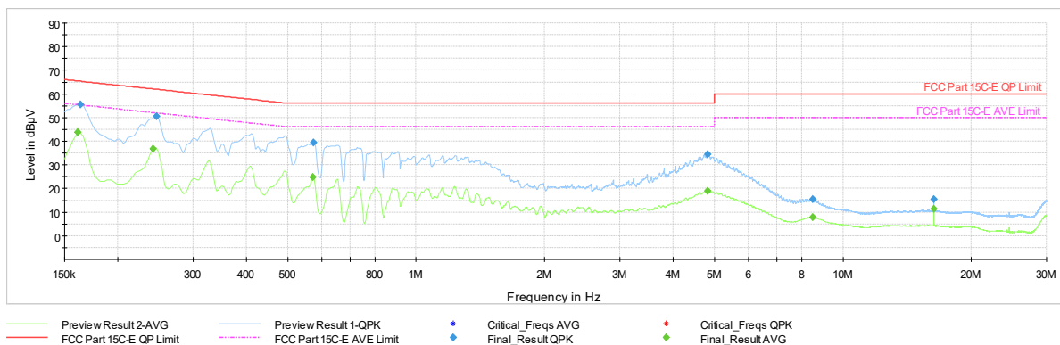
Plot 7-616. AC Line Conducted Plot with 802.11be CDD Primary – Ch.45 (L1), with AC/DC adapter
