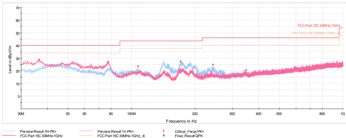
Plot 7-615. Radiated Spurious Emissions below 1GHz CDD Diversity, 802.11be, Ch.45 with AC/DC adapter
