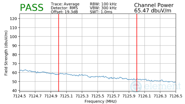
Plot 7-575 Antenna WF7 Radiated Upper Band Edge (Average – UNII Band 8)
