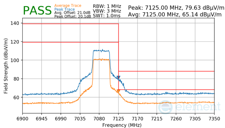
Plot 7-581 Antenna WF7 Radiated Upper Band Edge (Peak & Average – UNII Band 8)
