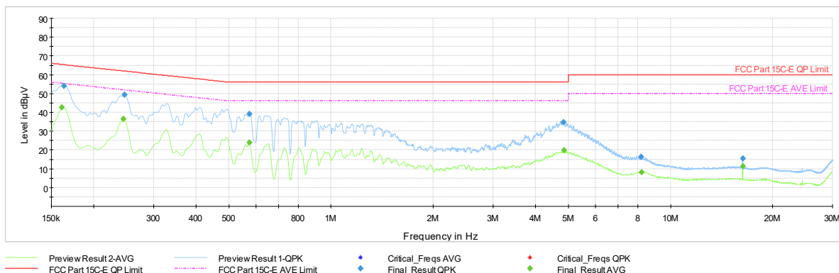
Plot 7-618. AC Line Conducted Plot with 802.11be CDD Diversity – Ch.45 (L1), with AC/DC adapter
