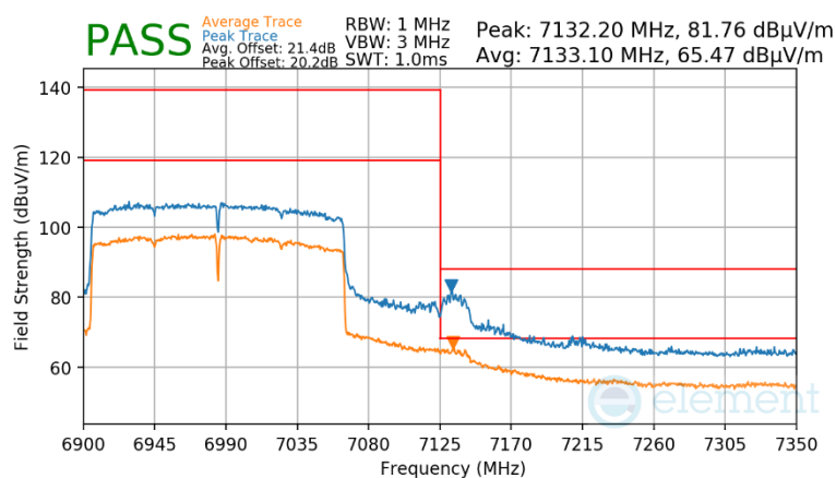
Plot 7-585 Antenna WF7 Radiated Upper Band Edge (Peak & Average – UNII Band 8)
