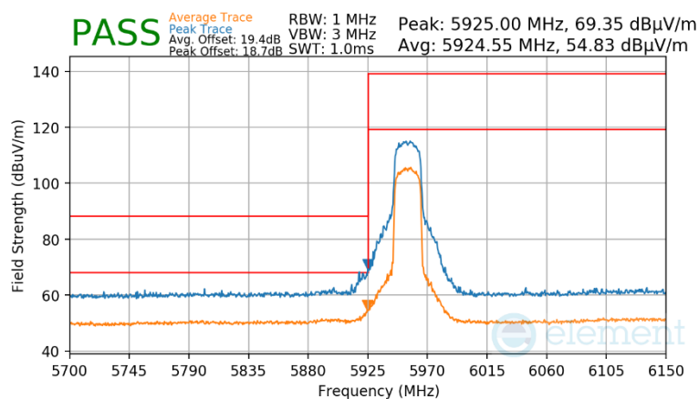
Plot 7-576 Antenna WF7 Radiated Lower Band Edge (Peak & Average – UNII Band 5)
