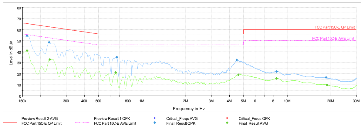
Plot 7-617. AC Line Conducted Plot with 802.11be CDD Primary – Ch. 45 (N), with AC/DC adapter
