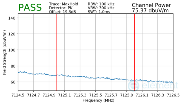
Plot 7-574 Antenna WF7 Radiated Upper Band Edge (Peak – UNII Band 8)
