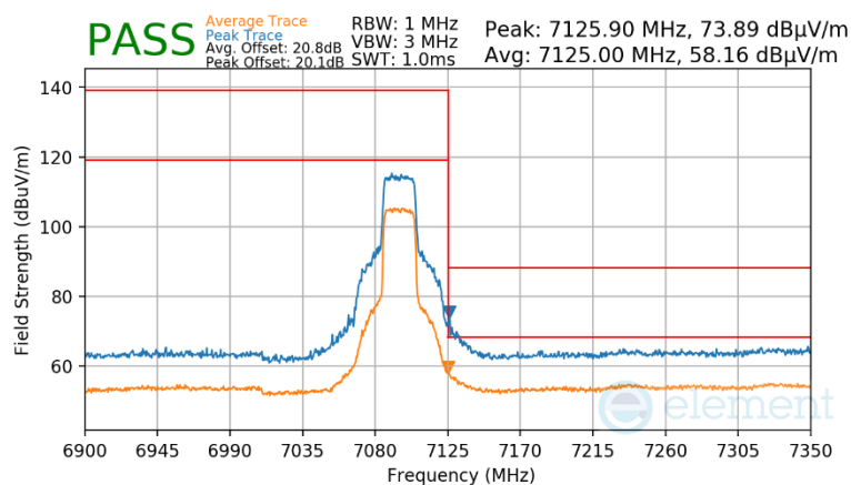
Plot 7-577 Antenna WF7 Radiated Upper Band Edge (Peak & Average – UNII Band 8)
