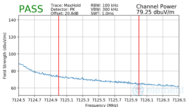
Plot 7-578 Antenna WF7 Radiated Upper Band Edge (Peak – UNII Band 8)
