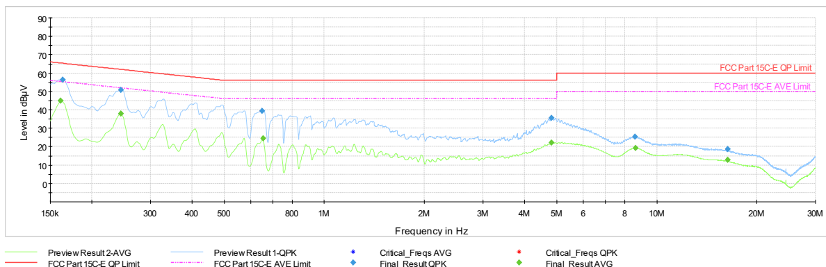
Plot 7-619. AC Line Conducted Plot with 802.11be CDD Diversity – Ch. 45 (N), with AC/DC adapter
