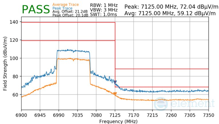
Plot 7-583 Antenna WF7 Radiated Upper Band Edge (Peak & Average – UNII Band 8)
