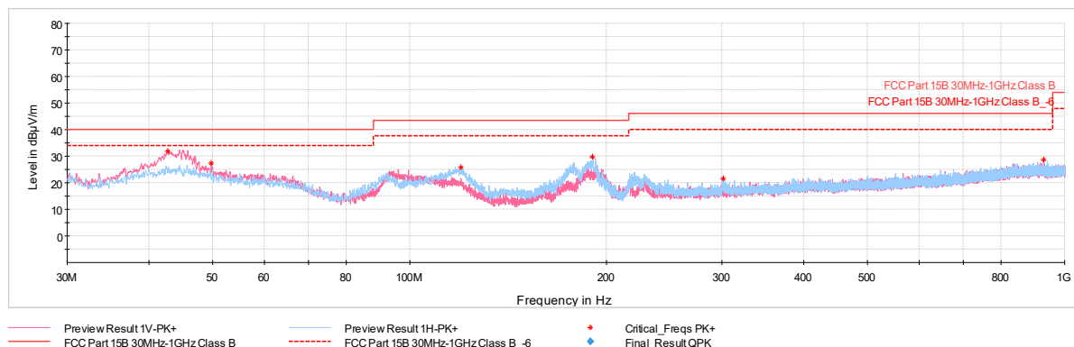
Plot 7-614. Radiated Spurious Emissions below 1GHz CDD Primary, 802.11be, Ch.45 with AC/DC adapter
