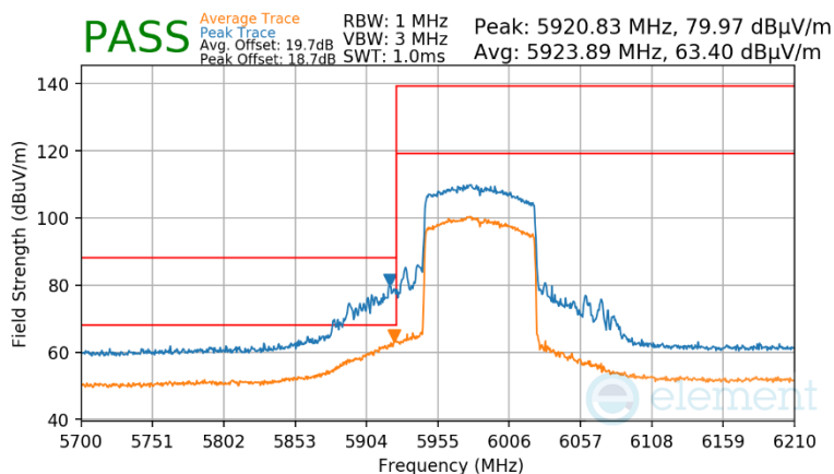
Plot 7-582 Antenna WF7 Radiated Lower Band Edge (Peak & Average – UNII Band 5)
