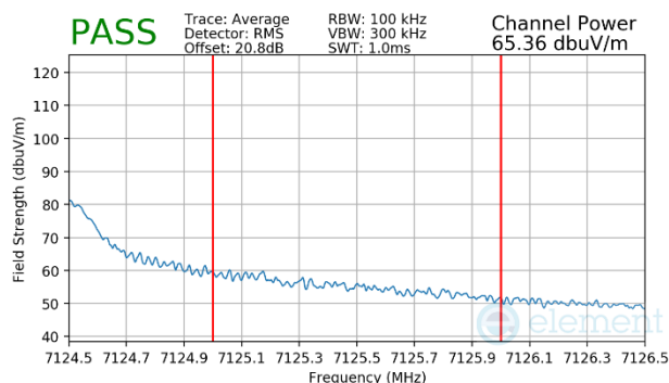
Plot 7-579 Antenna WF7 Radiated Upper Band Edge (Average – UNII Band 8)
