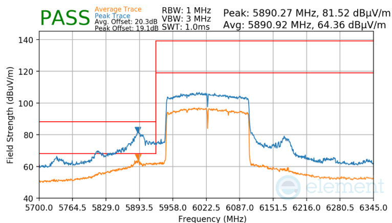
Plot 7-584 Antenna WF7 Radiated Lower Band Edge (Peak & Average – UNII Band 5)
