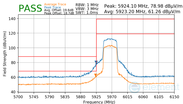
Plot 7-580 Antenna WF7 Radiated Lower Band Edge (Peak & Average – UNII Band 5)
