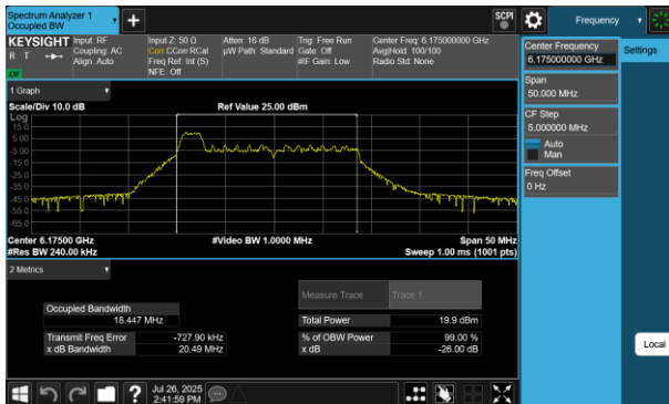
Plot 7-78 26dB BW & 99% OBW Antenna WF8 (20MHz BW 802.11be(RU) RU26 Index0 - Ch.45)
