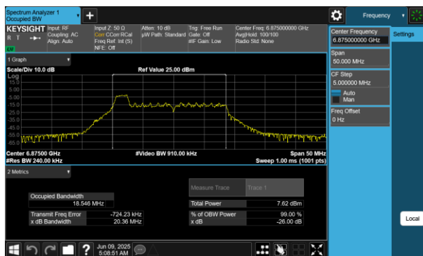
Plot 7-56 26dB BW & 99% OBW Antenna WF5B (20MHz BW 802.11be(RU) RU26 Index0 - Ch.185)
