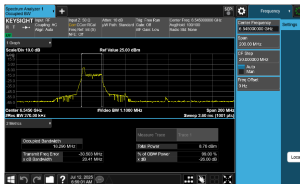
Plot 7-58 26dB BW & 99% OBW Antenna WF5B (80MHz BW 802.11be(RU) RU26 Index0 - Ch.119)
