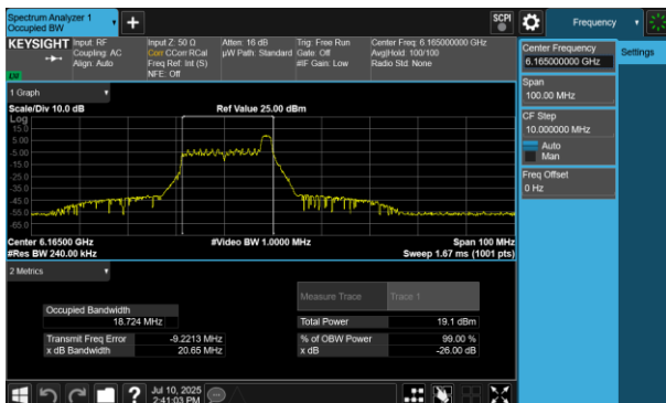
Plot 7-79 26dB BW & 99% OBW Antenna WF8 (40MHz BW 802.11be(RU) RU26 Index8 - Ch.43)
