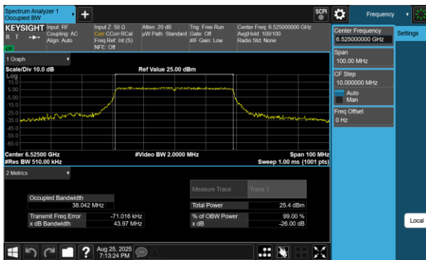
Plot 7-20 26dB BW & 99% OBW Antenna WF5B (40MHz BW 802.11be(RU) RU484 Index65 - Ch.115)
