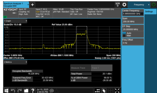
Plot 7-80 26dB BW & 99% OBW Antenna WF8 (80MHz BW 802.11be(RU) RU26 Index36 - Ch.7)
