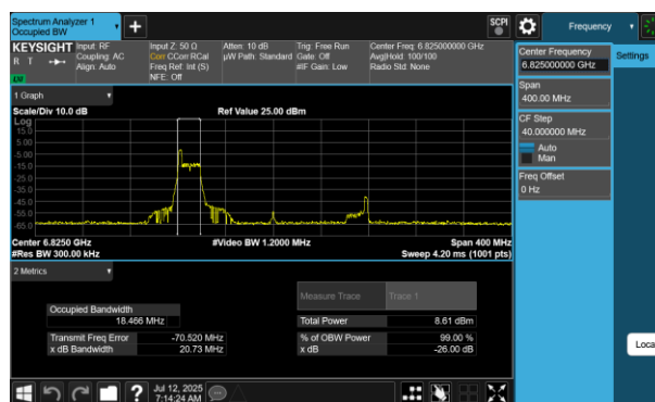
Plot 7-59 26dB BW & 99% OBW Antenna WF5B (160MHz BW 802.11be(RU) RU26 Index0 - Ch.175)
