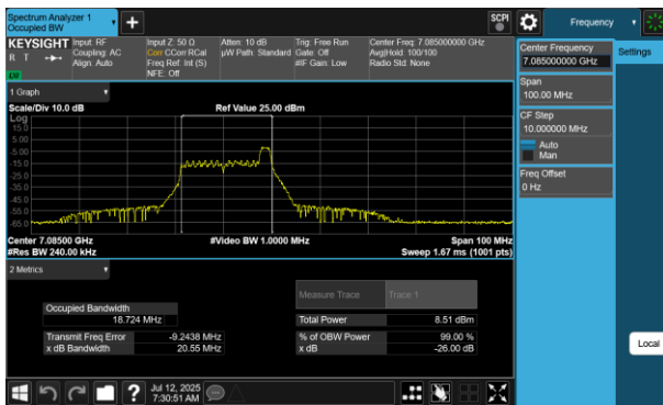
Plot 7-68 26dB BW & 99% OBW Antenna WF5B (40MHz BW 802.11be(RU) RU26 Index8 - Ch.227)
