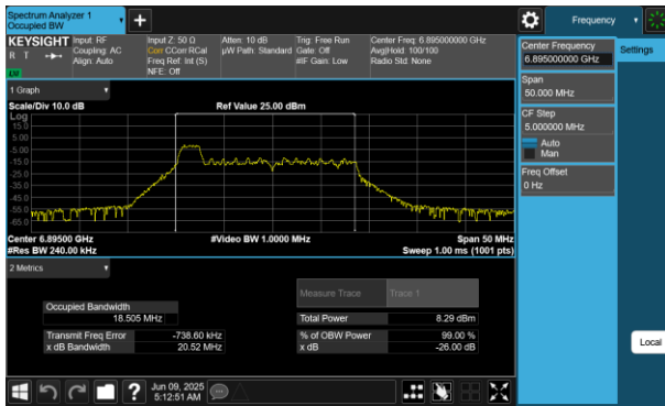
Plot 7-67 26dB BW & 99% OBW Antenna WF5B (20MHz BW 802.11be(RU) RU26 Index0 - Ch.189)
