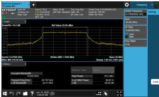
Plot 7-19 26dB BW & 99% OBW Antenna WF5B (20MHz BW 802.11be(RU) RU242 Index61 - Ch.105)
