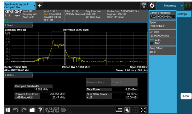
Plot 7-69 26dB BW & 99% OBW Antenna WF5B (80MHz BW 802.11be(RU) RU26 Index0 - Ch.215)
