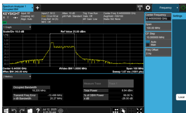
Plot 7-46 26dB BW & 99% OBW Antenna WF5B (40MHz BW 802.11be(RU) RU26 Index0 - Ch.99)
