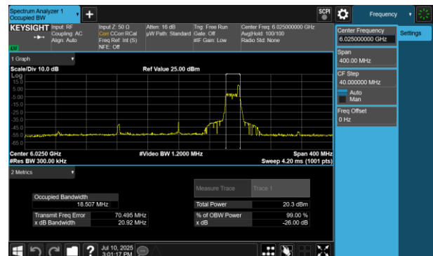
Plot 7-81 26dB BW & 99% OBW Antenna WF8 (160MHz BW 802.11be(RU) RU26 Index36 - Ch.15)
