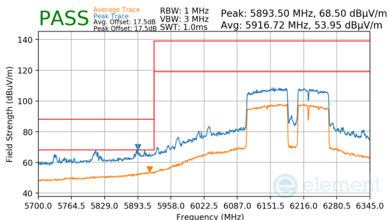
Plot 7-892 Antenna WF5B Radiated Lower Band Edge (Peak & Average – UNII Band 5) - RU996+484+242 (H)
