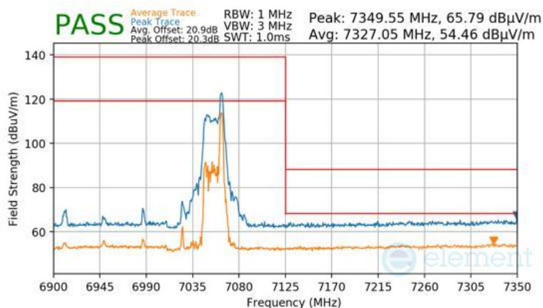
Plot 7-869 Antenna WF5B Radiated Upper Band Edge (Peak & Average – UNII Band 8) - RU26
