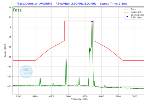
Plot 7-936 In-Band Emission Plot Antenna WF7 (160MHz BW 802.11be(RU) RU26 Index36 (UNII Band 7) - Ch.143)
