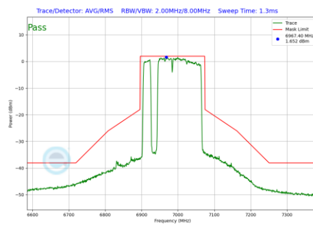
Plot 7-908 In-Band Emission Plot Antenna WF8 (160MHz BW 802.11be(RU) RU996+484+242 Index97 (UNII Band 8) - Ch.207)
