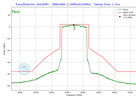
Plot 7-949 In-Band Emission Plot Antenna WF7 (160MHz BW 802.11be(RU) RU996X2 Index68 (UNII Band 5) - Ch.79)
