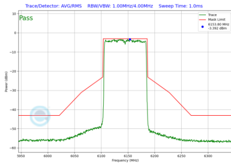
Plot 7-911 In-Band Emission Plot Antenna WF8 (80MHz BW 802.11be(RU) RU996 Index67 (UNII Band 5) - Ch.39)
