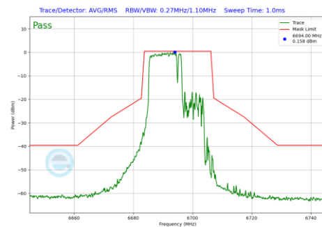
Plot 7-943 In-Band Emission Plot Antenna WF7 (20MHz BW 802.11be(RU) RU106+26 Index82 (UNII Band 7) - Ch.149)
