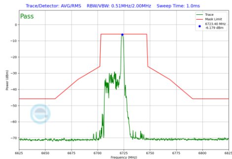
Plot 7-967 In-Band Emission Plot Antenna WF7 (40MHz BW 802.11be(RU) RU26 Index8 (UNII Band 7) - Ch.155)
