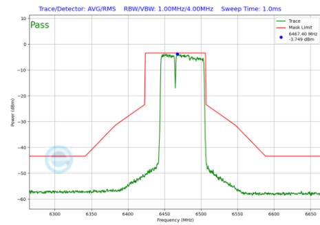
Plot 7-978 In-Band Emission Plot Antenna WF7 (80MHz BW 802.11be(RU) RU484+242 Index90 (UNII Band 6) - Ch.103)
