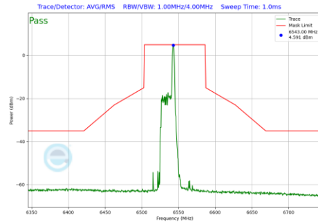
Plot 7-935 In-Band Emission Plot Antenna WF7 (80MHz BW 802.11be(RU) RU26 Index17 (UNII Band 7) - Ch.119)
