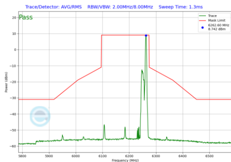
Plot 7-851 In-Band Emission Plot Antenna WF8 (160MHz BW 802.11be(RU) RU26 Index36 (UNII Band 5) - Ch.47)
