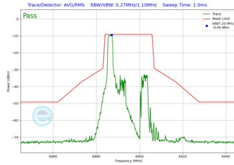
Plot 7-970 In-Band Emission Plot Antenna WF7 (20MHz BW 802.11be(RU) RU26 Index0 (UNII Band 8) - Ch.189)
