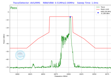
Plot 7-971 In-Band Emission Plot Antenna WF7 (40MHz BW 802.11be(RU) RU26 Index17 (UNII Band 8) - Ch.187)
