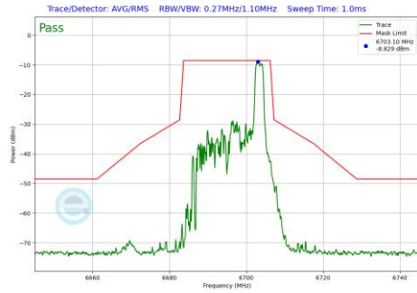
Plot 7-966 In-Band Emission Plot Antenna WF7 (20MHz BW 802.11be(RU) RU26 Index8 (UNII Band 7) - Ch.149)
