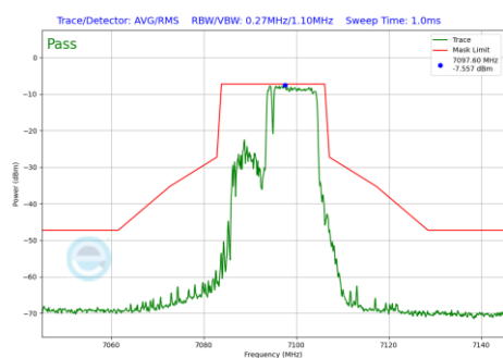
Plot 7-906 In-Band Emission Plot Antenna WF8 (20MHz BW 802.11be(RU) RU106+26 Index83 (UNII Band 8) - Ch.229)
