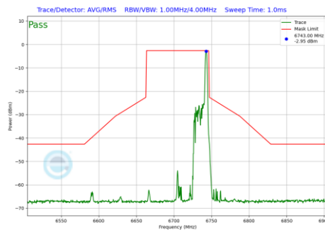
Plot 7-891 In-Band Emission Plot Antenna WF8 (80MHz BW 802.11be(RU) RU26 Index36 (UNII Band 7) - Ch.151)
