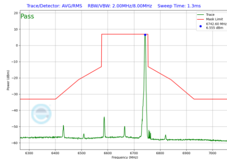
Plot 7-859 In-Band Emission Plot Antenna WF8 (160MHz BW 802.11be(RU) RU26 Index36 (UNII Band 7) - Ch.143)
