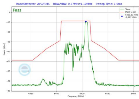
Plot 7-958 In-Band Emission Plot Antenna WF7 (20MHz BW 802.11be(RU) RU26 Index8 (UNII Band 5) - Ch.93)
