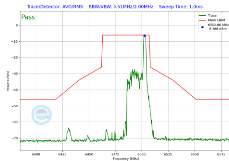
Plot 7-963 In-Band Emission Plot Antenna WF7 (40MHz BW 802.11be(RU) RU26 Index17 (UNII Band 6) - Ch.107)
