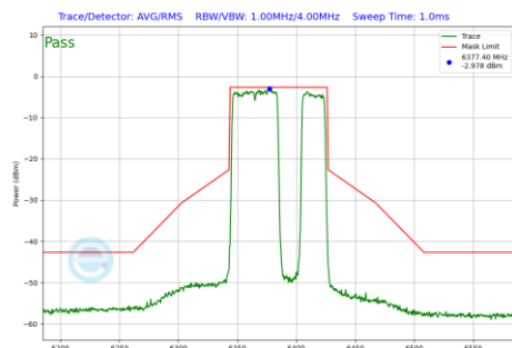
Plot 7-975 In-Band Emission Plot Antenna WF7 (80MHz BW 802.11be(RU) RU484+242 Index92 (UNII Band 5) - Ch.87)
