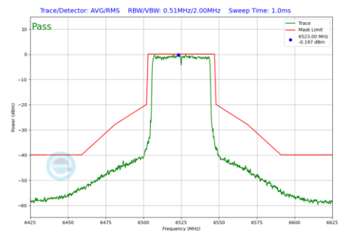
Plot 7-951 In-Band Emission Plot Antenna WF7 (40MHz BW 802.11be(RU) RU484 Index65 (UNII Band 6) - Ch.115)
