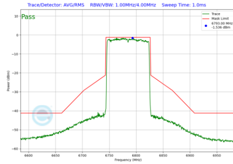
Plot 7-956 In-Band Emission Plot Antenna WF7 (80MHz BW 802.11be(RU) RU996 Index67 (UNII Band 7) - Ch.167)
