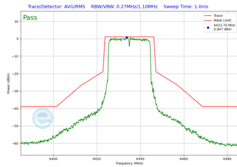
Plot 7-873 In-Band Emission Plot Antenna WF8 (20MHz BW 802.11be(RU) RU242 Index61 (UNII Band 6) - Ch.97)
