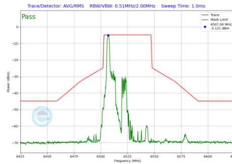
Plot 7-886 In-Band Emission Plot Antenna WF8 (40MHz BW 802.11be(RU) RU26 Index0 (UNII Band 6) - Ch.115)
