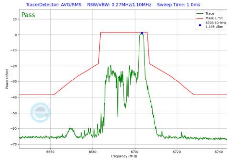
Plot 7-856 In-Band Emission Plot Antenna WF8 (20MHz BW 802.11be(RU) RU26 Index8 (UNII Band 7) - Ch.149)
