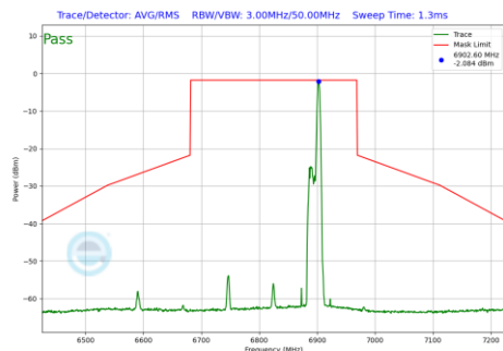
Plot 7-969 In-Band Emission Plot Antenna WF7 (160MHz BW 802.11be(RU) RU26 Index36 (UNII Band 7) - Ch.175)
