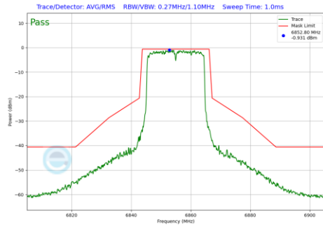
Plot 7-954 In-Band Emission Plot Antenna WF7 (20MHz BW 802.11be(RU) RU242 Index61 (UNII Band 7) - Ch.181)
