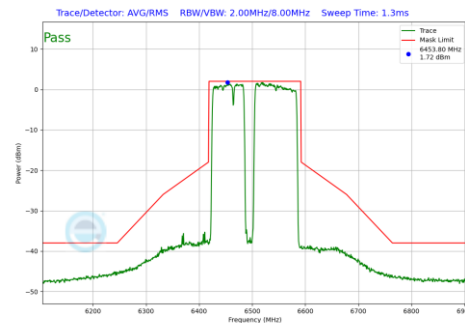
Plot 7-865 In-Band Emission Plot Antenna WF8 (160MHz BW 802.11be(RU) RU996+484+242 Index99 (UNII Band 6) - Ch.111)
