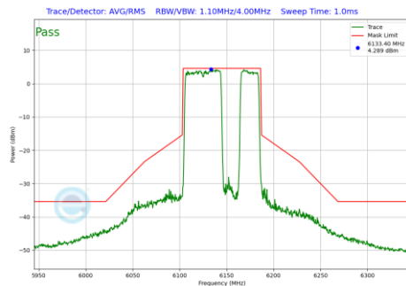
Plot 7-861 In-Band Emission Plot Antenna WF8 (80MHz BW 802.11be(RU) RU484+242 Index92 (UNII Band 5) - Ch.39)
