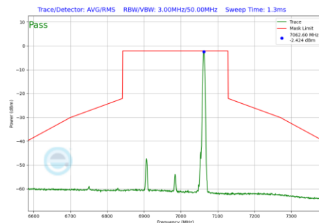
Plot 7-973 In-Band Emission Plot Antenna WF7 (160MHz BW 802.11be(RU) RU26 Index36 (UNII Band 8) - Ch.207)
