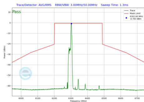
Plot 7-961 In-Band Emission Plot Antenna WF7 (160MHz BW 802.11be(RU) RU26 Index17 (UNII Band 5) - Ch.79)
