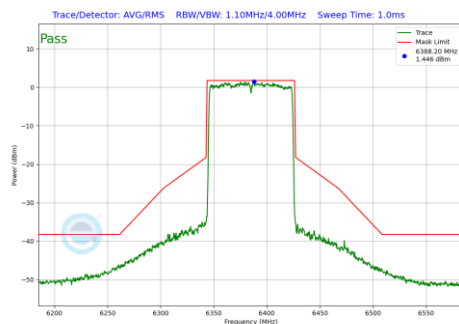
Plot 7-948 In-Band Emission Plot Antenna WF7 (80MHz BW 802.11be(RU) RU996 Index67 (UNII Band 5) - Ch.87)
