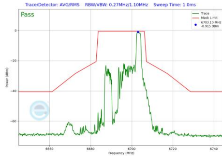
Plot 7-933 In-Band Emission Plot Antenna WF7 (20MHz BW 802.11be(RU) RU26 Index8 (UNII Band 7) - Ch.149)
