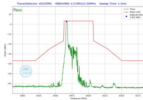
Plot 7-853 In-Band Emission Plot Antenna WF8 (40MHz BW 802.11be(RU) RU26 Index0 (UNII Band 6) - Ch.107)
