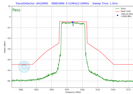
Plot 7-922 In-Band Emission Plot Antenna WF8 (40MHz BW 802.11be(RU) RU484 Index65 (UNII Band 8) - Ch.227)
