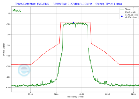
Plot 7-909 In-Band Emission Plot Antenna WF8 (20MHz BW 802.11be(RU) RU242 Index61 (UNII Band 5) - Ch.45)
