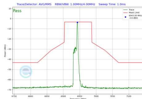
Plot 7-972 In-Band Emission Plot Antenna WF7 (80MHz BW 802.11be(RU) RU26 Index17 (UNII Band 8) - Ch.199)
