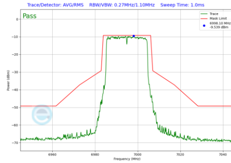
Plot 7-844 In-Band Emission Plot Antenna WF5B (20MHz BW 802.11be(RU) RU242 Index61 (UNII Band 8) - Ch.209)
