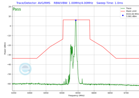
Plot 7-858 In-Band Emission Plot Antenna WF8 (80MHz BW 802.11be(RU) RU26 Index17 (UNII Band 7) - Ch.119)
