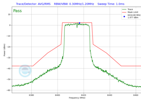
Plot 7-946 In-Band Emission Plot Antenna WF7 (20MHz BW 802.11be(RU) RU242 Index61 (UNII Band 5) - Ch.93)
