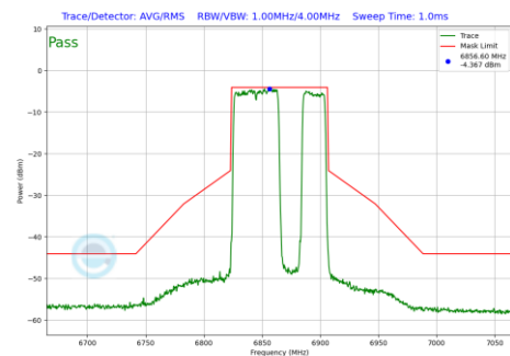
Plot 7-981 In-Band Emission Plot Antenna WF7 (80MHz BW 802.11be(RU) RU484+242 Index92 (UNII Band 7) - Ch.183)
