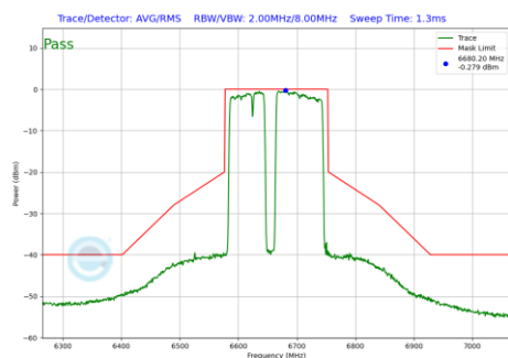
Plot 7-945 In-Band Emission Plot Antenna WF7 (160MHz BW 802.11be(RU) RU996+484+242 Index99 (UNII Band 7) - Ch.143)
