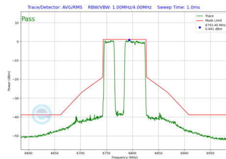
Plot 7-944 In-Band Emission Plot Antenna WF7 (80MHz BW 802.11be(RU) RU484+242 Index91 (UNII Band 7) - Ch.167)
