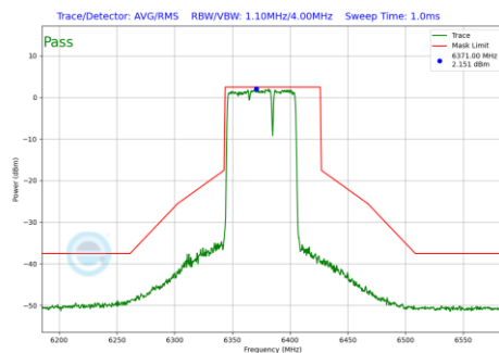
Plot 7-938 In-Band Emission Plot Antenna WF7 (80MHz BW 802.11be(RU) RU484+242 Index93 (UNII Band 5) - Ch.87)
