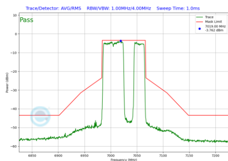
Plot 7-983 In-Band Emission Plot Antenna WF7 (80MHz BW 802.11be(RU) RU484+242 Index92 (UNII Band 8) - Ch.215)
