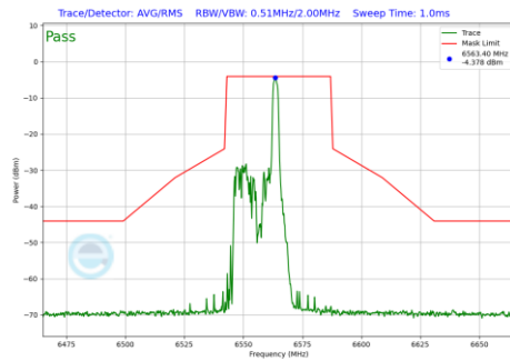
Plot 7-890 In-Band Emission Plot Antenna WF8 (40MHz BW 802.11be(RU) RU26 Index8 (UNII Band 7) - Ch.123)
