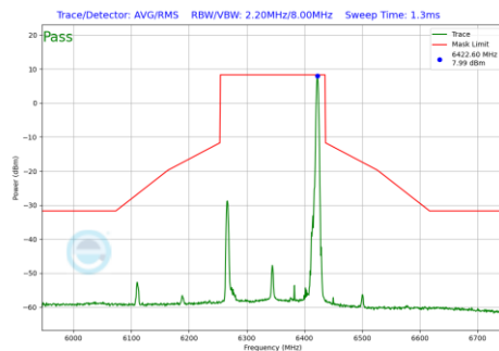
Plot 7-928 In-Band Emission Plot Antenna WF7 (160MHz BW 802.11be(RU) RU26 Index36 (UNII Band 5) - Ch.79)
