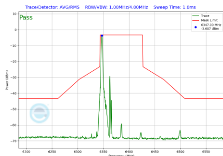
Plot 7-960 In-Band Emission Plot Antenna WF7 (80MHz BW 802.11be(RU) RU26 Index0 (UNII Band 5) - Ch.87)
