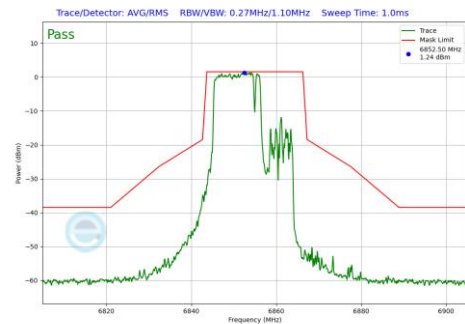
Plot 7-866 In-Band Emission Plot Antenna WF8 (20MHz BW 802.11be(RU) RU106+26 Index82 (UNII Band 7) - Ch.181)
