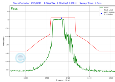
Plot 7-937 In-Band Emission Plot Antenna WF7 (20MHz BW 802.11be(RU) RU106+26 Index82 (UNII Band 5) - Ch.93)
