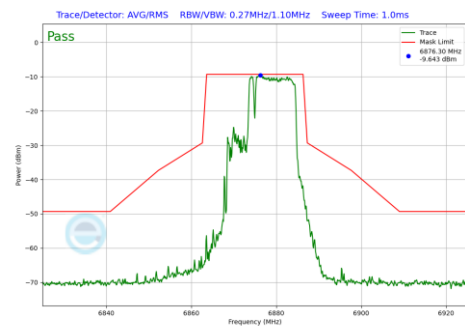
Plot 7-980 In-Band Emission Plot Antenna WF7 (20MHz BW 802.11be(RU) RU106+26 Index83 (UNII Band 7) - Ch.185)
