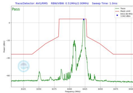
Plot 7-926 In-Band Emission Plot Antenna WF7 (40MHz BW 802.11be(RU) RU26 Index17 (UNII Band 5) - Ch.91)
