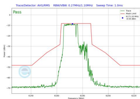
Plot 7-897 In-Band Emission Plot Antenna WF8 (20MHz BW 802.11be(RU) RU106+26 Index82 (UNII Band 5) - Ch.45)
