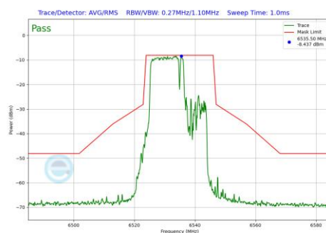
Plot 7-903 In-Band Emission Plot Antenna WF8 (20MHz BW 802.11be(RU) RU106+26 Index82 (UNII Band 7) - Ch.117)
