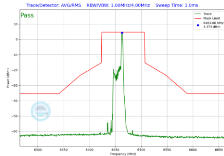
Plot 7-931 In-Band Emission Plot Antenna WF7 (80MHz BW 802.11be(RU) RU26 Index17 (UNII Band 6) - Ch.103)
