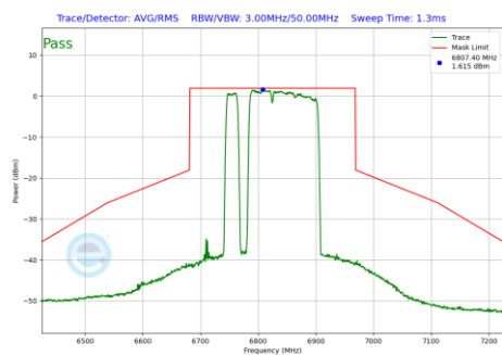
Plot 7-905 In-Band Emission Plot Antenna WF8 (160MHz BW 802.11be(RU) RU996+484+242 Index97 (UNII Band 7) - Ch.175)
