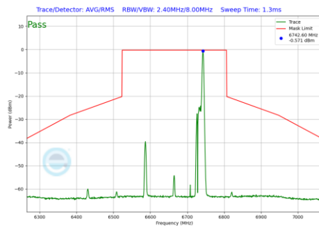
Plot 7-892 In-Band Emission Plot Antenna WF8 (160MHz BW 802.11be(RU) RU26 Index36 (UNII Band 7) - Ch.143)
