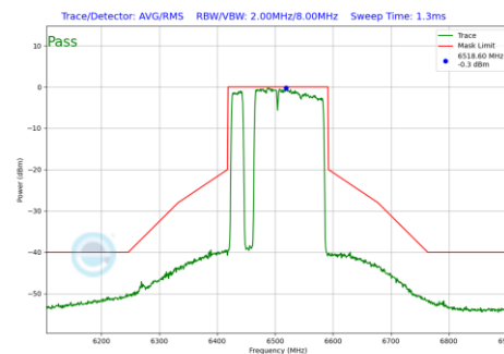
Plot 7-942 In-Band Emission Plot Antenna WF7 (160MHz BW 802.11be(RU) RU996+484+242 Index97 (UNII Band 6) - Ch.111)
