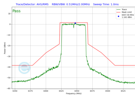
Plot 7-874 In-Band Emission Plot Antenna WF8 (40MHz BW 802.11be(RU) RU484 Index65 (UNII Band 6) - Ch.99)
