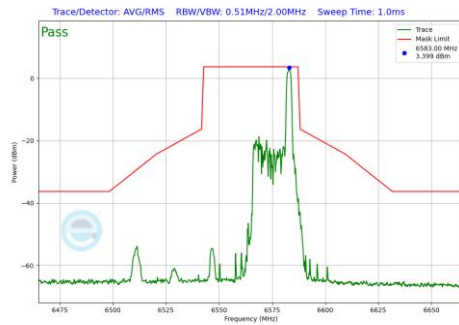
Plot 7-934 In-Band Emission Plot Antenna WF7 (40MHz BW 802.11be(RU) RU26 Index17 (UNII Band 7) - Ch.123)
