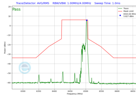
Plot 7-854 In-Band Emission Plot Antenna WF8 (80MHz BW 802.11be(RU) RU26 Index36 (UNII Band 6) - Ch.103)
