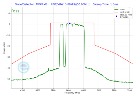
Plot 7-828 In-Band Emission Plot Antenna WF5B (160MHz BW 802.11be(RU) RU996+484+242 Index97 (UNII Band 7) - Ch.175)
