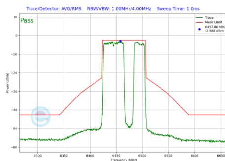
Plot 7-901 In-Band Emission Plot Antenna WF8 (80MHz BW 802.11be(RU) RU484+242 Index92 (UNII Band 6) - Ch.103)
