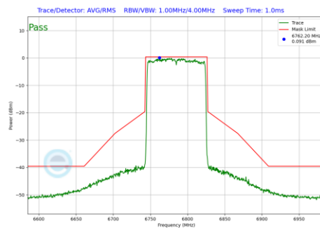
Plot 7-879 In-Band Emission Plot Antenna WF8 (80MHz BW 802.11be(RU) RU996 Index67 (UNII Band 7) - Ch.167)
