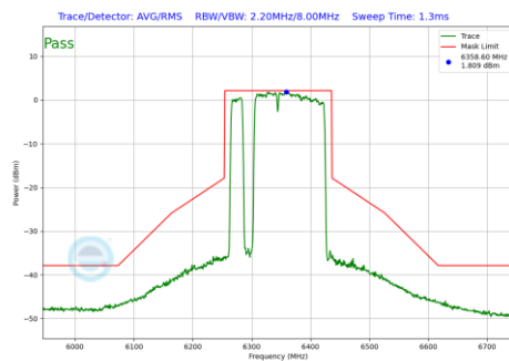
Plot 7-939 In-Band Emission Plot Antenna WF7 (160MHz BW 802.11be(RU) RU996+484+242 Index97 (UNII Band 5) - Ch.79)
