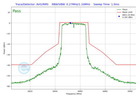
Plot 7-877 In-Band Emission Plot Antenna WF8 (20MHz BW 802.11be(RU) RU242 Index61 (UNII Band 7) - Ch.181)
