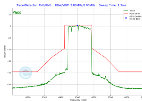
Plot 7-902 In-Band Emission Plot Antenna WF8 (160MHz BW 802.11be(RU) RU996+484+242 Index96 (UNII Band 6) - Ch.111)
