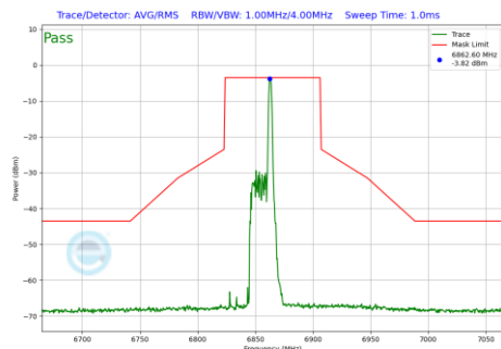
Plot 7-968 In-Band Emission Plot Antenna WF7 (80MHz BW 802.11be(RU) RU26 Index17 (UNII Band 7) - Ch.183)
