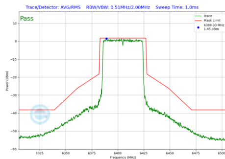
Plot 7-947 In-Band Emission Plot Antenna WF7 (40MHz BW 802.11be(RU) RU484 Index65 (UNII Band 5) - Ch.91)
