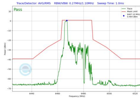
Plot 7-852 In-Band Emission Plot Antenna WF8 (20MHz BW 802.11be(RU) RU26 Index0 (UNII Band 6) - Ch.105)
