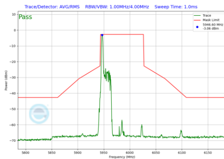
Plot 7-883 In-Band Emission Plot Antenna WF8 (80MHz BW 802.11be(RU) RU26 Index0 (UNII Band 5) - Ch.7)
