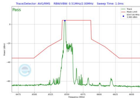
Plot 7-857 In-Band Emission Plot Antenna WF8 (40MHz BW 802.11be(RU) RU26 Index0 (UNII Band 7) - Ch.123)
