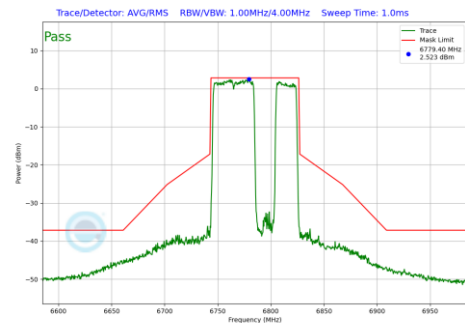
Plot 7-867 In-Band Emission Plot Antenna WF8 (80MHz BW 802.11be(RU) RU484+242 Index92 (UNII Band 7) - Ch.167)
