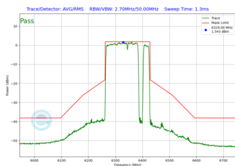
Plot 7-899 In-Band Emission Plot Antenna WF8 (160MHz BW 802.11be(RU) RU996+484+242 Index98 (UNII Band 5) - Ch.79)
