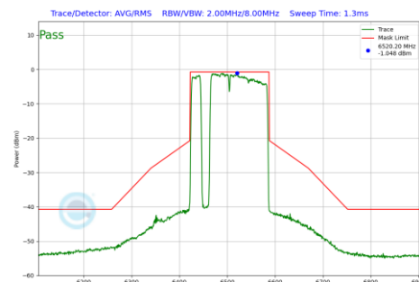
Plot 7-979 In-Band Emission Plot Antenna WF7 (160MHz BW 802.11be(RU) RU996+484+242 Index97 (UNII Band 6) - Ch.111)
