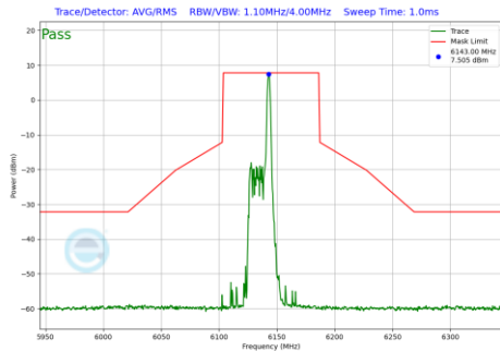
Plot 7-850 In-Band Emission Plot Antenna WF8 (80MHz BW 802.11be(RU) RU26 Index17 (UNII Band 5) - Ch.39)
