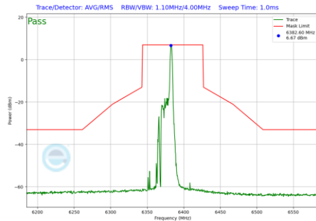
Plot 7-927 In-Band Emission Plot Antenna WF7 (80MHz BW 802.11be(RU) RU26 Index17 (UNII Band 5) - Ch.87)
