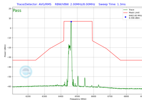
Plot 7-932 In-Band Emission Plot Antenna WF7 (160MHz BW 802.11be(RU) RU26 Index17 (UNII Band 6) - Ch.111)
