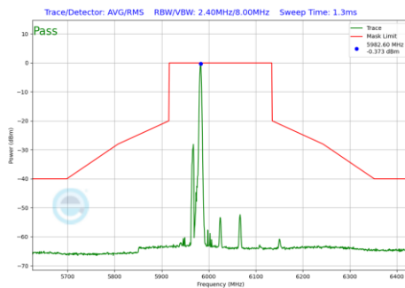
Plot 7-884 In-Band Emission Plot Antenna WF8 (160MHz BW 802.11be(RU) RU26 Index17 (UNII Band 5) - Ch.15)
