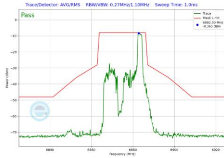
Plot 7-889 In-Band Emission Plot Antenna WF8 (20MHz BW 802.11be(RU) RU26 Index8 (UNII Band 7) - Ch.185)
