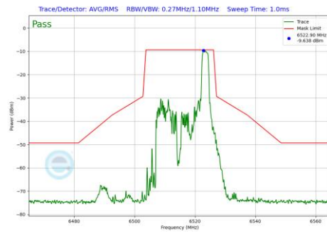
Plot 7-962 In-Band Emission Plot Antenna WF7 (20MHz BW 802.11be(RU) RU26 Index8 (UNII Band 6) - Ch.113)
