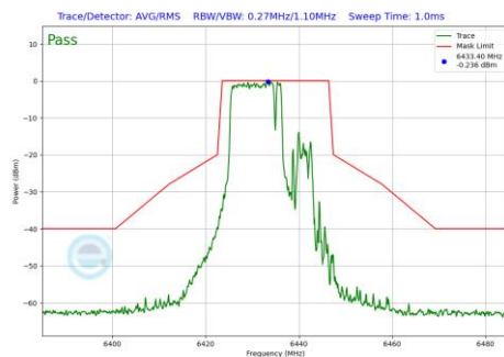
Plot 7-940 In-Band Emission Plot Antenna WF7 (20MHz BW 802.11be(RU) RU106+26 Index82 (UNII Band 6) - Ch.97)
