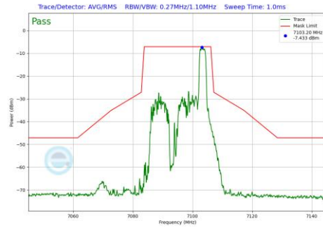
Plot 7-893 In-Band Emission Plot Antenna WF8 (20MHz BW 802.11be(RU) RU26 Index8 (UNII Band 8) - Ch.229)
