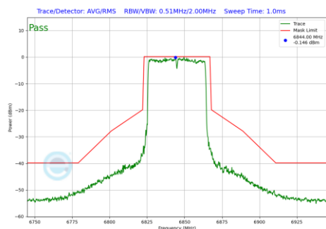
Plot 7-878 In-Band Emission Plot Antenna WF8 (40MHz BW 802.11be(RU) RU484 Index65 (UNII Band 7) - Ch.179)
