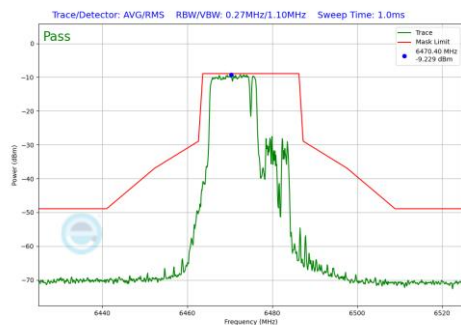
Plot 7-977 In-Band Emission Plot Antenna WF7 (20MHz BW 802.11be(RU) RU106+26 Index82 (UNII Band 6) - Ch.105)
