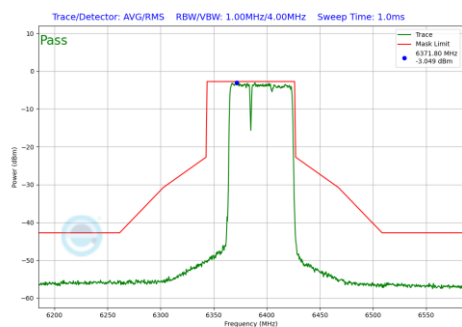
Plot 7-898 In-Band Emission Plot Antenna WF8 (80MHz BW 802.11be(RU) RU484+242 Index90 (UNII Band 5) - Ch.87)
