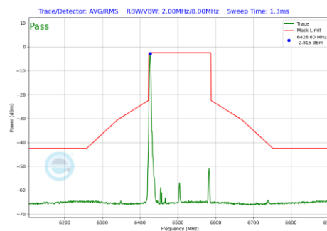
Plot 7-965 In-Band Emission Plot Antenna WF7 (160MHz BW 802.11be(RU) RU26 Index0 (UNII Band 6) - Ch.111)
