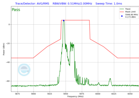
Plot 7-849 In-Band Emission Plot Antenna WF8 (40MHz BW 802.11be(RU) RU26 Index0 (UNII Band 5) - Ch.3)
