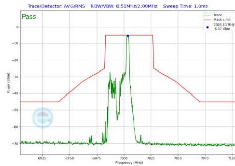
Plot 7-894 In-Band Emission Plot Antenna WF8 (40MHz BW 802.11be(RU) RU26 Index8 (UNII Band 8) - Ch.211)
