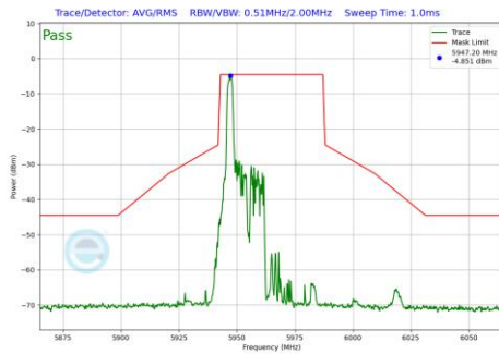
Plot 7-882 In-Band Emission Plot Antenna WF8 (40MHz BW 802.11be(RU) RU26 Index0 (UNII Band 5) - Ch.3)
