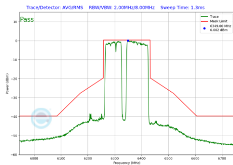
Plot 7-976 In-Band Emission Plot Antenna WF7 (160MHz BW 802.11be(RU) RU996+484+242 Index99 (UNII Band 5) - Ch.79)
