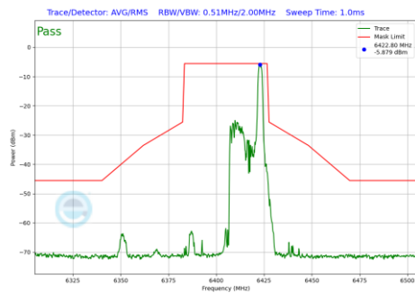
Plot 7-959 In-Band Emission Plot Antenna WF7 (40MHz BW 802.11be(RU) RU26 Index17 (UNII Band 5) - Ch.91)
