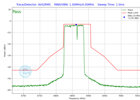
Plot 7-904 In-Band Emission Plot Antenna WF8 (80MHz BW 802.11be(RU) RU484+242 Index93 (UNII Band 7) - Ch.183)
