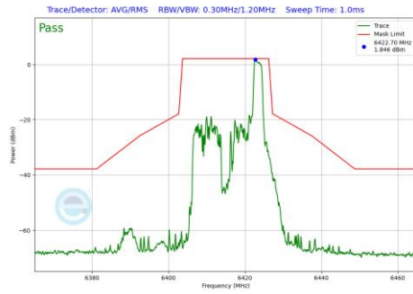
Plot 7-925 In-Band Emission Plot Antenna WF7 (20MHz BW 802.11be(RU) RU26 Index8 (UNII Band 5) - Ch.93)
