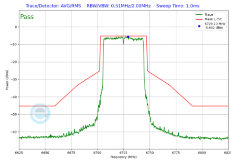
Plot 7-918 In-Band Emission Plot Antenna WF8 (40MHz BW 802.11be(RU) RU484 Index65 (UNII Band 7) - Ch.155)
