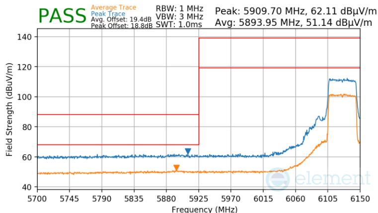
Plot 7-988 Antenna WF7 Radiated Lower Band Edge (Peak & Average – UNII Band 5) - RU484
