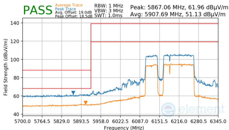
Plot 7-958 Antenna WF8 Radiated Lower Band Edge (Peak & Average – UNII Band 5) - RU996+484+242 (L)
