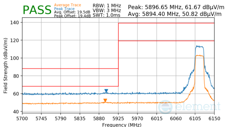
Plot 7-918 Antenna WF8 Radiated Lower Band Edge (Peak & Average – UNII Band 5) - RU242
