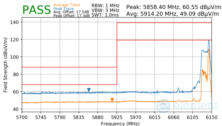
Plot 7-923 Antenna WF8 Radiated Lower Band Edge (Peak & Average – UNII Band 5) - RU26
