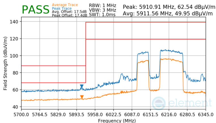
Plot 7-949 Antenna WF8 Radiated Lower Band Edge (Peak & Average – UNII Band 5) - RU996+484 (L)
