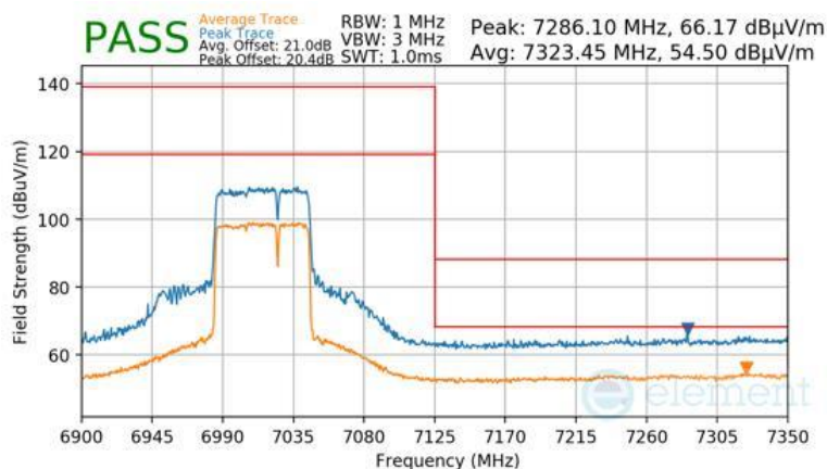
Plot 7-939 Antenna WF8 Radiated Upper Band Edge (Peak & Average – UNII Band 8) - RU484+242
