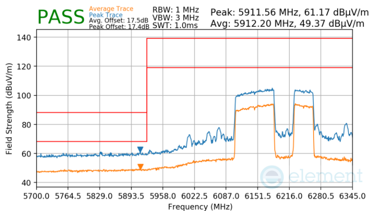
Plot 7-947 Antenna WF8 Radiated Lower Band Edge (Peak & Average – UNII Band 5) - RU996+484 (H)
