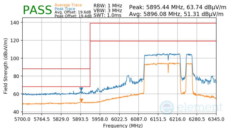
Plot 7-959 Antenna WF8 Radiated Lower Band Edge (Peak & Average – UNII Band 5) - RU996+484+242 (H)
