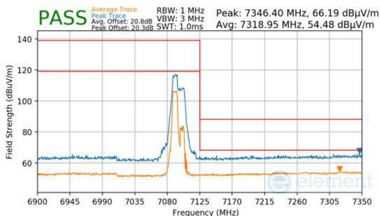
Plot 7-916 Antenna WF8 Radiated Upper Band Edge (Peak & Average – UNII Band 8) - RU52+26
