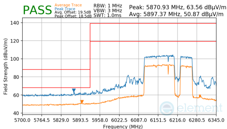
Plot 7-957 Antenna WF8 Radiated Lower Band Edge (Peak & Average – UNII Band 5) - RU996+484+242 (H)
