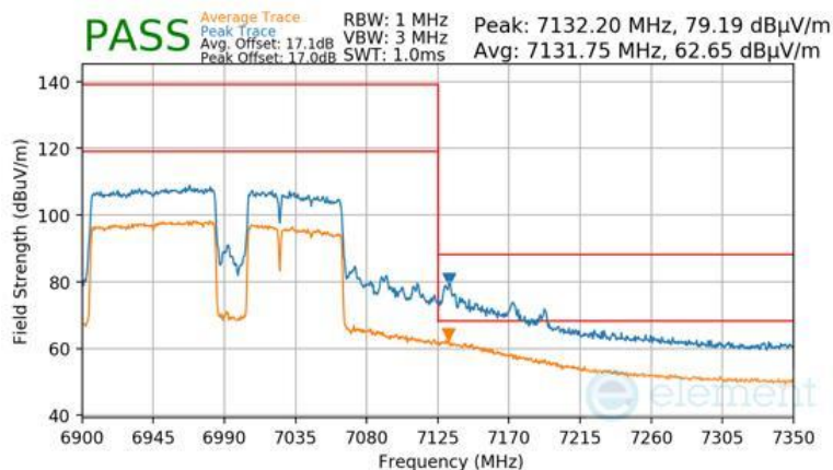
Plot 7-963 Antenna WF8 Radiated Upper Band Edge (Peak & Average – UNII Band 8) - RU996+484+242 (H)
