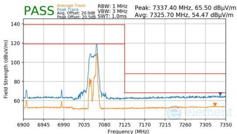
Plot 7-945 Antenna WF8 Radiated Upper Band Edge (Peak & Average – UNII Band 8) - RU26
