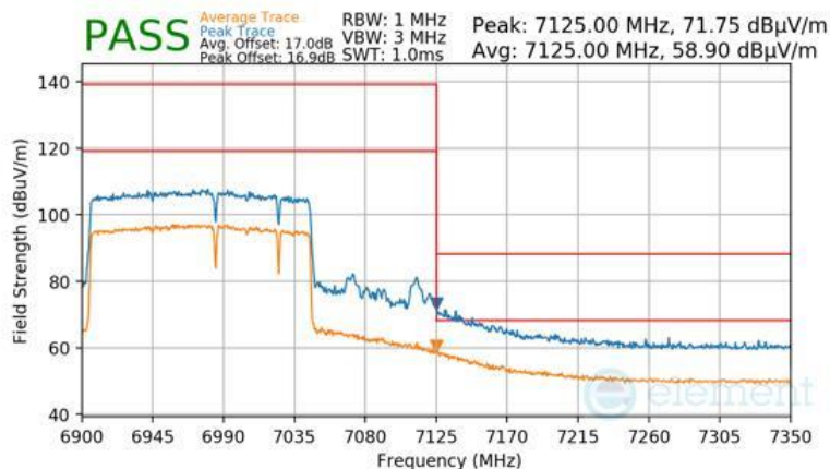
Plot 7-969 Antenna WF8 Radiated Upper Band Edge (Peak & Average – UNII Band 8) - RU996+484+242 (H)
