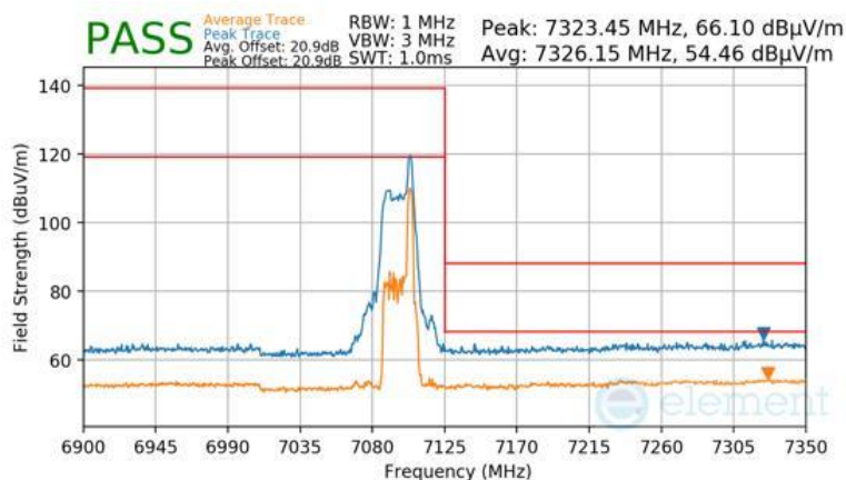
Plot 7-975 Antenna WF7 Radiated Upper Band Edge (Peak & Average – UNII Band 8) - RU26
