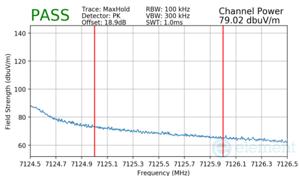
Plot 7-920 Antenna WF8 Radiated Upper Band Edge (Peak – UNII Band 8)
