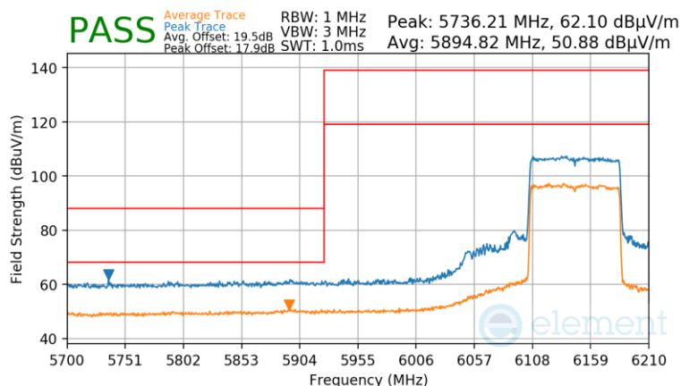
Plot 7-940 Antenna WF8 Radiated Lower Band Edge (Peak & Average – UNII Band 5) - RU996
