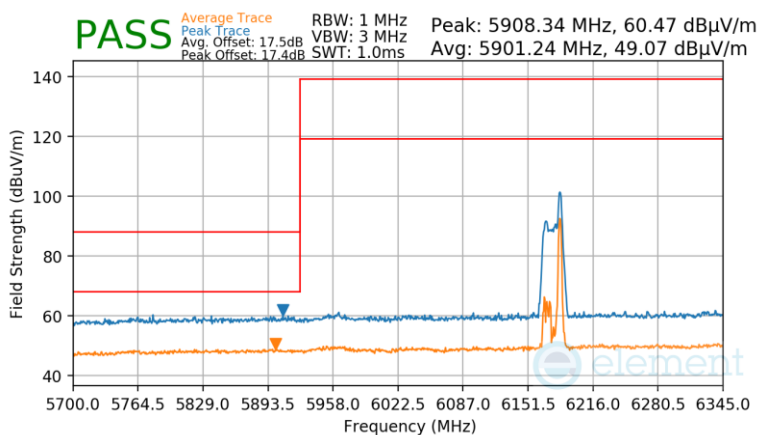
Plot 7-943 Antenna WF8 Radiated Lower Band Edge (Peak & Average – UNII Band 5) - RU26
