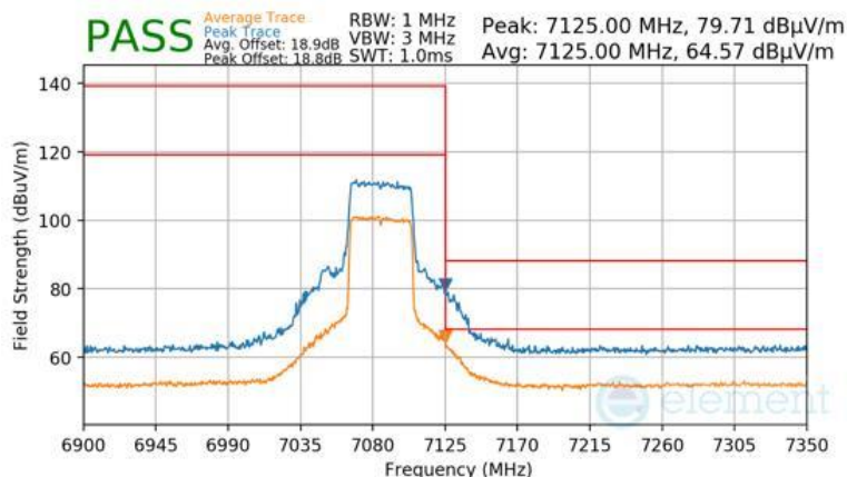
Plot 7-927 Antenna WF8 Radiated Upper Band Edge (Peak & Average – UNII Band 8) - RU484
