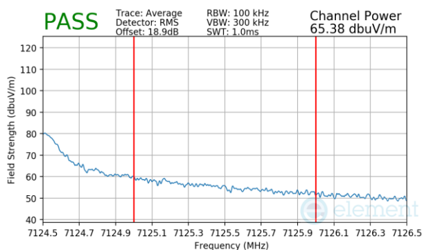
Plot 7-921 Antenna WF8 Radiated Upper Band Edge (Average – UNII Band 8)
