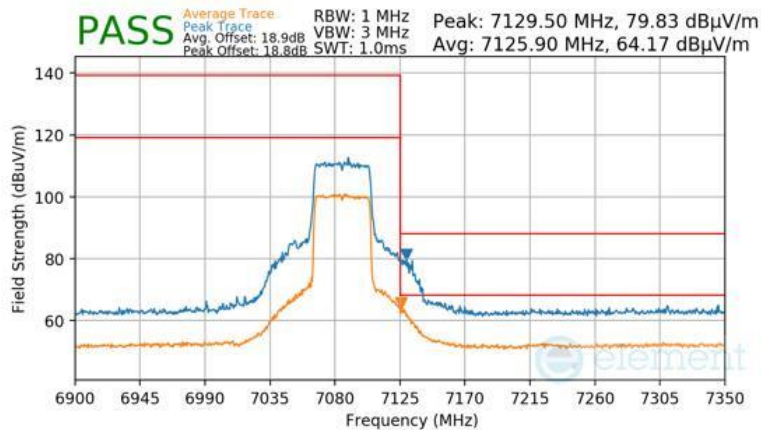
Plot 7-989 Antenna WF7 Radiated Upper Band Edge (Peak & Average – UNII Band 8) - RU484
