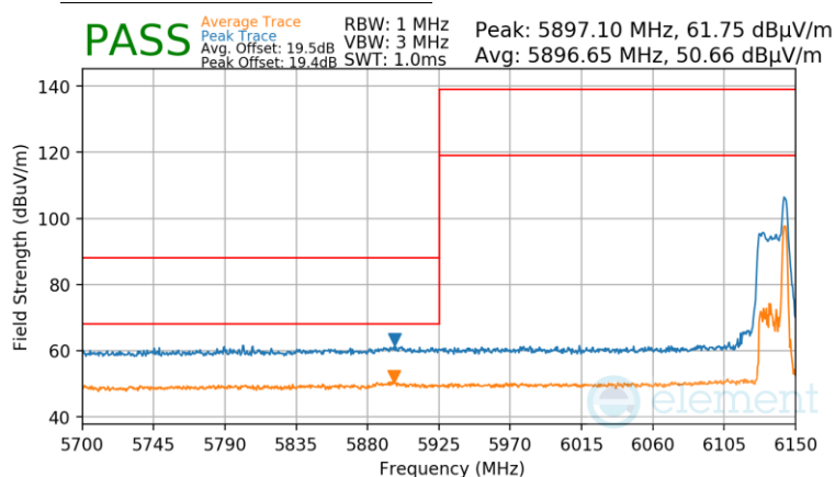
Plot 7-985 Antenna WF7 Radiated Lower Band Edge (Peak & Average – UNII Band 5) - RU26
