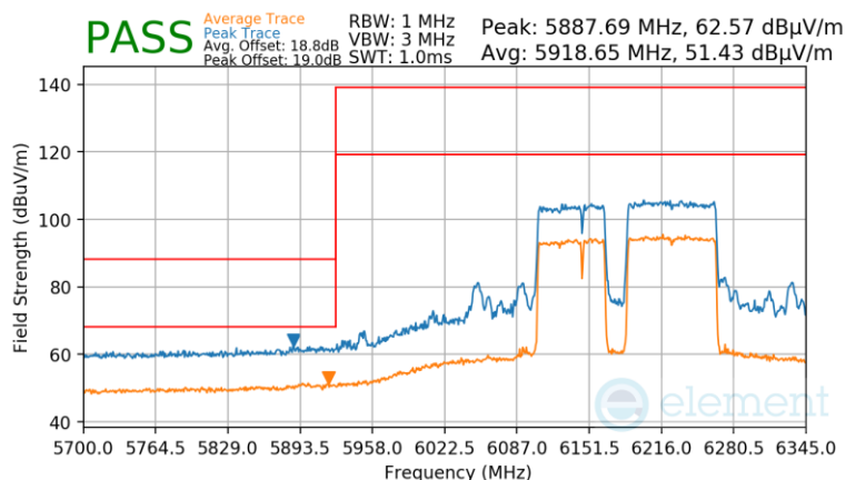
Plot 7-960 Antenna WF8 Radiated Lower Band Edge (Peak & Average – UNII Band 5) - RU996+484+242 (L)
