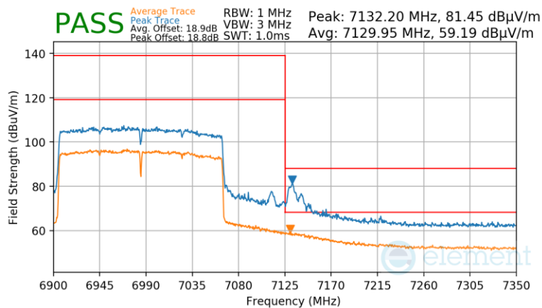
Plot 7-971 Antenna WF8 Radiated Upper Band Edge (Peak & Average – UNII Band 8) - RU996X2
