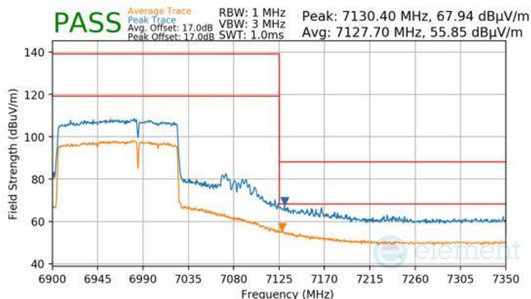
Plot 7-953 Antenna WF8 Radiated Upper Band Edge (Peak & Average – UNII Band 8) - RU996+484 (H)
