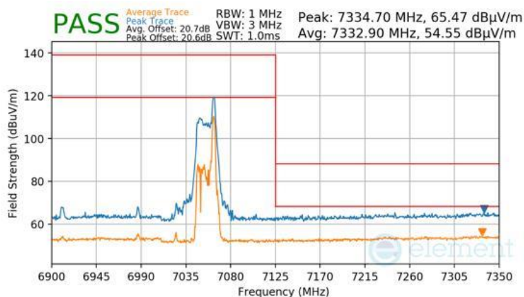
Plot 7-931 Antenna WF8 Radiated Upper Band Edge (Peak & Average – UNII Band 8) - RU26
