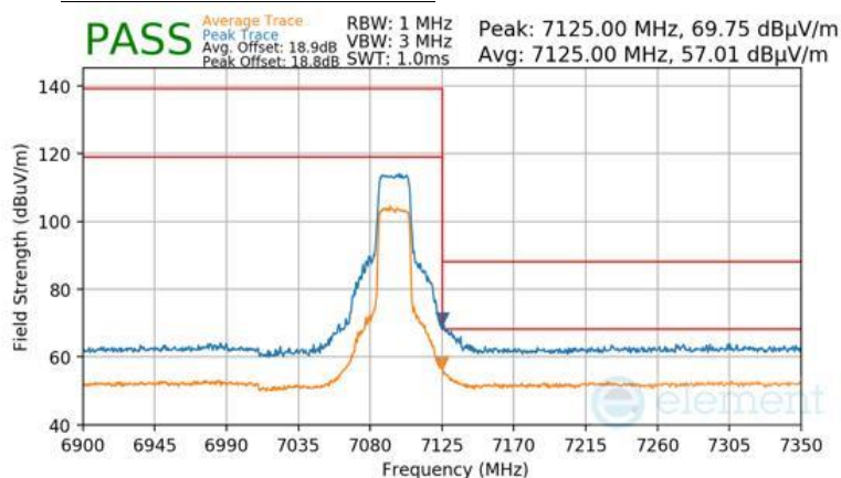
Plot 7-919 Antenna WF8 Radiated Upper Band Edge (Peak & Average – UNII Band 8) - RU242
