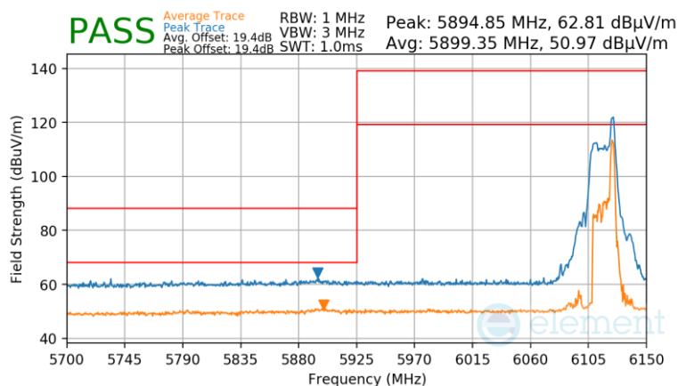
Plot 7-973 Antenna WF7 Radiated Lower Band Edge (Peak & Average – UNII Band 5) - RU26
