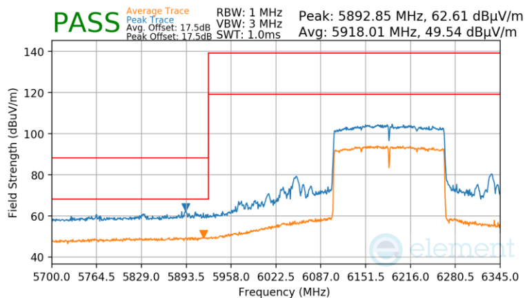
Plot 7-970 Antenna WF8 Radiated Lower Band Edge (Peak & Average – UNII Band 5) - RU996X2
