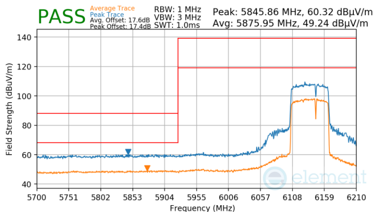
Plot 7-935 Antenna WF8 Radiated Lower Band Edge (Peak & Average – UNII Band 5) - RU484+242
