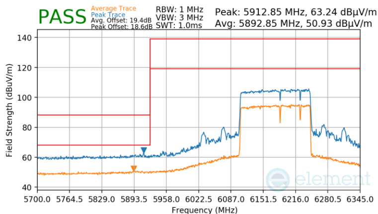
Plot 7-961 Antenna WF8 Radiated Lower Band Edge (Peak & Average – UNII Band 5) - RU996+484+242 (H)
