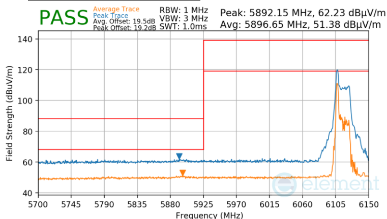
Plot 7-984 Antenna WF7 Radiated Lower Band Edge (Peak & Average – UNII Band 5) - RU26
