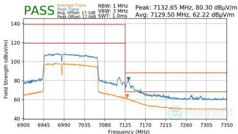
Plot 7-950 Antenna WF8 Radiated Upper Band Edge (Peak & Average – UNII Band 8) - RU996+484 (L)
