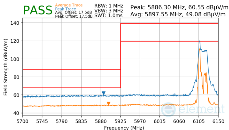
Plot 7-910 Antenna WF8 Radiated Lower Band Edge (Peak & Average – UNII Band 5) - RU26
