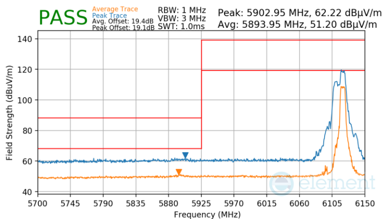
Plot 7-977 Antenna WF7 Radiated Lower Band Edge (Peak & Average – UNII Band 5) - RU52+26
