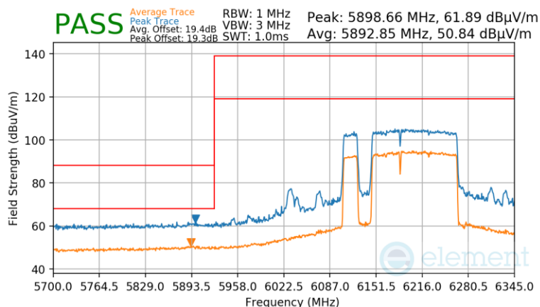
Plot 7-956 Antenna WF8 Radiated Lower Band Edge (Peak & Average – UNII Band 5) - RU996+484+242 (L)
