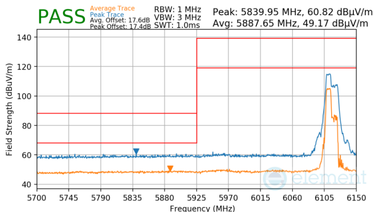
Plot 7-914 Antenna WF8 Radiated Lower Band Edge (Peak & Average – UNII Band 5) - RU52+26
