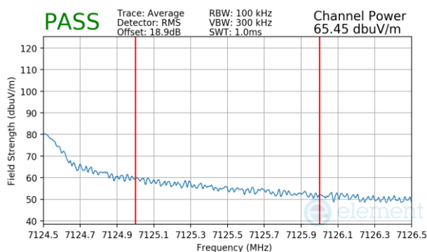
Plot 7-983 Antenna WF7 Radiated Upper Band Edge (Average – UNII Band 8)
