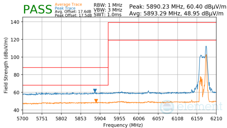
Plot 7-929 Antenna WF8 Radiated Lower Band Edge (Peak & Average – UNII Band 5) - RU26
