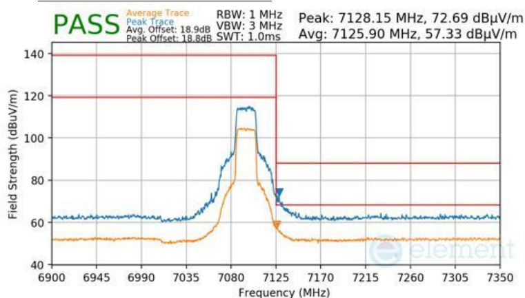
Plot 7-981 Antenna WF7 Radiated Upper Band Edge (Peak & Average – UNII Band 8) - RU242
