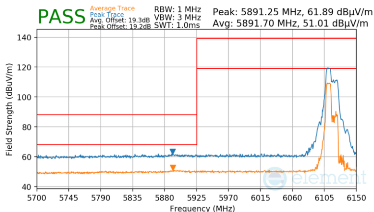
Plot 7-976 Antenna WF7 Radiated Lower Band Edge (Peak & Average – UNII Band 5) - RU52+26
