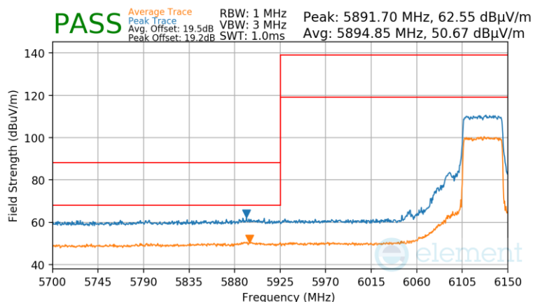
Plot 7-926 Antenna WF8 Radiated Lower Band Edge (Peak & Average – UNII Band 5) - RU484
