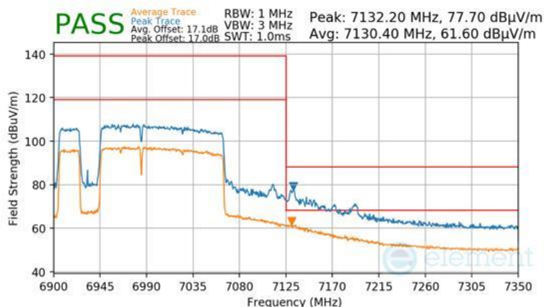
Plot 7-964 Antenna WF8 Radiated Upper Band Edge (Peak & Average – UNII Band 8) - RU996+484+242 (L)
