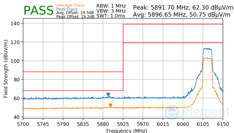
Plot 7-980 Antenna WF7 Radiated Lower Band Edge (Peak & Average – UNII Band 5) - RU242
