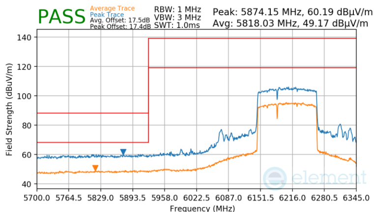
Plot 7-946 Antenna WF8 Radiated Lower Band Edge (Peak & Average – UNII Band 5) - RU996+484 (L)
