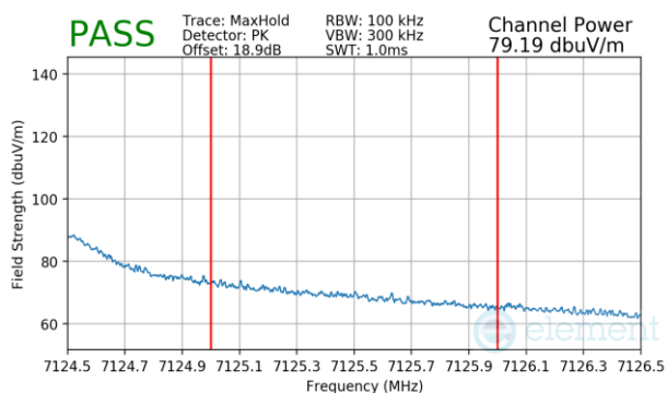
Plot 7-982 Antenna WF7 Radiated Upper Band Edge (Peak – UNII Band 8)
