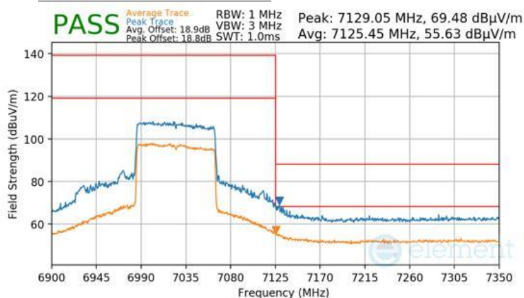
Plot 7-941 Antenna WF8 Radiated Upper Band Edge (Peak & Average – UNII Band 8) - RU996
