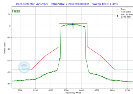
Plot 7-1212 In-Band Emission Plot CDD Diversity Antenna WF8 (160MHz BW 802.11be(RU) RU996X2 Index68 (UNII Band 5) - Ch.79)
