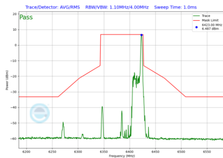
Plot 7-1157 In-Band Emission Plot CDD Diversity Antenna WF7 (80MHz BW 802.11be(RU) RU26 Index36 (UNII Band 5) - Ch.87)
