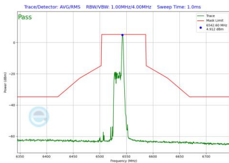
Plot 7-1165 In-Band Emission Plot CDD Diversity Antenna WF7 (80MHz BW 802.11be(RU) RU26 Index17 (UNII Band 7) - Ch.119)
