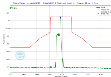
Plot 7-1177 In-Band Emission Plot CDD Diversity Antenna WF8 (80MHz BW 802.11be(RU) RU26 Index17 (UNII Band 7) - Ch.119)
