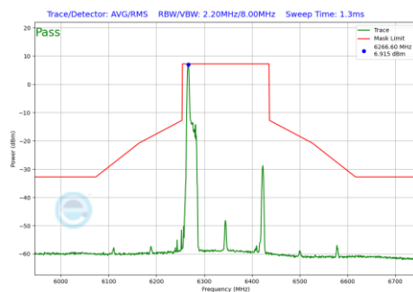
Plot 7-1158 In-Band Emission Plot CDD Diversity Antenna WF7 (160MHz BW 802.11be(RU) RU26 Index0 (UNII Band 5) - Ch.79)
