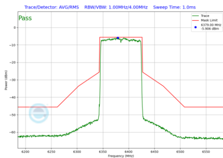
Plot 7-1279 In-Band Emission Plot SDM Diversity Antenna WF7 (80MHz BW 802.11be(RU) RU996 Index67 (UNII Band 5) - Ch.87)
