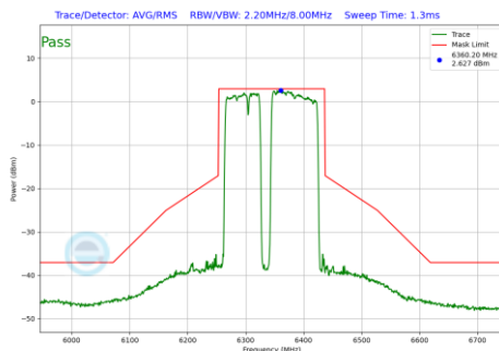
Plot 7-1190 In-Band Emission Plot CDD Diversity Antenna WF8 (160MHz BW 802.11be(RU) RU996+484+242 Index99 (UNII Band 5) - Ch.79)
