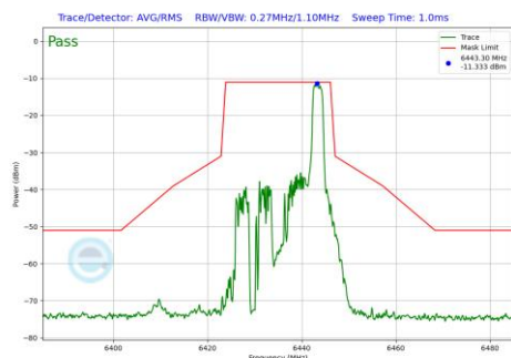
Plot 7-1241 In-Band Emission Plot SDM Diversity Antenna WF8 (20MHz BW 802.11be(RU) RU26 Index8 (UNII Band 6) - Ch.97)
