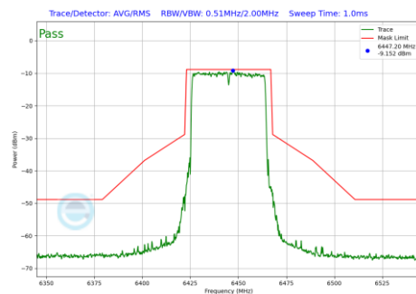
Plot 7-1282 In-Band Emission Plot SDM Diversity Antenna WF7 (40MHz BW 802.11be(RU) RU484 Index65 (UNII Band 6) - Ch.99)
