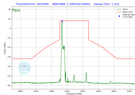
Plot 7-1170 In-Band Emission Plot CDD Diversity Antenna WF8 (160MHz BW 802.11be(RU) RU26 Index0 (UNII Band 5) - Ch.79)
