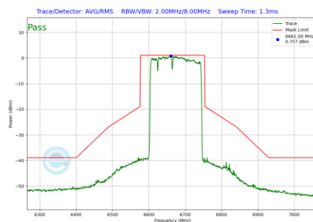
Plot 7-1196 In-Band Emission Plot CDD Diversity Antenna WF8 (160MHz BW 802.11be(RU) RU996+484+242 Index96 (UNII Band 7) - Ch.143)
