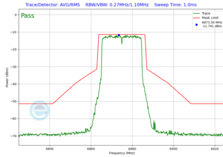
Plot 7-1147 In-Band Emission Plot SDM Primary Antenna WF8 (20MHz BW 802.11be(RU) RU242 Index61 (UNII Band 7) - Ch.185)
