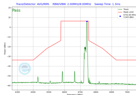
Plot 7-1178 In-Band Emission Plot CDD Diversity Antenna WF8 (160MHz BW 802.11be(RU) RU26 Index36 (UNII Band 7) - Ch.143)
