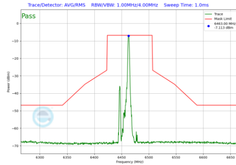
Plot 7-1243 In-Band Emission Plot SDM Diversity Antenna WF8 (80MHz BW 802.11be(RU) RU26 Index17 (UNII Band 6) - Ch.103)
