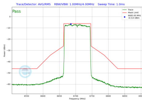
Plot 7-1287 In-Band Emission Plot SDM Diversity Antenna WF7 (80MHz BW 802.11be(RU) RU996 Index67 (UNII Band 7) - Ch.151)
