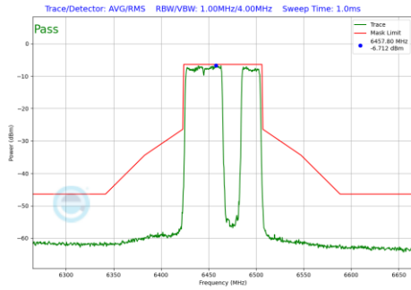
Plot 7-1269 In-Band Emission Plot SDM Diversity Antenna WF8 (80MHz BW 802.11be(RU) RU484+242 Index92 (UNII Band 6) - Ch.103)
