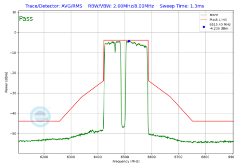
Plot 7-1270 In-Band Emission Plot SDM Diversity Antenna WF8 (160MHz BW 802.11be(RU) RU996+484+242 Index99 (UNII Band 6) - Ch.111)
