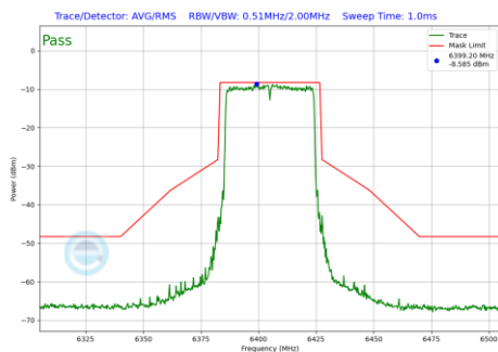
Plot 7-1278 In-Band Emission Plot SDM Diversity Antenna WF7 (40MHz BW 802.11be(RU) RU484 Index65 (UNII Band 5) - Ch.91)
