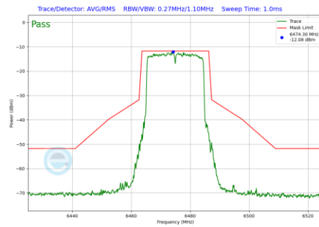
Plot 7-1281 In-Band Emission Plot SDM Diversity Antenna WF7 (20MHz BW 802.11be(RU) RU242 Index61 (UNII Band 6) - Ch.105)
