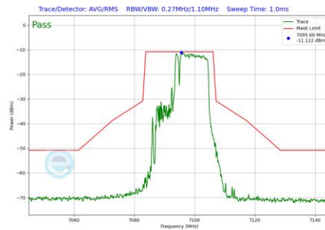
Plot 7-1274 In-Band Emission Plot SDM Diversity Antenna WF8 (20MHz BW 802.11be(RU) RU106+26 Index83 (UNII Band 8) - Ch.229)
