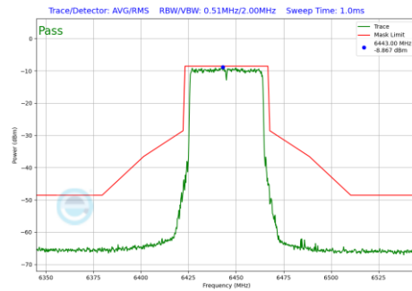
Plot 7-1298 In-Band Emission Plot SDM Diversity Antenna WF8 (40MHz BW 802.11be(RU) RU484 Index65 (UNII Band 6) - Ch.99)
