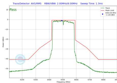
Plot 7-1216 In-Band Emission Plot CDD Diversity Antenna WF8 (160MHz BW 802.11be(RU) RU996X2 Index68 (UNII Band 6) - Ch.111)
