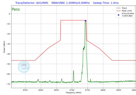
Plot 7-1247 In-Band Emission Plot SDM Diversity Antenna WF8 (80MHz BW 802.11be(RU) RU26 Index36 (UNII Band 7) - Ch.151)
