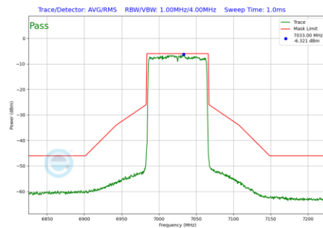
Plot 7-1291 In-Band Emission Plot SDM Diversity Antenna WF7 (80MHz BW 802.11be(RU) RU996 Index67 (UNII Band 8) - Ch.215)
