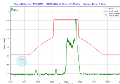
Plot 7-1246 In-Band Emission Plot SDM Diversity Antenna WF8 (40MHz BW 802.11be(RU) RU26 Index17 (UNII Band 7) - Ch.155)
