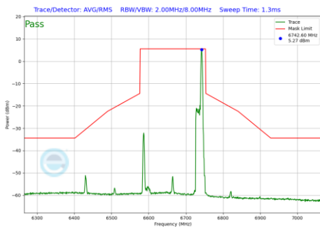
Plot 7-1166 In-Band Emission Plot CDD Diversity Antenna WF7 (160MHz BW 802.11be(RU) RU26 Index36 (UNII Band 7) - Ch.143)
