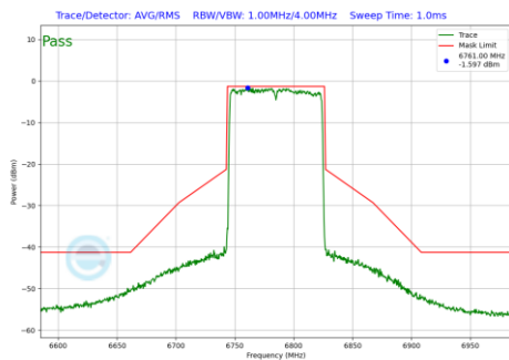
Plot 7-1207 In-Band Emission Plot CDD Diversity Antenna WF7 (80MHz BW 802.11be(RU) RU996 Index67 (UNII Band 7) - Ch.167)
