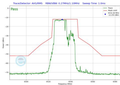
Plot 7-1271 In-Band Emission Plot SDM Diversity Antenna WF8 (20MHz BW 802.11be(RU) RU106+26 Index82 (UNII Band 7) - Ch.117)
