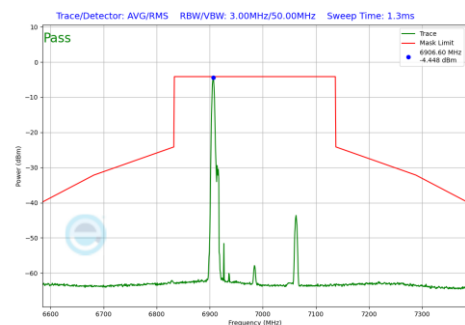
Plot 7-1252 In-Band Emission Plot SDM Diversity Antenna WF8 (160MHz BW 802.11be(RU) RU26 Index0 (UNII Band 8) - Ch.207)
