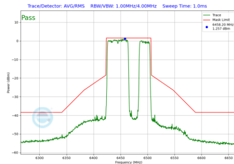
Plot 7-1192 In-Band Emission Plot CDD Diversity Antenna WF8 (80MHz BW 802.11be(RU) RU484+242 Index92 (UNII Band 6) - Ch.103)
