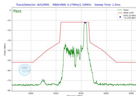
Plot 7-1245 In-Band Emission Plot SDM Diversity Antenna WF8 (20MHz BW 802.11be(RU) RU26 Index8 (UNII Band 7) - Ch.117)
