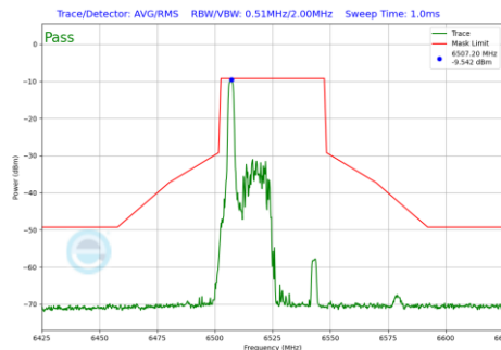
Plot 7-1226 In-Band Emission Plot SDM Diversity Antenna WF7 (40MHz BW 802.11be(RU) RU26 Index0 (UNII Band 6) - Ch.115)
