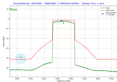
Plot 7-1296 In-Band Emission Plot SDM Diversity Antenna WF8 (160MHz BW 802.11be(RU) RU996X2 Index68 (UNII Band 5) - Ch.79)
