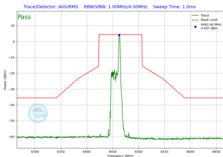
Plot 7-1173 In-Band Emission Plot CDD Diversity Antenna WF8 (80MHz BW 802.11be(RU) RU26 Index17 (UNII Band 6) - Ch.103)
