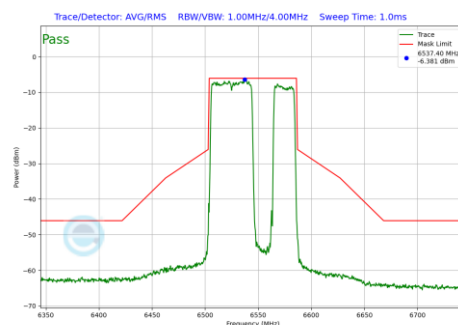
Plot 7-1260 In-Band Emission Plot SDM Diversity Antenna WF7 (80MHz BW 802.11be(RU) RU484+242 Index92 (UNII Band 7) - Ch.119)
