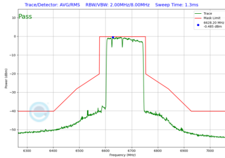
Plot 7-1187 In-Band Emission Plot CDD Diversity Antenna WF7 (160MHz BW 802.11be(RU) RU996+484+242 Index96 (UNII Band 7) - Ch.143)
