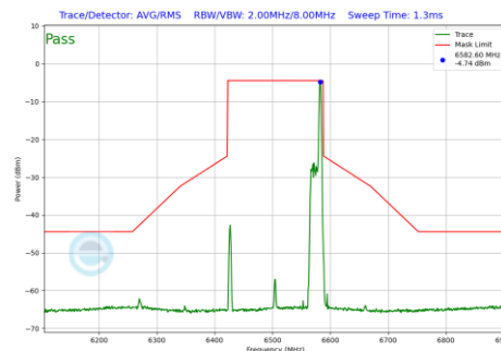
Plot 7-1244 In-Band Emission Plot SDM Diversity Antenna WF8 (160MHz BW 802.11be(RU) RU26 Index36 (UNII Band 6) - Ch.111)
