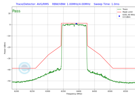
Plot 7-1211 In-Band Emission Plot CDD Diversity Antenna WF8 (80MHz BW 802.11be(RU) RU996 Index67 (UNII Band 5) - Ch.87)
