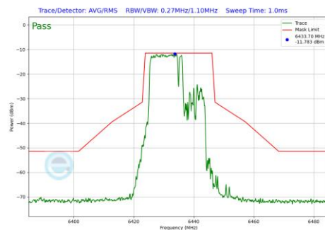
Plot 7-1268 In-Band Emission Plot SDM Diversity Antenna WF8 (20MHz BW 802.11be(RU) RU106+26 Index82 (UNII Band 6) - Ch.97)
