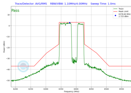
Plot 7-1180 In-Band Emission Plot CDD Diversity Antenna WF7 (80MHz BW 802.11be(RU) RU484+242 Index92 (UNII Band 5) - Ch.87)
