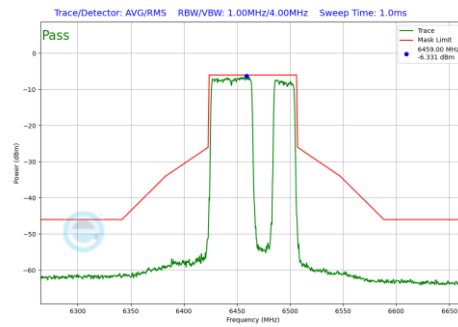
Plot 7-1257 In-Band Emission Plot SDM Diversity Antenna WF7 (80MHz BW 802.11be(RU) RU484+242 Index92 (UNII Band 6) - Ch.103)
