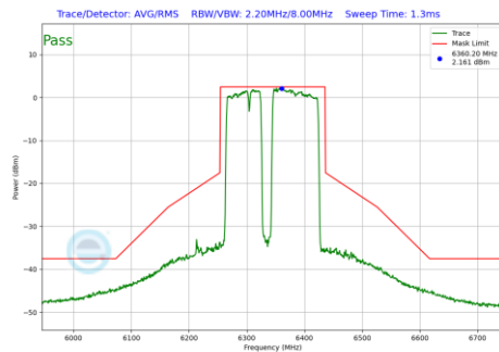
Plot 7-1181 In-Band Emission Plot CDD Diversity Antenna WF7 (160MHz BW 802.11be(RU) RU996+484+242 Index99 (UNII Band 5) - Ch.79)
