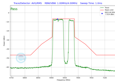
Plot 7-1275 In-Band Emission Plot SDM Diversity Antenna WF8 (80MHz BW 802.11be(RU) RU484+242 Index92 (UNII Band 8) - Ch.199)
