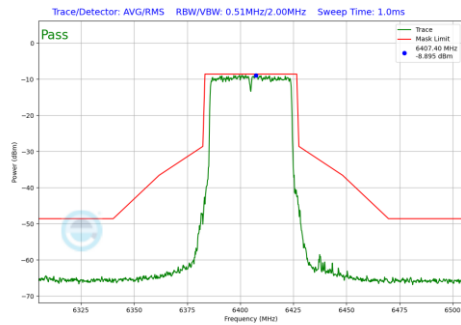
Plot 7-1294 In-Band Emission Plot SDM Diversity Antenna WF8 (40MHz BW 802.11be(RU) RU484 Index65 (UNII Band 5) - Ch.91)
