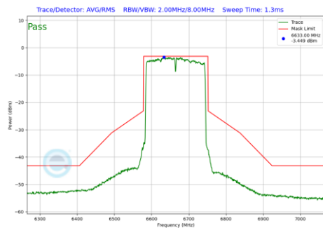
Plot 7-1288 In-Band Emission Plot SDM Diversity Antenna WF7 (160MHz BW 802.11be(RU) RU996X2 Index68 (UNII Band 7) - Ch.143)
