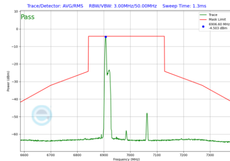
Plot 7-1236 In-Band Emission Plot SDM Diversity Antenna WF7 (160MHz BW 802.11be(RU) RU26 Index0 (UNII Band 8) - Ch.207)
