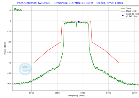
Plot 7-1217 In-Band Emission Plot CDD Diversity Antenna WF8 (20MHz BW 802.11be(RU) RU242 Index61 (UNII Band 7) - Ch.149)
