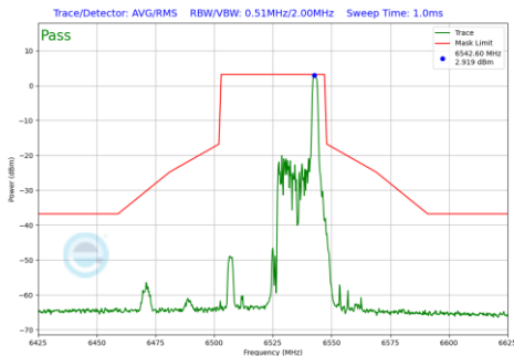
Plot 7-1172 In-Band Emission Plot CDD Diversity Antenna WF8 (40MHz BW 802.11be(RU) RU26 Index17 (UNII Band 6) - Ch.115)
