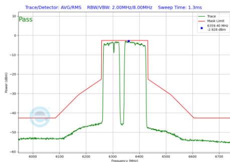
Plot 7-1255 In-Band Emission Plot SDM Diversity Antenna WF7 (160MHz BW 802.11be(RU) RU996+484+242 Index99 (UNII Band 5) - Ch.79)
