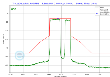
Plot 7-1263 In-Band Emission Plot SDM Diversity Antenna WF7 (80MHz BW 802.11be(RU) RU484+242 Index92 (UNII Band 8) - Ch.199)
