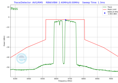
Plot 7-1273 In-Band Emission Plot SDM Diversity Antenna WF8 (160MHz BW 802.11be(RU) RU996+484+242 Index99 (UNII Band 7) - Ch.143)
