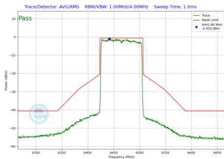
Plot 7-1215 In-Band Emission Plot CDD Diversity Antenna WF8 (80MHz BW 802.11be(RU) RU996 Index67 (UNII Band 6) - Ch.103)
