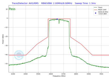
Plot 7-1208 In-Band Emission Plot CDD Diversity Antenna WF7 (160MHz BW 802.11be(RU) RU996X2 Index68 (UNII Band 7) - Ch.143)
