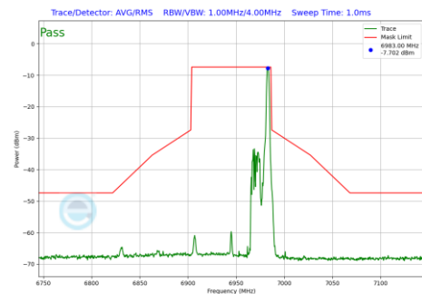
Plot 7-1251 In-Band Emission Plot SDM Diversity Antenna WF8 (80MHz BW 802.11be(RU) RU26 Index36 (UNII Band 8) - Ch.199)
