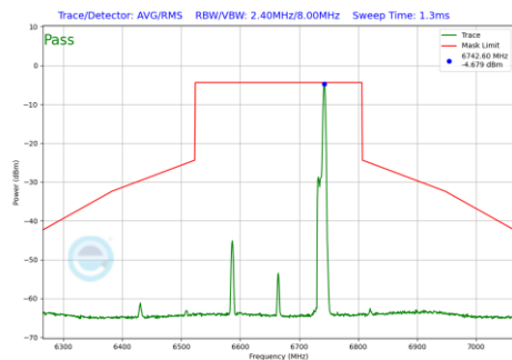
Plot 7-1248 In-Band Emission Plot SDM Diversity Antenna WF8 (160MHz BW 802.11be(RU) RU26 Index36 (UNII Band 7) - Ch.143)
