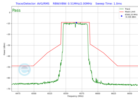
Plot 7-1148 In-Band Emission Plot SDM Primary Antenna WF8 (40MHz BW 802.11be(RU) RU484 Index65 (UNII Band 7) - Ch.123)
