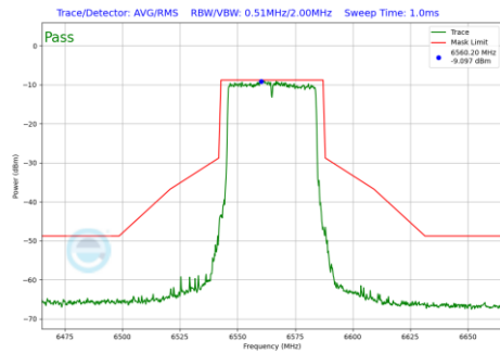
Plot 7-1286 In-Band Emission Plot SDM Diversity Antenna WF7 (40MHz BW 802.11be(RU) RU484 Index65 (UNII Band 7) - Ch.123)
