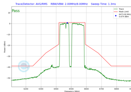
Plot 7-1193 In-Band Emission Plot CDD Diversity Antenna WF8 (160MHz BW 802.11be(RU) RU996+484+242 Index99 (UNII Band 6) - Ch.111)
