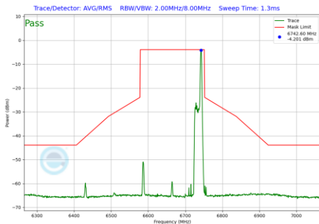
Plot 7-1232 In-Band Emission Plot SDM Diversity Antenna WF7 (160MHz BW 802.11be(RU) RU26 Index36 (UNII Band 7) - Ch.143)
