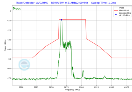
Plot 7-1250 In-Band Emission Plot SDM Diversity Antenna WF8 (40MHz BW 802.11be(RU) RU26 Index0 (UNII Band 8) - Ch.187)
