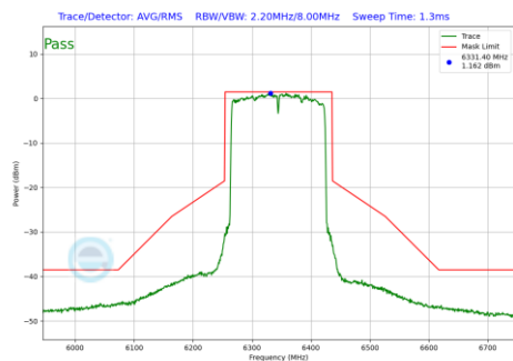
Plot 7-1200 In-Band Emission Plot CDD Diversity Antenna WF7 (160MHz BW 802.11be(RU) RU996X2 Index68 (UNII Band 5) - Ch.79)
