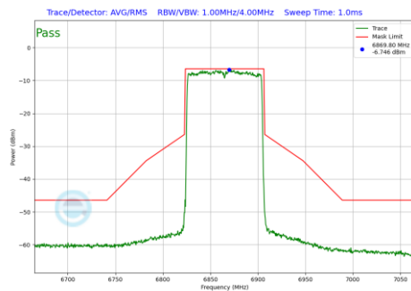
Plot 7-1149 In-Band Emission Plot SDM Primary Antenna WF8 (80MHz BW 802.11be(RU) RU996 Index67 (UNII Band 7) - Ch.183)
