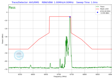
Plot 7-1231 In-Band Emission Plot SDM Diversity Antenna WF7 (80MHz BW 802.11be(RU) RU26 Index36 (UNII Band 7) - Ch.151)
