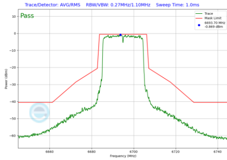
Plot 7-1205 In-Band Emission Plot CDD Diversity Antenna WF7 (20MHz BW 802.11be(RU) RU242 Index61 (UNII Band 7) - Ch.149)
