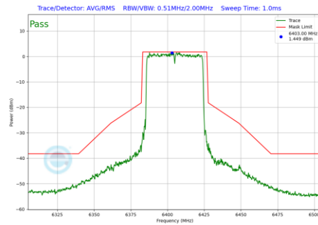
Plot 7-1210 In-Band Emission Plot CDD Diversity Antenna WF8 (40MHz BW 802.11be(RU) RU484 Index65 (UNII Band 5) - Ch.91)
