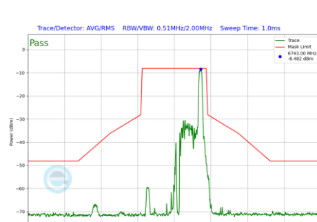
Plot 7-1230 In-Band Emission Plot SDM Diversity Antenna WF7 (40MHz BW 802.11be(RU) RU26 Index17 (UNII Band 7) - Ch.155)
