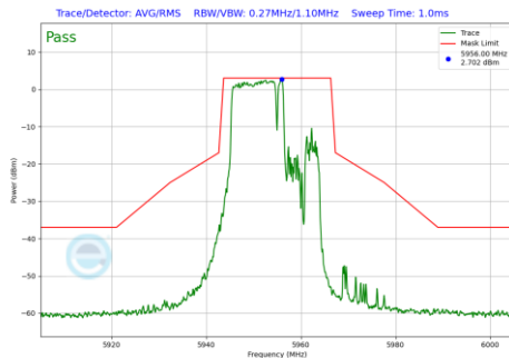
Plot 7-1188 In-Band Emission Plot CDD Diversity Antenna WF8 (20MHz BW 802.11be(RU) RU106+26 Index82 (UNII Band 5) - Ch.1)
