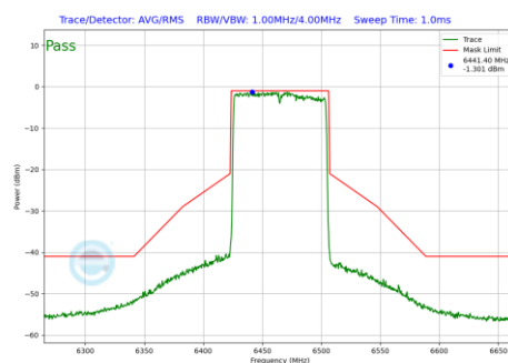
Plot 7-1203 In-Band Emission Plot CDD Diversity Antenna WF7 (80MHz BW 802.11be(RU) RU996 Index67 (UNII Band 6) - Ch.103)
