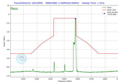
Plot 7-1228 In-Band Emission Plot SDM Diversity Antenna WF7 (160MHz BW 802.11be(RU) RU26 Index36 (UNII Band 6) - Ch.111)
