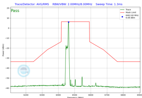
Plot 7-1174 In-Band Emission Plot CDD Diversity Antenna WF8 (160MHz BW 802.11be(RU) RU26 Index17 (UNII Band 6) - Ch.111)
