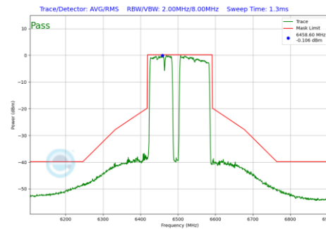
Plot 7-1184 In-Band Emission Plot CDD Diversity Antenna WF7 (160MHz BW 802.11be(RU) RU996+484+242 Index99 (UNII Band 6) - Ch.111)
