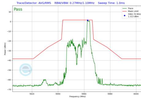
Plot 7-1167 In-Band Emission Plot CDD Diversity Antenna WF8 (20MHz BW 802.11be(RU) RU26 Index8 (UNII Band 5) - Ch.1)
