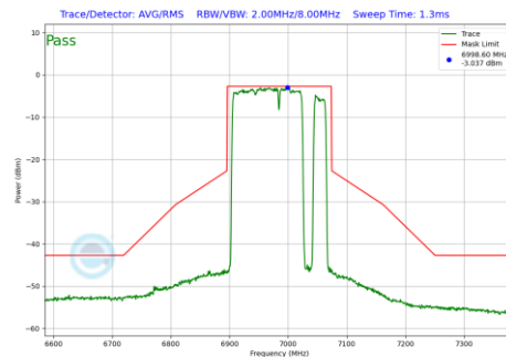
Plot 7-1276 In-Band Emission Plot SDM Diversity Antenna WF8 (160MHz BW 802.11be(RU) RU996+484+242 Index98 (UNII Band 8) - Ch.207)
