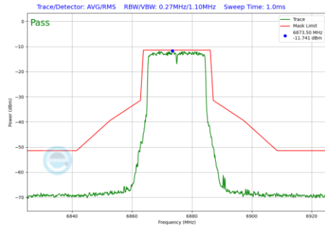
Plot 7-1301 In-Band Emission Plot SDM Diversity Antenna WF8 (20MHz BW 802.11be(RU) RU242 Index61 (UNII Band 7) - Ch.185)
