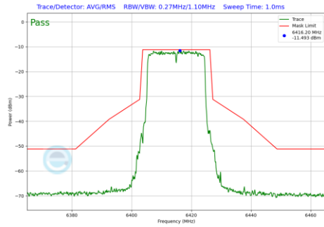
Plot 7-1293 In-Band Emission Plot SDM Diversity Antenna WF8 (20MHz BW 802.11be(RU) RU242 Index61 (UNII Band 5) - Ch.93)
