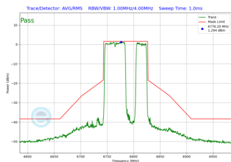
Plot 7-1195 In-Band Emission Plot CDD Diversity Antenna WF8 (80MHz BW 802.11be(RU) RU484+242 Index92 (UNII Band 7) - Ch.167)
