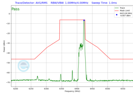
Plot 7-1239 In-Band Emission Plot SDM Diversity Antenna WF8 (80MHz BW 802.11be(RU) RU26 Index36 (UNII Band 5) - Ch.87)
