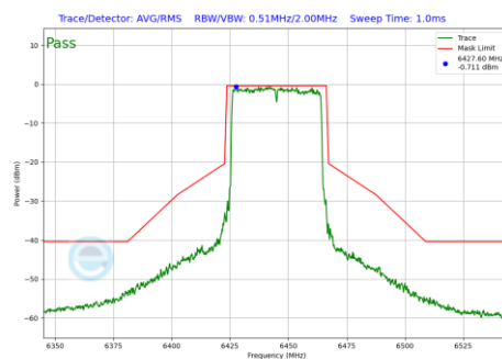
Plot 7-1202 In-Band Emission Plot CDD Diversity Antenna WF7 (40MHz BW 802.11be(RU) RU484 Index65 (UNII Band 6) - Ch.99)
