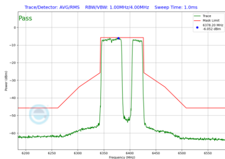
Plot 7-1254 In-Band Emission Plot SDM Diversity Antenna WF7 (80MHz BW 802.11be(RU) RU484+242 Index92 (UNII Band 5) - Ch.87)
