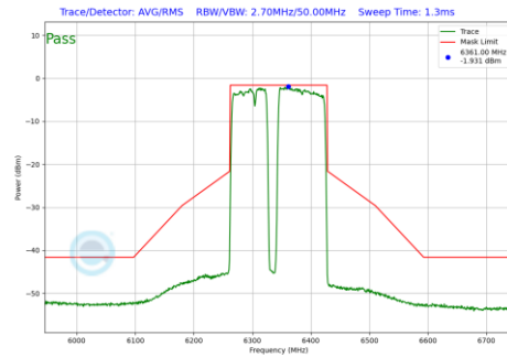
Plot 7-1267 In-Band Emission Plot SDM Diversity Antenna WF8 (160MHz BW 802.11be(RU) RU996+484+242 Index99 (UNII Band 5) - Ch.79)
