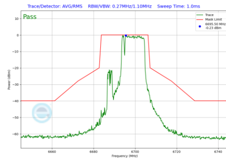
Plot 7-1185 In-Band Emission Plot CDD Diversity Antenna WF7 (20MHz BW 802.11be(RU) RU106+26 Index83 (UNII Band 7) - Ch.149)
