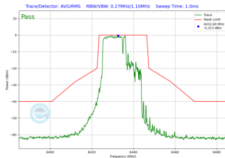
Plot 7-1182 In-Band Emission Plot CDD Diversity Antenna WF7 (20MHz BW 802.11be(RU) RU106+26 Index82 (UNII Band 6) - Ch.97)
