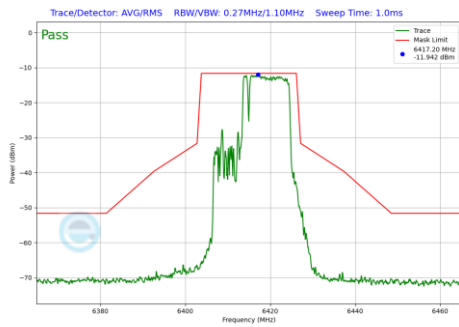
Plot 7-1253 In-Band Emission Plot SDM Diversity Antenna WF7 (20MHz BW 802.11be(RU) RU106+26 Index83 (UNII Band 5) - Ch.93)
