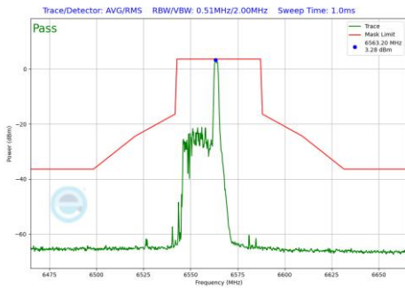
Plot 7-1164 In-Band Emission Plot CDD Diversity Antenna WF7 (40MHz BW 802.11be(RU) RU26 Index8 (UNII Band 7) - Ch.123)
