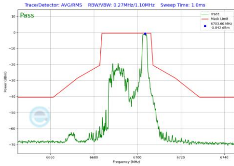
Plot 7-1163 In-Band Emission Plot CDD Diversity Antenna WF7 (20MHz BW 802.11be(RU) RU26 Index8 (UNII Band 7) - Ch.149)
