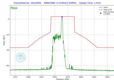
Plot 7-1176 In-Band Emission Plot CDD Diversity Antenna WF8 (40MHz BW 802.11be(RU) RU26 Index8 (UNII Band 7) - Ch.123)
