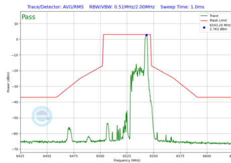
Plot 7-1160 In-Band Emission Plot CDD Diversity Antenna WF7 (40MHz BW 802.11be(RU) RU26 Index17 (UNII Band 6) - Ch.115)
