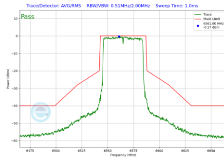
Plot 7-1218 In-Band Emission Plot CDD Diversity Antenna WF8 (40MHz BW 802.11be(RU) RU484 Index65 (UNII Band 7) - Ch.123)
