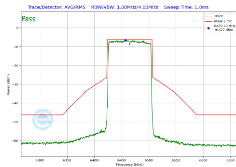
Plot 7-1299 In-Band Emission Plot SDM Diversity Antenna WF8 (80MHz BW 802.11be(RU) RU996 Index67 (UNII Band 6) - Ch.103)
