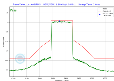
Plot 7-1199 In-Band Emission Plot CDD Diversity Antenna WF7 (80MHz BW 802.11be(RU) RU996 Index67 (UNII Band 5) - Ch.87)
