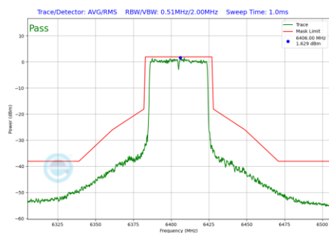
Plot 7-1198 In-Band Emission Plot CDD Diversity Antenna WF7 (40MHz BW 802.11be(RU) RU484 Index65 (UNII Band 5) - Ch.91)
