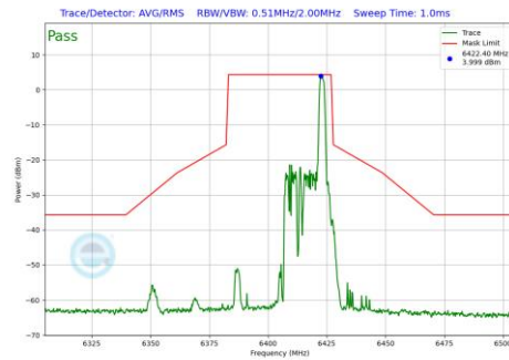
Plot 7-1168 In-Band Emission Plot CDD Diversity Antenna WF8 (40MHz BW 802.11be(RU) RU26 Index17 (UNII Band 5) - Ch.91)
