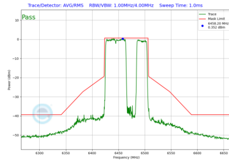
Plot 7-1183 In-Band Emission Plot CDD Diversity Antenna WF7 (80MHz BW 802.11be(RU) RU484+242 Index92 (UNII Band 6) - Ch.103)
