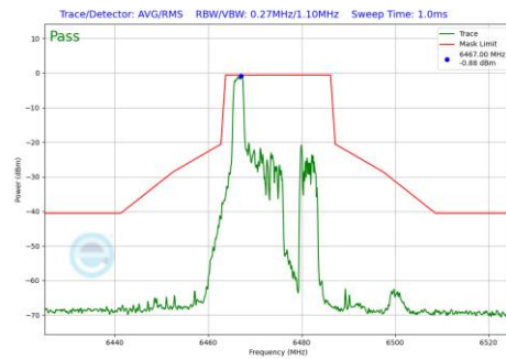
Plot 7-1159 In-Band Emission Plot CDD Diversity Antenna WF7 (20MHz BW 802.11be(RU) RU26 Index0 (UNII Band 6) - Ch.105)
