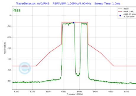
Plot 7-1266 In-Band Emission Plot SDM Diversity Antenna WF8 (80MHz BW 802.11be(RU) RU484+242 Index92 (UNII Band 5) - Ch.87)
