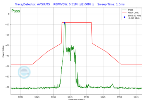
Plot 7-1234 In-Band Emission Plot SDM Diversity Antenna WF7 (40MHz BW 802.11be(RU) RU26 Index0 (UNII Band 8) - Ch.187)
