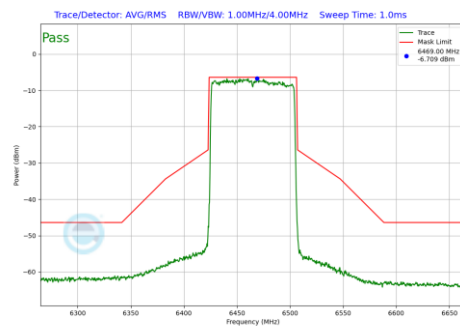
Plot 7-1283 In-Band Emission Plot SDM Diversity Antenna WF7 (80MHz BW 802.11be(RU) RU996 Index67 (UNII Band 6) - Ch.103)
