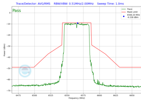
Plot 7-1302 In-Band Emission Plot SDM Diversity Antenna WF8 (40MHz BW 802.11be(RU) RU484 Index65 (UNII Band 7) - Ch.123)
