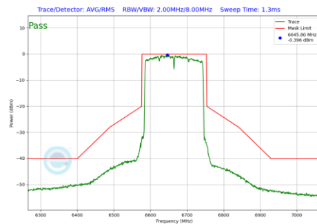
Plot 7-1220 In-Band Emission Plot CDD Diversity Antenna WF8 (160MHz BW 802.11be(RU) RU996X2 Index68 (UNII Band 7) - Ch.143)
