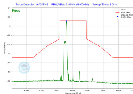
Plot 7-1162 In-Band Emission Plot CDD Diversity Antenna WF7 (160MHz BW 802.11be(RU) RU26 Index17 (UNII Band 6) - Ch.111)
