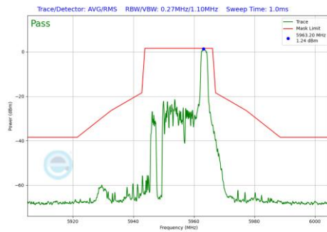
Plot 7-1155 In-Band Emission Plot CDD Diversity Antenna WF7 (20MHz BW 802.11be(RU) RU26 Index8 (UNII Band 5) - Ch.1)
