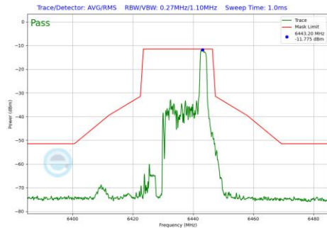
Plot 7-1225 In-Band Emission Plot SDM Diversity Antenna WF7 (20MHz BW 802.11be(RU) RU26 Index8 (UNII Band 6) - Ch.97)
