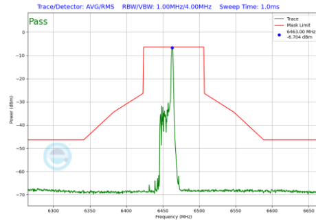
Plot 7-1227 In-Band Emission Plot SDM Diversity Antenna WF7 (80MHz BW 802.11be(RU) RU26 Index17 (UNII Band 6) - Ch.103)
