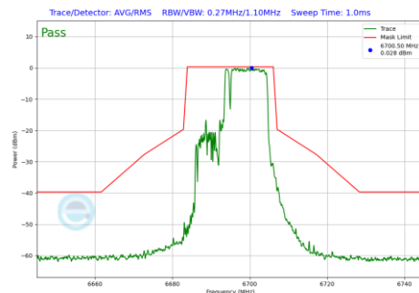
Plot 7-1194 In-Band Emission Plot CDD Diversity Antenna WF8 (20MHz BW 802.11be(RU) RU106+26 Index83 (UNII Band 7) - Ch.149)
