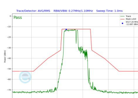
Plot 7-1259 In-Band Emission Plot SDM Diversity Antenna WF7 (20MHz BW 802.11be(RU) RU106+26 Index82 (UNII Band 7) - Ch.117)
