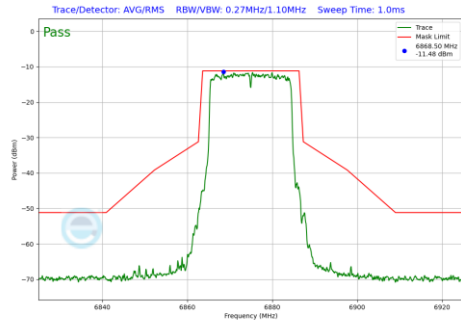
Plot 7-1285 In-Band Emission Plot SDM Diversity Antenna WF7 (20MHz BW 802.11be(RU) RU242 Index61 (UNII Band 7) - Ch.185)
