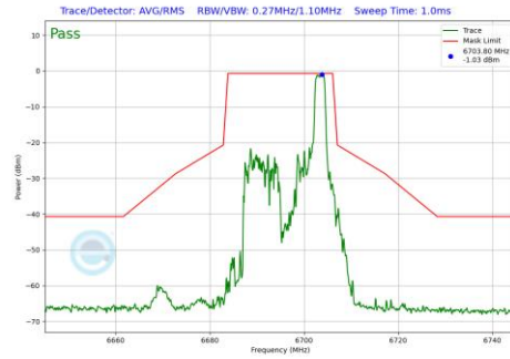
Plot 7-1175 In-Band Emission Plot CDD Diversity Antenna WF8 (20MHz BW 802.11be(RU) RU26 Index8 (UNII Band 7) - Ch.149)
