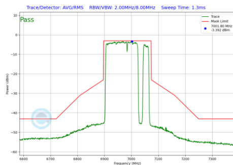
Plot 7-1264 In-Band Emission Plot SDM Diversity Antenna WF7 (160MHz BW 802.11be(RU) RU996+484+242 Index98 (UNII Band 8) - Ch.207)
