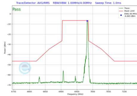
Plot 7-1235 In-Band Emission Plot SDM Diversity Antenna WF7 (80MHz BW 802.11be(RU) RU26 Index36 (UNII Band 8) - Ch.199)
