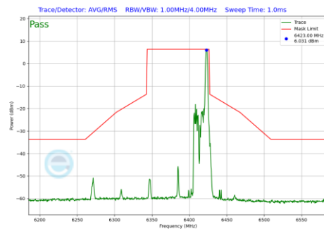
Plot 7-1169 In-Band Emission Plot CDD Diversity Antenna WF8 (80MHz BW 802.11be(RU) RU26 Index36 (UNII Band 5) - Ch.87)
