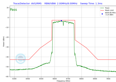
Plot 7-1150 In-Band Emission Plot SDM Primary Antenna WF8 (160MHz BW 802.11be(RU) RU996X2 Index68 (UNII Band 7) - Ch.143)
