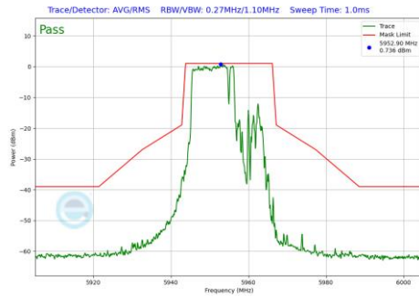
Plot 7-1179 In-Band Emission Plot CDD Diversity Antenna WF7 (20MHz BW 802.11be(RU) RU106+26 Index82 (UNII Band 5) - Ch.1)
