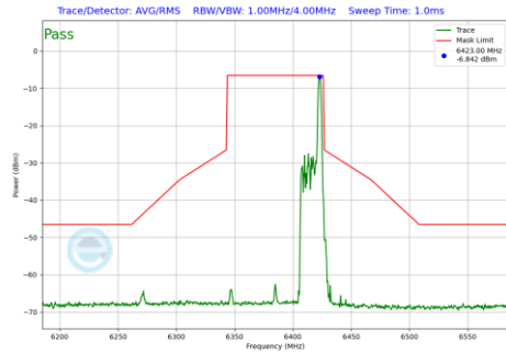
Plot 7-1223 In-Band Emission Plot SDM Diversity Antenna WF7 (80MHz BW 802.11be(RU) RU26 Index36 (UNII Band 5) - Ch.87)
