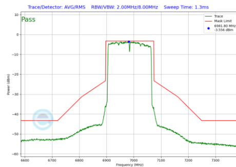
Plot 7-1292 In-Band Emission Plot SDM Diversity Antenna WF7 (160MHz BW 802.11be(RU) RU996X2 Index68 (UNII Band 8) - Ch.207)
