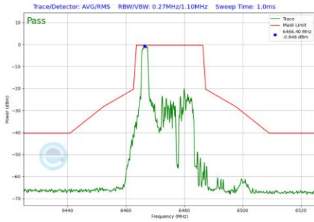
Plot 7-1171 In-Band Emission Plot CDD Diversity Antenna WF8 (20MHz BW 802.11be(RU) RU26 Index0 (UNII Band 6) - Ch.105)
