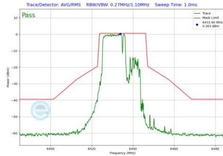
Plot 7-1191 In-Band Emission Plot CDD Diversity Antenna WF8 (20MHz BW 802.11be(RU) RU106+26 Index82 (UNII Band 6) - Ch.97)
