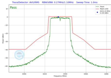
Plot 7-1213 In-Band Emission Plot CDD Diversity Antenna WF8 (20MHz BW 802.11be(RU) RU242 Index61 (UNII Band 6) - Ch.97)
