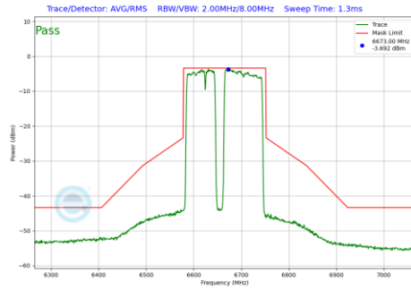
Plot 7-1261 In-Band Emission Plot SDM Diversity Antenna WF7 (160MHz BW 802.11be(RU) RU996+484+242 Index99 (UNII Band 7) - Ch.143)
