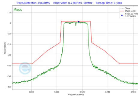
Plot 7-1209 In-Band Emission Plot CDD Diversity Antenna WF8 (20MHz BW 802.11be(RU) RU242 Index61 (UNII Band 5) - Ch.93)
