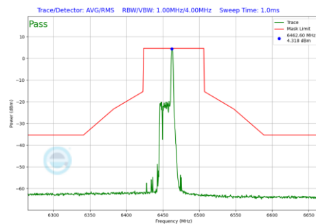
Plot 7-1161 In-Band Emission Plot CDD Diversity Antenna WF7 (80MHz BW 802.11be(RU) RU26 Index17 (UNII Band 6) - Ch.103)
