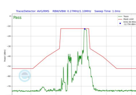
Plot 7-1229 In-Band Emission Plot SDM Diversity Antenna WF7 (20MHz BW 802.11be(RU) RU26 Index8 (UNII Band 7) - Ch.117)
