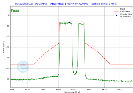
Plot 7-1272 In-Band Emission Plot SDM Diversity Antenna WF8 (80MHz BW 802.11be(RU) RU484+242 Index92 (UNII Band 7) - Ch.119)
