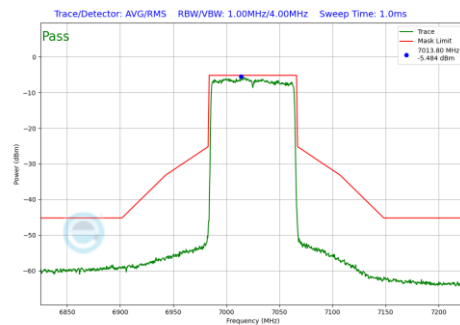
Plot 7-1153 In-Band Emission Plot SDM Primary Antenna WF8 (80MHz BW 802.11be(RU) RU996 Index67 (UNII Band 8) - Ch.215)
