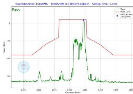
Plot 7-1156 In-Band Emission Plot CDD Diversity Antenna WF7 (40MHz BW 802.11be(RU) RU26 Index17 (UNII Band 5) - Ch.91)
