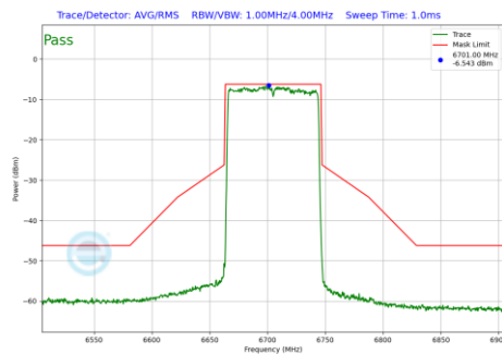
Plot 7-1303 In-Band Emission Plot SDM Diversity Antenna WF8 (80MHz BW 802.11be(RU) RU996 Index67 (UNII Band 7) - Ch.151)
