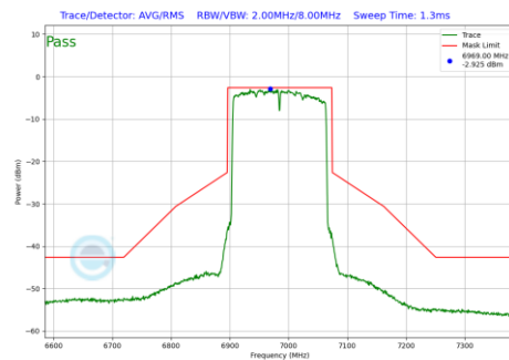
Plot 7-1154 In-Band Emission Plot SDM Primary Antenna WF8 (160MHz BW 802.11be(RU) RU996X2 Index68 (UNII Band 8) - Ch.207)
