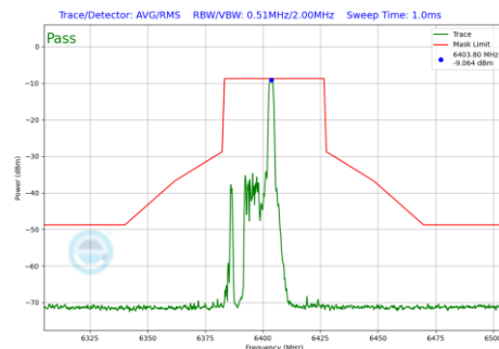
Plot 7-1238 In-Band Emission Plot SDM Diversity Antenna WF8 (40MHz BW 802.11be(RU) RU26 Index8 (UNII Band 5) - Ch.91)
