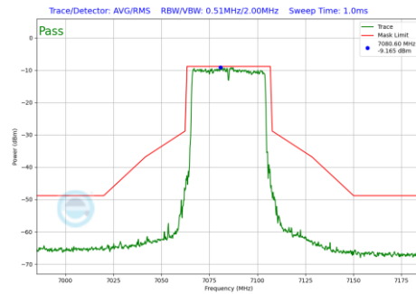
Plot 7-1290 In-Band Emission Plot SDM Diversity Antenna WF7 (40MHz BW 802.11be(RU) RU484 Index65 (UNII Band 8) - Ch.227)
