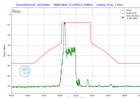
Plot 7-1242 In-Band Emission Plot SDM Diversity Antenna WF8 (40MHz BW 802.11be(RU) RU26 Index0 (UNII Band 6) - Ch.115)
