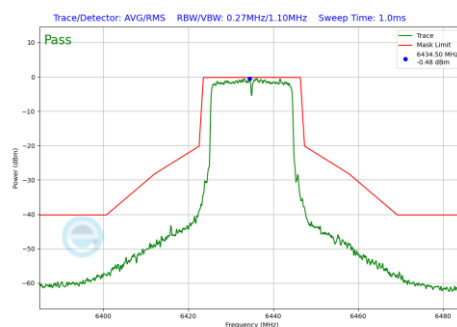
Plot 7-1201 In-Band Emission Plot CDD Diversity Antenna WF7 (20MHz BW 802.11be(RU) RU242 Index61 (UNII Band 6) - Ch.97)
