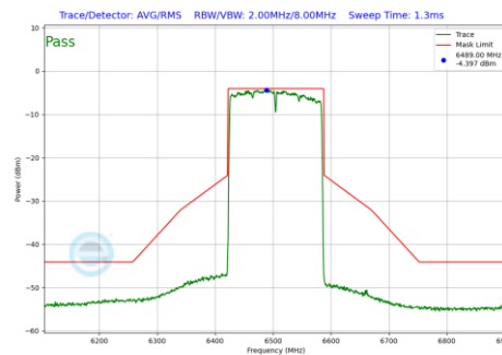
Plot 7-1300 In-Band Emission Plot SDM Diversity Antenna WF8 (160MHz BW 802.11be(RU) RU996X2 Index68 (UNII Band 6) - Ch.111)
