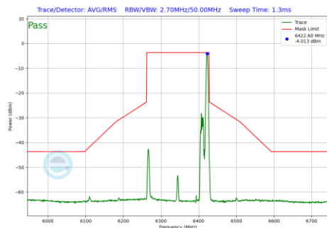
Plot 7-1240 In-Band Emission Plot SDM Diversity Antenna WF8 (160MHz BW 802.11be(RU) RU26 Index36 (UNII Band 5) - Ch.79)
