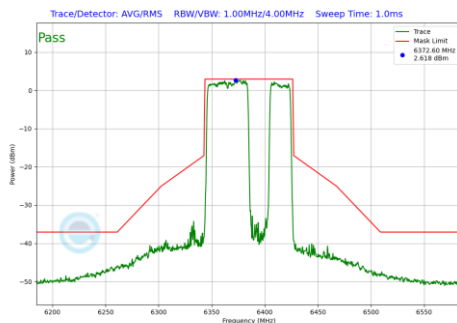
Plot 7-1189 In-Band Emission Plot CDD Diversity Antenna WF8 (80MHz BW 802.11be(RU) RU484+242 Index92 (UNII Band 5) - Ch.87)
