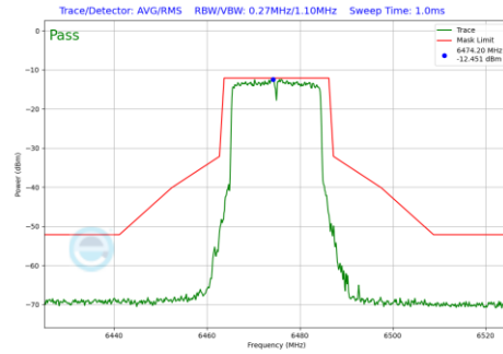
Plot 7-1297 In-Band Emission Plot SDM Diversity Antenna WF8 (20MHz BW 802.11be(RU) RU242 Index61 (UNII Band 6) - Ch.105)
