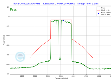
Plot 7-1258 In-Band Emission Plot SDM Diversity Antenna WF7 (160MHz BW 802.11be(RU) RU996+484+242 Index99 (UNII Band 6) - Ch.111)
