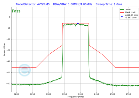
Plot 7-1295 In-Band Emission Plot SDM Diversity Antenna WF8 (80MHz BW 802.11be(RU) RU996 Index67 (UNII Band 5) - Ch.87)
