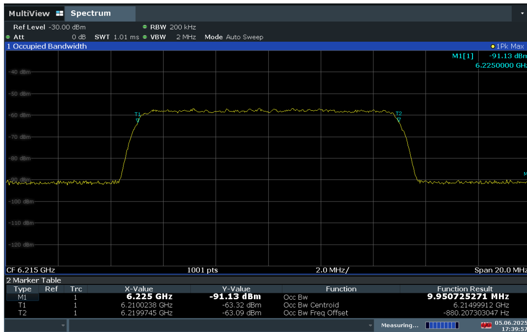
Plot 7-1309. AWGN Signal – UNII 5 – 20MHz
