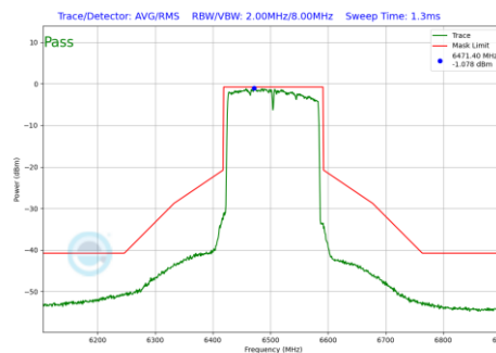
Plot 7-1204 In-Band Emission Plot CDD Diversity Antenna WF7 (160MHz BW 802.11be(RU) RU996X2 Index68 (UNII Band 6) - Ch.111)
