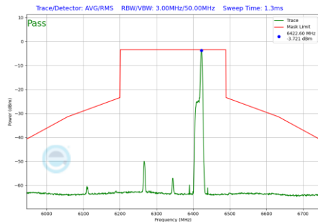
Plot 7-1224 In-Band Emission Plot SDM Diversity Antenna WF7 (160MHz BW 802.11be(RU) RU26 Index36 (UNII Band 5) - Ch.79)
