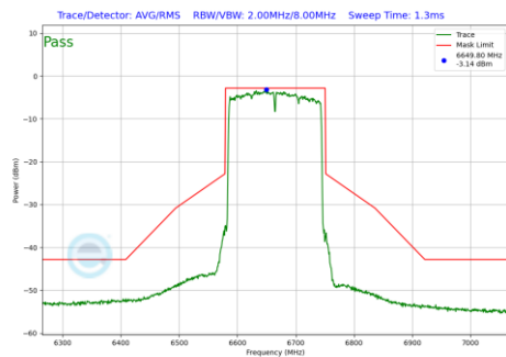
Plot 7-1304 In-Band Emission Plot SDM Diversity Antenna WF8 (160MHz BW 802.11be(RU) RU996X2 Index68 (UNII Band 7) - Ch.143)
