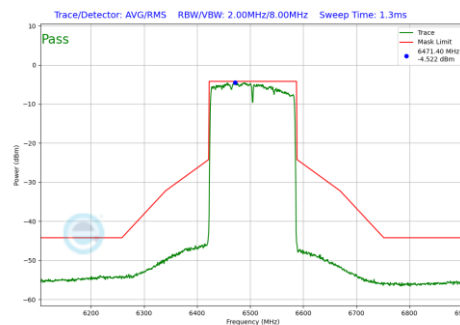
Plot 7-1284 In-Band Emission Plot SDM Diversity Antenna WF7 (160MHz BW 802.11be(RU) RU996X2 Index68 (UNII Band 6) - Ch.111)
