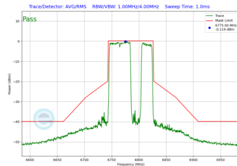
Plot 7-1186 In-Band Emission Plot CDD Diversity Antenna WF7 (80MHz BW 802.11be(RU) RU484+242 Index92 (UNII Band 7) - Ch.167)
