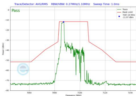
Plot 7-1233 In-Band Emission Plot SDM Diversity Antenna WF7 (20MHz BW 802.11be(RU) RU26 Index0 (UNII Band 8) - Ch.229)
