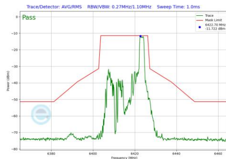
Plot 7-1237 In-Band Emission Plot SDM Diversity Antenna WF8 (20MHz BW 802.11be(RU) RU26 Index8 (UNII Band 5) - Ch.93)
