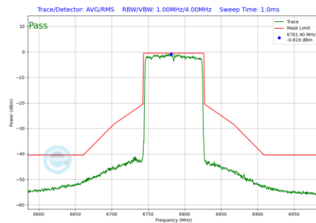
Plot 7-1219 In-Band Emission Plot CDD Diversity Antenna WF8 (80MHz BW 802.11be(RU) RU996 Index67 (UNII Band 7) - Ch.167)
