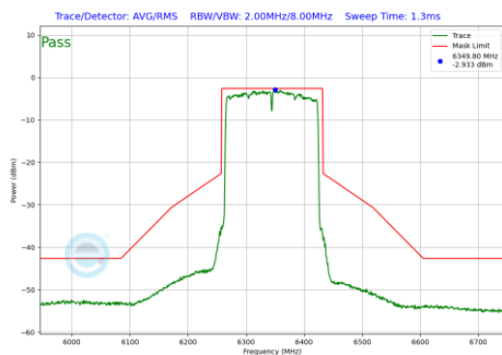
Plot 7-1280 In-Band Emission Plot SDM Diversity Antenna WF7 (160MHz BW 802.11be(RU) RU996X2 Index68 (UNII Band 5) - Ch.79)
