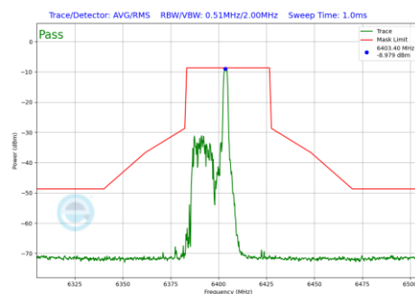
Plot 7-1222 In-Band Emission Plot SDM Diversity Antenna WF7 (40MHz BW 802.11be(RU) RU26 Index8 (UNII Band 5) - Ch.91)
