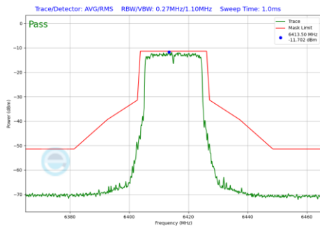
Plot 7-1277 In-Band Emission Plot SDM Diversity Antenna WF7 (20MHz BW 802.11be(RU) RU242 Index61 (UNII Band 5) - Ch.93)
