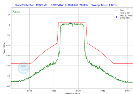
Plot 7-1197 In-Band Emission Plot CDD Diversity Antenna WF7 (20MHz BW 802.11be(RU) RU242 Index61 (UNII Band 5) - Ch.93)
