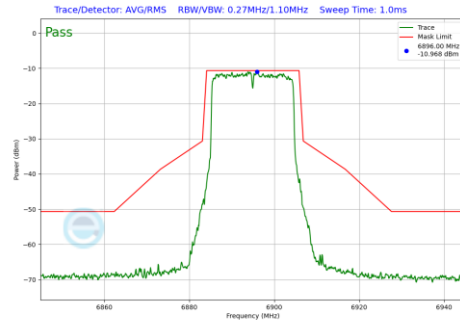
Plot 7-1289 In-Band Emission Plot SDM Diversity Antenna WF7 (20MHz BW 802.11be(RU) RU242 Index61 (UNII Band 8) - Ch.189)
