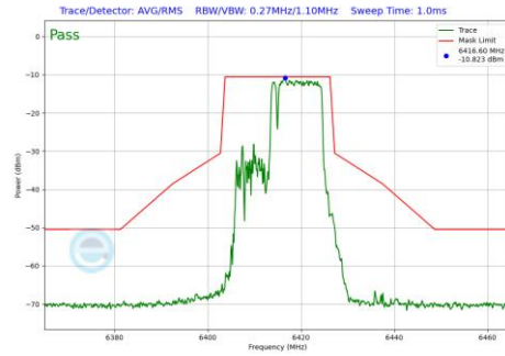
Plot 7-1265 In-Band Emission Plot SDM Diversity Antenna WF8 (20MHz BW 802.11be(RU) RU106+26 Index83 (UNII Band 5) - Ch.93)
