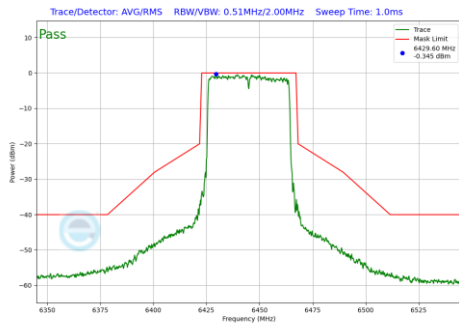
Plot 7-1214 In-Band Emission Plot CDD Diversity Antenna WF8 (40MHz BW 802.11be(RU) RU484 Index65 (UNII Band 6) - Ch.99)
