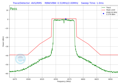
Plot 7-1206 In-Band Emission Plot CDD Diversity Antenna WF7 (40MHz BW 802.11be(RU) RU484 Index65 (UNII Band 7) - Ch.123)
