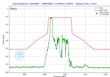
Plot 7-1249 In-Band Emission Plot SDM Diversity Antenna WF8 (20MHz BW 802.11be(RU) RU26 Index0 (UNII Band 8) - Ch.229)
