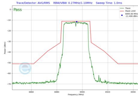
Plot 7-1151 In-Band Emission Plot SDM Primary Antenna WF8 (20MHz BW 802.11be(RU) RU242 Index61 (UNII Band 8) - Ch.189)
