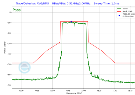
Plot 7-1306 In-Band Emission Plot SDM Diversity Antenna WF8 (40MHz BW 802.11be(RU) RU484 Index65 (UNII Band 8) - Ch.227)
