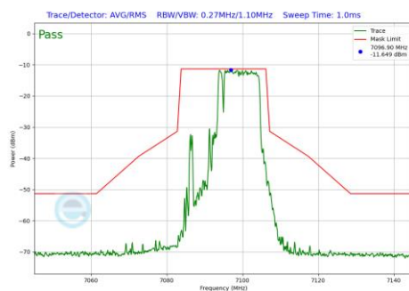
Plot 7-1262 In-Band Emission Plot SDM Diversity Antenna WF7 (20MHz BW 802.11be(RU) RU106+26 Index83 (UNII Band 8) - Ch.229)
