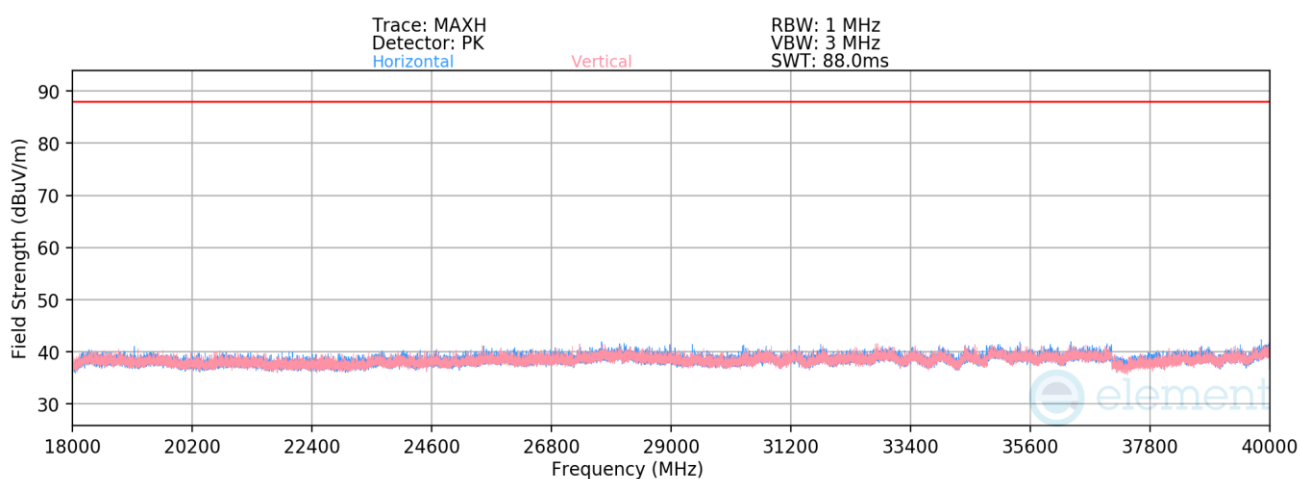
Plot 7-1394. Radiated Spurious Emissions 18-40GHz CDD Diversity (802.11be – Ch. 45 – RU242)
