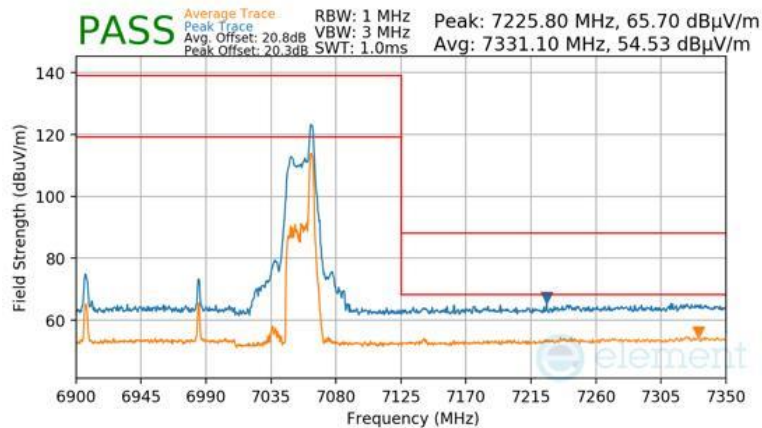
Plot 7-1443 Antenna WF5B Radiated Upper Band Edge (Peak & Average – UNII Band 8) - RU26
