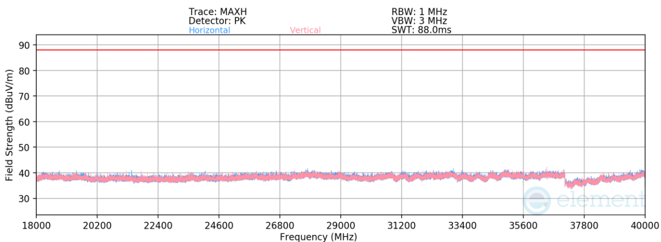
Plot 7-1402. Radiated Spurious Emissions 18-40GHz CDD Diversity (802.11be – Ch. 149 – RU242)
