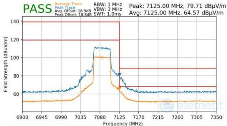
Plot 7-1487 Antenna WF8 Radiated Upper Band Edge (Peak & Average – UNII Band 8) - RU484
