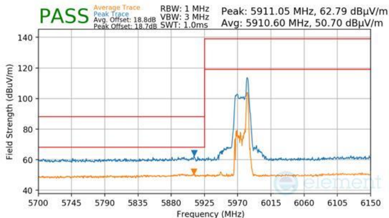
Plot 7-1421 Antenna WF5B Radiated Lower Band Edge (Peak & Average – UNII Band 5) - RU26
