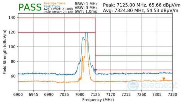
Plot 7-1415 Antenna WF5B Radiated Upper Band Edge (Peak & Average – UNII Band 8) - RU52+26
