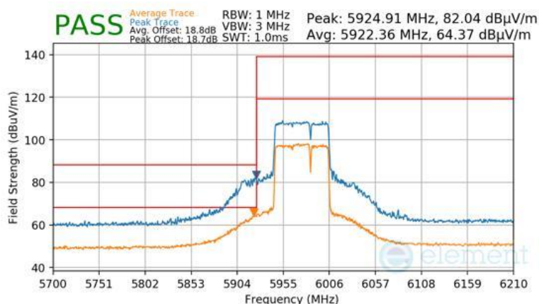
Plot 7-1495 Antenna WF8 Radiated Lower Band Edge (Peak & Average – UNII Band 5) - RU484+242
