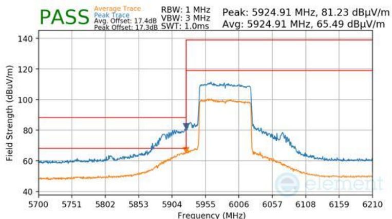
Plot 7-1438 Antenna WF5B Radiated Lower Band Edge (Peak & Average – UNII Band 5) - RU996
