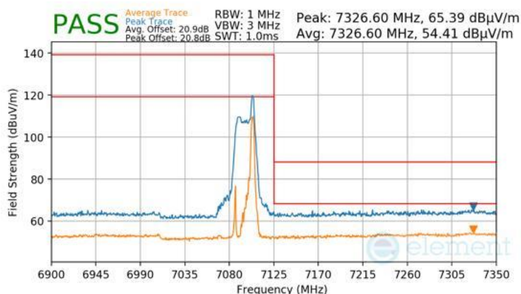
Plot 7-1473 Antenna WF8 Radiated Upper Band Edge (Peak & Average – UNII Band 8) - RU26
