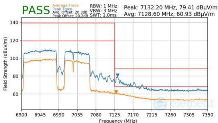
Plot 7-1461 Antenna WF5B Radiated Upper Band Edge (Peak & Average – UNII Band 8) - RU996+484+242 (H)
