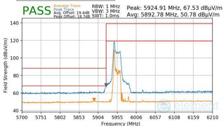
Plot 7-1488 Antenna WF8 Radiated Lower Band Edge (Peak & Average – UNII Band 5) - RU26
