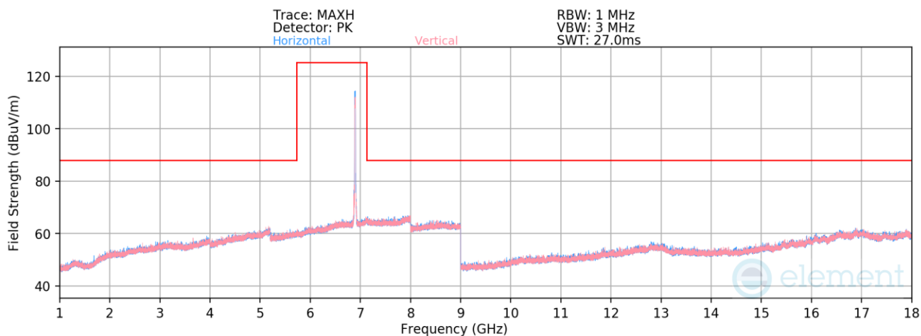
Plot 7-1404. Radiated Spurious Emissions above 1GHz CDD Diversity (802.11be – Ch. 189 – RU242)
