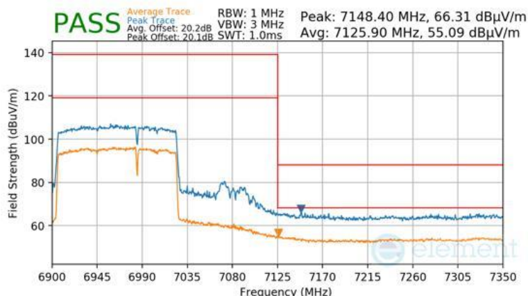
Plot 7-1450 Antenna WF5B Radiated Upper Band Edge (Peak & Average – UNII Band 8) - RU996+484 (H)
