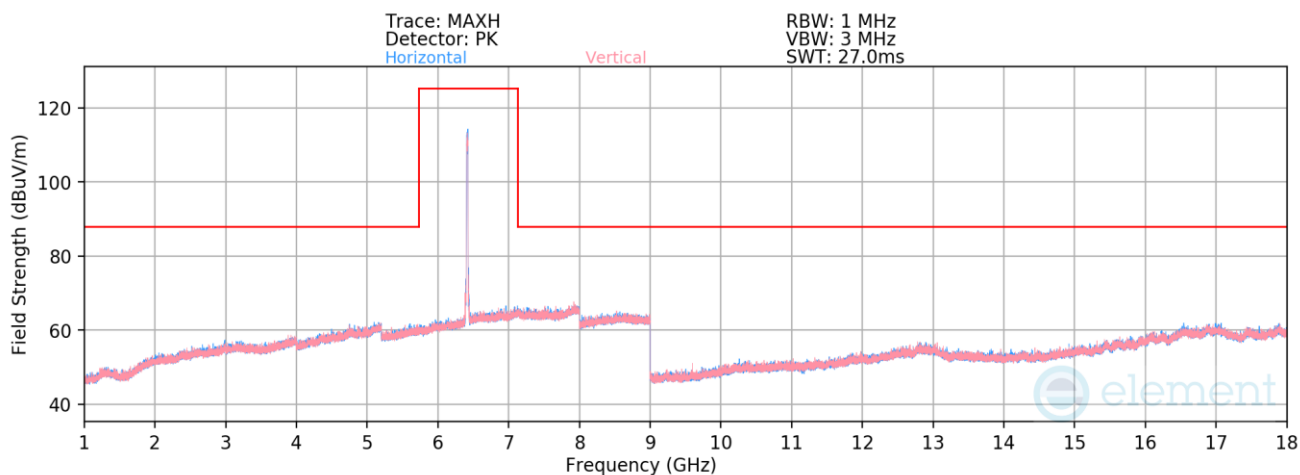
Plot 7-1395. Radiated Spurious Emissions above 1GHz CDD Diversity (802.11be – Ch. 93 – RU242)
