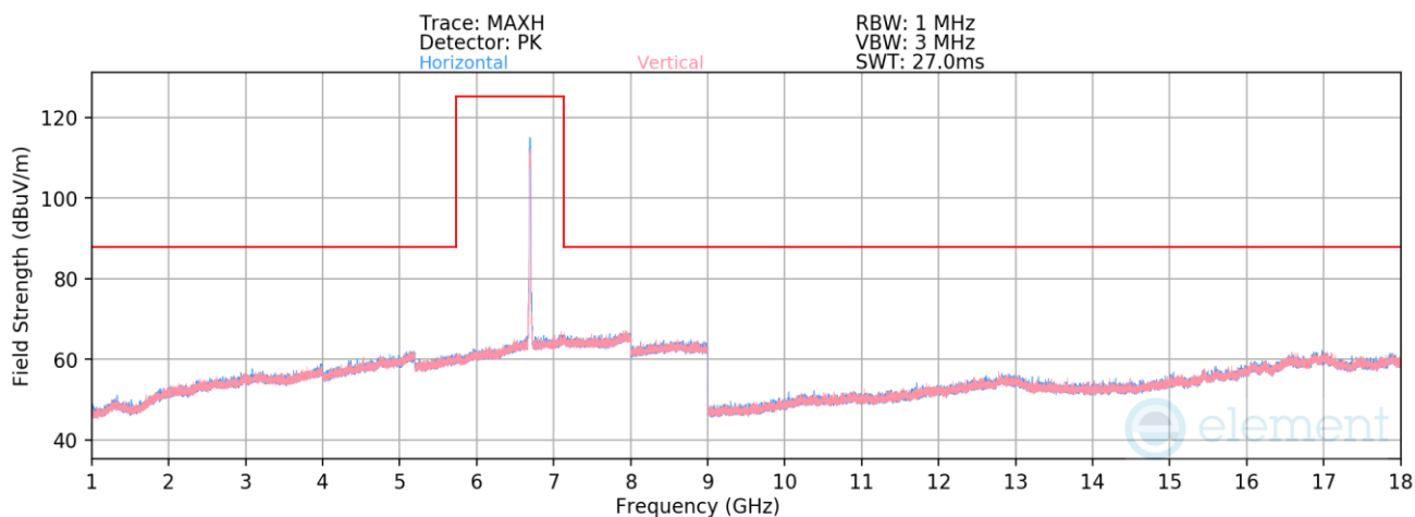
Plot 7-1401. Radiated Spurious Emissions above 1GHz CDD Diversity (802.11be – Ch. 149 – RU242)
