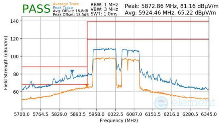
Plot 7-1452 Antenna WF5B Radiated Lower Band Edge (Peak & Average – UNII Band 5) - RU996+484+242 (H)
