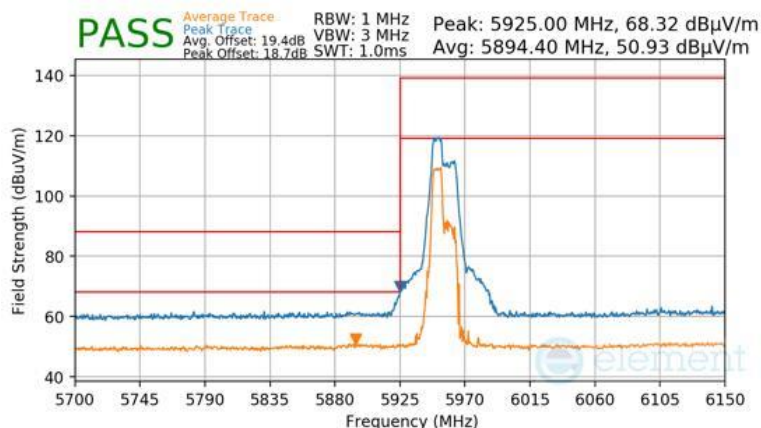
Plot 7-1412 Antenna WF5B Radiated Lower Band Edge (Peak & Average – UNII Band 5) - RU52+26
