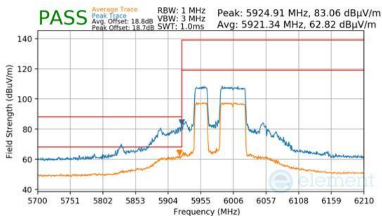
Plot 7-1493 Antenna WF8 Radiated Lower Band Edge (Peak & Average – UNII Band 5) - RU484+242
