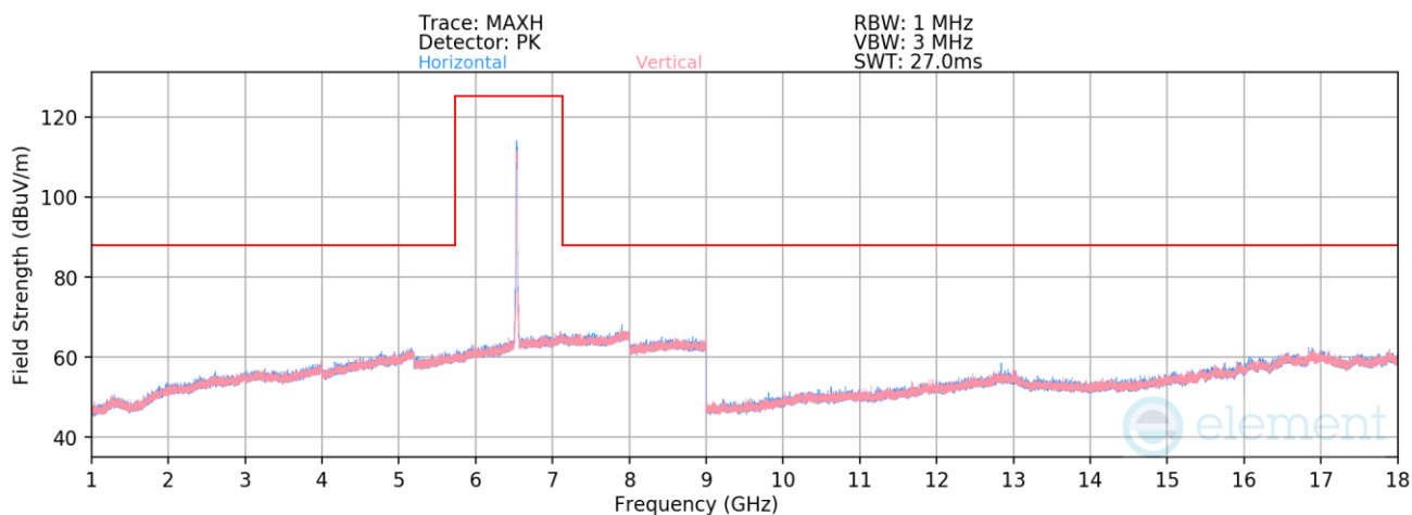
Plot 7-1400. Radiated Spurious Emissions above 1GHz CDD Diversity (802.11be – Ch. 117 – RU242)
