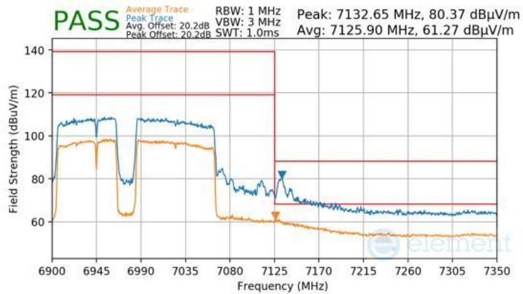
Plot 7-1466 Antenna WF5B Radiated Upper Band Edge (Peak & Average – UNII Band 8) - RU996+484+242 (L)
