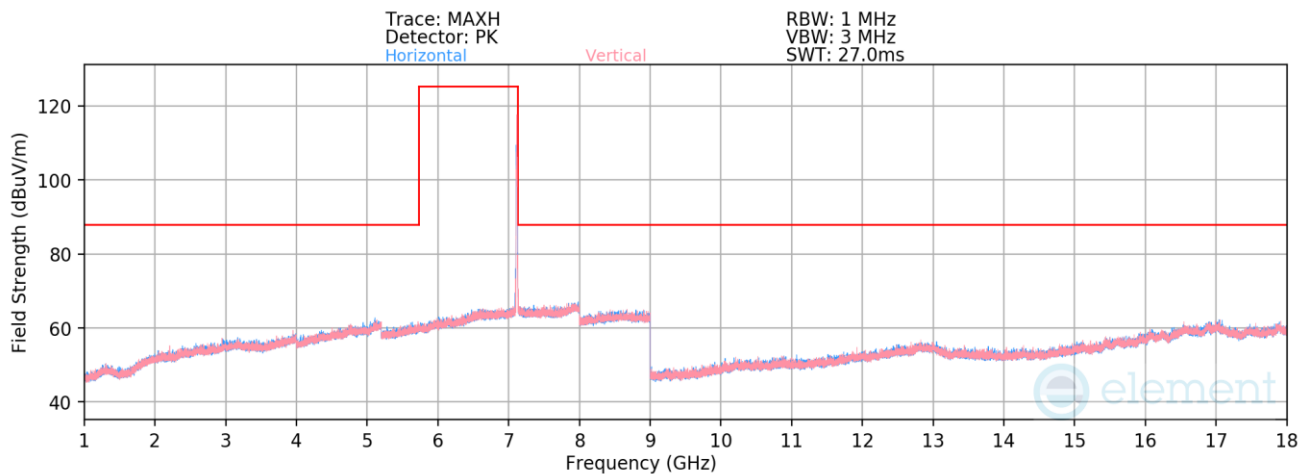
Plot 7-1391. Radiated Spurious Emissions above 1GHz CDD Diversity (802.11be – Ch. 229 – RU26)
