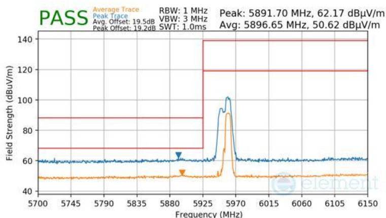
Plot 7-1475 Antenna WF8 Radiated Lower Band Edge (Peak & Average – UNII Band 5) - RU52+26
