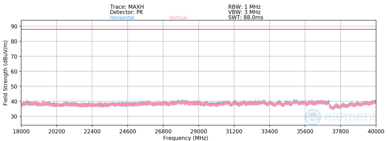
Plot 7-1398. Radiated Spurious Emissions 18-40GHz CDD Diversity (802.11be – Ch. 105 – RU242)
