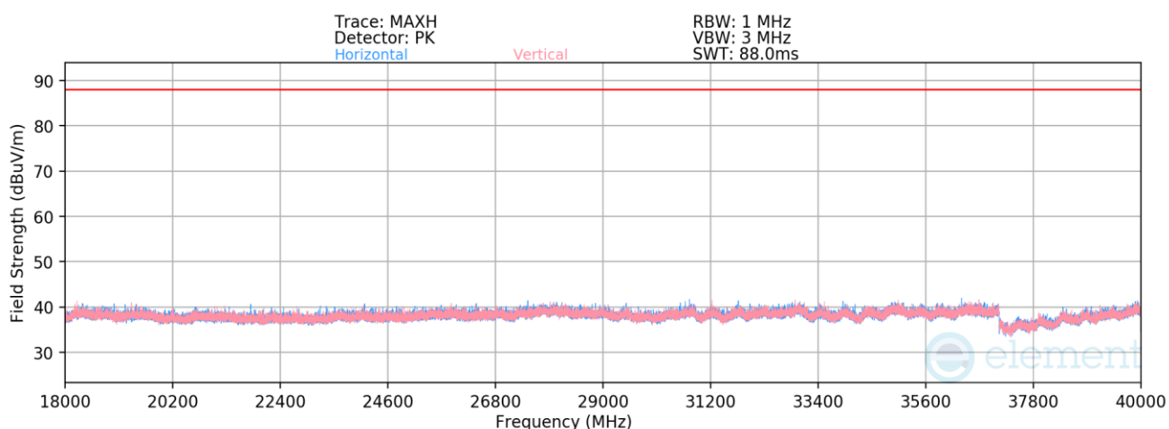
Plot 7-1386. Radiated Spurious Emissions 18-40GHz CDD Diversity (802.11be – Ch. 149 – RU26)
