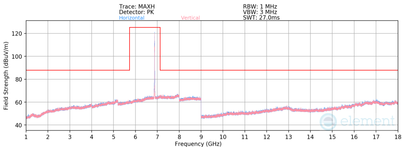
Plot 7-1387. Radiated Spurious Emissions above 1GHz CDD Diversity (802.11be – Ch. 185 – RU26)
