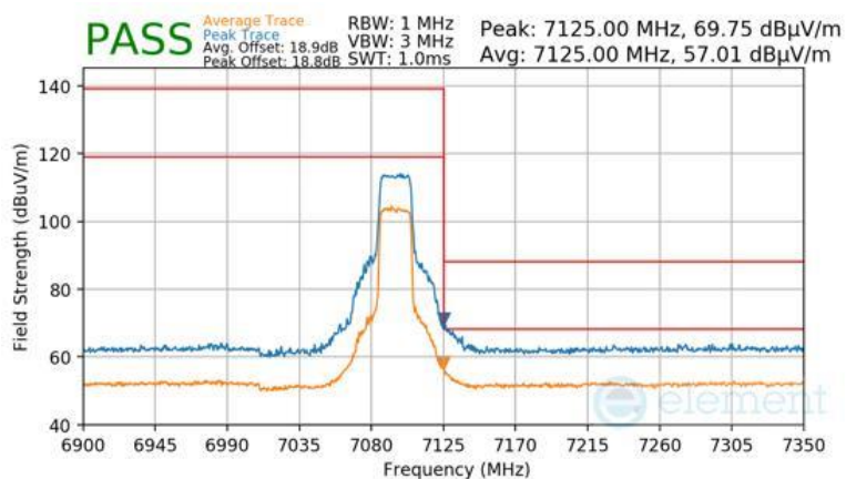
Plot 7-1479 Antenna WF8 Radiated Upper Band Edge (Peak & Average – UNII Band 8) - RU242
