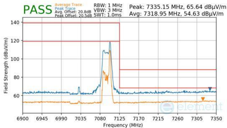
Plot 7-1485 Antenna WF8 Radiated Upper Band Edge (Peak & Average – UNII Band 8) - RU26
