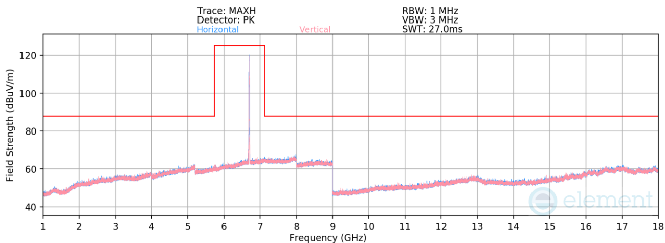
Plot 7-1385. Radiated Spurious Emissions above 1GHz CDD Diversity (802.11be – Ch. 149 – RU26)
