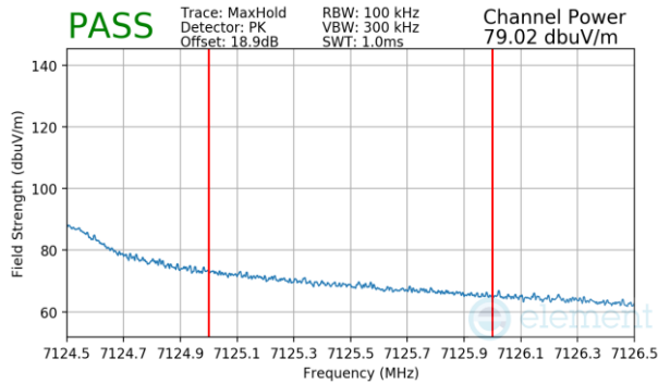
Plot 7-1480 Antenna WF8 Radiated Upper Band Edge (Peak – UNII Band 8)
