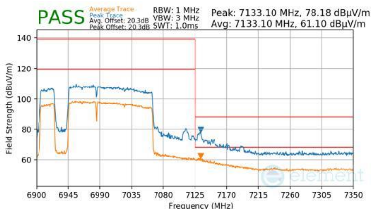
Plot 7-1462 Antenna WF5B Radiated Upper Band Edge (Peak & Average – UNII Band 8) - RU996+484+242 (L)
