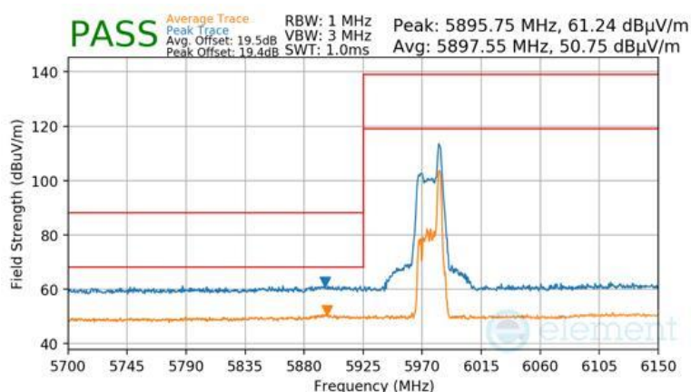
Plot 7-1483 Antenna WF8 Radiated Lower Band Edge (Peak & Average – UNII Band 5) - RU26
