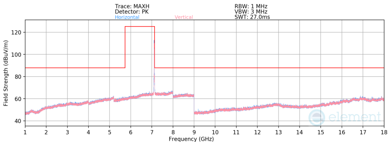
Plot 7-1407. Radiated Spurious Emissions above 1GHz CDD Diversity (802.11be – Ch. 233 – RU242)
