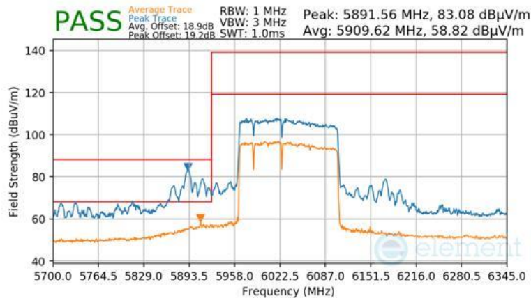
Plot 7-1453 Antenna WF5B Radiated Lower Band Edge (Peak & Average – UNII Band 5) - RU996+484+242 (L)
