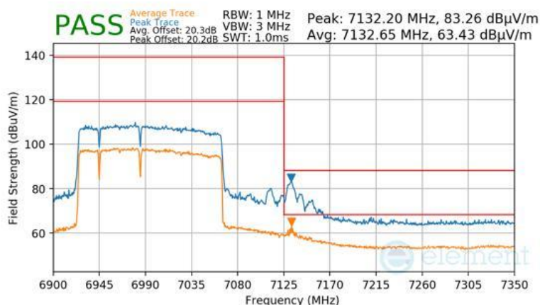
Plot 7-1460 Antenna WF5B Radiated Upper Band Edge (Peak & Average – UNII Band 8) - RU996+484+242 (L)
