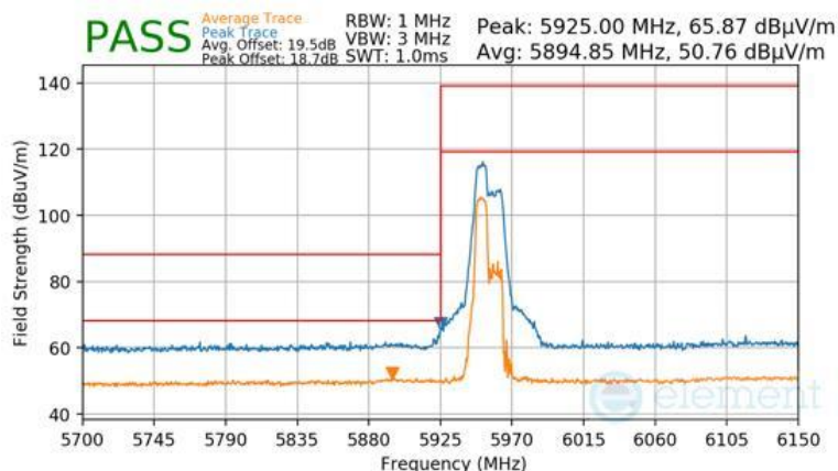
Plot 7-1474 Antenna WF8 Radiated Lower Band Edge (Peak & Average – UNII Band 5) - RU52+26
