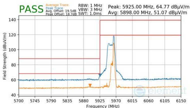
Plot 7-1471 Antenna WF8 Radiated Lower Band Edge (Peak & Average – UNII Band 5) - RU26
