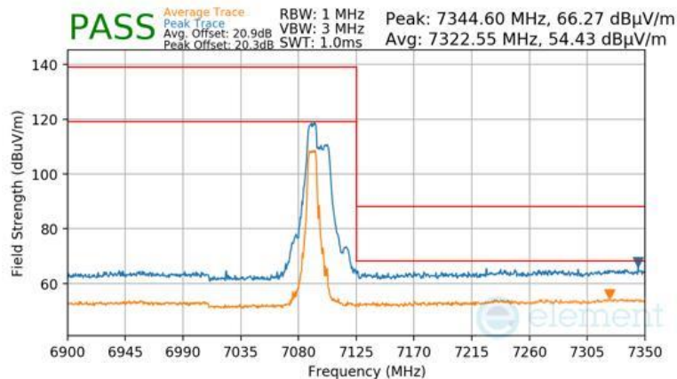
Plot 7-1414 Antenna WF5B Radiated Upper Band Edge (Peak & Average – UNII Band 8) - RU52+26
