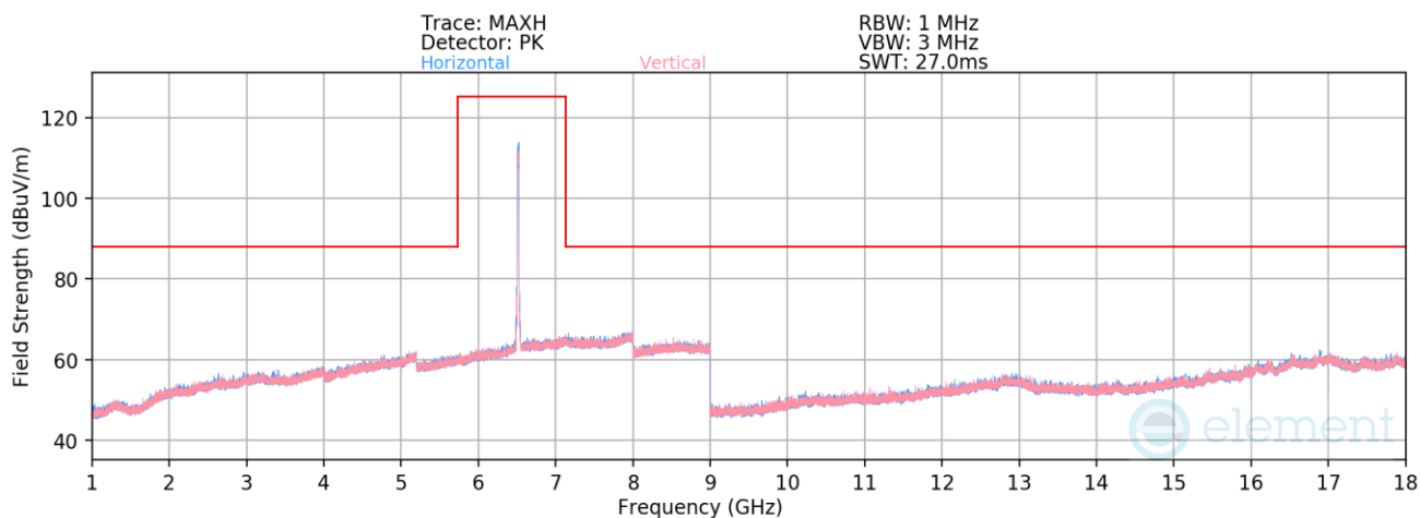
Plot 7-1399. Radiated Spurious Emissions above 1GHz CDD Diversity (802.11be – Ch. 113 – RU242)
