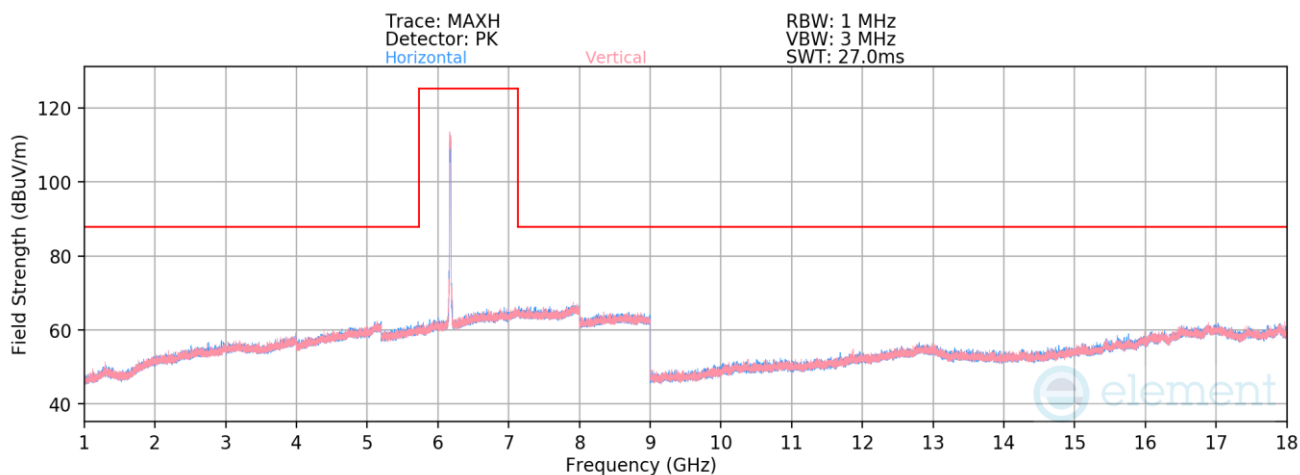
Plot 7-1393. Radiated Spurious Emissions above 1GHz CDD Diversity (802.11be – Ch. 45 – RU242)
