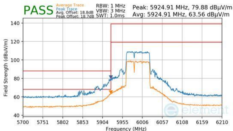
Plot 7-1492 Antenna WF8 Radiated Lower Band Edge (Peak & Average – UNII Band 5) - RU484+242
