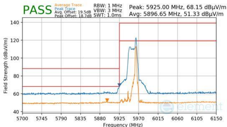
Plot 7-1409 Antenna WF5B Radiated Lower Band Edge (Peak & Average – UNII Band 5) - RU26
