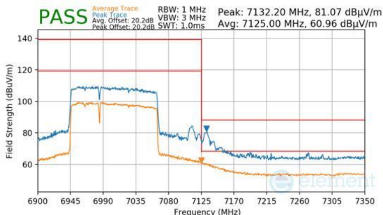
Plot 7-1448 Antenna WF5B Radiated Upper Band Edge (Peak & Average – UNII Band 8) - RU996+484 (L)
