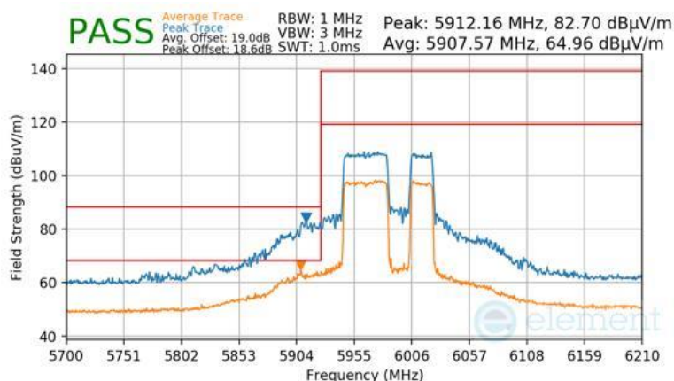
Plot 7-1494 Antenna WF8 Radiated Lower Band Edge (Peak & Average – UNII Band 5) - RU484+242
