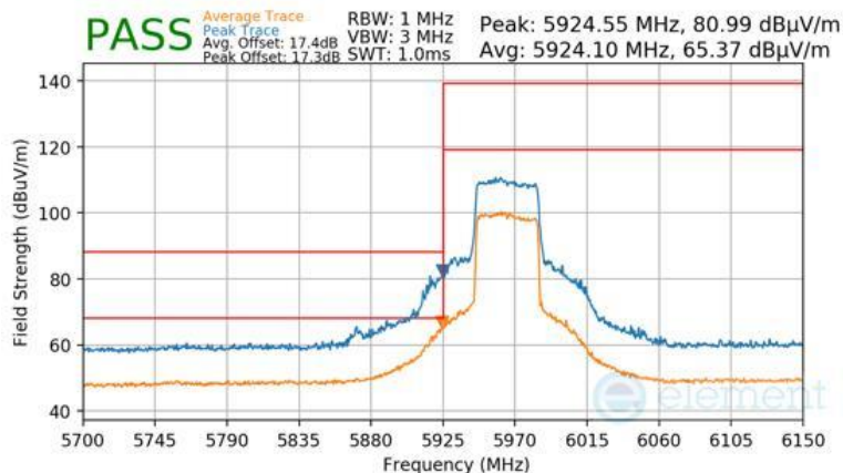
Plot 7-1486 Antenna WF8 Radiated Lower Band Edge (Peak & Average – UNII Band 5) - RU484
