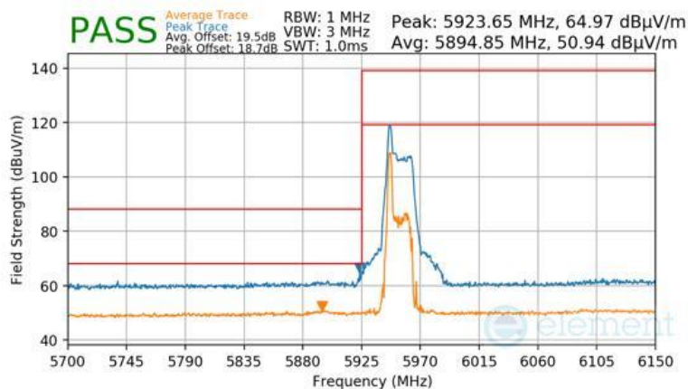
Plot 7-1470 Antenna WF8 Radiated Lower Band Edge (Peak & Average – UNII Band 5) - RU26
