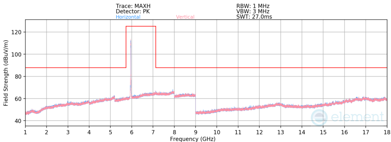
Plot 7-1392. Radiated Spurious Emissions above 1GHz CDD Diversity (802.11be – Ch. 1 – RU242)
