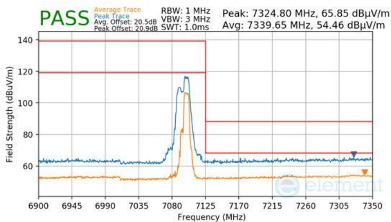
Plot 7-1477 Antenna WF8 Radiated Upper Band Edge (Peak & Average – UNII Band 8) - RU52+26
