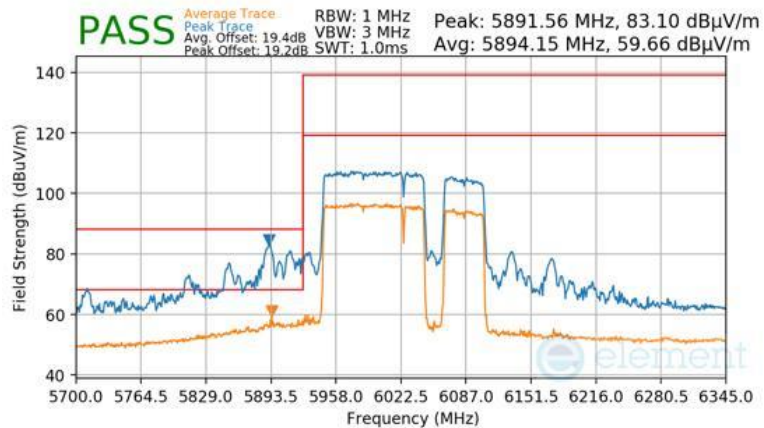
Plot 7-1455 Antenna WF5B Radiated Lower Band Edge (Peak & Average – UNII Band 5) - RU996+484+242 (H)
