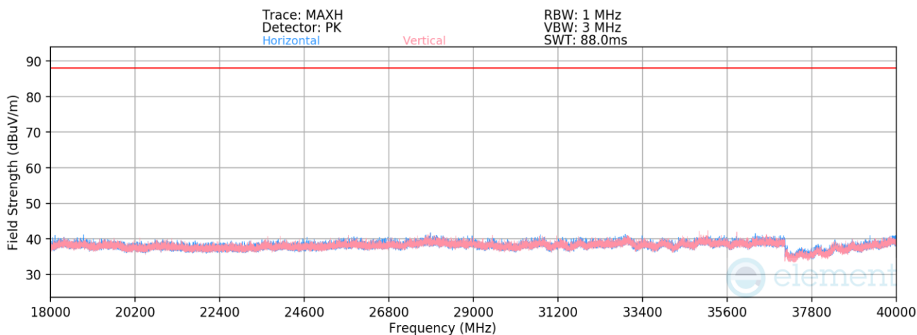
Plot 7-1406. Radiated Spurious Emissions 18-40GHz CDD Diversity (802.11be – Ch. 209 – RU242)
