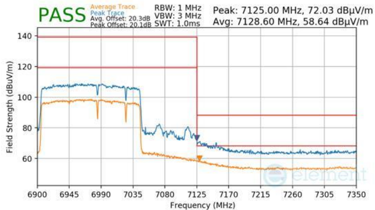
Plot 7-1467 Antenna WF5B Radiated Upper Band Edge (Peak & Average – UNII Band 8) - RU996+484+242 (H)
