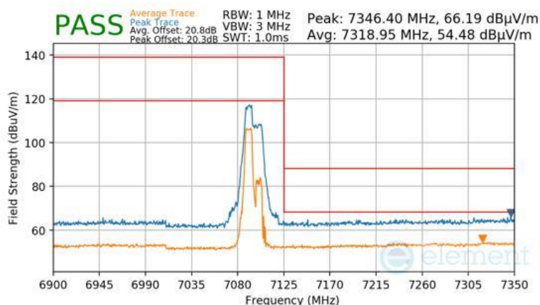
Plot 7-1476 Antenna WF8 Radiated Upper Band Edge (Peak & Average – UNII Band 8) - RU52+26
