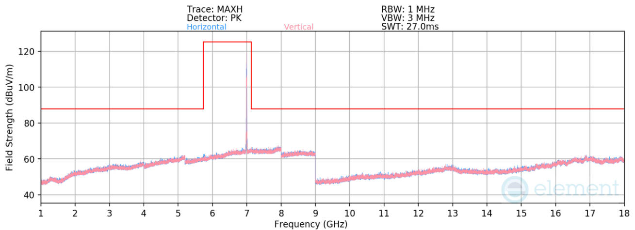
Plot 7-1389. Radiated Spurious Emissions above 1GHz CDD Diversity (802.11be – Ch. 209 – RU26)
