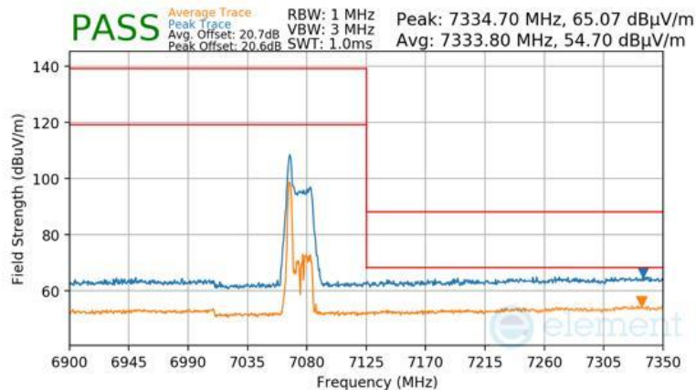
Plot 7-1484 Antenna WF8 Radiated Upper Band Edge (Peak & Average – UNII Band 8) - RU26
