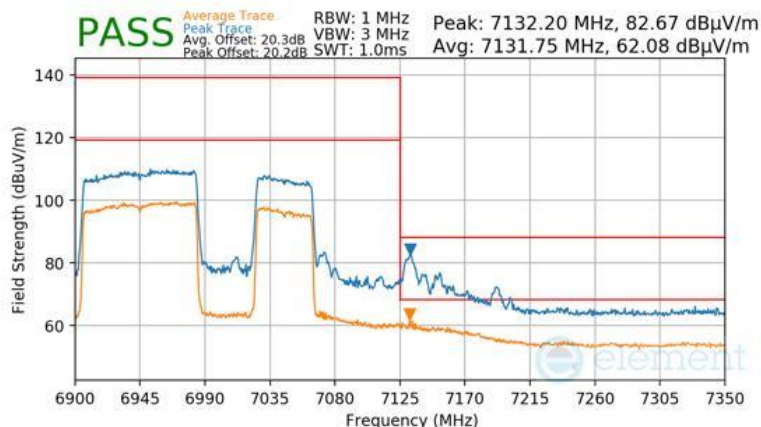
Plot 7-1449 Antenna WF5B Radiated Upper Band Edge (Peak & Average – UNII Band 8) - RU996+484 (H)
