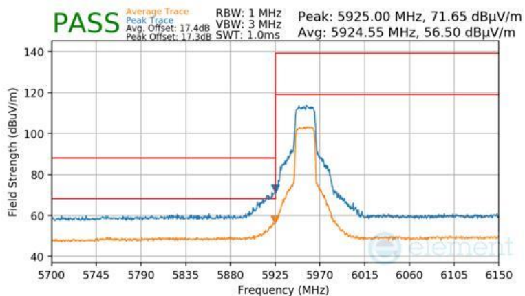
Plot 7-1478 Antenna WF8 Radiated Lower Band Edge (Peak & Average – UNII Band 5) - RU242
