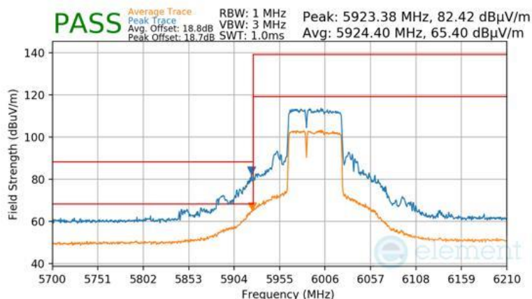
Plot 7-1430 Antenna WF5B Radiated Lower Band Edge (Peak & Average – UNII Band 5) - RU484+242
