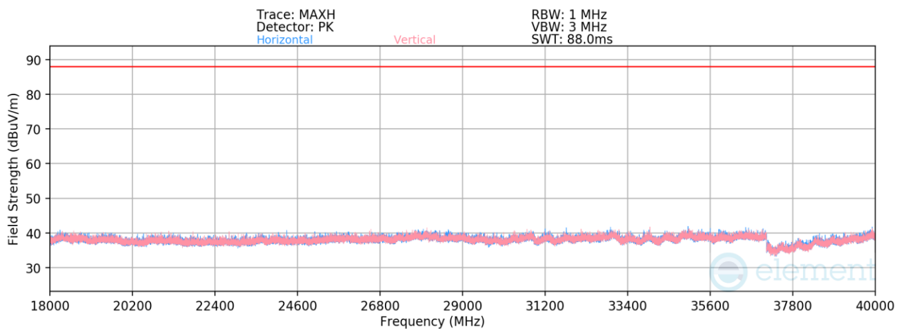
Plot 7-1390. Radiated Spurious Emissions 18-40GHz CDD Diversity (802.11be – Ch. 209 – RU26)
