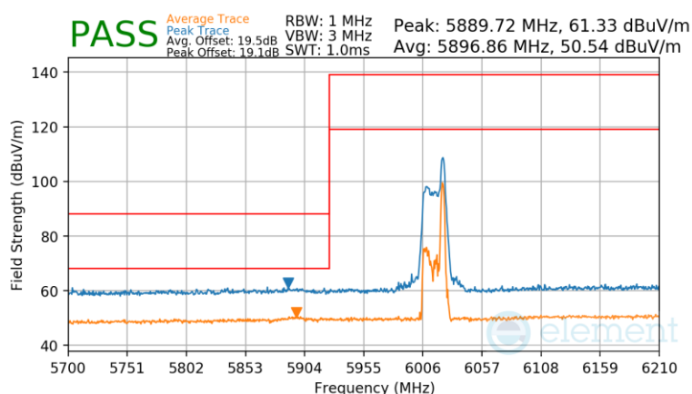
Plot 7-1489 Antenna WF8 Radiated Lower Band Edge (Peak & Average – UNII Band 5) - RU26
