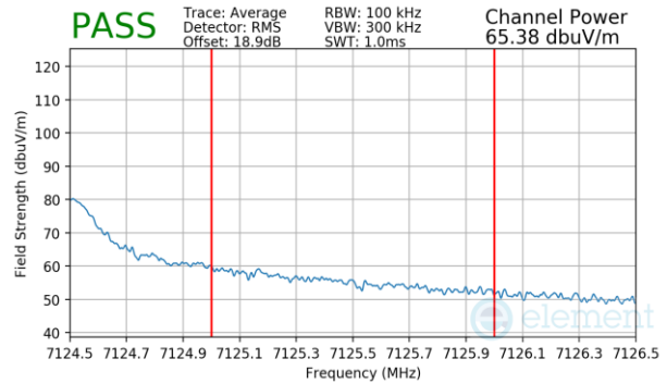
Plot 7-1481 Antenna WF8 Radiated Upper Band Edge (Average – UNII Band 8)
