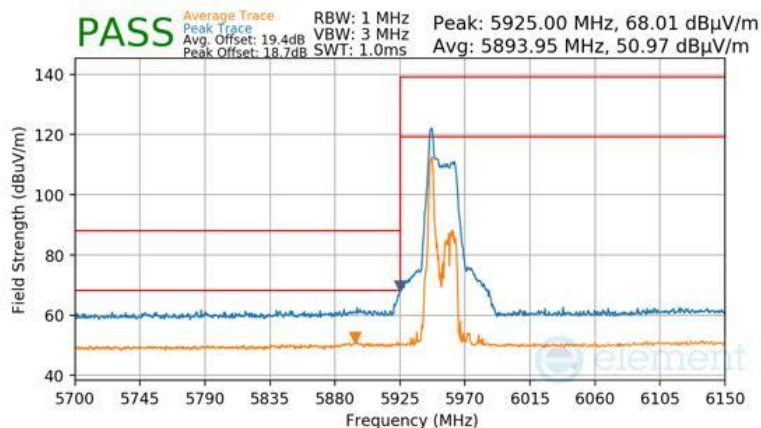
Plot 7-1408 Antenna WF5B Radiated Lower Band Edge (Peak & Average – UNII Band 5) - RU26
