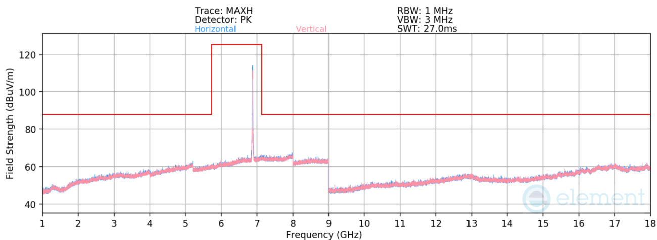
Plot 7-1403. Radiated Spurious Emissions above 1GHz CDD Diversity (802.11be – Ch. 185 – RU242)
