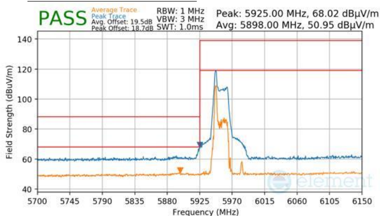
Plot 7-1482 Antenna WF8 Radiated Lower Band Edge (Peak & Average – UNII Band 5) - RU26
