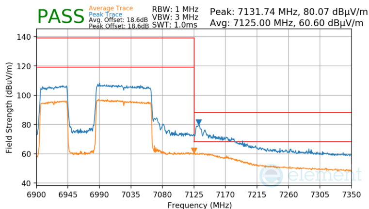
Plot 7-1451 Antenna WF5B Radiated Upper Band Edge (Peak & Average – UNII Band 8) - RU996+484 (L)
