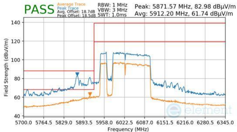
Plot 7-1454 Antenna WF5B Radiated Lower Band Edge (Peak & Average – UNII Band 5) - RU996+484+242 (L)
