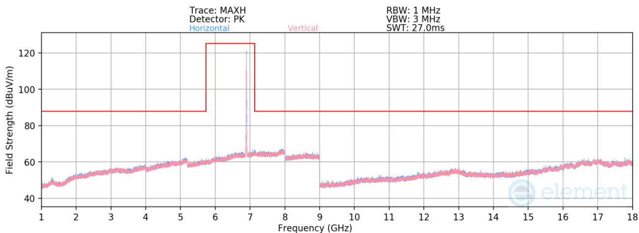
Plot 7-1388. Radiated Spurious Emissions above 1GHz CDD Diversity (802.11be – Ch. 189 – RU26)
