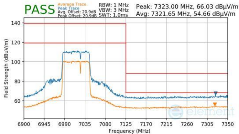
Plot 7-1437 Antenna WF5B Radiated Upper Band Edge (Peak & Average – UNII Band 8) - RU484+242
