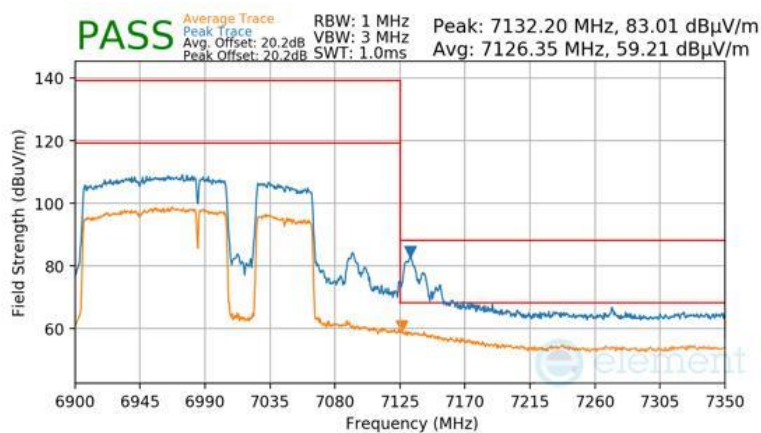
Plot 7-1463 Antenna WF5B Radiated Upper Band Edge (Peak & Average – UNII Band 8) - RU996+484+242 (H)
