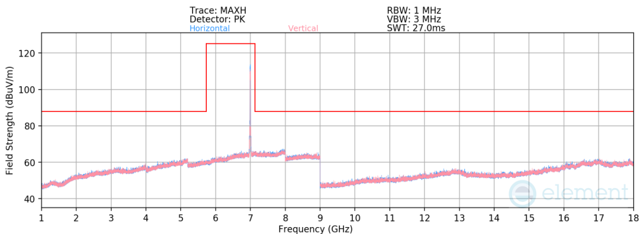
Plot 7-1405. Radiated Spurious Emissions above 1GHz CDD Diversity (802.11be – Ch. 209 – RU242)
