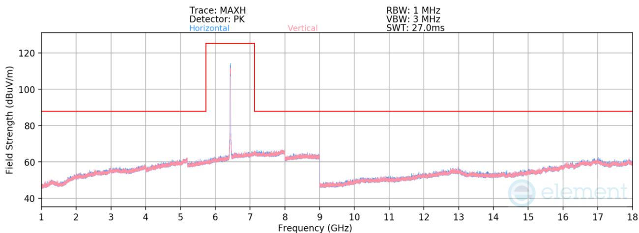
Plot 7-1396. Radiated Spurious Emissions above 1GHz CDD Diversity (802.11be – Ch. 97 – RU242)
