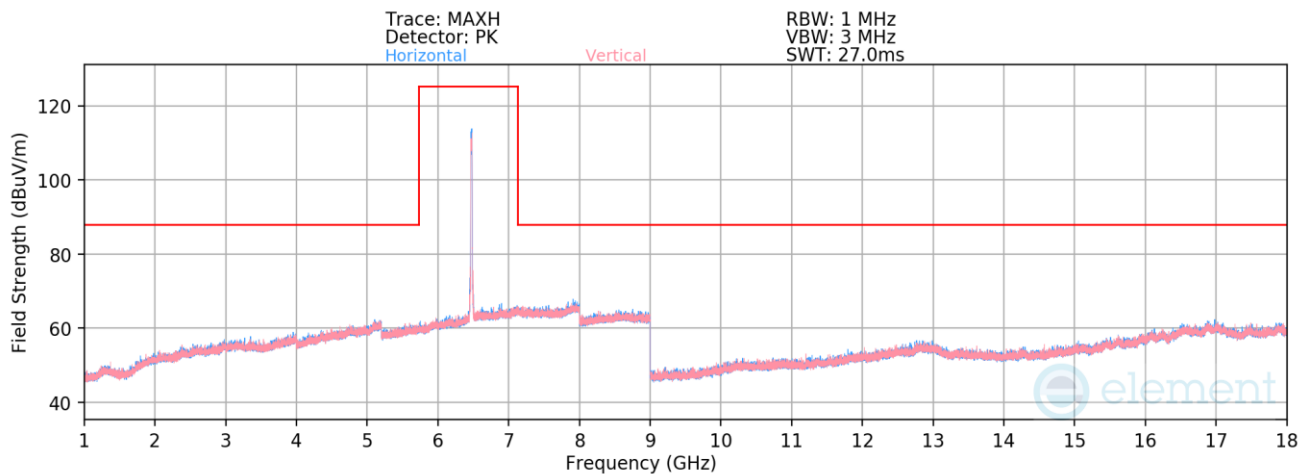
Plot 7-1397. Radiated Spurious Emissions above 1GHz CDD Diversity (802.11be – Ch. 105 – RU242)
