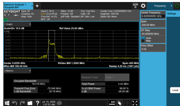
Plot 7-114 26dB BW & 99% OBW Antenna WF7 (160MHz BW 802.11be(RU) RU26 Index0 - Ch.175)
