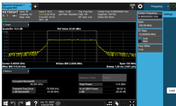
Plot 7-130 26dB BW & 99% OBW Antenna WF7 (40MHz BW 802.11be(RU) RU484 Index65 - Ch.187)
