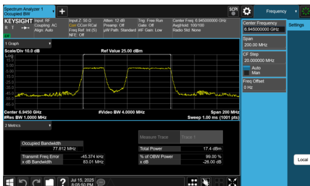
Plot 7-127 26dB BW & 99% OBW Antenna WF7 (80MHz BW 802.11be(RU) RU484+242 Index91 - Ch.199)
