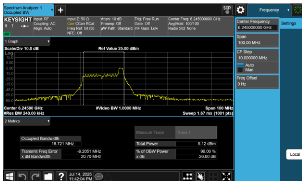
Plot 7-90 26dB BW & 99% OBW Antenna WF7 (40MHz BW 802.11be(RU) RU26 Index8 - Ch.59)
