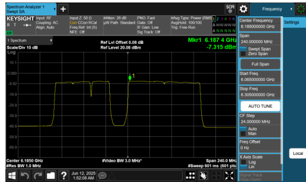
Plot 7-139 PSD Antenna WF5B (160MHz BW 802.11be(RU) RU996+484+242 Index99 - Ch.47)
