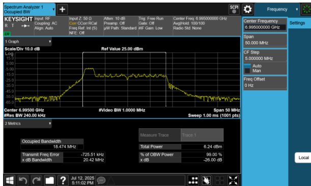
Plot 7-78 26dB BW & 99% OBW Antenna WF8 (20MHz BW 802.11be(RU) RU26 Index0 - Ch.209)
