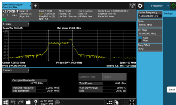
Plot 7-79 26dB BW & 99% OBW Antenna WF8 (40MHz BW 802.11be(RU) RU26 Index8 - Ch.227)
