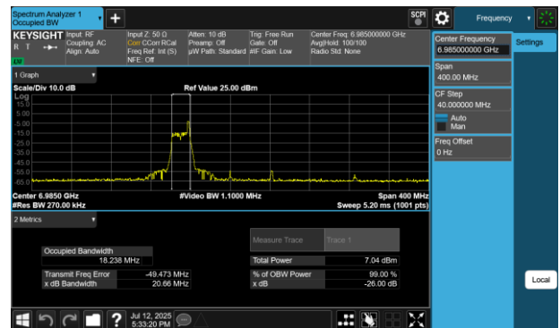
Plot 7-81 26dB BW & 99% OBW Antenna WF8 (160MHz BW 802.11be(RU) RU26 Index17 - Ch.207)
