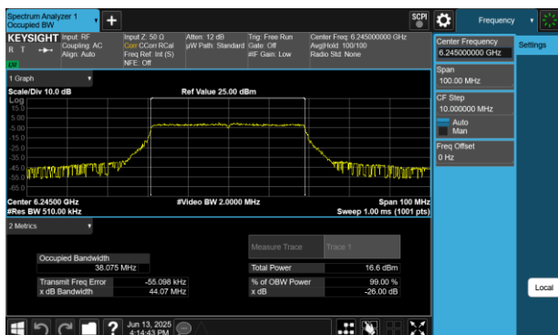
Plot 7-97 26dB BW & 99% OBW Antenna WF7 (40MHz BW 802.11be(RU) RU484 Index65 - Ch.59)
