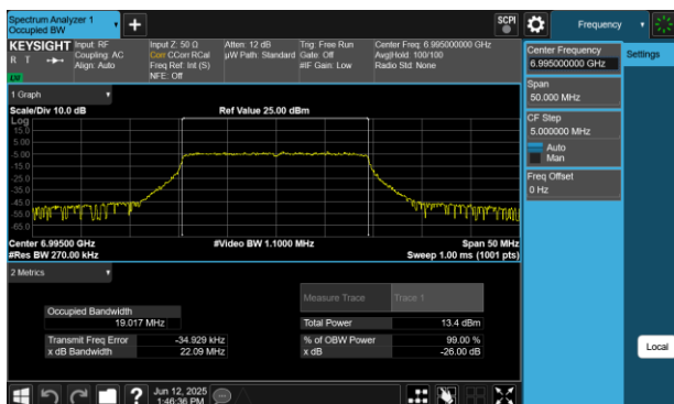
Plot 7-86 26dB BW & 99% OBW Antenna WF8 (20MHz BW 802.11be(RU) RU242 Index61 - Ch.209)
