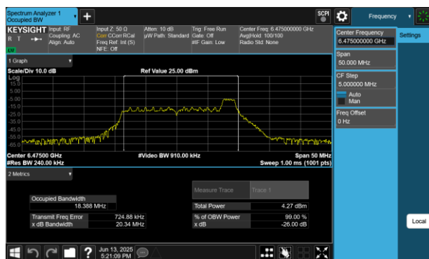
Plot 7-100 26dB BW & 99% OBW Antenna WF7 (20MHz BW 802.11be(RU) RU26 Index8 - Ch.105)
