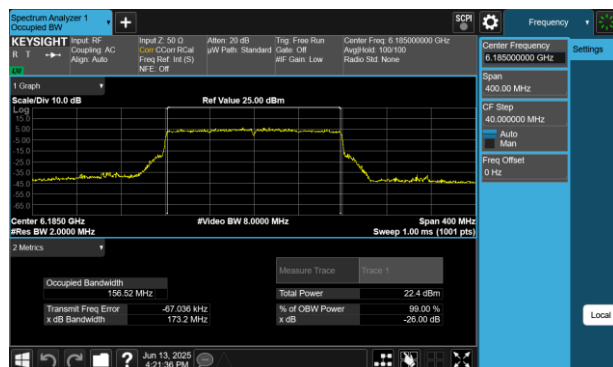
Plot 7-99 26dB BW & 99% OBW Antenna WF7 (160MHz BW 802.11be(RU) RU996X2 Index68 - Ch.47)
