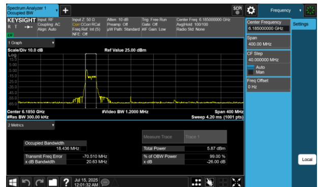
Plot 7-92 26dB BW & 99% OBW Antenna WF7 (160MHz BW 802.11be(RU) RU26 Index0 - Ch.47)
