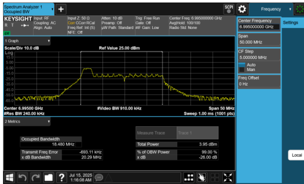
Plot 7-122 26dB BW & 99% OBW Antenna WF7 (20MHz BW 802.11be(RU) RU26 Index0 - Ch.209)
