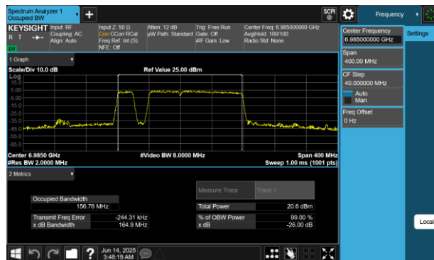
Plot 7-128 26dB BW & 99% OBW Antenna WF7 (160MHz BW 802.11be(RU) RU996+484+242 Index97 - Ch.207)
