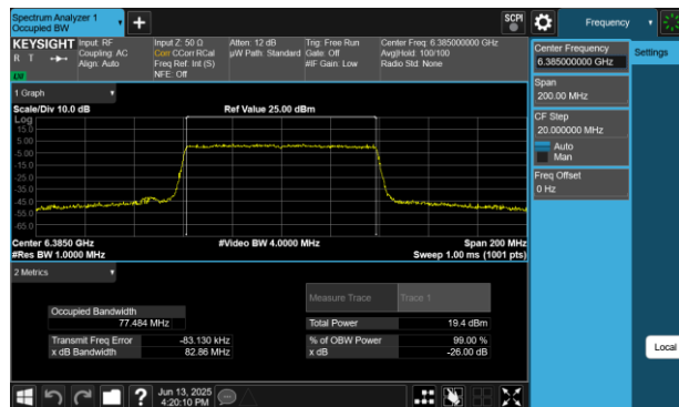
Plot 7-98 26dB BW & 99% OBW Antenna WF7 (80MHz BW 802.11be(RU) RU996 Index67 - Ch.87)
