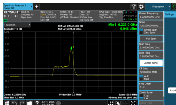
Plot 7-135 PSD Antenna WF5B (80MHz BW 802.11be(RU) RU26 Index17 - Ch.55)
