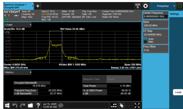
Plot 7-113 26dB BW & 99% OBW Antenna WF7 (80MHz BW 802.11be(RU) RU26 Index0 - Ch.183)
