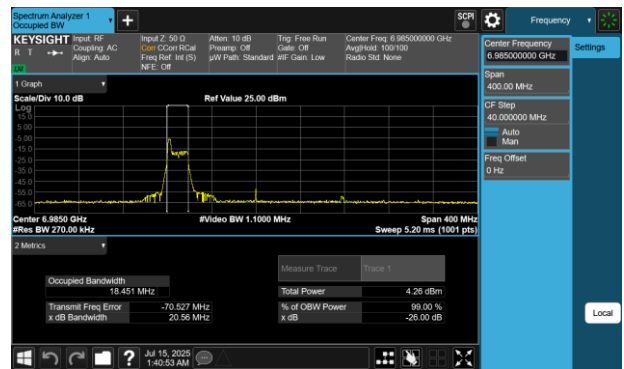
Plot 7-125 26dB BW & 99% OBW Antenna WF7 (160MHz BW 802.11be(RU) RU26 Index0 - Ch.207)
