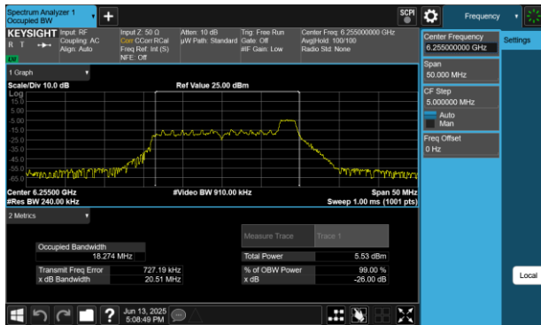
Plot 7-89 26dB BW & 99% OBW Antenna WF7 (20MHz BW 802.11be(RU) RU26 Index8 - Ch.61)
