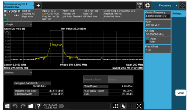
Plot 7-124 26dB BW & 99% OBW Antenna WF7 (80MHz BW 802.11be(RU) RU26 Index0 - Ch.199)
