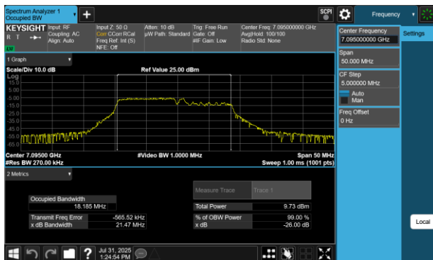
Plot 7-126 26dB BW & 99% OBW Antenna WF7 (20MHz BW 802.11be(RU) RU106+26 Index82 - Ch.229)
