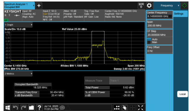
Plot 7-91 26dB BW & 99% OBW Antenna WF7 (80MHz BW 802.11be(RU) RU26 Index36 - Ch.39)
