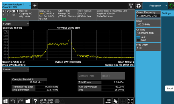
Plot 7-112 26dB BW & 99% OBW Antenna WF7 (40MHz BW 802.11be(RU) RU26 Index8 - Ch.155)
