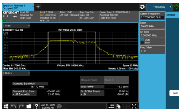
Plot 7-192 26dB BW & 99% OBW Antenna WF7 (20MHz BW 802.11be(RU) RU106+26 Index82 - Ch.45)
