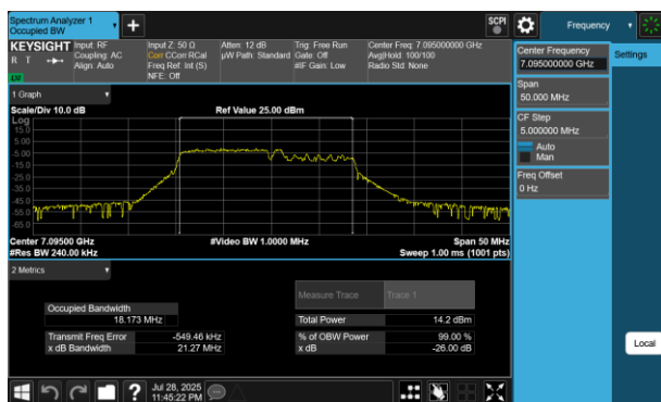
Plot 7-225 26dB BW & 99% OBW Antenna WF7 (20MHz BW 802.11be(RU) RU106+26 Index82 - Ch.229)
