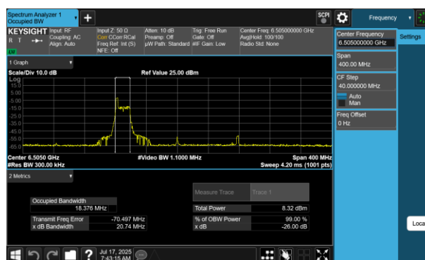
Plot 7-202 26dB BW & 99% OBW Antenna WF7 (160MHz BW 802.11be(RU) RU26 Index0 - Ch.111)
