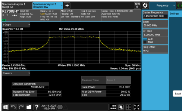
Plot 7-173 26dB BW & 99% OBW Antenna WF7 (20MHz BW 802.11be(RU) RU242 Index61 - Ch.97)
