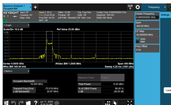
Plot 7-213 26dB BW & 99% OBW Antenna WF7 (160MHz BW 802.11be(RU) RU26 Index0 - Ch.143)
