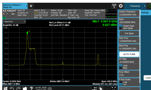
Plot 7-235 PSD Antenna WF5B (160MHz BW 802.11be(RU) RU26 Index0 - Ch.15)
