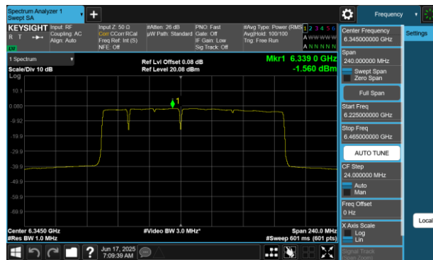
Plot 7-238 PSD Antenna WF5B (160MHz BW 802.11be(RU) RU996+484+242 Index96 - Ch.79)
