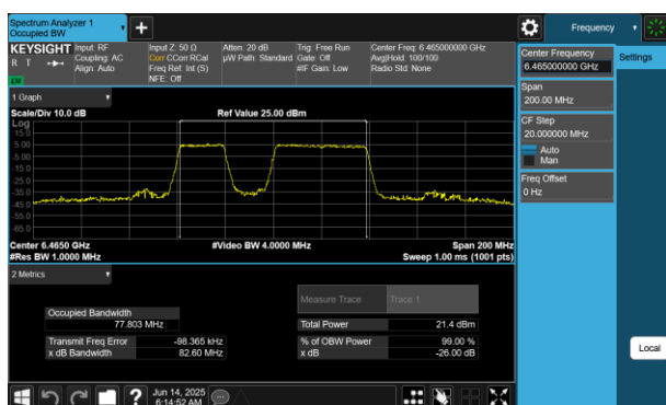
Plot 7-204 26dB BW & 99% OBW Antenna WF7 (80MHz BW 802.11be(RU) RU484+242 Index91 - Ch.103)
