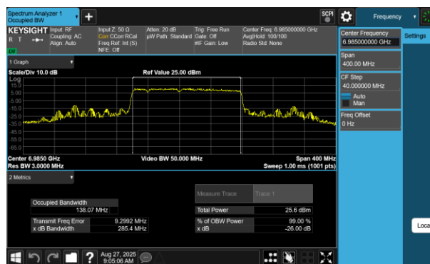
Plot 7-227 26dB BW & 99% OBW Antenna WF7 (160MHz BW 802.11be(RU) RU996+484+242 Index96 - Ch.207)
