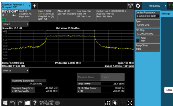
Plot 7-174 26dB BW & 99% OBW Antenna WF7 (40MHz BW 802.11be(RU) RU484 Index65 - Ch.115)
