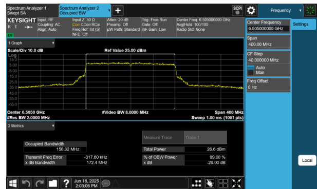
Plot 7-176 26dB BW & 99% OBW Antenna WF7 (160MHz BW 802.11be(RU) RU996X2 Index68 - Ch.111)
