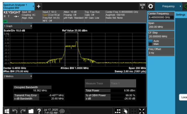
Plot 7-201 26dB BW & 99% OBW Antenna WF7 (80MHz BW 802.11be(RU) RU26 Index17 - Ch.103)
