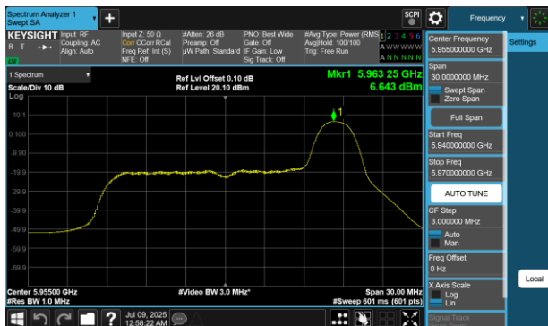
Plot 7-232 PSD Antenna WF5B (20MHz BW 802.11be(RU) RU26 Index8 - Ch.1)
