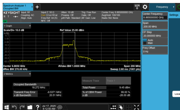
Plot 7-212 26dB BW & 99% OBW Antenna WF7 (80MHz BW 802.11be(RU) RU26 Index17 - Ch.183)
