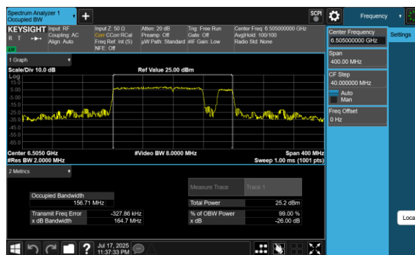
Plot 7-205 26dB BW & 99% OBW Antenna WF7 (160MHz BW 802.11be(RU) RU996+484+242 Index98 - Ch.111)
