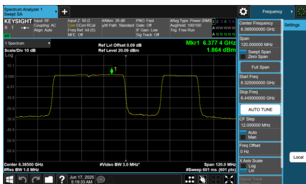
Plot 7-237 PSD Antenna WF5B (80MHz BW 802.11be(RU) RU484+242 Index92 - Ch.87)
