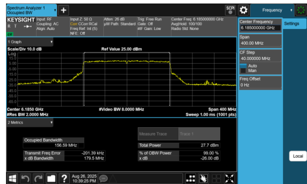
Plot 7-198 26dB BW & 99% OBW Antenna WF7 (160MHz BW 802.11be(RU) RU996X2 Index68 - Ch.47)
