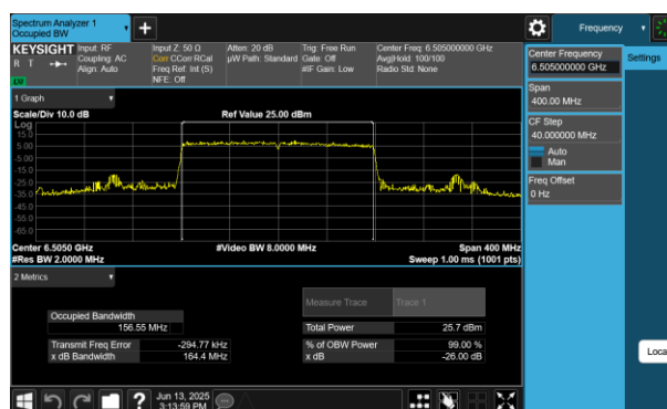
Plot 7-209 26dB BW & 99% OBW Antenna WF7 (160MHz BW 802.11be(RU) RU996X2 Index68 - Ch.111)
