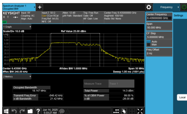
Plot 7-203 26dB BW & 99% OBW Antenna WF7 (20MHz BW 802.11be(RU) RU106+26 Index82 - Ch.97)
