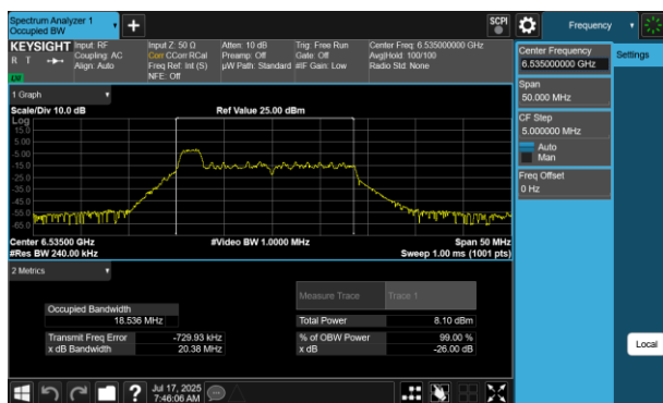
Plot 7-210 26dB BW & 99% OBW Antenna WF7 (20MHz BW 802.11be(RU) RU26 Index0 - Ch.117)
