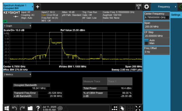
Plot 7-179 26dB BW & 99% OBW Antenna WF7 (80MHz BW 802.11be(RU) RU26 Index0 - Ch.167)
