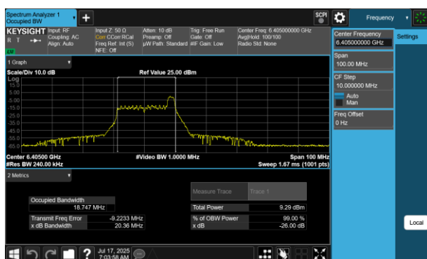
Plot 7-189 26dB BW & 99% OBW Antenna WF7 (40MHz BW 802.11be(RU) RU26 Index8 - Ch.91)
