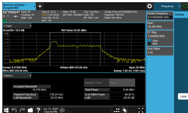
Plot 7-199 26dB BW & 99% OBW Antenna WF7 (20MHz BW 802.11be(RU) RU26 Index0 - Ch.113)
