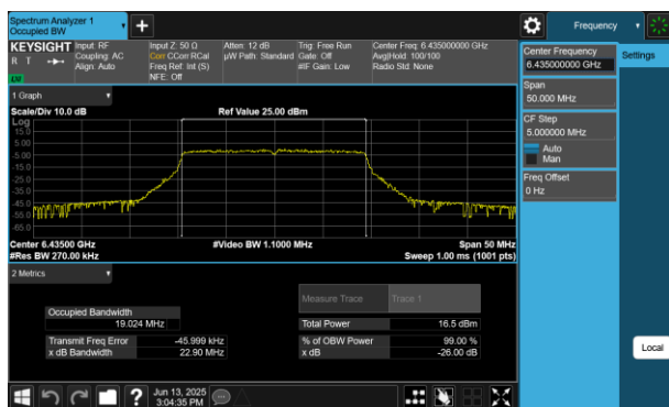
Plot 7-206 26dB BW & 99% OBW Antenna WF7 (20MHz BW 802.11be(RU) RU242 Index61 - Ch.97)
