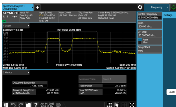
Plot 7-215 26dB BW & 99% OBW Antenna WF7 (80MHz BW 802.11be(RU) RU484+242 Index91 - Ch.119)
