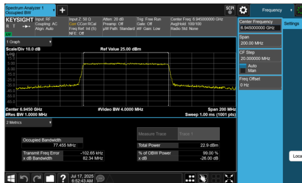
Plot 7-230 26dB BW & 99% OBW Antenna WF7 (80MHz BW 802.11be(RU) RU996 Index67 - Ch.199)
