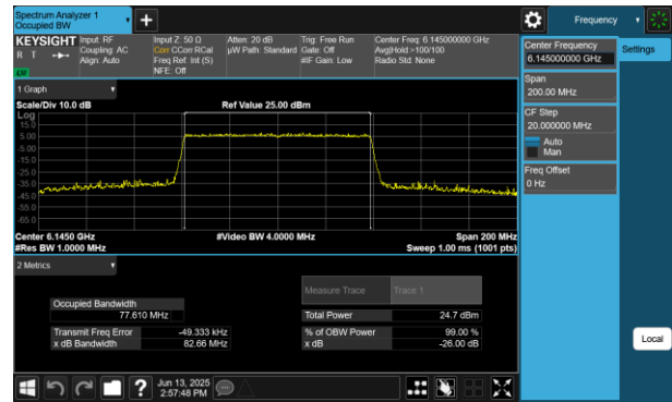
Plot 7-197 26dB BW & 99% OBW Antenna WF7 (80MHz BW 802.11be(RU) RU996 Index67 - Ch.39)
