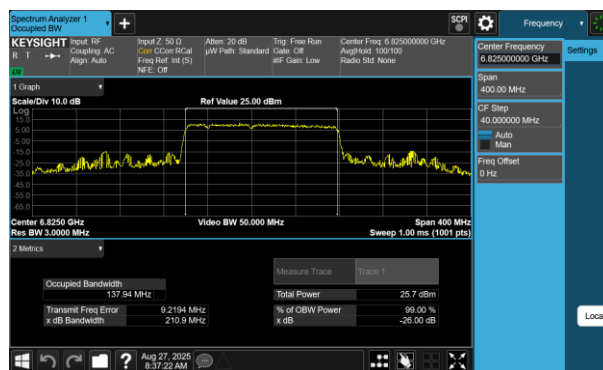
Plot 7-216 26dB BW & 99% OBW Antenna WF7 (160MHz BW 802.11be(RU) RU996+484+242 Index96 - Ch.175)
