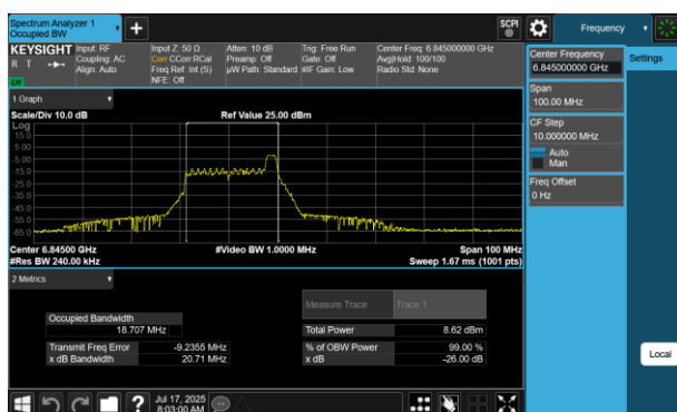
Plot 7-211 26dB BW & 99% OBW Antenna WF7 (40MHz BW 802.11be(RU) RU26 Index8 - Ch.179)
