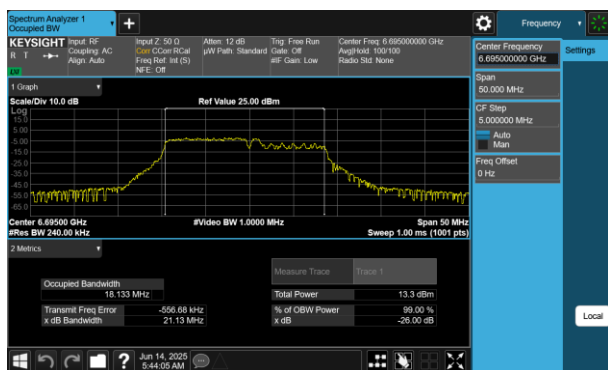
Plot 7-214 26dB BW & 99% OBW Antenna WF7 (20MHz BW 802.11be(RU) RU106+26 Index82 - Ch.149)
