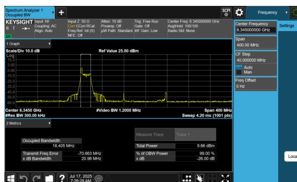
Plot 7-191 26dB BW & 99% OBW Antenna WF7 (160MHz BW 802.11be(RU) RU26 Index0 - Ch.79)
