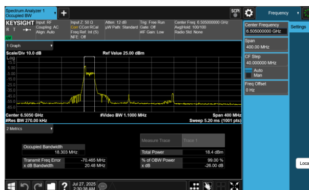
Plot 7-169 26dB BW & 99% OBW Antenna WF7 (160MHz BW 802.11be(RU) RU26 Index0 - Ch.111)
