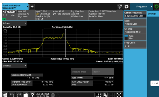
Plot 7-167 26dB BW & 99% OBW Antenna WF7 (40MHz BW 802.11be(RU) RU26 Index8 - Ch.115)
