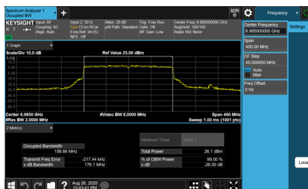
Plot 7-231 26dB BW & 99% OBW Antenna WF7 (160MHz BW 802.11be(RU) RU996X2 Index68 - Ch.207)
