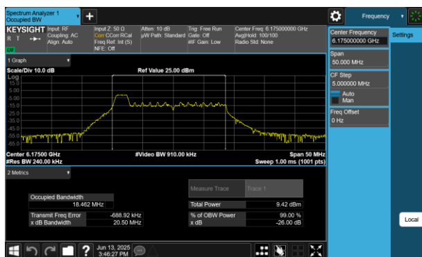
Plot 7-188 26dB BW & 99% OBW Antenna WF7 (20MHz BW 802.11be(RU) RU26 Index0 - Ch.45)
