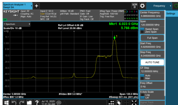
Plot 7-234 PSD Antenna WF5B (80MHz BW 802.11be(RU) RU26 Index36 - Ch.7)
