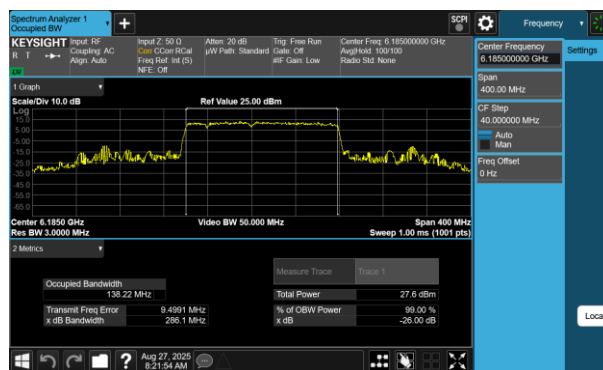
Plot 7-194 26dB BW & 99% OBW Antenna WF7 (160MHz BW 802.11be(RU) RU996+484+242 Index96 - Ch.47)
