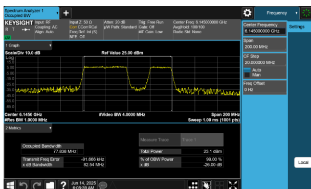
Plot 7-193 26dB BW & 99% OBW Antenna WF7 (80MHz BW 802.11be(RU) RU484+242 Index92 - Ch.39)
