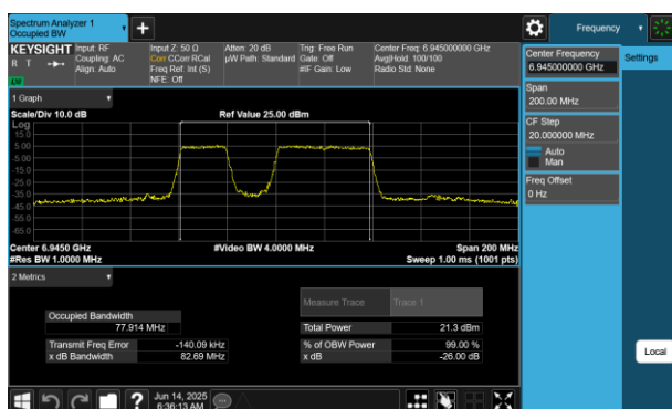
Plot 7-226 26dB BW & 99% OBW Antenna WF7 (80MHz BW 802.11be(RU) RU484+242 Index91 - Ch.199)
