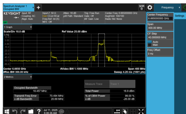
Plot 7-180 26dB BW & 99% OBW Antenna WF7 (160MHz BW 802.11be(RU) RU26 Index36 - Ch.143)
