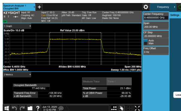
Plot 7-208 26dB BW & 99% OBW Antenna WF7 (80MHz BW 802.11be(RU) RU996 Index67 - Ch.103)
