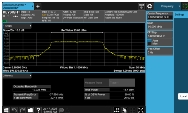
Plot 7-228 26dB BW & 99% OBW Antenna WF7 (20MHz BW 802.11be(RU) RU242 Index61 - Ch.209)
