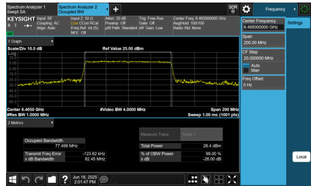
Plot 7-175 26dB BW & 99% OBW Antenna WF7 (80MHz BW 802.11be(RU) RU996 Index67 - Ch.103)
