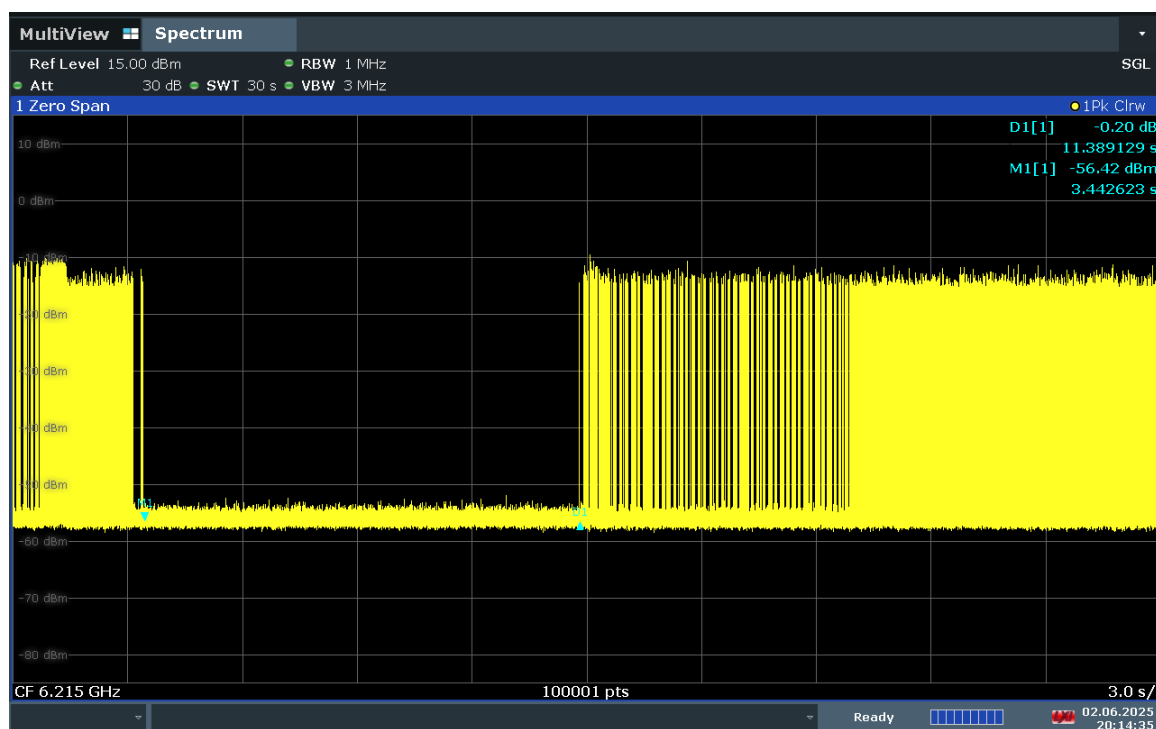
Plot 7-765. Contention Based Protocol Timing Plot – UNII 5 – 20MHz Channel 53
