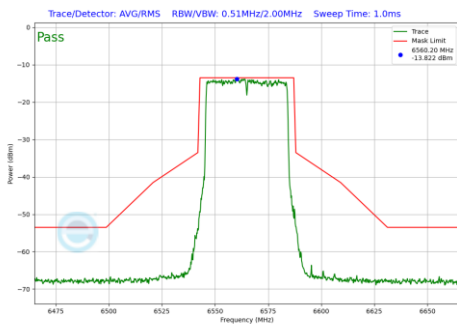
Plot 7-742 In-Band Emission Plot SDM Diversity Antenna WF8 (40MHz BW 802.11be(RU) RU484 Index65 (UNII Band 7) - Ch.123)
