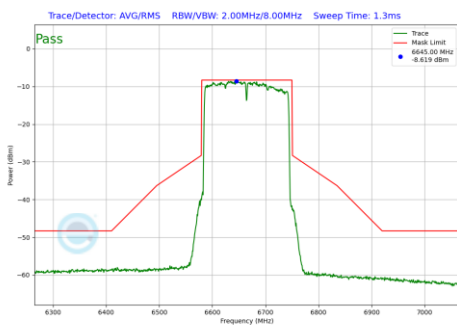
Plot 7-744 In-Band Emission Plot SDM Diversity Antenna WF8 (160MHz BW 802.11be(RU) RU996X2 Index68 (UNII Band 7) - Ch.143)
