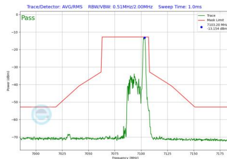
Plot 7-674 In-Band Emission Plot SDM Diversity Antenna WF7 (40MHz BW 802.11be(RU) RU26 Index17 (UNII Band 8) - Ch.227)
