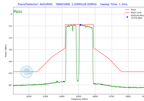
Plot 7-698 In-Band Emission Plot SDM Diversity Antenna WF7 (160MHz BW 802.11be(RU) RU996+484+242 Index99 (UNII Band 6) - Ch.111)
