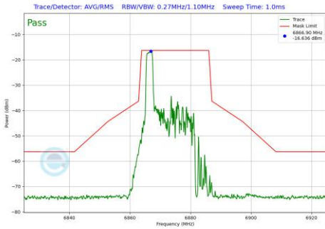
Plot 7-669 In-Band Emission Plot SDM Diversity Antenna WF7 (20MHz BW 802.11be(RU) RU26 Index0 (UNII Band 7) - Ch.185)
