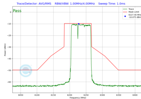
Plot 7-706 In-Band Emission Plot SDM Diversity Antenna WF8 (80MHz BW 802.11be(RU) RU484+242 Index90 (UNII Band 5) - Ch.55)
