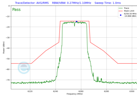
Plot 7-733 In-Band Emission Plot SDM Diversity Antenna WF8 (20MHz BW 802.11be(RU) RU242 Index61 (UNII Band 5) - Ch.61)
