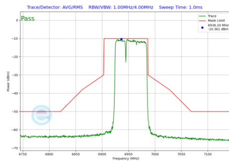
Plot 7-627 In-Band Emission Plot SDM Primary Antenna WF8 (80MHz BW 802.11be(RU) RU484+242 Index90 (UNII Band 8) - Ch.199)
