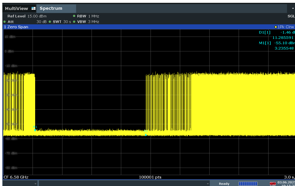
Plot 7-770. Contention Based Protocol Timing Plot – UNII 6 – 160MHz Channel 111 – Low
