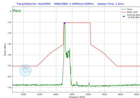
Plot 7-667 In-Band Emission Plot SDM Diversity Antenna WF7 (80MHz BW 802.11be(RU) RU26 Index0 (UNII Band 6) - Ch.103)
