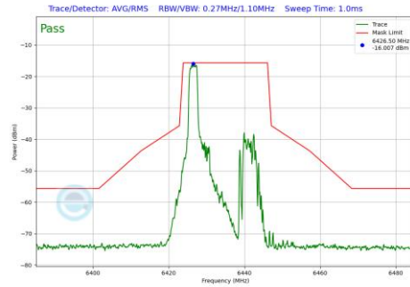
Plot 7-681 In-Band Emission Plot SDM Diversity Antenna WF8 (20MHz BW 802.11be(RU) RU26 Index0 (UNII Band 6) - Ch.97)
