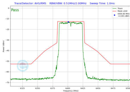
Plot 7-734 In-Band Emission Plot SDM Diversity Antenna WF8 (40MHz BW 802.11be(RU) RU484 Index65 (UNII Band 5) - Ch.91)
