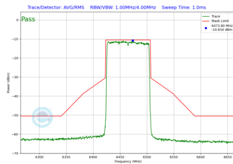
Plot 7-635 In-Band Emission Plot SDM Primary Antenna WF5B (80MHz BW 802.11be(RU) RU996 Index67 (UNII Band 6) - Ch.103)
