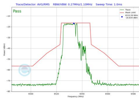
Plot 7-623 In-Band Emission Plot SDM Primary Antenna WF8 (20MHz BW 802.11be(RU) RU106+26 Index82 (UNII Band 7) - Ch.117)
