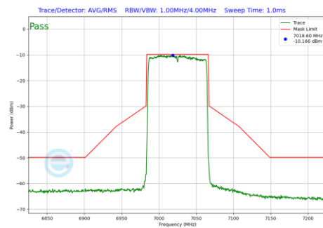
Plot 7-747 In-Band Emission Plot SDM Diversity Antenna WF8 (80MHz BW 802.11be(RU) RU996 Index67 (UNII Band 8) - Ch.215)
