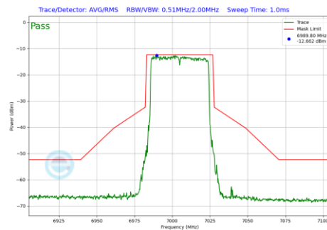
Plot 7-746 In-Band Emission Plot SDM Diversity Antenna WF8 (40MHz BW 802.11be(RU) RU484 Index65 (UNII Band 8) - Ch.211)
