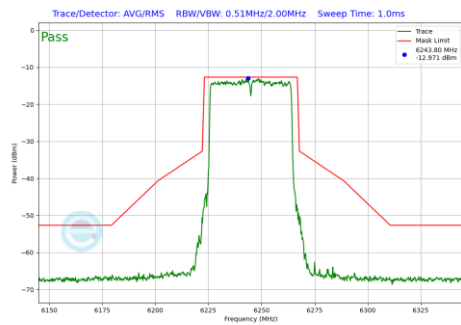
Plot 7-630 In-Band Emission Plot SDM Primary Antenna WF5B (40MHz BW 802.11be(RU) RU484 Index65 (UNII Band 5) - Ch.59)
