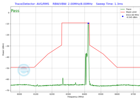
Plot 7-680 In-Band Emission Plot SDM Diversity Antenna WF8 (160MHz BW 802.11be(RU) RU26 Index36 (UNII Band 5) - Ch.79)
