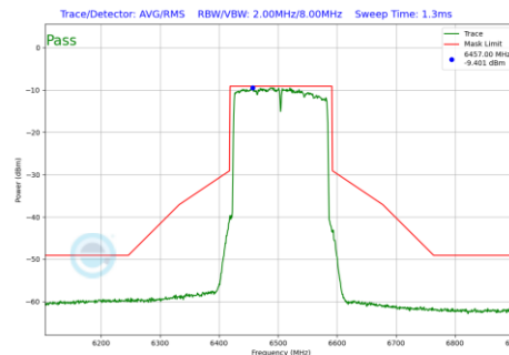
Plot 7-740 In-Band Emission Plot SDM Diversity Antenna WF8 (160MHz BW 802.11be(RU) RU996X2 Index68 (UNII Band 6) - Ch.111)
