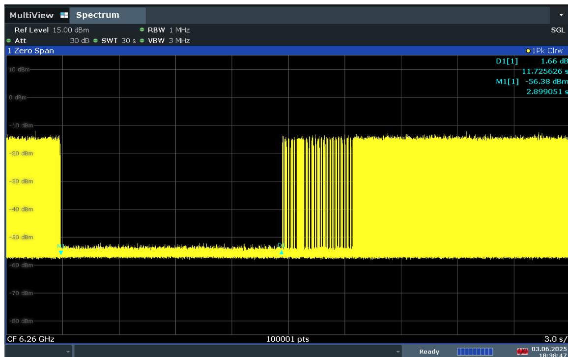
Plot 7-766. Contention Based Protocol Timing Plot – UNII 5 – 160MHz Channel 47 – Low
