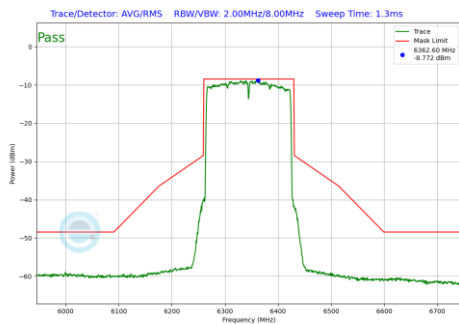
Plot 7-720 In-Band Emission Plot SDM Diversity Antenna WF7 (160MHz BW 802.11be(RU) RU996X2 Index68 (UNII Band 5) - Ch.79)
