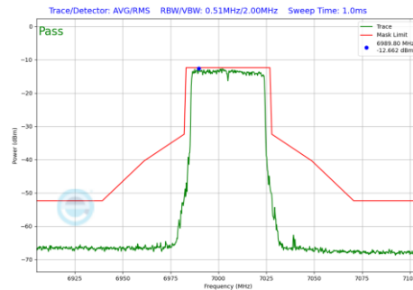
Plot 7-658 In-Band Emission Plot SDM Primary Antenna WF8 (40MHz BW 802.11be(RU) RU484 Index65 (UNII Band 8) - Ch.211)
