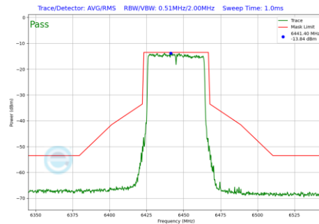
Plot 7-738 In-Band Emission Plot SDM Diversity Antenna WF8 (40MHz BW 802.11be(RU) RU484 Index65 (UNII Band 6) - Ch.99)
