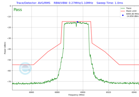
Plot 7-641 In-Band Emission Plot SDM Primary Antenna WF5B (20MHz BW 802.11be(RU) RU242 Index61 (UNII Band 8) - Ch.189)
