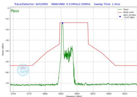
Plot 7-670 In-Band Emission Plot SDM Diversity Antenna WF7 (40MHz BW 802.11be(RU) RU26 Index0 (UNII Band 7) - Ch.179)
