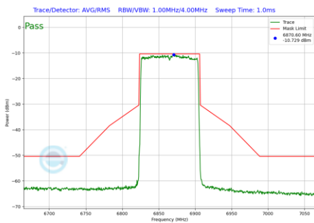
Plot 7-743 In-Band Emission Plot SDM Diversity Antenna WF8 (80MHz BW 802.11be(RU) RU996 Index67 (UNII Band 7) - Ch.183)
