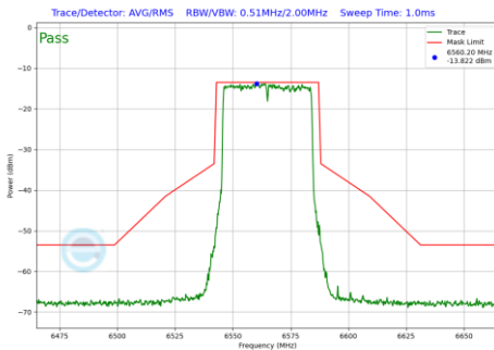
Plot 7-654 In-Band Emission Plot SDM Primary Antenna WF8 (40MHz BW 802.11be(RU) RU484 Index65 (UNII Band 7) - Ch.123)
