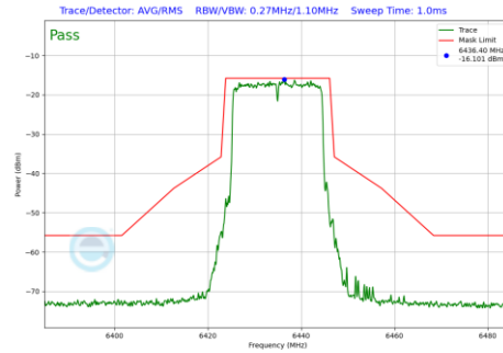
Plot 7-737 In-Band Emission Plot SDM Diversity Antenna WF8 (20MHz BW 802.11be(RU) RU242 Index61 (UNII Band 6) - Ch.97)
