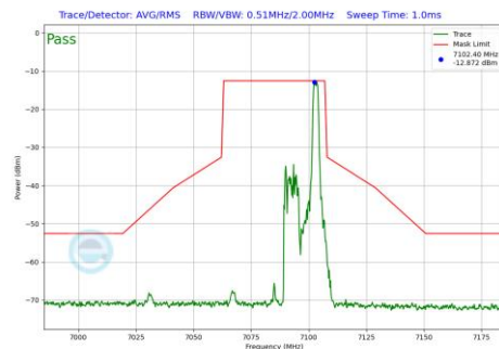
Plot 7-690 In-Band Emission Plot SDM Diversity Antenna WF8 (40MHz BW 802.11be(RU) RU26 Index17 (UNII Band 8) - Ch.227)
