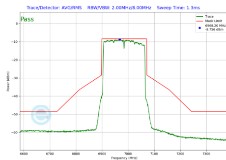
Plot 7-748 In-Band Emission Plot SDM Diversity Antenna WF8 (160MHz BW 802.11be(RU) RU996X2 Index68 (UNII Band 8) - Ch.207)
