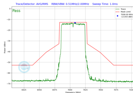
Plot 7-642 In-Band Emission Plot SDM Primary Antenna WF5B (40MHz BW 802.11be(RU) RU484 Index65 (UNII Band 8) - Ch.211)
