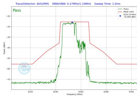
Plot 7-693 In-Band Emission Plot SDM Diversity Antenna WF7 (20MHz BW 802.11be(RU) RU106+26 Index82 (UNII Band 5) - Ch.61)
