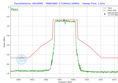
Plot 7-650 In-Band Emission Plot SDM Primary Antenna WF8 (40MHz BW 802.11be(RU) RU484 Index65 (UNII Band 6) - Ch.107)
