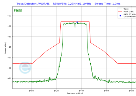
Plot 7-721 In-Band Emission Plot SDM Diversity Antenna WF7 (20MHz BW 802.11be(RU) RU242 Index61 (UNII Band 6) - Ch.97)
