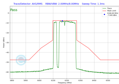
Plot 7-695 In-Band Emission Plot SDM Diversity Antenna WF7 (160MHz BW 802.11be(RU) RU996+484+242 Index97 (UNII Band 5) - Ch.47)
