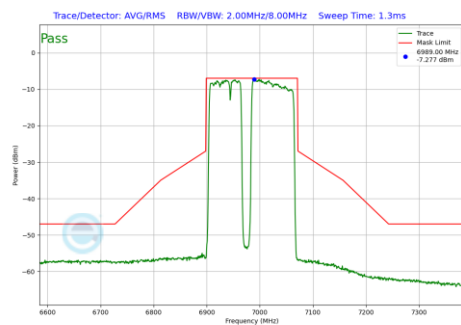
Plot 7-716 In-Band Emission Plot SDM Diversity Antenna WF8 (160MHz BW 802.11be(RU) RU996+484+242 Index99 (UNII Band 8) - Ch.207)
