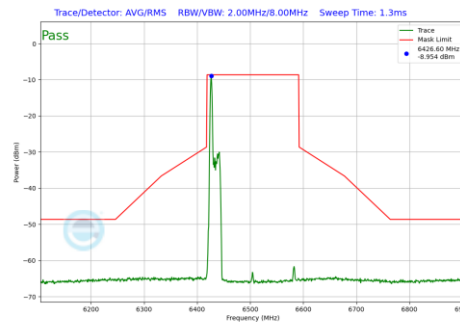
Plot 7-684 In-Band Emission Plot SDM Diversity Antenna WF8 (160MHz BW 802.11be(RU) RU26 Index0 (UNII Band 6) - Ch.111)
