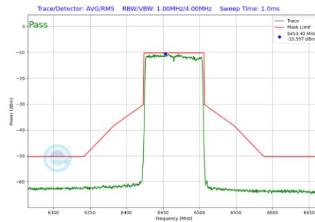
Plot 7-739 In-Band Emission Plot SDM Diversity Antenna WF8 (80MHz BW 802.11be(RU) RU996 Index67 (UNII Band 6) - Ch.103)
