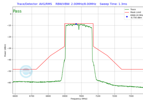
Plot 7-660 In-Band Emission Plot SDM Primary Antenna WF8 (160MHz BW 802.11be(RU) RU996X2 Index68 (UNII Band 8) - Ch.207)
