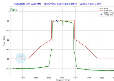
Plot 7-652 In-Band Emission Plot SDM Primary Antenna WF8 (160MHz BW 802.11be(RU) RU996X2 Index68 (UNII Band 6) - Ch.111)
