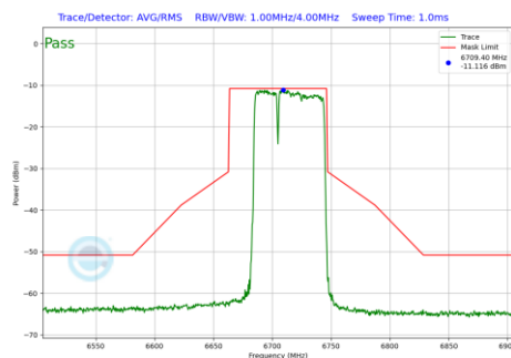
Plot 7-624 In-Band Emission Plot SDM Primary Antenna WF8 (80MHz BW 802.11be(RU) RU484+242 Index90 (UNII Band 7) - Ch.151)
