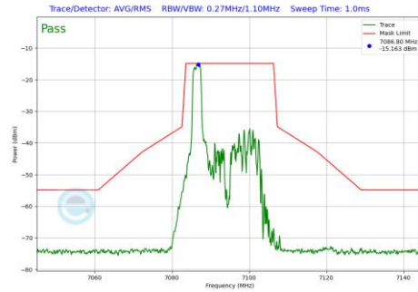
Plot 7-689 In-Band Emission Plot SDM Diversity Antenna WF8 (20MHz BW 802.11be(RU) RU26 Index0 (UNII Band 8) - Ch.229)
