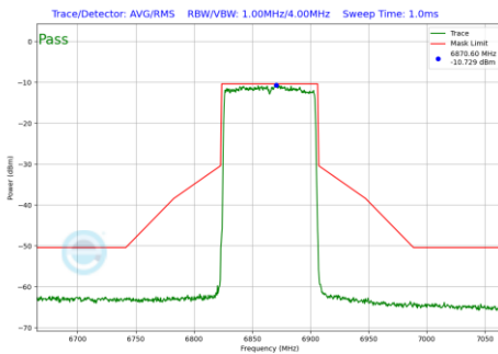
Plot 7-655 In-Band Emission Plot SDM Primary Antenna WF8 (80MHz BW 802.11be(RU) RU996 Index67 (UNII Band 7) - Ch.183)
