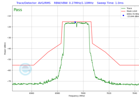
Plot 7-729 In-Band Emission Plot SDM Diversity Antenna WF7 (20MHz BW 802.11be(RU) RU242 Index61 (UNII Band 8) - Ch.209)
