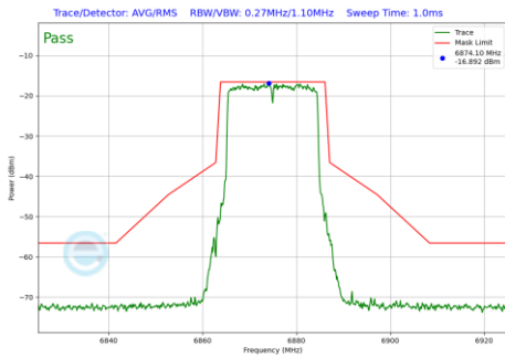
Plot 7-741 In-Band Emission Plot SDM Diversity Antenna WF8 (20MHz BW 802.11be(RU) RU242 Index61 (UNII Band 7) - Ch.185)
