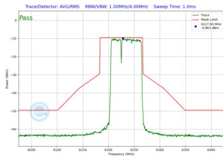
Plot 7-694 In-Band Emission Plot SDM Diversity Antenna WF7 (80MHz BW 802.11be(RU) RU484+242 Index90 (UNII Band 5) - Ch.55)
