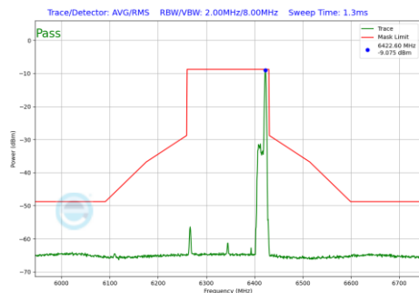
Plot 7-664 In-Band Emission Plot SDM Diversity Antenna WF7 (160MHz BW 802.11be(RU) RU26 Index36 (UNII Band 5) - Ch.79)
