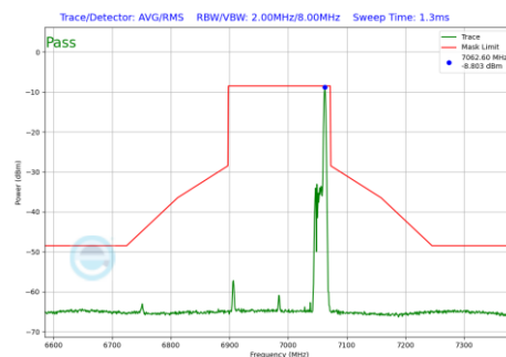
Plot 7-676 In-Band Emission Plot SDM Diversity Antenna WF7 (160MHz BW 802.11be(RU) RU26 Index36 (UNII Band 8) - Ch.207)
