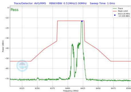
Plot 7-678 In-Band Emission Plot SDM Diversity Antenna WF8 (40MHz BW 802.11be(RU) RU26 Index17 (UNII Band 5) - Ch.91)
