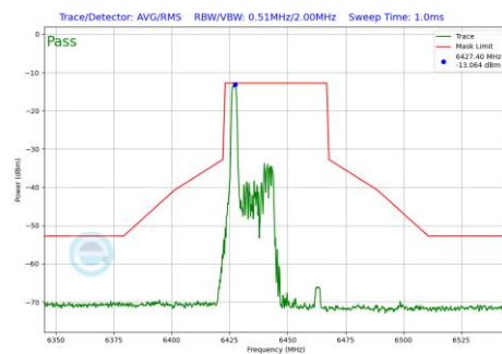
Plot 7-666 In-Band Emission Plot SDM Diversity Antenna WF7 (40MHz BW 802.11be(RU) RU26 Index0 (UNII Band 6) - Ch.99)
