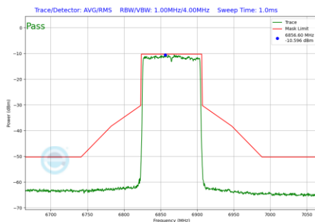
Plot 7-639 In-Band Emission Plot SDM Primary Antenna WF5B (80MHz BW 802.11be(RU) RU996 Index67 (UNII Band 7) - Ch.183)
