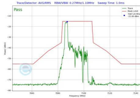
Plot 7-673 In-Band Emission Plot SDM Diversity Antenna WF7 (20MHz BW 802.11be(RU) RU26 Index0 (UNII Band 8) - Ch.229)
