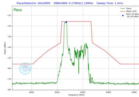
Plot 7-665 In-Band Emission Plot SDM Diversity Antenna WF7 (20MHz BW 802.11be(RU) RU26 Index0 (UNII Band 6) - Ch.97)
