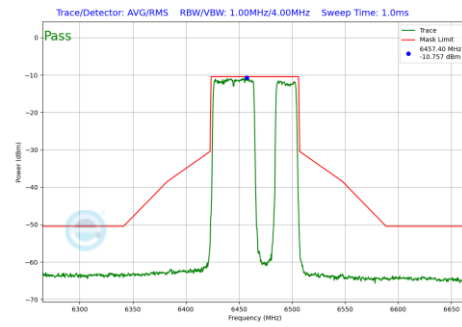
Plot 7-697 In-Band Emission Plot SDM Diversity Antenna WF7 (80MHz BW 802.11be(RU) RU484+242 Index92 (UNII Band 6) - Ch.103)
