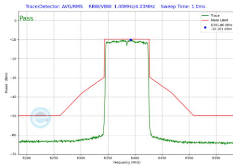
Plot 7-735 In-Band Emission Plot SDM Diversity Antenna WF8 (80MHz BW 802.11be(RU) RU996 Index67 (UNII Band 5) - Ch.87)
