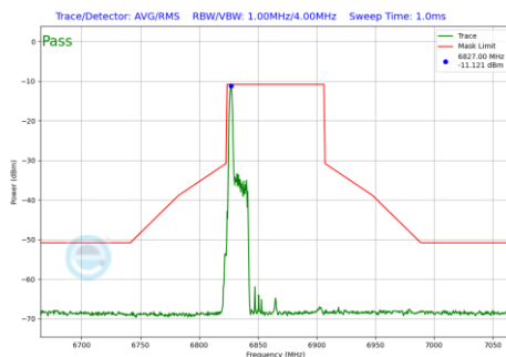
Plot 7-687 In-Band Emission Plot SDM Diversity Antenna WF8 (80MHz BW 802.11be(RU) RU26 Index0 (UNII Band 7) - Ch.183)
