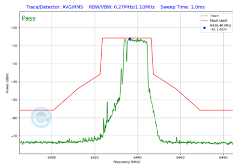
Plot 7-696 In-Band Emission Plot SDM Diversity Antenna WF7 (20MHz BW 802.11be(RU) RU106+26 Index83 (UNII Band 6) - Ch.97)
