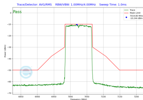
Plot 7-643 In-Band Emission Plot SDM Primary Antenna WF5B (80MHz BW 802.11be(RU) RU996 Index67 (UNII Band 8) - Ch.215)
