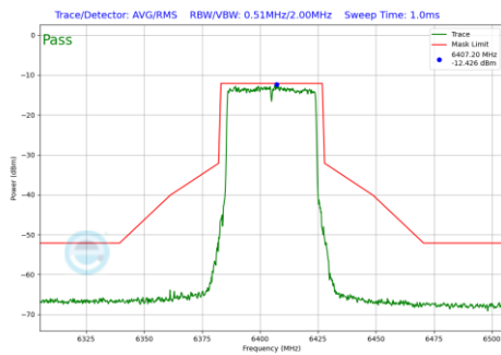
Plot 7-718 In-Band Emission Plot SDM Diversity Antenna WF7 (40MHz BW 802.11be(RU) RU484 Index65 (UNII Band 5) - Ch.91)
