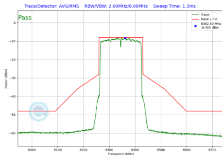
Plot 7-736 In-Band Emission Plot SDM Diversity Antenna WF8 (160MHz BW 802.11be(RU) RU996X2 Index68 (UNII Band 5) - Ch.79)
