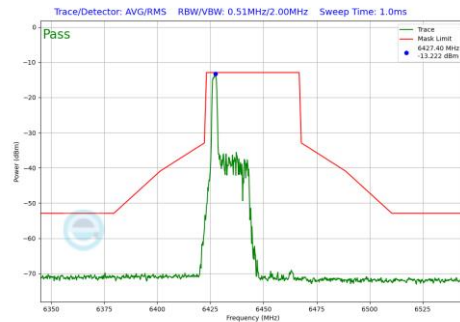
Plot 7-682 In-Band Emission Plot SDM Diversity Antenna WF8 (40MHz BW 802.11be(RU) RU26 Index0 (UNII Band 6) - Ch.99)
