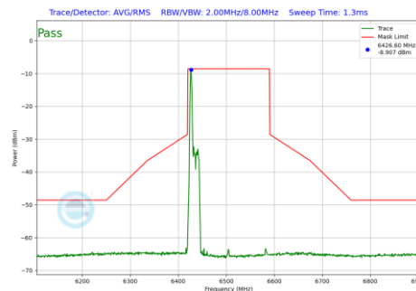
Plot 7-668 In-Band Emission Plot SDM Diversity Antenna WF7 (160MHz BW 802.11be(RU) RU26 Index0 (UNII Band 6) - Ch.111)
