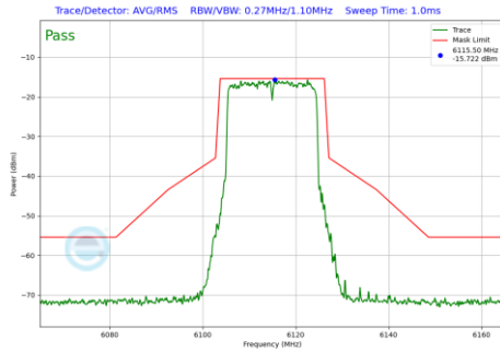
Plot 7-645 In-Band Emission Plot SDM Primary Antenna WF8 (20MHz BW 802.11be(RU) RU242 Index61 (UNII Band 5) - Ch.33)
