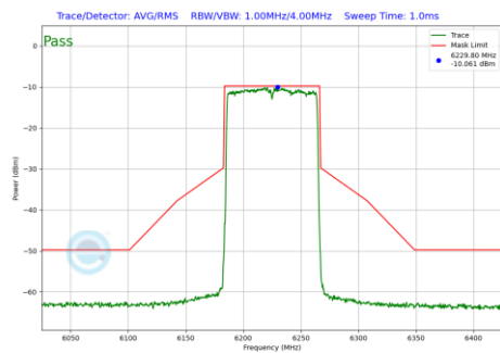
Plot 7-631 In-Band Emission Plot SDM Primary Antenna WF5B (80MHz BW 802.11be(RU) RU996 Index67 (UNII Band 5) - Ch.55)
