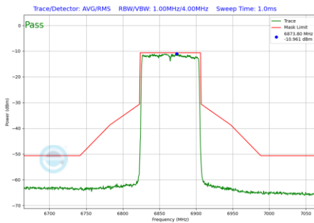
Plot 7-727 In-Band Emission Plot SDM Diversity Antenna WF7 (80MHz BW 802.11be(RU) RU996 Index67 (UNII Band 7) - Ch.183)
