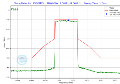
Plot 7-731 In-Band Emission Plot SDM Diversity Antenna WF7 (80MHz BW 802.11be(RU) RU996 Index67 (UNII Band 8) - Ch.215)
