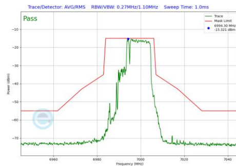
Plot 7-626 In-Band Emission Plot SDM Primary Antenna WF8 (20MHz BW 802.11be(RU) RU106+26 Index83 (UNII Band 8) - Ch.209)
