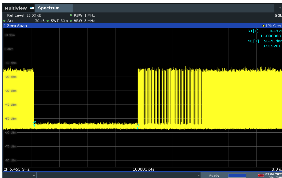
Plot 7-769. Contention Based Protocol Timing Plot – UNII 6 – 20MHz Channel 101
