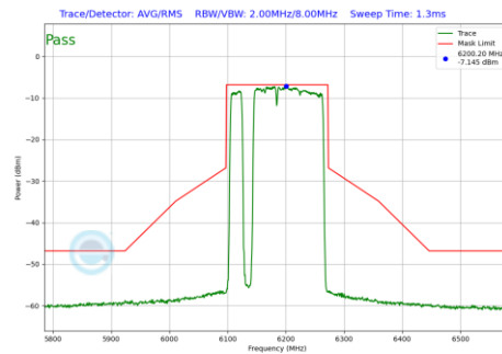
Plot 7-707 In-Band Emission Plot SDM Diversity Antenna WF8 (160MHz BW 802.11be(RU) RU996+484+242 Index97 (UNII Band 5) - Ch.47)
