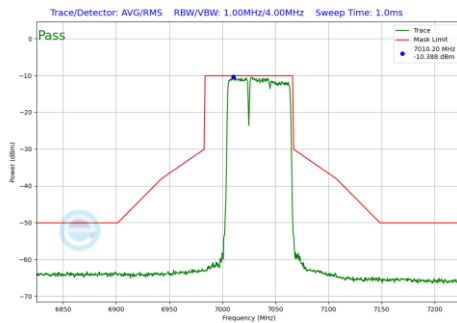
Plot 7-703 In-Band Emission Plot SDM Diversity Antenna WF7 (80MHz BW 802.11be(RU) RU484+242 Index90 (UNII Band 8) - Ch.215)
