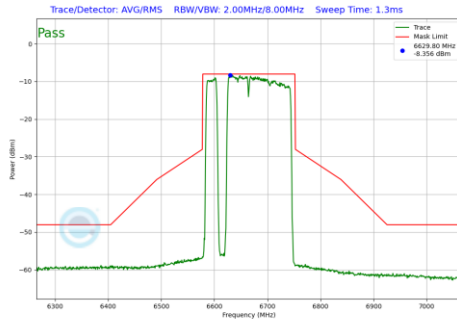
Plot 7-701 In-Band Emission Plot SDM Diversity Antenna WF7 (160MHz BW 802.11be(RU) RU996+484+242 Index97 (UNII Band 7) - Ch.143)
