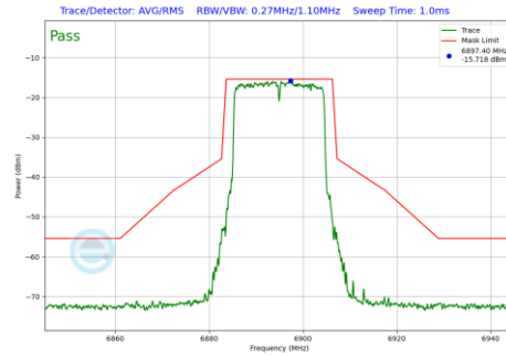
Plot 7-657 In-Band Emission Plot SDM Primary Antenna WF8 (20MHz BW 802.11be(RU) RU242 Index61 (UNII Band 8) - Ch.189)
