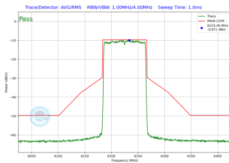
Plot 7-647 In-Band Emission Plot SDM Primary Antenna WF8 (80MHz BW 802.11be(RU) RU996 Index67 (UNII Band 5) - Ch.55)
