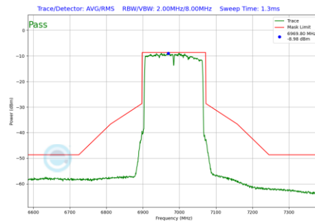
Plot 7-732 In-Band Emission Plot SDM Diversity Antenna WF7 (160MHz BW 802.11be(RU) RU996X2 Index68 (UNII Band 8) - Ch.207)
