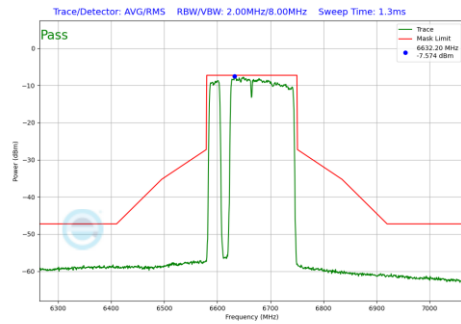
Plot 7-713 In-Band Emission Plot SDM Diversity Antenna WF8 (160MHz BW 802.11be(RU) RU996+484+242 Index97 (UNII Band 7) - Ch.143)
