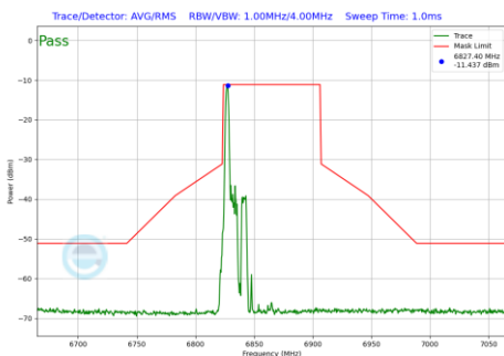
Plot 7-671 In-Band Emission Plot SDM Diversity Antenna WF7 (80MHz BW 802.11be(RU) RU26 Index0 (UNII Band 7) - Ch.183)
