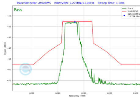
Plot 7-705 In-Band Emission Plot SDM Diversity Antenna WF8 (20MHz BW 802.11be(RU) RU106+26 Index82 (UNII Band 5) - Ch.61)
