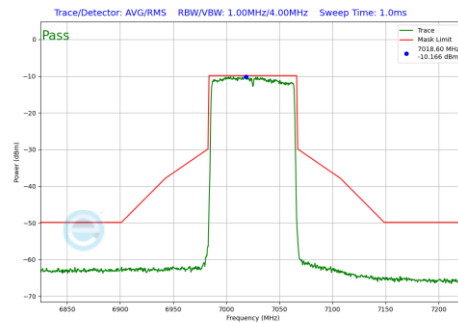
Plot 7-659 In-Band Emission Plot SDM Primary Antenna WF8 (80MHz BW 802.11be(RU) RU996 Index67 (UNII Band 8) - Ch.215)
