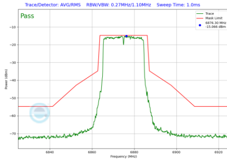
Plot 7-637 In-Band Emission Plot SDM Primary Antenna WF5B (20MHz BW 802.11be(RU) RU242 Index61 (UNII Band 7) - Ch.185)
