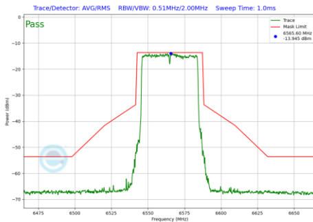
Plot 7-726 In-Band Emission Plot SDM Diversity Antenna WF7 (40MHz BW 802.11be(RU) RU484 Index65 (UNII Band 7) - Ch.123)
