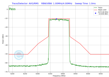
Plot 7-719 In-Band Emission Plot SDM Diversity Antenna WF7 (80MHz BW 802.11be(RU) RU996 Index67 (UNII Band 5) - Ch.87)
