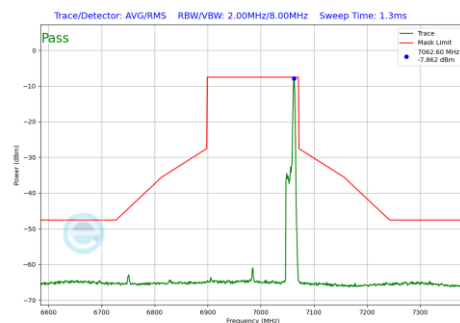
Plot 7-692 In-Band Emission Plot SDM Diversity Antenna WF8 (160MHz BW 802.11be(RU) RU26 Index36 (UNII Band 8) - Ch.207)
