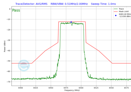
Plot 7-634 In-Band Emission Plot SDM Primary Antenna WF5B (40MHz BW 802.11be(RU) RU484 Index65 (UNII Band 6) - Ch.107)
