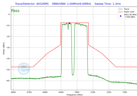
Plot 7-704 In-Band Emission Plot SDM Diversity Antenna WF7 (160MHz BW 802.11be(RU) RU996+484+242 Index99 (UNII Band 8) - Ch.207)
