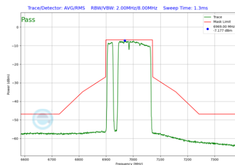
Plot 7-628 In-Band Emission Plot SDM Primary Antenna WF8 (160MHz BW 802.11be(RU) RU996+484+242 Index97 (UNII Band 8) - Ch.207)
