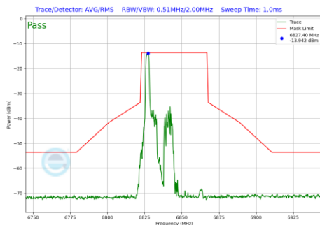
Plot 7-686 In-Band Emission Plot SDM Diversity Antenna WF8 (40MHz BW 802.11be(RU) RU26 Index0 (UNII Band 7) - Ch.179)
