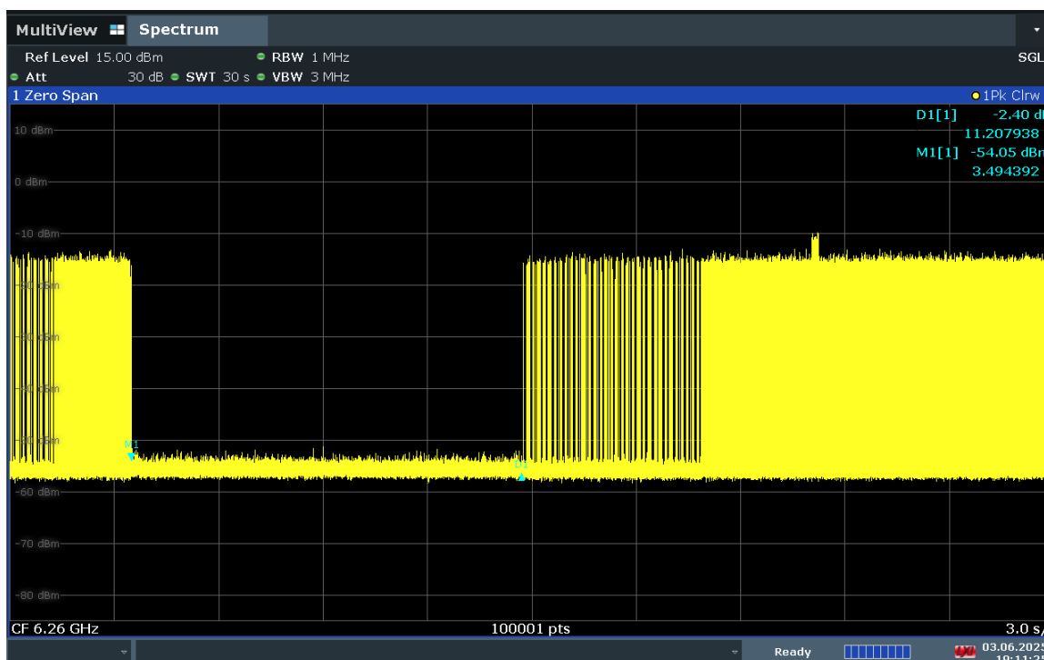
Plot 7-768. Contention Based Protocol Timing Plot – UNII 5 – 160MHz Channel 47 – High
