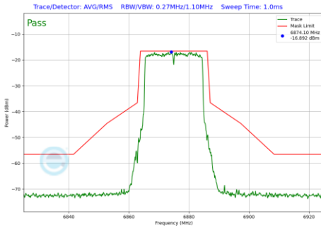
Plot 7-653 In-Band Emission Plot SDM Primary Antenna WF8 (20MHz BW 802.11be(RU) RU242 Index61 (UNII Band 7) - Ch.185)
