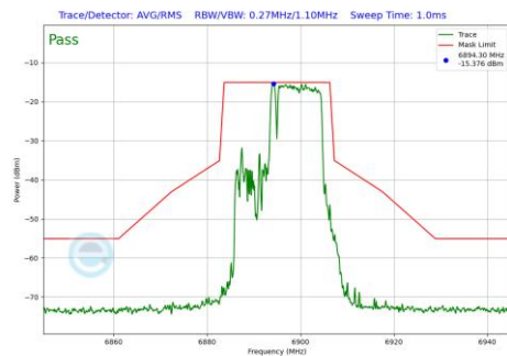
Plot 7-714 In-Band Emission Plot SDM Diversity Antenna WF8 (20MHz BW 802.11be(RU) RU106+26 Index83 (UNII Band 8) - Ch.189)
