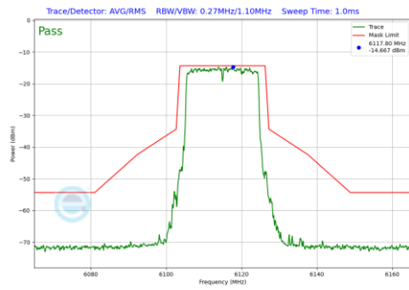
Plot 7-629 In-Band Emission Plot SDM Primary Antenna WF5B (20MHz BW 802.11be(RU) RU242 Index61 (UNII Band 5) - Ch.33)
