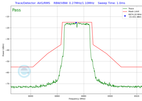
Plot 7-725 In-Band Emission Plot SDM Diversity Antenna WF7 (20MHz BW 802.11be(RU) RU242 Index61 (UNII Band 7) - Ch.185)
