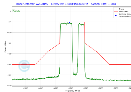
Plot 7-700 In-Band Emission Plot SDM Diversity Antenna WF7 (80MHz BW 802.11be(RU) RU484+242 Index92 (UNII Band 7) - Ch.151)
