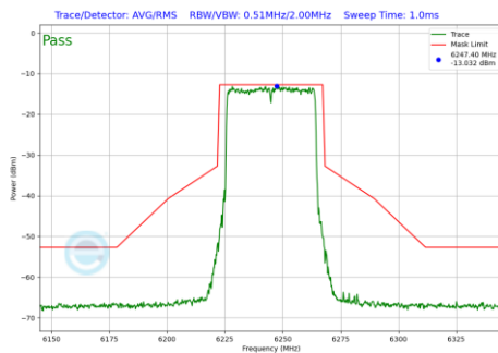
Plot 7-646 In-Band Emission Plot SDM Primary Antenna WF8 (40MHz BW 802.11be(RU) RU484 Index65 (UNII Band 5) - Ch.59)
