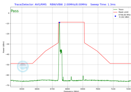
Plot 7-688 In-Band Emission Plot SDM Diversity Antenna WF8 (160MHz BW 802.11be(RU) RU26 Index0 (UNII Band 7) - Ch.175)
