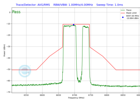
Plot 7-712 In-Band Emission Plot SDM Diversity Antenna WF8 (80MHz BW 802.11be(RU) RU484+242 Index92 (UNII Band 7) - Ch.151)
