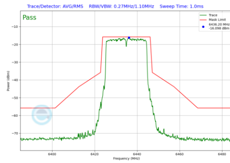
Plot 7-633 In-Band Emission Plot SDM Primary Antenna WF5B (20MHz BW 802.11be(RU) RU242 Index61 (UNII Band 6) - Ch.97)
