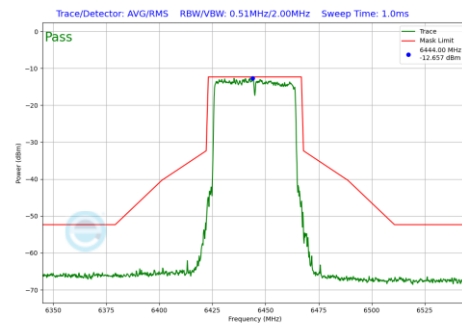
Plot 7-722 In-Band Emission Plot SDM Diversity Antenna WF7 (40MHz BW 802.11be(RU) RU484 Index65 (UNII Band 6) - Ch.99)
