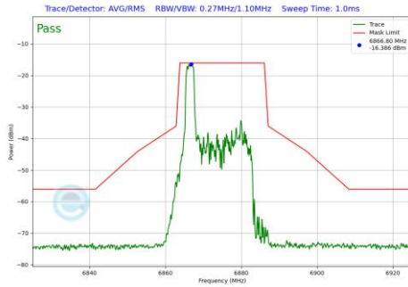
Plot 7-685 In-Band Emission Plot SDM Diversity Antenna WF8 (20MHz BW 802.11be(RU) RU26 Index0 (UNII Band 7) - Ch.185)
