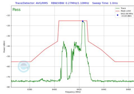
Plot 7-661 In-Band Emission Plot SDM Diversity Antenna WF7 (20MHz BW 802.11be(RU) RU26 Index8 (UNII Band 5) - Ch.93)
