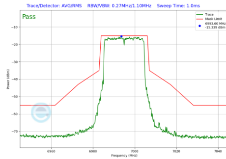
Plot 7-745 In-Band Emission Plot SDM Diversity Antenna WF8 (20MHz BW 802.11be(RU) RU242 Index61 (UNII Band 8) - Ch.209)
