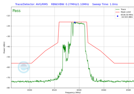
Plot 7-711 In-Band Emission Plot SDM Diversity Antenna WF8 (20MHz BW 802.11be(RU) RU106+26 Index83 (UNII Band 7) - Ch.117)
