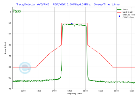
Plot 7-723 In-Band Emission Plot SDM Diversity Antenna WF7 (80MHz BW 802.11be(RU) RU996 Index67 (UNII Band 6) - Ch.103)
