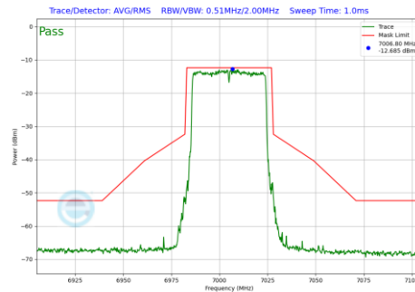
Plot 7-730 In-Band Emission Plot SDM Diversity Antenna WF7 (40MHz BW 802.11be(RU) RU484 Index65 (UNII Band 8) - Ch.211)
