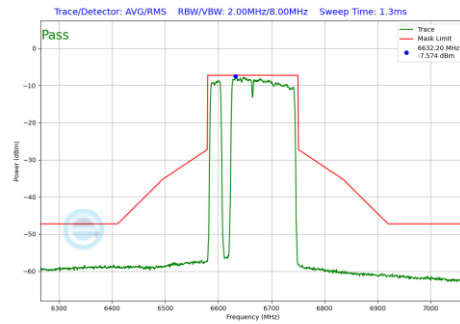
Plot 7-625 In-Band Emission Plot SDM Primary Antenna WF8 (160MHz BW 802.11be(RU) RU996+484+242 Index97 (UNII Band 7) - Ch.143)
