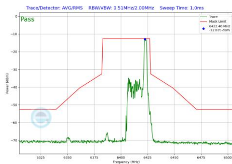
Plot 7-662 In-Band Emission Plot SDM Diversity Antenna WF7 (40MHz BW 802.11be(RU) RU26 Index17 (UNII Band 5) - Ch.91)
