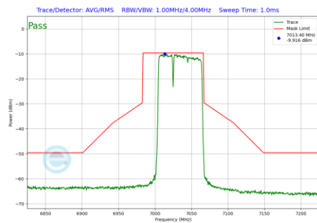
Plot 7-715 In-Band Emission Plot SDM Diversity Antenna WF8 (80MHz BW 802.11be(RU) RU484+242 Index90 (UNII Band 8) - Ch.215)
