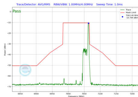
Plot 7-675 In-Band Emission Plot SDM Diversity Antenna WF7 (80MHz BW 802.11be(RU) RU26 Index36 (UNII Band 8) - Ch.215)
