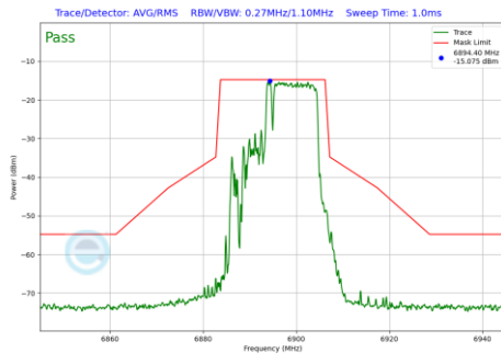
Plot 7-702 In-Band Emission Plot SDM Diversity Antenna WF7 (20MHz BW 802.11be(RU) RU106+26 Index83 (UNII Band 8) - Ch.189)
