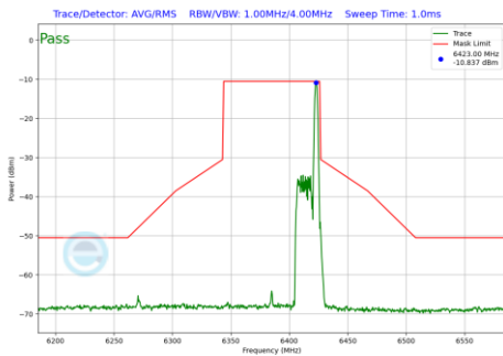
Plot 7-679 In-Band Emission Plot SDM Diversity Antenna WF8 (80MHz BW 802.11be(RU) RU26 Index36 (UNII Band 5) - Ch.87)
