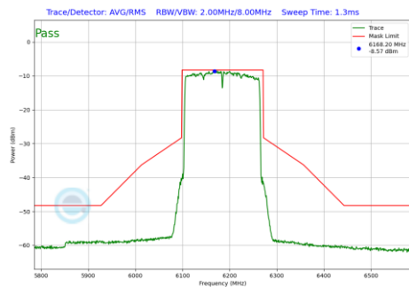
Plot 7-632 In-Band Emission Plot SDM Primary Antenna WF5B (160MHz BW 802.11be(RU) RU996X2 Index68 (UNII Band 5) - Ch.47)
