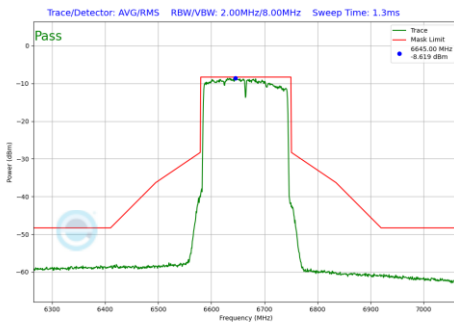
Plot 7-656 In-Band Emission Plot SDM Primary Antenna WF8 (160MHz BW 802.11be(RU) RU996X2 Index68 (UNII Band 7) - Ch.143)
