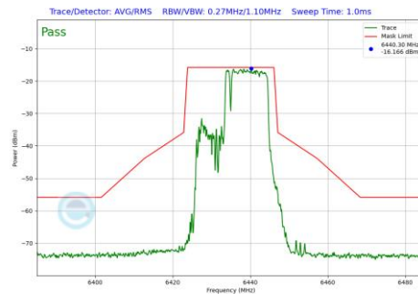
Plot 7-708 In-Band Emission Plot SDM Diversity Antenna WF8 (20MHz BW 802.11be(RU) RU106+26 Index83 (UNII Band 6) - Ch.97)
