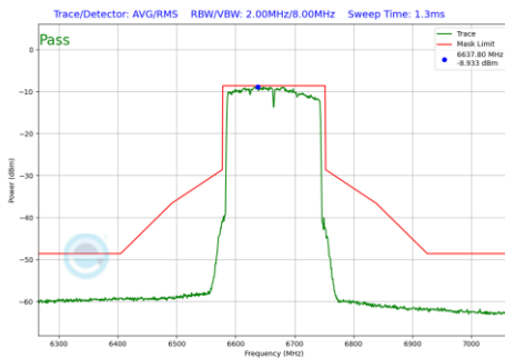
Plot 7-728 In-Band Emission Plot SDM Diversity Antenna WF7 (160MHz BW 802.11be(RU) RU996X2 Index68 (UNII Band 7) - Ch.143)
