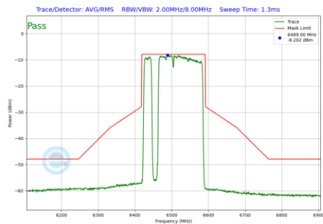
Plot 7-622 In-Band Emission Plot SDM Primary Antenna WF8 (160MHz BW 802.11be(RU) RU996+484+242 Index97 (UNII Band 6) - Ch.111)
