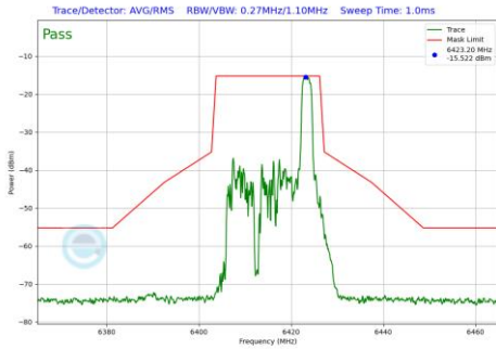
Plot 7-677 In-Band Emission Plot SDM Diversity Antenna WF8 (20MHz BW 802.11be(RU) RU26 Index8 (UNII Band 5) - Ch.93)
