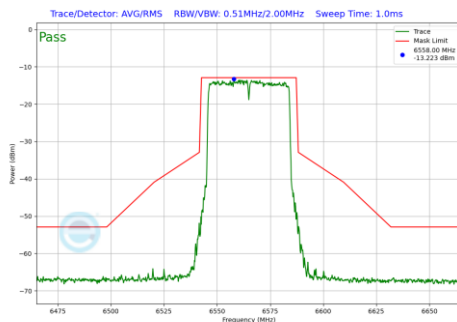
Plot 7-638 In-Band Emission Plot SDM Primary Antenna WF5B (40MHz BW 802.11be(RU) RU484 Index65 (UNII Band 7) - Ch.123)
