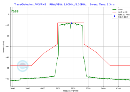
Plot 7-648 In-Band Emission Plot SDM Primary Antenna WF8 (160MHz BW 802.11be(RU) RU996X2 Index68 (UNII Band 5) - Ch.47)
