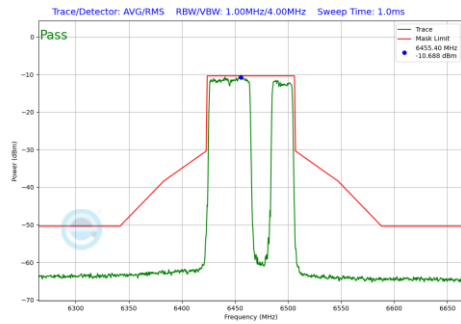
Plot 7-621 In-Band Emission Plot SDM Primary Antenna WF8 (80MHz BW 802.11be(RU) RU484+242 Index92 (UNII Band 6) - Ch.103)
