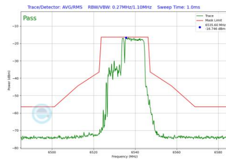
Plot 7-699 In-Band Emission Plot SDM Diversity Antenna WF7 (20MHz BW 802.11be(RU) RU106+26 Index83 (UNII Band 7) - Ch.117)
