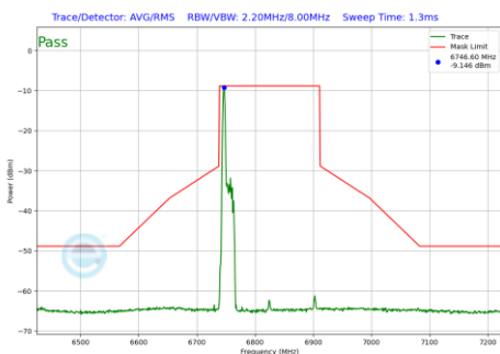
Plot 7-672 In-Band Emission Plot SDM Diversity Antenna WF7 (160MHz BW 802.11be(RU) RU26 Index0 (UNII Band 7) - Ch.175)
