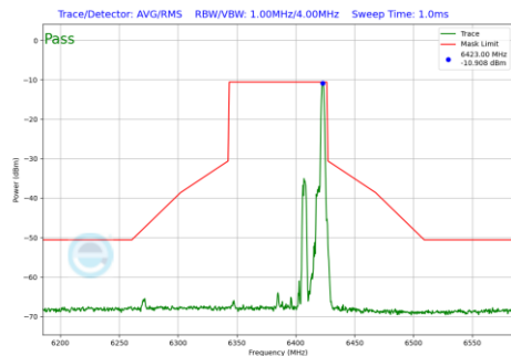
Plot 7-663 In-Band Emission Plot SDM Diversity Antenna WF7 (80MHz BW 802.11be(RU) RU26 Index36 (UNII Band 5) - Ch.87)
