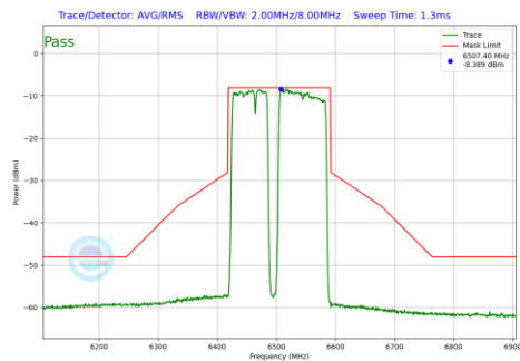
Plot 7-710 In-Band Emission Plot SDM Diversity Antenna WF8 (160MHz BW 802.11be(RU) RU996+484+242 Index99 (UNII Band 6) - Ch.111)
