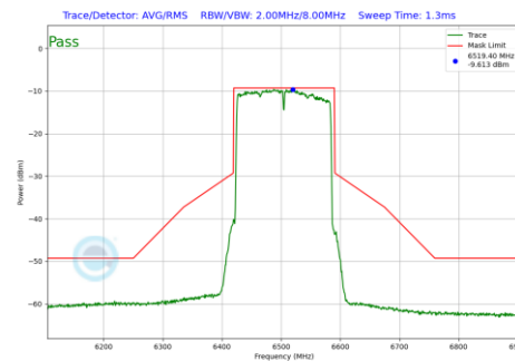
Plot 7-724 In-Band Emission Plot SDM Diversity Antenna WF7 (160MHz BW 802.11be(RU) RU996X2 Index68 (UNII Band 6) - Ch.111)
