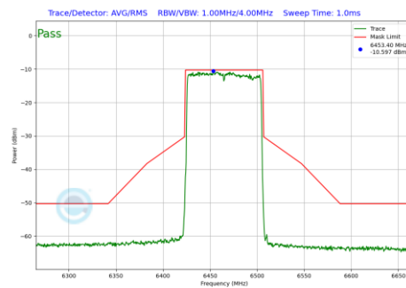
Plot 7-651 In-Band Emission Plot SDM Primary Antenna WF8 (80MHz BW 802.11be(RU) RU996 Index67 (UNII Band 6) - Ch.103)
