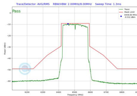
Plot 7-636 In-Band Emission Plot SDM Primary Antenna WF5B (160MHz BW 802.11be(RU) RU996X2 Index68 (UNII Band 6) - Ch.111)
