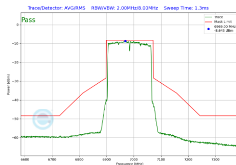
Plot 7-644 In-Band Emission Plot SDM Primary Antenna WF5B (160MHz BW 802.11be(RU) RU996X2 Index68 (UNII Band 8) - Ch.207)
