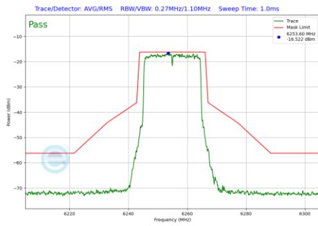
Plot 7-717 In-Band Emission Plot SDM Diversity Antenna WF7 (20MHz BW 802.11be(RU) RU242 Index61 (UNII Band 5) - Ch.61)
