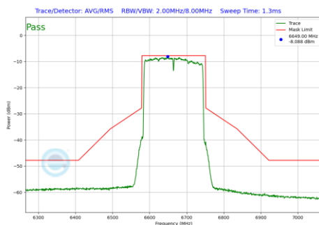
Plot 7-640 In-Band Emission Plot SDM Primary Antenna WF5B (160MHz BW 802.11be(RU) RU996X2 Index68 (UNII Band 7) - Ch.143)
