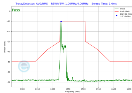
Plot 7-683 In-Band Emission Plot SDM Diversity Antenna WF8 (80MHz BW 802.11be(RU) RU26 Index0 (UNII Band 6) - Ch.103)
