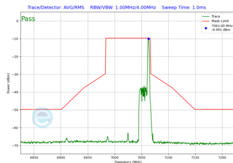
Plot 7-691 In-Band Emission Plot SDM Diversity Antenna WF8 (80MHz BW 802.11be(RU) RU26 Index36 (UNII Band 8) - Ch.215)
