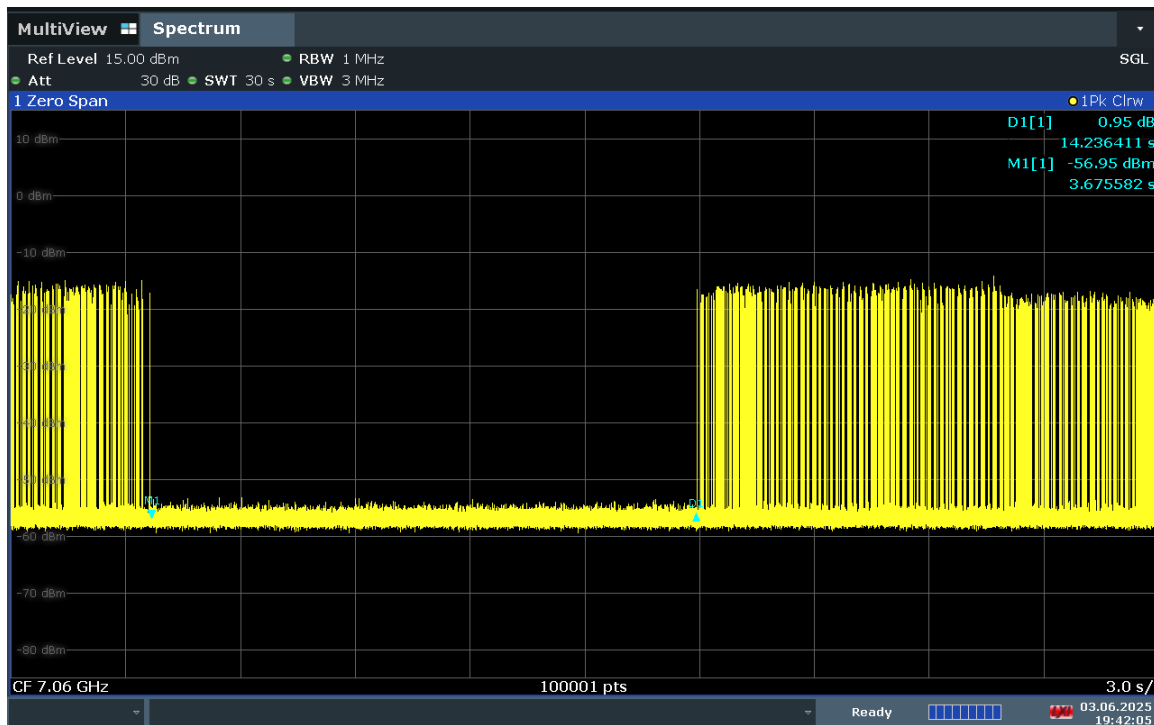
Plot 7-779. Contention Based Protocol Timing Plot – UNII 8 – 160MHz Channel 207 – Mid
