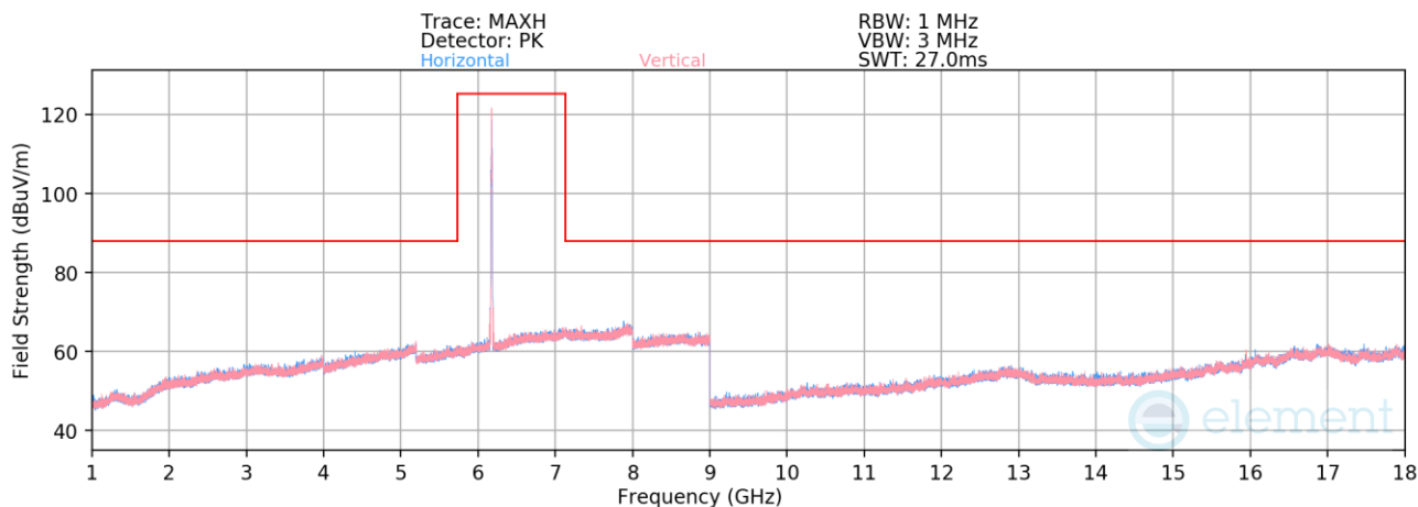
Plot 7-816. Radiated Spurious Emissions above 1GHz SDM Diversity (802.11be – Ch. 33 – RU26)
