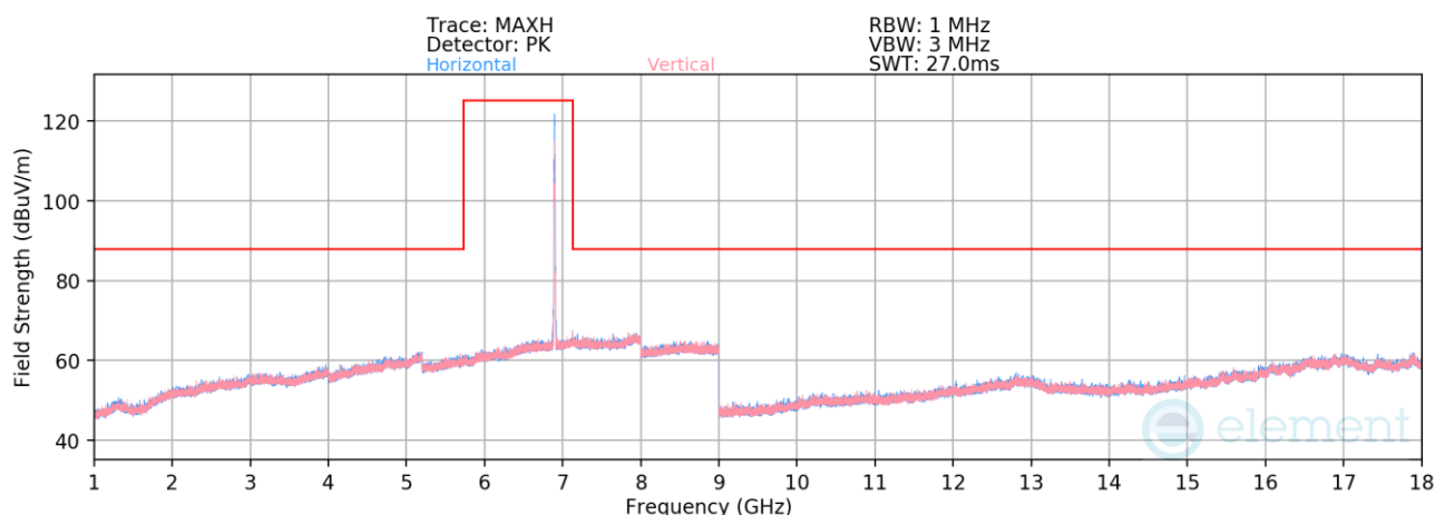
Plot 7-796. Radiated Spurious Emissions above 1GHz SDM Primary (802.11be – Ch. 189 – RU26)
