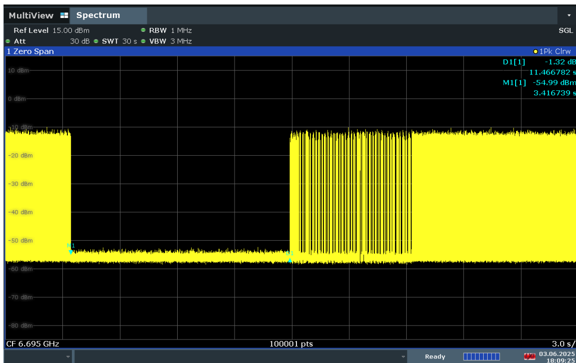
Plot 7-773. Contention Based Protocol Timing Plot – UNII 7 – 20MHz Channel 149
