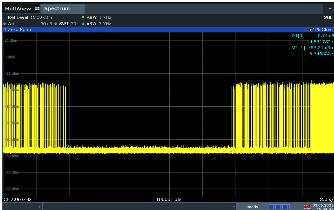
Plot 7-780. Contention Based Protocol Timing Plot – UNII 8 – 160MHz Channel 207 – High
