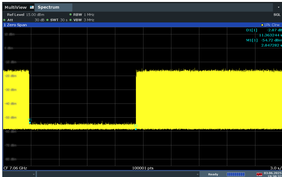
Plot 7-778. Contention Based Protocol Timing Plot – UNII 8 – 160MHz Channel 207 – Low
