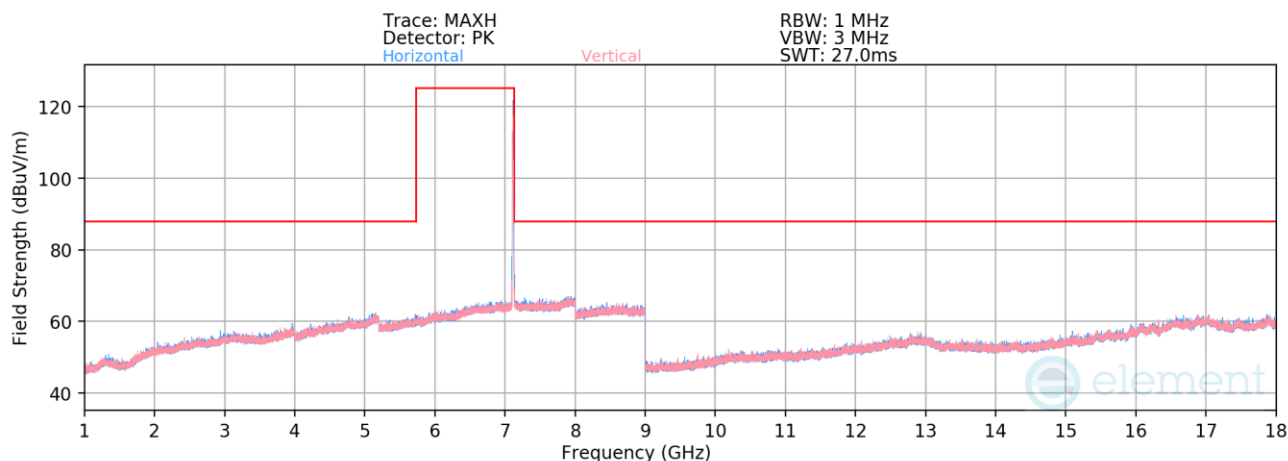
Plot 7-799. Radiated Spurious Emissions above 1GHz SDM Primary (802.11be – Ch. 229 – RU26)
