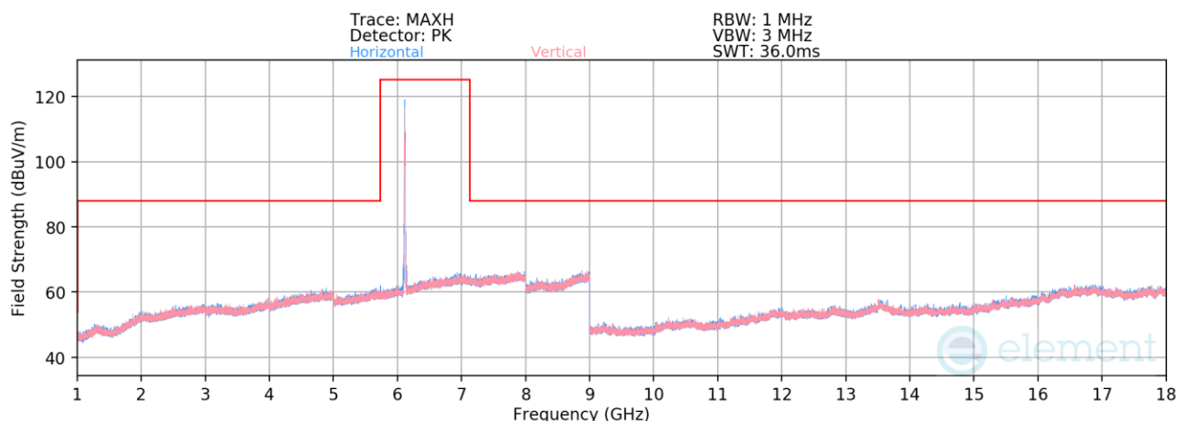
Plot 7-784. Radiated Spurious Emissions above 1GHz SDM Primary (802.11be – Ch. 33 – RU26)
