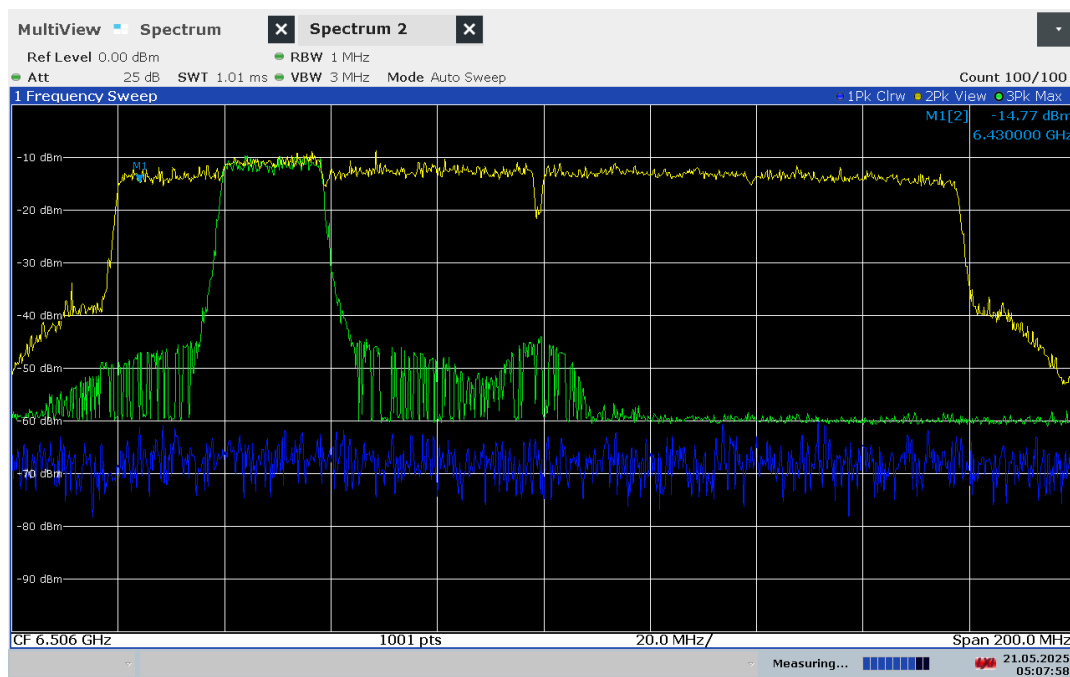
Plot 7-781. 160MHz Bandwidth, AWGN Signal Injected – 6430Mhz
