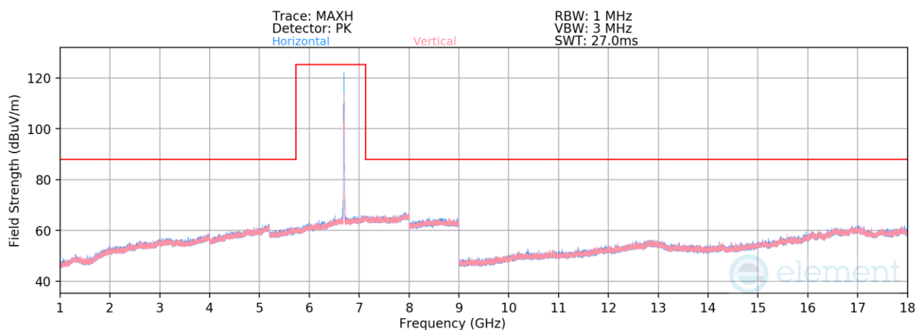
Plot 7-793. Radiated Spurious Emissions above 1GHz SDM Primary (802.11be – Ch. 149 – RU26)
