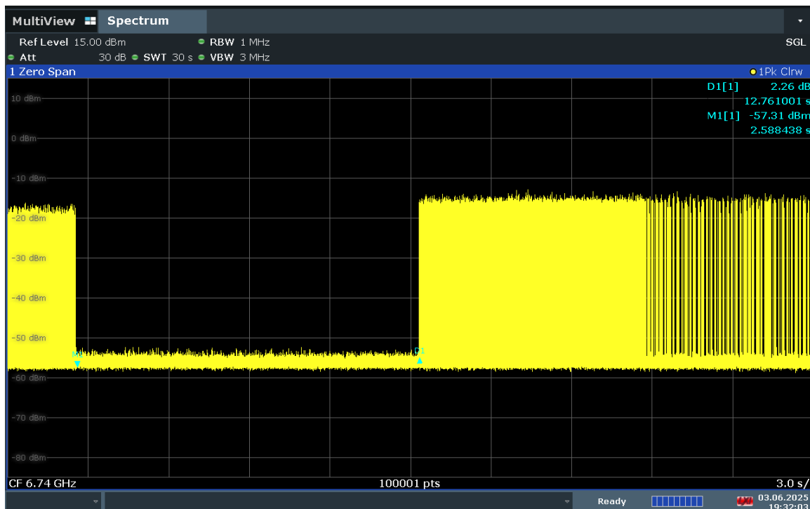
Plot 7-776. Contention Based Protocol Timing Plot – UNII 7 – 160MHz Channel 143 – High
