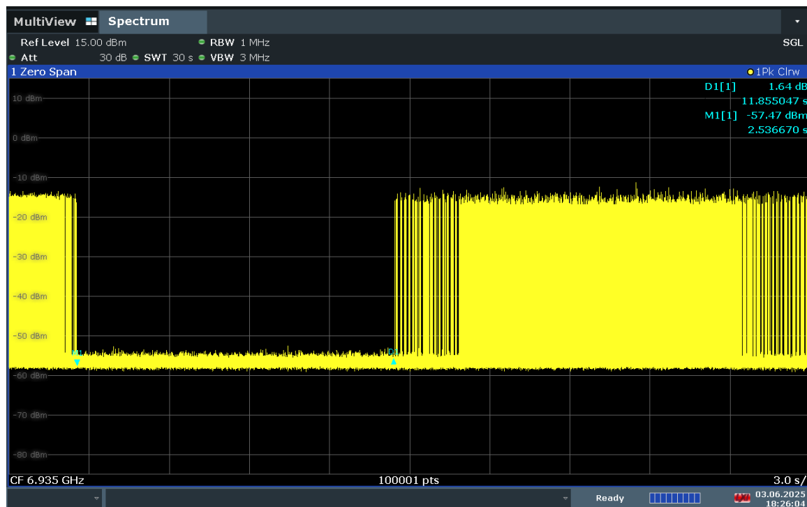
Plot 7-777. Contention Based Protocol Timing Plot – UNII 8 – 20MHz Channel 197
