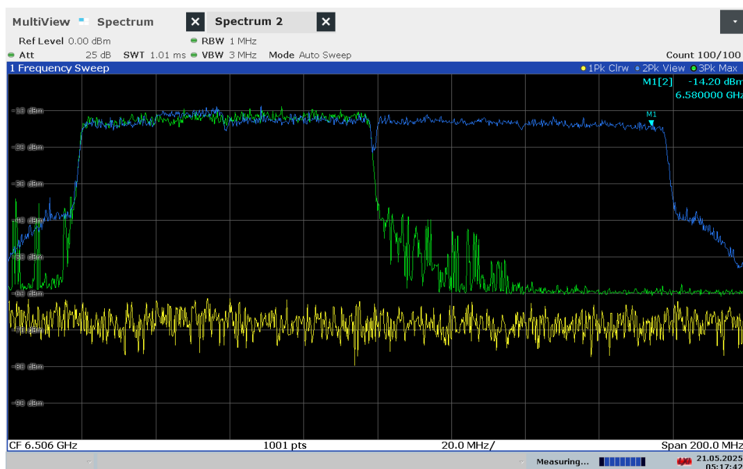
Plot 7-783. 160MHz Bandwidth, AWGN Signal Injected – 6580MHz
