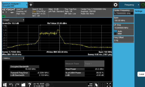
Plot 7-35 6dB BW & 99% OBW Antenna WF5B (40MHz BW 802.11be(RU) RU26 Index8 - Ch.151)
