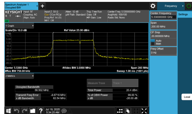
Plot 7-28 26dB BW & 99% OBW Antenna WF7 (80MHz BW 802.11be(RU) RU484+242 Index93 - Ch.106)
