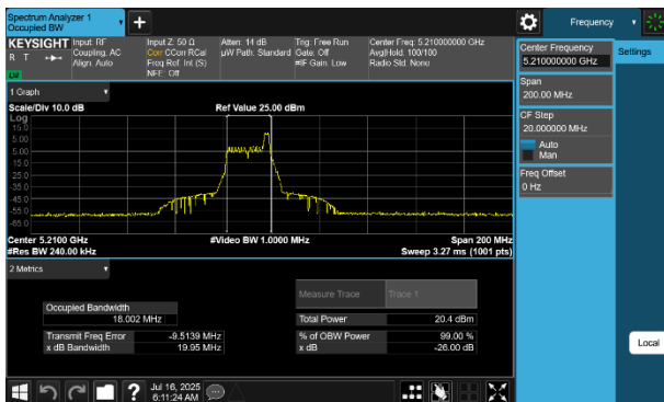
Plot 7-3 26dB BW & 99% OBW Antenna WF5B (80MHz BW 802.11be(RU) RU26 Index17 - Ch.42)
