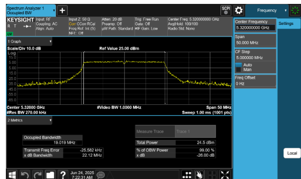
Plot 7-30 26dB BW & 99% OBW Antenna WF7 (20MHz BW 802.11be(RU) RU242 Index61 - Ch.64)
