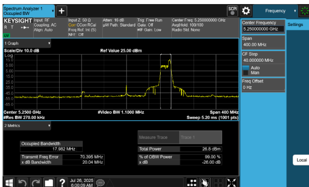
Plot 7-26 26dB BW & 99% OBW Antenna WF7 (160MHz BW 802.11be(RU) RU52 Index52 - Ch.50)
