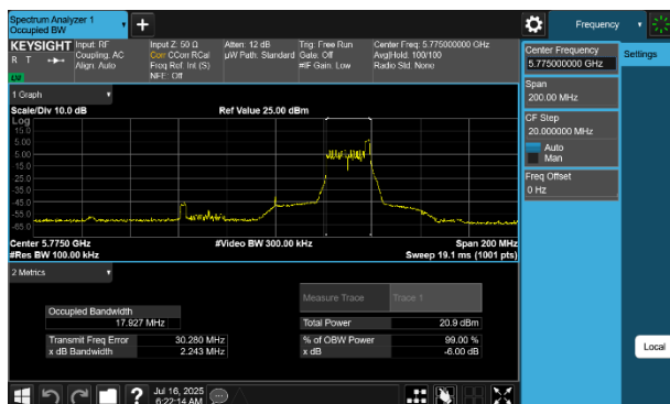
Plot 7-36 6dB BW & 99% OBW Antenna WF5B (80MHz BW 802.11be(RU) RU26 Index36 - Ch.155)
