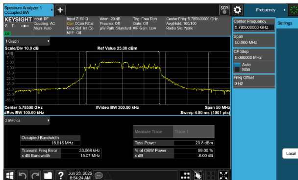
Plot 7-37 6dB BW & 99% OBW Antenna WF5B (20MHz BW 802.11be(RU) RU52+26 Index71 - Ch.157)
