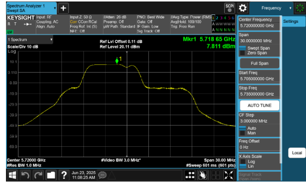
Plot 7-62 PSD Antenna WF5B (20MHz BW 802.11be(RU) RU52+26 Index71 - Ch.144)
