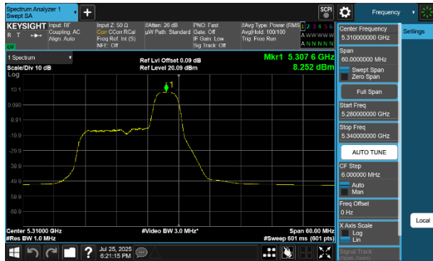
Plot 7-59 PSD Antenna WF5B (40MHz BW 802.11be(RU) RU52 Index40 - Ch.62)
