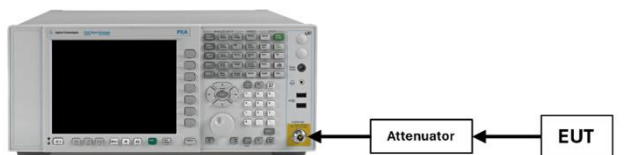
Figure 7-4. Test Instrument & Measurement Setup
