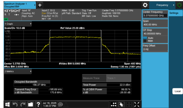
Plot 7-22 26dB BW & 99% OBW Antenna WF8 (160MHz BW 802.11be(RU) RU996X2 Index68 - Ch.114)
