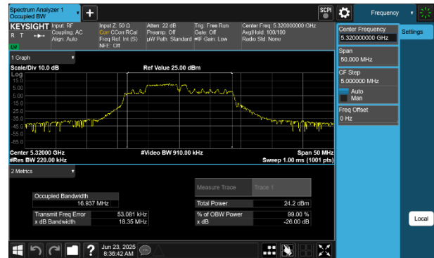
Plot 7-5 26dB BW & 99% OBW Antenna WF5B (20MHz BW 802.11be(RU) RU52+26 Index71 - Ch.64)
