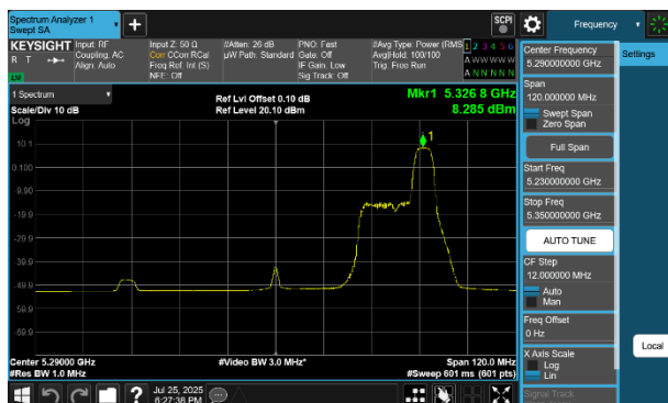
Plot 7-60 PSD Antenna WF5B (80MHz BW 802.11be(RU) RU52 Index52 - Ch.58)
