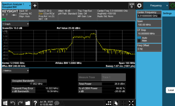
Plot 7-24 26dB BW & 99% OBW Antenna WF7 (40MHz BW 802.11be(RU) RU52 Index44 - Ch.102)
