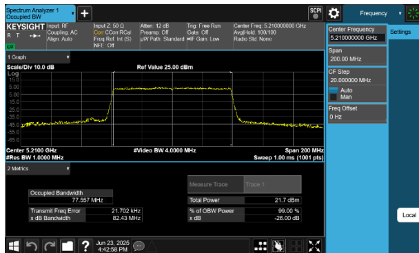
Plot 7-21 26dB BW & 99% OBW Antenna WF8 (80MHz BW 802.11be(RU) RU996 Index67 - Ch.42)
