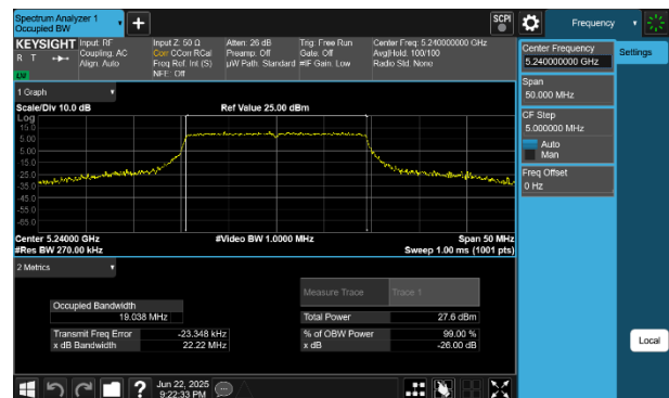
Plot 7-8 26dB BW & 99% OBW Antenna WF5B (20MHz BW 802.11be(RU) RU242 Index61 - Ch.48)
