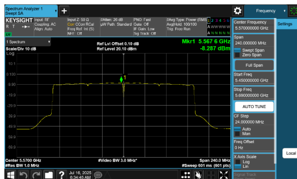
Plot 7-68 PSD Antenna WF5B (160MHz BW 802.11be(RU) RU996X2 Index68 - Ch.114)
