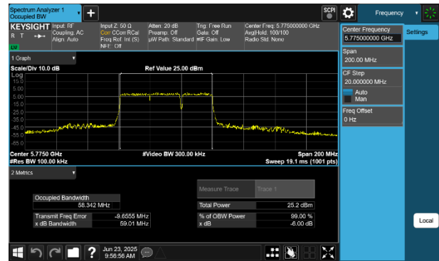
Plot 7-38 6dB BW & 99% OBW Antenna WF5B (80MHz BW 802.11be(RU) RU484+242 Index93 - Ch.155)
