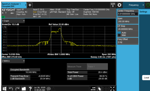
Plot 7-25 26dB BW & 99% OBW Antenna WF7 (80MHz BW 802.11be(RU) RU52 Index44 - Ch.122)
