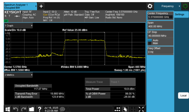
Plot 7-7 26dB BW & 99% OBW Antenna WF5B (160MHz BW 802.11be(RU) RU996+484 Index94 - Ch.114)
