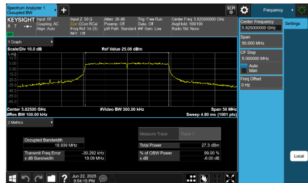
Plot 7-39 6dB BW & 99% OBW Antenna WF5B (20MHz BW 802.11be(RU) RU242 Index61 - Ch.165)
