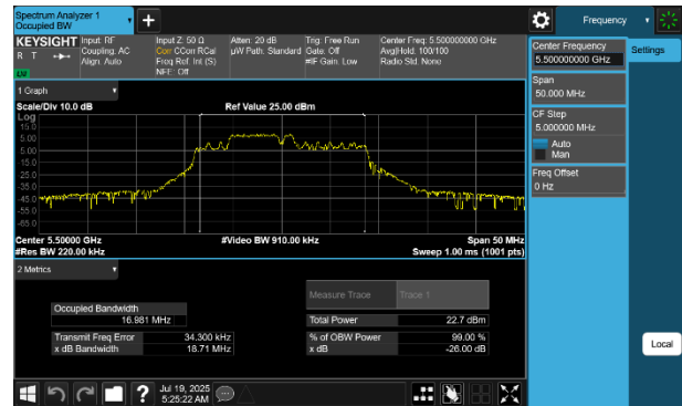
Plot 7-27 26dB BW & 99% OBW Antenna WF7 (20MHz BW 802.11be(RU) RU52+26 Index71 - Ch.100)
