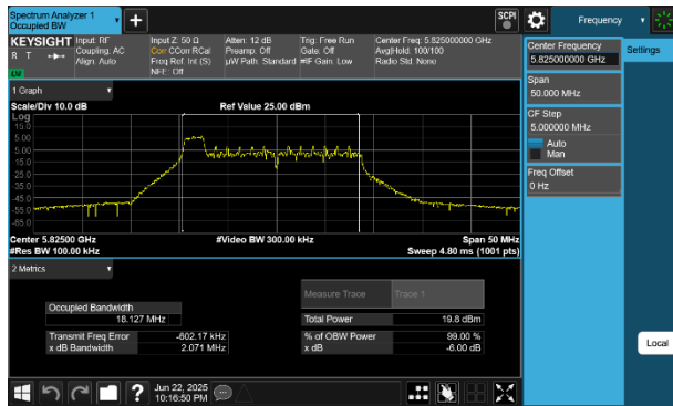
Plot 7-34 6dB BW & 99% OBW Antenna WF5B (20MHz BW 802.11be(RU) RU26 Index0 - Ch.165)
