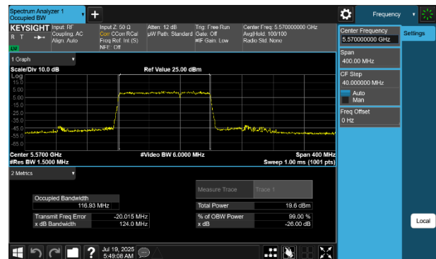
Plot 7-29 26dB BW & 99% OBW Antenna WF7 (160MHz BW 802.11be(RU) RU996+484 Index95 - Ch.114)
