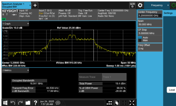
Plot 7-23 26dB BW & 99% OBW Antenna WF7 (20MHz BW 802.11be(RU) RU26 Index4 - Ch.40)
