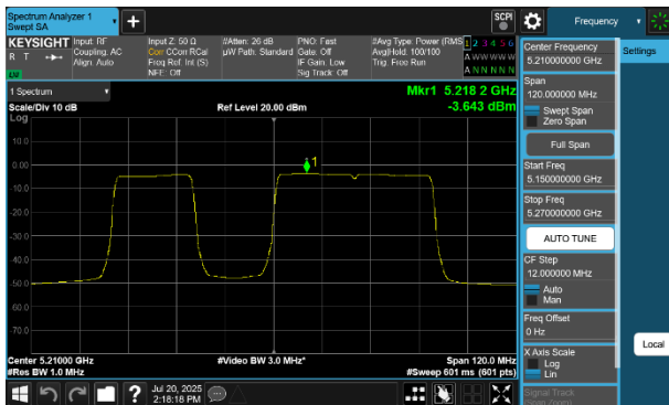
Plot 7-255 PSD CDD Diversity Antenna WF7 (80MHz BW 802.11be(RU) RU484+242 Index91 - Ch.42)
