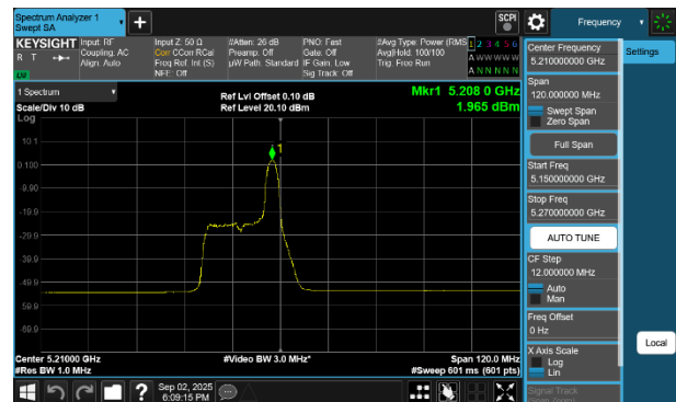
Plot 7-252 PSD SDM Diversity Antenna WF8 (80MHz BW 802.11be(RU) RU26 Index17 - Ch.42)
