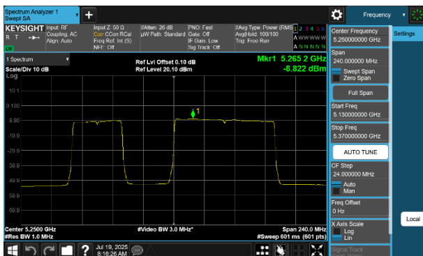
Plot 7-256 PSD CDD Diversity Antenna WF7 (160MHz BW 802.11be(RU) RU996+484 Index95 - Ch.50)
