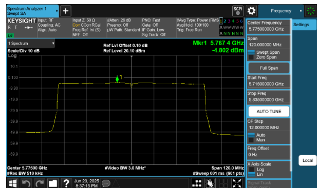
Plot 7-245 PSD CDD Diversity Antenna WF8 (80MHz BW 802.11be(RU) RU996 Index67 - Ch.155)
