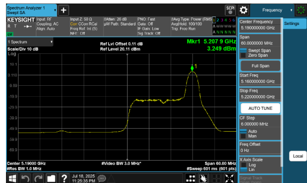
Plot 7-251 PSD SDM Diversity Antenna WF8 (40MHz BW 802.11be(RU) RU26 Index17 - Ch.38)
