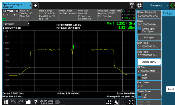
Plot 7-263 PSD CDD Diversity Antenna WF7 (160MHz BW 802.11be(RU) RU996X2 Index68 - Ch.50)
