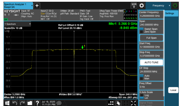
Plot 7-267 PSD CDD Diversity Antenna WF8 (160MHz BW 802.11be(RU) RU996X2 Index68 - Ch.50)
