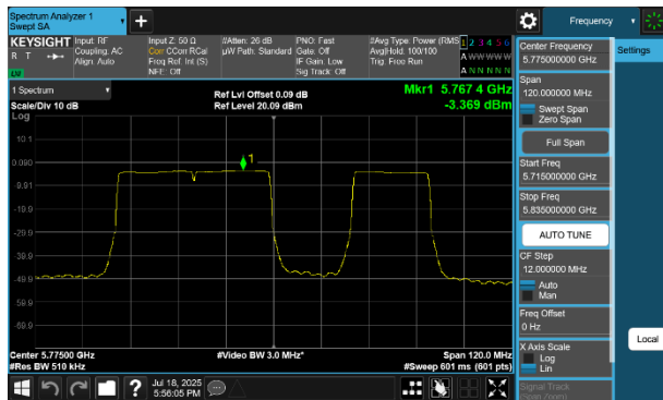
Plot 7-239 PSD CDD Diversity Antenna WF8 (80MHz BW 802.11be(RU) RU484+242 Index92 - Ch.155)
