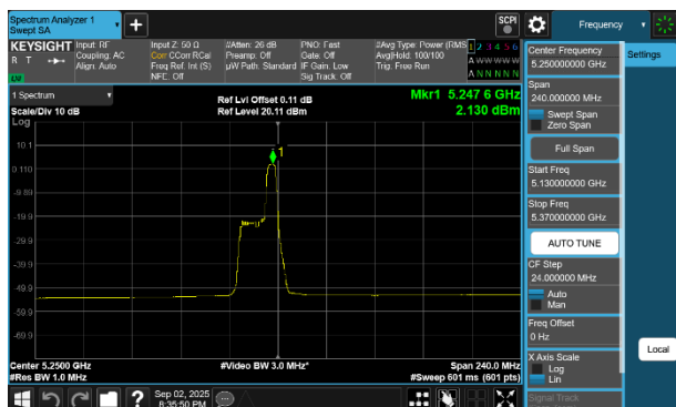
Plot 7-249 PSD SDM Diversity Antenna WF7 (80MHz BW 802.11be(RU) RU26 Index52-L - Ch.50)
