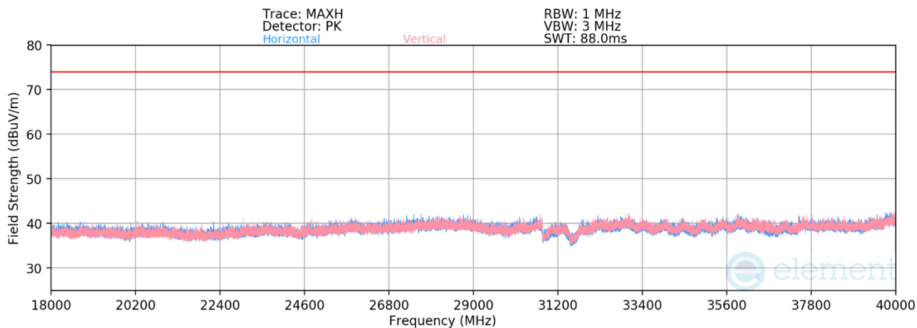
Plot 7-270. RSE 18GHz – 40 GHz CDD Primary (11be Ch.40 — RU26)
