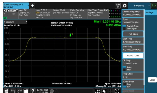
Plot 7-260 PSD SDM Diversity Antenna WF7 (20MHz BW 802.11be(RU) RU242 Index61 - Ch.40)
