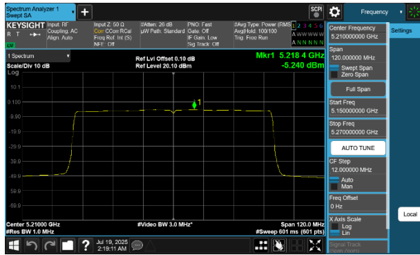
Plot 7-262 PSD CDD Diversity Antenna WF7 (80MHz BW 802.11be(RU) RU996 Index67 - Ch.42)
