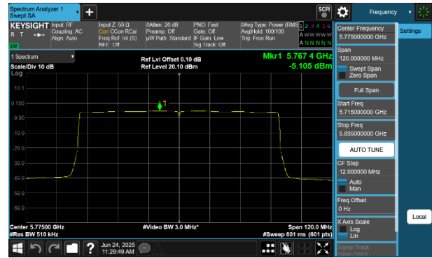
Plot 7-242 PSD CDD Diversity Antenna WF7 (80MHz BW 802.11be(RU) RU996 Index67 - Ch.155)
