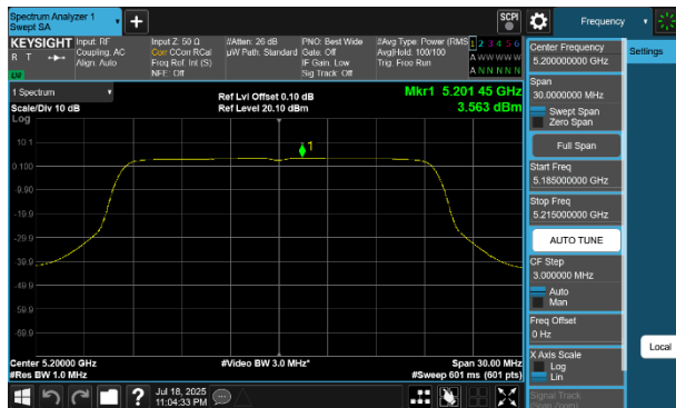
Plot 7-264 PSD SDM Diversity Antenna WF8 (20MHz BW 802.11be(RU) RU242 Index61 - Ch.40)
