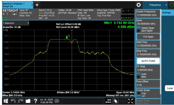
Plot 7-238 PSD CDD Diversity Antenna WF8 (20MHz BW 802.11be(RU) RU52+26 Index71 - Ch.149)
