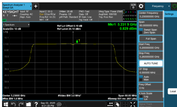
Plot 7-265 PSD SDM Diversity Antenna WF8 (40MHz BW 802.11be(RU) RU484 Index65 - Ch.46)
