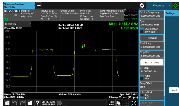
Plot 7-259 PSD CDD Diversity Antenna WF8 (160MHz BW 802.11be(RU) RU996+484 Index95 - Ch.50)
