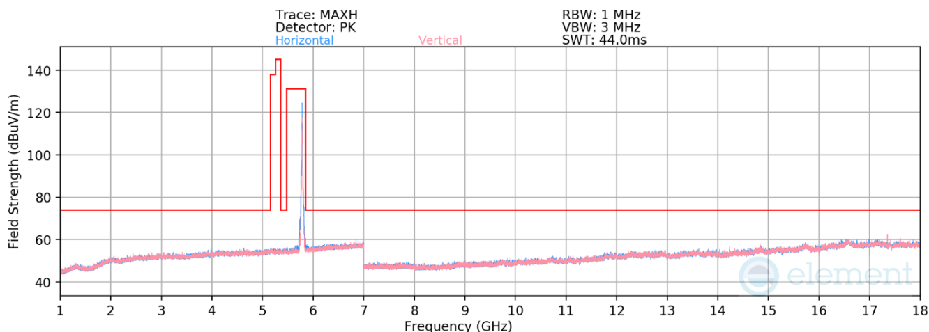
Plot 7-281. RSE above 1GHz CDD Primary (11be – Ch.157 – RU26)
