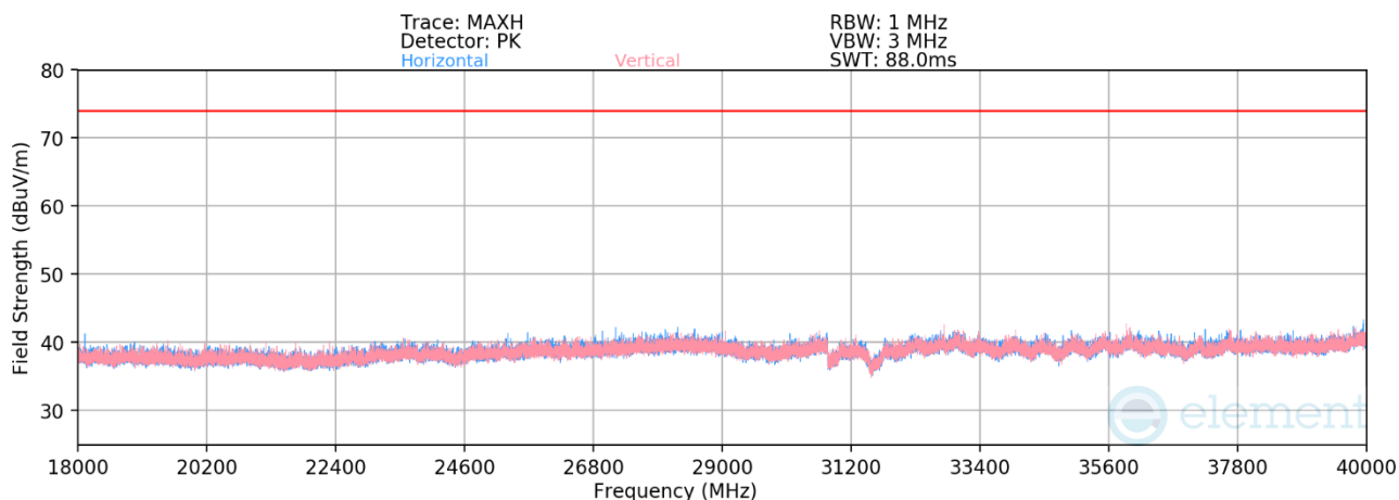
Plot 7-278. RSE 18GHz – 40 GHz CDD Primary (11be Ch.116 — RU52)
