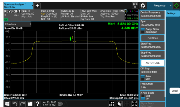
Plot 7-243 PSD CDD Diversity Antenna WF8 (20MHz BW 802.11be(RU) RU242 Index61 - Ch.165)
