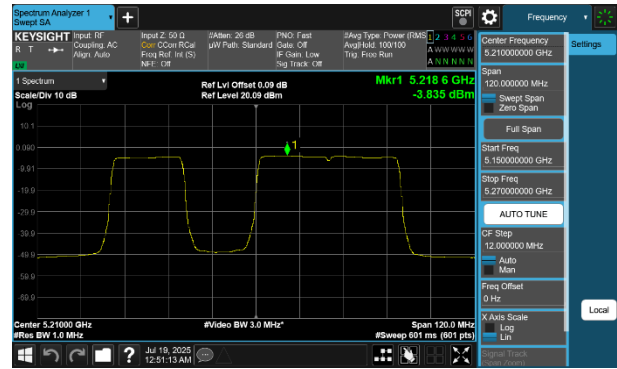
Plot 7-258 PSD CDD Diversity Antenna WF8 (80MHz BW 802.11be(RU) RU484+242 Index91 - Ch.42)
