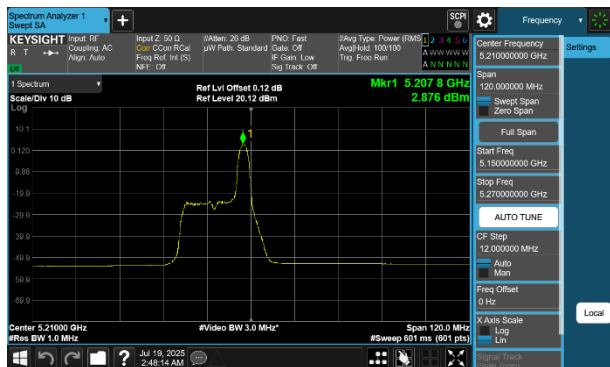
Plot 7-248 PSD SDM Diversity Antenna WF7 (80MHz BW 802.11be(RU) RU26 Index17 - Ch.42)
