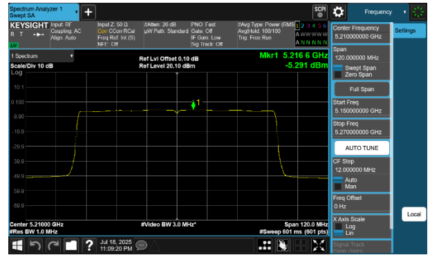
Plot 7-266 PSD CDD Diversity Antenna WF8 (80MHz BW 802.11be(RU) RU996 Index67 - Ch.42)
