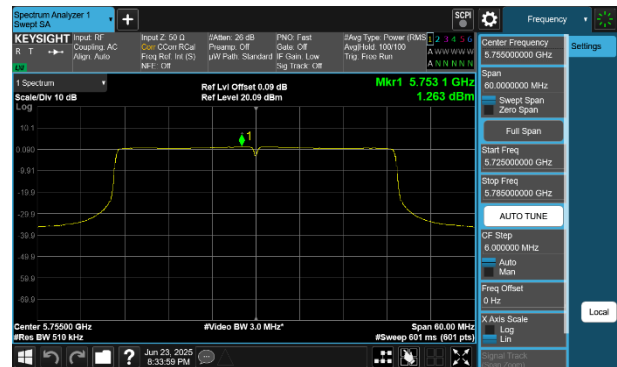
Plot 7-244 PSD CDD Diversity Antenna WF8 (40MHz BW 802.11be(RU) RU484 Index65 - Ch.151)
