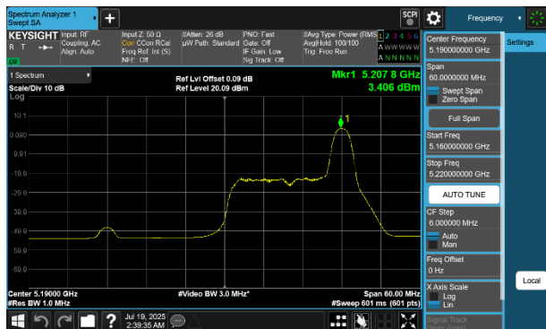
Plot 7-247 PSD SDM Diversity Antenna WF7 (40MHz BW 802.11be(RU) RU26 Index17 - Ch.38)
