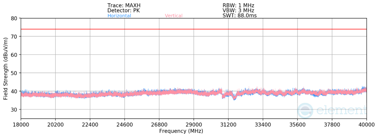
Plot 7-274. RSE 18GHz – 40 GHz CDD Primary (11be Ch.56 — RU52)
