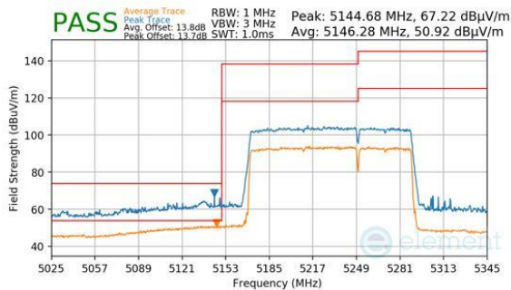
Plot 7-464. Antenna WF5B (Peak & Average, RU996+484+242, Index 95, Ch.50, MCS11)
