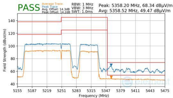
Plot 7-470. Antenna WF5B (Peak & Average, RU996+484+242, Index 97, Ch.50, MCS11)
