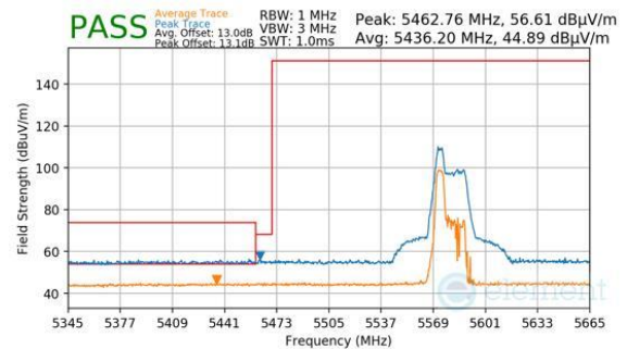
Plot 7-447. Antenna WF5B (Peak & Average, RU52, Index 37, Ch.114 (FCC ONLY), MCS11)
