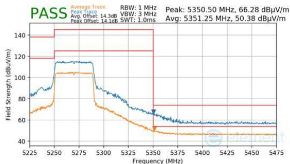
Plot 7-548. Antenna WF8 (Peak & Average, RU484, Index 65, Ch.54, MCS11)
