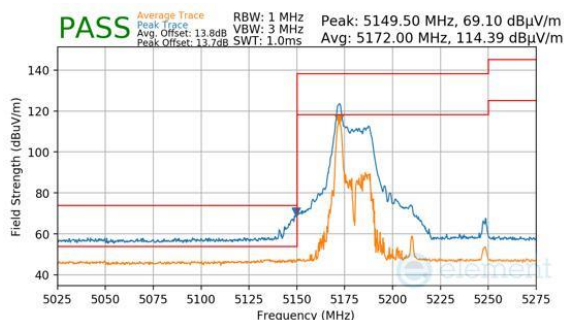
Plot 7-558. Antenna WF8 (Peak & Average, RU26, Index 0, Ch.42, MCS11)
