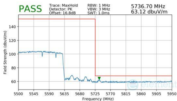
Plot 7-487. Antenna WF5B (Peak, RU996+484+242, Index 99 (H), Ch.114 (FCC ONLY), MCS11)
