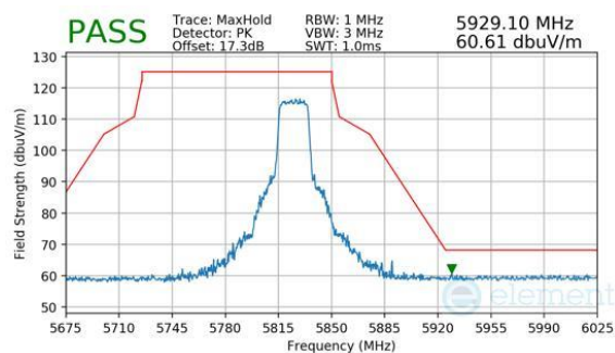
Plot 7-531. Antenna WF8 (Peak, RU242, Index 61, Ch.165, MCS11)
