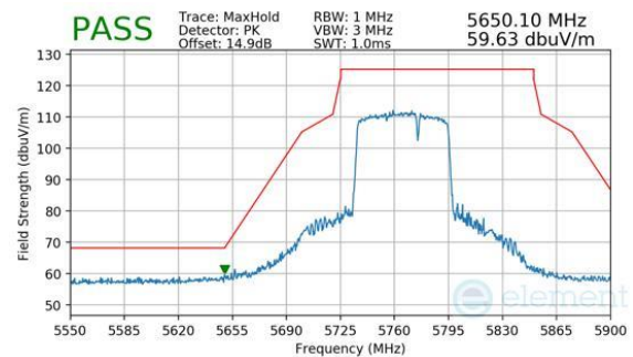
Plot 7-431. Antenna WF5B (Peak, RU484+242, Index 93, Ch.155, MCS11)
