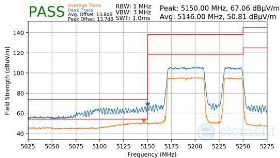
Plot 7-572. Antenna WF8 (Peak & Average, RU484+242, Index 92, Ch.42, MCS11)
