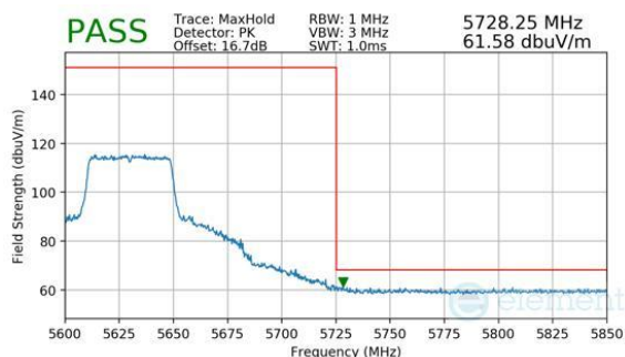
Plot 7-554. Antenna WF8 (Peak, RU484, Index 65, Ch.126 (FCC ONLY), MCS11)
