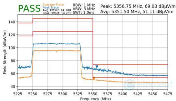
Plot 7-437. Antenna WF5B (Peak & Average, RU996, Index 67, Ch.58, MCS11)
