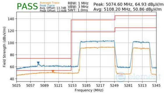
Plot 7-463. Antenna WF5B (Peak & Average, RU996+484+242, Index 94, Ch.50, MCS11)
