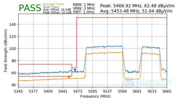
Plot 7-456. Antenna WF5B (Peak & Average, RU996+484, Index 94 (H), Ch.114 (FCC ONLY), MCS11)
