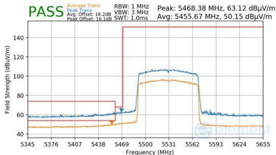
Plot 7-438. Antenna WF5B (Peak & Average, RU996, Index 67, Ch.106, MCS11)
