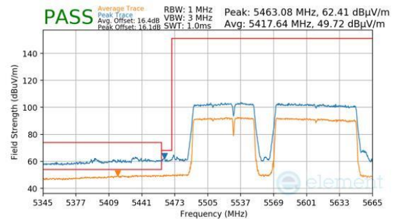
Plot 7-479. Antenna WF5B (Peak & Average, RU996+484+242, Index 99 (L), Ch.114 (FCC ONLY), MCS11)
