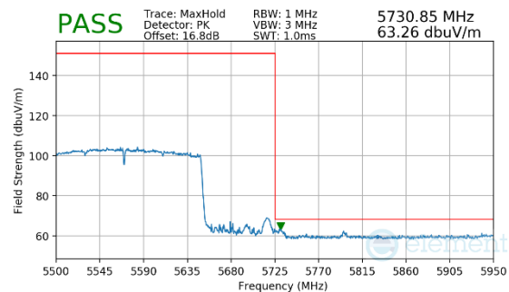
Plot 7-492. Antenna WF5B (Peak RU996X2, Index 68, Ch.114, MCS11)
