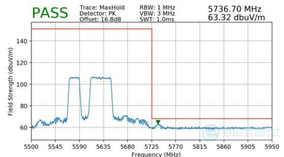
Plot 7-425. Antenna WF5B (Peak, RU484+242, Index 91, Ch.122 (FCC ONLY), MCS11)
