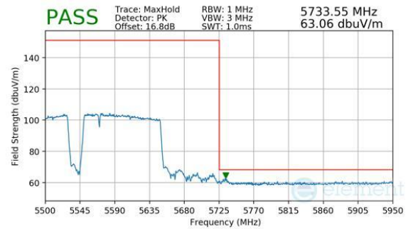
Plot 7-485. Antenna WF5B (Peak, RU996+484+242, Index 98 (L), Ch.114 (FCC ONLY), MCS11)
