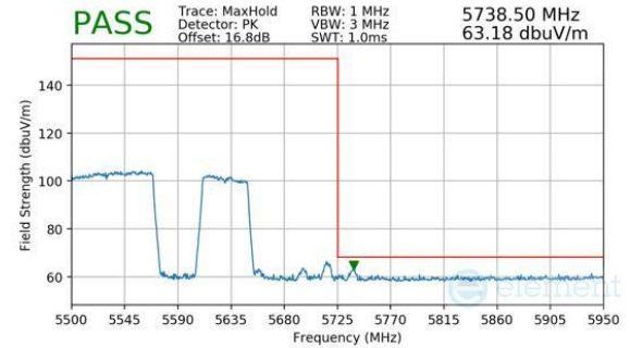
Plot 7-460. Antenna WF5B (Peak, RU996+484, Index 94 (H), Ch.114 (FCC ONLY), MCS11)
