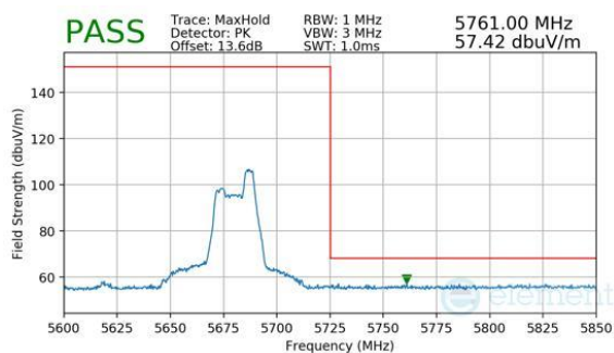
Plot 7-545. Antenna WF8 (Peak, RU52, Index 44, Ch.134, MCS11)
