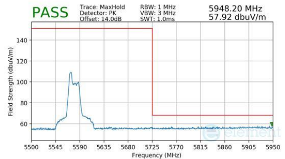
Plot 7-406. Antenna WF5B (Peak, RU52, Index 37, Ch.122 (FCC ONLY), MCS11)
