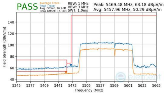
Plot 7-458. Antenna WF5B (Peak & Average, RU996+484, Index 95 (H), Ch.114 (FCC ONLY), MCS11)
