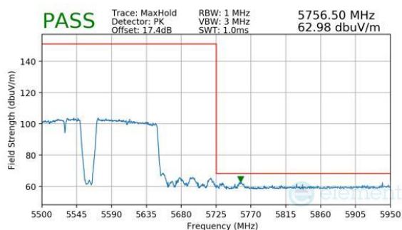
Plot 7-488. Antenna WF5B (Peak, RU996+484+242, Index 99 (L), Ch.114 (FCC ONLY), MCS11)
