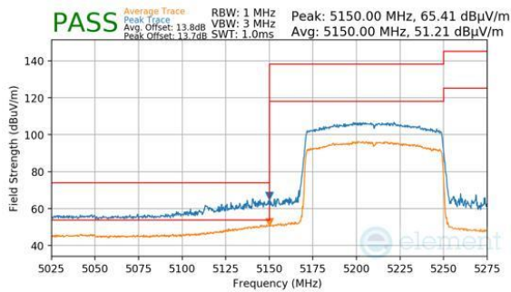
Plot 7-436. Antenna WF5B (Peak & Average, RU996, Index 67, Ch.42, MCS11)
