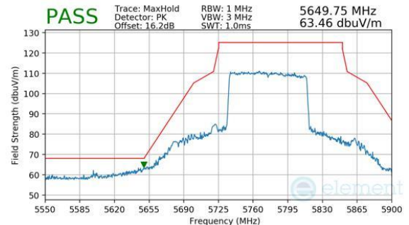
Plot 7-441. Antenna WF5B (Peak, RU996, Index 67, Ch.155, MCS11)
