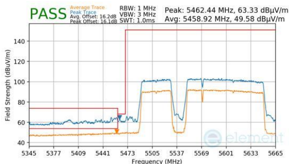
Plot 7-477. Antenna WF5B (Peak & Average, RU996+484+242, Index 98 (L), Ch.114 (FCC ONLY), MCS11)
