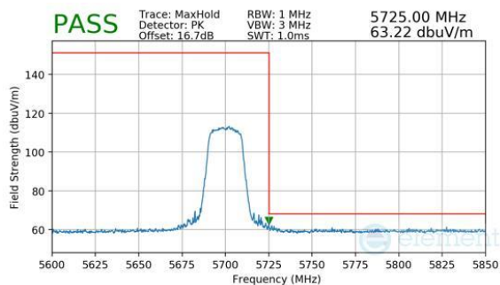
Plot 7-529. Antenna WF8 (Peak, RU242, Index 61, Ch.140, MCS11)
