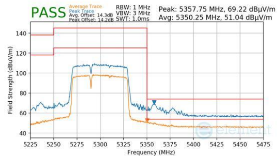
Plot 7-574. Antenna WF8 (Peak & Average, RU484+242, Index 90, Ch.58, MCS11)
