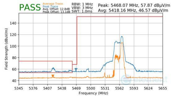
Plot 7-567. Antenna WF8 (Peak & Average, RU52, Index 52, Ch.106, MCS11)
