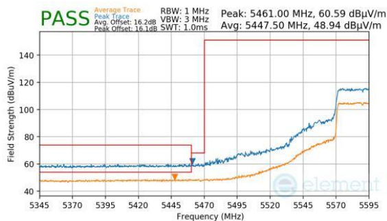
Plot 7-552. Antenna WF8 (Peak & Average, RU484, Index 65, Ch.118 (FCC ONLY), MCS11)
