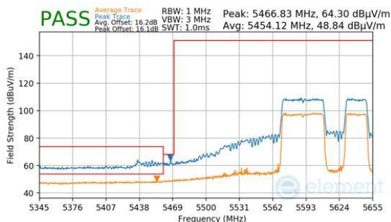
Plot 7-422. Antenna WF5B (Peak & Average, RU484+242, Index 92, Ch.122 (FCC ONLY), MCS11)
