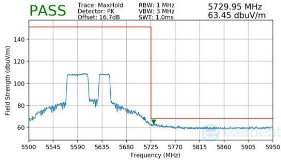
Plot 7-426. Antenna WF5B (Peak, RU484+242, Index 92, Ch.122 (FCC ONLY), MCS11)
