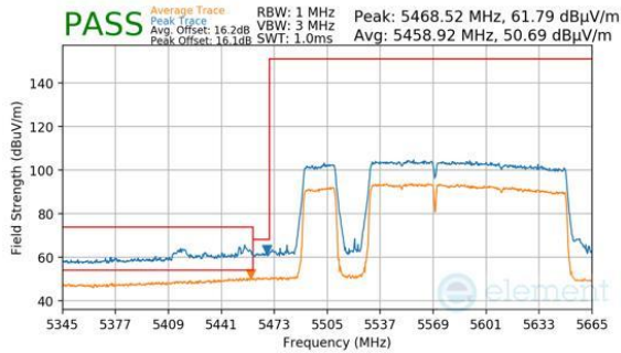
Plot 7-475. Antenna WF5B (Peak & Average, RU996+484+242, Index 97 (L), Ch.114 (FCC ONLY), MCS11)
