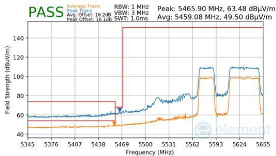
Plot 7-421. Antenna WF5B (Peak & Average, RU484+242, Index 91, Ch.122 (FCC ONLY), MCS11)
