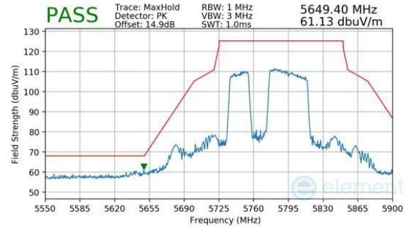
Plot 7-429. Antenna WF5B (Peak, RU484+242, Index 91, Ch.155, MCS11)
