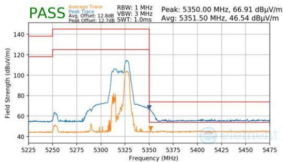
Plot 7-403. Antenna WF5B (Peak & Average, RU52, Index 52, Ch.58, MCS11)
