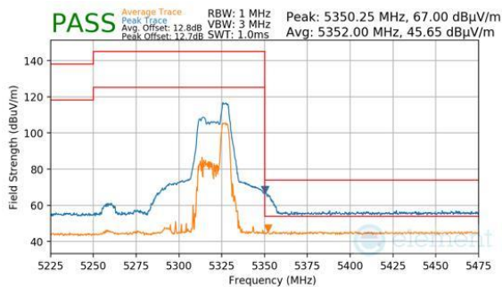
Plot 7-539. Antenna WF8 (Peak & Average, RU52, Index 44, Ch.62, MCS11)
