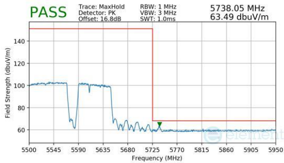
Plot 7-481. Antenna WF5B (Peak, RU996+484+242, Index 96 (H), Ch.114 (FCC ONLY), MCS11)
