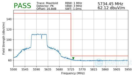
Plot 7-427. Antenna WF5B (Peak, RU484+242, Index 93, Ch.122 (FCC ONLY), MCS11)
