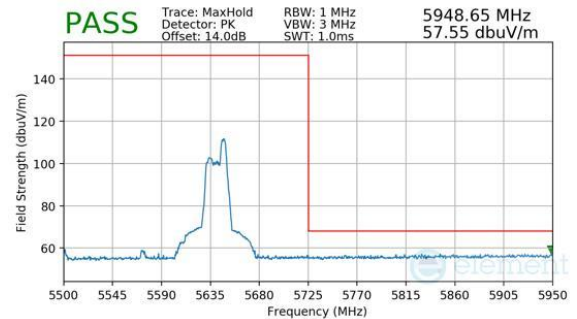
Plot 7-407. Antenna WF5B (Peak, RU52, Index 52, Ch.122 (FCC ONLY), MCS11)
