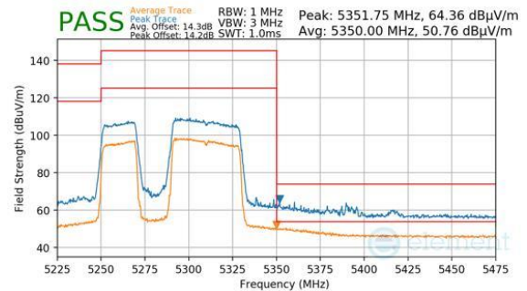
Plot 7-575. Antenna WF8 (Peak & Average, RU484+242, Index 91, Ch.58, MCS11)
