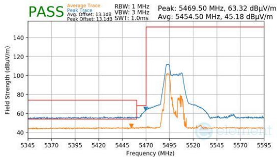
Plot 7-540. Antenna WF8 (Peak & Average, RU52, Index 37, Ch.102, MCS11)
