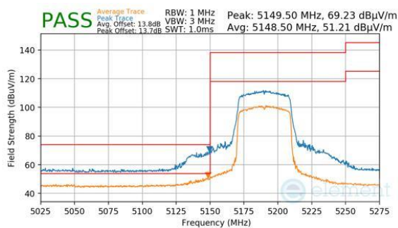
Plot 7-546. Antenna WF8 (Peak & Average, RU484, Index 65, Ch.38, MCS11)
