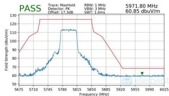
Plot 7-557. Antenna WF8 (Peak, RU484, Index 65, Ch.159, MCS11)
