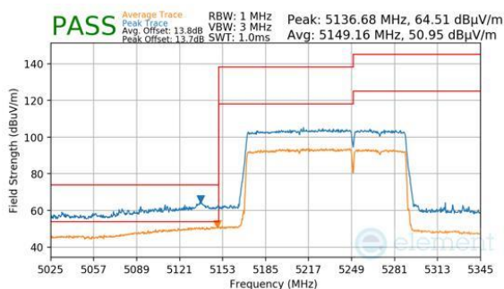
Plot 7-452. Antenna WF5B (Peak & Average, RU996+484, Index 95, Ch.50, MCS11)
