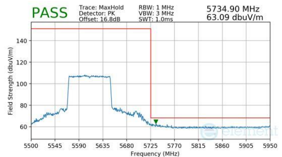
Plot 7-440. Antenna WF5B (Peak, RU996, Index 67, Ch.122 (FCC ONLY), MCS11)
