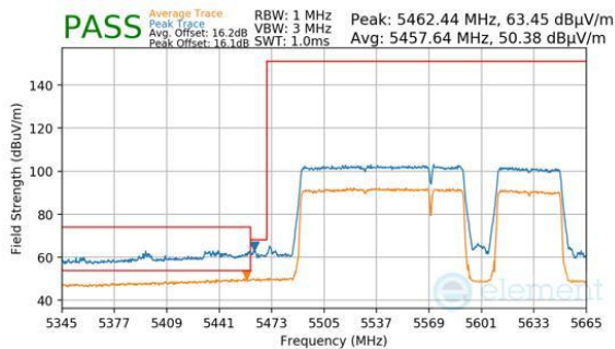
Plot 7-476. Antenna WF5B (Peak & Average, RU996+484+242, Index 97 (H), Ch.114 (FCC ONLY), MCS11)
