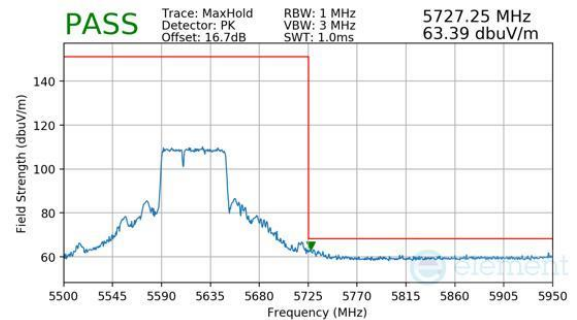
Plot 7-424. Antenna WF5B (Peak, RU484+242, Index 90, Ch.122 (FCC ONLY), MCS11)
