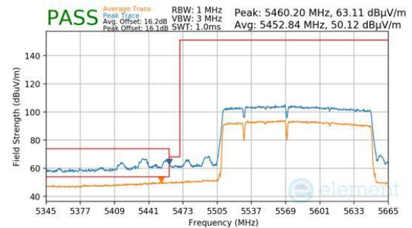
Plot 7-473. Antenna WF5B (Peak & Average, RU996+484+242, Index 96 (L), Ch.114 (FCC ONLY), MCS11)
