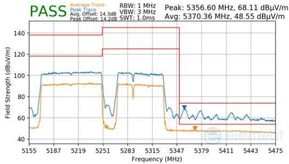
Plot 7-469. Antenna WF5B (Peak & Average, RU996+484+242, Index 96, Ch.50, MCS11)
