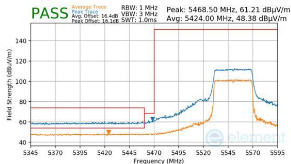
Plot 7-551. Antenna WF8 (Peak & Average, RU484, Index 65, Ch.110, MCS11)
