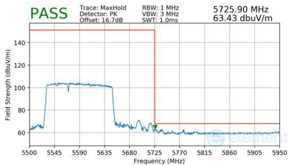
Plot 7-459. Antenna WF5B (Peak, RU996+484, Index 94 (L), Ch.114 (FCC ONLY), MCS11)
