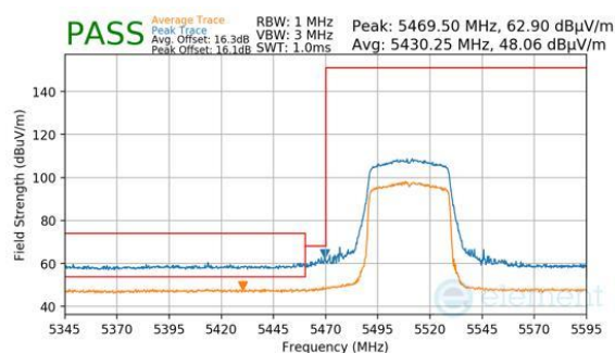
Plot 7-550. Antenna WF8 (Peak & Average, RU484, Index 65, Ch.102, MCS11)
