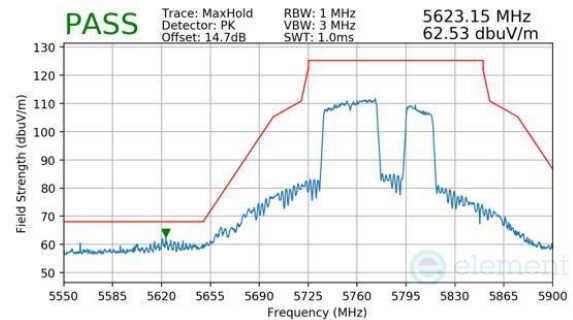
Plot 7-430. Antenna WF5B (Peak, RU484+242, Index 92, Ch.155, MCS11)
