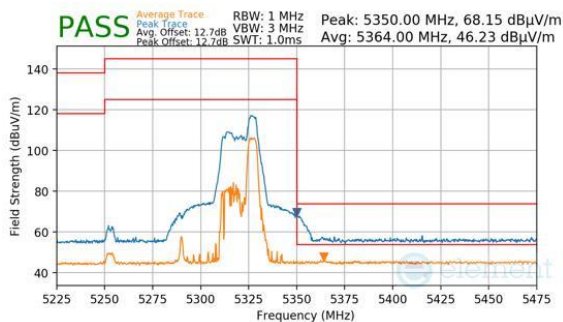
Plot 7-565. Antenna WF8 (Peak & Average, RU52, Index 52, Ch.58, MCS11)
