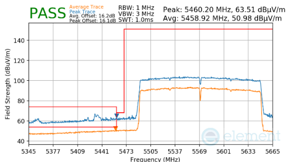
Plot 7-491. Antenna WF5B (Peak & Average, RU996X2, Index 68, Ch.114, MCS11)
