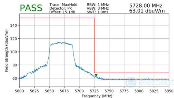
Plot 7-555. Antenna WF8 (Peak, RU484, Index 65, Ch.134, MCS11)
