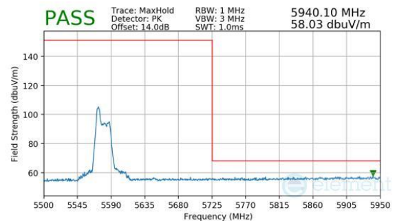
Plot 7-568. Antenna WF8 (Peak, RU52, Index 37, Ch.122 (FCC ONLY), MCS11)
