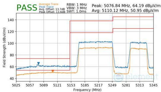
Plot 7-451. Antenna WF5B (Peak & Average, RU996+484, Index 94, Ch.50, MCS11)
