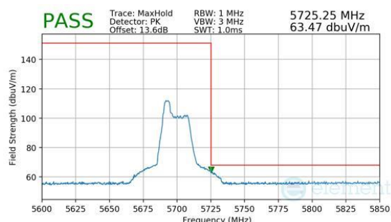
Plot 7-503. Antenna WF8 (Peak, RU52, Index 37, Ch.140, MCS11)
