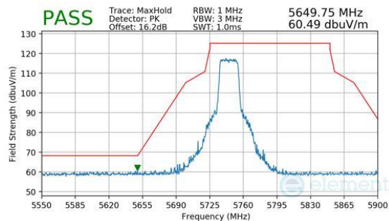
Plot 7-530. Antenna WF8 (Peak, RU242, Index 61, Ch.149, MCS11)
