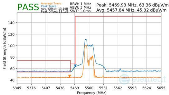
Plot 7-404. Antenna WF5B (Peak & Average, RU52, Index 37, Ch.106, MCS11)
