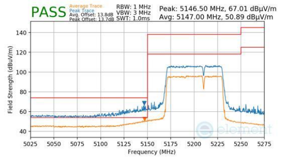
Plot 7-573. Antenna WF8 (Peak & Average, RU484+242, Index 93, Ch.42, MCS11)
