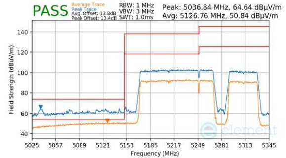
Plot 7-466. Antenna WF5B (Peak & Average, RU996+484+242, Index 97, Ch.50, MCS11)
