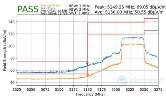
Plot 7-547. Antenna WF8 (Peak & Average, RU484, Index 65, Ch.46, MCS11)
