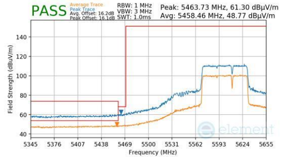
Plot 7-423. Antenna WF5B (Peak & Average, RU484+242, Index 93, Ch.122 (FCC ONLY), MCS11)
