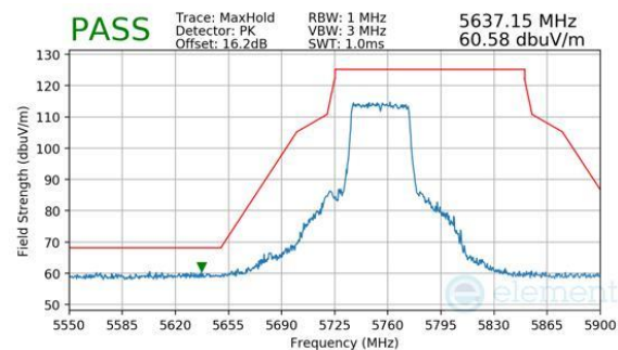
Plot 7-556. Antenna WF8 (Peak, RU484, Index 65, Ch.151, MCS11)
