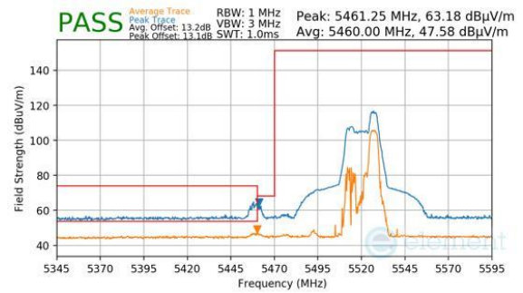
Plot 7-541. Antenna WF8 (Peak & Average, RU52, Index 44, Ch.102, MCS11)
