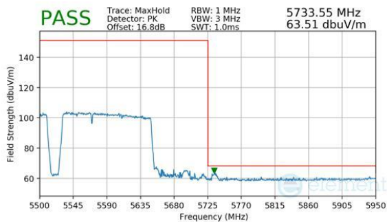
Plot 7-483. Antenna WF5B (Peak, RU996+484+242, Index 97 (L), Ch.114 (FCC ONLY), MCS11)
