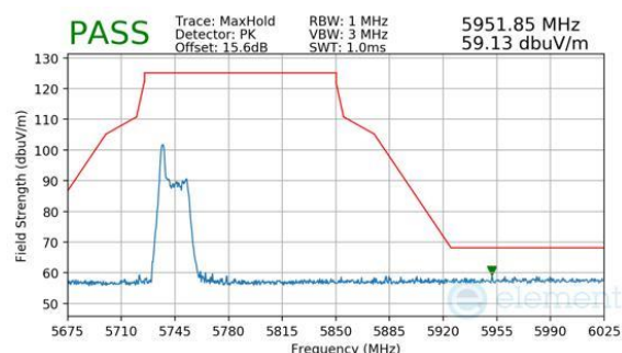
Plot 7-562. Antenna WF8 (Peak, RU26, Index 0, Ch.155, MCS11)
