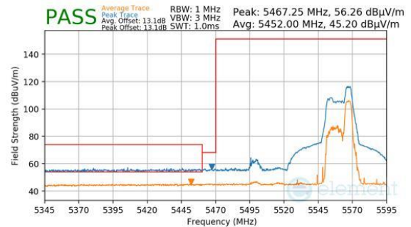
Plot 7-543. Antenna WF8 (Peak & Average, RU52, Index 44, Ch.110, MCS11)
