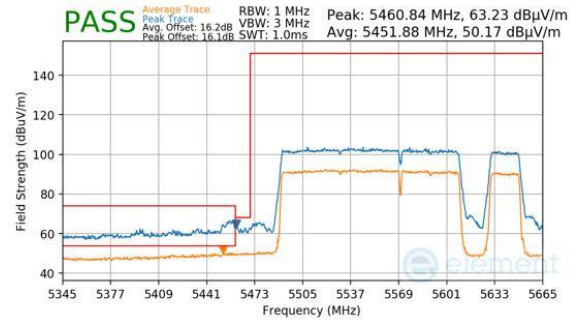
Plot 7-478. Antenna WF5B (Peak & Average, RU996+484+242, Index 98 (H), Ch.114 (FCC ONLY), MCS11)
