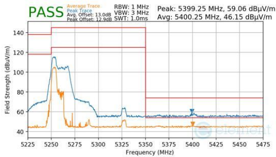
Plot 7-564. Antenna WF8 (Peak & Average, RU52, Index 37, Ch.58, MCS11)
