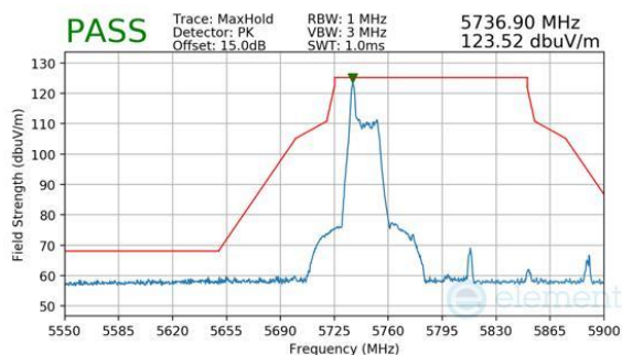
Plot 7-560. Antenna WF8 (Peak, RU26, Index 0, Ch.155, MCS11)
