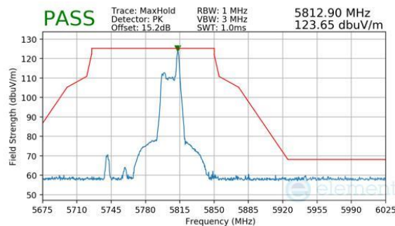
Plot 7-537. Antenna WF8 (Peak, RU26, Index 17, Ch.159, MCS11)
