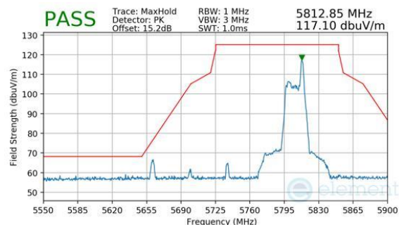
Plot 7-561. Antenna WF8 (Peak, RU26, Index 36, Ch.155, MCS11)
