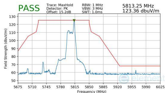
Plot 7-563. Antenna WF8 (Peak, RU26, Index 36, Ch.155, MCS11)
