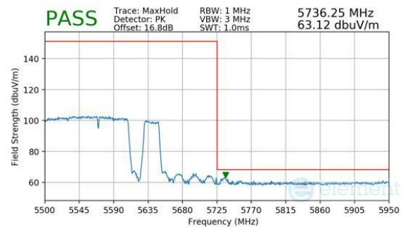
Plot 7-486. Antenna WF5B (Peak, RU996+484+242, Index 98 (H), Ch.114 (FCC ONLY), MCS11)
