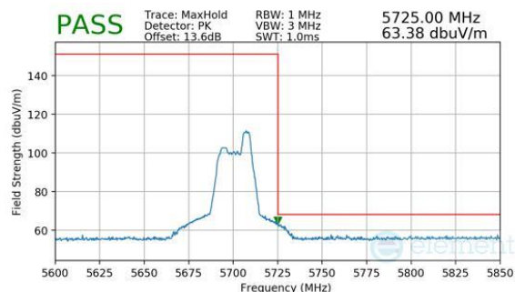
Plot 7-504. Antenna WF8 (Peak, RU52, Index 40, Ch.140, MCS11)
