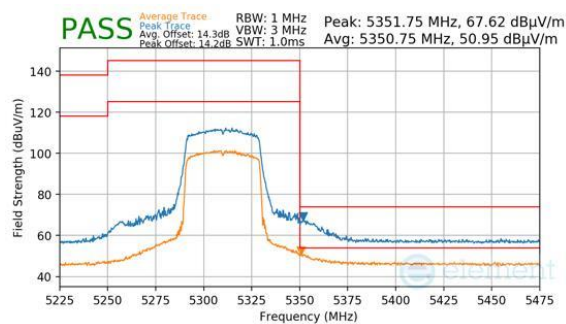
Plot 7-549. Antenna WF8 (Peak & Average, RU484, Index 65, Ch.62, MCS11)
