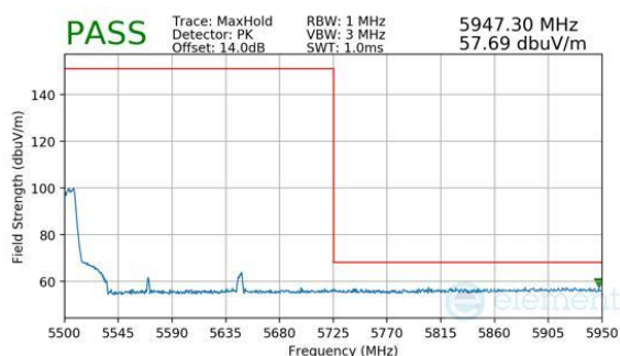
Plot 7-449. Antenna WF5B (Peak, RU52, Index 37, Ch.114 (FCC ONLY), MCS11)
