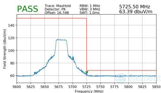
Plot 7-528. Antenna WF8 (Peak, RU242, Index 61, Ch.136, MCS11)
