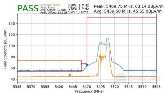
Plot 7-502. Antenna WF8 (Peak & Average, RU52, Index 40, Ch.100, MCS11)
