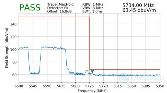
Plot 7-462. Antenna WF5B (Peak, RU996+484, Index 95 (L), Ch.114 (FCC ONLY), MCS11)
