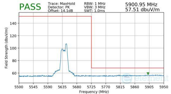
Plot 7-569. Antenna WF8 (Peak, RU52, Index 52, Ch.122 (FCC ONLY), MCS11)
