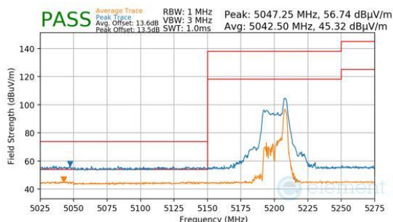
Plot 7-533. Antenna WF8 (Peak & Average, RU26, Index 17, Ch.38, MCS11)
