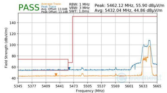
Plot 7-448. Antenna WF5B (Peak & Average, RU52, Index 52 (H), Ch.114 (FCC ONLY), MCS11)
