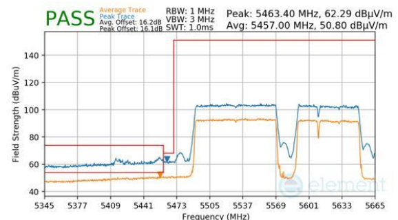
Plot 7-474. Antenna WF5B (Peak & Average, RU996+484+242, Index 96 (H), Ch.114 (FCC ONLY), MCS11)
