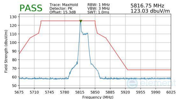
Plot 7-497. Antenna WF8 (Peak, RU26, Index 0, Ch.165, MCS11)
