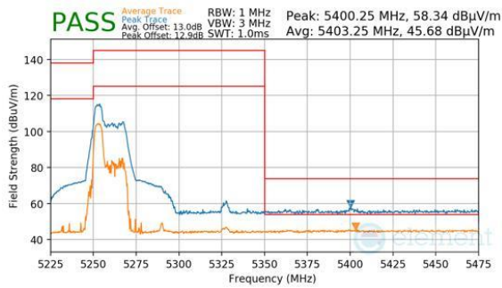
Plot 7-402. Antenna WF5B (Peak & Average, RU52, Index 37, Ch.58, MCS11)
