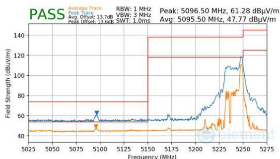
Plot 7-559. Antenna WF8 (Peak & Average, RU26, Index 36, Ch.42, MCS11)
