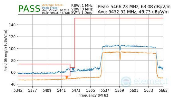
Plot 7-455. Antenna WF5B (Peak & Average, RU996+484, Index 94 (L), Ch.114 (FCC ONLY), MCS11)
