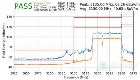
Plot 7-570. Antenna WF8 (Peak & Average, RU484+242, Index 90, Ch.42, MCS11)
