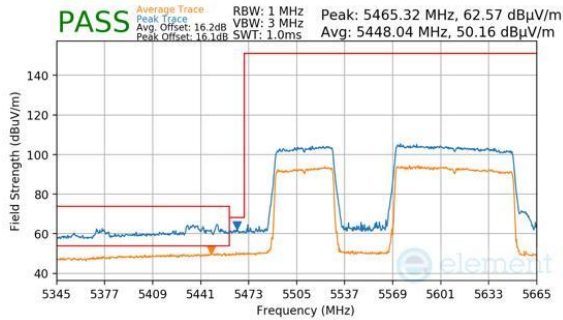
Plot 7-457. Antenna WF5B (Peak & Average, RU996+484, Index 95 (L), Ch.114 (FCC ONLY), MCS11)
