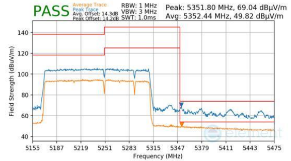
Plot 7-472. Antenna WF5B (Peak & Average, RU996+484+242, Index 99, Ch.50, MCS11)
