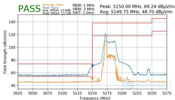
Plot 7-532. Antenna WF8 (Peak & Average, RU26, Index 0, Ch.38, MCS11)
