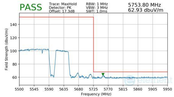
Plot 7-484. Antenna WF5B (Peak, RU996+484+242, Index 97 (H), Ch.114 (FCC ONLY), MCS11)
