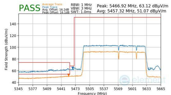
Plot 7-480. Antenna WF5B (Peak & Average, RU996+484+242, Index 99 (H), Ch.114 (FCC ONLY), MCS11)
