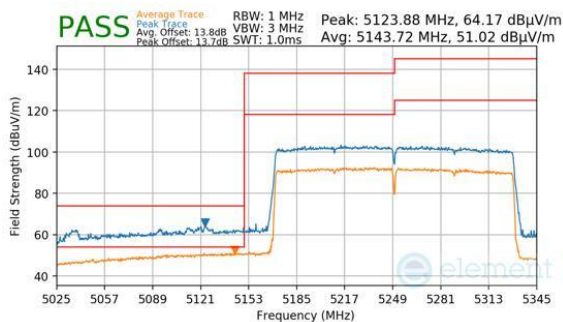
Plot 7-489. Antenna WF5B (Peak & Average, RU996X2, Index 68, Ch.50, MCS11)
