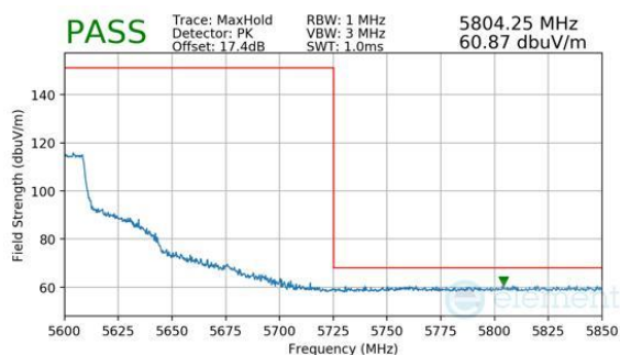
Plot 7-553. Antenna WF8 (Peak, RU484, Index 65, Ch.118 (FCC ONLY), MCS11)
