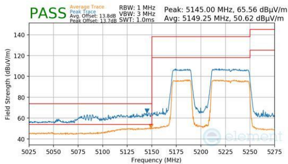
Plot 7-571. Antenna WF8 (Peak & Average, RU484+242, Index 91, Ch.42, MCS11)
