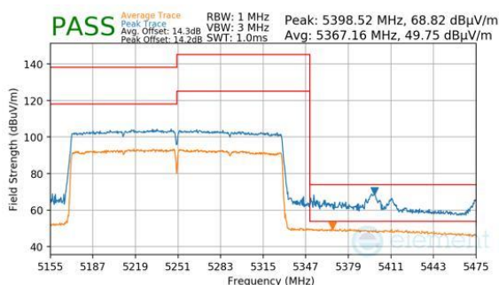
Plot 7-490. Antenna WF5B (Peak & Average, RU996X2, Index 68, Ch.50, MCS11)
