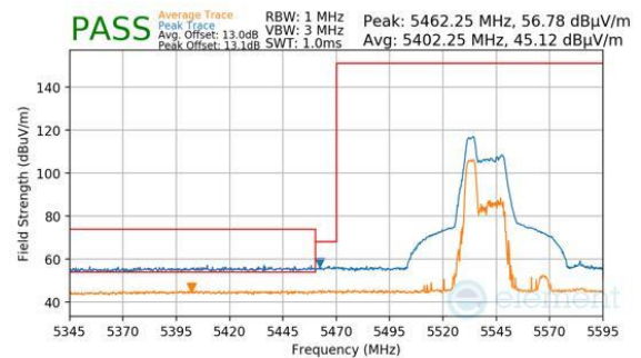
Plot 7-542. Antenna WF8 (Peak & Average, RU52, Index 37, Ch.110, MCS11)
