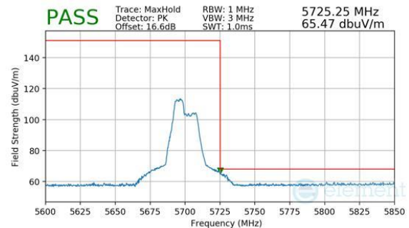
Plot 7-515. Antenna WF8 (Peak, RU52+26, Index 70, Ch.140, MCS11)
