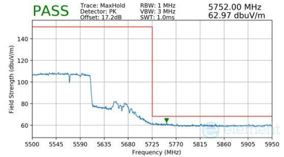
Plot 7-461. Antenna WF5B (Peak, RU996+484, Index 95 (H), Ch.114 (FCC ONLY), MCS11)
