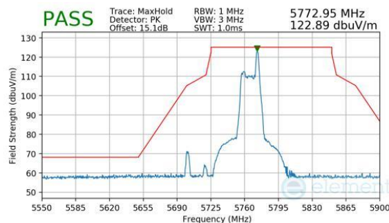
Plot 7-535. Antenna WF8 (Peak, RU26, Index 17, Ch.151, MCS11)
