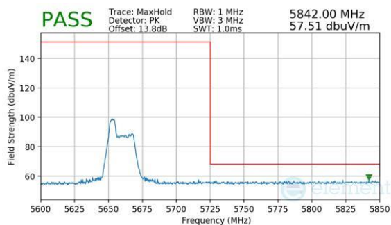
Plot 7-544. Antenna WF8 (Peak, RU52, Index 37, Ch.134, MCS11)
