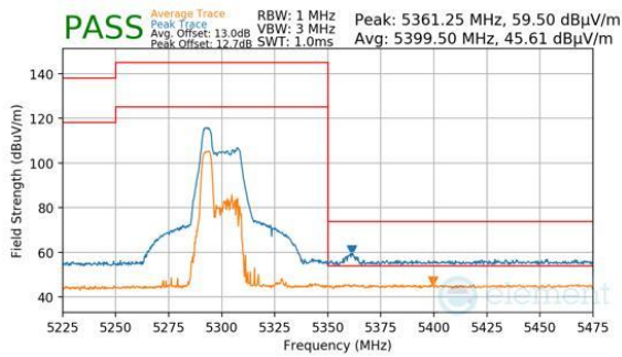
Plot 7-538. Antenna WF8 (Peak & Average, RU52, Index 37, Ch.62, MCS11)
