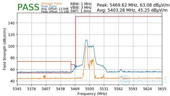
Plot 7-566. Antenna WF8 (Peak & Average, RU52, Index 37, Ch.106, MCS11)
