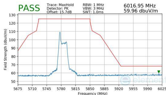
Plot 7-536. Antenna WF8 (Peak, RU26, Index 0, Ch.159, MCS11)
