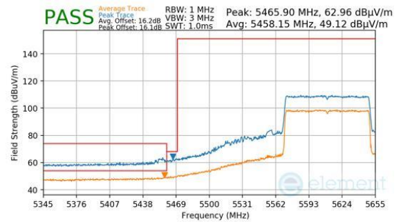
Plot 7-439. Antenna WF5B (Peak & Average, RU996, Index 67, Ch.122 (FCC ONLY), MCS11)
