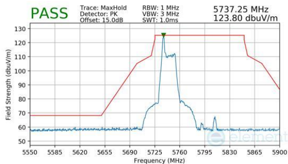
Plot 7-534. Antenna WF8 (Peak, RU26, Index 0, Ch.151, MCS11)
