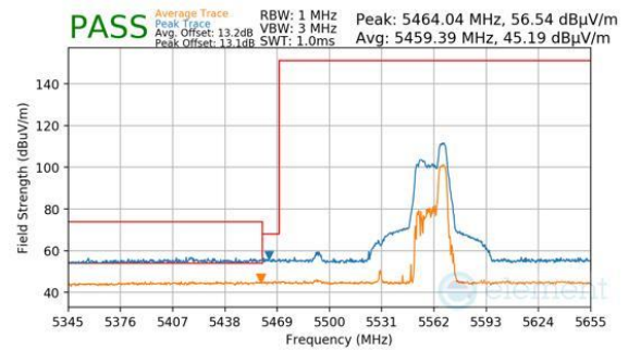
Plot 7-405. Antenna WF5B (Peak & Average, RU52, Index 52, Ch.106, MCS11)
