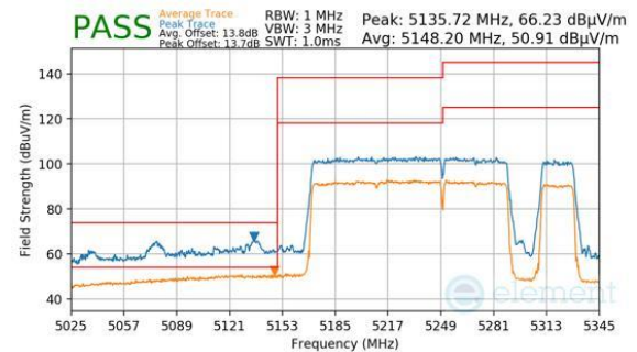
Plot 7-467. Antenna WF5B (Peak & Average, RU996+484+242, Index 98, Ch.50, MCS11)
