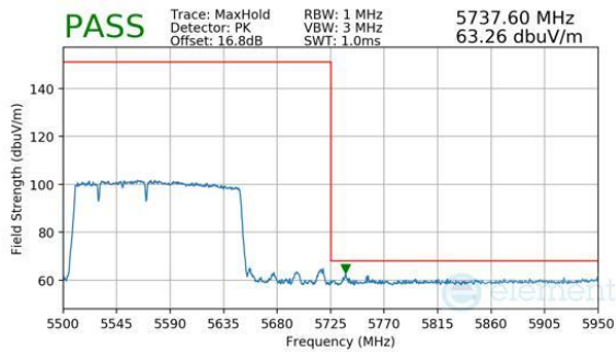
Plot 7-482. Antenna WF5B (Peak, RU996+484+242, Index 96 (L), Ch.114 (FCC ONLY), MCS11)
