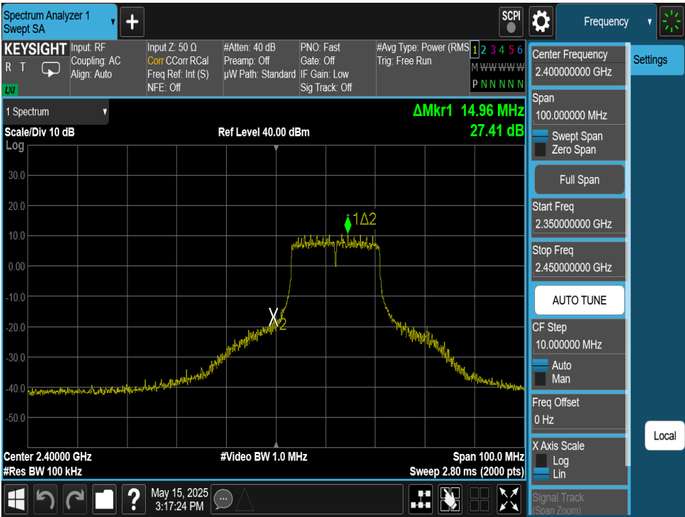
Plot 7-64. Band Edge Plot Antenna WF8 (802.11n (2.4GHz) – Ch. 1)
