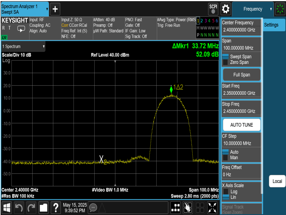
Plot 7-94. Band Edge Plot Antenna WF7 (802.11b – Ch. 4)
