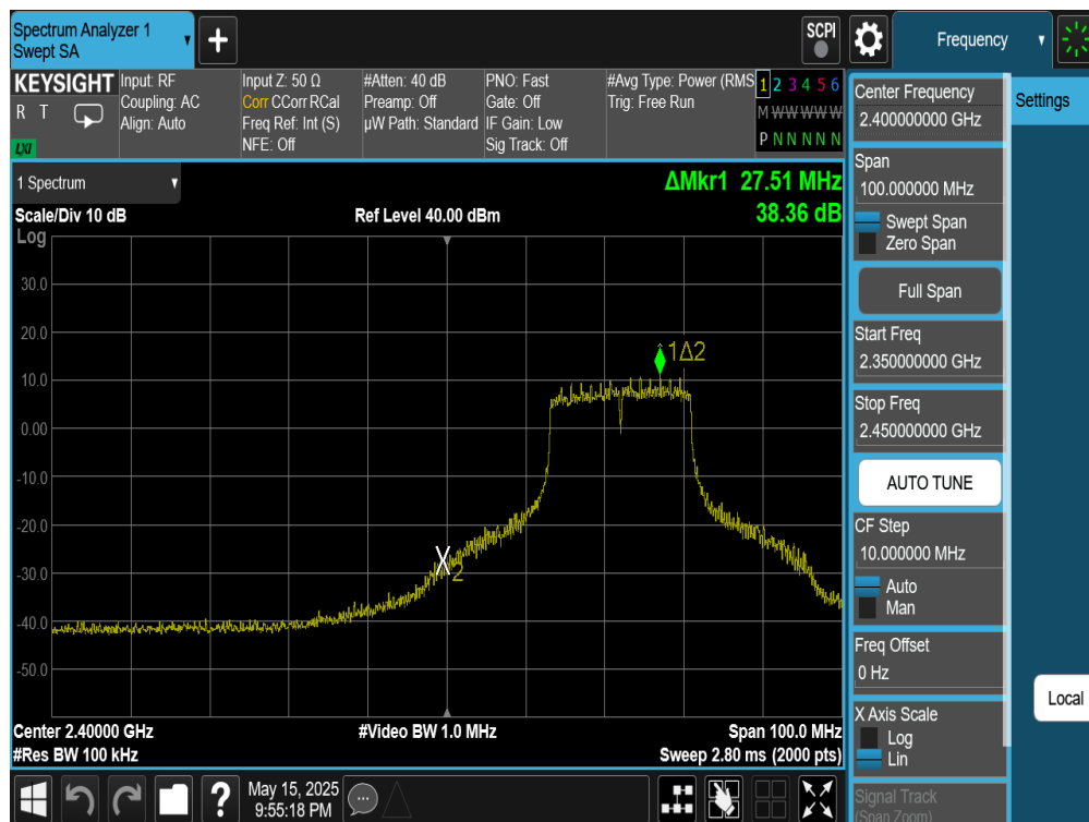
Plot 7-103. Band Edge Plot Antenna WF7 (802.11g – Ch. 3)
