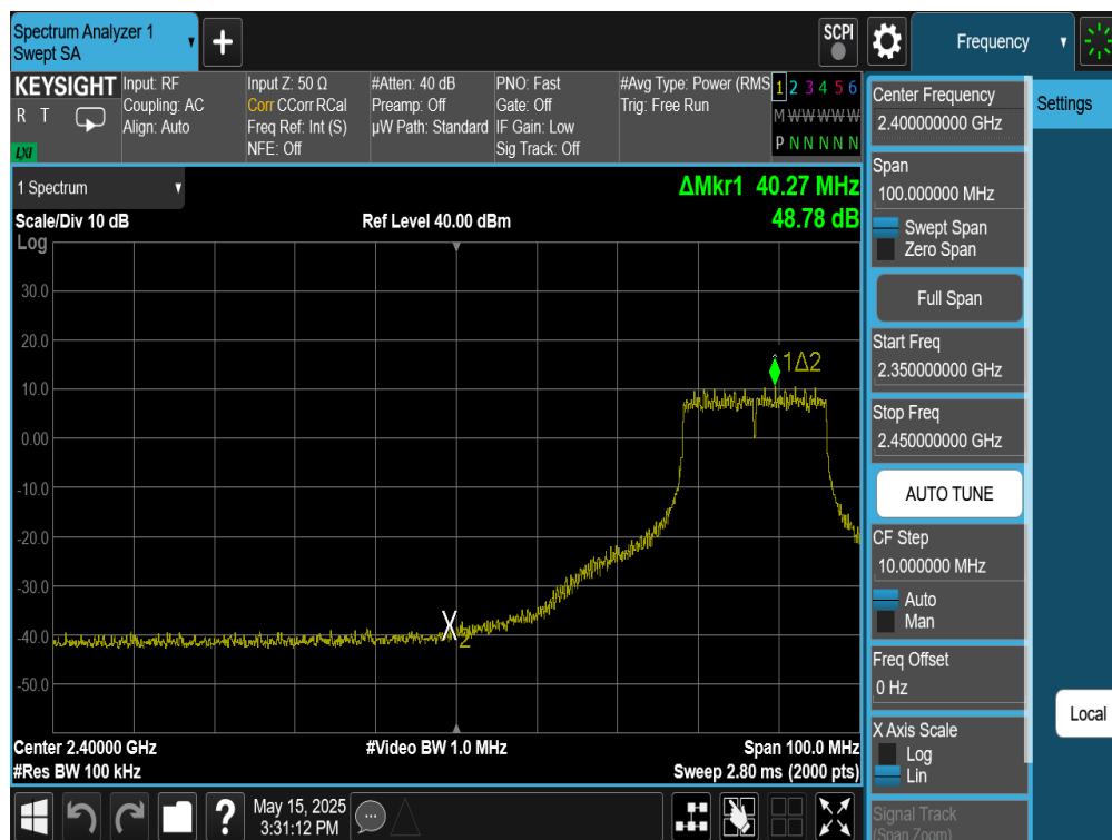
Plot 7-69. Band Edge Plot Antenna WF8 (802.11n (2.4GHz) – Ch. 6)
