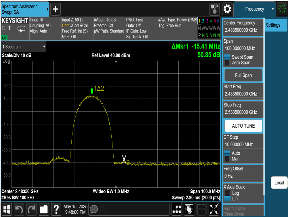
Plot 7-100. Band Edge Plot Antenna WF7 (802.11b – Ch. 13)
