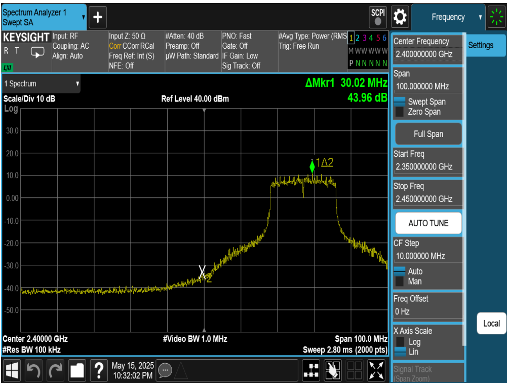
Plot 7-117. Band Edge Plot Antenna WF7 (802.11n (2.4GHz) – Ch. 4)
