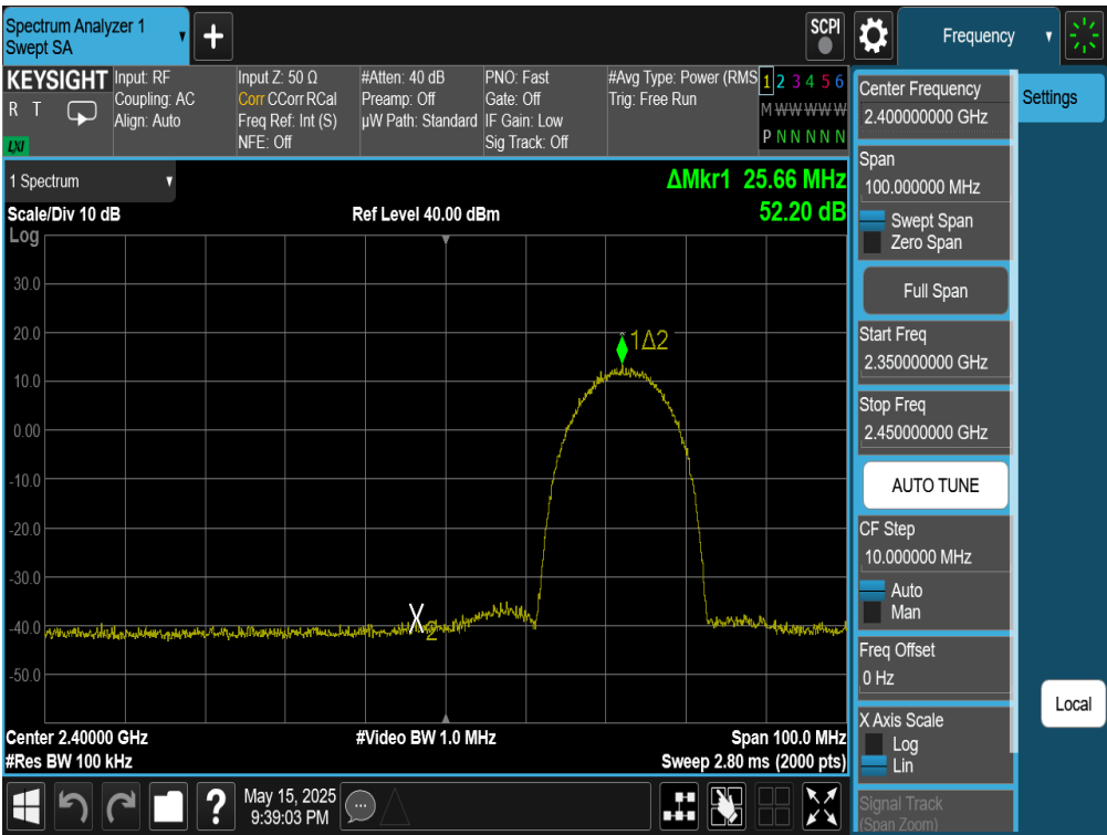
Plot 7-93. Band Edge Plot Antenna WF7 (802.11b – Ch. 3)
