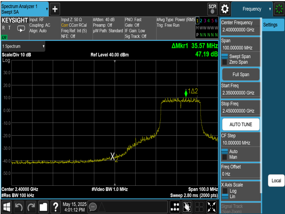
Plot 7-81. Band Edge Plot Antenna WF8 (802.11be (SU - 2.4GHz) – Ch. 5)
