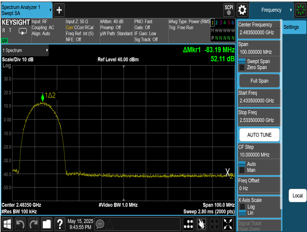
Plot 7-95. Band Edge Plot Antenna WF7 (802.11b – Ch. 8)
