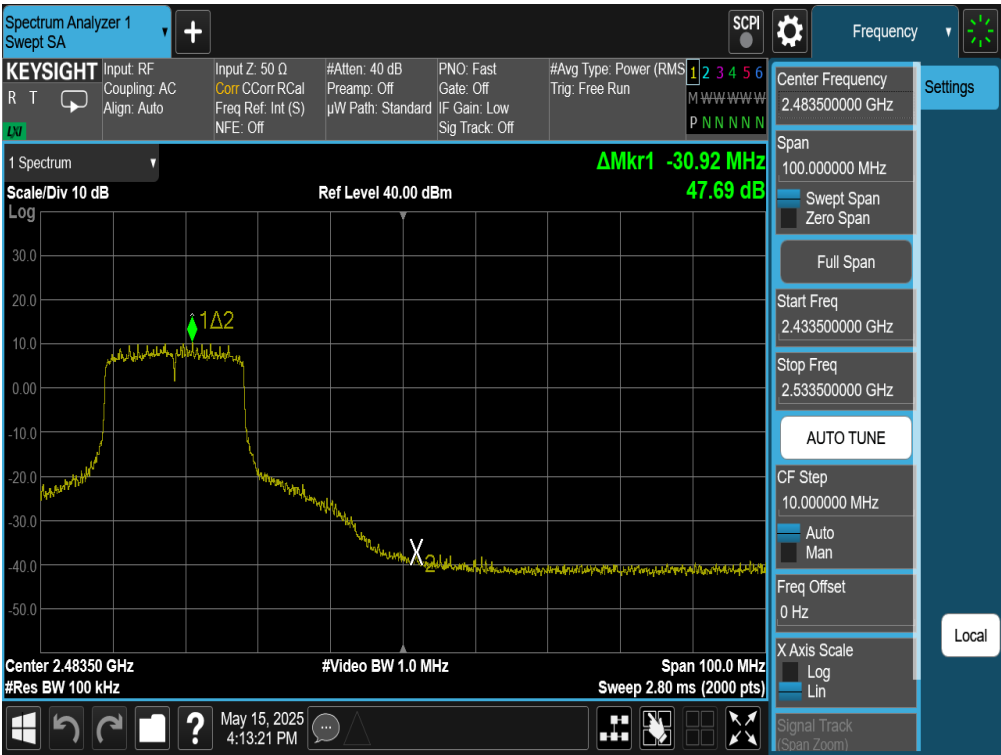
Plot 7-86. Band Edge Plot Antenna WF8 (802.11be (SU - 2.4GHz) – Ch. 9)
