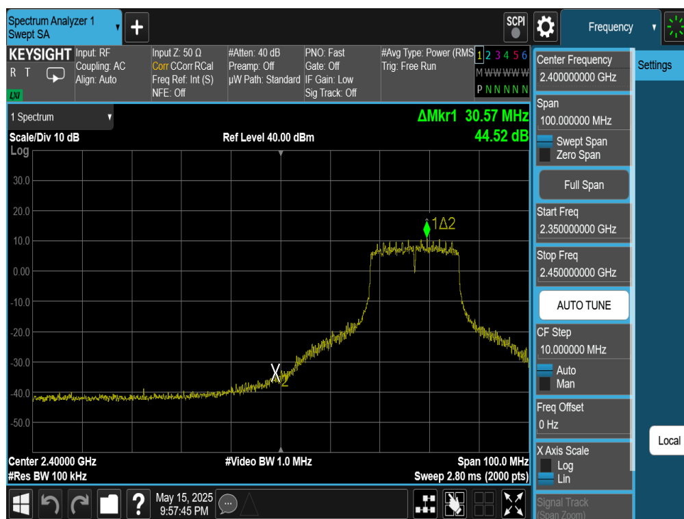
Plot 7-104. Band Edge Plot Antenna WF7 (802.11g – Ch. 4)
