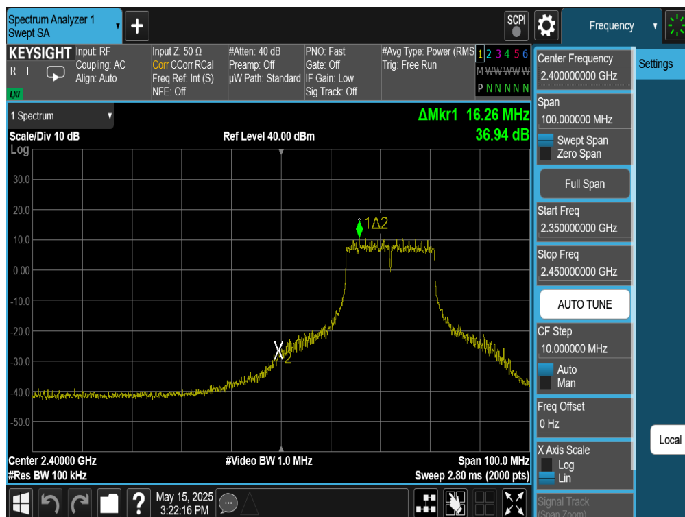
Plot 7-66. Band Edge Plot Antenna WF8 (802.11n (2.4GHz) – Ch. 3)
