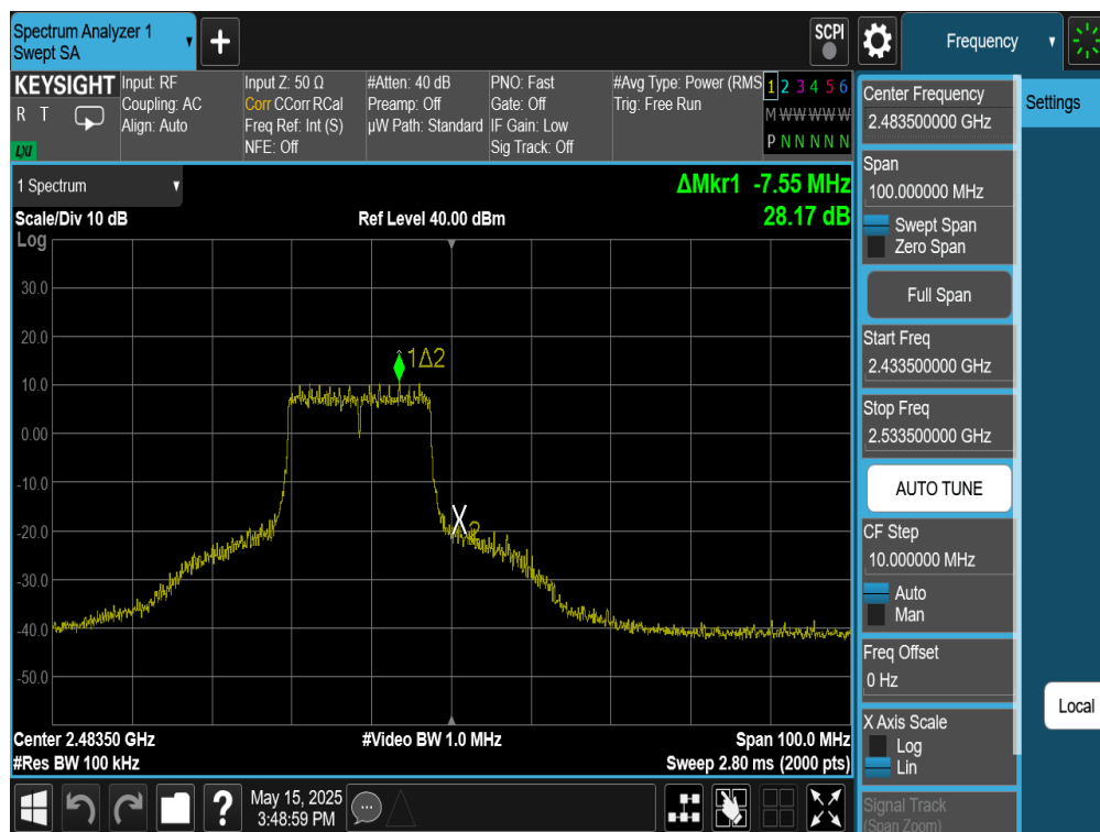
Plot 7-76. Band Edge Plot Antenna WF8 (802.11n (2.4GHz) – Ch. 13)
