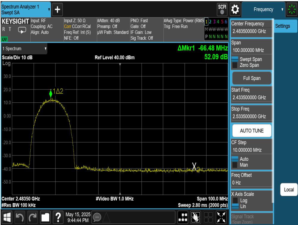
Plot 7-96. Band Edge Plot Antenna WF7 (802.11b – Ch. 9)
