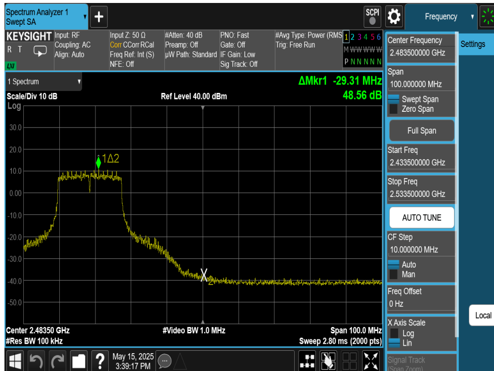
Plot 7-72. Band Edge Plot Antenna WF8 (802.11n (2.4GHz) – Ch. 9)
