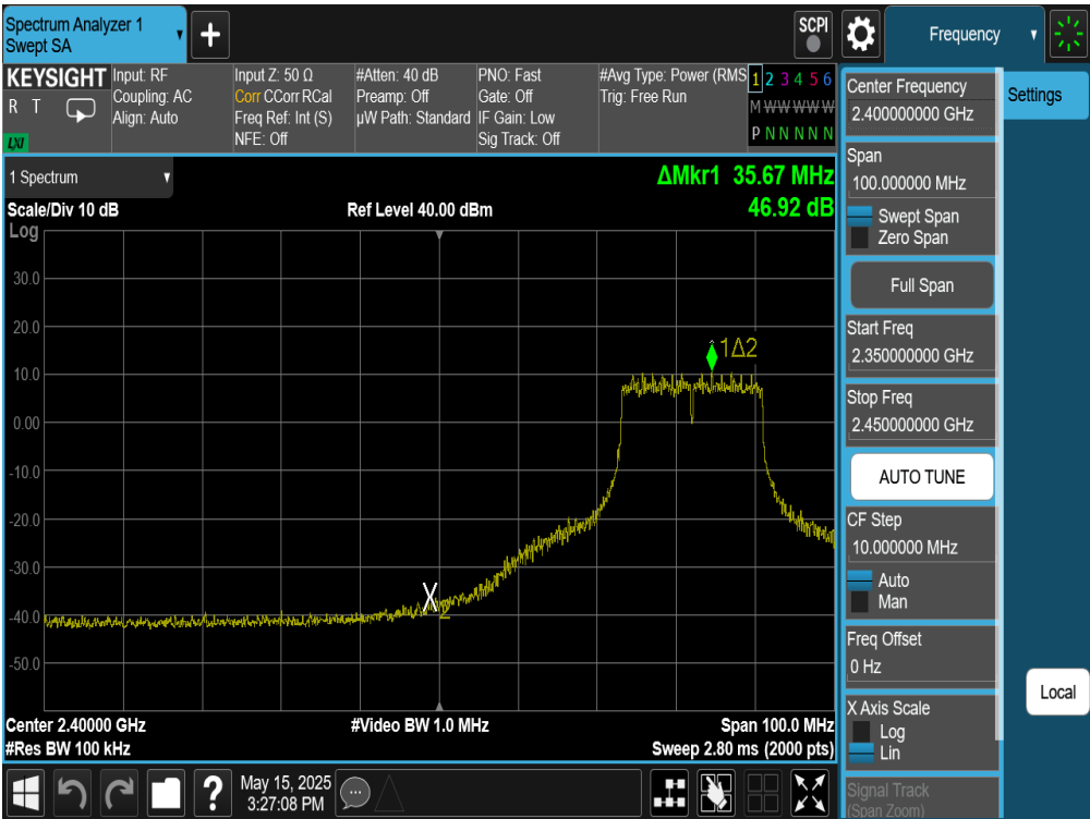
Plot 7-68. Band Edge Plot Antenna WF8 (802.11n (2.4GHz) – Ch. 5)
