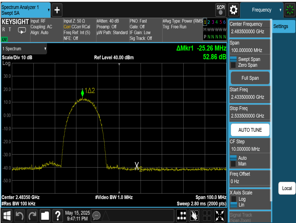
Plot 7-99. Band Edge Plot Antenna WF7 (802.11b – Ch. 12)
