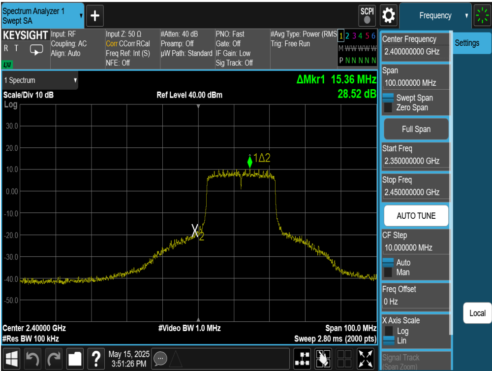
Plot 7-77. Band Edge Plot Antenna WF8 (802.11be (SU - 2.4GHz) – Ch. 1)
