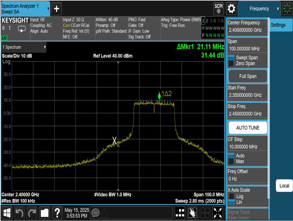
Plot 7-78. Band Edge Plot Antenna WF8 (802.11be (SU - 2.4GHz) – Ch. 2)
