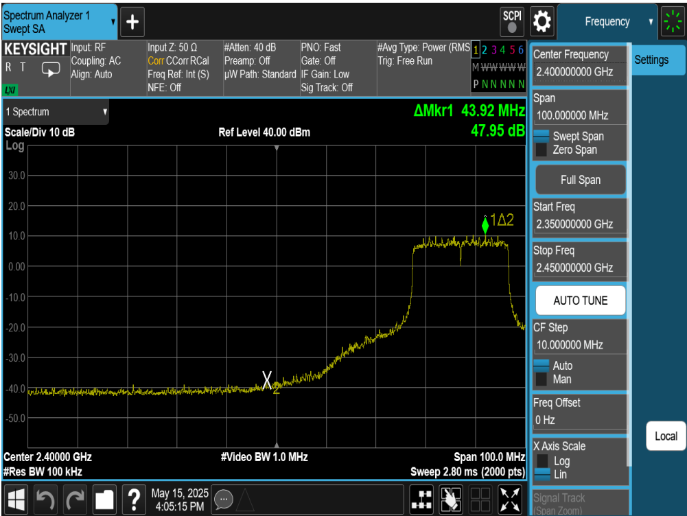
Plot 7-82. Band Edge Plot Antenna WF8 (802.11be (SU - 2.4GHz) – Ch. 6)
