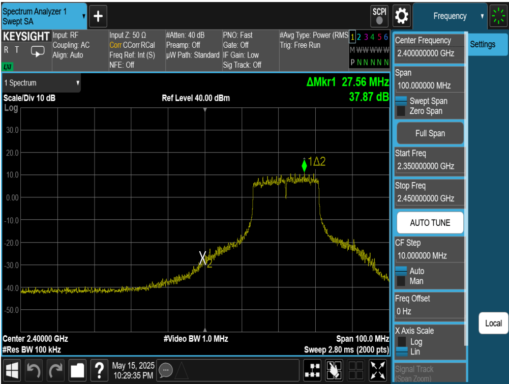
Plot 7-116. Band Edge Plot Antenna WF7 (802.11n (2.4GHz) – Ch. 3)
