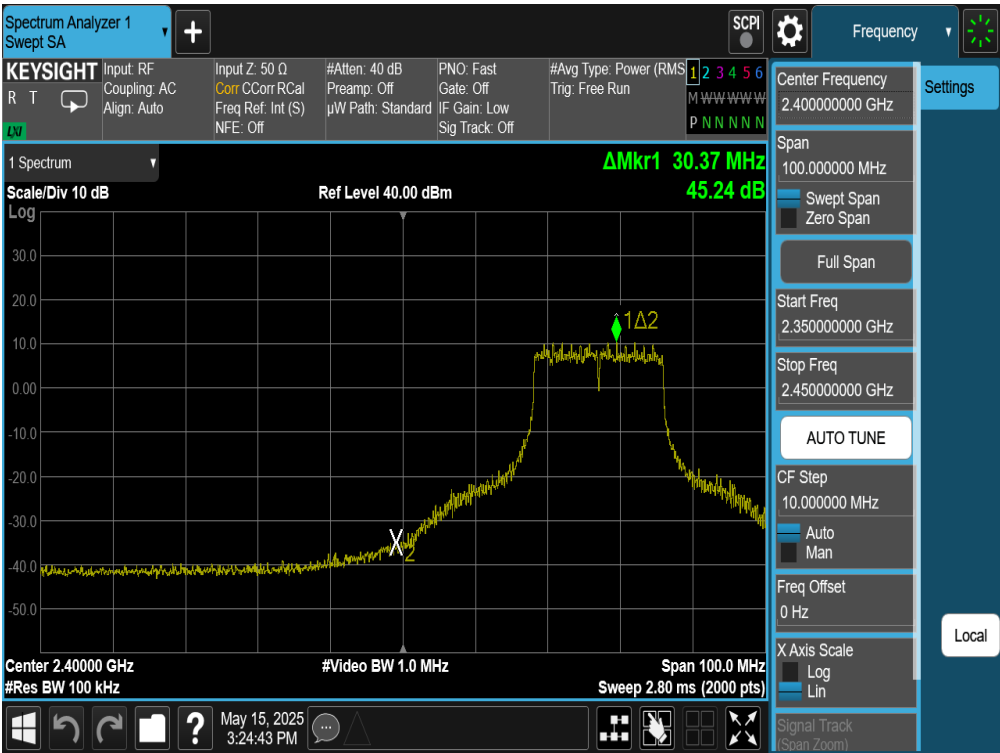
Plot 7-67. Band Edge Plot Antenna WF8 (802.11n (2.4GHz) – Ch. 4)
