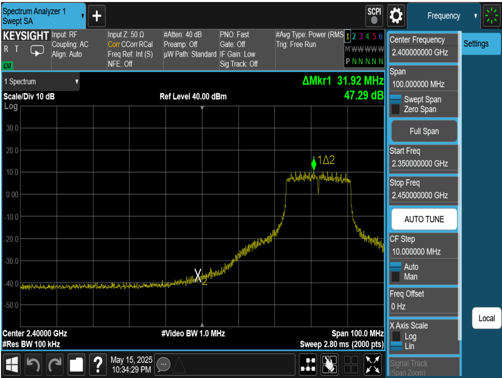
Plot 7-118. Band Edge Plot Antenna WF7 (802.11n (2.4GHz) – Ch. 5)
