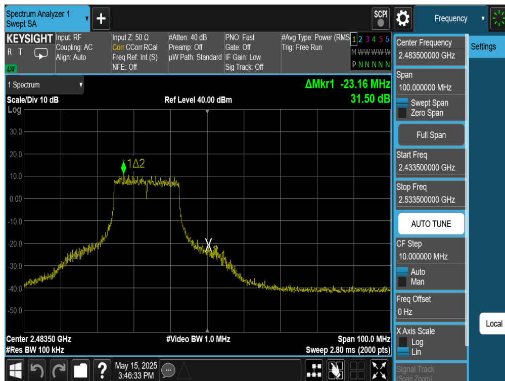
Plot 7-75. Band Edge Plot Antenna WF8 (802.11n (2.4GHz) – Ch. 12)
