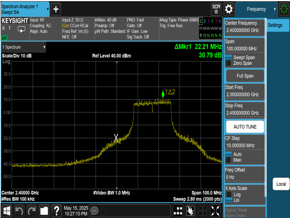
Plot 7-115. Band Edge Plot Antenna WF7 (802.11n (2.4GHz) – Ch. 2)
