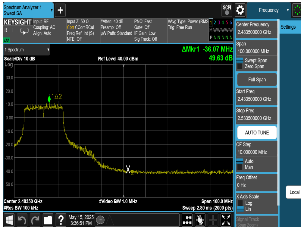
Plot 7-71. Band Edge Plot Antenna WF8 (802.11n (2.4GHz) – Ch. 8)
