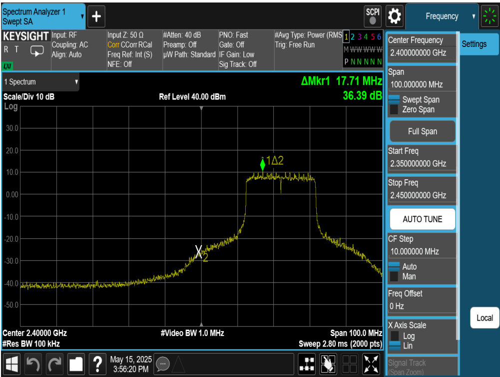
Plot 7-79. Band Edge Plot Antenna WF8 (802.11be (SU - 2.4GHz) – Ch. 3)
