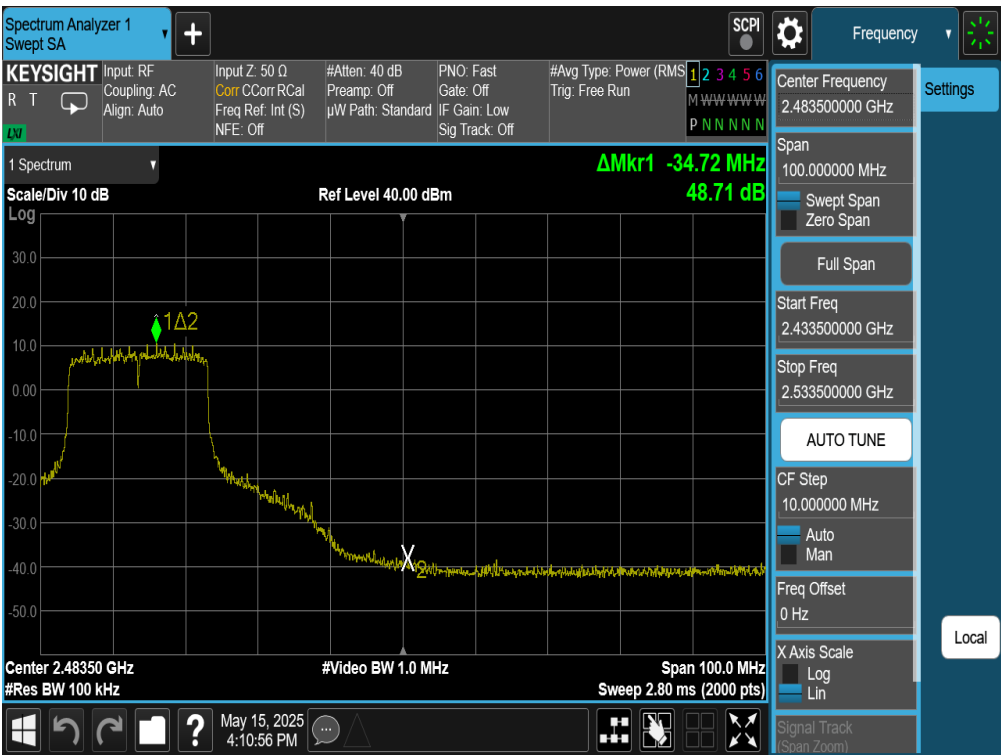
Plot 7-85. Band Edge Plot Antenna WF8 (802.11be (SU - 2.4GHz) – Ch. 8)
