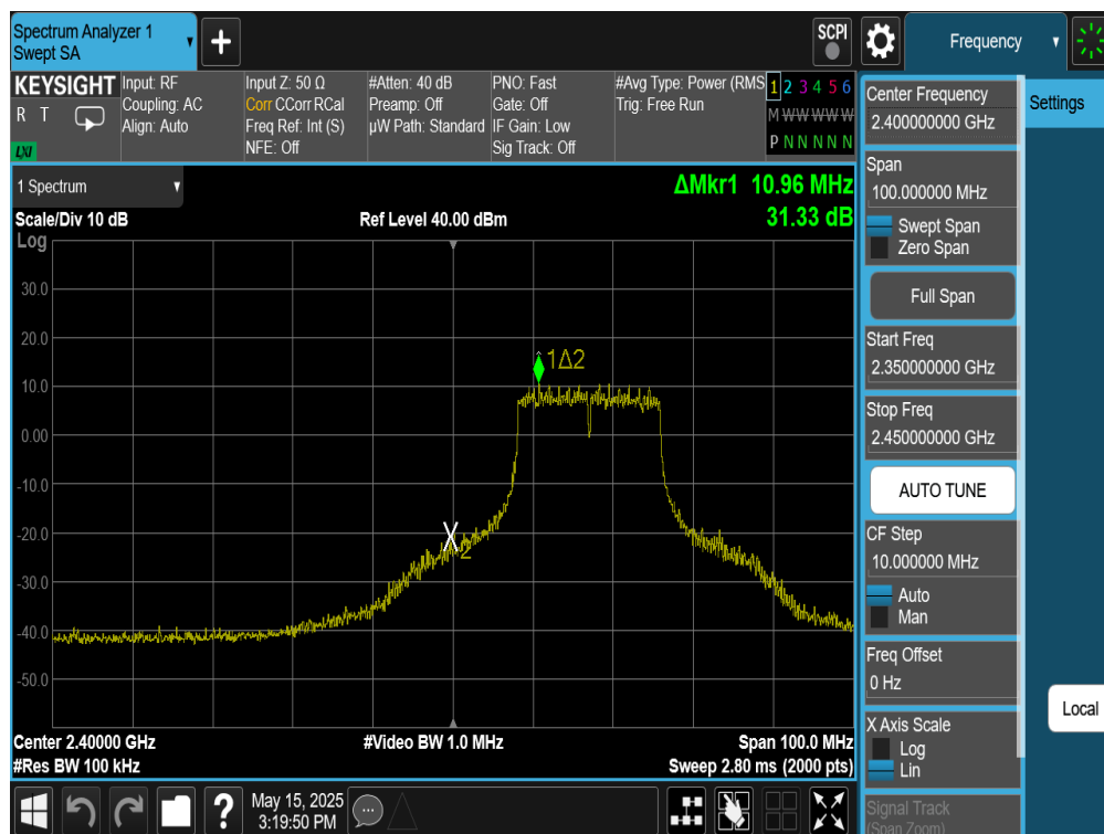
Plot 7-65. Band Edge Plot Antenna WF8 (802.11n (2.4GHz) – Ch. 2)
