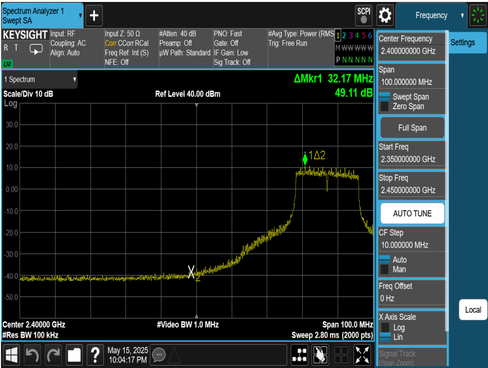
Plot 7-106. Band Edge Plot Antenna WF7 (802.11g – Ch. 6)
