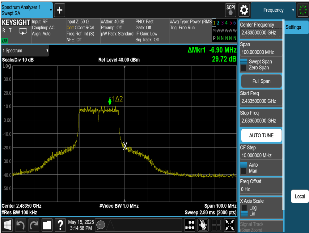
Plot 7-63. Band Edge Plot Antenna WF8 (802.11g – Ch. 13)
