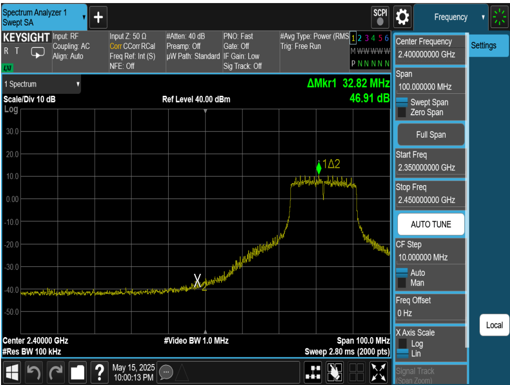
Plot 7-105. Band Edge Plot Antenna WF7 (802.11g – Ch. 5)
