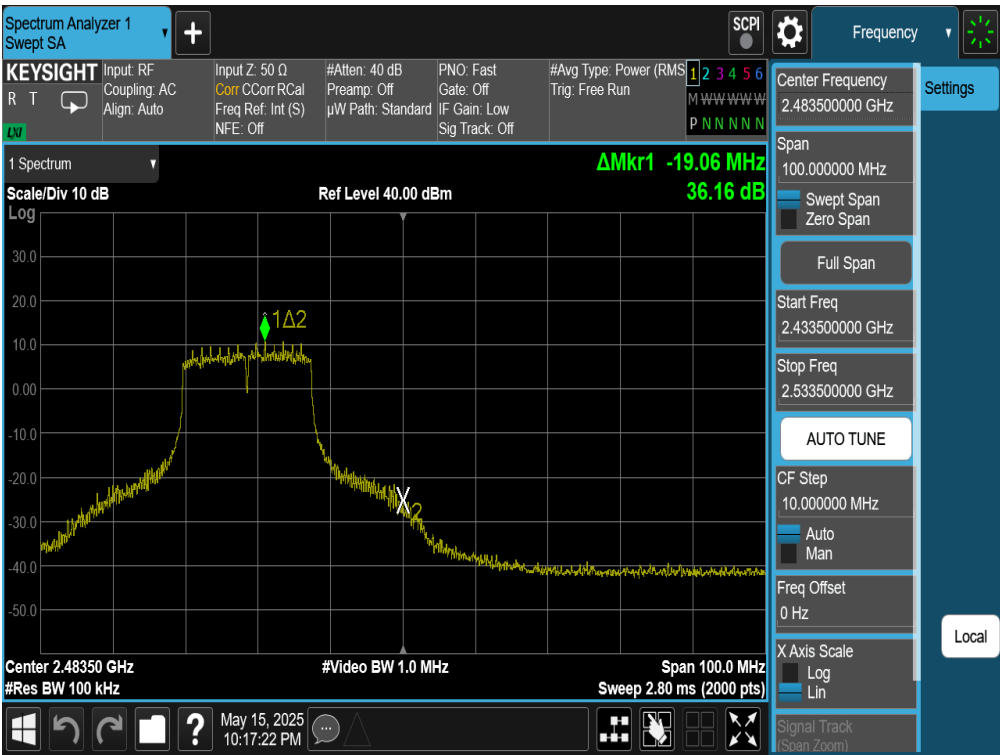
Plot 7-111. Band Edge Plot Antenna WF7 (802.11g – Ch. 11)
