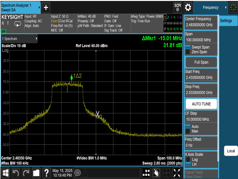
Plot 7-112. Band Edge Plot Antenna WF7 (802.11g – Ch. 12)
