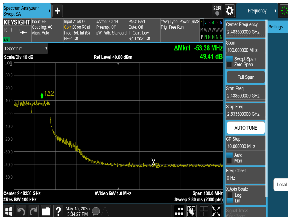
Plot 7-70. Band Edge Plot Antenna WF8 (802.11n (2.4GHz) – Ch. 7)
