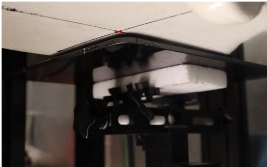
SAR Test Setup Photo 2: Body, Back Side at 5mm – Antenna WF8
