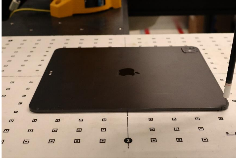
Near Field Power Density Test Setup Photo 20: Body, Back side at 9.22mm – WF7
