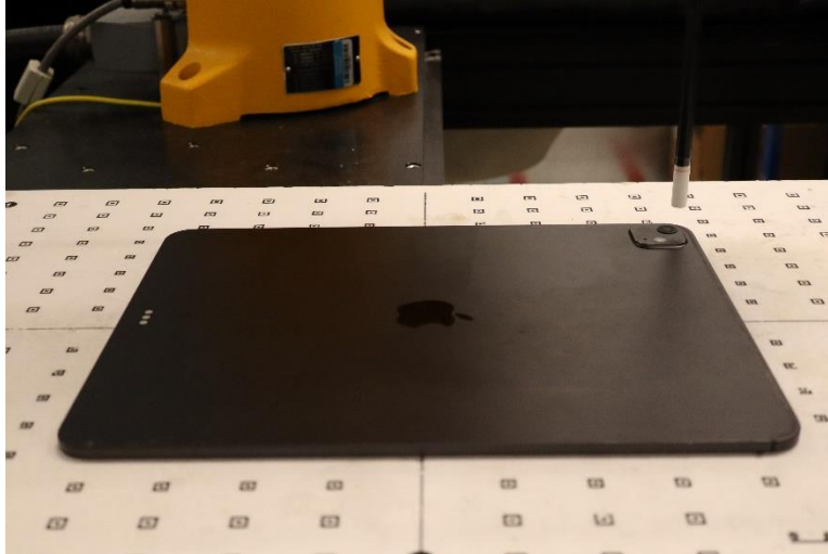
Near Field Power Density Test Setup Photo 24: Body, Back side at 9.57mm – WF8
