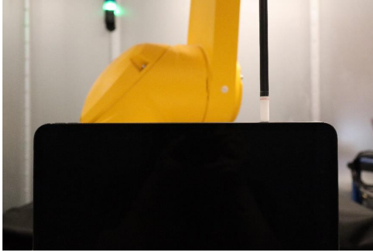
Near Field Power Density Test Setup Photo 16: Body, Right Edge at 2mm – WF5B
