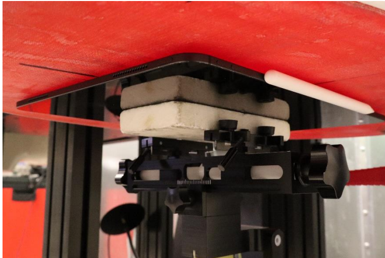
Wireless Power Transfer (wPT) Test Setup Photo 11: Body, Back Side at 5mm
