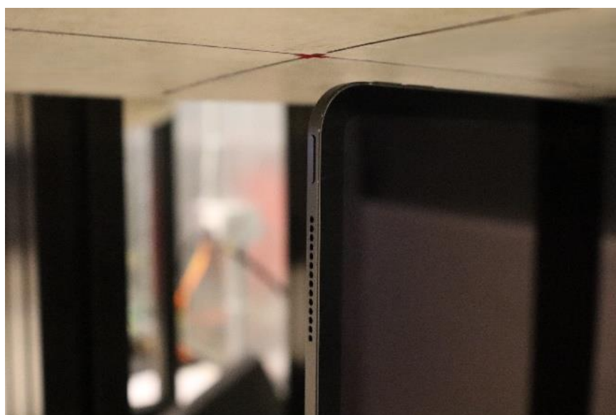
SAR Test Setup Photo 5: Body, Right Edge at 5mm – Antenna WF8/WF9/WF7
