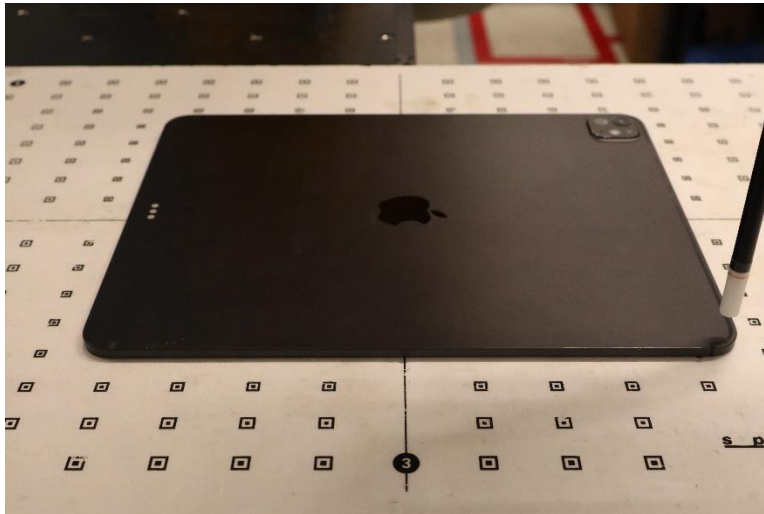
Near Field Power Density Test Setup Photo 21: Body, Back side at 9.34mm – WF7
