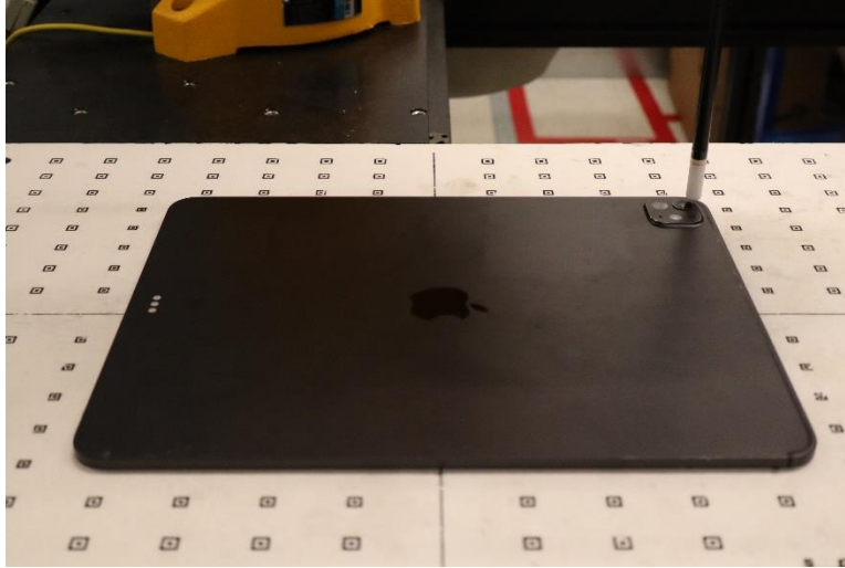
Near Field Power Density Test Setup Photo 22: Body, Back side at 2mm – WF8
