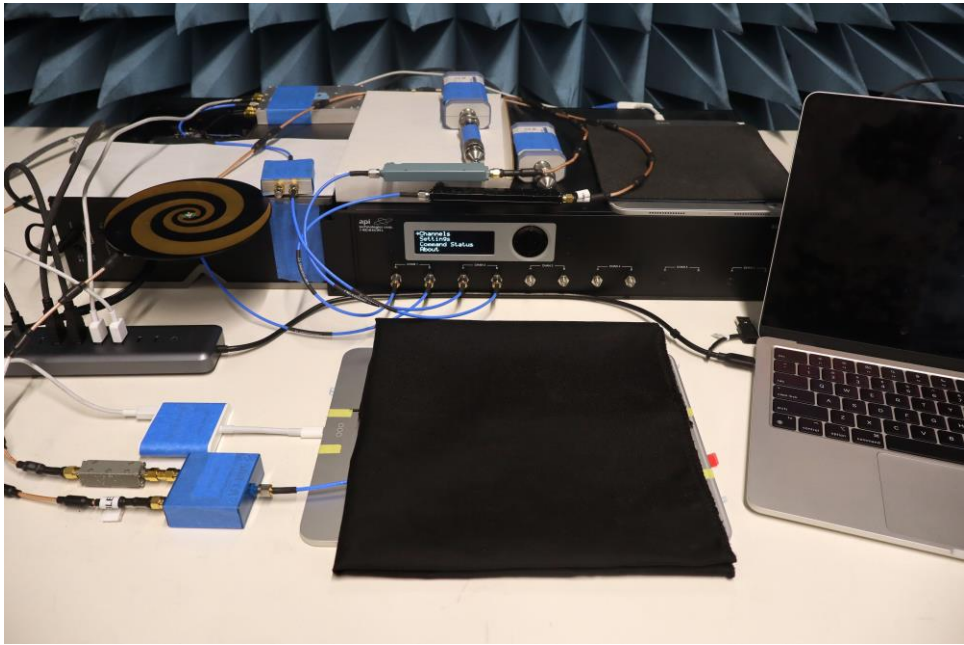
Test Setup Photo 3 – Conducted Test Setup (Figure 5-1c)
