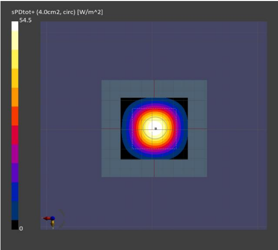
10 GHz System Verification
