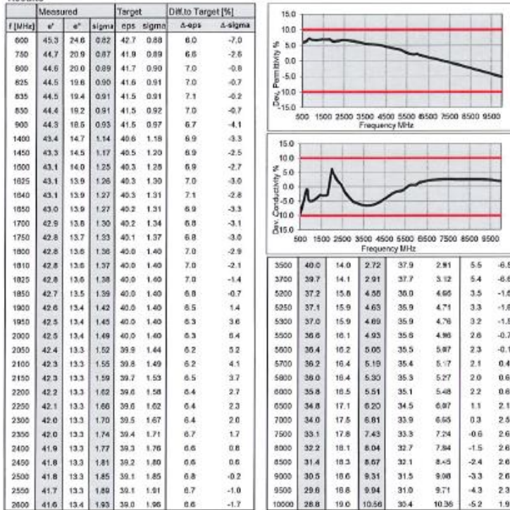
Figure D-2 600 – 10000 MHz Head Tissue Equivalent Matter
