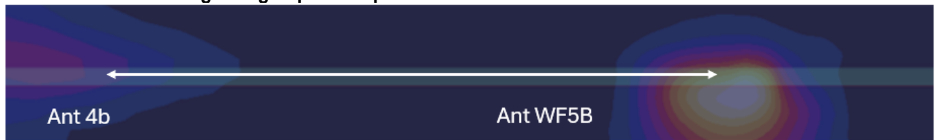
Figure F-22 Right Edge Spatial Separation for Antenna 4b and Antenna WF5B
