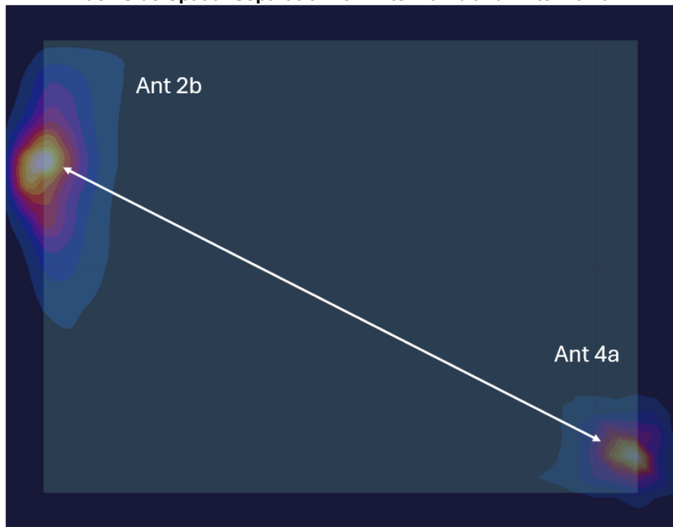
Figure F-8 Back Side Spatial Separation for Antenna 2b and Antenna 4a
