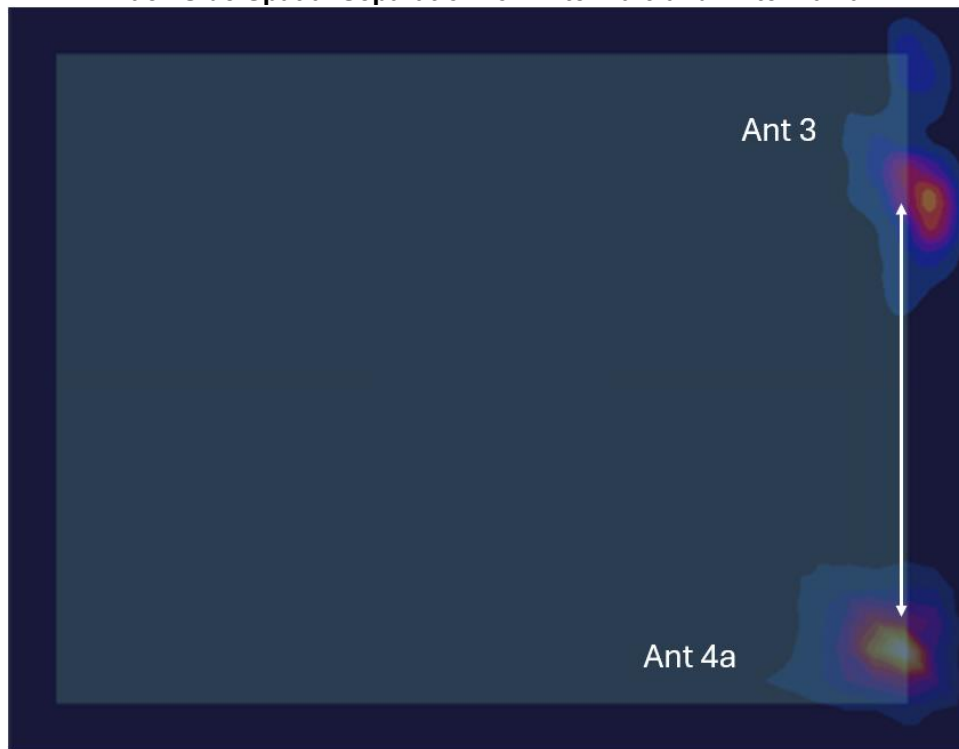
Figure F-10 Back Side Spatial Separation for Antenna 3 and Antenna 4a
