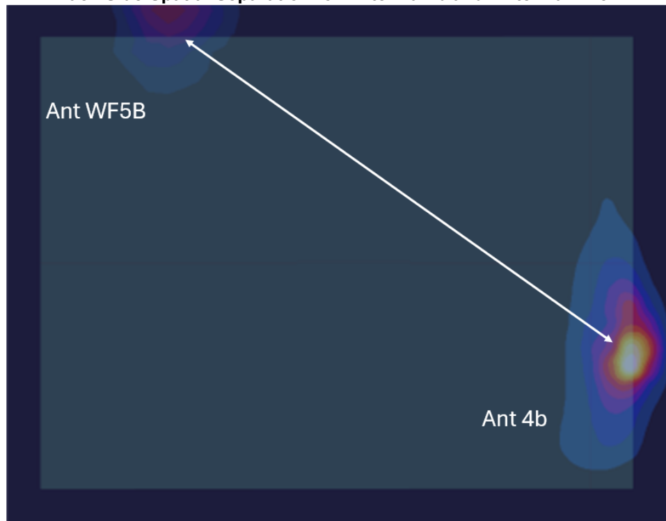
Figure F-13 Back Side Spatial Separation for Antenna 4b and Antenna WF5B
