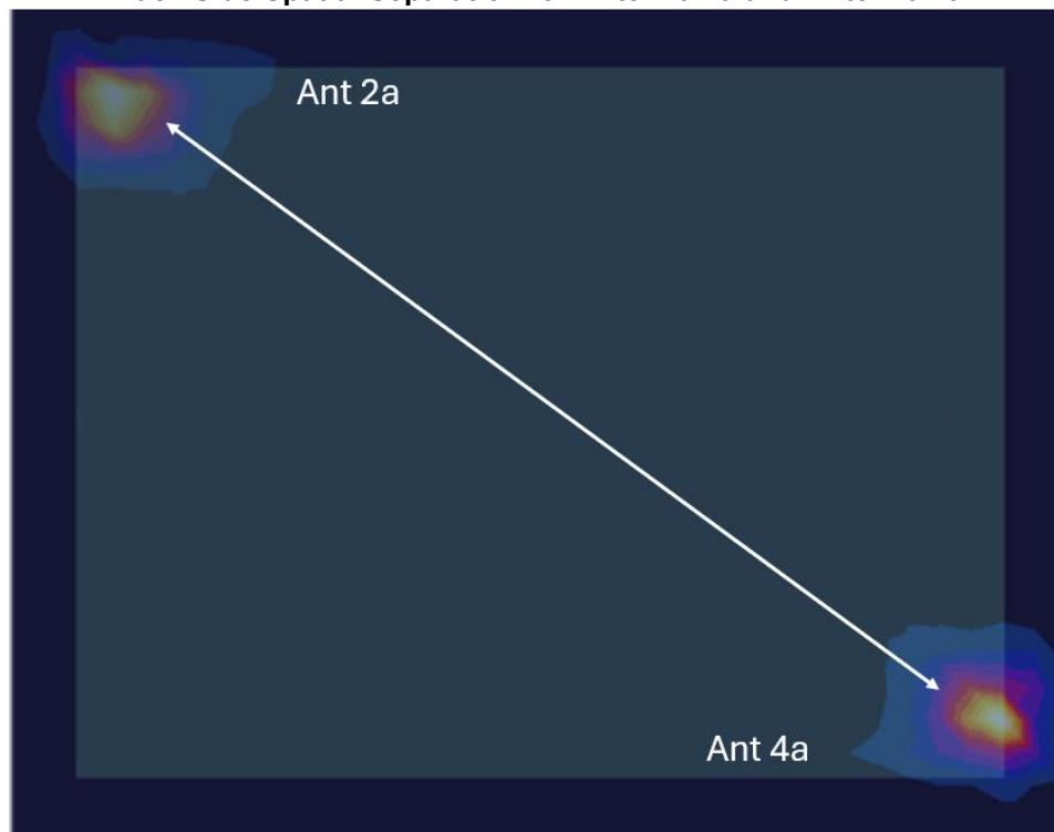
Figure F-5 Back Side Spatial Separation for Antenna 2a and Antenna 4a
