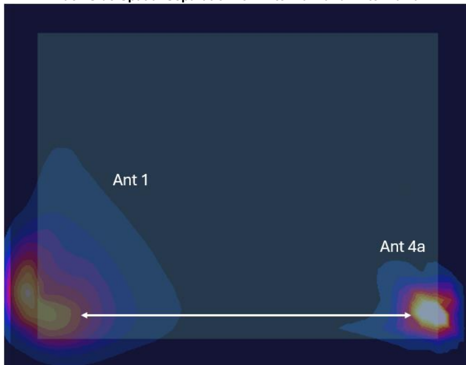
Figure F-2 Back Side Spatial Separation for Antenna 1 and Antenna 4a
