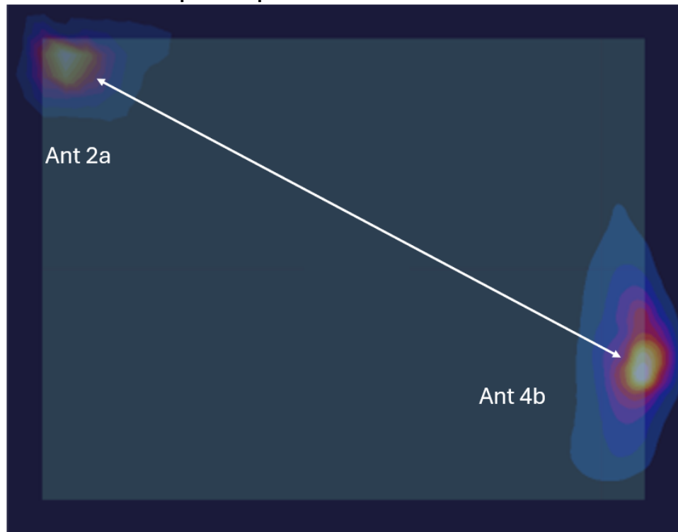
Figure F-6 Back Side Spatial Separation for Antenna 2a and Antenna 4b
