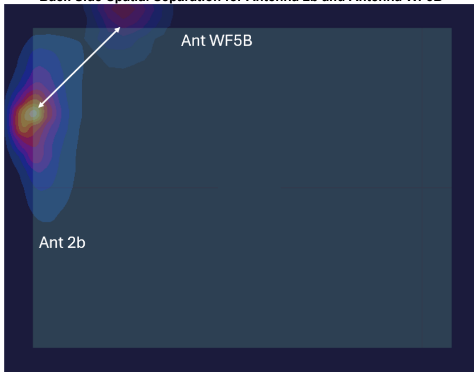
Figure F-9 Back Side Spatial Separation for Antenna 2b and Antenna WF5B
