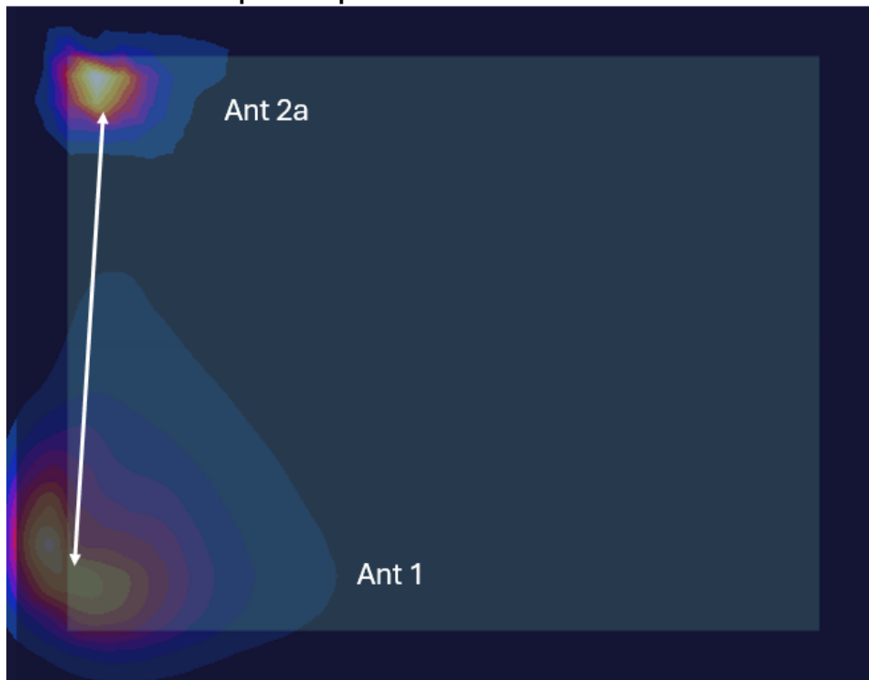
Figure F-1 Back Side Spatial Separation for Antenna 1 and Antenna 2a
