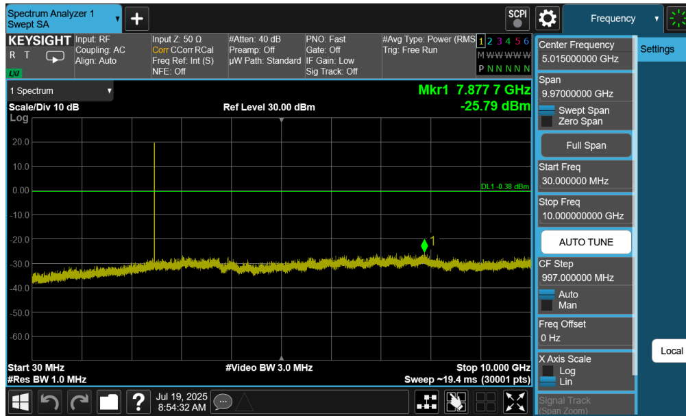
Plot 7-27. Conducted Spurious Antenna 4a (802.15.4, ePA – Ch. 25)
