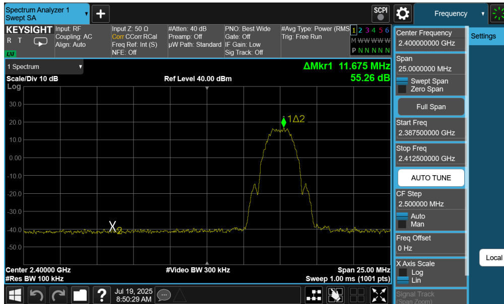
Plot 7-19. Band Edge Antenna 4a (802.15.4, ePA – Ch. 11)
