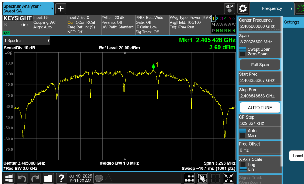
Plot 7-13. Power Spectral Density Antenna 2a (802.15.4, ePA – Ch. 11)
