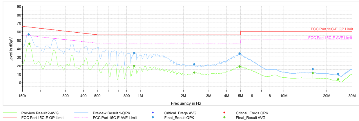
Plot 7-48. AC Line Conducted Emission with 802.15.4 Antenna 4a (L1, Ch.18 - ePA, with AC/DC Adaptor)
