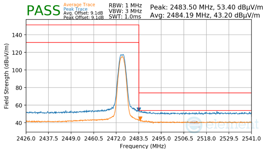
Plot 7-46. Radiated Restricted Upper Band Edge Measurement Antenna 2a
