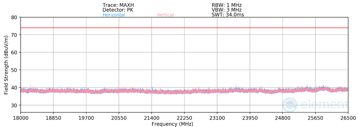
Plot 7-37. Radiated Spurious Emissions Above 18GHz Antenna 4a (802.15.4 ePA – Ch. 18)
