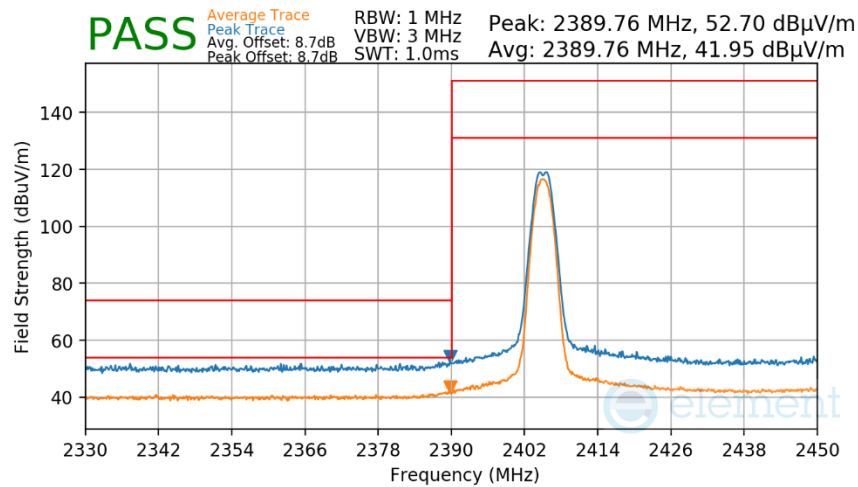
Plot 7-43. Radiated Restricted Lower Band Edge Measurement Antenna 4a
