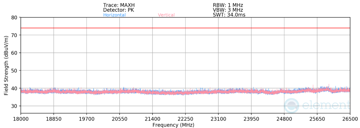
Plot 7-41. Radiated Spurious Emissions Above 18GHz Antenna 2a (802.15.4 ePA – Ch. 18)
