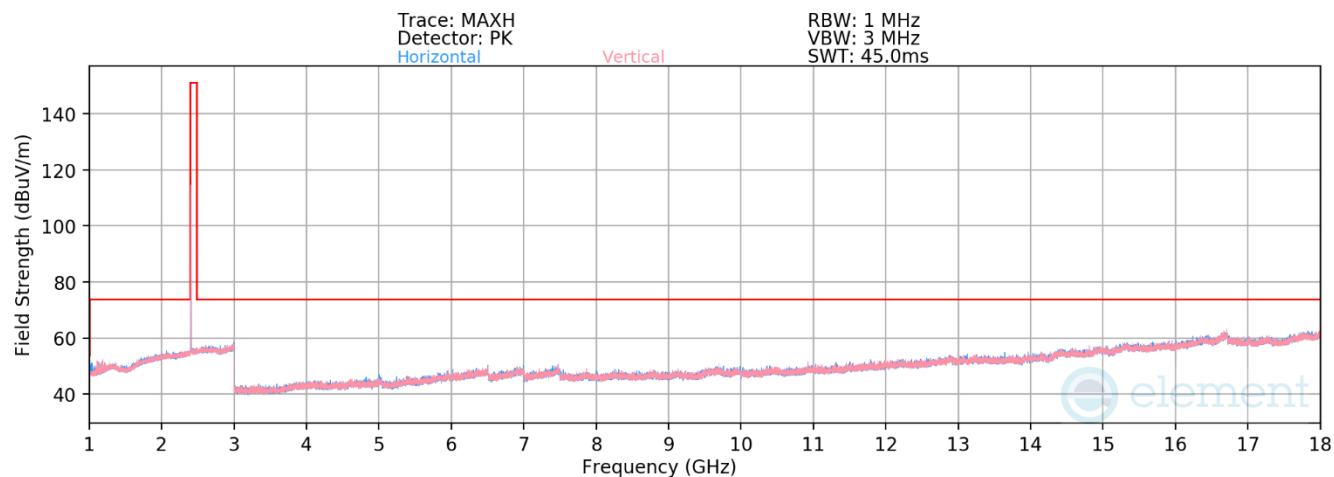
Plot 7-39. Radiated Spurious Emissions 1-18GHz Antenna 2a (802.15.4 ePA – Ch. 11)
