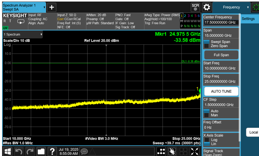
Plot 7-28. Conducted Spurious Antenna 4a (802.15.4, ePA – Ch. 25)
