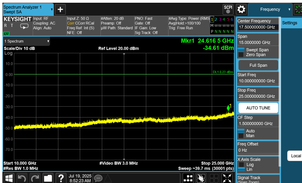
Plot 7-24. Conducted Spurious Antenna 4a (802.15.4, ePA – Ch. 11)
