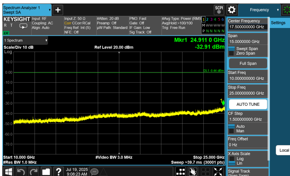
Plot 7-32. Conducted Spurious Antenna 2a (802.15.4, ePA – Ch. 18)
