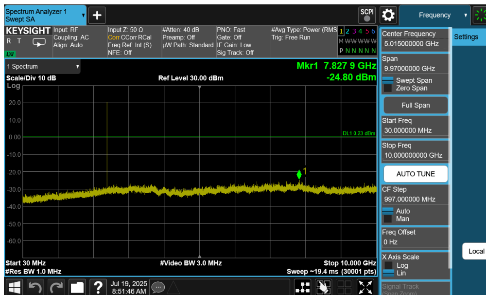
Plot 7-23. Conducted Spurious Antenna 4a (802.15.4, ePA – Ch. 11)
