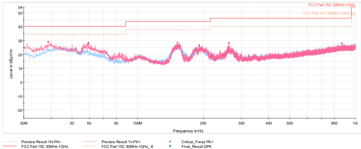
Plot 7-47. Radiated Spurious Emissions 30MHz-1GHz Antenna 4a (ePA - Ch.18, with AC/DC Adaptor)
