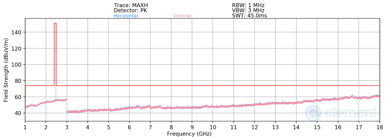
Plot 7-42. Radiated Spurious Emissions 1-18GHz Antenna 2a (802.15.4 ePA – Ch. 25)
