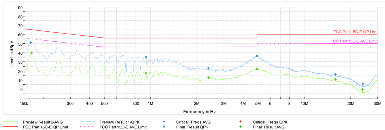
Plot 7-49. AC Line Conducted Emission with 802.15.4 Antenna 4a (N, Ch.18 - ePA, with AC/DC Adaptor)
