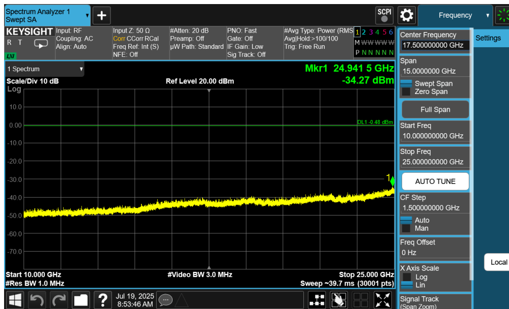
Plot 7-26. Conducted Spurious Antenna 4a (802.15.4, ePA – Ch. 18)
