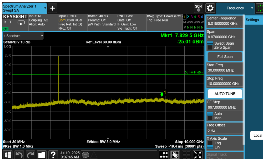
Plot 7-31. Conducted Spurious Antenna 2a (802.15.4, ePA – Ch. 18)
