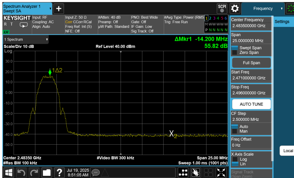
Plot 7-20. Band Edge Antenna 4a (802.15.4, ePA – Ch. 25)
