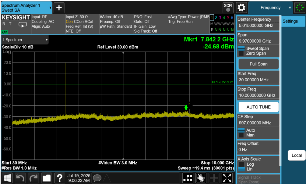
Plot 7-29. Conducted Spurious Antenna 2a (802.15.4, ePA – Ch. 11)
