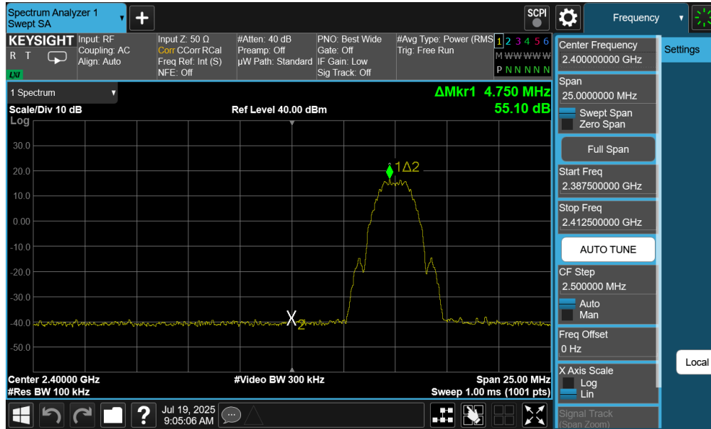
Plot 7-21. Band Edge Antenna 2a (802.15.4, ePA – Ch. 11)
