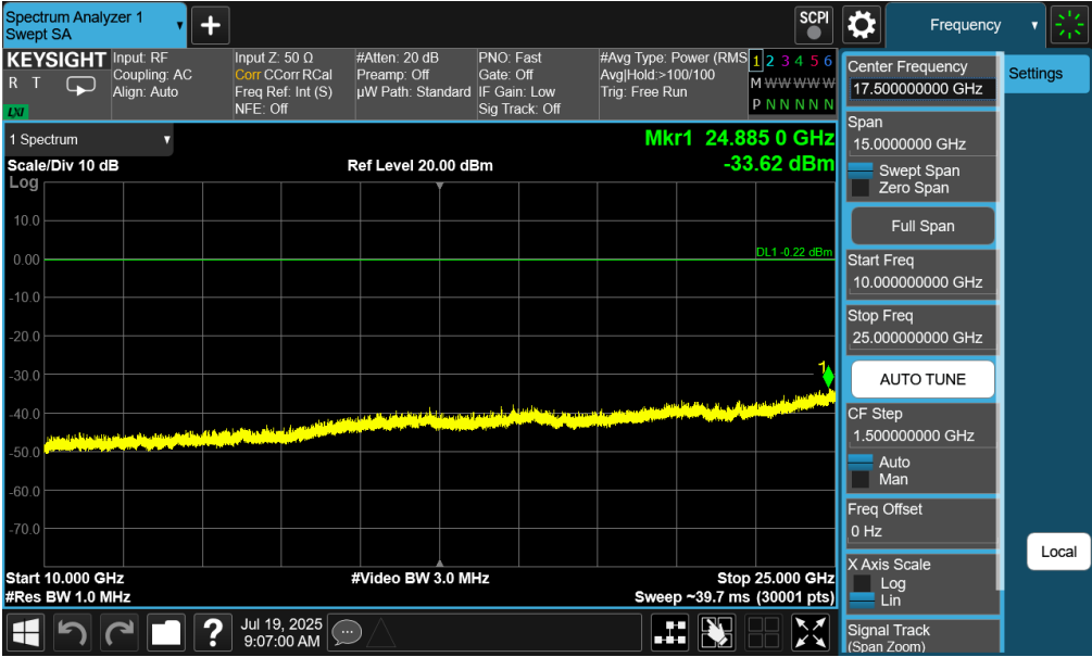
Plot 7-30. Conducted Spurious Antenna 2a (802.15.4, ePA – Ch. 11)
