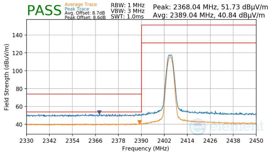
Plot 7-45. Radiated Restricted Lower Band Edge Measurement Antenna 2a
