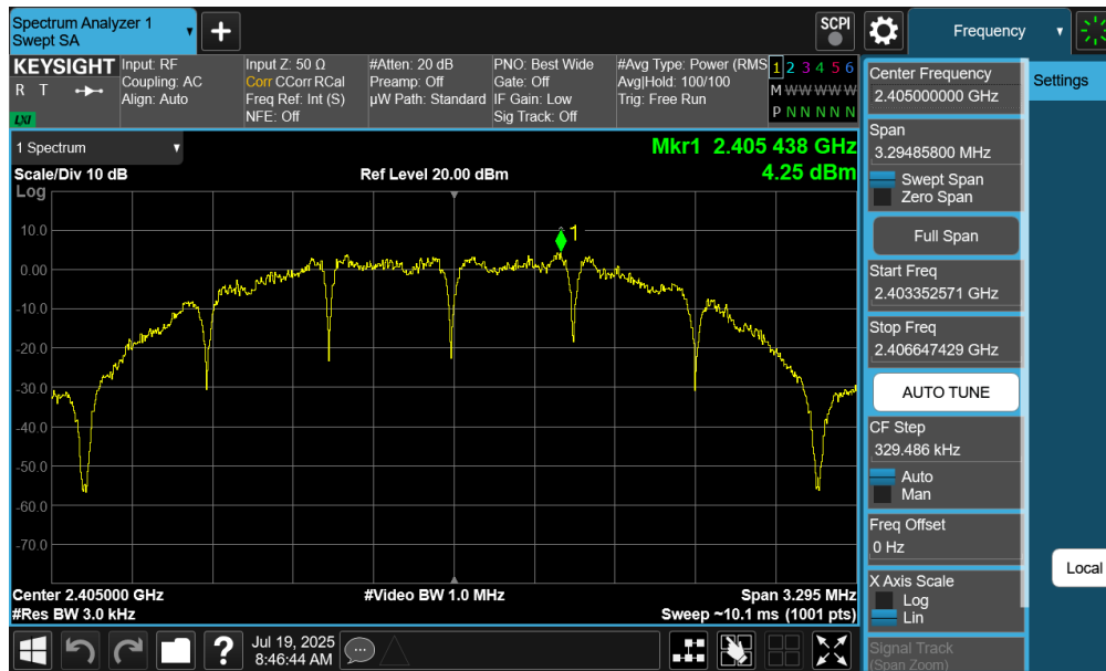
Plot 7-7. Power Spectral Density Antenna 4a (802.15.4, ePA – Ch. 11)
