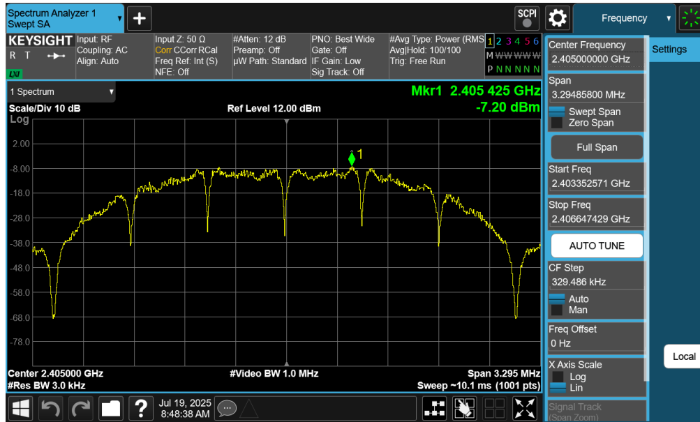
Plot 7-10. Power Spectral Density Antenna 4a (802.15.4, iPA – Ch. 11)
