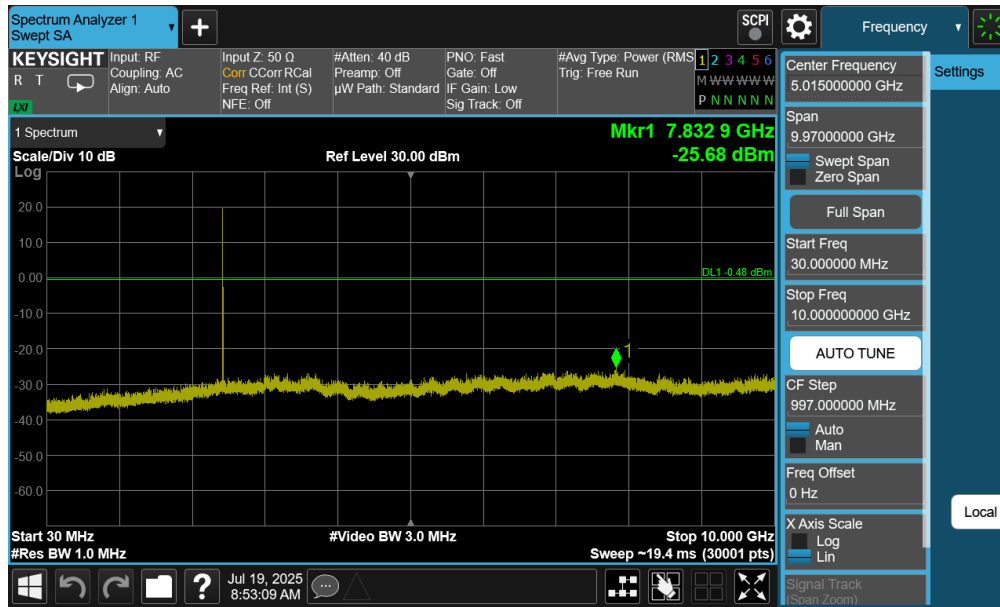
Plot 7-25. Conducted Spurious Antenna 4a (802.15.4, ePA – Ch. 18)
