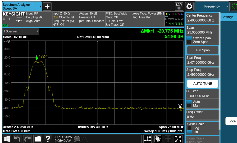
Plot 7-22. Band Edge Antenna 2a (802.15.4, ePA – Ch. 25)
