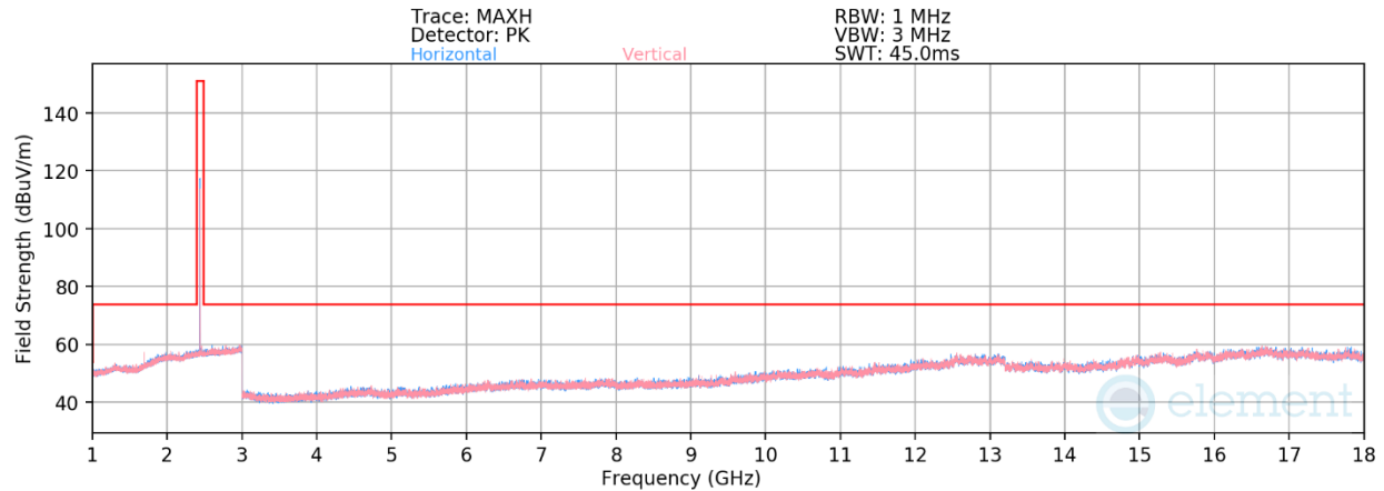
Plot 7-40. Radiated Spurious Emissions 1-18GHz Antenna 2a (802.15.4 ePA – Ch. 18)
