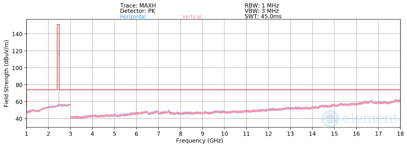
Plot 7-38. Radiated Spurious Emissions 1-18GHz Antenna 4a (802.15.4 ePA – Ch. 25)
