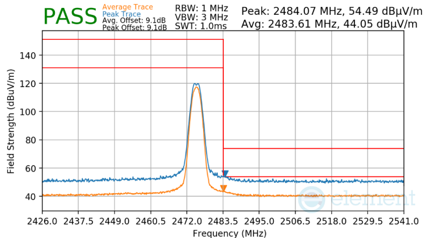
Plot 7-44. Radiated Restricted Upper Band Edge Measurement Antenna 4a
