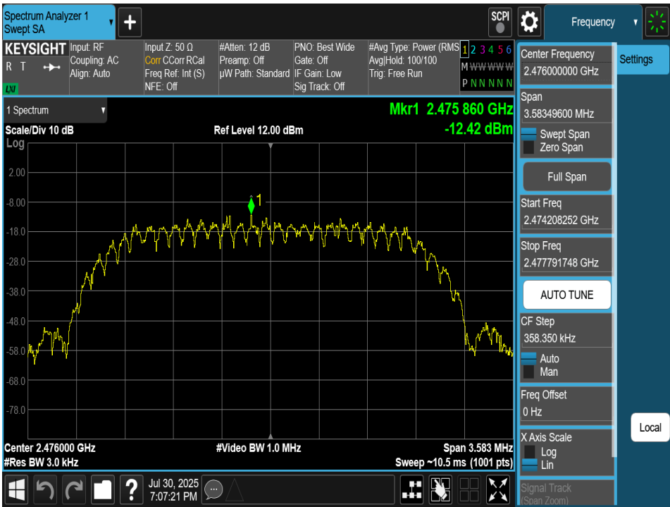
Plot 7-72. Power Spectral Density Plot Antenna 4a (Bluetooth (HDT2), 2Mbps, iPA – Ch. 73)
