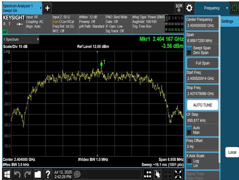
Plot 7-79. Power Spectral Density Plot Antenna 2a (Bluetooth (HDR8), 8Mbps, ePA – Ch. 1)
