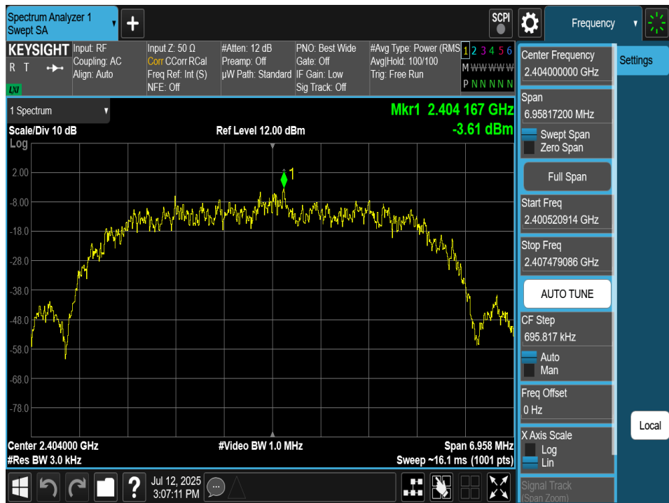
Plot 7-122. Power Spectral Density Plot TxBF Antenna 2a (Bluetooth (HDR8), 8Mbps, ePA – Ch. 1)
