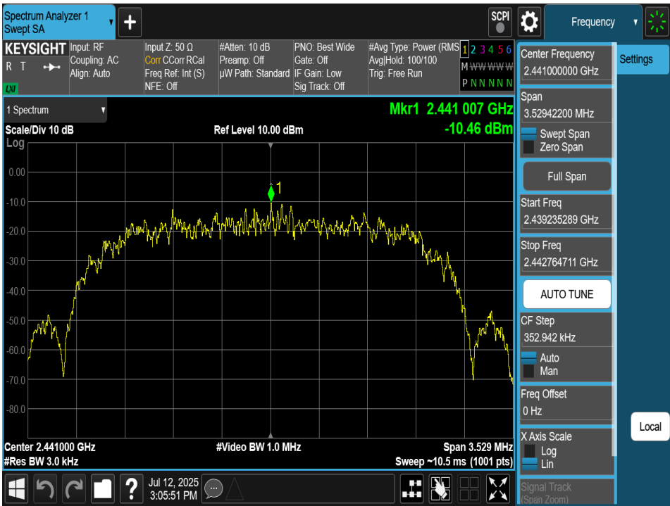
Plot 7-118. Power Spectral Density Plot TxBF Antenna 2a (Bluetooth (HDR4), 4Mbps, iPA – Ch. 38)
