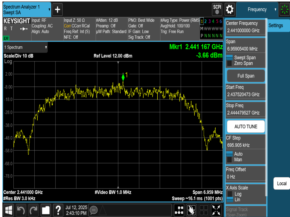
Plot 7-80. Power Spectral Density Plot Antenna 2a (Bluetooth (HDR8), 8Mbps, ePA – Ch. 38)
