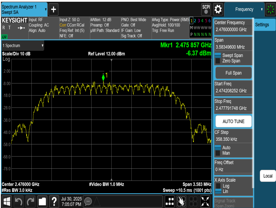
Plot 7-69. Power Spectral Density Plot Antenna 4a (Bluetooth (HDT2), 2Mbps, ePA – Ch. 73)
