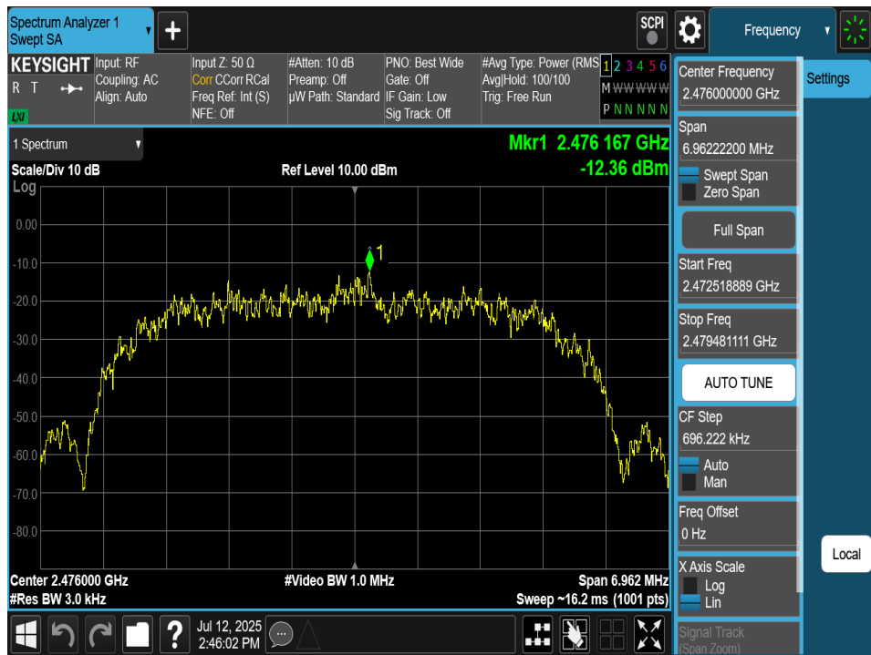
Plot 7-84. Power Spectral Density Plot Antenna 2a (Bluetooth (HDR8), 8Mbps, iPA – Ch. 73)
