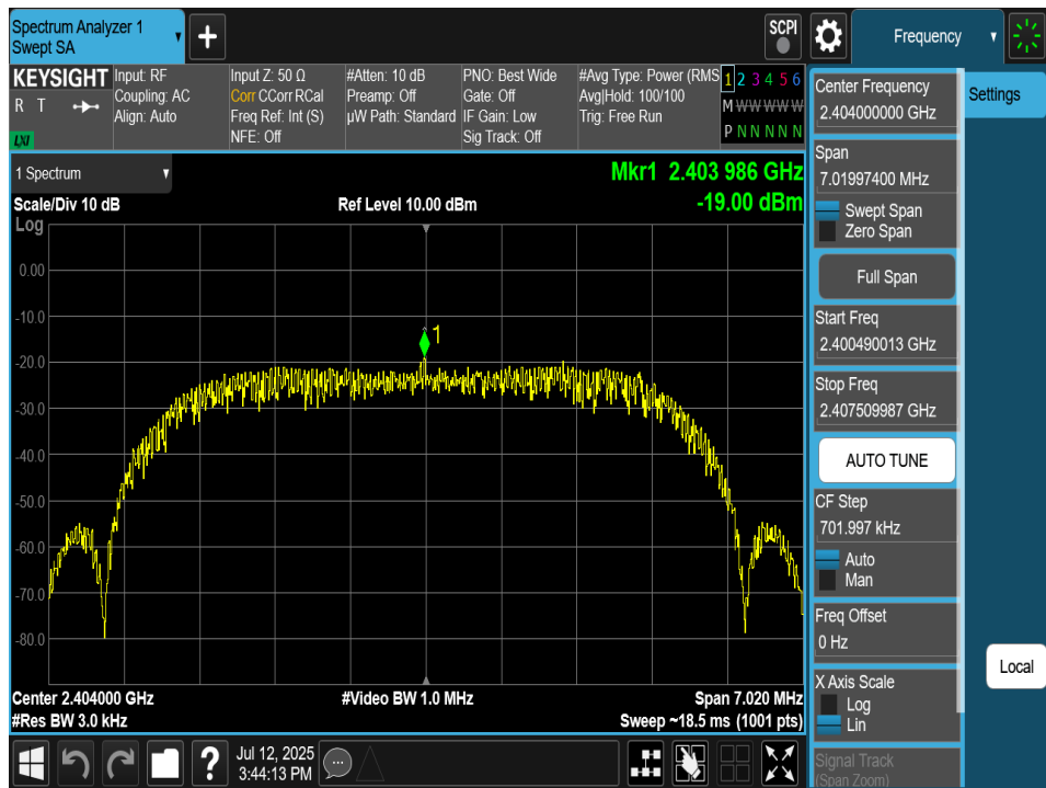
Plot 7-100. Power Spectral Density Plot Antenna 2a (Bluetooth (HDRPM16), 16Mbps, iPA – Ch. 1)
