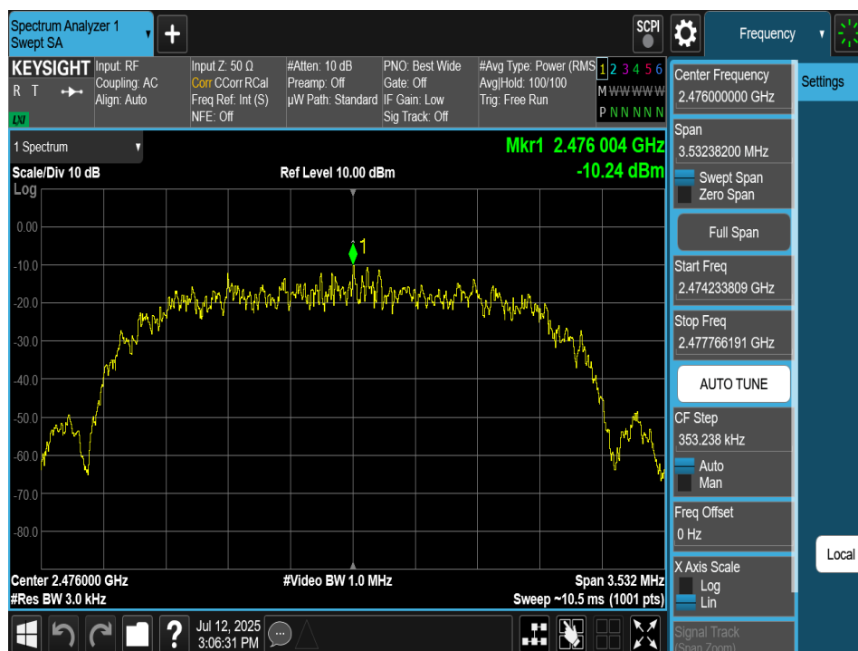
Plot 7-120. Power Spectral Density Plot TxBF Antenna 2a (Bluetooth (HDR4), 4Mbps, iPA – Ch. 73)
