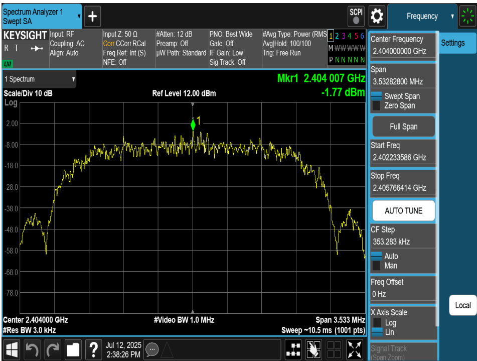
Plot 7-73. Power Spectral Density Plot Antenna 2a (Bluetooth (HDR4), 4Mbps, ePA – Ch. 1)
