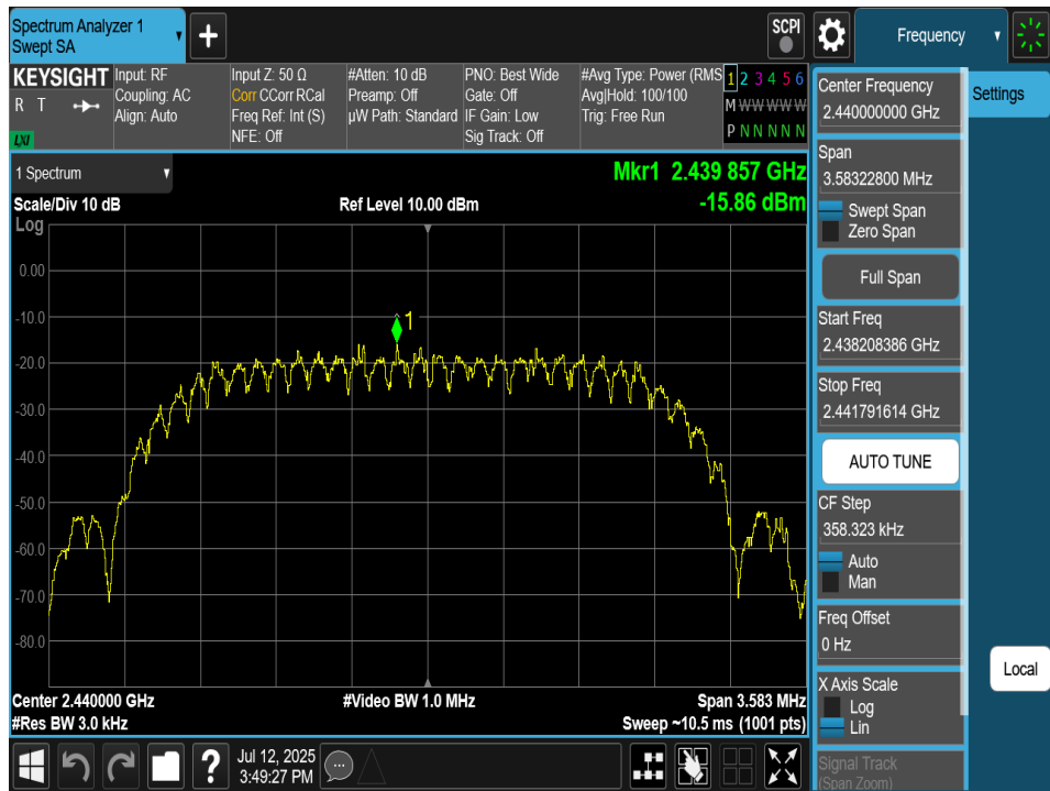
Plot 7-107. Power Spectral Density Plot Antenna 2a (Bluetooth (HDT2), 2Mbps, iPA – Ch. 37)
