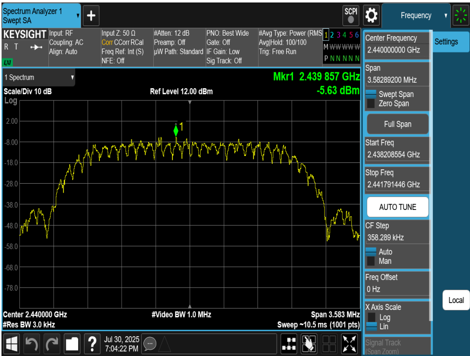
Plot 7-68. Power Spectral Density Plot Antenna 4a (Bluetooth (HDT2), 2Mbps, ePA – Ch. 37)
