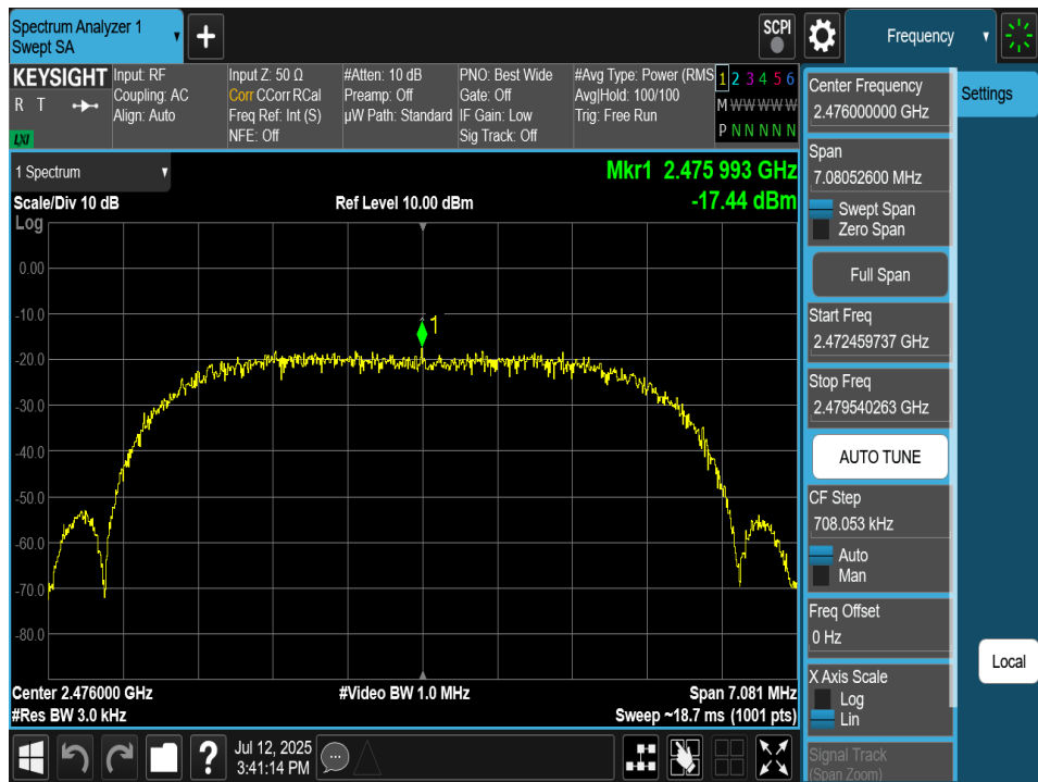
Plot 7-96. Power Spectral Density Plot Antenna 2a (Bluetooth (XHDRPM6), 6Mbps, iPA – Ch. 73)
