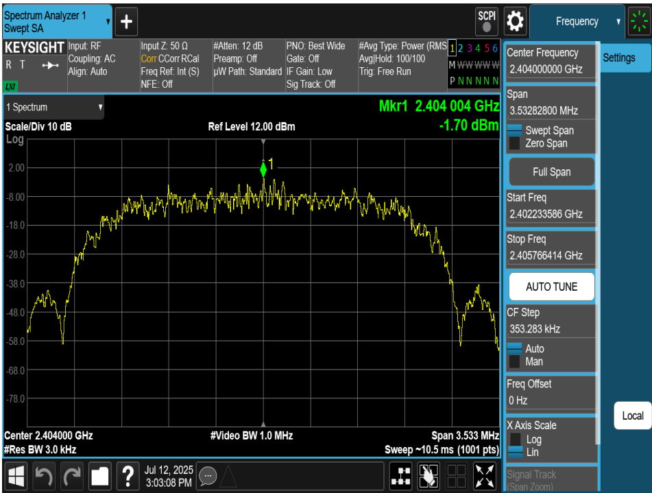
Plot 7-110. Power Spectral Density Plot TxBF Antenna 2a (Bluetooth (HDR4), 4Mbps, ePA – Ch. 1)
