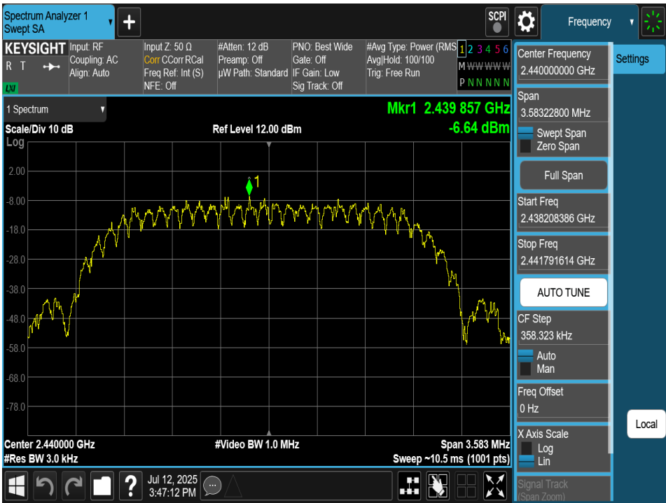
Plot 7-104. Power Spectral Density Plot Antenna 2a (Bluetooth (HDT2), 2Mbps, ePA – Ch. 37)
