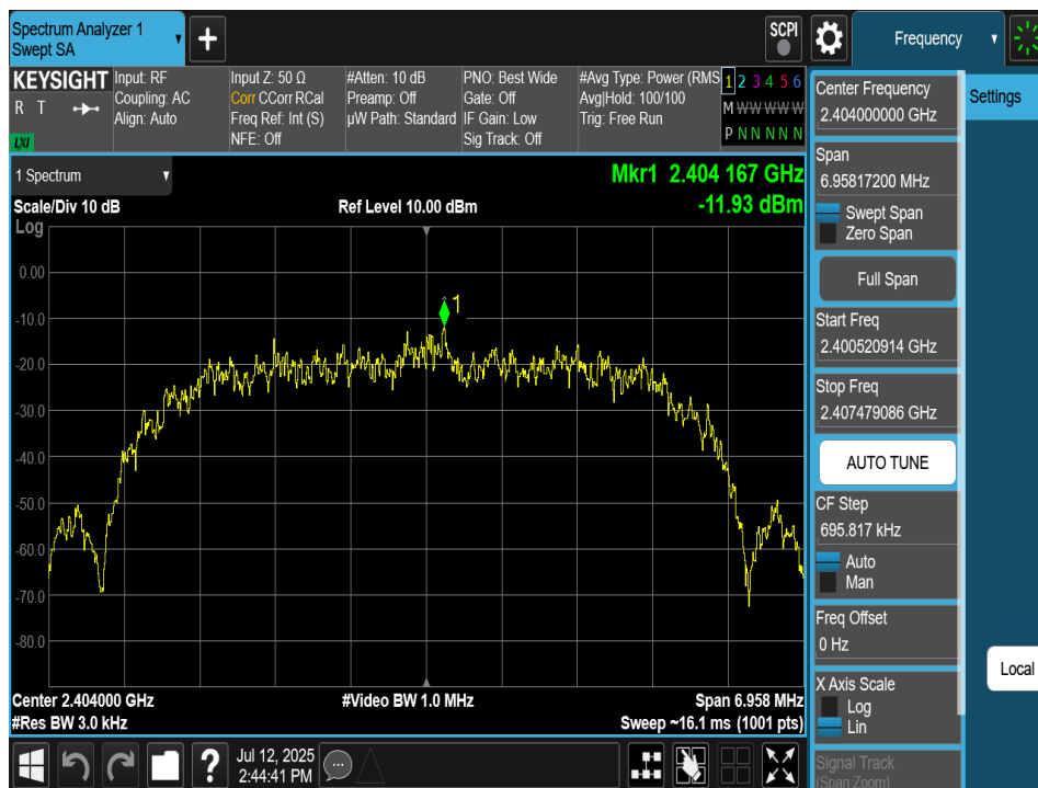
Plot 7-82. Power Spectral Density Plot Antenna 2a (Bluetooth (HDR8), 8Mbps, iPA – Ch. 1)
