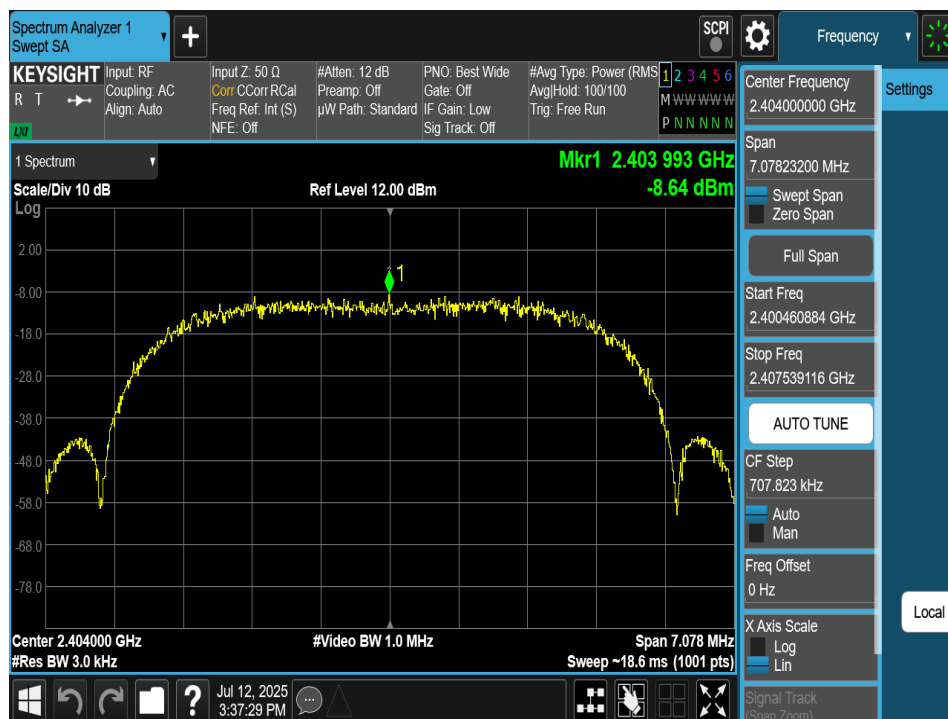
Plot 7-91. Power Spectral Density Plot Antenna 2a (Bluetooth (XHDRPM6), 6Mbps, ePA – Ch. 1)
