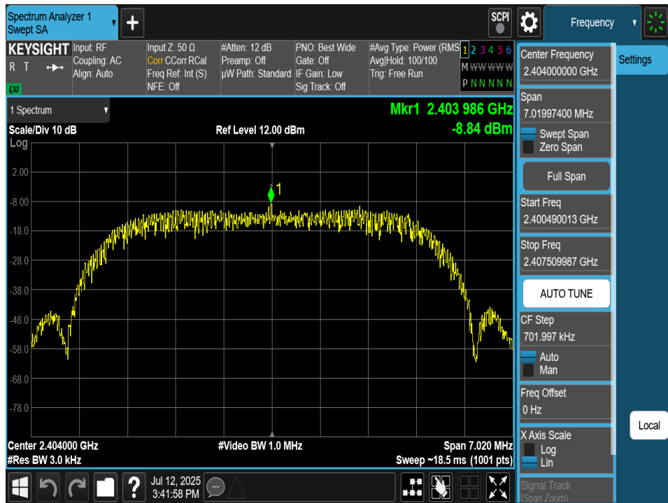
Plot 7-97. Power Spectral Density Plot Antenna 2a (Bluetooth (HDRPM16), 16Mbps, ePA – Ch. 1)
