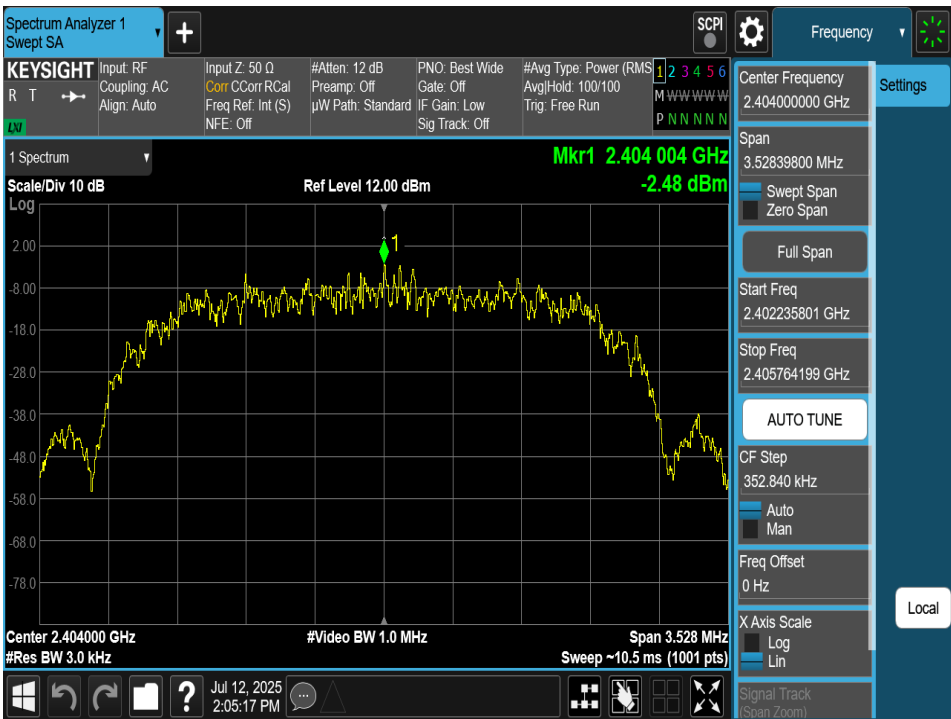
Plot 7-109. Power Spectral Density Plot TxBF Antenna 4a (Bluetooth (HDR4), 4Mbps, ePA – Ch. 1)
