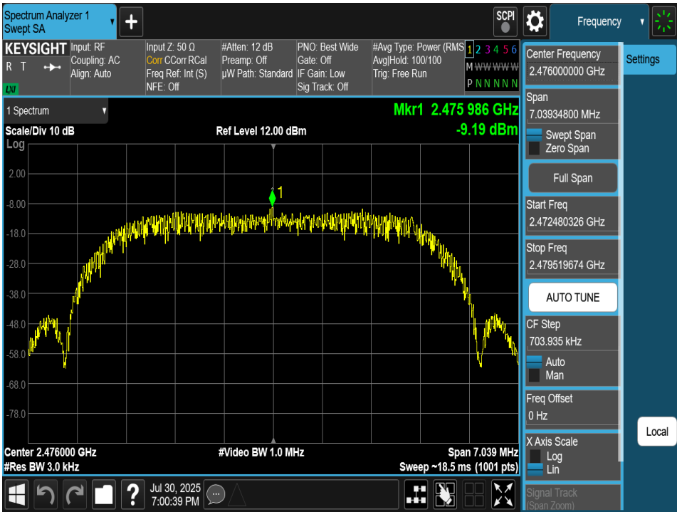
Plot 7-63. Power Spectral Density Plot Antenna 4a (Bluetooth (HDRPM16), 16Mbps, ePA – Ch. 73)
