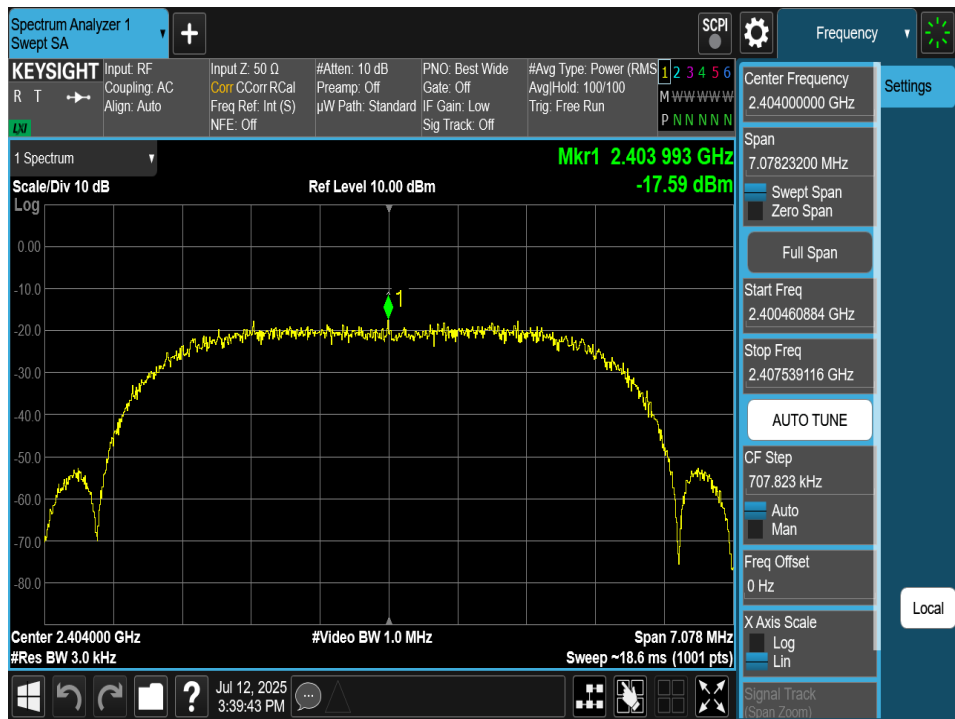
Plot 7-94. Power Spectral Density Plot Antenna 2a (Bluetooth (XHDRPM6), 6Mbps, iPA – Ch. 1)
