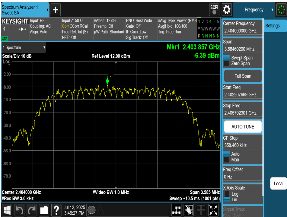
Plot 7-103. Power Spectral Density Plot Antenna 2a (Bluetooth (HDT2), 2Mbps, ePA – Ch. 1)
