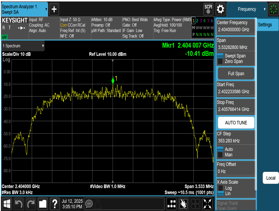
Plot 7-116. Power Spectral Density Plot TxBF Antenna 2a (Bluetooth (HDR4), 4Mbps, iPA – Ch. 1)
