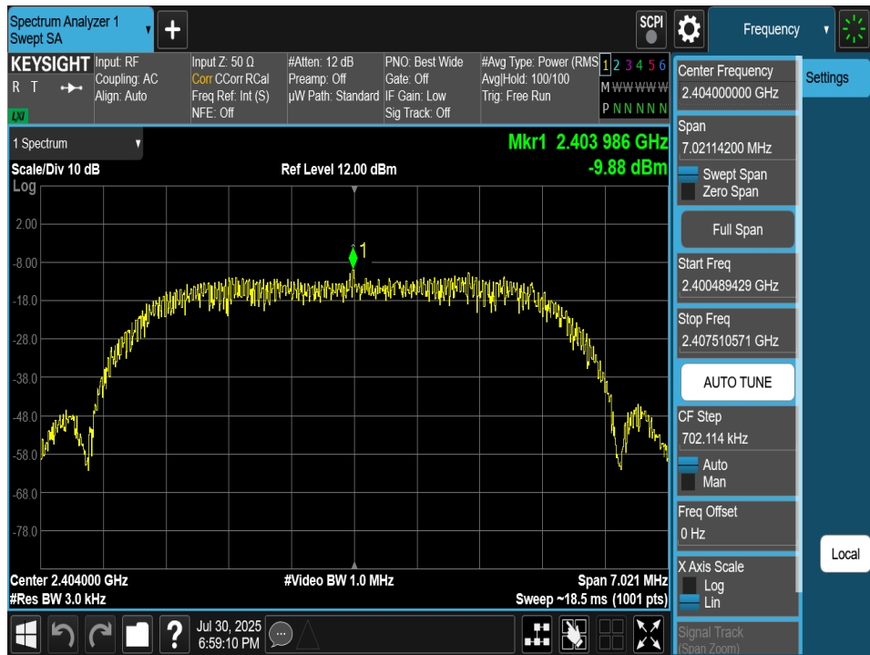
Plot 7-61. Power Spectral Density Plot Antenna 4a (Bluetooth (HDRPM16), 16Mbps, ePA – Ch. 1)
