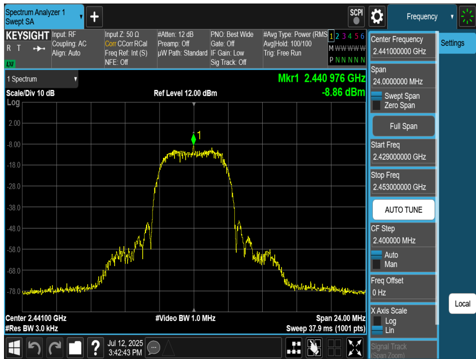
Plot 7-98. Power Spectral Density Plot Antenna 2a (Bluetooth (HDRPM16), 16Mbps, ePA – Ch. 38)
