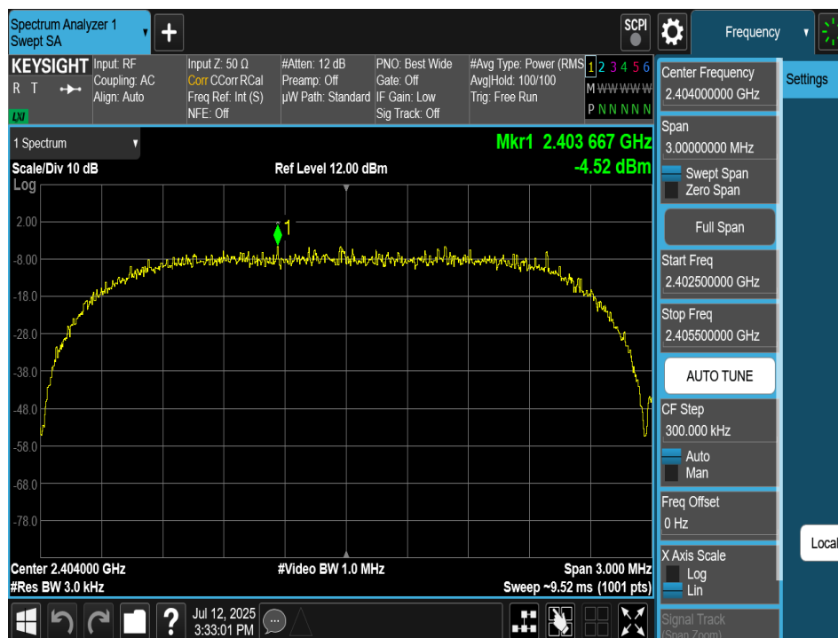
Plot 7-85. Power Spectral Density Plot Antenna 2a (Bluetooth (HDRPS2), 2Mbps, ePA – Ch. 1)
