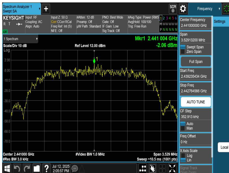
Plot 7-111. Power Spectral Density Plot TxBF Antenna 4a (Bluetooth (HDR4), 4Mbps, ePA – Ch. 38)
