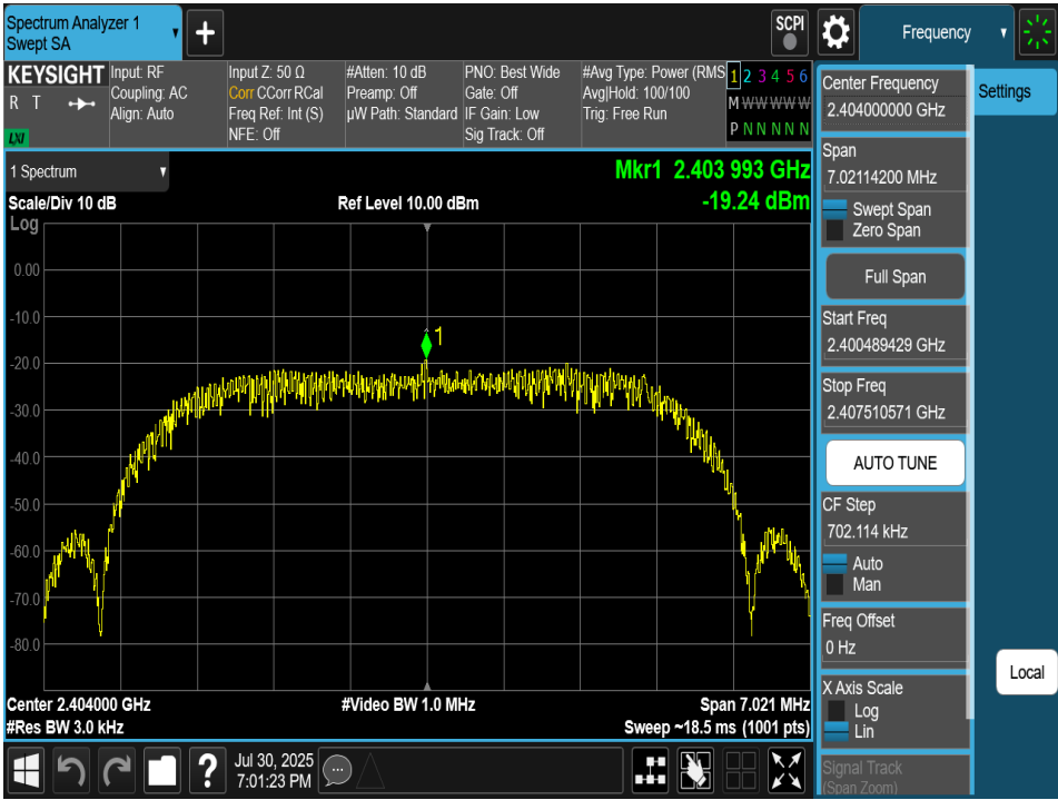
Plot 7-64. Power Spectral Density Plot Antenna 4a (Bluetooth (HDRPM16), 16Mbps, iPA – Ch. 1)
