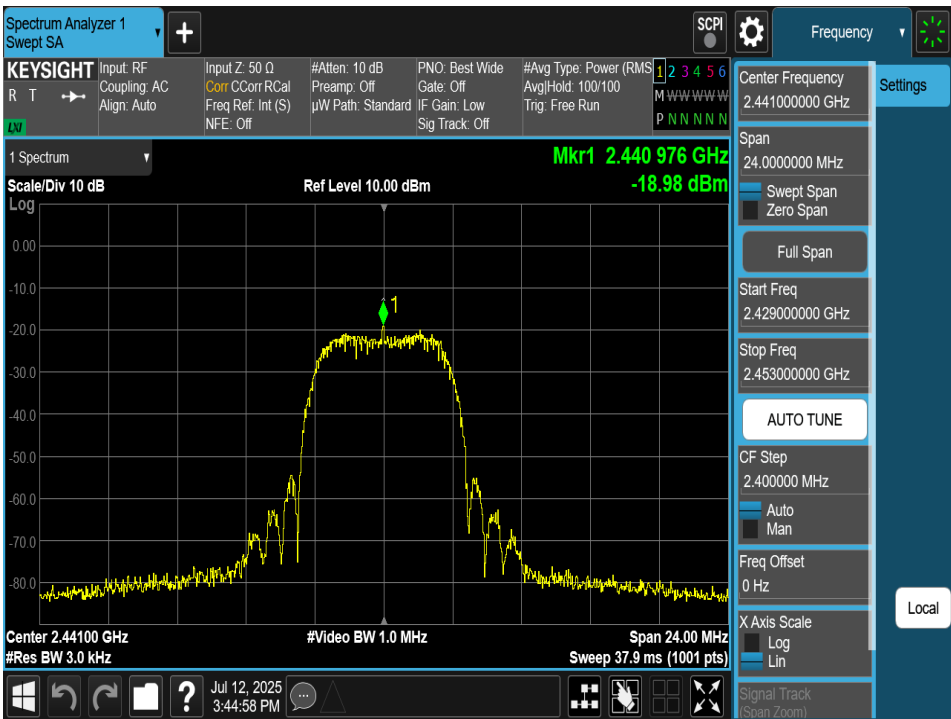
Plot 7-101. Power Spectral Density Plot Antenna 2a (Bluetooth (HDRPM16), 16Mbps, iPA – Ch. 38)
