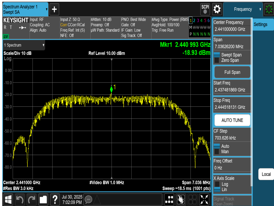
Plot 7-65. Power Spectral Density Plot Antenna 4a (Bluetooth (HDRPM16), 16Mbps, iPA – Ch. 38)
