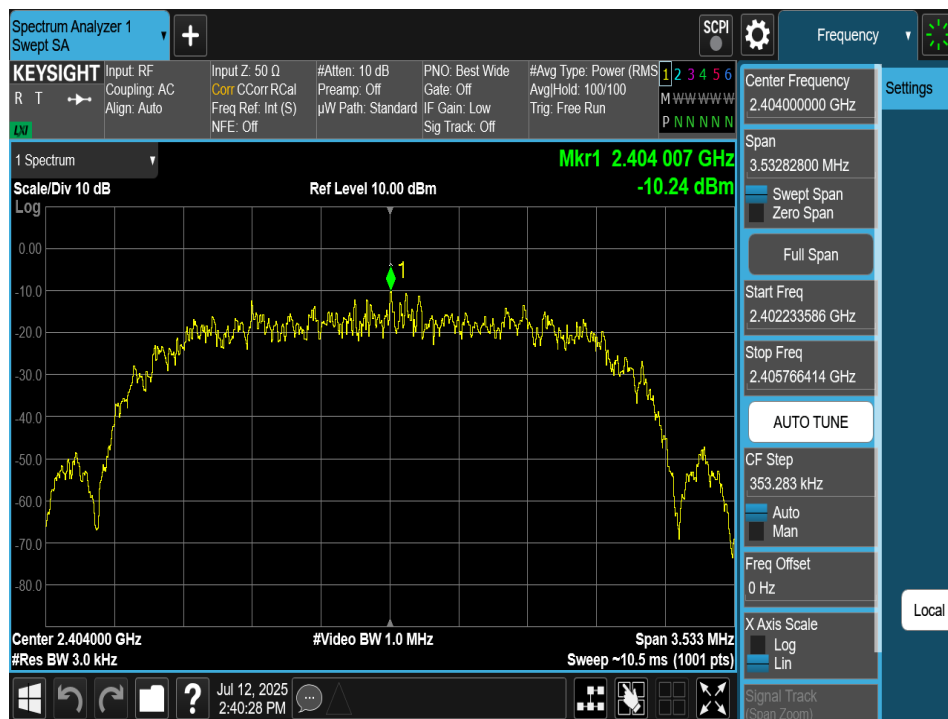
Plot 7-76. Power Spectral Density Plot Antenna 2a (Bluetooth (HDR4), 4Mbps, iPA – Ch. 1)
