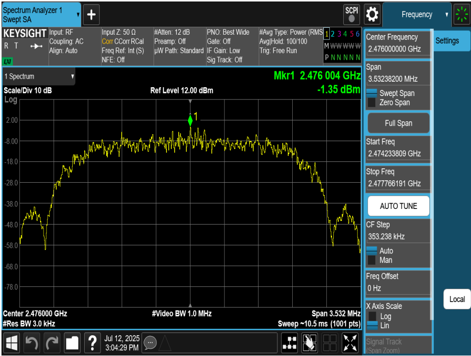
Plot 7-114. Power Spectral Density Plot Tx BF Antenna 2a (Bluetooth (HDR4), 4Mbps, ePA – Ch. 73)
