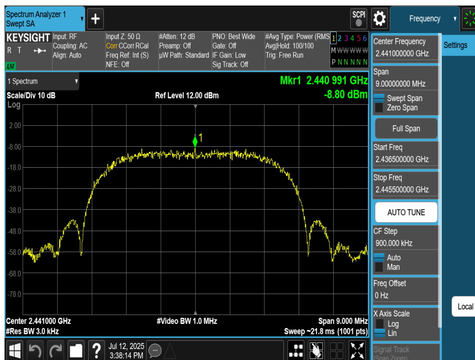
Plot 7-92. Power Spectral Density Plot Antenna 2a (Bluetooth (XHDRPM6), 6Mbps, ePA – Ch. 38)
