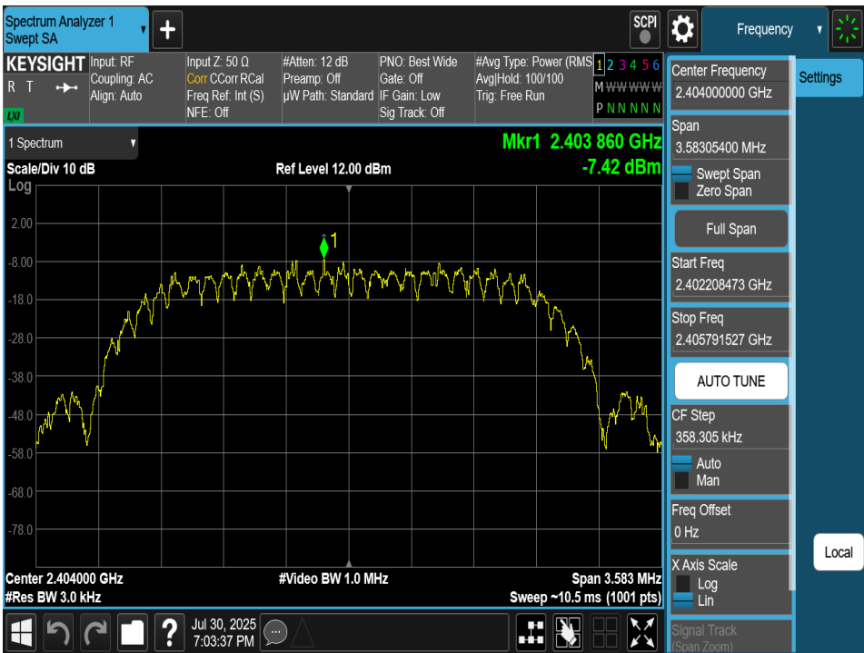
Plot 7-67. Power Spectral Density Plot Antenna 4a (Bluetooth (HDT2), 2Mbps, ePA – Ch. 1)
