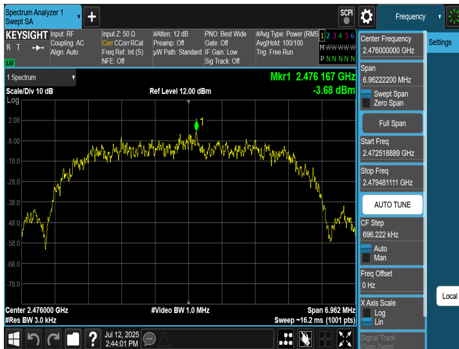
Plot 7-81. Power Spectral Density Plot Antenna 2a (Bluetooth (HDR8), 8Mbps, ePA – Ch. 73)
