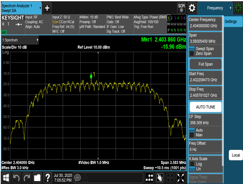
Plot 7-70. Power Spectral Density Plot Antenna 4a (Bluetooth (HDT2), 2Mbps, iPA – Ch. 1)
