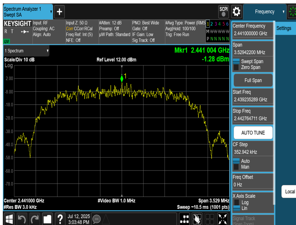
Plot 7-112. Power Spectral Density Plot TxBF Antenna 2a (Bluetooth (HDR4), 4Mbps, ePA – Ch. 38)
