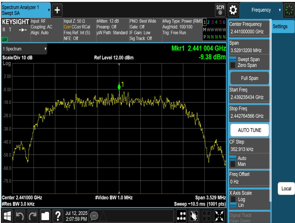
Plot 7-117. Power Spectral Density Plot TxBF Antenna 4a (Bluetooth (HDR4), 4Mbps, iPA – Ch. 38)
