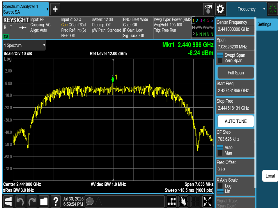
Plot 7-62. Power Spectral Density Plot Antenna 4a (Bluetooth (HDRPM16), 16Mbps, ePA – Ch. 38)
