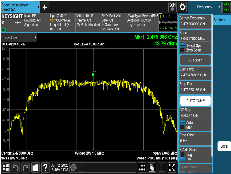
Plot 7-102. Power Spectral Density Plot Antenna 2a (Bluetooth (HDRPM16), 16Mbps, iPA – Ch. 73)
