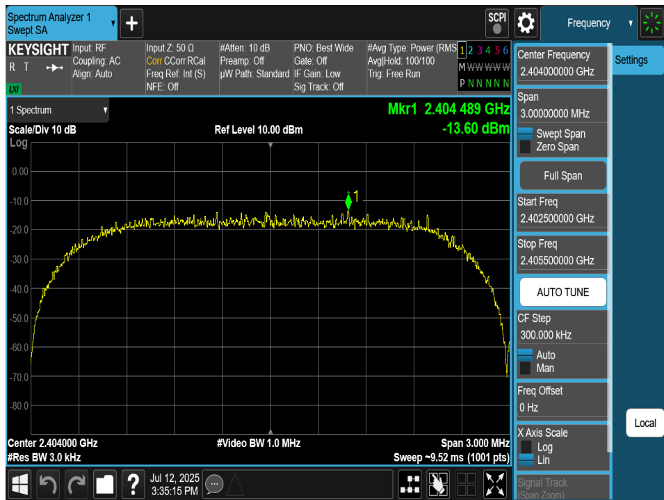
Plot 7-88. Power Spectral Density Plot Antenna 2a (Bluetooth (HDRPS2), 2Mbps, iPA – Ch. 1)
