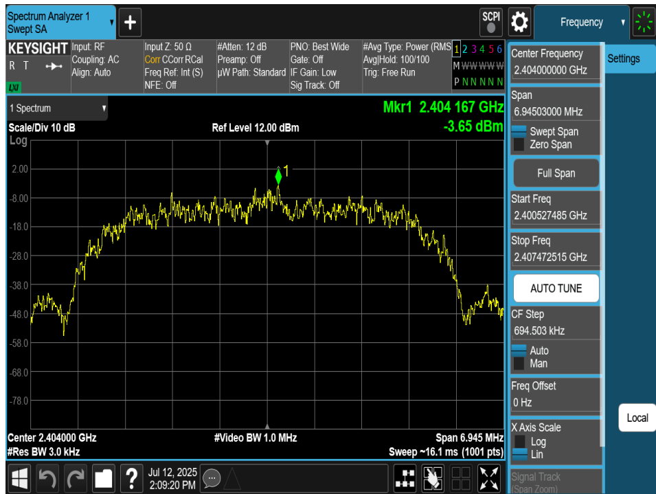
Plot 7-121. Power Spectral Density Plot TxBF Antenna 4a (Bluetooth (HDR8), 8Mbps, ePA – Ch. 1)
