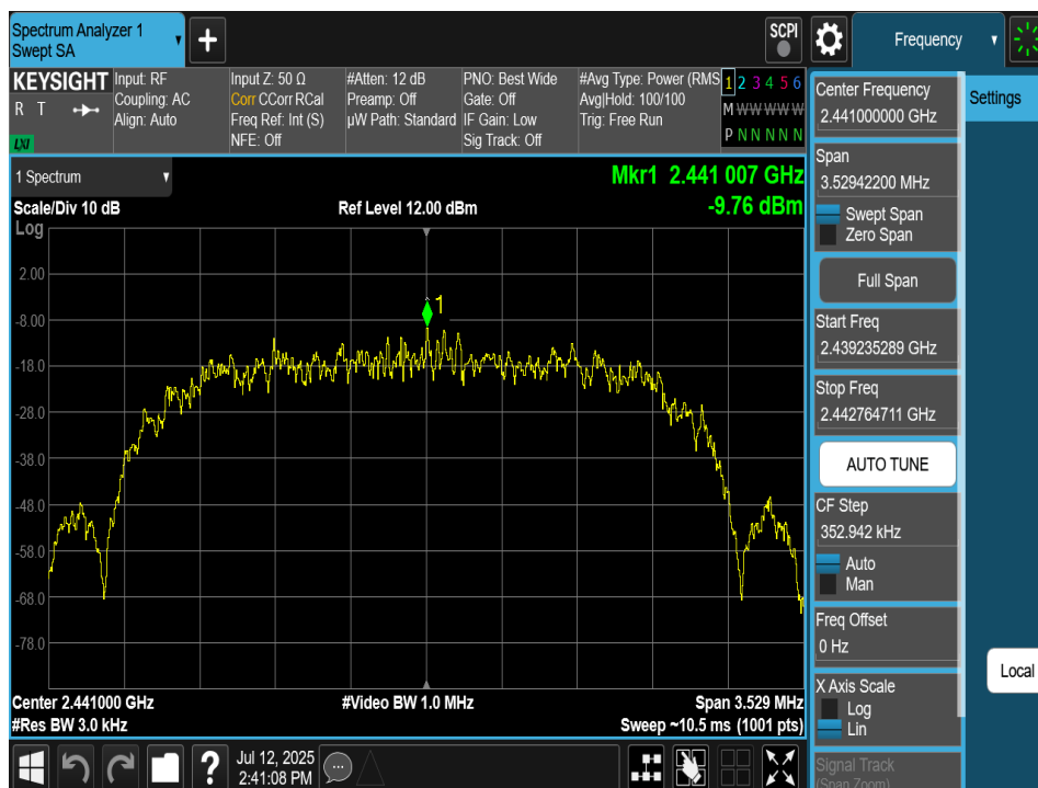
Plot 7-77. Power Spectral Density Plot Antenna 2a (Bluetooth (HDR4), 4Mbps, iPA – Ch. 38)
