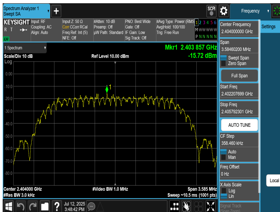
Plot 7-106. Power Spectral Density Plot Antenna 2a (Bluetooth (HDT2), 2Mbps, iPA – Ch. 1)
