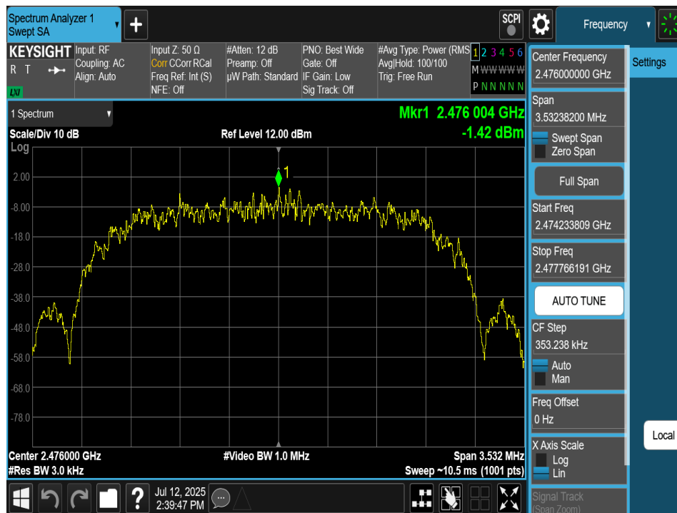
Plot 7-75. Power Spectral Density Plot Antenna 2a (Bluetooth (HDR4), 4Mbps, ePA – Ch. 73)
