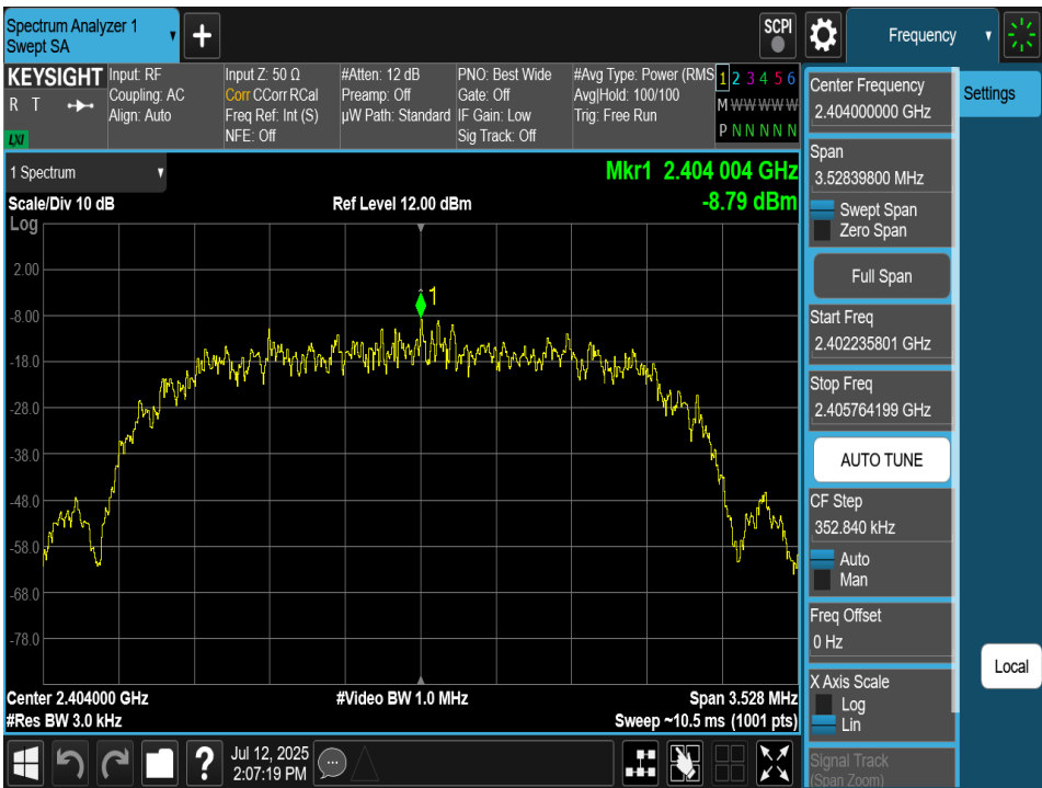
Plot 7-115. Power Spectral Density Plot TxBF Antenna 4a (Bluetooth (HDR4), 4Mbps, iPA – Ch. 1)
