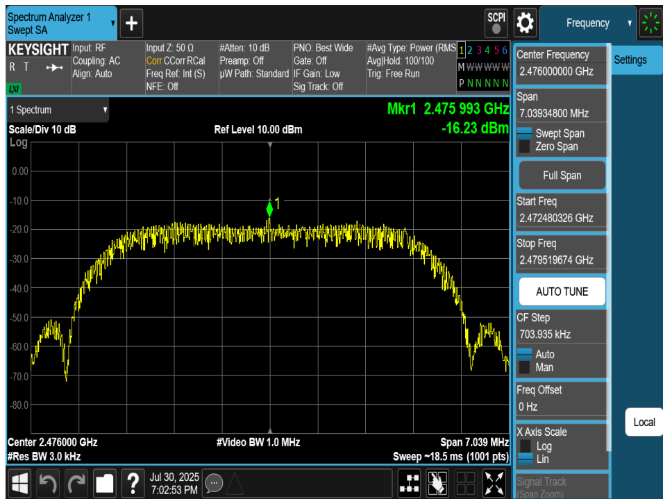
Plot 7-66. Power Spectral Density Plot Antenna 4a (Bluetooth (HDRPM16), 16Mbps, iPA – Ch. 73)
