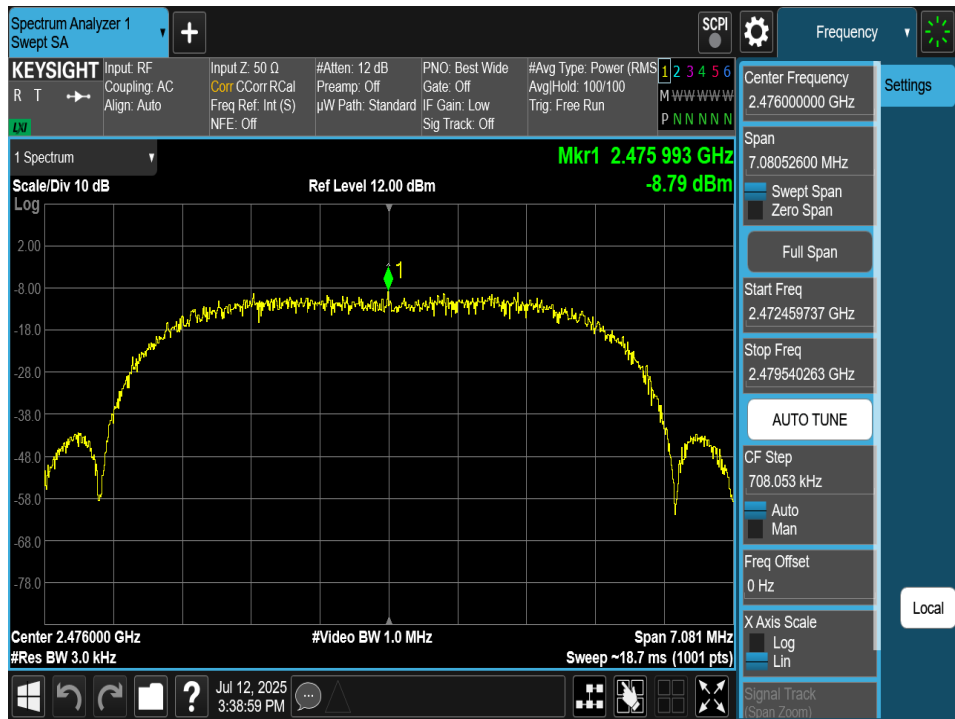
Plot 7-93. Power Spectral Density Plot Antenna 2a (Bluetooth (XHDRPM6), 6Mbps, ePA – Ch. 73)
