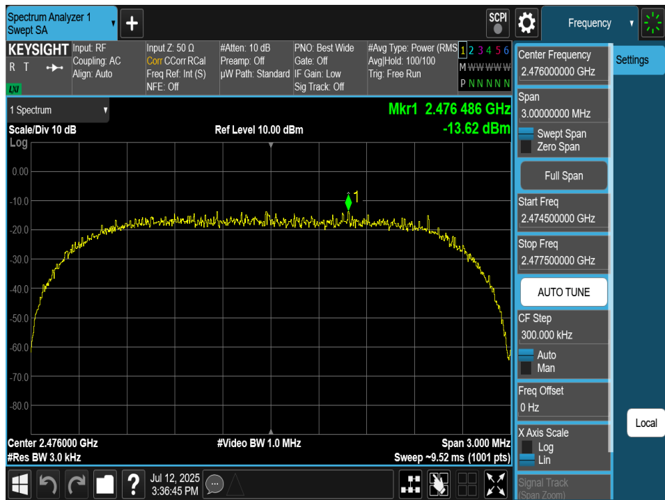
Plot 7-90. Power Spectral Density Plot Antenna 2a (Bluetooth (HDRPS2), 2Mbps, iPA – Ch. 73)
