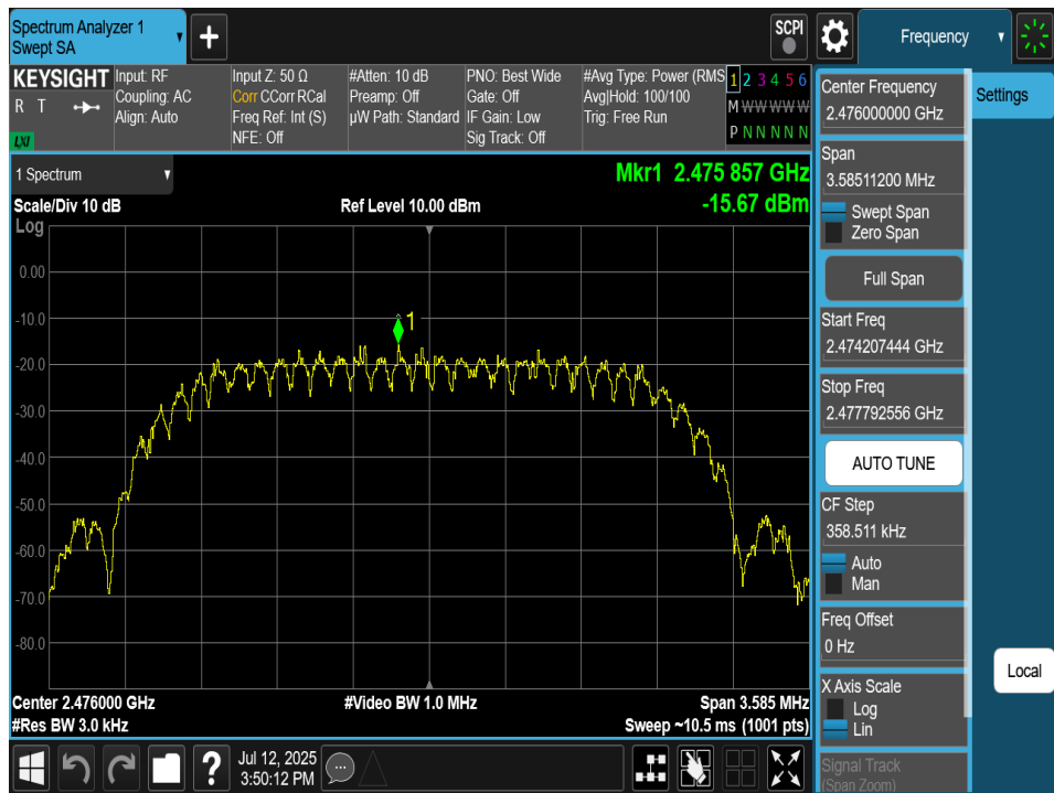
Plot 7-108. Power Spectral Density Plot Antenna 2a (Bluetooth (HDT2), 2Mbps, iPA – Ch. 73)
