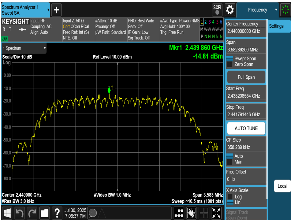
Plot 7-71. Power Spectral Density Plot Antenna 4a (Bluetooth (HDT2), 2Mbps, iPA – Ch. 37)
