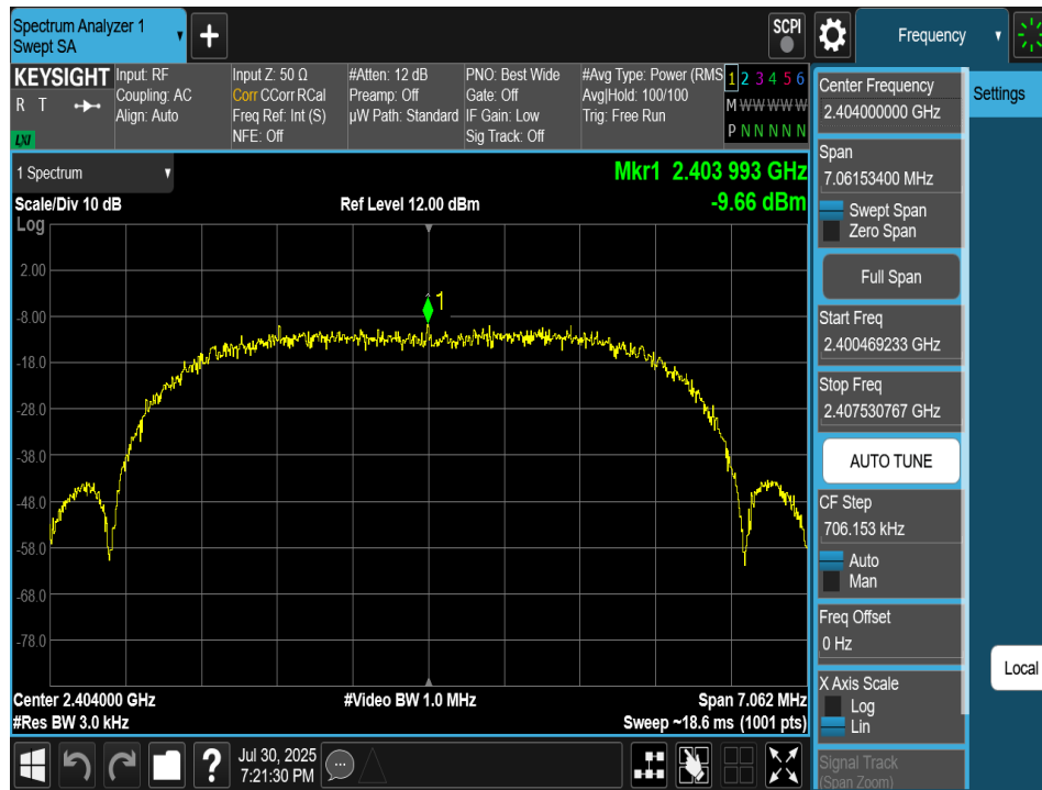
Plot 7-145. Power Spectral Density Plot TxBF Antenna 4a (Bluetooth (XHDRPM6), 6Mbps, ePA – Ch. 1)
