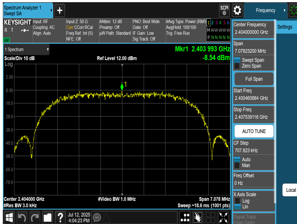
Plot 7-146. Power Spectral Density Plot TxBF Antenna 2a (Bluetooth (XHDRPM6), 6Mbps, ePA – Ch. 1)
