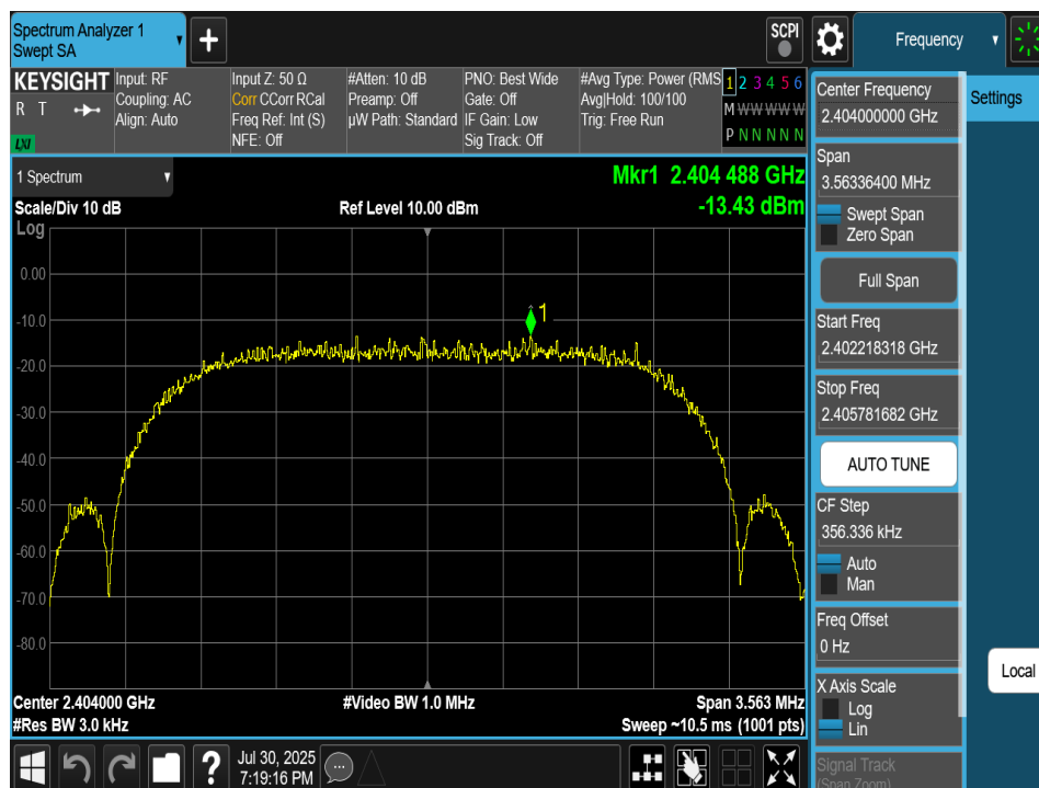
Plot 7-139. Power Spectral Density Plot TxBF Antenna 4a (Bluetooth (HDRPS2), 2Mbps, iPA – Ch. 1)
