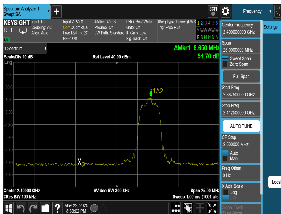
Plot 7-181. Band Edge Plot Antenna 4a (Bluetooth (HDR4), 4Mbps, ePA – Ch. 1)
