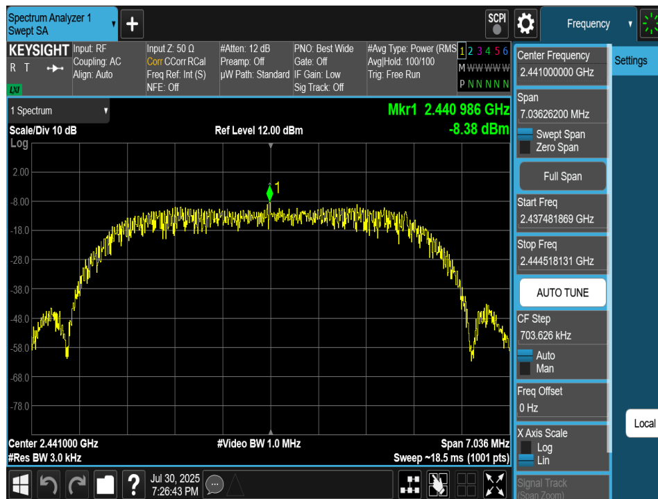
Plot 7-159. Power Spectral Density Plot Tx BF Antenna 4a (Bluetooth (HDRPM16), 16Mbps, ePA – Ch. 38)
