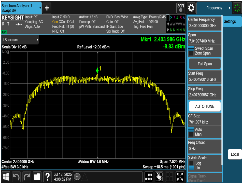
Plot 7-158. Power Spectral Density Plot TxBF Antenna 2a (Bluetooth (HDRPM16), 16Mbps, ePA – Ch. 1)
