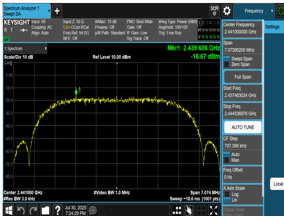
Plot 7-153. Power Spectral Density Plot TxBF Antenna 4a (Bluetooth (XHDRPM6), 6Mbps, iPA – Ch. 38)
