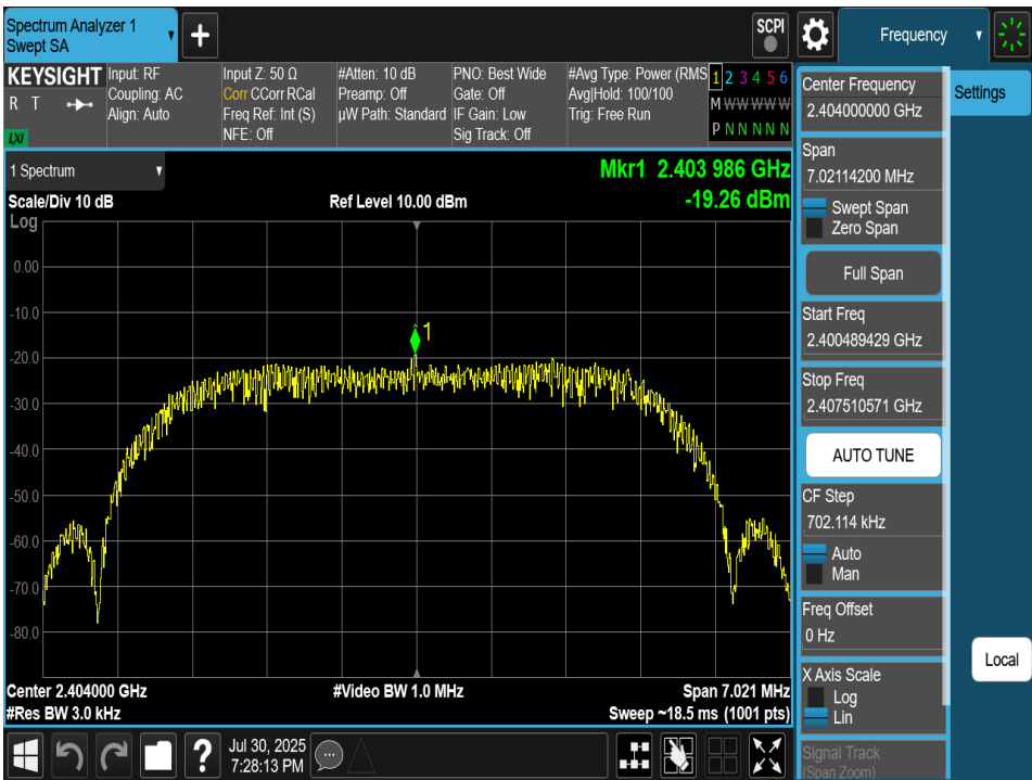
Plot 7-163. Power Spectral Density Plot TxBF Antenna 4a (Bluetooth (HDRPM16), 16Mbps, iPA – Ch. 1)
