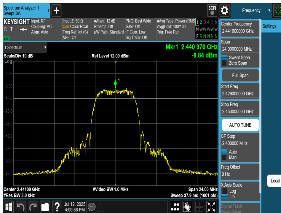
Plot 7-160. Power Spectral Density Plot Tx BF Antenna 2a (Bluetooth (HDRPM16), 16Mbps, ePA – Ch. 38)
