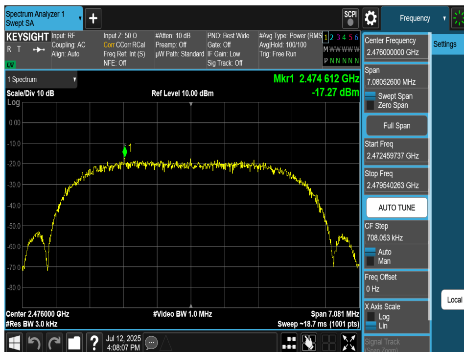
Plot 7-156. Power Spectral Density Plot TxBF Antenna 2a (Bluetooth (XHDRPM6), 6Mbps, iPA – Ch. 73)
