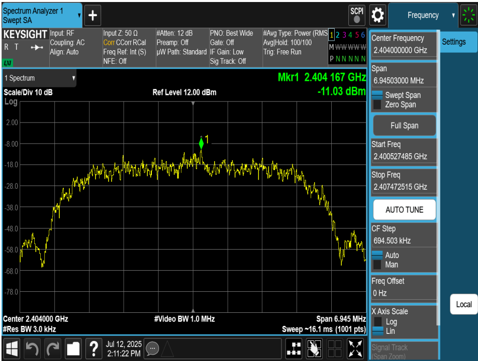
Plot 7-127. Power Spectral Density Plot TxBF Antenna 4a (Bluetooth (HDR8), 8Mbps, iPA – Ch. 1)
