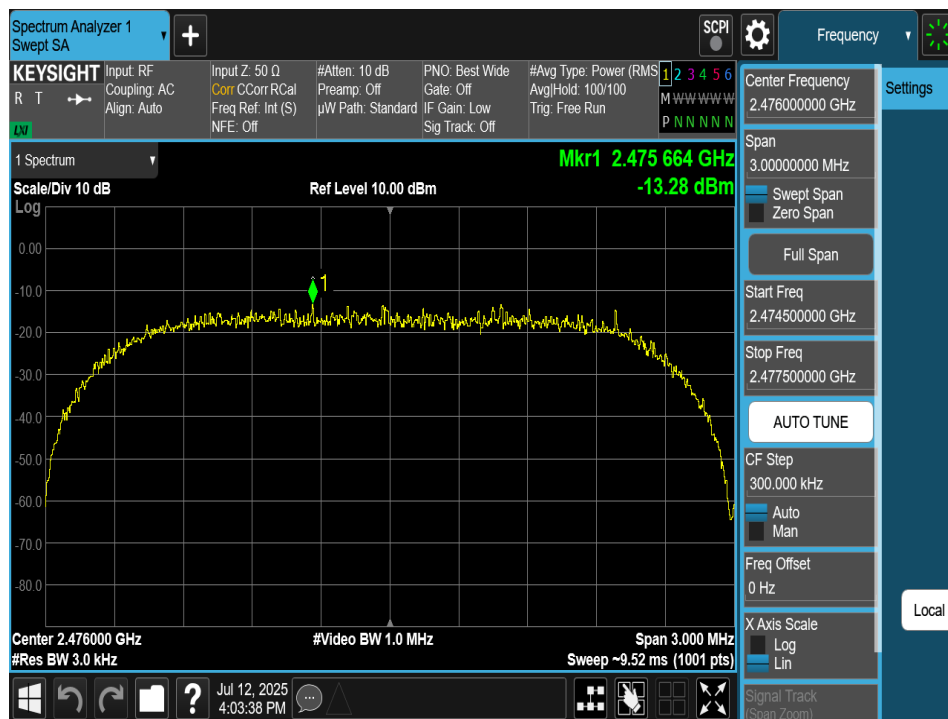
Plot 7-144. Power Spectral Density Plot TxBF Antenna 2a (Bluetooth (HDRPS2), 2Mbps, iPA – Ch. 73)
