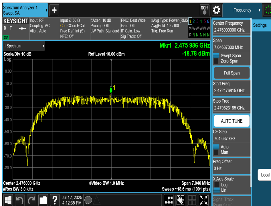
Plot 7-168. Power Spectral Density Plot TxBF Antenna 2a (Bluetooth (HDRPM16), 16Mbps, iPA – Ch. 73)
