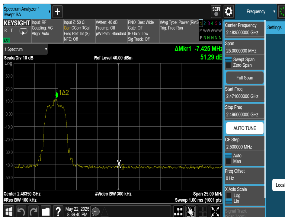
Plot 7-182. Band Edge Plot Antenna 4a (Bluetooth (HDR4), 4Mbps, ePA – Ch. 73)
