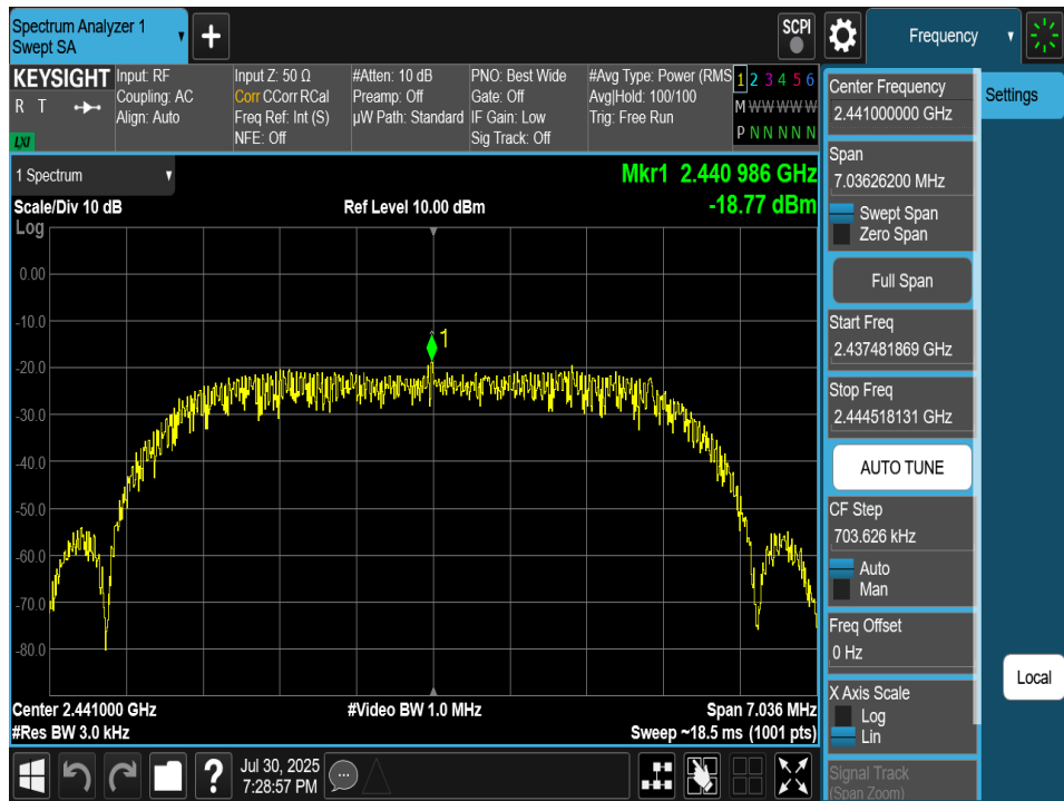
Plot 7-165. Power Spectral Density Plot TxBF Antenna 4a (Bluetooth (HDRPM16), 16Mbps, iPA – Ch. 38)
