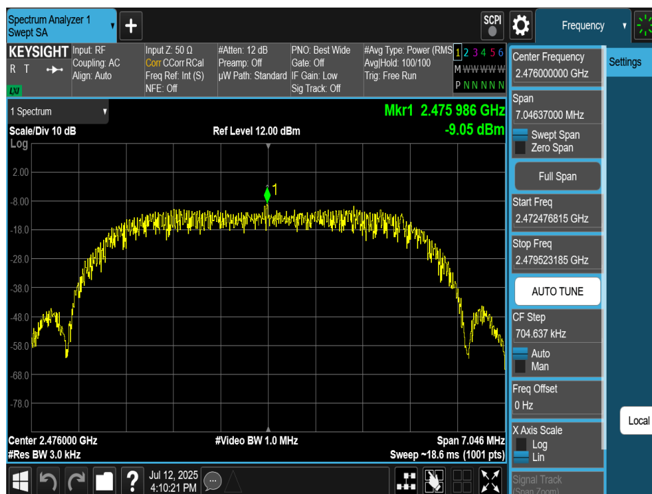
Plot 7-162. Power Spectral Density Plot Tx BF Antenna 2a (Bluetooth (HDRPM16), 16Mbps, ePA – Ch. 73)
