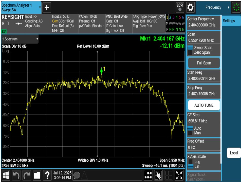
Plot 7-128. Power Spectral Density Plot TxBF Antenna 2a (Bluetooth (HDR8), 8Mbps, iPA – Ch. 1)
