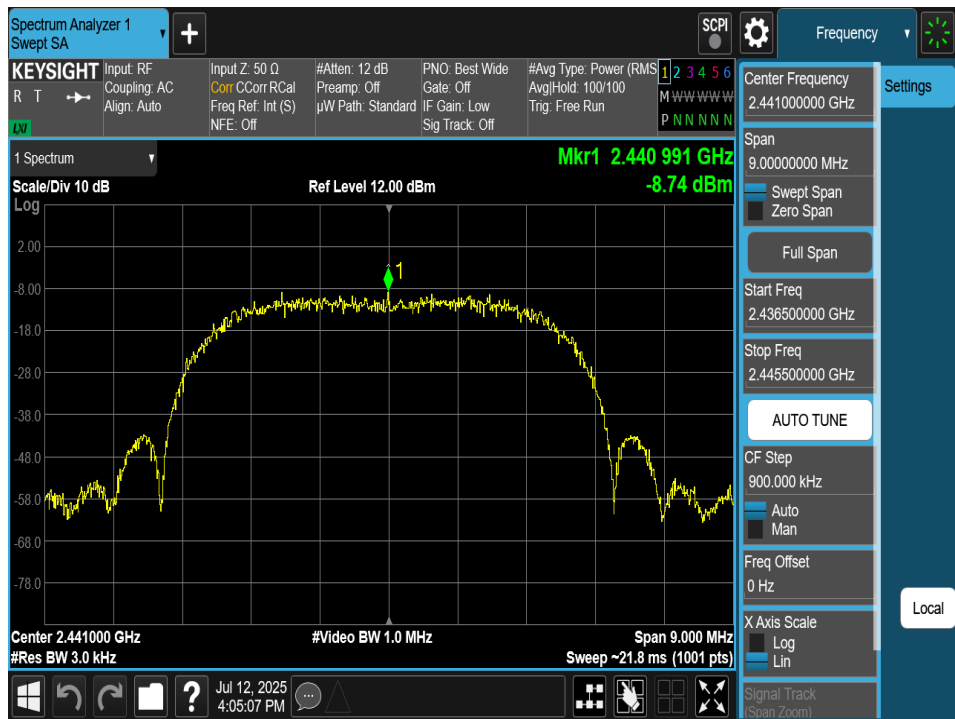
Plot 7-148. Power Spectral Density Plot TxBF Antenna 2a (Bluetooth (XHDRPM6), 6Mbps, ePA – Ch. 38)
