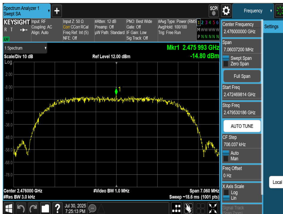
Plot 7-155. Power Spectral Density Plot TxBF Antenna 4a (Bluetooth (XHDRPM6), 6Mbps, iPA – Ch. 73)
