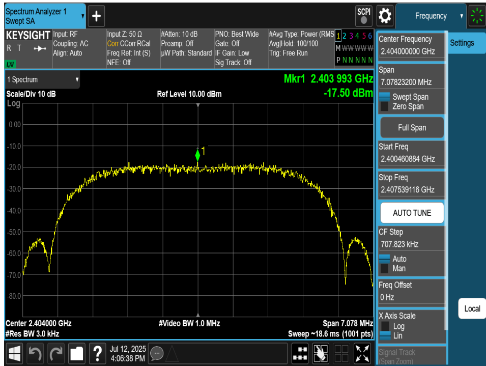
Plot 7-152. Power Spectral Density Plot TxBF Antenna 2a (Bluetooth (XHDRPM6), 6Mbps, iPA – Ch. 1)
