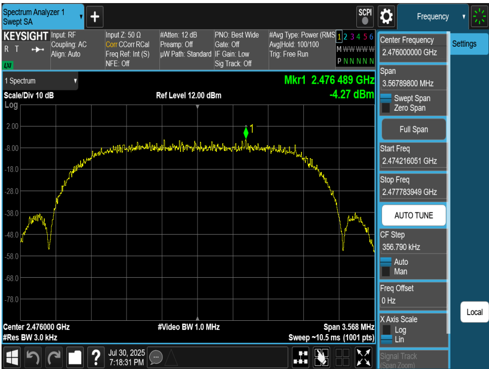
Plot 7-137. Power Spectral Density Plot TxBF Antenna 4a (Bluetooth (HDRPS2), 2Mbps, ePA – Ch. 73)
