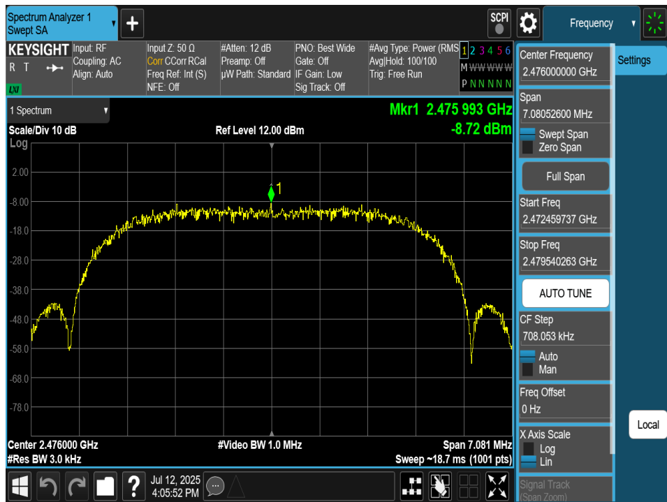
Plot 7-150. Power Spectral Density Plot TxBF Antenna 2a (Bluetooth (XHDRPM6), 6Mbps, ePA – Ch. 73)
