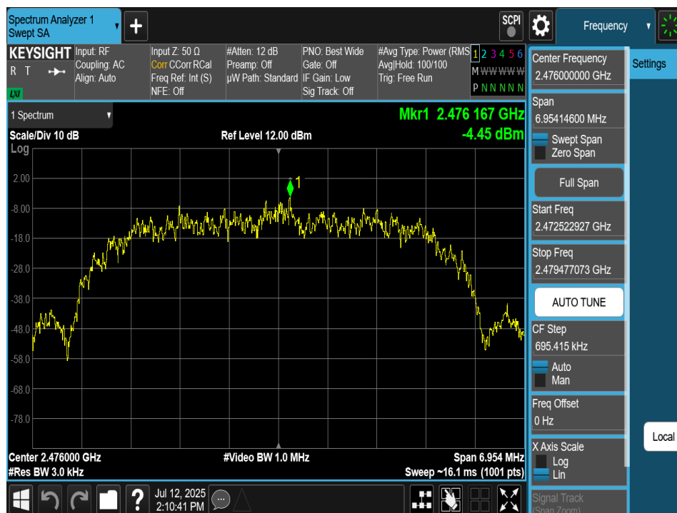
Plot 7-125. Power Spectral Density Plot TxBF Antenna 4a (Bluetooth (HDR8), 8Mbps, ePA – Ch. 73)
