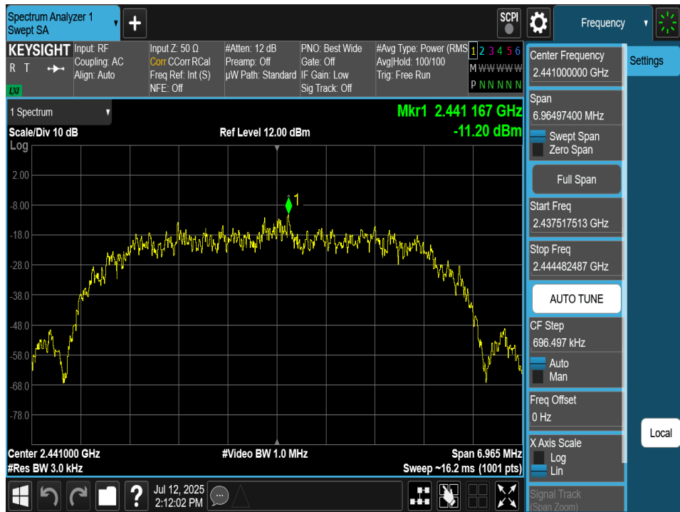
Plot 7-129. Power Spectral Density Plot TxBF Antenna 4a (Bluetooth (HDR8), 8Mbps, iPA – Ch. 38)
