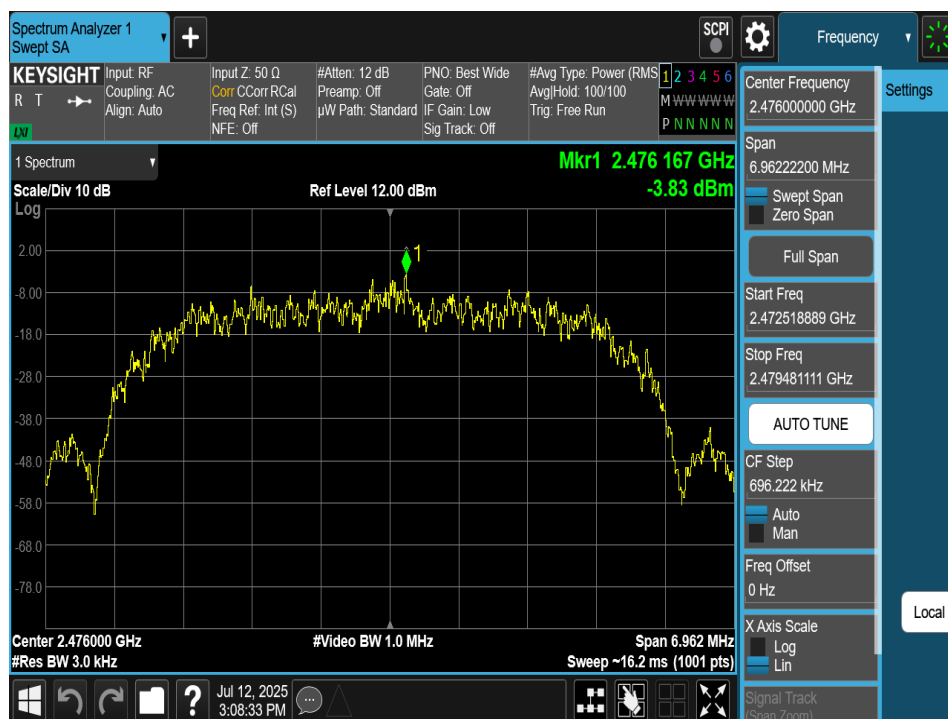
Plot 7-126. Power Spectral Density Plot TxBF Antenna 2a (Bluetooth (HDR8), 8Mbps, ePA – Ch. 73)
