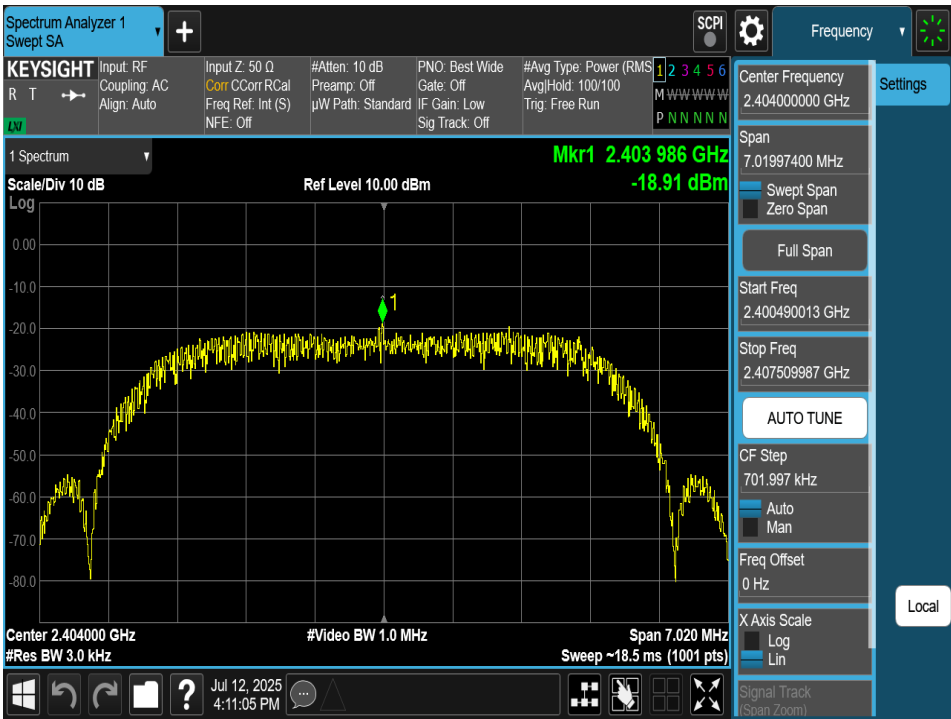
Plot 7-164. Power Spectral Density Plot TxBF Antenna 2a (Bluetooth (HDRPM16), 16Mbps, iPA – Ch. 1)
