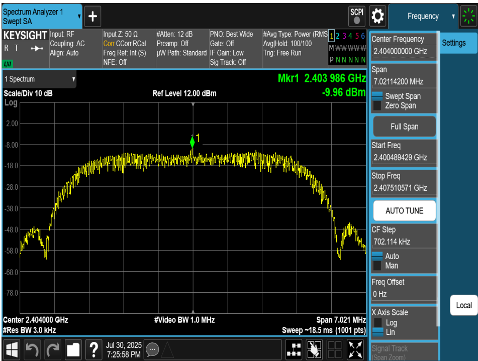
Plot 7-157. Power Spectral Density Plot TxBF Antenna 4a (Bluetooth (HDRPM16), 16Mbps, ePA – Ch. 1)
