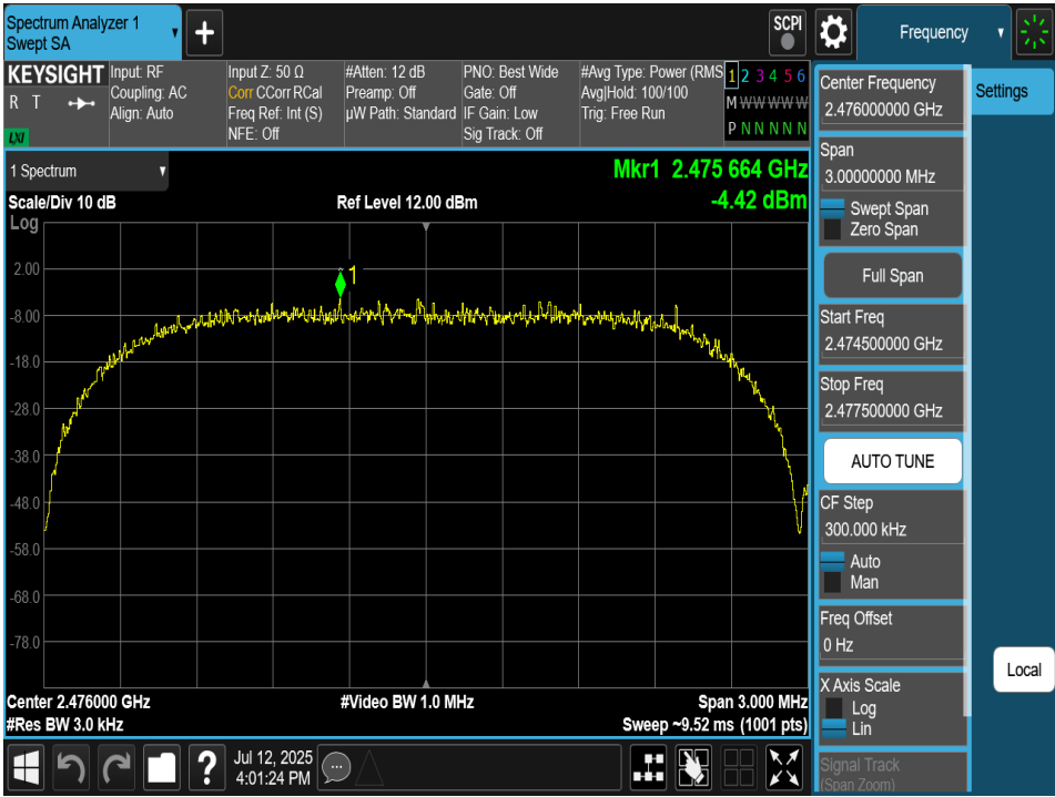
Plot 7-138. Power Spectral Density Plot TxBF Antenna 2a (Bluetooth (HDRPS2), 2Mbps, ePA – Ch. 73)
