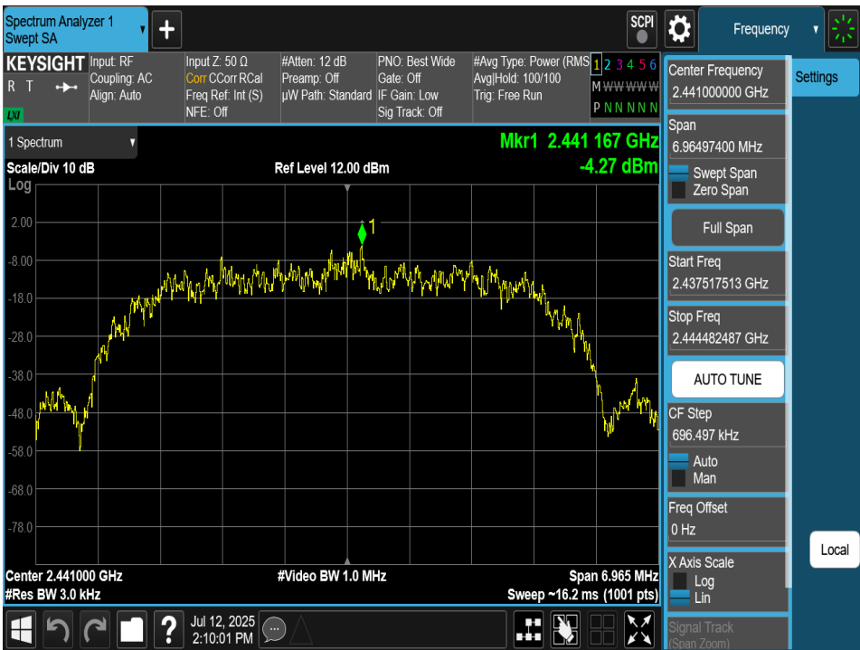
Plot 7-123. Power Spectral Density Plot TxBF Antenna 4a (Bluetooth (HDR8), 8Mbps, ePA – Ch. 38)
