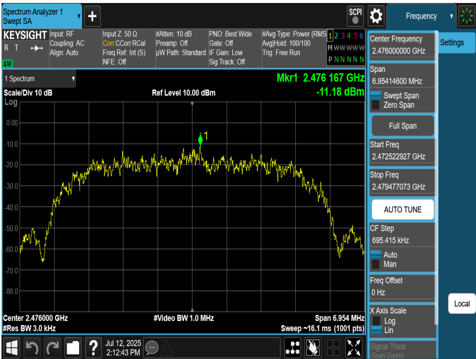
Plot 7-131. Power Spectral Density Plot TxBF Antenna 4a (Bluetooth (HDR8), 8Mbps, iPA – Ch. 73)
