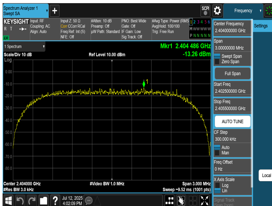
Plot 7-140. Power Spectral Density Plot TxBF Antenna 2a (Bluetooth (HDRPS2), 2Mbps, iPA – Ch. 1)
