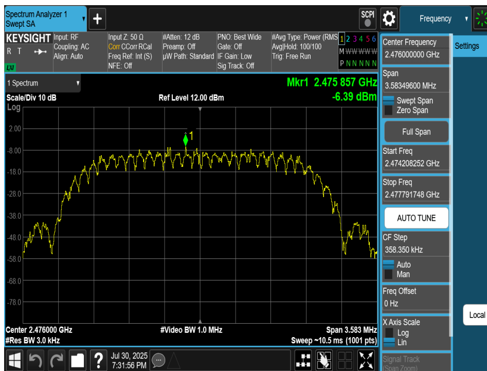
Plot 7-173. Power Spectral Density Plot TxBF Antenna 4a (Bluetooth (HDT2), 2Mbps, ePA – Ch. 73)
