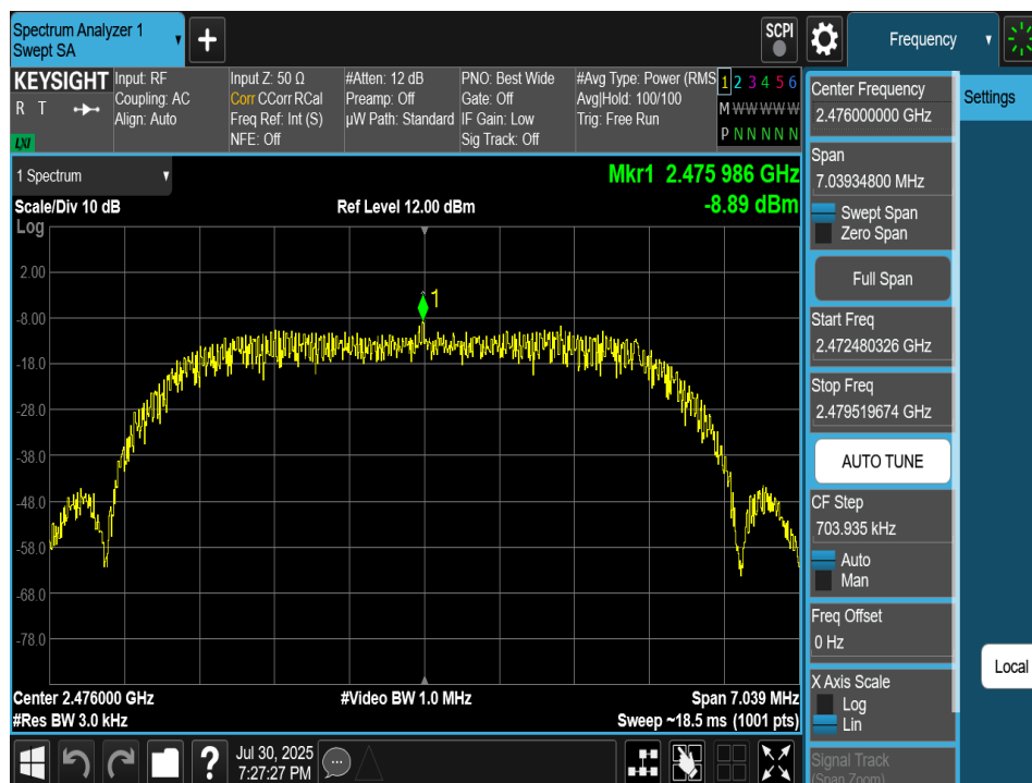
Plot 7-161. Power Spectral Density Plot Tx BF Antenna 4a (Bluetooth (HDRPM16), 16Mbps, ePA – Ch. 73)
