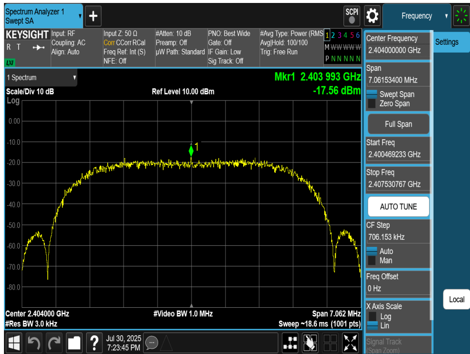
Plot 7-151. Power Spectral Density Plot TxBF Antenna 4a (Bluetooth (XHDRPM6), 6Mbps, iPA – Ch. 1)
