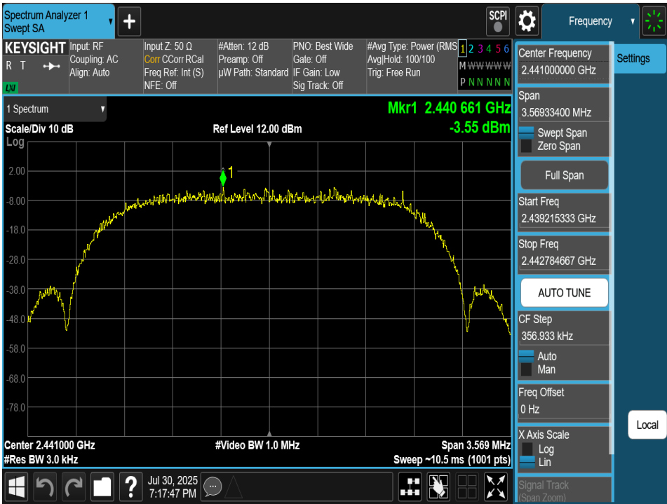
Plot 7-135. Power Spectral Density Plot TxBF Antenna 4a (Bluetooth (HDRPS2), 2Mbps, ePA – Ch. 38)
