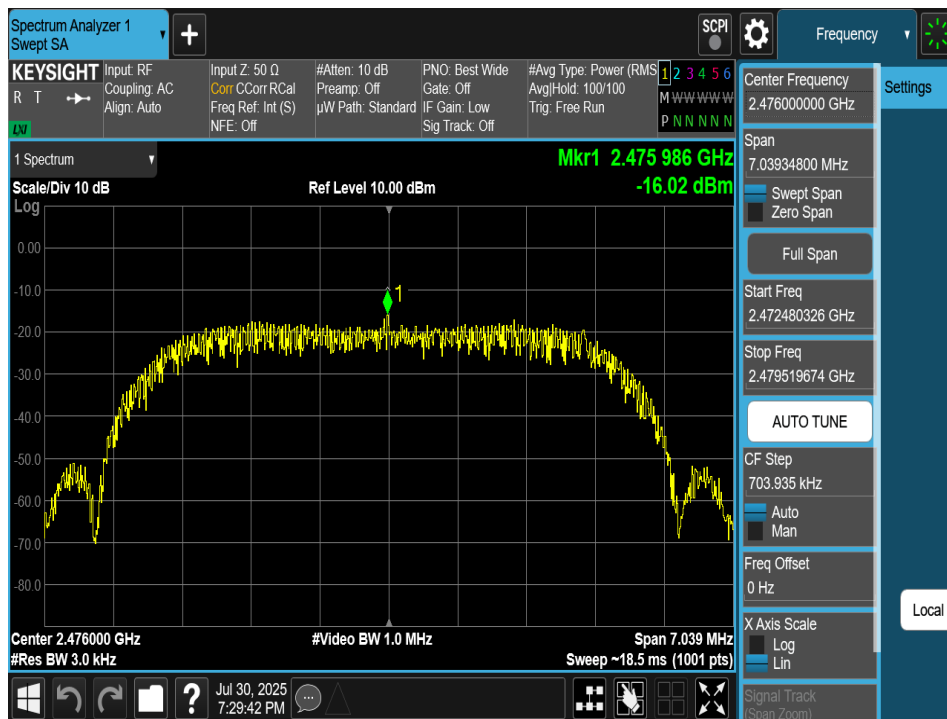
Plot 7-167. Power Spectral Density Plot TxBF Antenna 4a (Bluetooth (HDRPM16), 16Mbps, iPA – Ch. 73)
