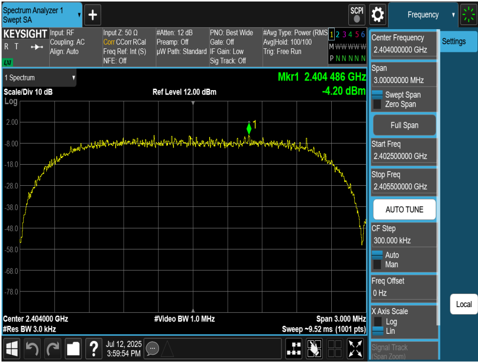
Plot 7-134. Power Spectral Density Plot TxBF Antenna 2a (Bluetooth (HDRPS2), 2Mbps, ePA – Ch. 1)
