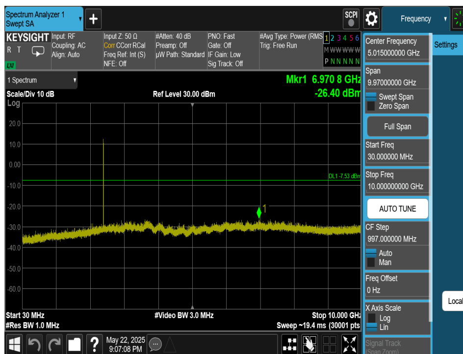
Plot 7-205. Conducted Spurious Plot Antenna 4a (Bluetooth (HDR4), 4Mbps, ePA – Ch. 1)
