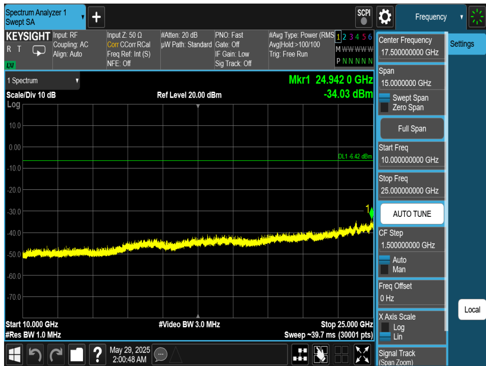
Plot 7-232. Conducted Spurious Plot Antenna 4a (Bluetooth (HDT2), 2Mbps, ePA – Ch. 37)
