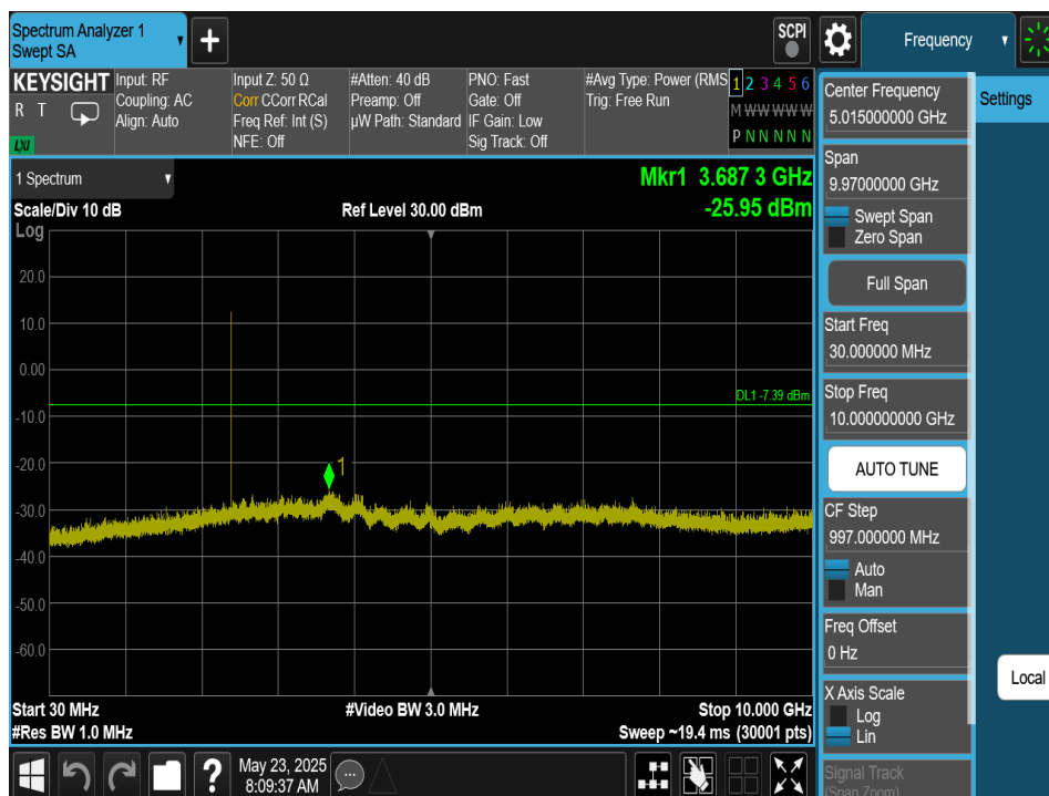
Plot 7-241. Conducted Spurious Plot Antenna 2a (Bluetooth (HDRPS2), 2Mbps, ePA – Ch. 1)
