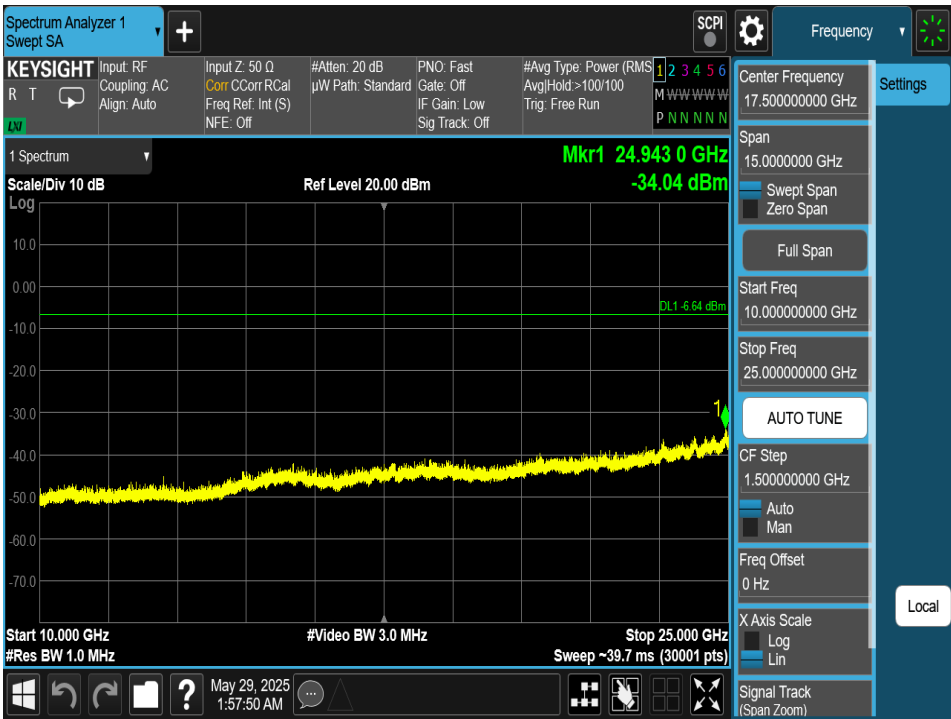
Plot 7-228. Conducted Spurious Plot Antenna 4a (Bluetooth (HDRPM16), 16Mbps, ePA – Ch. 73)
