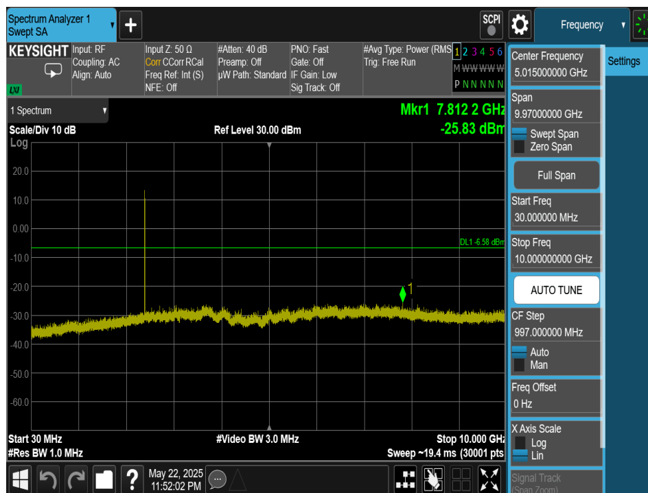
Plot 7-235. Conducted Spurious Plot Antenna 2a (Bluetooth (HDR4), 4Mbps, ePA – Ch. 1)
