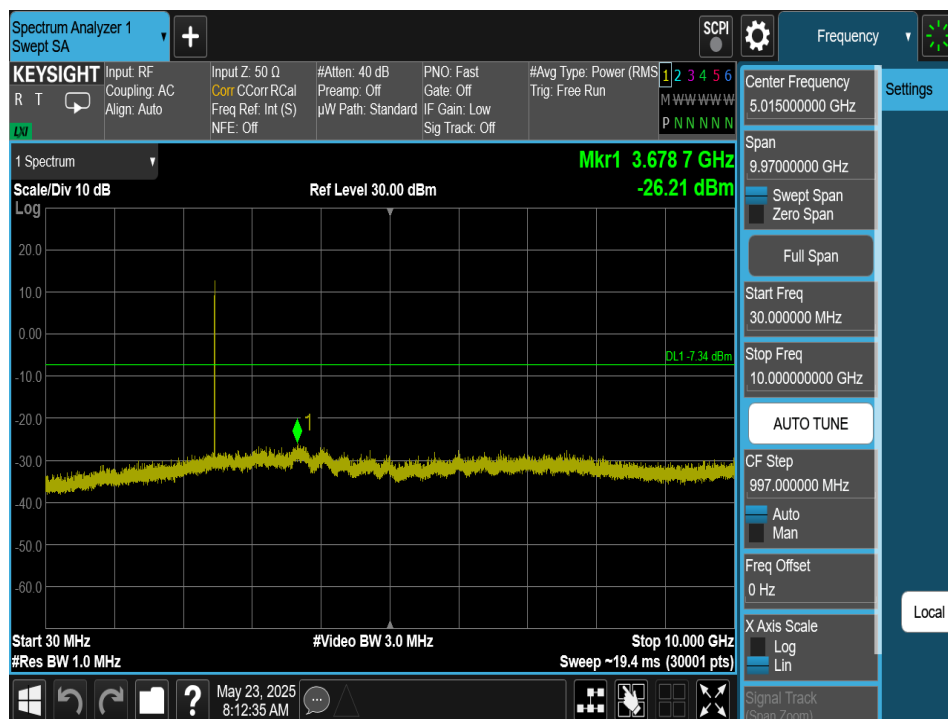
Plot 7-245. Conducted Spurious Plot Antenna 2a (Bluetooth (HDRPS2), 2Mbps, ePA – Ch. 73)
