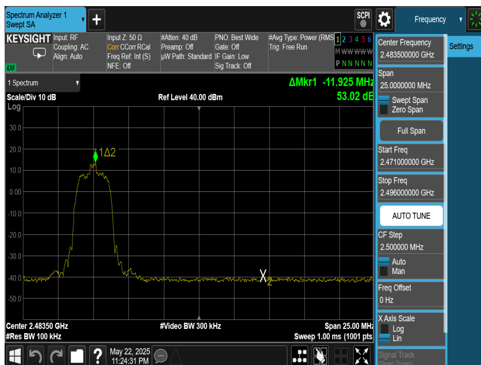
Plot 7-194. Band Edge Plot Antenna 2a (Bluetooth (HDR4), 4Mbps, ePA – Ch. 73)
