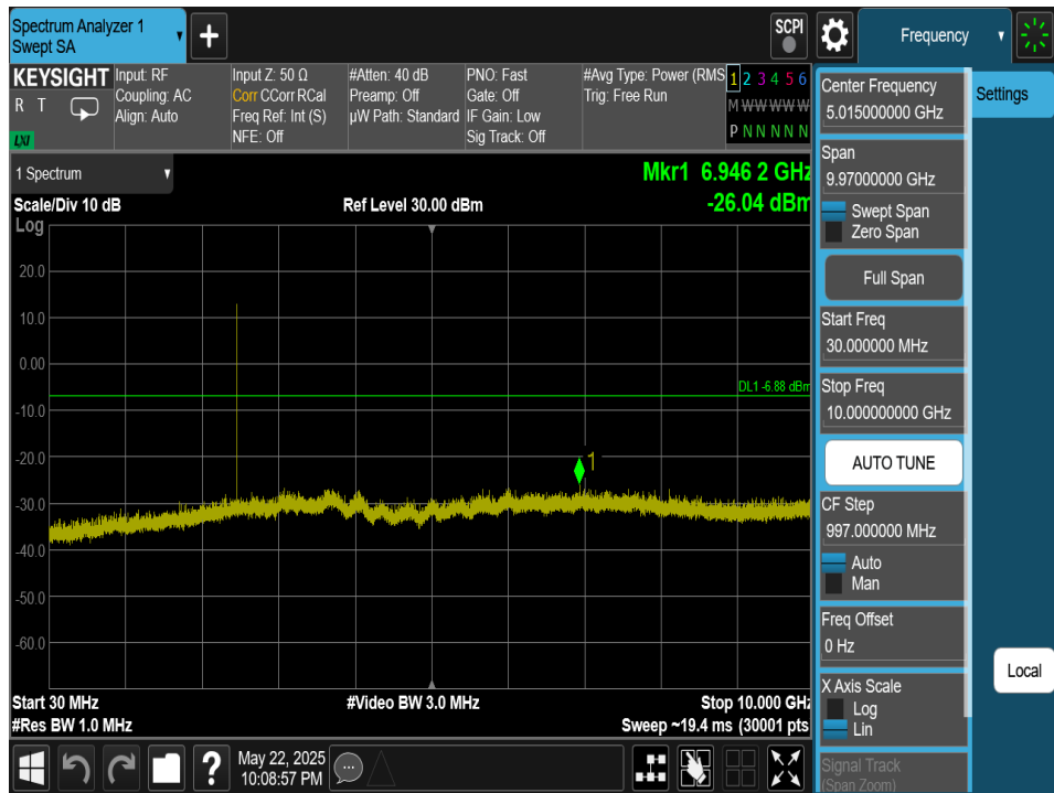
Plot 7-215. Conducted Spurious Plot Antenna 4a (Bluetooth (HDRPS2), 2Mbps, ePA – Ch. 73)
