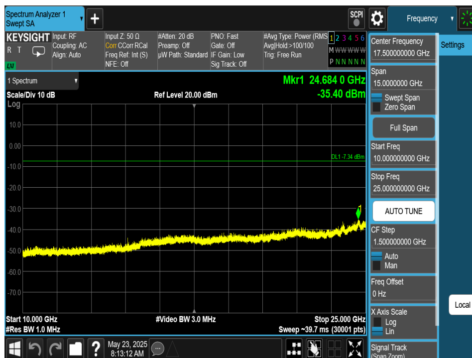
Plot 7-246. Conducted Spurious Plot Antenna 2a (Bluetooth (HDRPS2), 2Mbps, ePA – Ch. 73)
