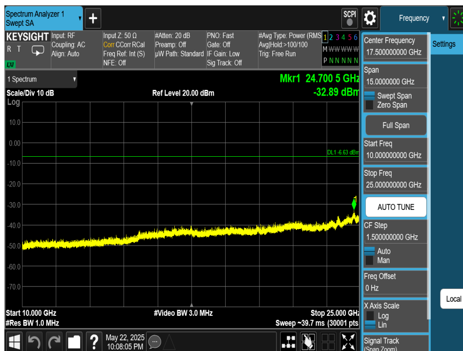
Plot 7-214. Conducted Spurious Plot Antenna 4a (Bluetooth (HDRPS2), 2Mbps, ePA – Ch. 38)
