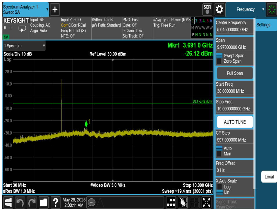
Plot 7-231. Conducted Spurious Plot Antenna 4a (Bluetooth (HDT2), 2Mbps, ePA – Ch. 37)
