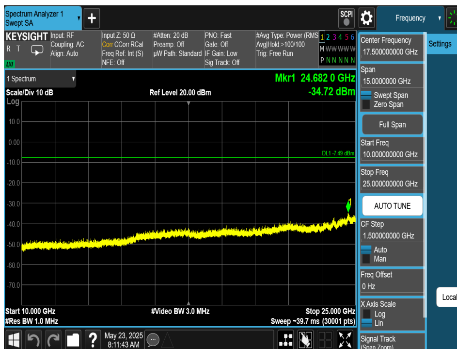
Plot 7-244. Conducted Spurious Plot Antenna 2a (Bluetooth (HDRPS2), 2Mbps, ePA – Ch. 38)
