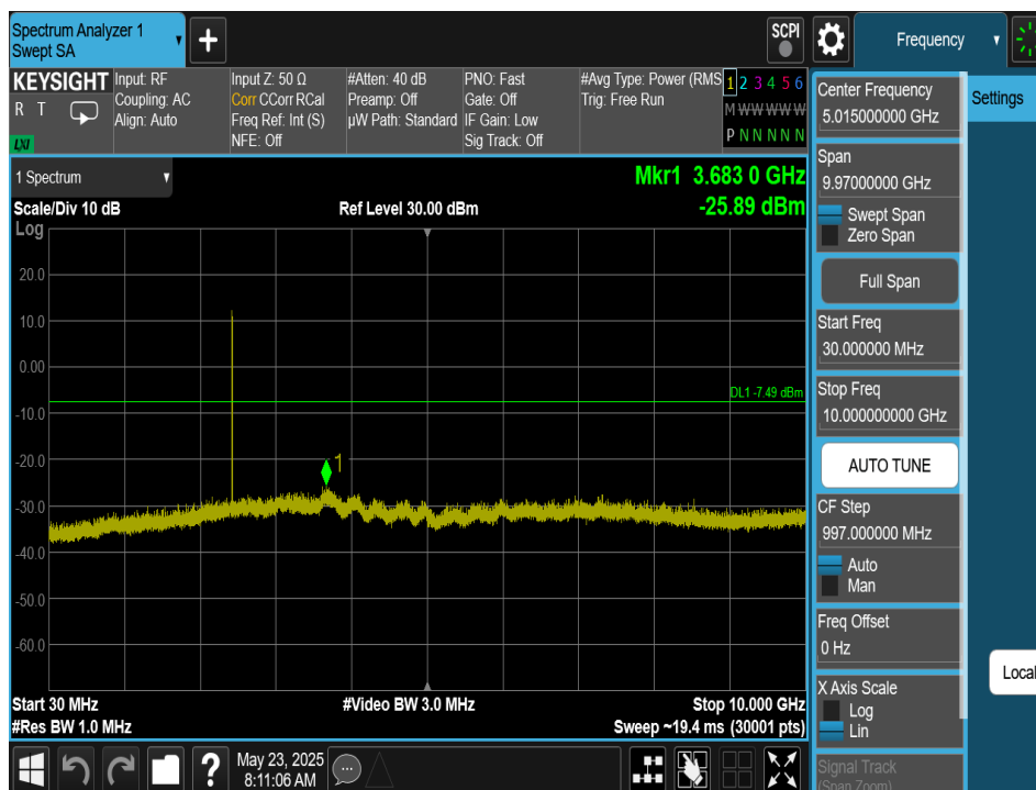
Plot 7-243. Conducted Spurious Plot Antenna 2a (Bluetooth (HDRPS2), 2Mbps, ePA – Ch. 38)
