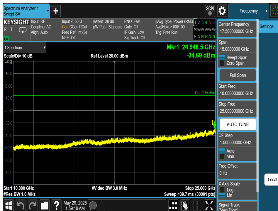
Plot 7-230. Conducted Spurious Plot Antenna 4a (Bluetooth (HDT2), 2Mbps, ePA – Ch. 1)
