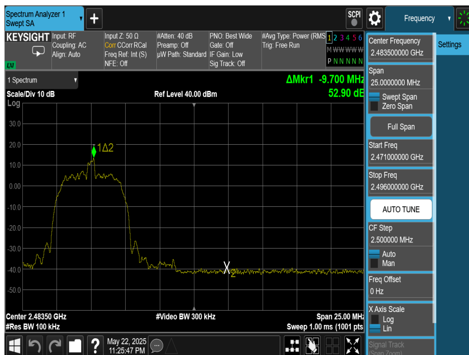
Plot 7-196. Band Edge Plot Antenna 2a (Bluetooth (HDR8), 8Mbps, ePA – Ch. 73)
