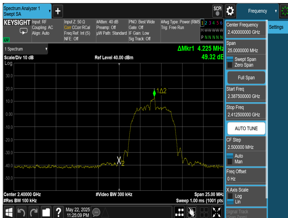
Plot 7-195. Band Edge Plot Antenna 2a (Bluetooth (HDR8), 8Mbps, ePA – Ch. 1)
