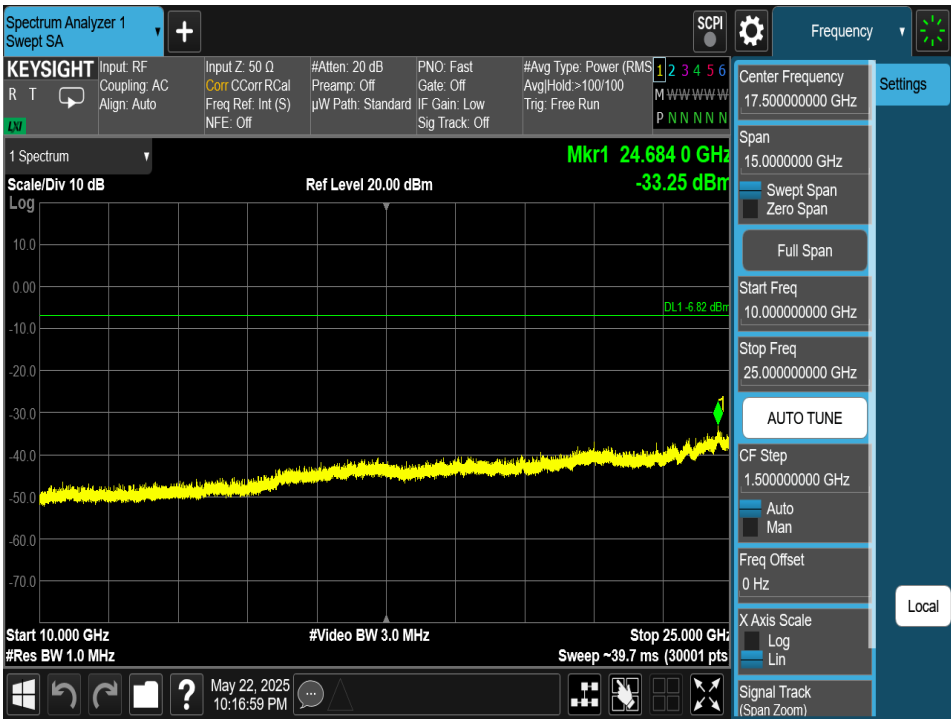
Plot 7-226. Conducted Spurious Plot Antenna 4a (Bluetooth (HDRPM16), 16Mbps, ePA – Ch. 38)
