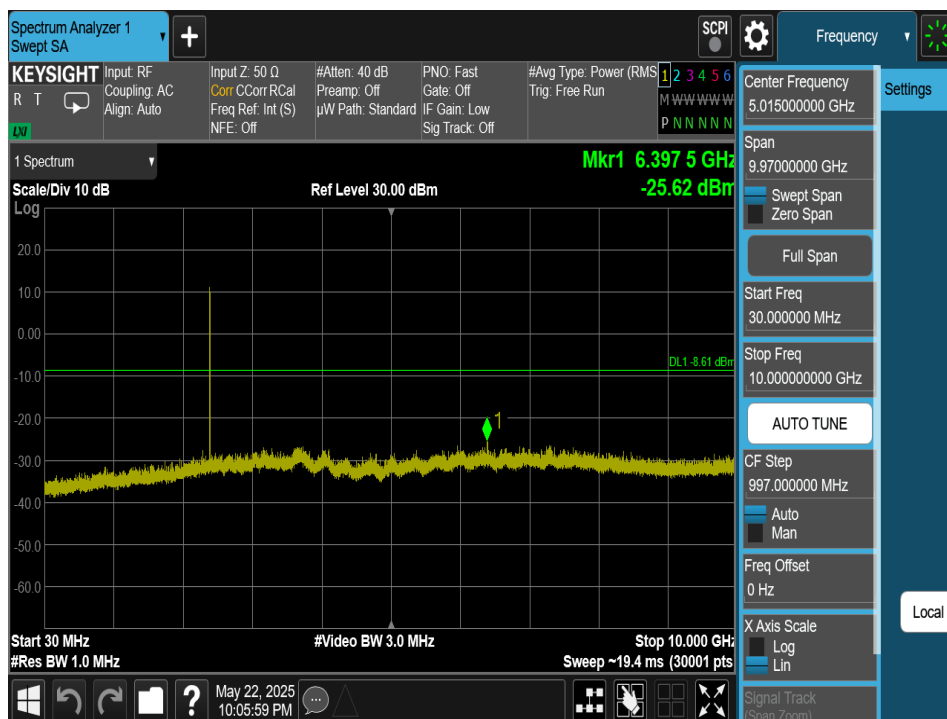
Plot 7-211. Conducted Spurious Plot Antenna 4a (Bluetooth (HDRPS2), 2Mbps, ePA – Ch. 1)
