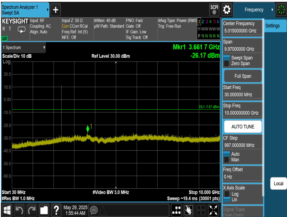
Plot 7-223. Conducted Spurious Plot Antenna 4a (Bluetooth (HDRPM16), 16Mbps, ePA – Ch. 1)
