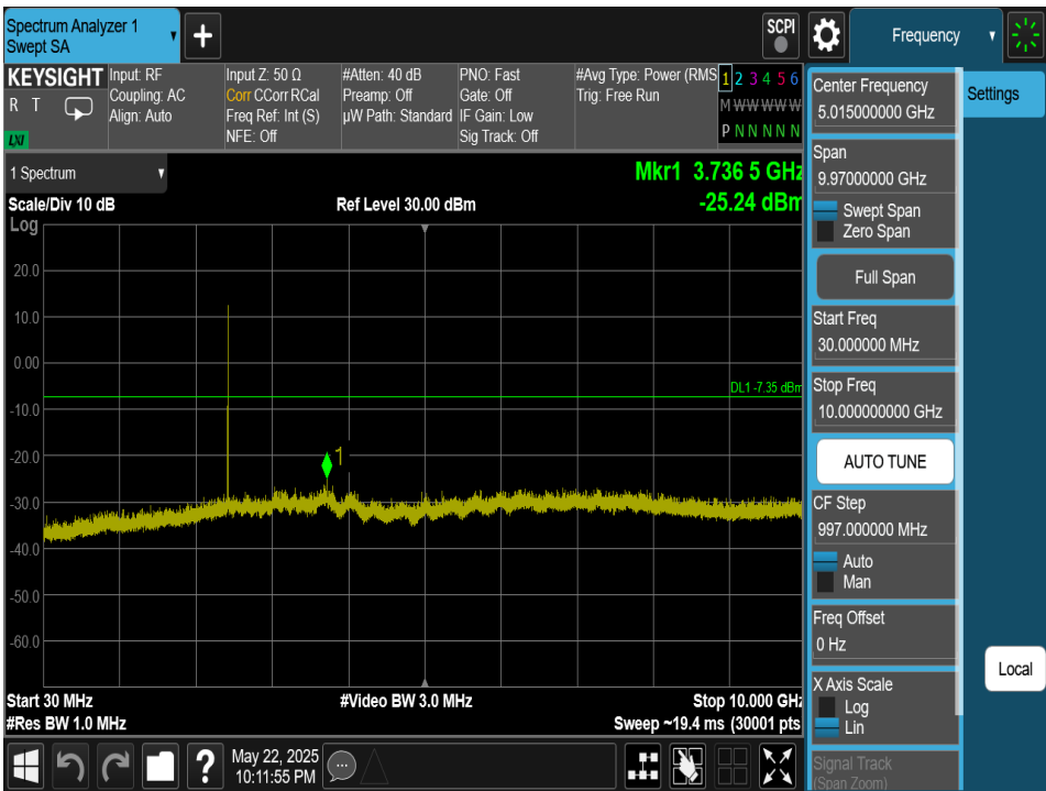
Plot 7-219. Conducted Spurious Plot Antenna 4a (Bluetooth (XHDRPM6), 6Mbps, ePA – Ch. 38)
