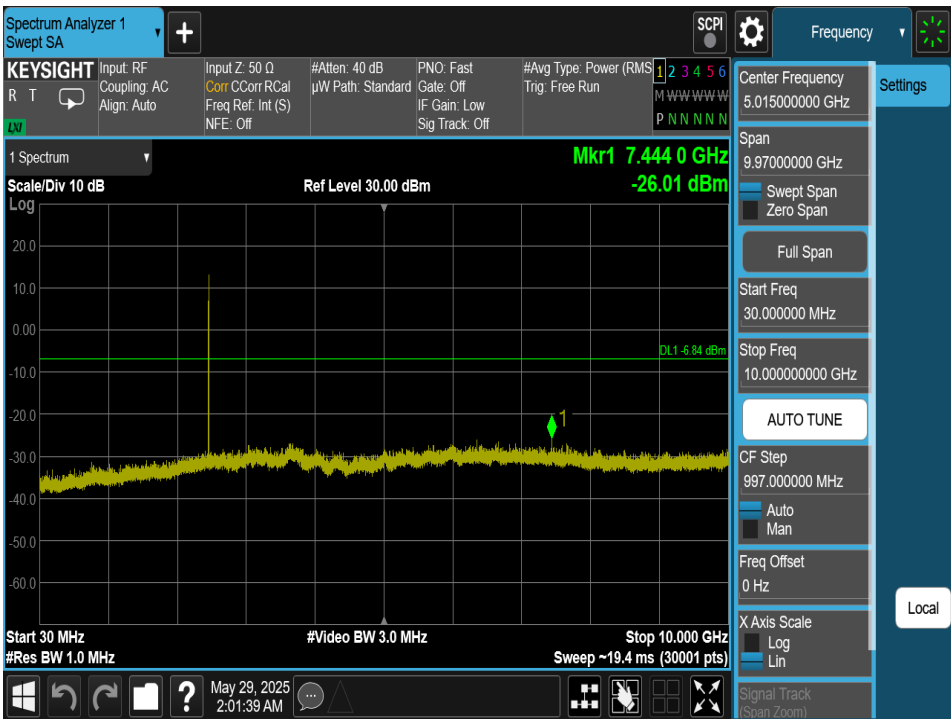
Plot 7-233. Conducted Spurious Plot Antenna 4a (Bluetooth (HDT2), 2Mbps, ePA – Ch. 73)
