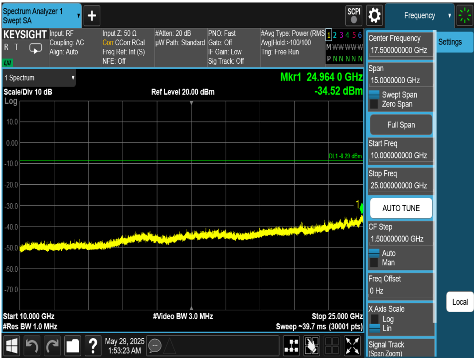
Plot 7-218. Conducted Spurious Plot Antenna 4a (Bluetooth (XHDRPM6), 6Mbps, ePA – Ch. 1)
