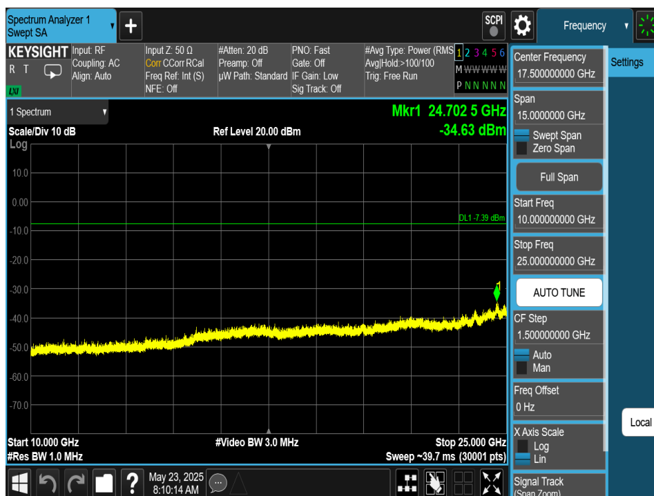
Plot 7-242. Conducted Spurious Plot Antenna 2a (Bluetooth (HDRPS2), 2Mbps, ePA – Ch. 1)
