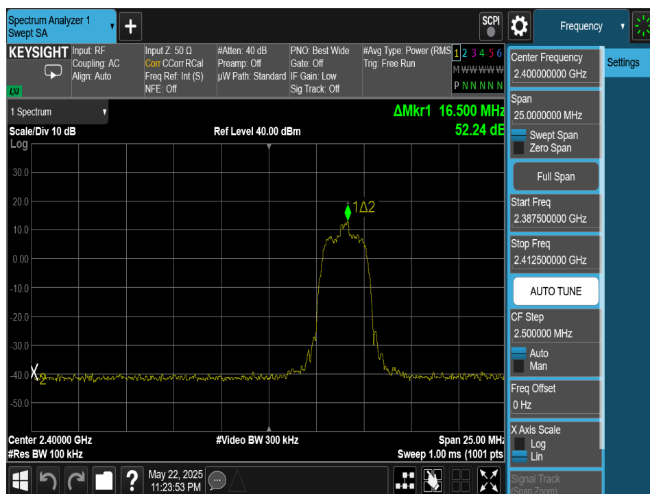
Plot 7-193. Band Edge Plot Antenna 2a (Bluetooth (HDR4), 4Mbps, ePA – Ch. 1)
