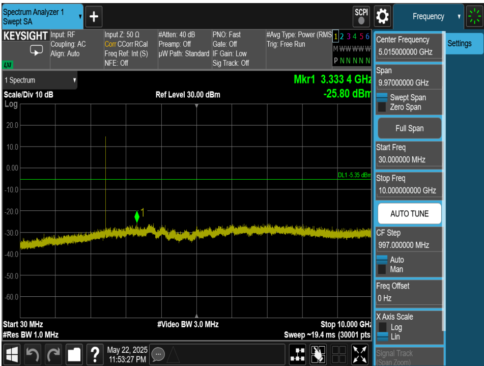
Plot 7-237. Conducted Spurious Plot Antenna 2a (Bluetooth (HDR4), 4Mbps, ePA – Ch. 38)
