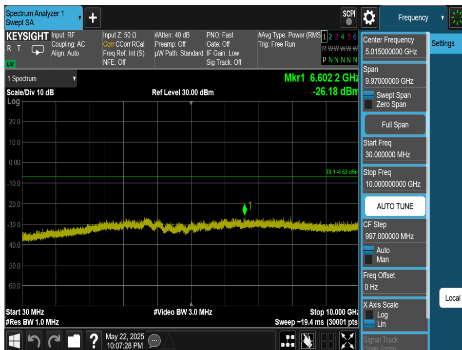
Plot 7-213. Conducted Spurious Plot Antenna 4a (Bluetooth (HDRPS2), 2Mbps, ePA – Ch. 38)
