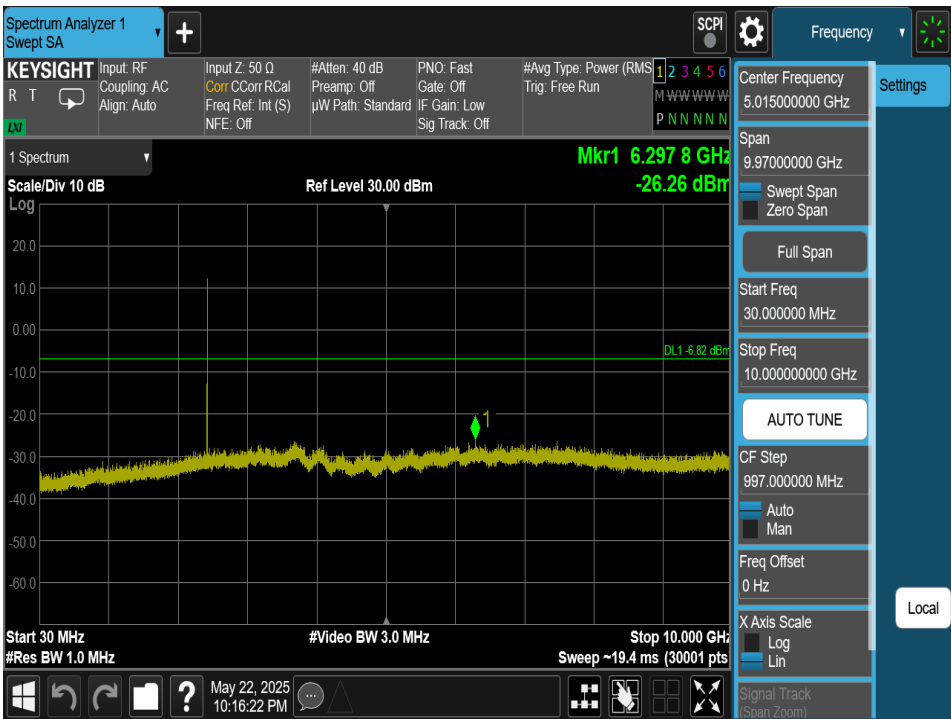
Plot 7-225. Conducted Spurious Plot Antenna 4a (Bluetooth (HDRPM16), 16Mbps, ePA – Ch. 38)
