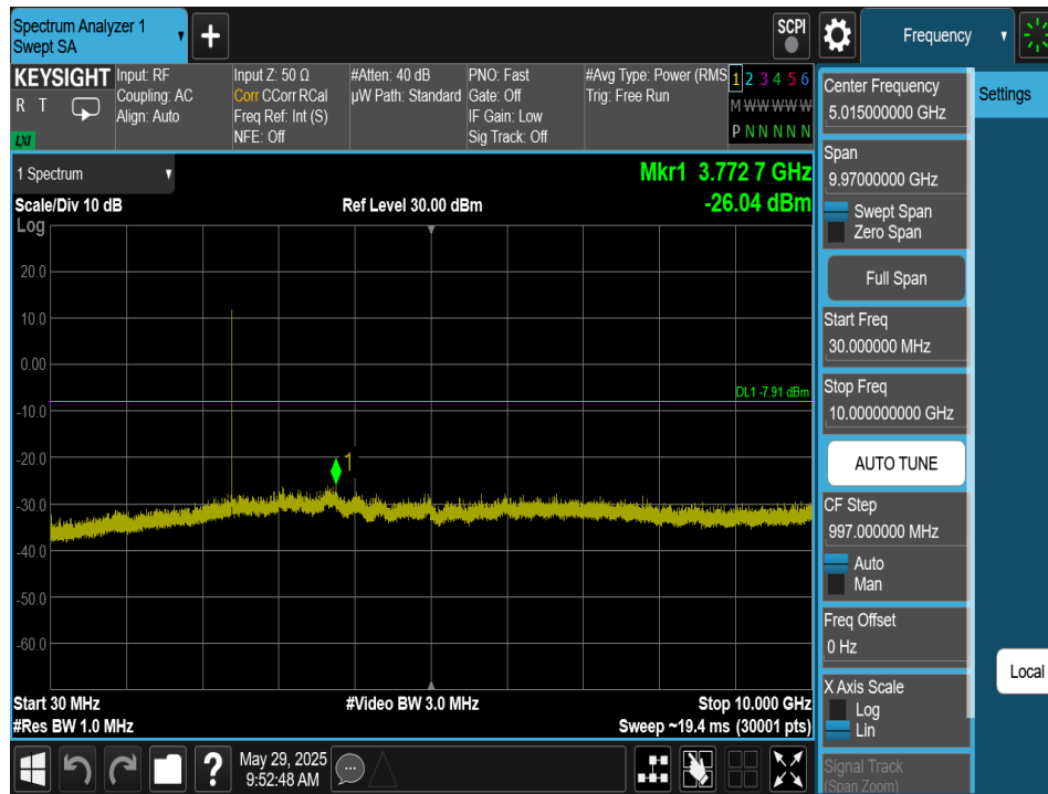
Plot 7-247. Conducted Spurious Plot Antenna 2a (Bluetooth (XHDRPM6), 6Mbps, ePA – Ch. 1)
