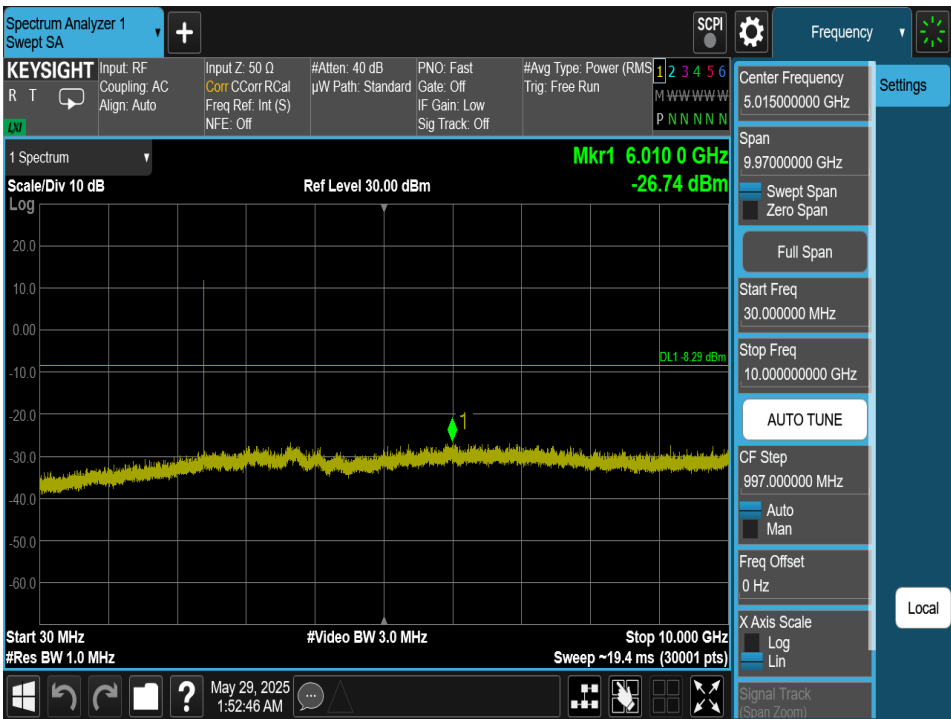
Plot 7-217. Conducted Spurious Plot Antenna 4a (Bluetooth (XHDRPM6), 6Mbps, ePA – Ch. 1)
