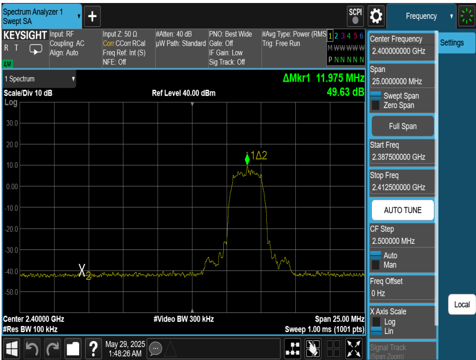
Plot 7-191. Band Edge Plot Antenna 4a (Bluetooth (HDT2), 2Mbps, ePA – Ch. 1)
