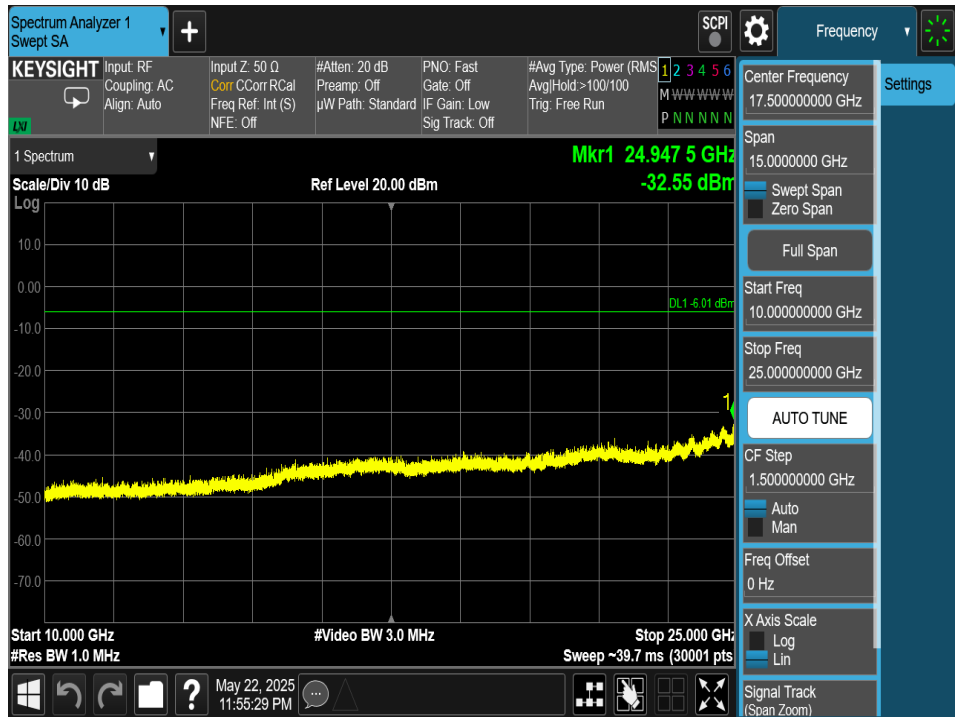
Plot 7-240. Conducted Spurious Plot Antenna 2a (Bluetooth (HDR4), 4Mbps, ePA – Ch. 73)
