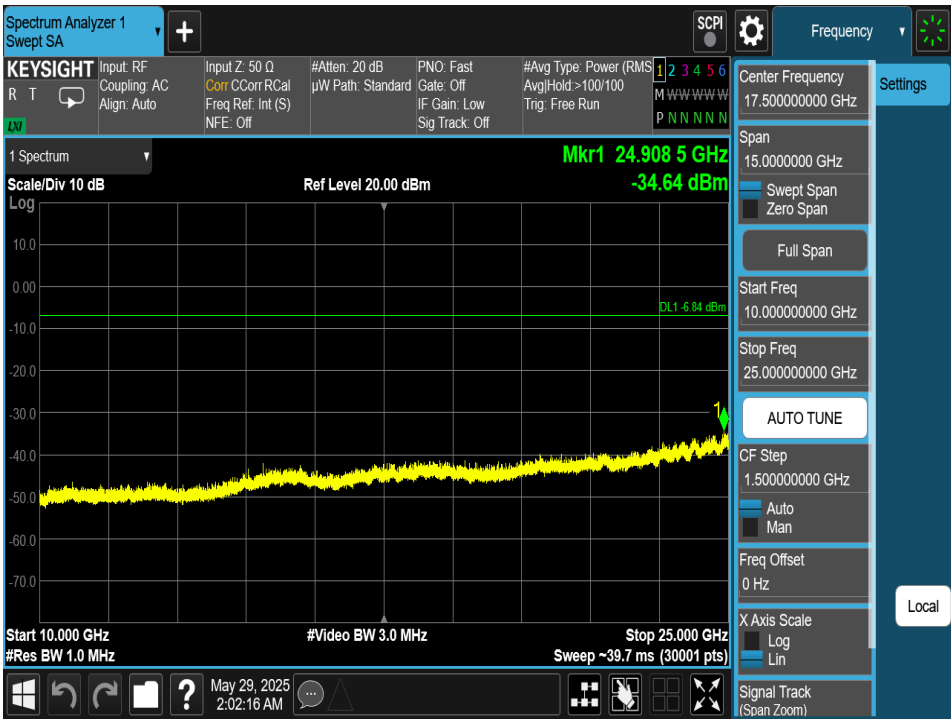
Plot 7-234. Conducted Spurious Plot Antenna 4a (Bluetooth (HDT2), 2Mbps, ePA – Ch. 73)
