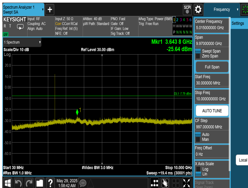
Plot 7-229. Conducted Spurious Plot Antenna 4a (Bluetooth (HDT2), 2Mbps, ePA – Ch. 1)
