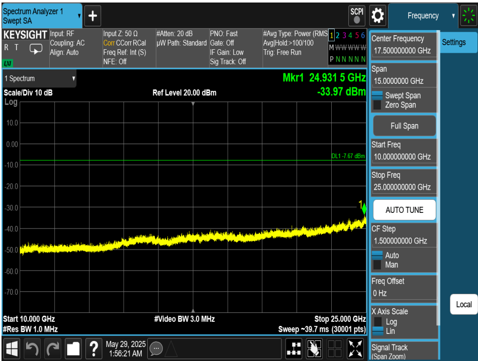
Plot 7-224. Conducted Spurious Plot Antenna 4a (Bluetooth (HDRPM16), 16Mbps, ePA – Ch. 1)
