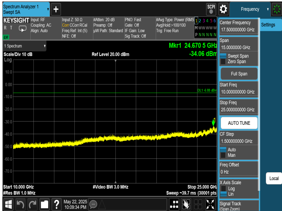
Plot 7-216. Conducted Spurious Plot Antenna 4a (Bluetooth (HDRPS2), 2Mbps, ePA – Ch. 73)
