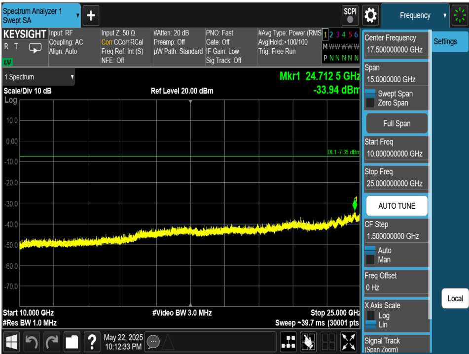
Plot 7-220. Conducted Spurious Plot Antenna 4a (Bluetooth (XHDRPM6), 6Mbps, ePA – Ch. 38)
