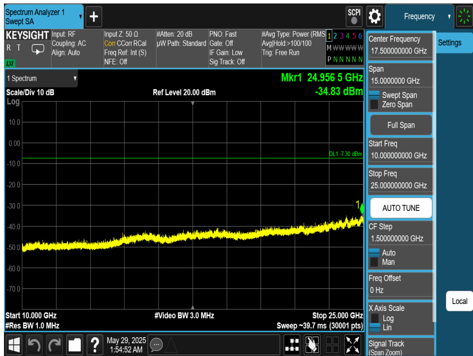
Plot 7-222. Conducted Spurious Plot Antenna 4a (Bluetooth (XHDRPM6), 6Mbps, ePA – Ch. 73)
