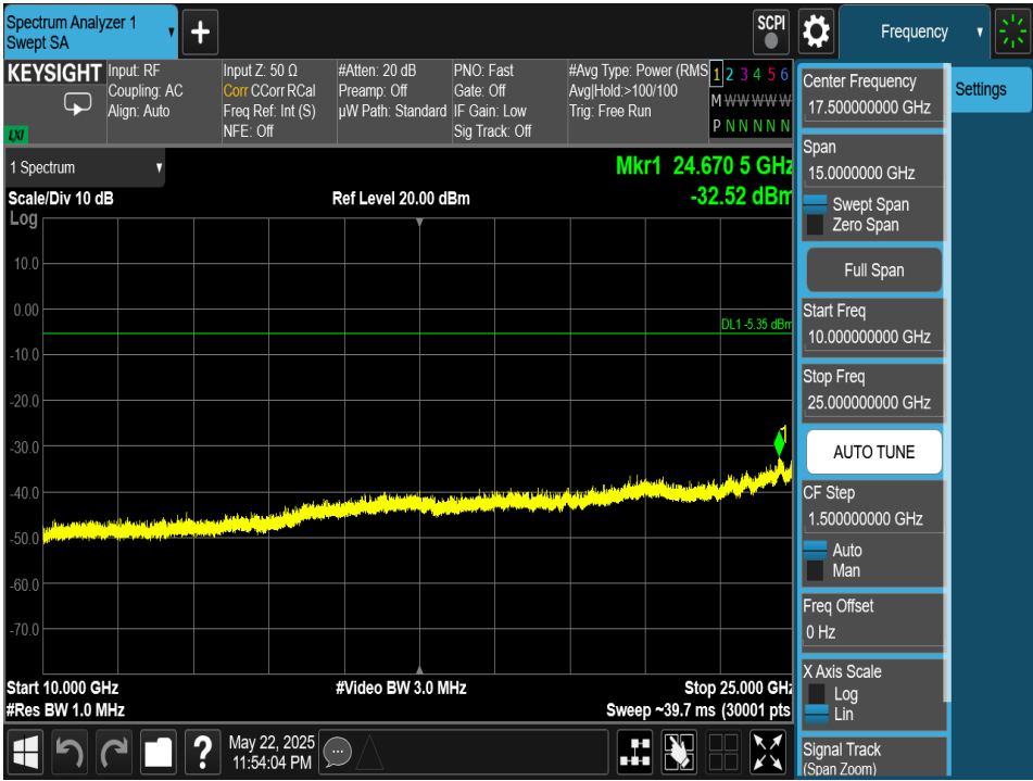
Plot 7-238. Conducted Spurious Plot Antenna 2a (Bluetooth (HDR4), 4Mbps, ePA – Ch. 38)
