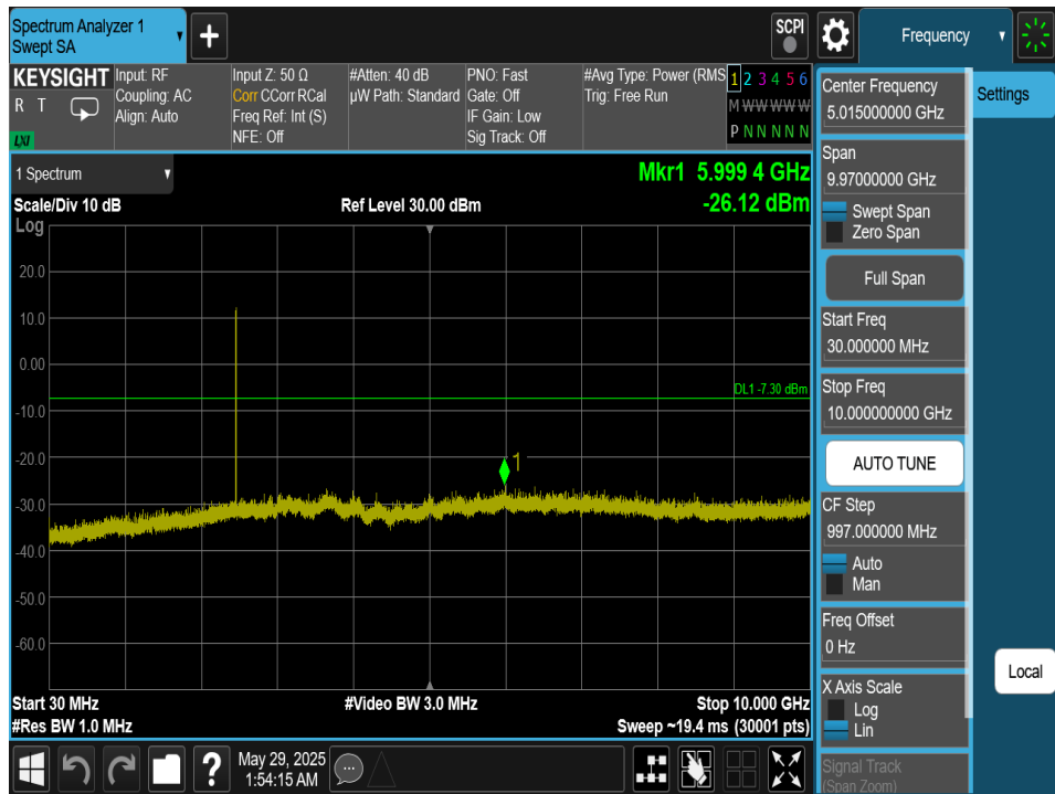
Plot 7-221. Conducted Spurious Plot Antenna 4a (Bluetooth (XHDRPM6), 6Mbps, ePA – Ch. 73)
