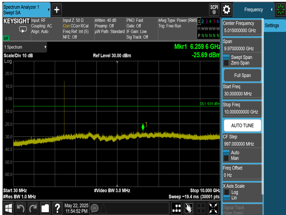
Plot 7-239. Conducted Spurious Plot Antenna 2a (Bluetooth (HDR4), 4Mbps, ePA – Ch. 73)
