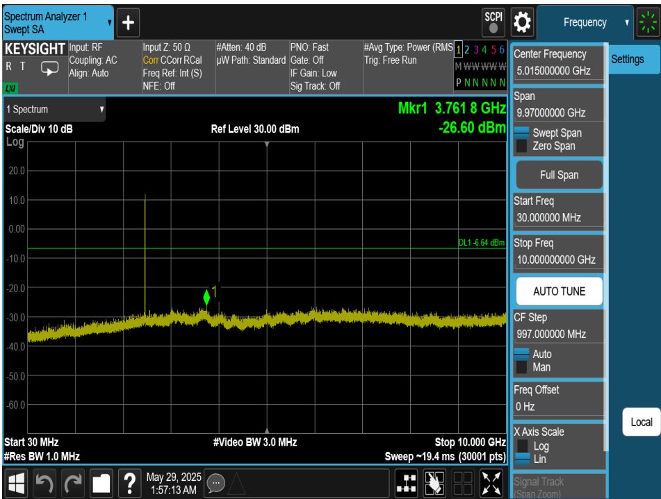
Plot 7-227. Conducted Spurious Plot Antenna 4a (Bluetooth (HDRPM16), 16Mbps, ePA – Ch. 73)
