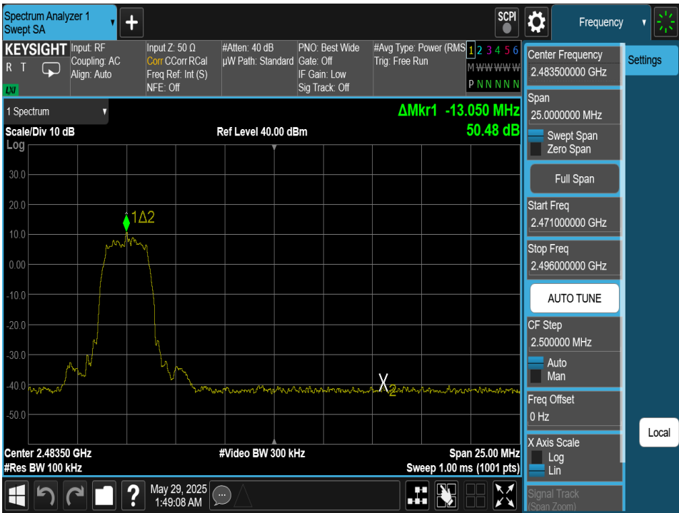
Plot 7-192. Band Edge Plot Antenna 4a (Bluetooth (HDT2), 2Mbps, ePA – Ch. 73)
