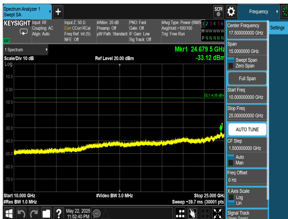
Plot 7-236. Conducted Spurious Plot Antenna 2a (Bluetooth (HDR4), 4Mbps, ePA – Ch. 1)
