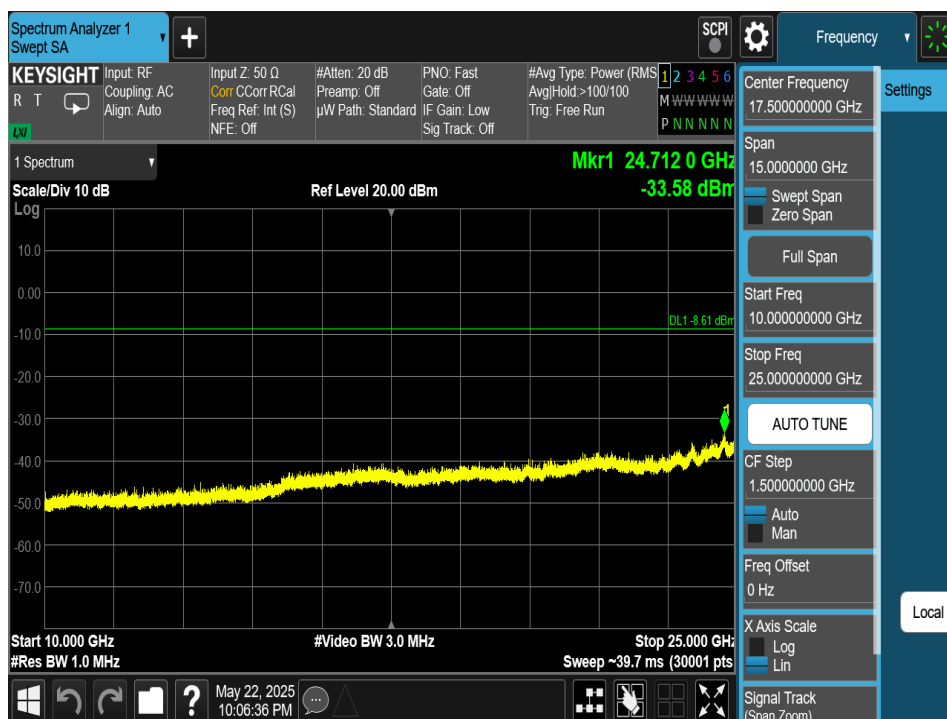
Plot 7-212. Conducted Spurious Plot Antenna 4a (Bluetooth (HDRPS2), 2Mbps, ePA – Ch. 1)
