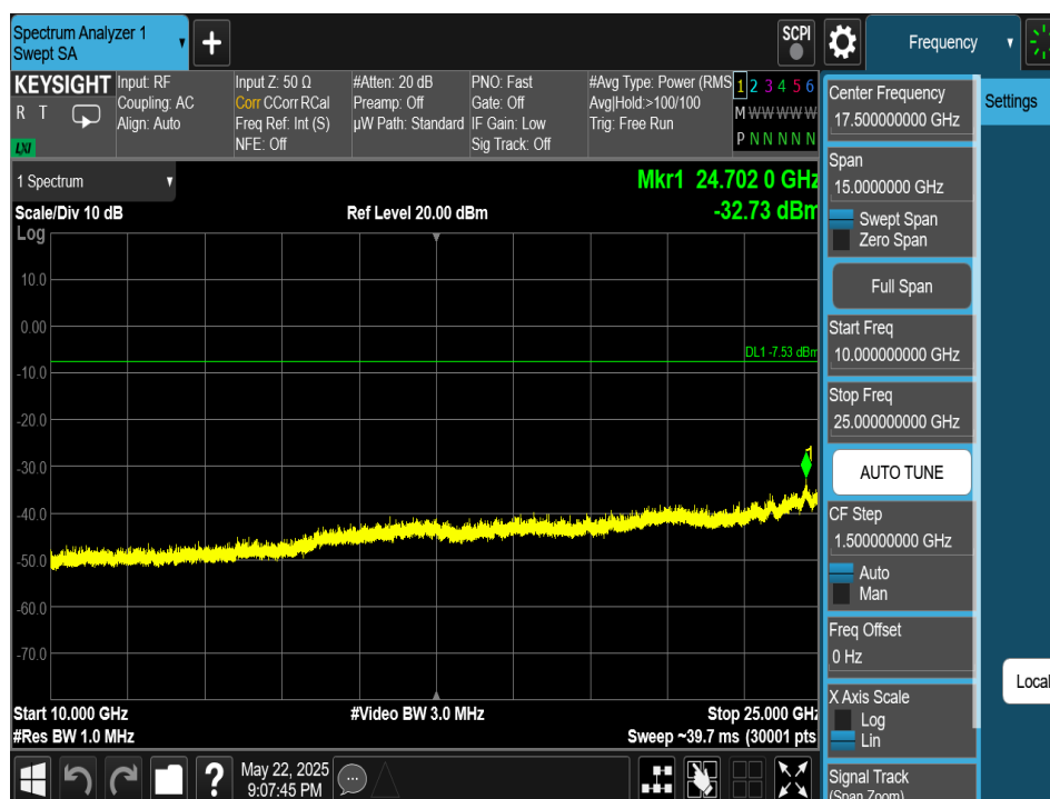
Plot 7-206. Conducted Spurious Plot Antenna 4a (Bluetooth (HDR4), 4Mbps, ePA – Ch. 1)
